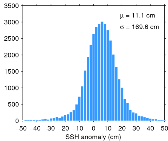
Figure 7. Histogram of flag-valid SSH anomaly over oceans and lakes for 05/10/2018. The mean ( \mu ) and standard deviation ( \sigma ) are also shown. Note that values outside [-50 50] cm are excluded from the histogram for the sake of readability but not from the computation of \mu and \sigma .
