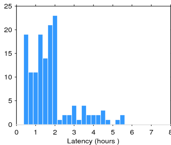
Figure 2. Histogram of the data latency for 05/10/2018. The y-axis denotes the number of files that are made available with a delay of x-hours with respect to the mean time of the records stored in the file.
