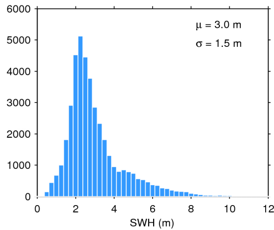
Figure 17. Histogram of flag-valid SWH over oceans and lakes for 05/10/2018. The mean ( \mu ) and standard deviation ( \sigma ) are also shown. Note that values larger than 12 m are excluded from the histogram for the sake of readability but not from the computation of \mu and \sigma .
