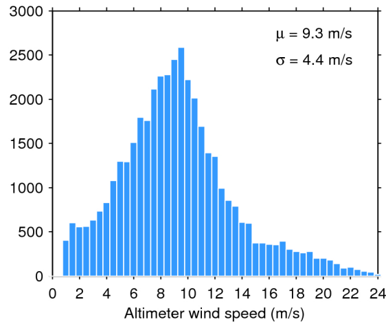
Figure 33. Histogram of flag-valid wind over oceans and lakes for 05/10/2018. The mean ( \mu ) and standard deviation ( \sigma ) are also shown. Note that values larger than 24 m/s are excluded from the histogram for the sake of readability but not from the computation of \mu and \sigma .
