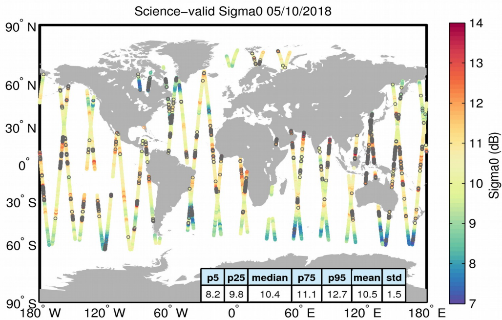
Figure 27. Geographical distribution of science-valid sigma0 data over oceans and lakes for 05/10/2018. The statistical values shown in the table refer to the sigma0 in dB and are calculated over all measurements shown in the figure. Gray circles denote records that have been rejected based on the editing criteria described in Table 4.
