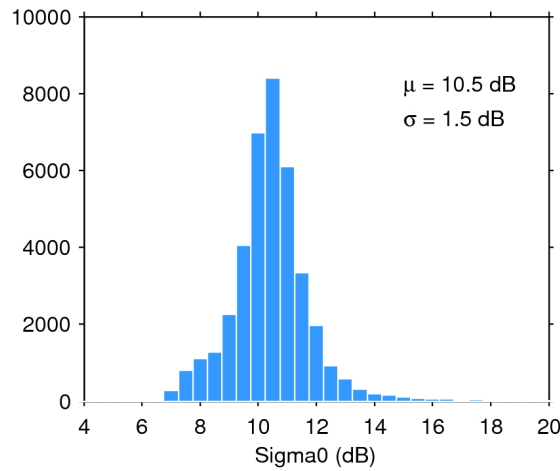
Figure 28. Histogram of science-valid sigma0 over oceans and lakes for 05/10/2018. The mean ( \mu ) and standard deviation ( \sigma ) are also shown. Note that values outside [4 20] dB are excluded from the histogram for the sake of readability but not from the computation of \mu and \sigma .
