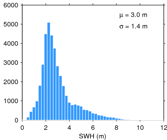
Figure 20. Histogram of science-valid SWH over oceans and lakes for 05/10/2018. The mean ( \mu ) and standard deviation ( \sigma ) are also shown. Note that values larger than 12 m are excluded from the histogram for the sake of readability but not from the computation of \mu and \sigma .
