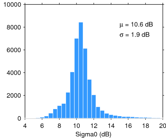
Figure 25. Histogram of flag-valid sigma0 over oceans and lakes for 05/10/2018. The mean ( \mu ) and standard deviation ( \sigma ) are also shown. Note that values outside [4 20] dB are excluded from the histogram for the sake of readability but not from the computation of \mu and \sigma .
