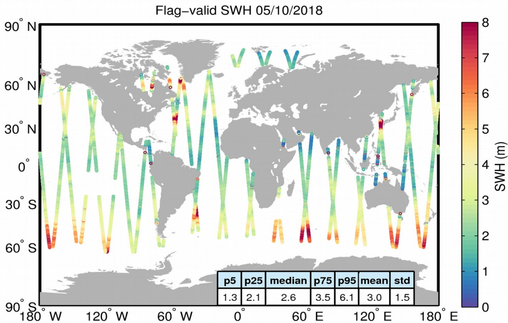
Figure 15. Geographical distribution of flag-valid SWH data over oceans and lakes for 05/10/2018. The statistical values shown in the table refer to the SWH in m and are calculated over all measurements shown in the figure.
