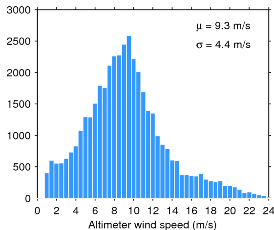
Figure 35. Histogram of science-valid wind over oceans and lakes for 05/10/2018. The mean ( \mu ) and standard deviation ( \sigma ) are also shown. Note that values larger than 24 m/s are excluded from the histogram for the sake of readability but not from the computation of \mu and \sigma .
