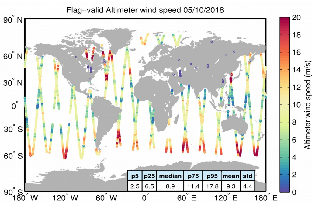
Figure 31. Geographical distribution of flag-valid wind data over oceans and lakes for 05/10/2018. The statistical values shown in the table refer to the wind in m/s and are calculated over all measurements shown in the figure.
