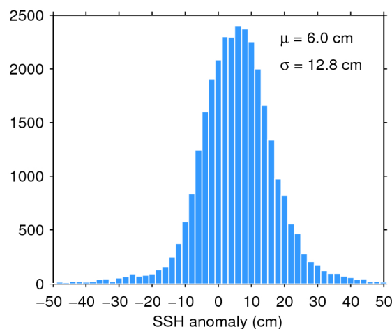
Figure 11. Histogram of science-valid SSH anomaly over oceans and lakes for 05/10/2018. The mean ( \mu ) and standard deviation ( \sigma ) are also shown. Note that values outside [-50 50] cm are excluded from the histogram for the sake of readability but not from the computation of \mu and \sigma .
