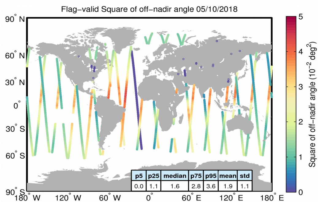
Figure 37. Geographical distribution of flag-valid mispointing data over oceans and lakes for 05/10/2018. The statistical values shown in the table refer to the mispointing in 10^{-2} \text{ deg}^2 and are calculated over all measurements shown in the figure.
