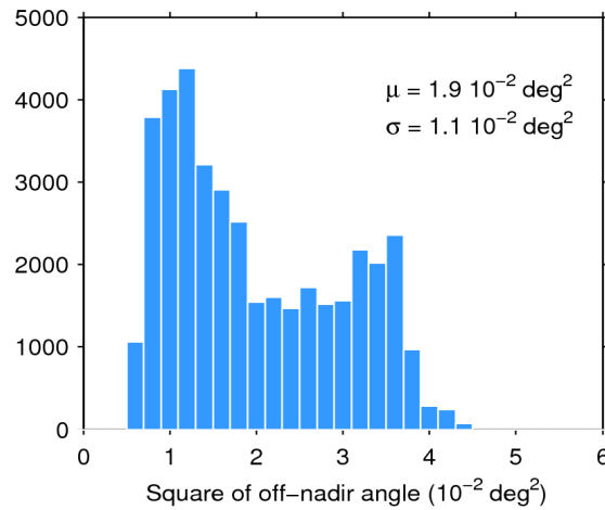
Figure 39. Histogram of flag-valid mispointing over oceans and lakes for 05/10/2018. The mean ( \mu ) and standard deviation ( \sigma ) are also shown. Note that values larger than 6 \cdot 10^{-2} \text{ deg}^2 are excluded from the histogram for the sake of readability but not from the computation of \mu and \sigma .
