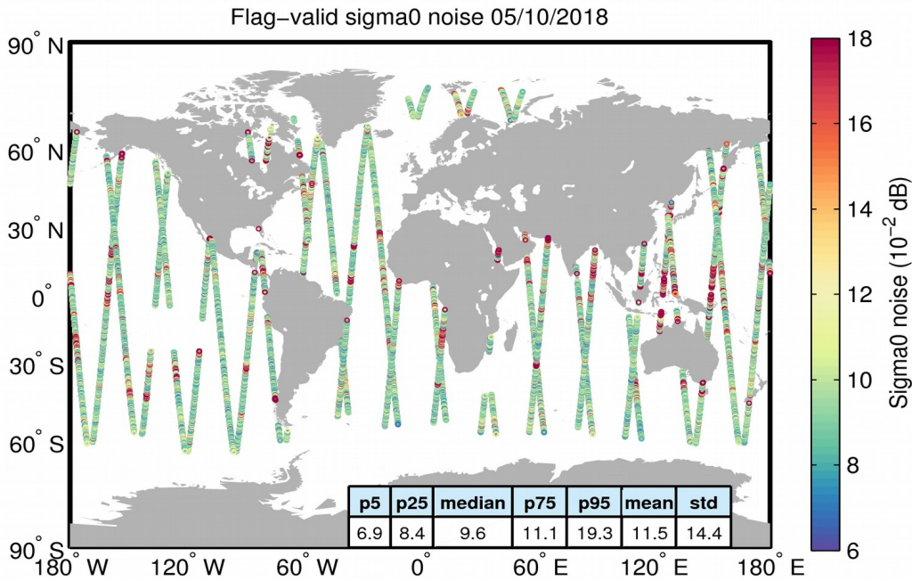
Figure 26. Geographical distribution of flag-valid 20-Hz sigma0 measurement noise over oceans and lakes for 05/10/2018. The statistical values shown in the table refer to the sigma0 noise and are calculated over all measurements shown in the figure.
