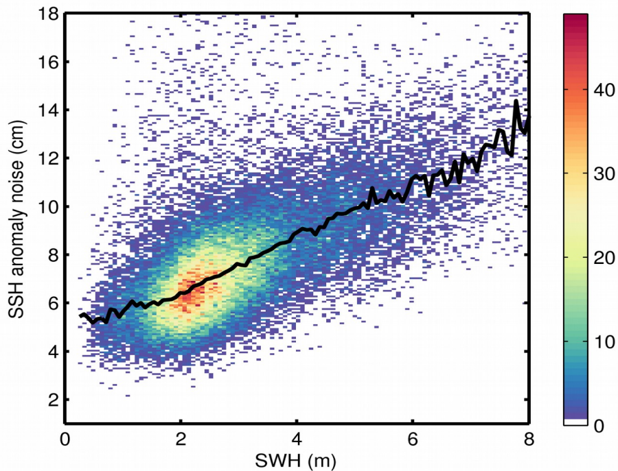
Figure 9. 2D histogram showing flag-valid SSH anomaly noise as a function of SWH for 05/10/2018. The black line denotes the median SSH anomaly noise as a function of SWH.
