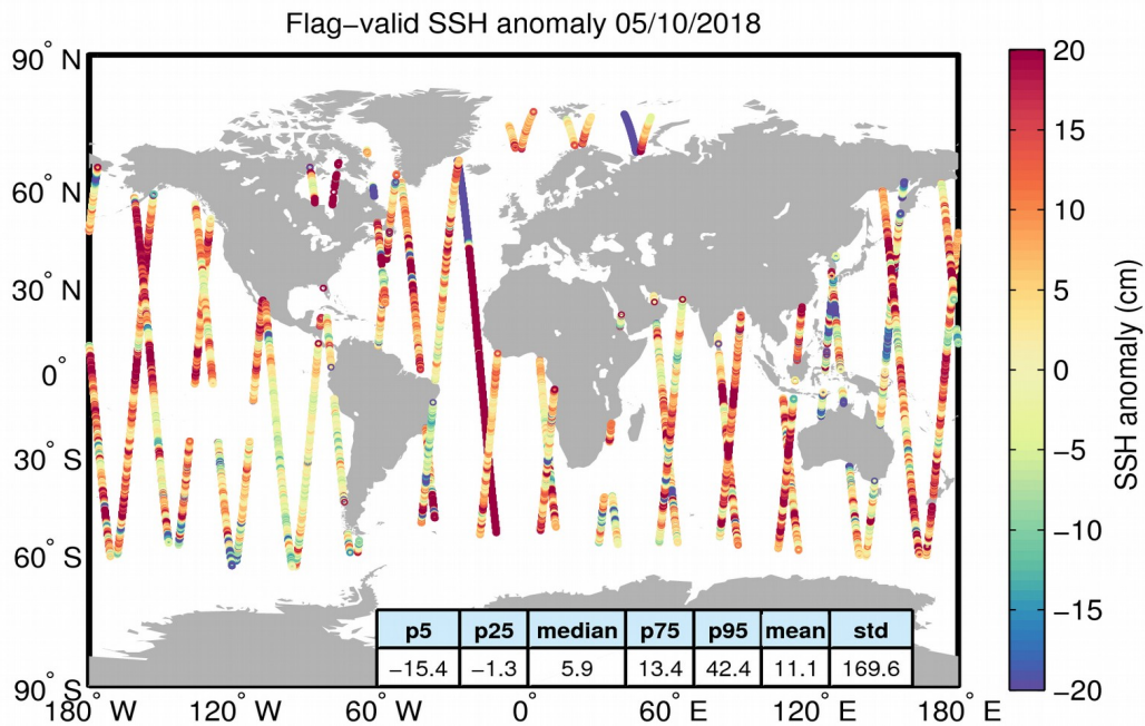
Figure 5. Geographical distribution of flag-valid 1-Hz SSH anomaly data over oceans and lakes for 05/10/2018. The statistical values shown in the table refer to the SSH anomaly in cm and are calculated over all measurements shown in the figure.
