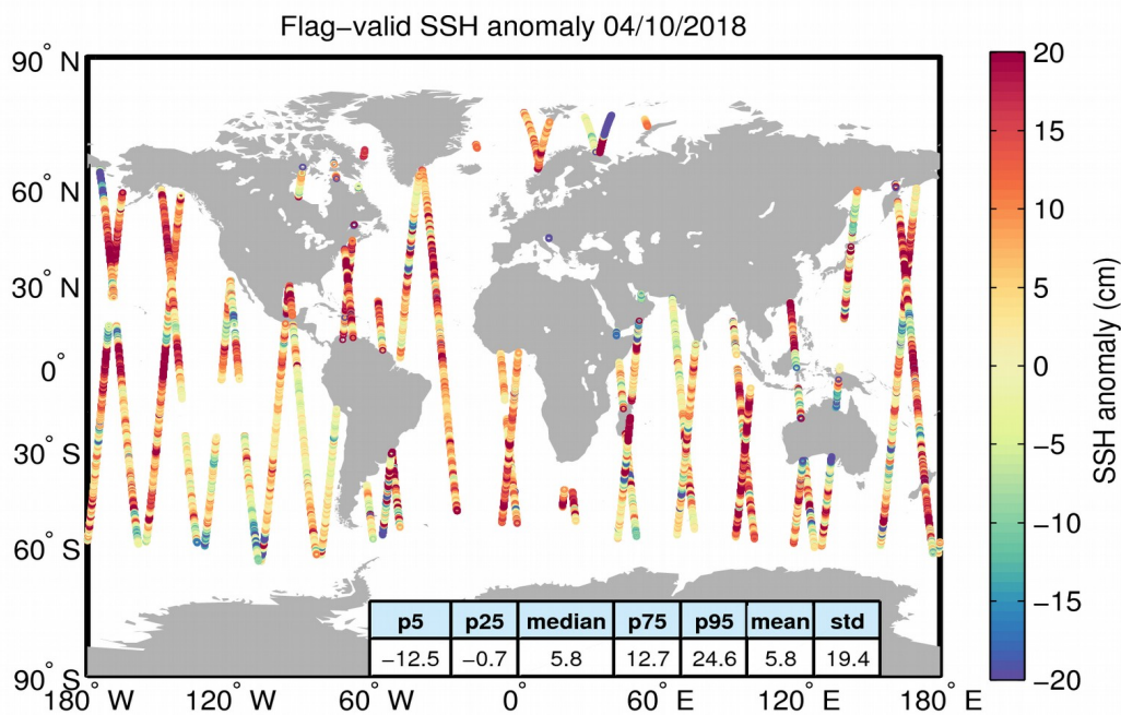
Figure 5. Geographical distribution of flag-valid 1-Hz SSH anomaly data over oceans and lakes for 04/10/2018. The statistical values shown in the table refer to the SSH anomaly in cm and are calculated over all measurements shown in the figure.
