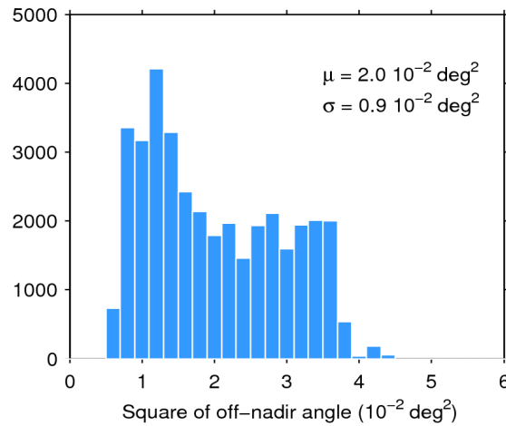
Figure 39. Histogram of flag-valid mispointing over oceans and lakes for 04/10/2018. The mean ( \mu ) and standard deviation ( \sigma ) are also shown. Note that values larger than 6 \cdot 10^{-2} \text{ deg}^2 are excluded from the histogram for the sake of readability but not from the computation of \mu and \sigma .
