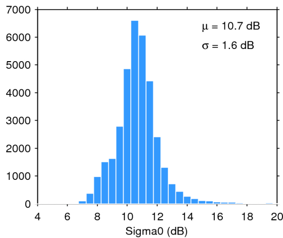
Figure 28. Histogram of science-valid sigma0 over oceans and lakes for 04/10/2018. The mean ( \mu ) and standard deviation ( \sigma ) are also shown. Note that values outside [4 20] dB are excluded from the histogram for the sake of readability but not from the computation of \mu and \sigma .
