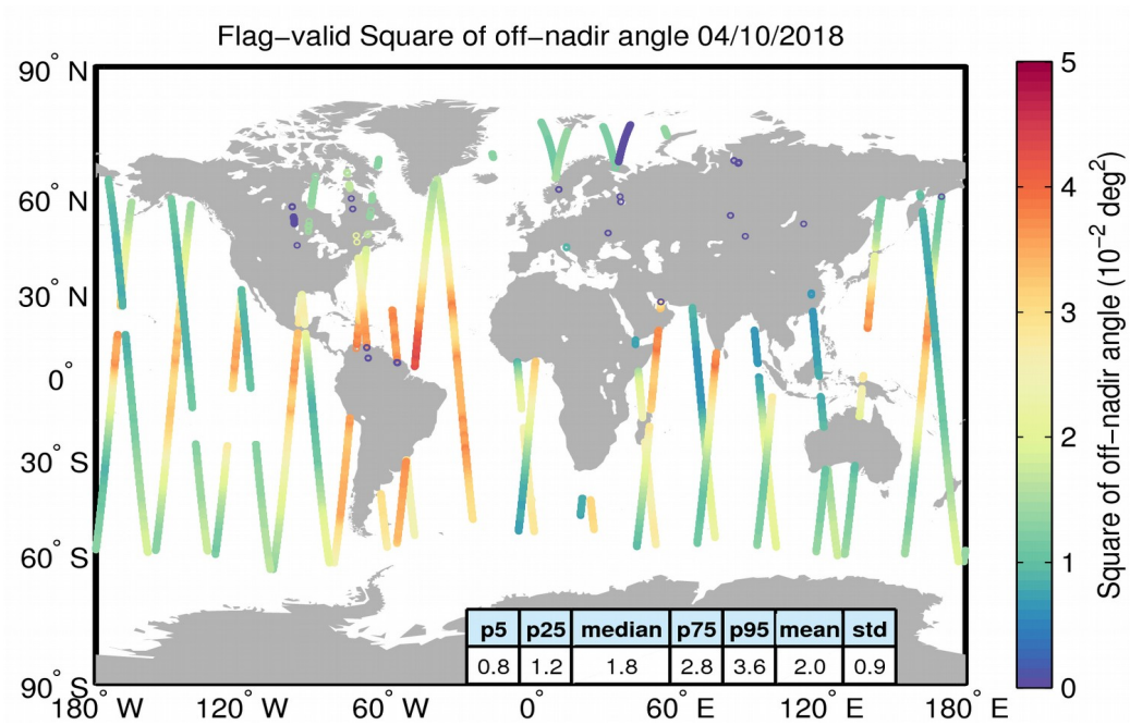
Figure 37. Geographical distribution of flag-valid mispointing data over oceans and lakes for 04/10/2018. The statistical values shown in the table refer to the mispointing in 10^{-2} \text{ deg}^2 and are calculated over all measurements shown in the figure.
