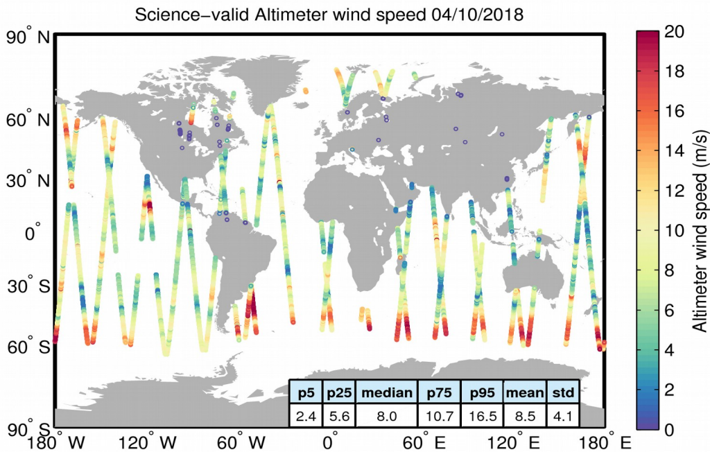
Figure 34. Geographical distribution of science-valid wind data over oceans and lakes for 04/10/2018. The statistical values shown in the table refer to the wind in m/s and are calculated over all measurements shown in the figure. Gray circles denote records that have been rejected based on the editing criteria described in Table 5.
