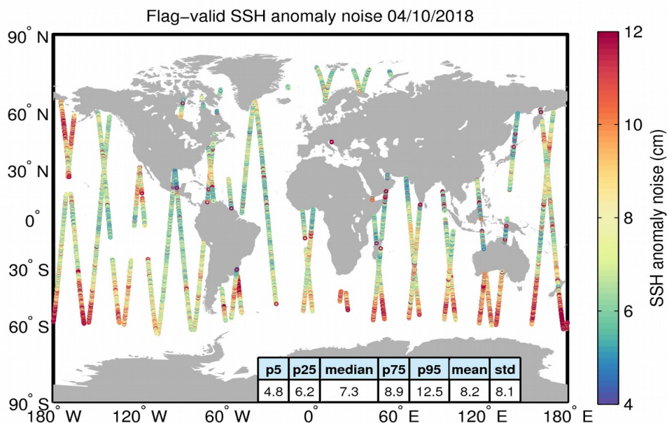
Figure 8. Geographical distribution of flag-valid 20-Hz SSH anomaly measurement noise over oceans and lakes for 04/10/2018. The statistical values shown in the table refer to the SSH anomaly noise and are calculated over all measurements shown in the figure.
