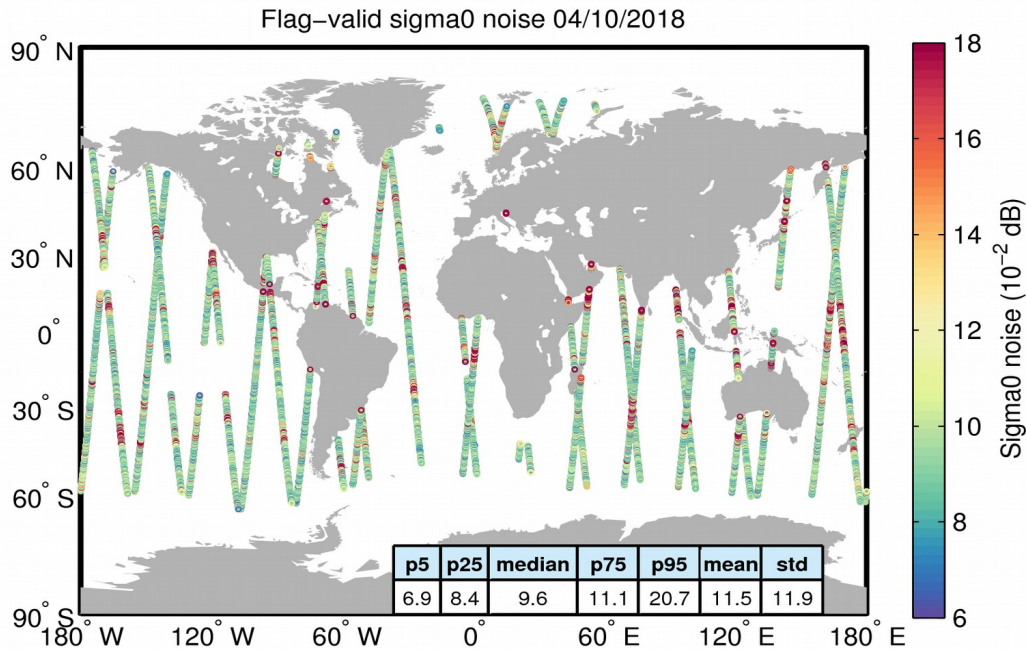
Figure 26. Geographical distribution of flag-valid 20-Hz sigma0 measurement noise over oceans and lakes for 04/10/2018. The statistical values shown in the table refer to the sigma0 noise and are calculated over all measurements shown in the figure.
