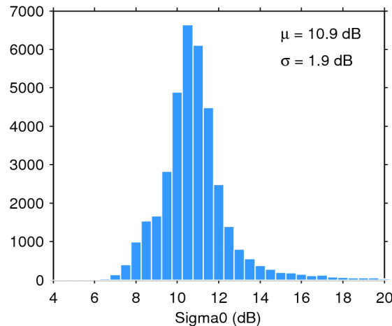
Figure 25. Histogram of flag-valid sigma0 over oceans and lakes for 04/10/2018. The mean ( \mu ) and standard deviation ( \sigma ) are also shown. Note that values outside [4 20] dB are excluded from the histogram for the sake of readability but not from the computation of \mu and \sigma .
