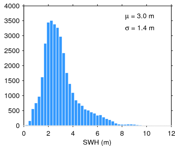
Figure 20. Histogram of science-valid SWH over oceans and lakes for 04/10/2018. The mean ( \mu ) and standard deviation ( \sigma ) are also shown. Note that values larger than 12 m are excluded from the histogram for the sake of readability but not from the computation of \mu and \sigma .
