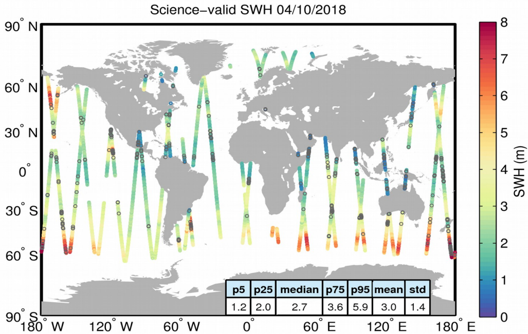
Figure 19. Geographical distribution of science-valid SWH data over oceans and lakes for 04/10/2018. The statistical values shown in the table refer to the SWH in m and are calculated over all measurements shown in the figure. Gray circles denote records that have been rejected based on the editing criteria described in Table 3.
