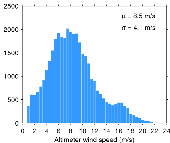
Figure 35. Histogram of science-valid wind over oceans and lakes for 04/10/2018. The mean ( \mu ) and standard deviation ( \sigma ) are also shown. Note that values larger than 24 m/s are excluded from the histogram for the sake of readability but not from the computation of \mu and \sigma .
