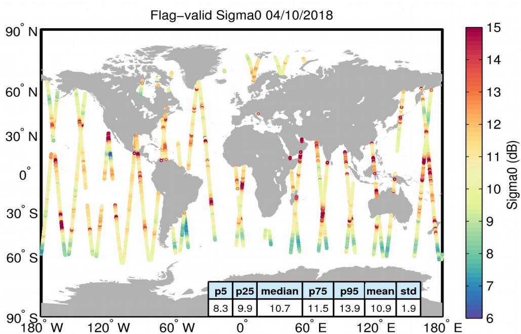
Figure 23. Geographical distribution of flag-valid sigma0 data over oceans and lakes for 04/10/2018. The statistical values shown in the table refer to the sigma0 in dB and are calculated over all measurements shown in the figure.
