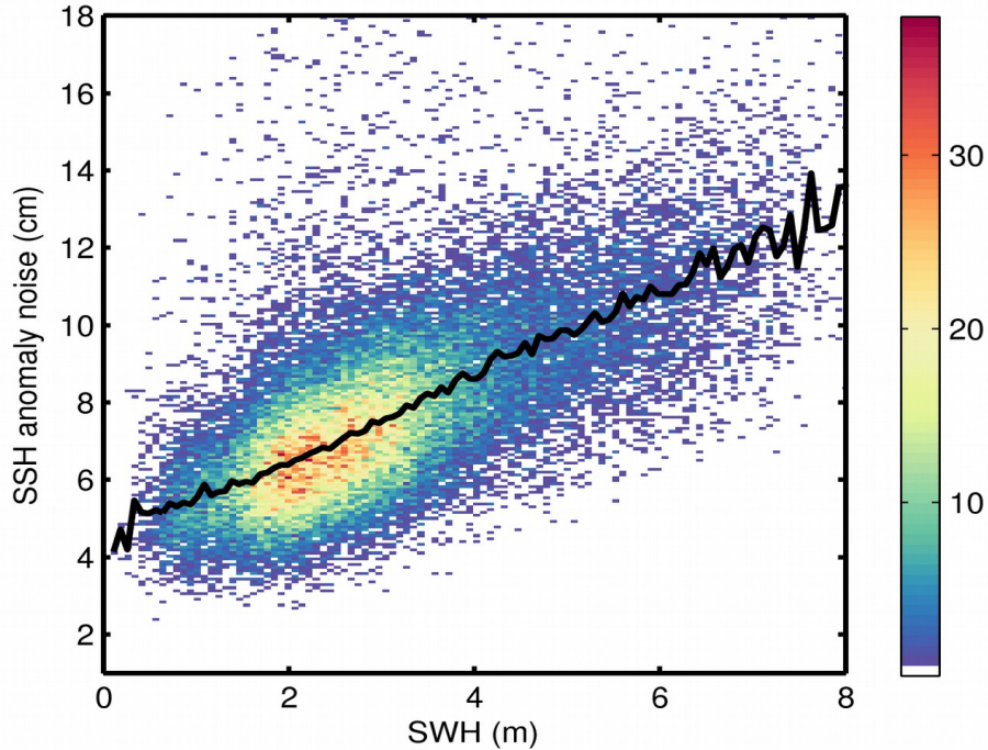
Figure 9. 2D histogram showing flag-valid SSH anomaly noise as a function of SWH for 04/10/2018. The black line denotes the median SSH anomaly noise as a function of SWH.
