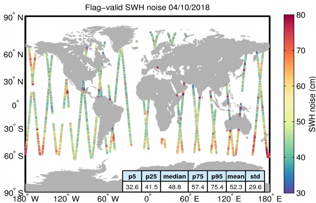
Figure 18. Geographical distribution of flag-valid 20-Hz SWH measurement noise over oceans and lakes for 04/10/2018. The statistical values shown in the table refer to the SWH noise and are calculated over all measurements shown in the figure.
