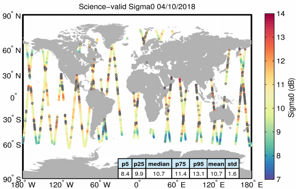
Figure 27. Geographical distribution of science-valid sigma0 data over oceans and lakes for 04/10/2018. The statistical values shown in the table refer to the sigma0 in dB and are calculated over all measurements shown in the figure. Gray circles denote records that have been rejected based on the editing criteria described in Table 4.
