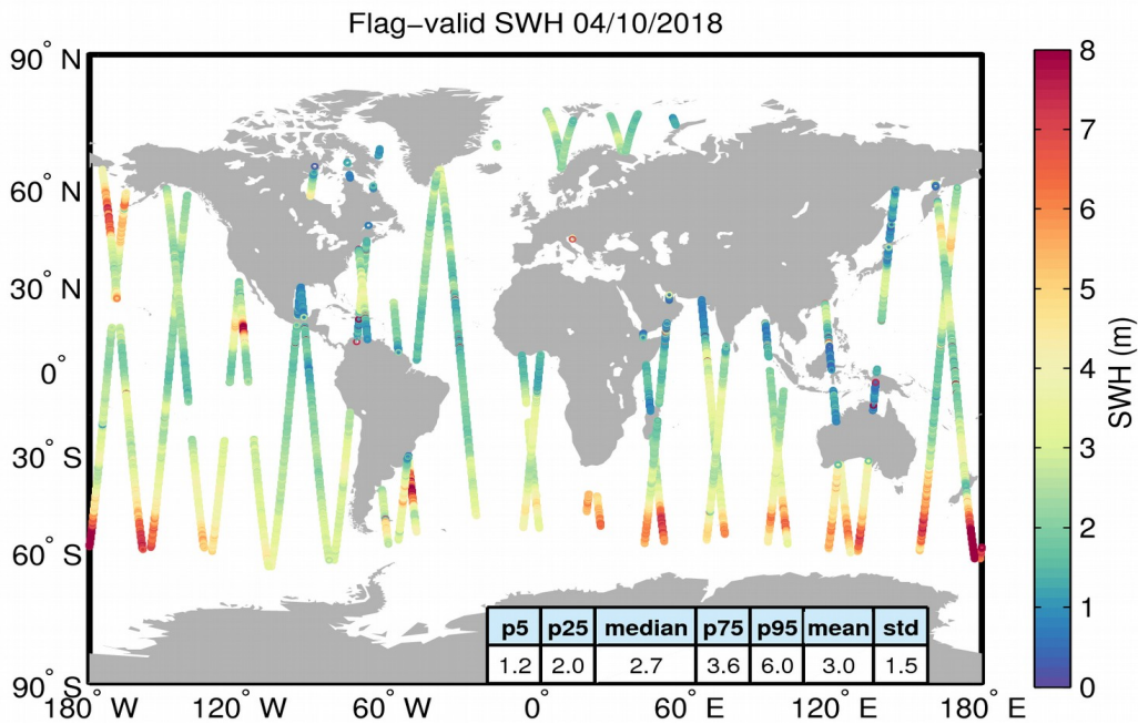
Figure 15. Geographical distribution of flag-valid SWH data over oceans and lakes for 04/10/2018. The statistical values shown in the table refer to the SWH in m and are calculated over all measurements shown in the figure.
