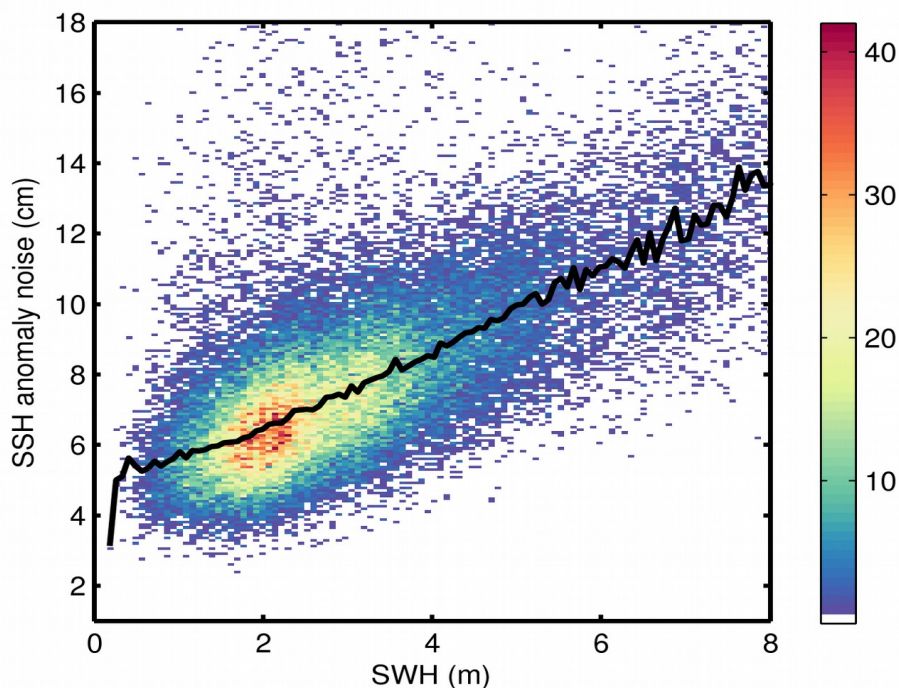
Figure 9. 2D histogram showing flag-valid SSH anomaly noise as a function of SWH for 03/10/2018. The black line denotes the median SSH anomaly noise as a function of SWH.
