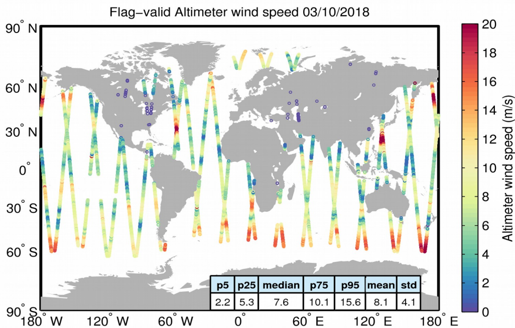
Figure 31. Geographical distribution of flag-valid wind data over oceans and lakes for 03/10/2018. The statistical values shown in the table refer to the wind in m/s and are calculated over all measurements shown in the figure.
