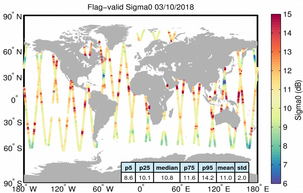
Figure 23. Geographical distribution of flag-valid sigma0 data over oceans and lakes for 03/10/2018. The statistical values shown in the table refer to the sigma0 in dB and are calculated over all measurements shown in the figure.
