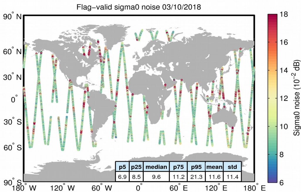
Figure 26. Geographical distribution of flag-valid 20-Hz sigma0 measurement noise over oceans and lakes for 03/10/2018. The statistical values shown in the table refer to the sigma0 noise and are calculated over all measurements shown in the figure.
