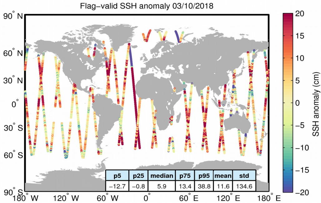
Figure 5. Geographical distribution of flag-valid 1-Hz SSH anomaly data over oceans and lakes for 03/10/2018. The statistical values shown in the table refer to the SSH anomaly in cm and are calculated over all measurements shown in the figure.
