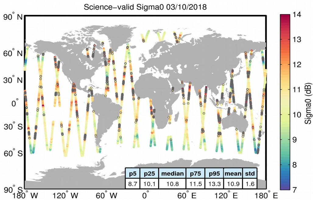
Figure 27. Geographical distribution of science-valid sigma0 data over oceans and lakes for 03/10/2018. The statistical values shown in the table refer to the sigma0 in dB and are calculated over all measurements shown in the figure. Gray circles denote records that have been rejected based on the editing criteria described in Table 4.
