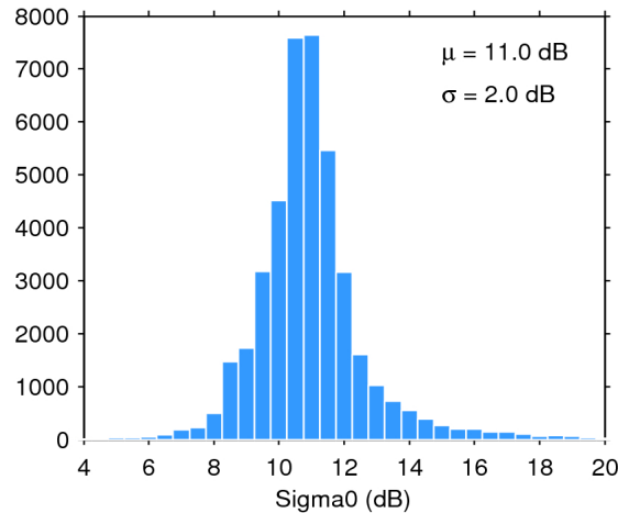
Figure 25. Histogram of flag-valid sigma0 over oceans and lakes for 03/10/2018. The mean ( \mu ) and standard deviation ( \sigma ) are also shown. Note that values outside [4 20] dB are excluded from the histogram for the sake of readability but not from the computation of \mu and \sigma .
