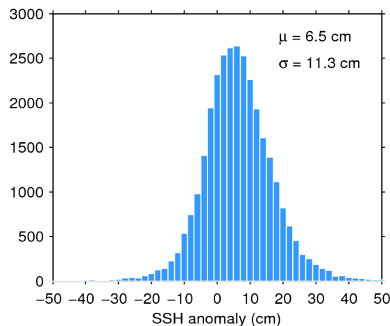
Figure 11. Histogram of science-valid SSH anomaly over oceans and lakes for 03/10/2018. The mean ( \mu ) and standard deviation ( \sigma ) are also shown. Note that values outside [-50 50] cm are excluded from the histogram for the sake of readability but not from the computation of \mu and \sigma .
