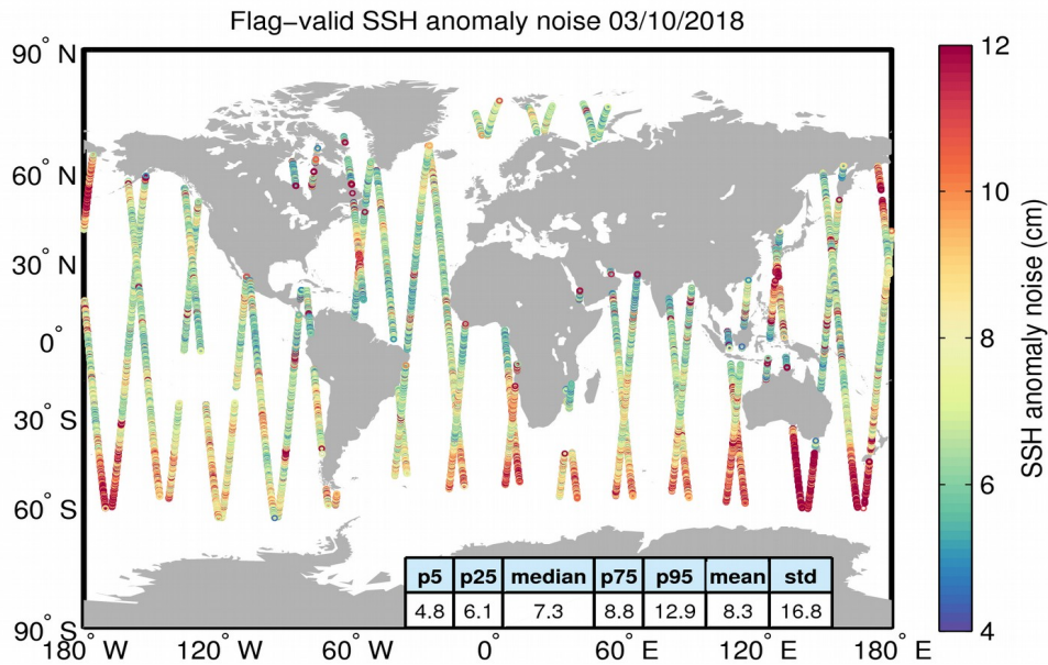
Figure 8. Geographical distribution of flag-valid 20-Hz SSH anomaly measurement noise over oceans and lakes for 03/10/2018. The statistical values shown in the table refer to the SSH anomaly noise and are calculated over all measurements shown in the figure.
