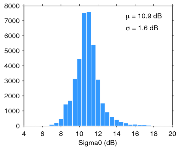
Figure 28. Histogram of science-valid sigma0 over oceans and lakes for 03/10/2018. The mean ( \mu ) and standard deviation ( \sigma ) are also shown. Note that values outside [4 20] dB are excluded from the histogram for the sake of readability but not from the computation of \mu and \sigma .
