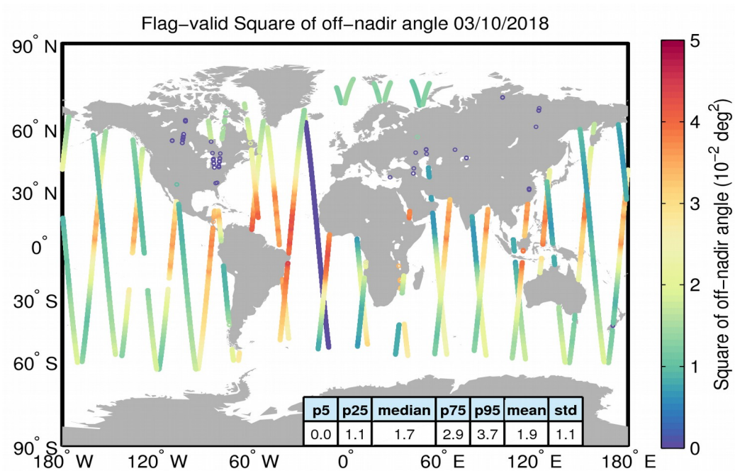
Figure 37. Geographical distribution of flag-valid mispointing data over oceans and lakes for 03/10/2018. The statistical values shown in the table refer to the mispointing in 10^{-2} \text{ deg}^2 and are calculated over all measurements shown in the figure.
