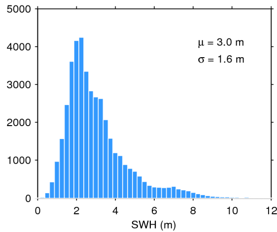
Figure 17. Histogram of flag-valid SWH over oceans and lakes for 03/10/2018. The mean ( \mu ) and standard deviation ( \sigma ) are also shown. Note that values larger than 12 m are excluded from the histogram for the sake of readability but not from the computation of \mu and \sigma .
