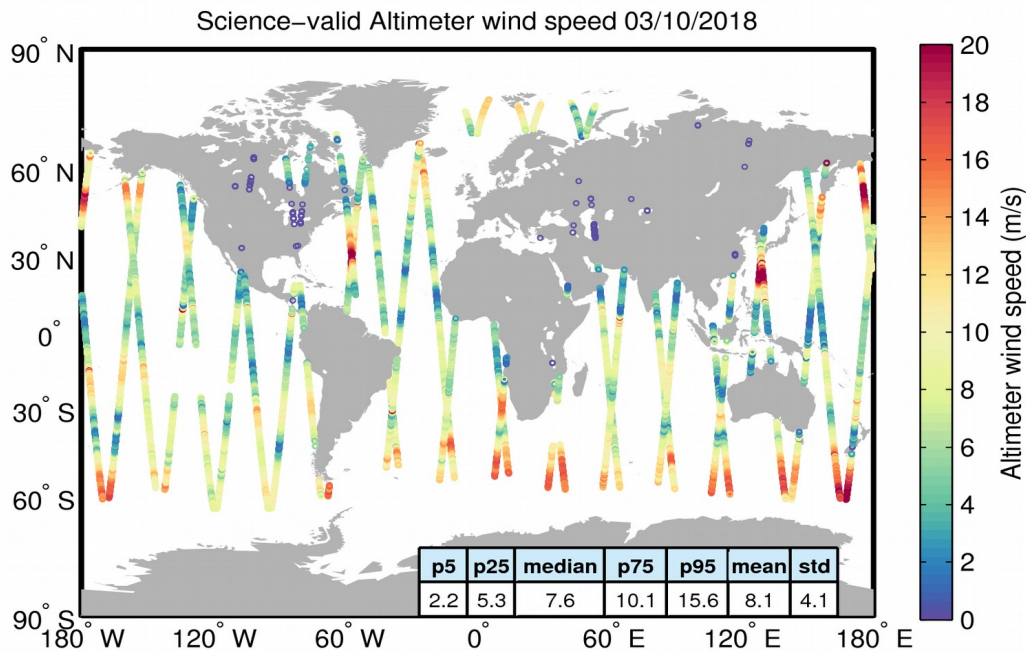
Figure 34. Geographical distribution of science-valid wind data over oceans and lakes for 03/10/2018. The statistical values shown in the table refer to the wind in m/s and are calculated over all measurements shown in the figure. Gray circles denote records that have been rejected based on the editing criteria described in Table 5.
