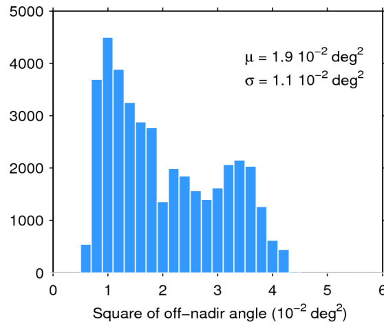
Figure 39. Histogram of flag-valid mispointing over oceans and lakes for 03/10/2018. The mean ( \mu ) and standard deviation ( \sigma ) are also shown. Note that values larger than 6 \cdot 10^{-2} \text{ deg}^2 are excluded from the histogram for the sake of readability but not from the computation of \mu and \sigma .
