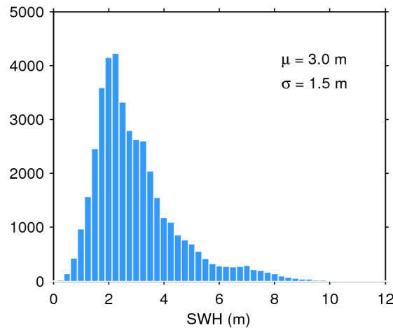
Figure 20. Histogram of science-valid SWH over oceans and lakes for 03/10/2018. The mean ( \mu ) and standard deviation ( \sigma ) are also shown. Note that values larger than 12 m are excluded from the histogram for the sake of readability but not from the computation of \mu and \sigma .
