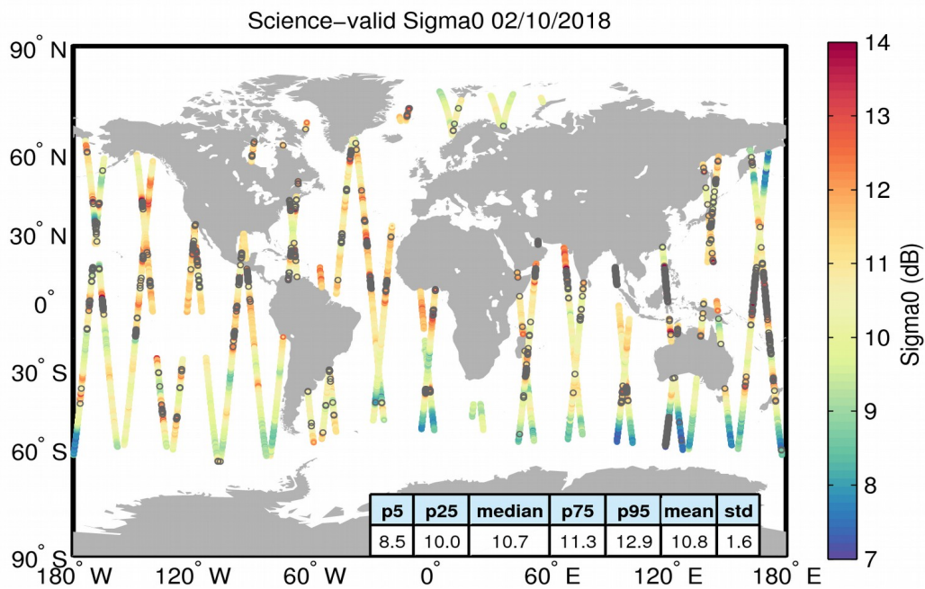
Figure 27. Geographical distribution of science-valid sigma0 data over oceans and lakes for 02/10/2018. The statistical values shown in the table refer to the sigma0 in dB and are calculated over all measurements shown in the figure. Gray circles denote records that have been rejected based on the editing criteria described in Table 4.
