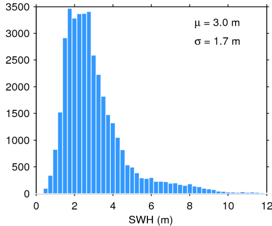
Figure 20. Histogram of science-valid SWH over oceans and lakes for 02/10/2018. The mean ( \mu ) and standard deviation ( \sigma ) are also shown. Note that values larger than 12 m are excluded from the histogram for the sake of readability but not from the computation of \mu and \sigma .
