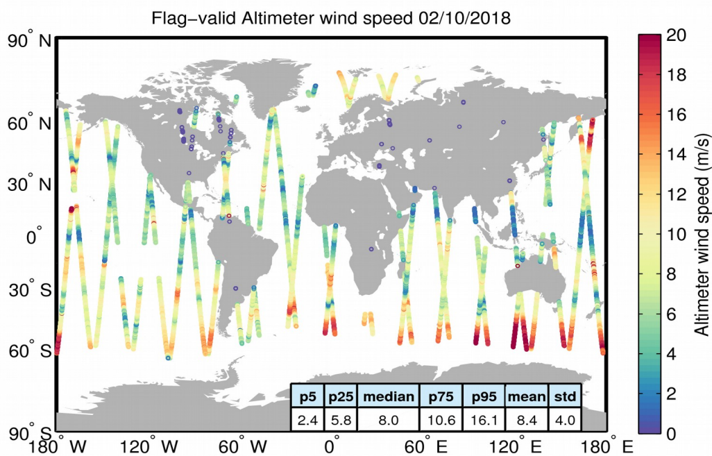
Figure 31. Geographical distribution of flag-valid wind data over oceans and lakes for 02/10/2018. The statistical values shown in the table refer to the wind in m/s and are calculated over all measurements shown in the figure.
