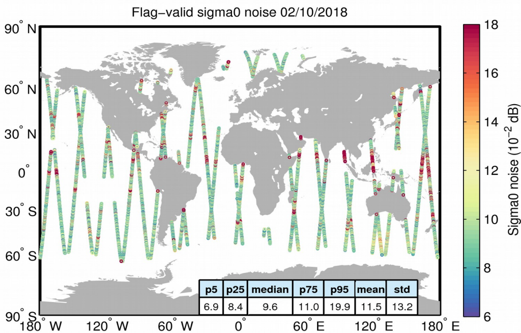
Figure 26. Geographical distribution of flag-valid 20-Hz sigma0 measurement noise over oceans and lakes for 02/10/2018. The statistical values shown in the figure refer to the sigma0 noise and are calculated over all measurements shown in the figure.
