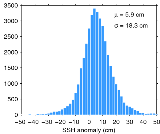
Figure 7. Histogram of flag-valid SSH anomaly over oceans and lakes for 02/10/2018. The mean ( \mu ) and standard deviation ( \sigma ) are also shown. Note that values outside [-50\ 50] cm are excluded from the histogram for the sake of readability but not from the computation of \mu and \sigma .
