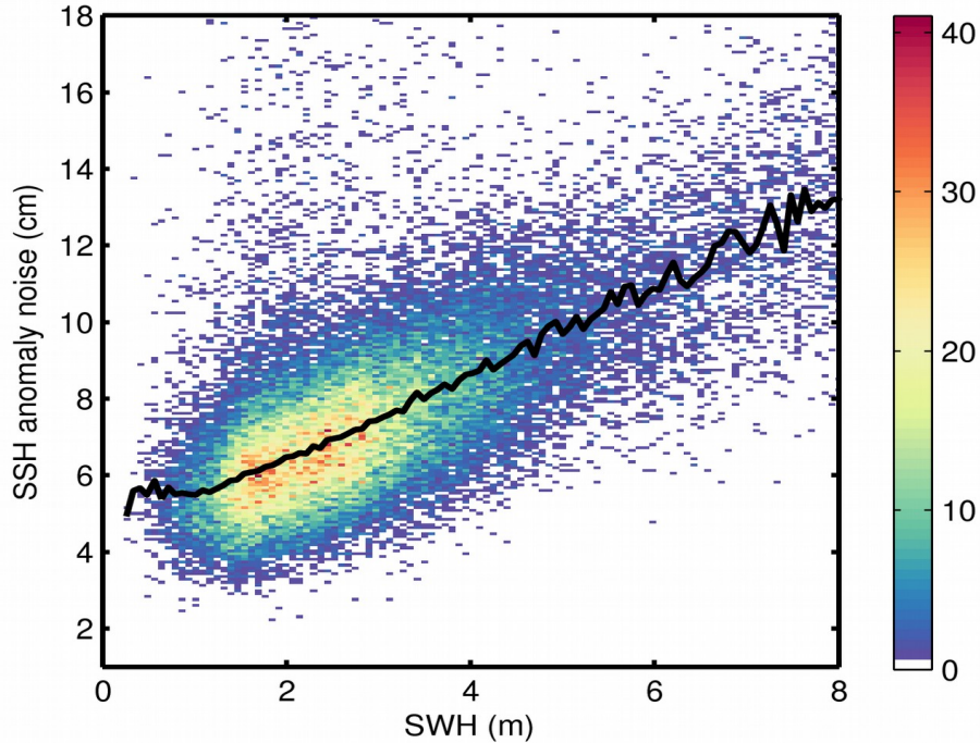
Figure 9. 2D histogram showing flag-valid SSH anomaly noise as a function of SWH for 02/10/2018. The black line denotes the median SSH anomaly noise as a function of SWH.
