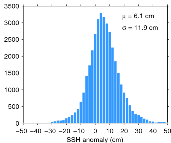
Figure 11. Histogram of science-valid SSH anomaly over oceans and lakes for 02/10/2018. The mean ( \mu ) and standard deviation ( \sigma ) are also shown. Note that values outside [-50 50] cm are excluded from the histogram for the sake of readability but not from the computation of \mu and \sigma .
