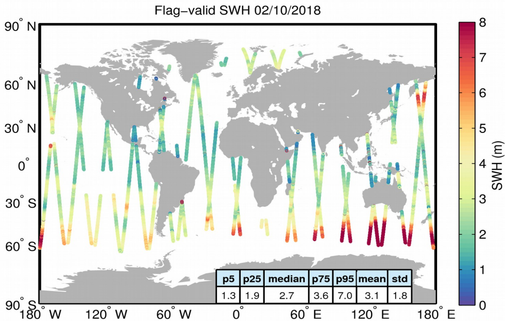
Figure 15. Geographical distribution of flag-valid SWH data over oceans and lakes for 02/10/2018. The statistical values shown in the table refer to the SWH in m and are calculated over all measurements shown in the figure.
