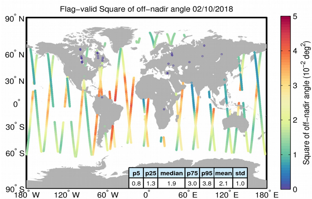
Figure 37. Geographical distribution of flag-valid mispointing data over oceans and lakes for 02/10/2018. The statistical values shown in the table refer to the mispointing in 10^{-2} deg 2 and are calculated over all measurements shown in the figure.
