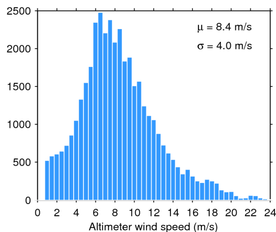
Figure 35. Histogram of science-valid wind over oceans and lakes for 02/10/2018. The mean ( \mu ) and standard deviation ( \sigma ) are also shown. Note that values larger than 24 m/s are excluded from the histogram for the sake of readability but not from the computation of \mu and \sigma .
