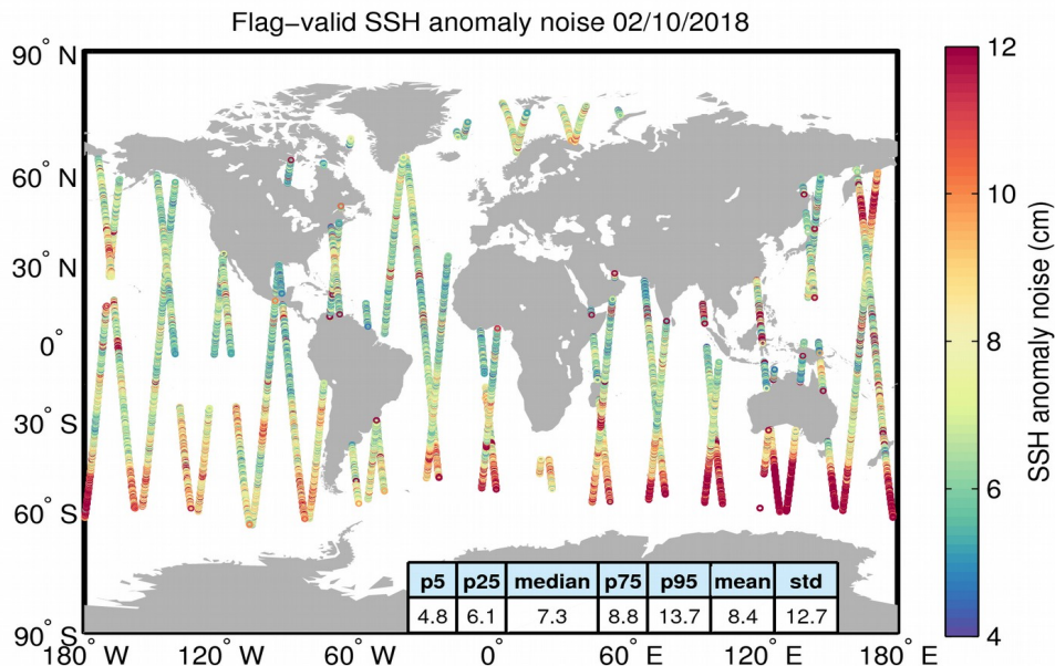
Figure 8. Geographical distribution of flag-valid 20-Hz SSH anomaly measurement noise over oceans and lakes for 02/10/2018. The statistical values shown in the table refer to the SSH anomaly noise and are calculated over all measurements shown in the figure.
