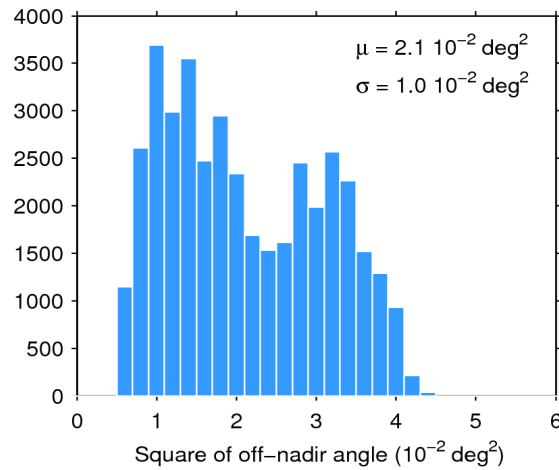
Figure 39. Histogram of flag-valid mispointing over oceans and lakes for 02/10/2018. The mean ( \mu ) and standard deviation ( \sigma ) are also shown. Note that values larger than 6 \cdot 10^{-2} \text{ deg}^2 are excluded from the histogram for the sake of readability but not from the computation of \mu and \sigma .
