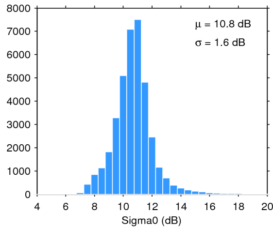
Figure 28. Histogram of science-valid sigma0 over oceans and lakes for 02/10/2018. The mean ( \mu ) and standard deviation ( \sigma ) are also shown. Note that values outside [4 20] dB are excluded from the histogram for the sake of readability but not from the computation of \mu and \sigma .
