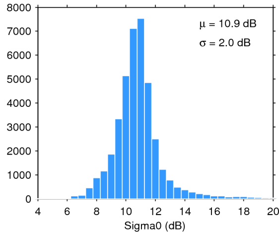
Figure 25. Histogram of flag-valid sigma0 over oceans and lakes for 02/10/2018. The mean ( \mu ) and standard deviation ( \sigma ) are also shown. Note that values outside [4 20] dB are excluded from the histogram for the sake of readability but not from the computation of \mu and \sigma .
