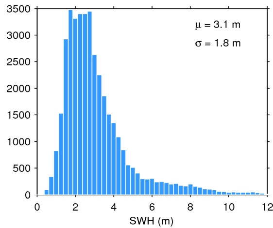
Figure 17. Histogram of flag-valid SWH over oceans and lakes for 02/10/2018. The mean ( \mu ) and standard deviation ( \sigma ) are also shown. Note that values larger than 12 m are excluded from the histogram for the sake of readability but not from the computation of \mu and \sigma .
