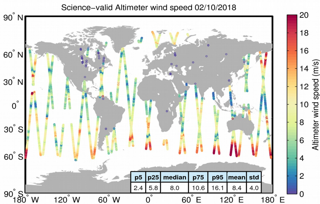
Figure 34. Geographical distribution of science-valid wind data over oceans and lakes for 02/10/2018. The statistical values shown in the table refer to the wind in m/s and are calculated over all measurements shown in the figure. Gray circles denote records that have been rejected based on the editing criteria described in Table 5.
