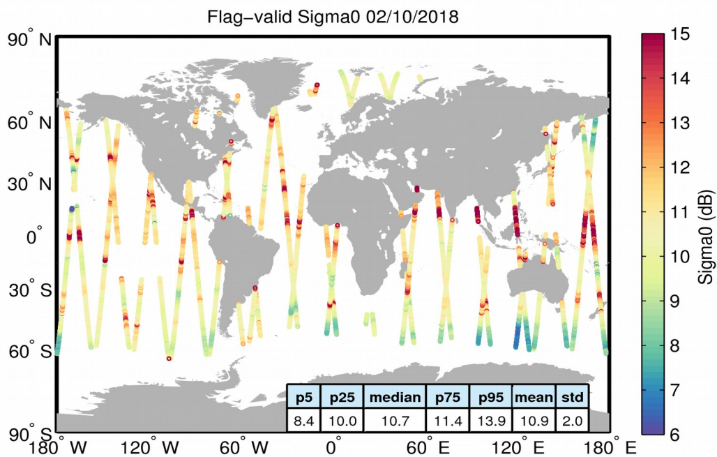
Figure 23. Geographical distribution of flag-valid sigma0 data over oceans and lakes for 02/10/2018. The statistical values shown in the table refer to the sigma0 in dB and are calculated over all measurements shown in the figure.
