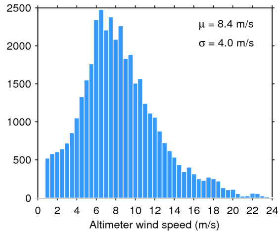
Figure 33. Histogram of flag-valid wind over oceans and lakes for 02/10/2018. The mean ( \mu ) and standard deviation ( \sigma ) are also shown. Note that values larger than 24 m/s are excluded from the histogram for the sake of readability but not from the computation of \mu and \sigma .
