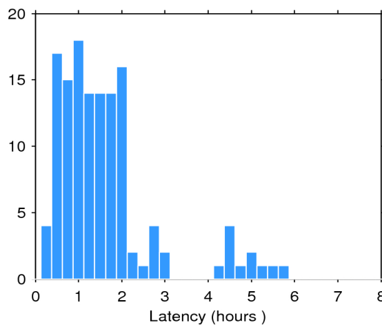
Figure 2. Histogram of the data latency for 02/10/2018. The y-axis denotes the number of files that are made available with a delay of x-hours with respect to the mean time of the records stored in the file.
