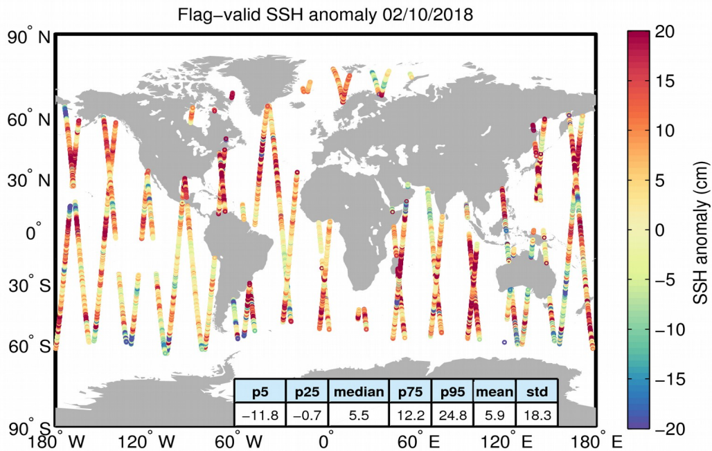
Figure 5. Geographical distribution of flag-valid 1-Hz SSH anomaly data over oceans and lakes for 02/10/2018. The statistical values shown in the table refer to the SSH anomaly in cm and are calculated over all measurements shown in the figure.
