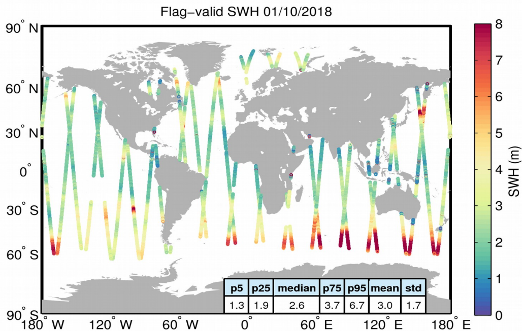
Figure 15. Geographical distribution of flag-valid SWH data over oceans and lakes for 01/10/2018. The statistical values shown in the table refer to the SWH in m and are calculated over all measurements shown in the figure.
