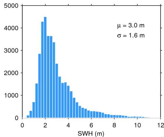
Figure 20. Histogram of science-valid SWH over oceans and lakes for 01/10/2018. The mean ( \mu ) and standard deviation ( \sigma ) are also shown. Note that values larger than 12 m are excluded from the histogram for the sake of readability but not from the computation of \mu and \sigma .
