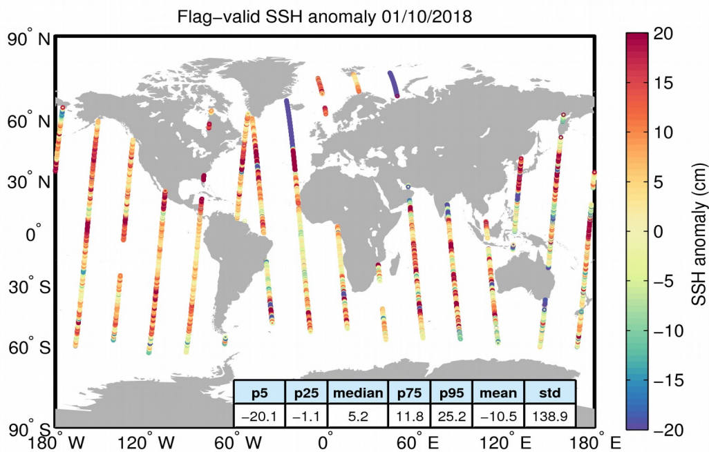
Figure 5. Geographical distribution of flag-valid 1-Hz SSH anomaly data over oceans and lakes for 01/10/2018. The statistical values shown in the table refer to the SSH anomaly in cm and are calculated over all measurements shown in the figure.
