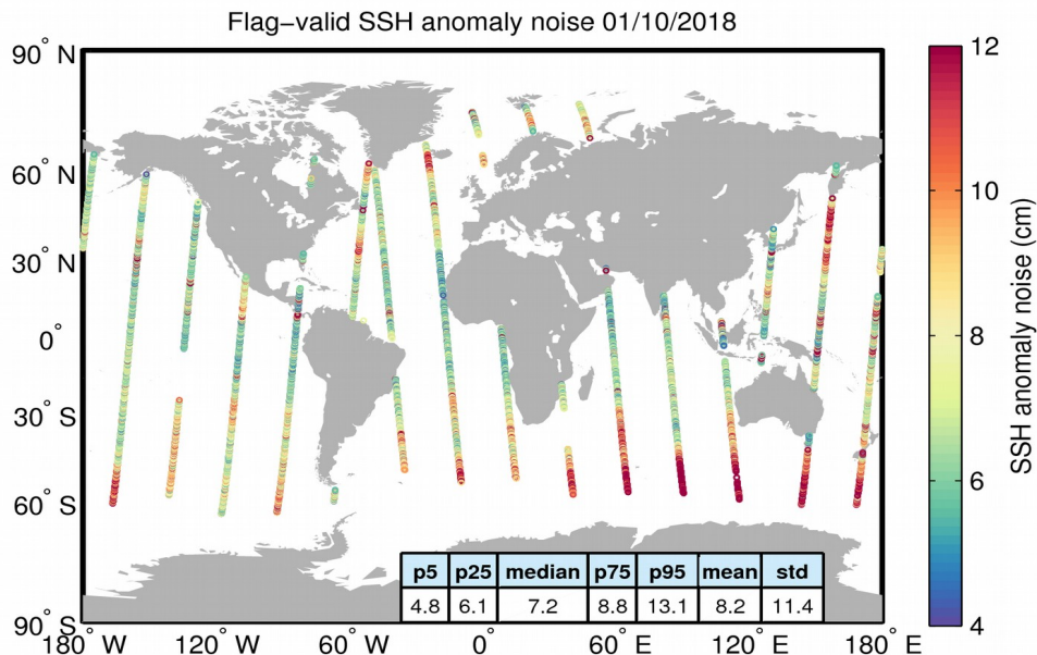
Figure 8. Geographical distribution of flag-valid 20-Hz SSH anomaly measurement noise over oceans and lakes for 01/10/2018. The statistical values shown in the table refer to the SSH anomaly noise and are calculated over all measurements shown in the figure.
