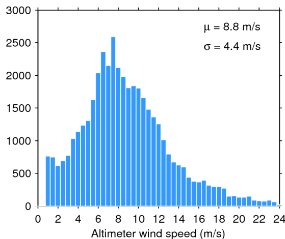
Figure 35. Histogram of science-valid wind over oceans and lakes for 01/10/2018. The mean ( \mu ) and standard deviation ( \sigma ) are also shown. Note that values larger than 24 m/s are excluded from the histogram for the sake of readability but not from the computation of \mu and \sigma .
