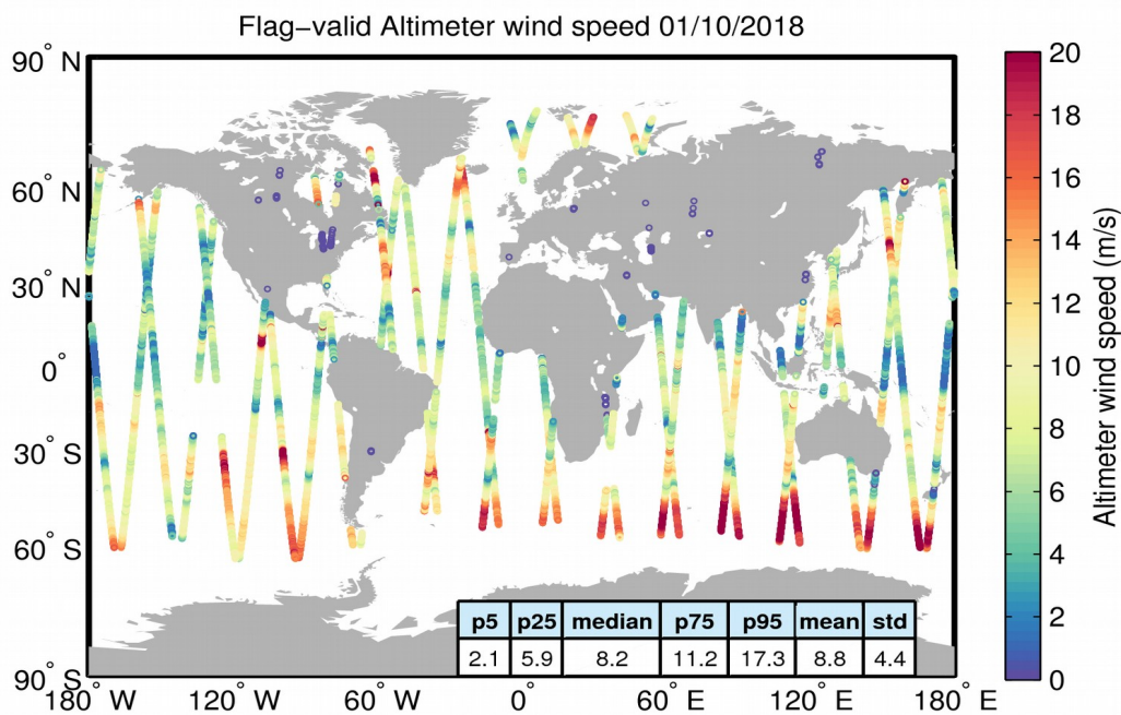
Figure 31. Geographical distribution of flag-valid wind data over oceans and lakes for 01/10/2018. The statistical values shown in the table refer to the wind in m/s and are calculated over all measurements shown in the figure.
