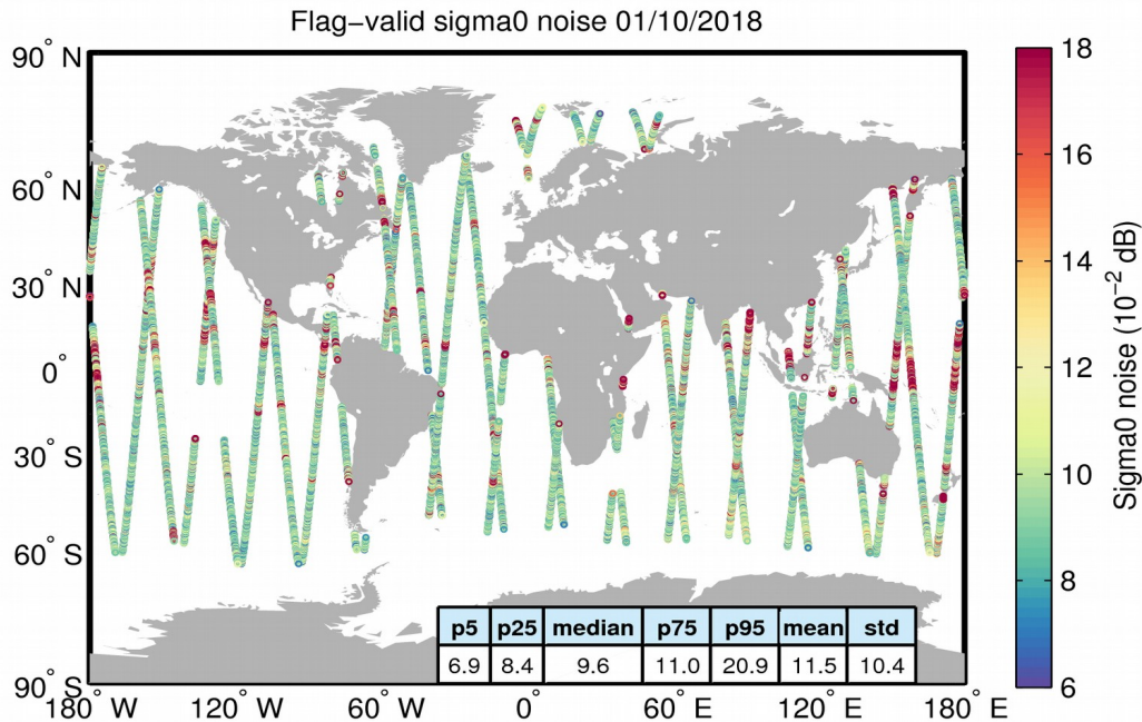
Figure 26. Geographical distribution of flag-valid 20-Hz sigma0 measurement noise over oceans and lakes for 01/10/2018. The statistical values shown in the table refer to the sigma0 noise and are calculated over all measurements shown in the figure.
