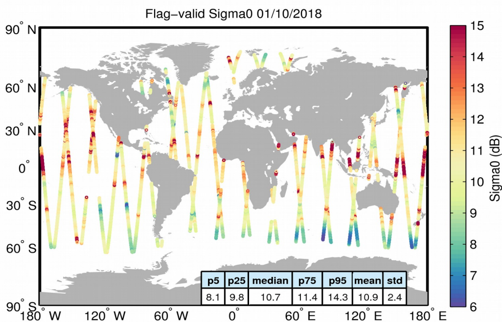
Figure 23. Geographical distribution of flag-valid sigma0 data over oceans and lakes for 01/10/2018. The statistical values shown in the table refer to the sigma0 in dB and are calculated over all measurements shown in the figure.
