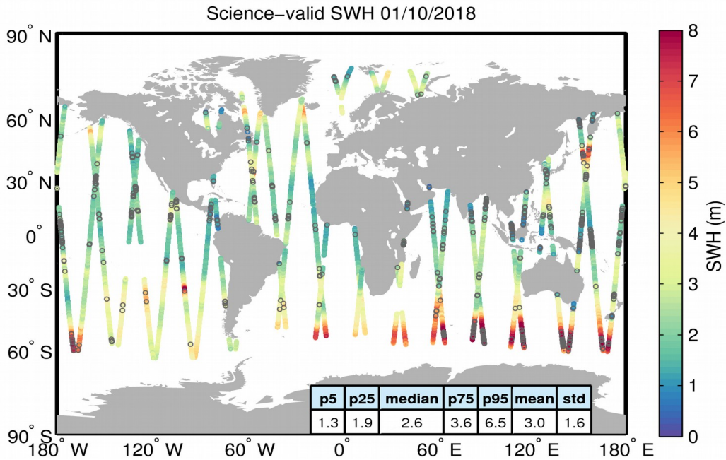
Figure 19. Geographical distribution of science-valid SWH data over oceans and lakes for 01/10/2018. The statistical values shown in the table refer to the SWH in m and are calculated over all measurements shown in the figure. Gray circles denote records that have been rejected based on the editing criteria described in Table 3.
