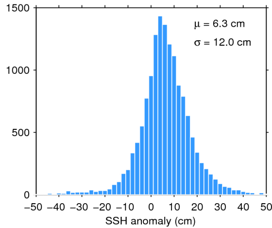
Figure 11. Histogram of science-valid SSH anomaly over oceans and lakes for 01/10/2018. The mean ( \mu ) and standard deviation ( \sigma ) are also shown. Note that values outside [-50 50] cm are excluded from the histogram for the sake of readability but not from the computation of \mu and \sigma .
