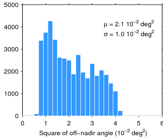
Figure 39. Histogram of flag-valid mispointing over oceans and lakes for 01/10/2018. The mean ( \mu ) and standard deviation ( \sigma ) are also shown. Note that values larger than 6 \cdot 10^{-2} \text{ deg}^2 are excluded from the histogram for the sake of readability but not from the computation of \mu and \sigma .
