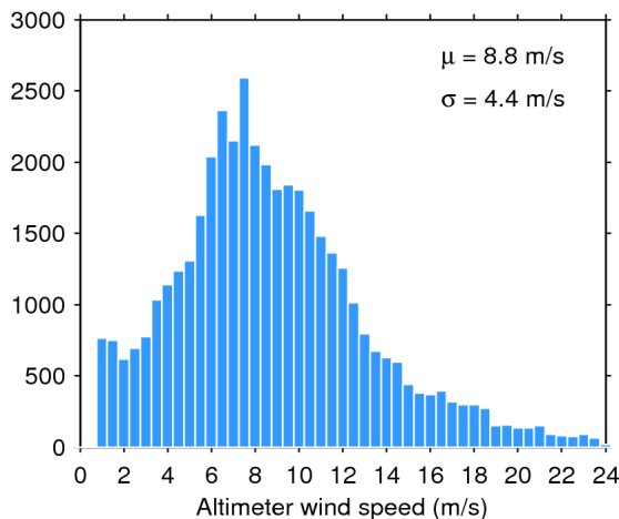
Figure 33. Histogram of flag-valid wind over oceans and lakes for 01/10/2018. The mean ( \mu ) and standard deviation ( \sigma ) are also shown. Note that values larger than 24 m/s are excluded from the histogram for the sake of readability but not from the computation of \mu and \sigma .
