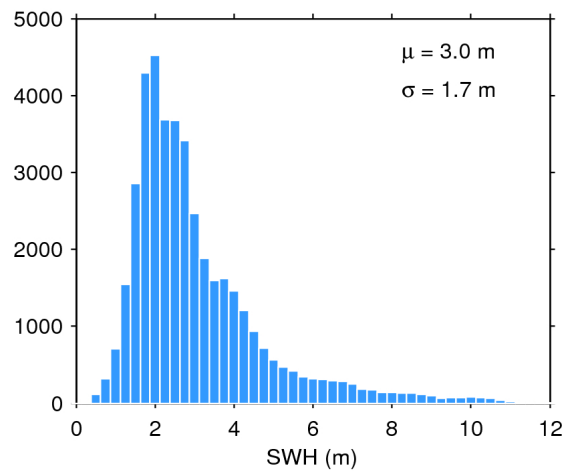
Figure 17. Histogram of flag-valid SWH over oceans and lakes for 01/10/2018. The mean ( \mu ) and standard deviation ( \sigma ) are also shown. Note that values larger than 12 m are excluded from the histogram for the sake of readability but not from the computation of \mu and \sigma .
