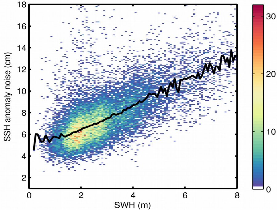
Figure 9. 2D histogram showing flag-valid SSH anomaly noise as a function of SWH for 01/10/2018. The black line denotes the median SSH anomaly noise as a function of SWH.
