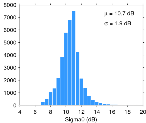
Figure 28. Histogram of science-valid sigma0 over oceans and lakes for 01/10/2018. The mean ( \mu ) and standard deviation ( \sigma ) are also shown. Note that values outside [4 20] dB are excluded from the histogram for the sake of readability but not from the computation of \mu and \sigma .
