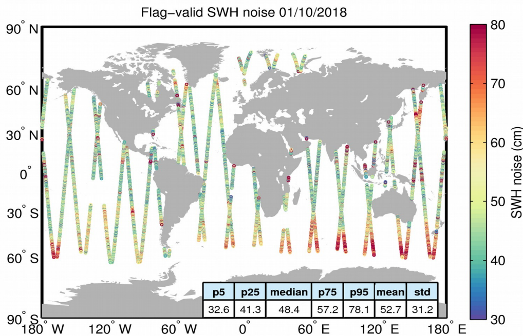
Figure 18. Geographical distribution of flag-valid 20-Hz SWH measurement noise over oceans and lakes for 01/10/2018. The statistical values shown in the table refer to the SWH noise and are calculated over all measurements shown in the figure.
