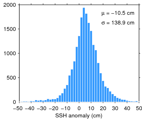
Figure 7. Histogram of flag-valid SSH anomaly over oceans and lakes for 01/10/2018. The mean ( \mu ) and standard deviation ( \sigma ) are also shown. Note that values outside [-50\ 50] cm are excluded from the histogram for the sake of readability but not from the computation of \mu and \sigma .
