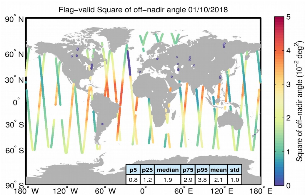
Figure 37. Geographical distribution of flag-valid mispointing data over oceans and lakes for 01/10/2018. The statistical values shown in the table refer to the mispointing in 10^{-2} deg 2 and are calculated over all measurements shown in the figure.
