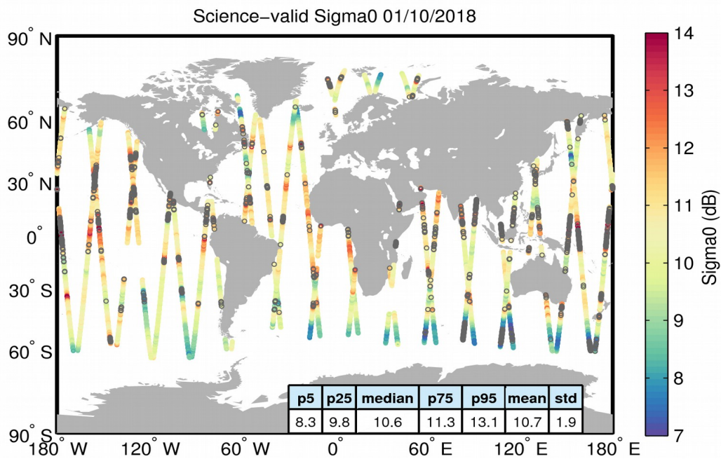
Figure 27. Geographical distribution of science-valid sigma0 data over oceans and lakes for 01/10/2018. The statistical values shown in the table refer to the sigma0 in dB and are calculated over all measurements shown in the figure. Gray circles denote records that have been rejected based on the editing criteria described in Table 4.
