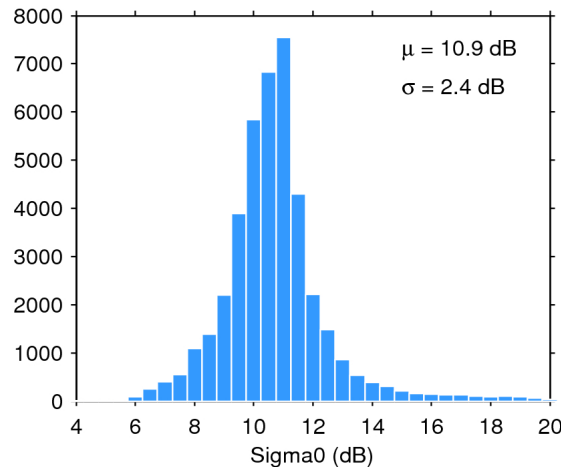
Figure 25. Histogram of flag-valid sigma0 over oceans and lakes for 01/10/2018. The mean ( \mu ) and standard deviation ( \sigma ) are also shown. Note that values outside [4 20] dB are excluded from the histogram for the sake of readability but not from the computation of \mu and \sigma .
