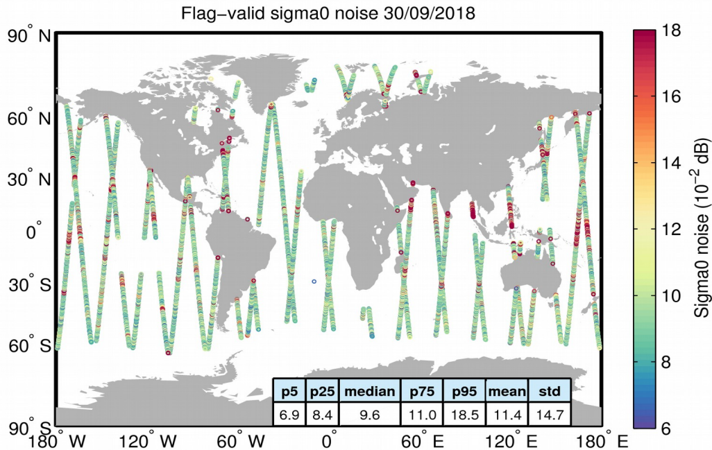
Figure 26. Geographical distribution of flag-valid 20-Hz sigma0 measurement noise over oceans and lakes for 30/09/2018. The statistical values shown in the table refer to the sigma0 noise and are calculated over all measurements shown in the figure.
