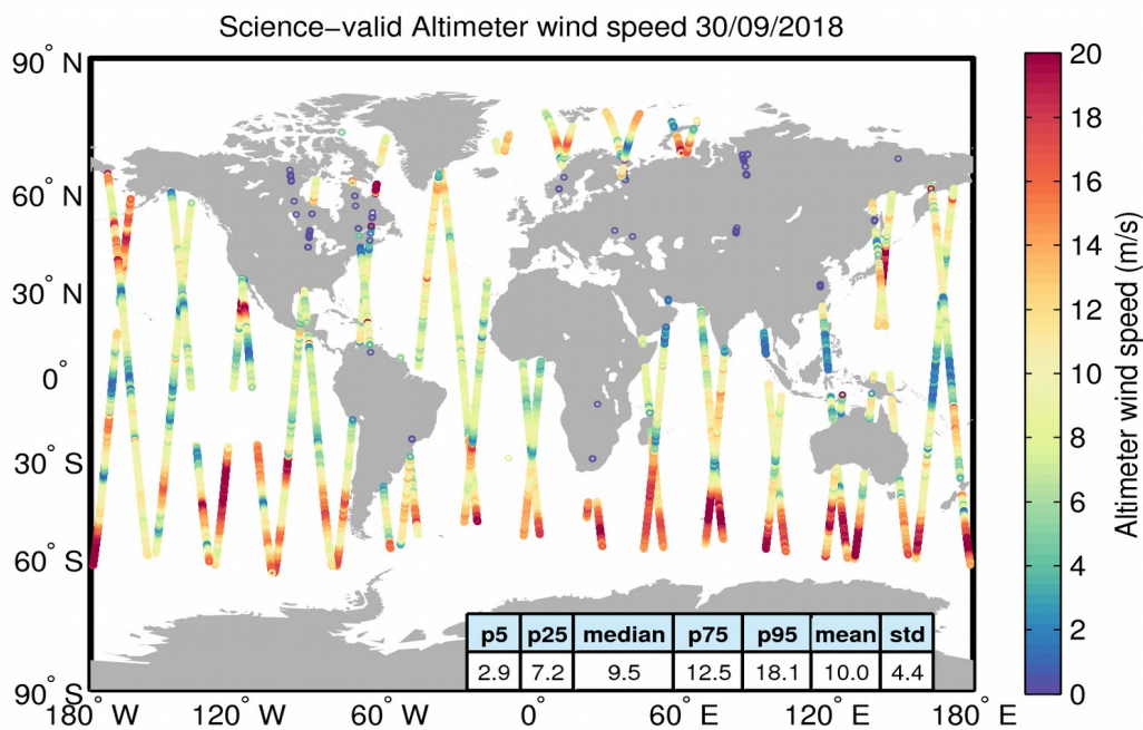
Figure 34. Geographical distribution of science-valid wind data over oceans and lakes for 30/09/2018. The statistical values shown in the table refer to the wind in m/s and are calculated over all measurements shown in the figure. Gray circles denote records that have been rejected based on the editing criteria described in Table 5.
