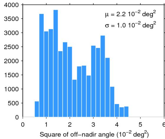
Figure 39. Histogram of flag-valid mispointing over oceans and lakes for 30/09/2018. The mean ( \mu ) and standard deviation ( \sigma ) are also shown. Note that values larger than 6 \cdot 10^{-2} \text{ deg}^2 are excluded from the histogram for the sake of readability but not from the computation of \mu and \sigma .
