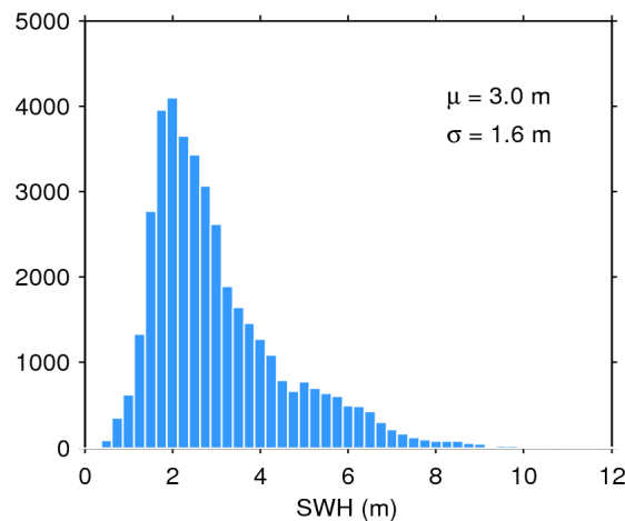
Figure 17. Histogram of flag-valid SWH over oceans and lakes for 30/09/2018. The mean ( \mu ) and standard deviation ( \sigma ) are also shown. Note that values larger than 12 m are excluded from the histogram for the sake of readability but not from the computation of \mu and \sigma .
