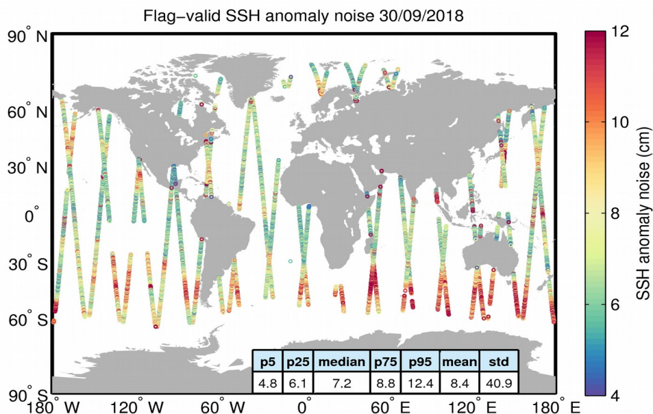
Figure 8. Geographical distribution of flag-valid 20-Hz SSH anomaly measurement noise over oceans and lakes for 30/09/2018. The statistical values shown in the table refer to the SSH anomaly noise and are calculated over all measurements shown in the figure.
