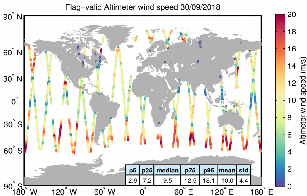
Figure 31. Geographical distribution of flag-valid wind data over oceans and lakes for 30/09/2018. The statistical values shown in the table refer to the wind in m/s and are calculated over all measurements shown in the figure.
