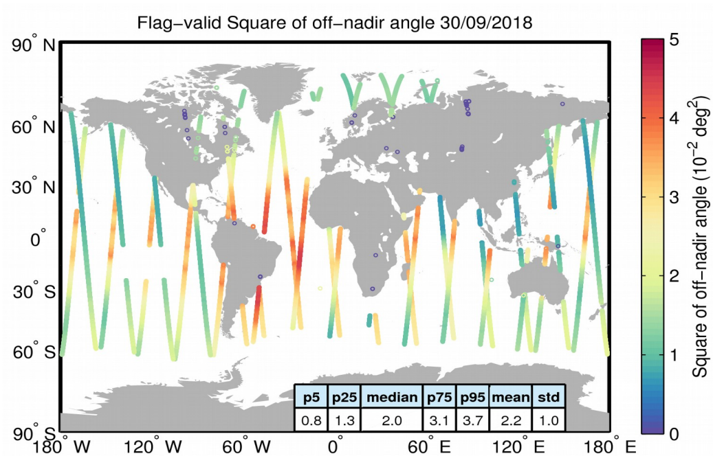
Figure 37. Geographical distribution of flag-valid mispointing data over oceans and lakes for 30/09/2018. The statistical values shown in the table refer to the mispointing in 10^{-2} \text{ deg}^2 and are calculated over all measurements shown in the figure.
