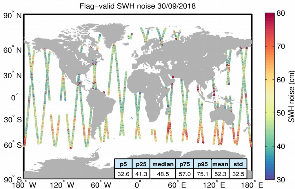
Figure 18. Geographical distribution of flag-valid 20-Hz SWH measurement noise over oceans and lakes for 30/09/2018. The statistical values shown in the figure refer to the SWH noise and are calculated over all measurements shown in the figure.
