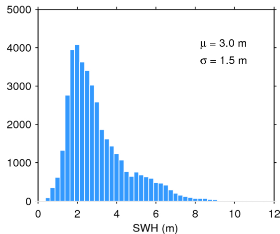
Figure 20. Histogram of science-valid SWH over oceans and lakes for 30/09/2018. The mean ( \mu ) and standard deviation ( \sigma ) are also shown. Note that values larger than 12 m are excluded from the histogram for the sake of readability but not from the computation of \mu and \sigma .
