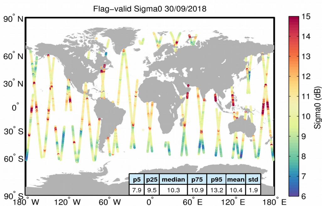
Figure 23. Geographical distribution of flag-valid sigma0 data over oceans and lakes for 30/09/2018. The statistical values shown in the table refer to the sigma0 in dB and are calculated over all measurements shown in the figure.
