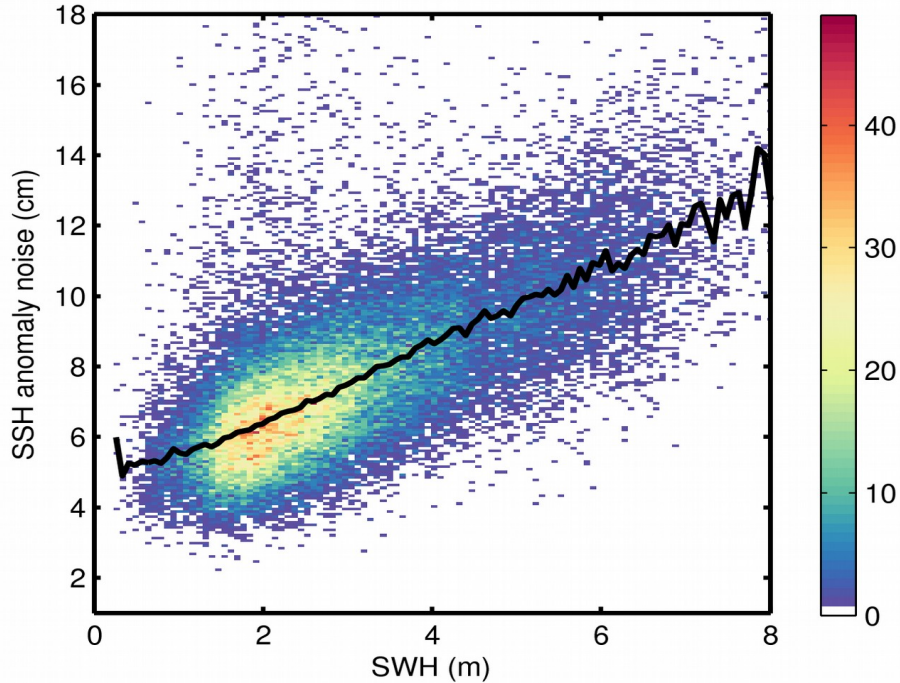
Figure 9. 2D histogram showing flag-valid SSH anomaly noise as a function of SWH for 30/09/2018. The black line denotes the median SSH anomaly noise as a function of SWH.
