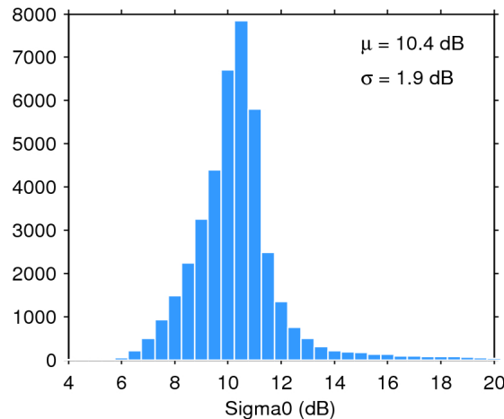
Figure 25. Histogram of flag-valid sigma0 over oceans and lakes for 30/09/2018. The mean ( \mu ) and standard deviation ( \sigma ) are also shown. Note that values outside [4 20] dB are excluded from the histogram for the sake of readability but not from the computation of \mu and \sigma .
