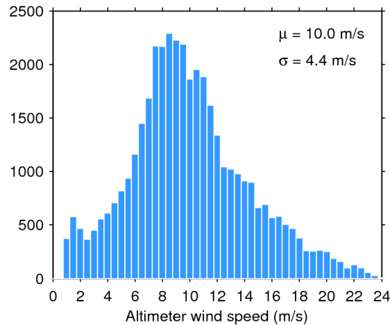
Figure 33. Histogram of flag-valid wind over oceans and lakes for 30/09/2018. The mean ( \mu ) and standard deviation ( \sigma ) are also shown. Note that values larger than 24 m/s are excluded from the histogram for the sake of readability but not from the computation of \mu and \sigma .
