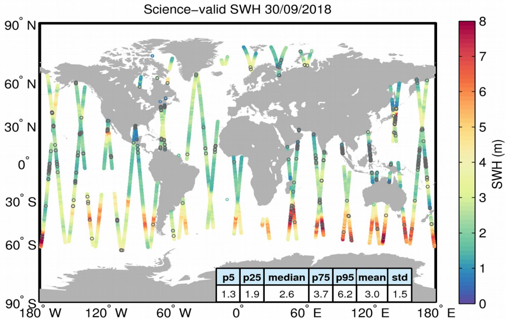
Figure 19. Geographical distribution of science-valid SWH data over oceans and lakes for 30/09/2018. The statistical values shown in the table refer to the SWH in m and are calculated over all measurements shown in the figure. Gray circles denote records that have been rejected based on the editing criteria described in Table 3.
