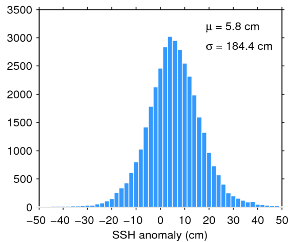
Figure 7. Histogram of flag-valid SSH anomaly over oceans and lakes for 30/09/2018. The mean ( \mu ) and standard deviation ( \sigma ) are also shown. Note that values outside [-50 50] cm are excluded from the histogram for the sake of readability but not from the computation of \mu and \sigma .
