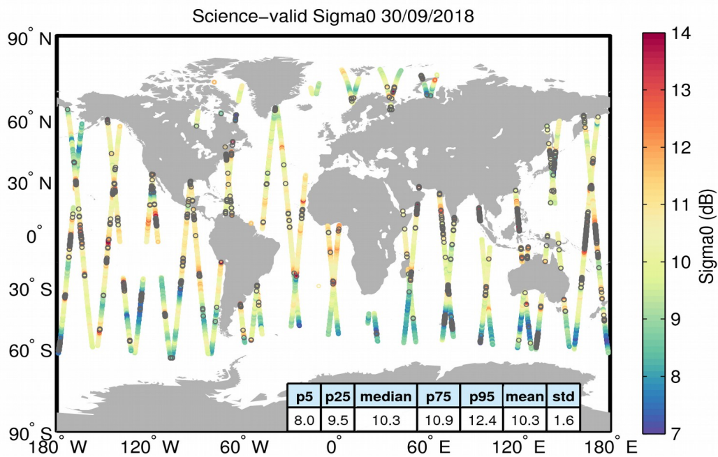
Figure 27. Geographical distribution of science-valid sigma0 data over oceans and lakes for 30/09/2018. The statistical values shown in the table refer to the sigma0 in dB and are calculated over all measurements shown in the figure. Gray circles denote records that have been rejected based on the editing criteria described in Table 4.
