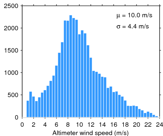
Figure 35. Histogram of science-valid wind over oceans and lakes for 30/09/2018. The mean ( \mu ) and standard deviation ( \sigma ) are also shown. Note that values larger than 24 m/s are excluded from the histogram for the sake of readability but not from the computation of \mu and \sigma .
