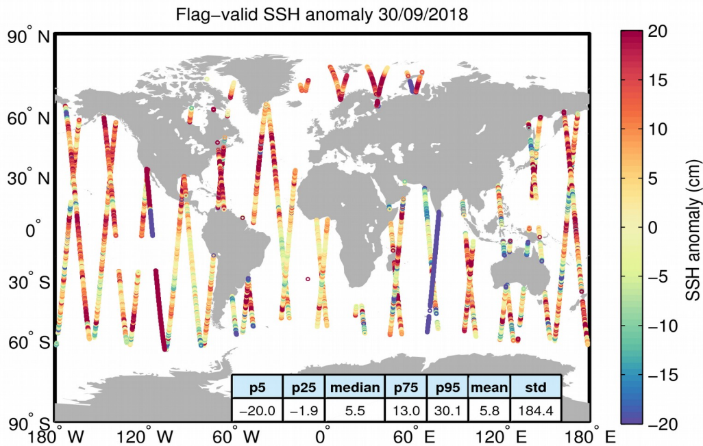
Figure 5. Geographical distribution of flag-valid 1-Hz SSH anomaly data over oceans and lakes for 30/09/2018. The statistical values shown in the table refer to the SSH anomaly in cm and are calculated over all measurements shown in the figure.
