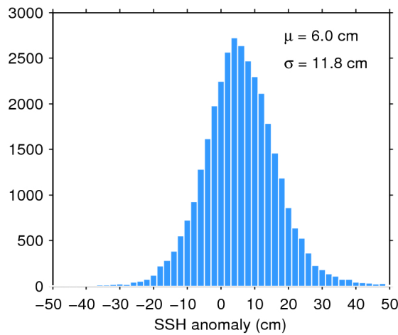
Figure 11. Histogram of science-valid SSH anomaly over oceans and lakes for 30/09/2018. The mean ( \mu ) and standard deviation ( \sigma ) are also shown. Note that values outside [-50 50] cm are excluded from the histogram for the sake of readability but not from the computation of \mu and \sigma .
