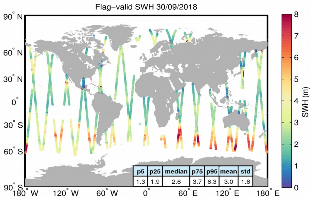
Figure 15. Geographical distribution of flag-valid SWH data over oceans and lakes for 30/09/2018. The statistical values shown in the table refer to the SWH in m and are calculated over all measurements shown in the figure.
