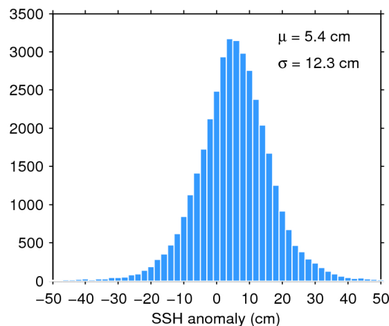
Figure 11. Histogram of science-valid SSH anomaly over oceans and lakes for 15/09/2018. The mean ( \mu ) and standard deviation ( \sigma ) are also shown. Note that values outside [-50 50] cm are excluded from the histogram for the sake of readability but not from the computation of \mu and \sigma .
