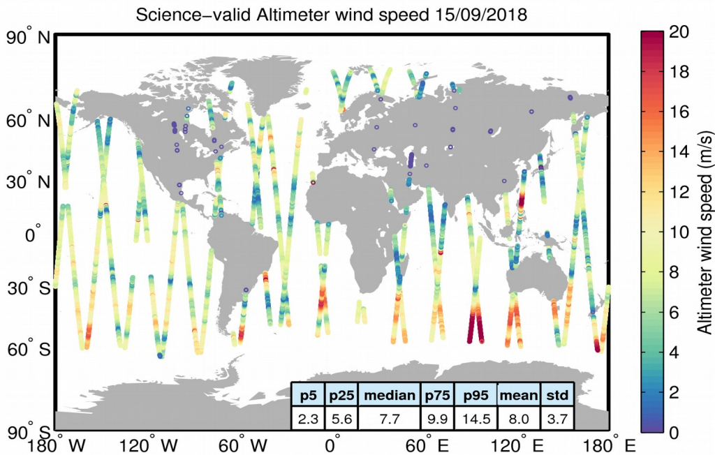
Figure 34. Geographical distribution of science-valid wind data over oceans and lakes for 15/09/2018. The statistical values shown in the table refer to the wind in m/s and are calculated over all measurements shown in the figure. Gray circles denote records that have been rejected based on the editing criteria described in Table 5.
