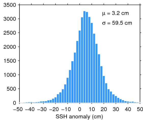
Figure 7. Histogram of flag-valid SSH anomaly over oceans and lakes for 15/09/2018. The mean ( \mu ) and standard deviation ( \sigma ) are also shown. Note that values outside [-50\ 50] cm are excluded from the histogram for the sake of readability but not from the computation of \mu and \sigma .
