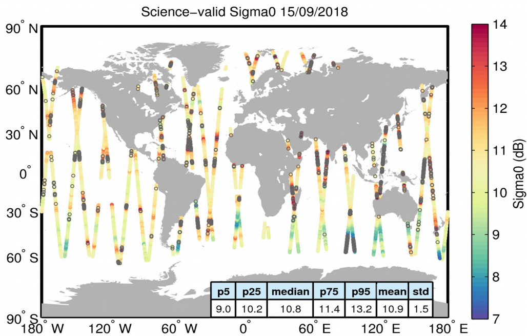
Figure 27. Geographical distribution of science-valid sigma0 data over oceans and lakes for 15/09/2018. The statistical values shown in the table refer to the sigma0 in dB and are calculated over all measurements shown in the figure. Gray circles denote records that have been rejected based on the editing criteria described in Table 4.
