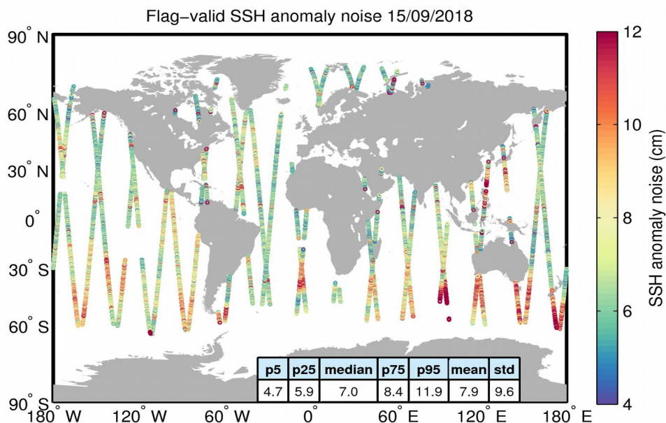
Figure 8. Geographical distribution of flag-valid 20-Hz SSH anomaly measurement noise over oceans and lakes for 15/09/2018. The statistical values shown in the table refer to the SSH anomaly noise and are calculated over all measurements shown in the figure.
