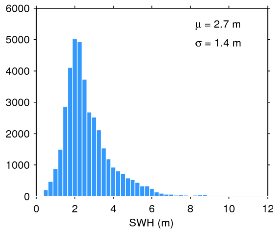
Figure 20. Histogram of science-valid SWH over oceans and lakes for 15/09/2018. The mean ( \mu ) and standard deviation ( \sigma ) are also shown. Note that values larger than 12 m are excluded from the histogram for the sake of readability but not from the computation of \mu and \sigma .
