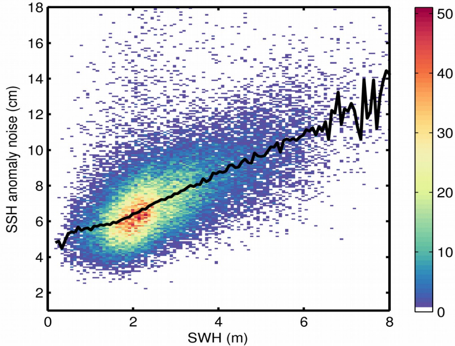
Figure 9. 2D histogram showing flag-valid SSH anomaly noise as a function of SWH for 15/09/2018. The black line denotes the median SSH anomaly noise as a function of SWH.
