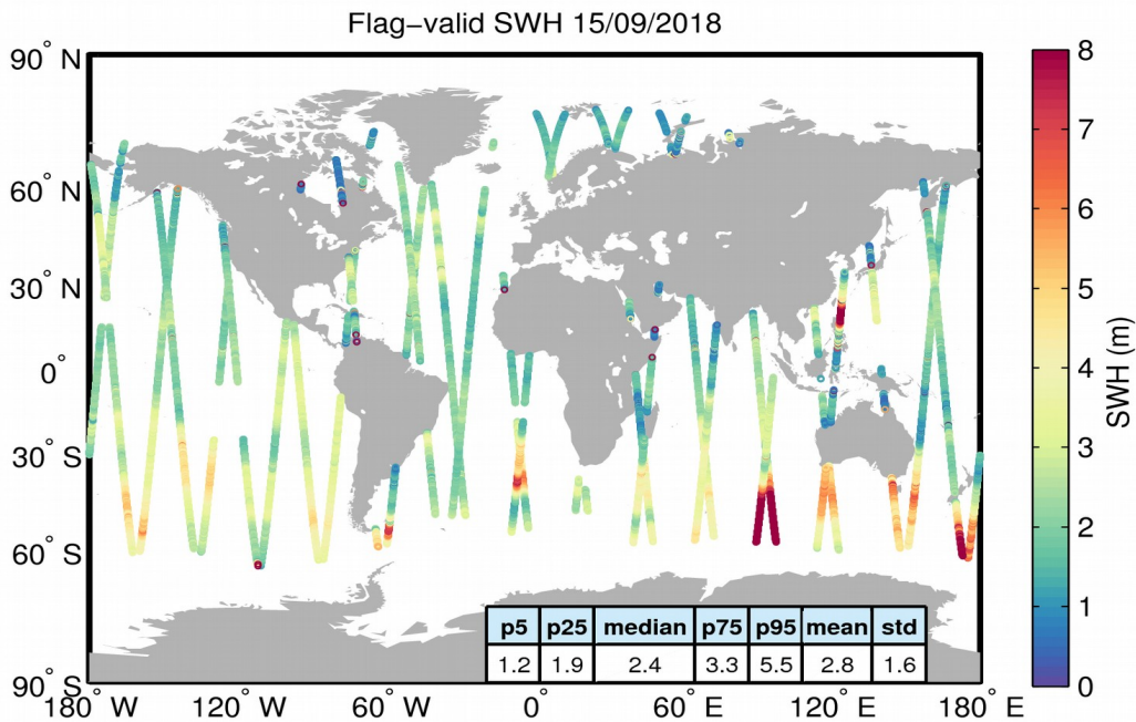
Figure 15. Geographical distribution of flag-valid SWH data over oceans and lakes for 15/09/2018. The statistical values shown in the table refer to the SWH in m and are calculated over all measurements shown in the figure.
