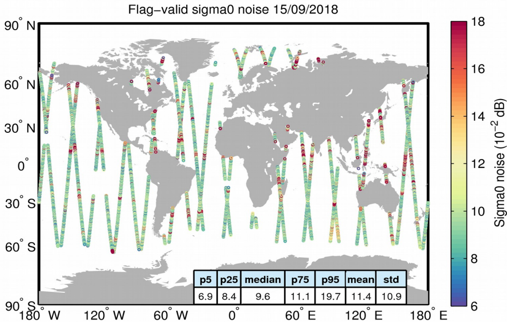
Figure 26. Geographical distribution of flag-valid 20-Hz sigma0 measurement noise over oceans and lakes for 15/09/2018. The statistical values shown in the table refer to the sigma0 noise and are calculated over all measurements shown in the figure.
