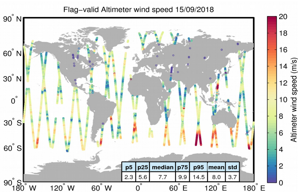
Figure 31. Geographical distribution of flag-valid wind data over oceans and lakes for 15/09/2018. The statistical values shown in the table refer to the wind in m/s and are calculated over all measurements shown in the figure.
