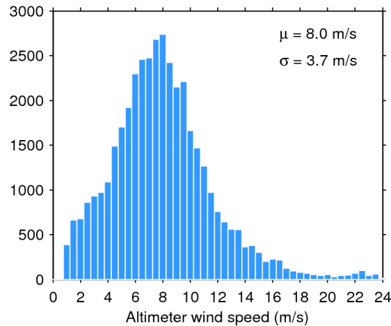
Figure 33. Histogram of flag-valid wind over oceans and lakes for 15/09/2018. The mean ( \mu ) and standard deviation ( \sigma ) are also shown. Note that values larger than 24 m/s are excluded from the histogram for the sake of readability but not from the computation of \mu and \sigma .
