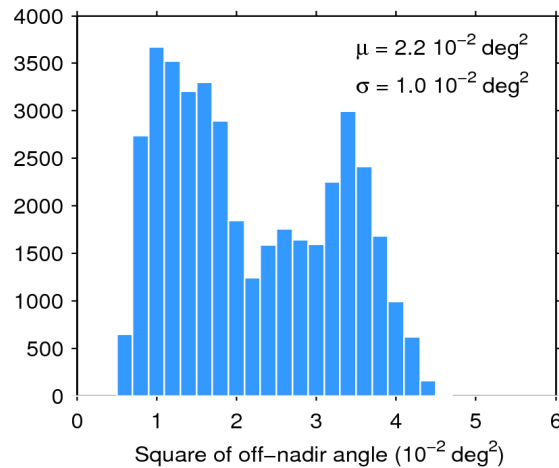
Figure 39. Histogram of flag-valid mispointing over oceans and lakes for 15/09/2018. The mean ( \mu ) and standard deviation ( \sigma ) are also shown. Note that values larger than 6 \cdot 10^{-2} \text{ deg}^2 are excluded from the histogram for the sake of readability but not from the computation of \mu and \sigma .
