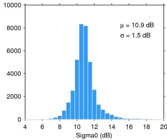
Figure 28. Histogram of science-valid sigma0 over oceans and lakes for 15/09/2018. The mean ( \mu ) and standard deviation ( \sigma ) are also shown. Note that values outside [4 20] dB are excluded from the histogram for the sake of readability but not from the computation of \mu and \sigma .
