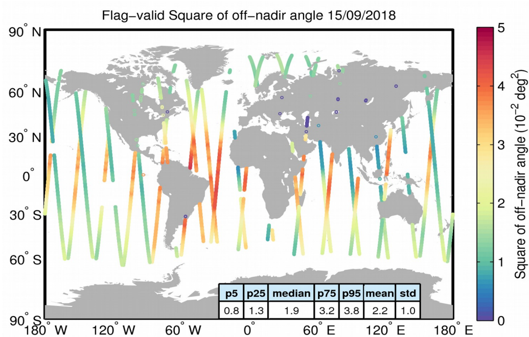
Figure 37. Geographical distribution of flag-valid mispointing data over oceans and lakes for 15/09/2018. The statistical values shown in the table refer to the mispointing in 10^{-2} \text{ deg}^2 and are calculated over all measurements shown in the figure.
