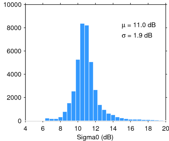
Figure 25. Histogram of flag-valid sigma0 over oceans and lakes for 15/09/2018. The mean ( \mu ) and standard deviation ( \sigma ) are also shown. Note that values outside [4 20] dB are excluded from the histogram for the sake of readability but not from the computation of \mu and \sigma .
