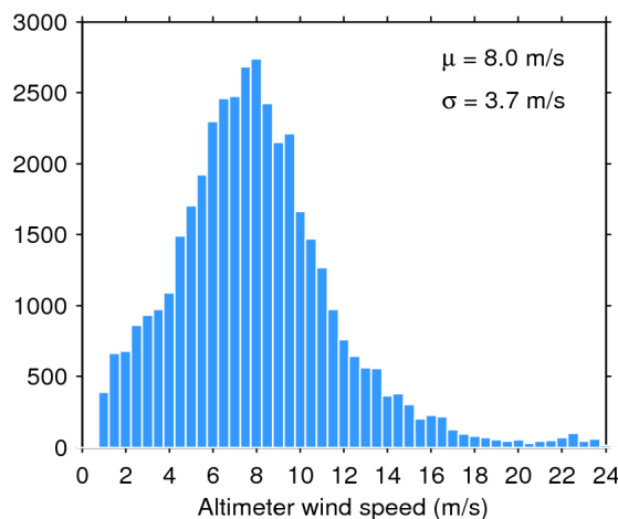
Figure 35. Histogram of science-valid wind over oceans and lakes for 15/09/2018. The mean ( \mu ) and standard deviation ( \sigma ) are also shown. Note that values larger than 24 m/s are excluded from the histogram for the sake of readability but not from the computation of \mu and \sigma .
