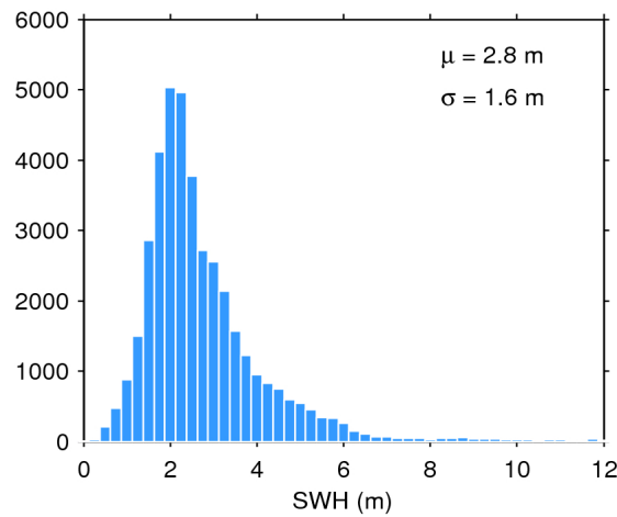
Figure 17. Histogram of flag-valid SWH over oceans and lakes for 15/09/2018. The mean ( \mu ) and standard deviation ( \sigma ) are also shown. Note that values larger than 12 m are excluded from the histogram for the sake of readability but not from the computation of \mu and \sigma .
