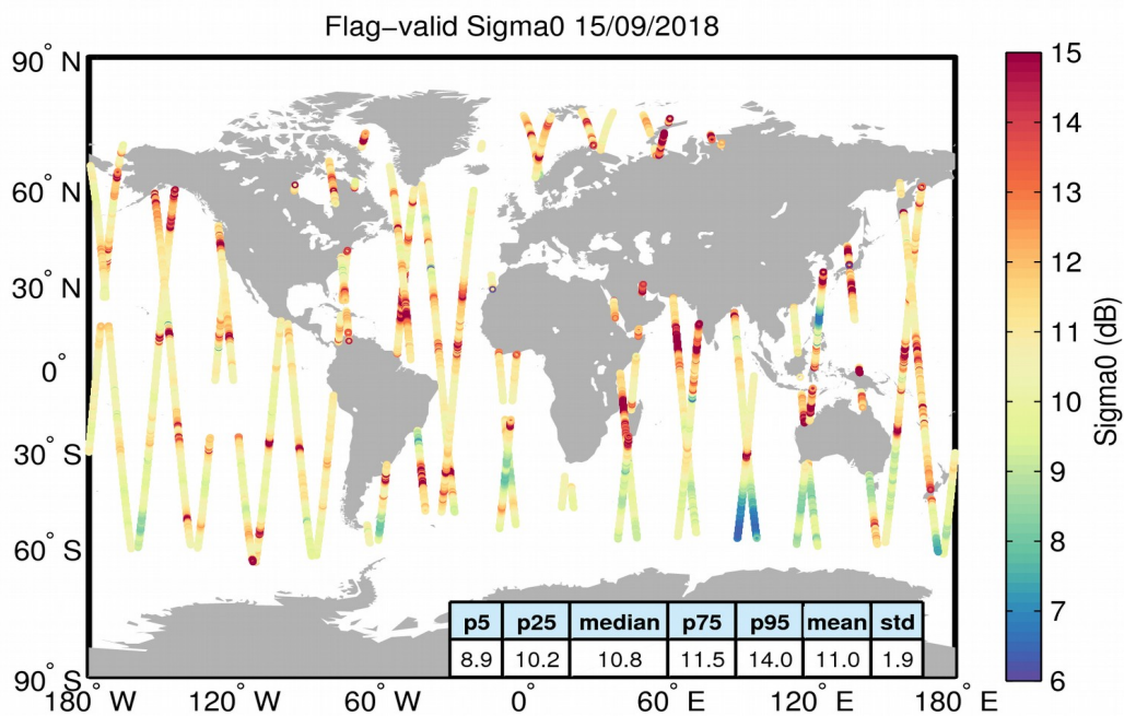
Figure 23. Geographical distribution of flag-valid sigma0 data over oceans and lakes for 15/09/2018. The statistical values shown in the table refer to the sigma0 in dB and are calculated over all measurements shown in the figure.
