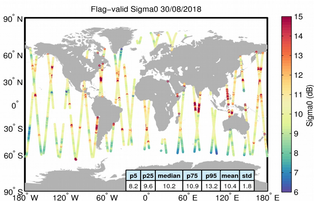
Figure 23. Geographical distribution of flag-valid sigma0 data over oceans and lakes for 30/08/2018. The statistical values shown in the table refer to the sigma0 in dB and are calculated over all measurements shown in the figure.
