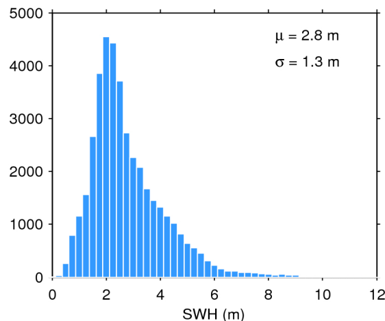
Figure 20. Histogram of science-valid SWH over oceans and lakes for 30/08/2018. The mean ( \mu ) and standard deviation ( \sigma ) are also shown. Note that values larger than 12 m are excluded from the histogram for the sake of readability but not from the computation of \mu and \sigma .
