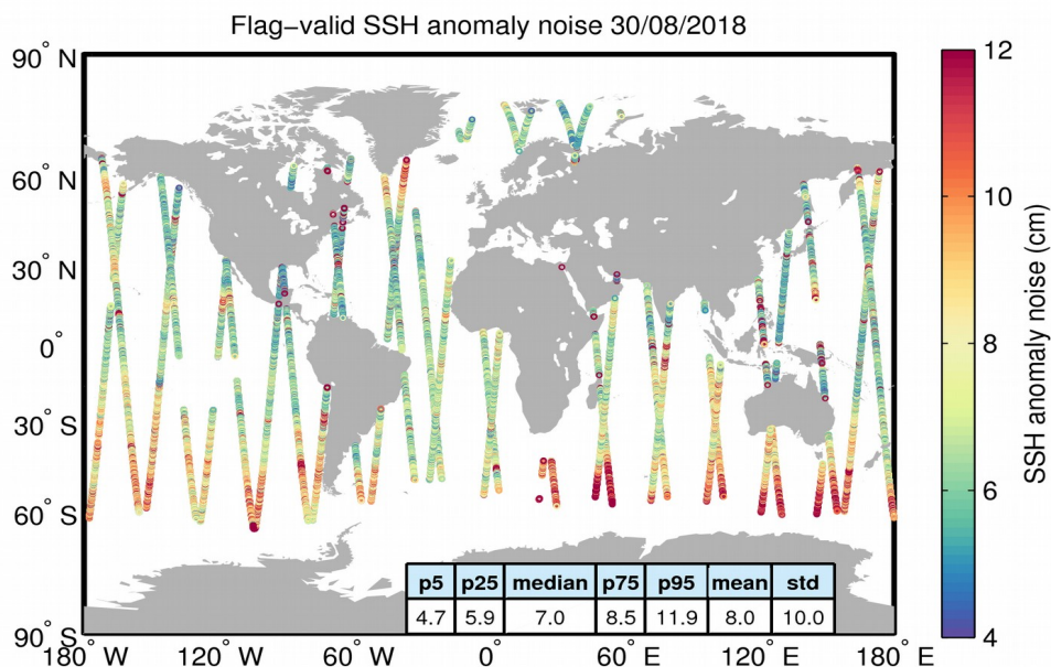
Figure 8. Geographical distribution of flag-valid 20-Hz SSH anomaly measurement noise over oceans and lakes for 30/08/2018. The statistical values shown in the table refer to the SSH anomaly noise and are calculated over all measurements shown in the figure.
