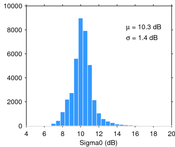
Figure 28. Histogram of science-valid sigma0 over oceans and lakes for 30/08/2018. The mean ( \mu ) and standard deviation ( \sigma ) are also shown. Note that values outside [4 20] dB are excluded from the histogram for the sake of readability but not from the computation of \mu and \sigma .
