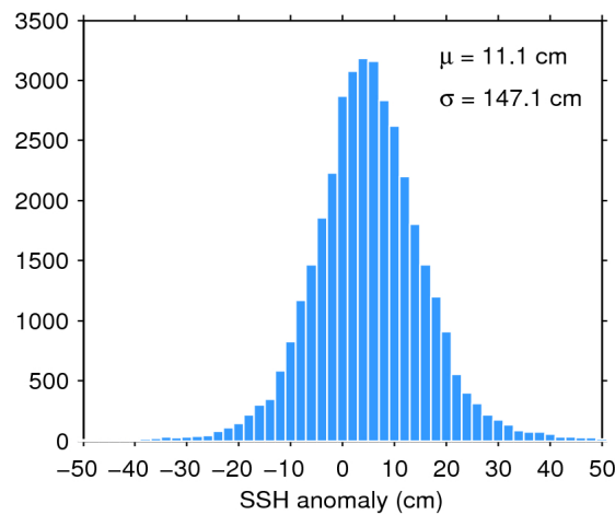
Figure 7. Histogram of flag-valid SSH anomaly over oceans and lakes for 30/08/2018. The mean ( \mu ) and standard deviation ( \sigma ) are also shown. Note that values outside [-50\ 50] cm are excluded from the histogram for the sake of readability but not from the computation of \mu and \sigma .
