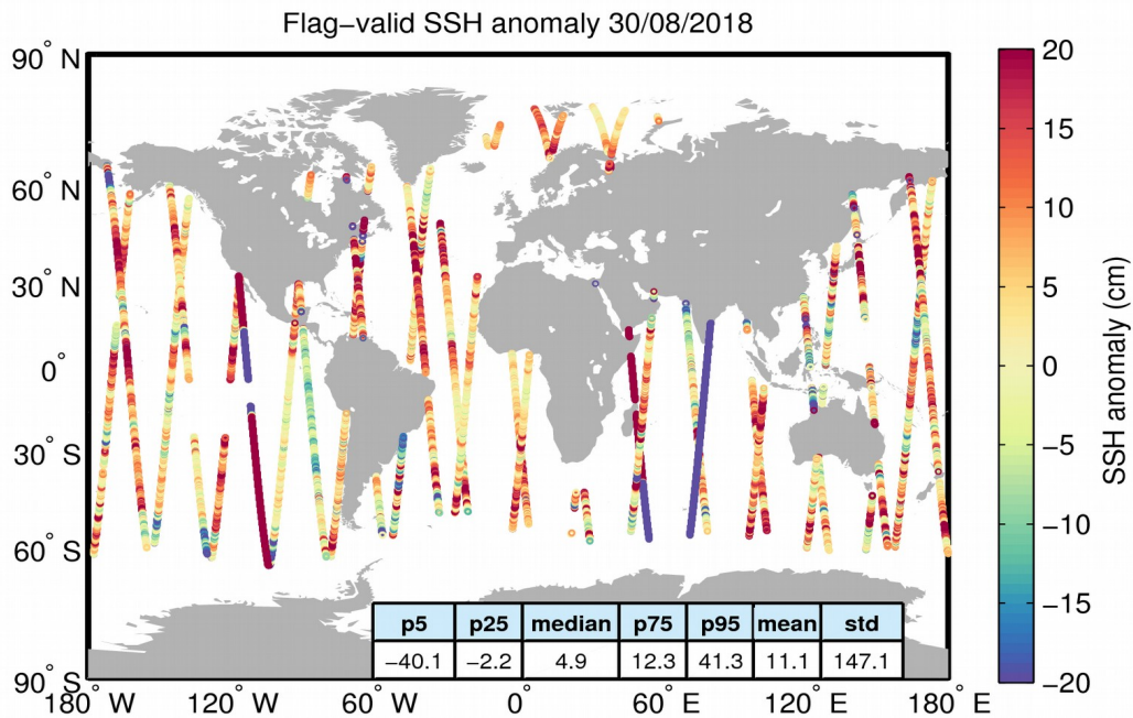
Figure 5. Geographical distribution of flag-valid 1-Hz SSH anomaly data over oceans and lakes for 30/08/2018. The statistical values shown in the table refer to the SSH anomaly in cm and are calculated over all measurements shown in the figure.
