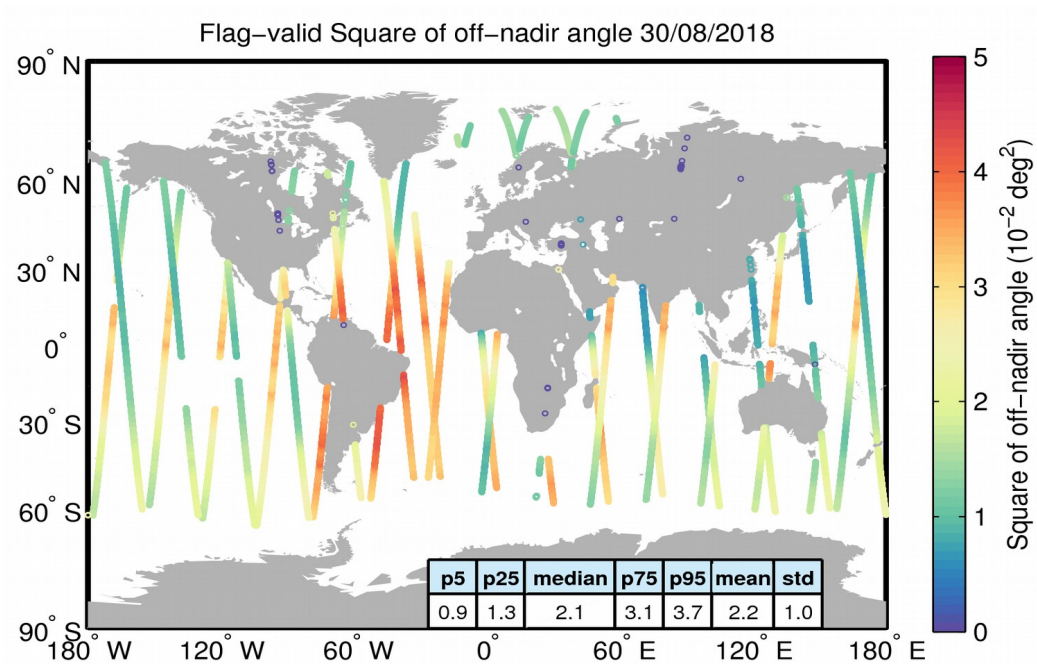
Figure 37. Geographical distribution of flag-valid mispointing data over oceans and lakes for 30/08/2018. The statistical values shown in the table refer to the mispointing in 10^{-2} \text{ deg}^2 and are calculated over all measurements shown in the figure.
