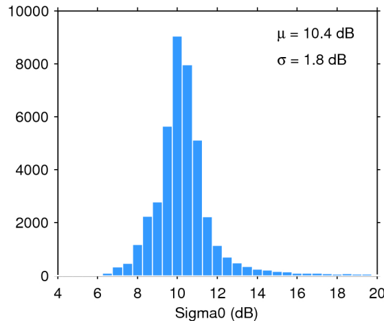
Figure 25. Histogram of flag-valid sigma0 over oceans and lakes for 30/08/2018. The mean ( \mu ) and standard deviation ( \sigma ) are also shown. Note that values outside [4 20] dB are excluded from the histogram for the sake of readability but not from the computation of \mu and \sigma .
