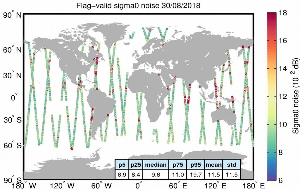
Figure 26. Geographical distribution of flag-valid 20-Hz sigma0 measurement noise over oceans and lakes for 30/08/2018. The statistical values shown in the table refer to the sigma0 noise and are calculated over all measurements shown in the figure.
