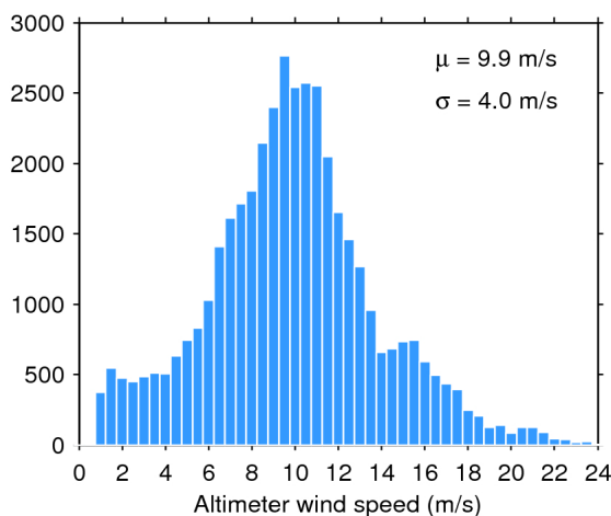
Figure 33. Histogram of flag-valid wind over oceans and lakes for 30/08/2018. The mean ( \mu ) and standard deviation ( \sigma ) are also shown. Note that values larger than 24 m/s are excluded from the histogram for the sake of readability but not from the computation of \mu and \sigma .
