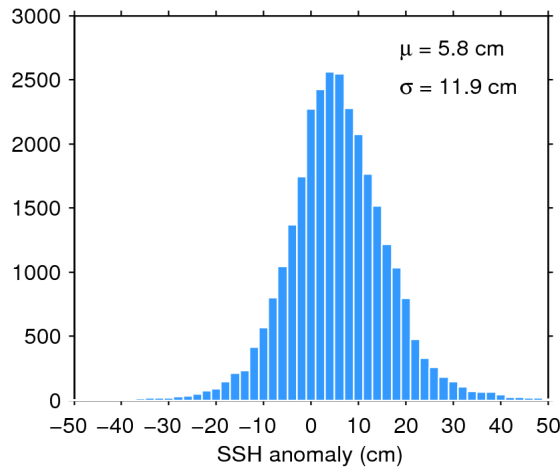
Figure 11. Histogram of science-valid SSH anomaly over oceans and lakes for 30/08/2018. The mean ( \mu ) and standard deviation ( \sigma ) are also shown. Note that values outside [-50 50] cm are excluded from the histogram for the sake of readability but not from the computation of \mu and \sigma .
