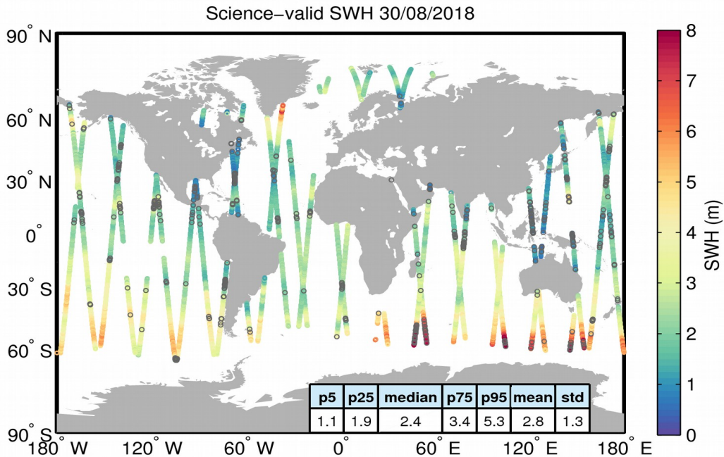
Figure 19. Geographical distribution of science-valid SWH data over oceans and lakes for 30/08/2018. The statistical values shown in the table refer to the SWH in m and are calculated over all measurements shown in the figure. Gray circles denote records that have been rejected based on the editing criteria described in Table 3.
