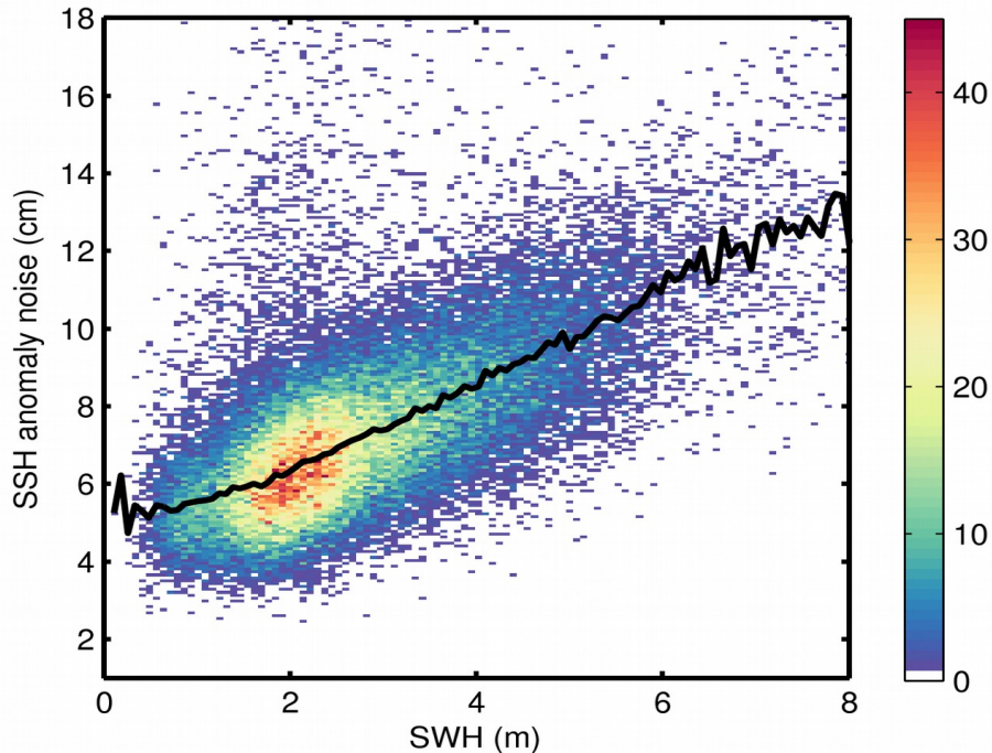
Figure 9. 2D histogram showing flag-valid SSH anomaly noise as a function of SWH for 30/08/2018. The black line denotes the median SSH anomaly noise as a function of SWH.
