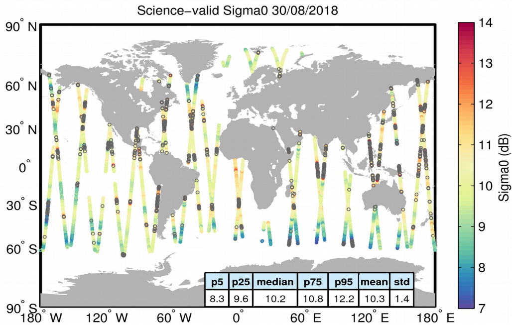
Figure 27. Geographical distribution of science-valid sigma0 data over oceans and lakes for 30/08/2018. The statistical values shown in the table refer to the sigma0 in dB and are calculated over all measurements shown in the figure. Gray circles denote records that have been rejected based on the editing criteria described in Table 4.
