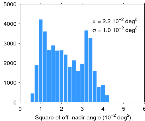
Figure 39. Histogram of flag-valid mispointing over oceans and lakes for 30/08/2018. The mean ( \mu ) and standard deviation ( \sigma ) are also shown. Note that values larger than 6 \cdot 10^{-2} \text{ deg}^2 are excluded from the histogram for the sake of readability but not from the computation of \mu and \sigma .
