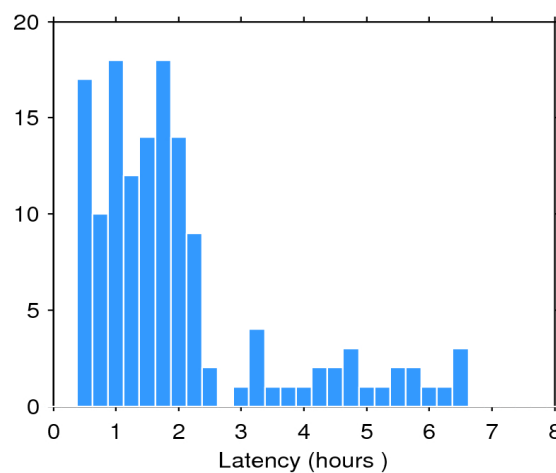
Figure 2. Histogram of the data latency for 30/08/2018. The y-axis denotes the number of files that are made available with a delay of x-hours with respect to the mean time of the records stored in the file.
