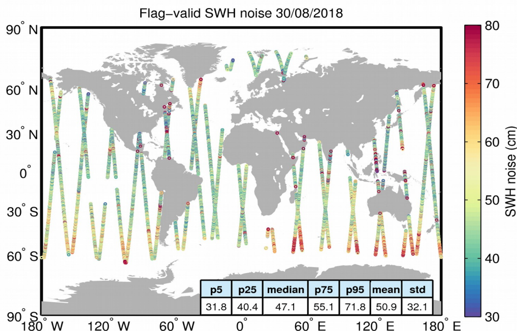
Figure 18. Geographical distribution of flag-valid 20-Hz SWH measurement noise over oceans and lakes for 30/08/2018. The statistical values shown in the figure refer to the SWH noise and are calculated over all measurements shown in the figure.
