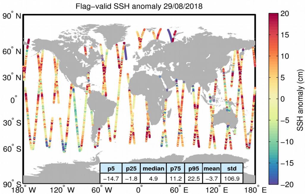
Figure 5. Geographical distribution of flag-valid 1-Hz SSH anomaly data over oceans and lakes for 29/08/2018. The statistical values shown in the table refer to the SSH anomaly in cm and are calculated over all measurements shown in the figure.
