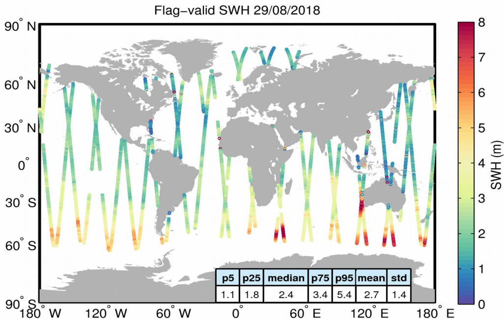
Figure 15. Geographical distribution of flag-valid SWH data over oceans and lakes for 29/08/2018. The statistical values shown in the table refer to the SWH in m and are calculated over all measurements shown in the figure.
