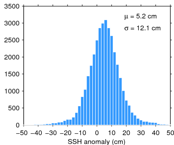
Figure 11. Histogram of science-valid SSH anomaly over oceans and lakes for 29/08/2018. The mean ( \mu ) and standard deviation ( \sigma ) are also shown. Note that values outside [-50 50] cm are excluded from the histogram for the sake of readability but not from the computation of \mu and \sigma .
