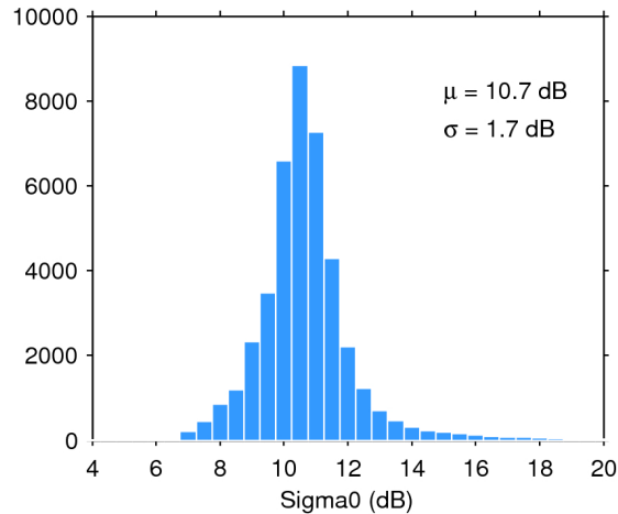
Figure 25. Histogram of flag-valid sigma0 over oceans and lakes for 29/08/2018. The mean ( \mu ) and standard deviation ( \sigma ) are also shown. Note that values outside [4 20] dB are excluded from the histogram for the sake of readability but not from the computation of \mu and \sigma .
