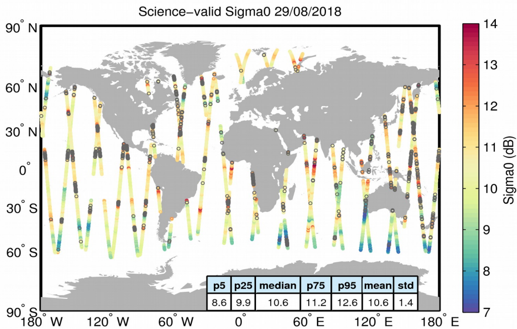
Figure 27. Geographical distribution of science-valid sigma0 data over oceans and lakes for 29/08/2018. The statistical values shown in the table refer to the sigma0 in dB and are calculated over all measurements shown in the figure. Gray circles denote records that have been rejected based on the editing criteria described in Table 4.
