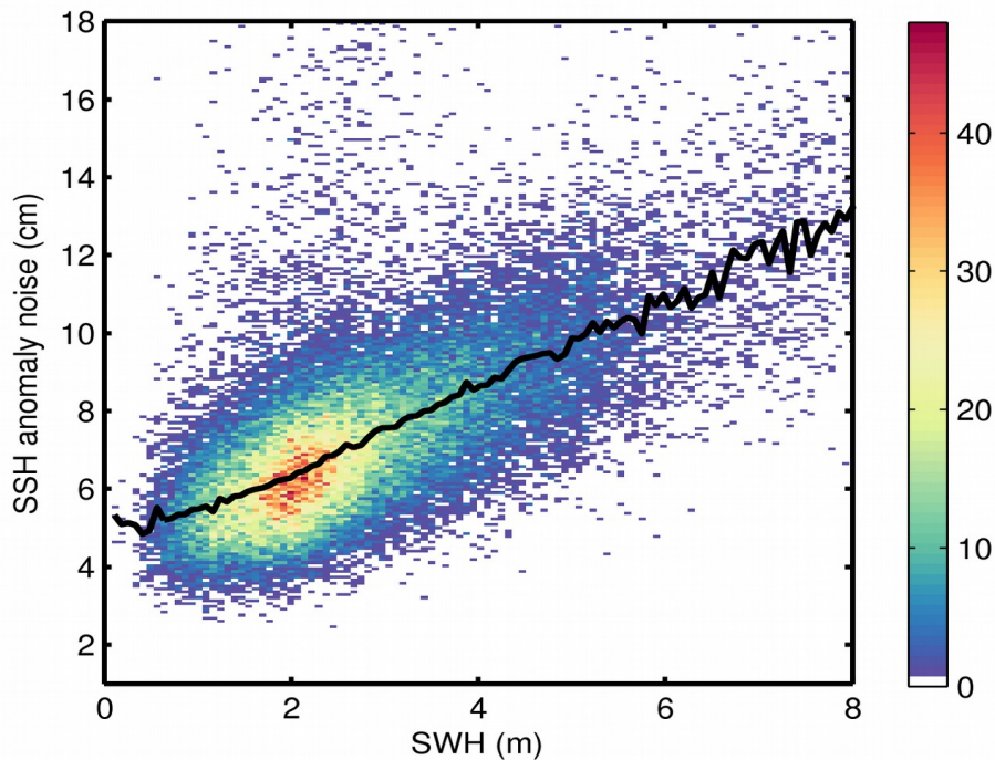
Figure 9. 2D histogram showing flag-valid SSH anomaly noise as a function of SWH for 29/08/2018. The black line denotes the median SSH anomaly noise as a function of SWH.
