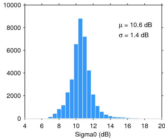
Figure 28. Histogram of science-valid sigma0 over oceans and lakes for 29/08/2018. The mean ( \mu ) and standard deviation ( \sigma ) are also shown. Note that values outside [4 20] dB are excluded from the histogram for the sake of readability but not from the computation of \mu and \sigma .
