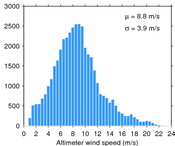
Figure 35. Histogram of science-valid wind over oceans and lakes for 29/08/2018. The mean ( \mu ) and standard deviation ( \sigma ) are also shown. Note that values larger than 24 m/s are excluded from the histogram for the sake of readability but not from the computation of \mu and \sigma .
