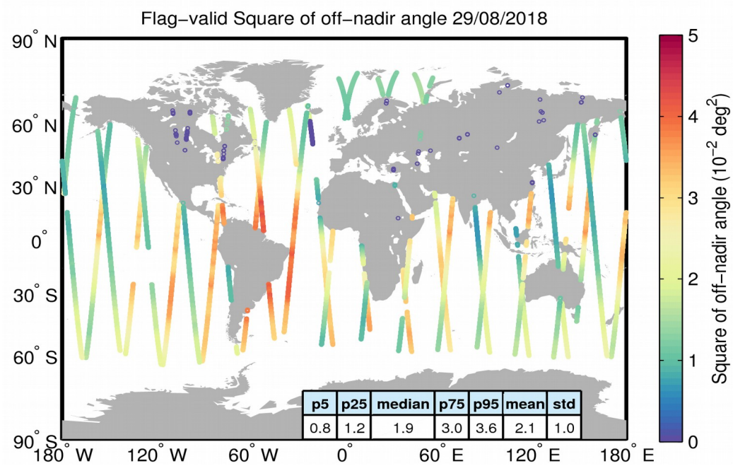
Figure 37. Geographical distribution of flag-valid mispointing data over oceans and lakes for 29/08/2018. The statistical values shown in the table refer to the mispointing in 10^{-2} \text{ deg}^2 and are calculated over all measurements shown in the figure.
