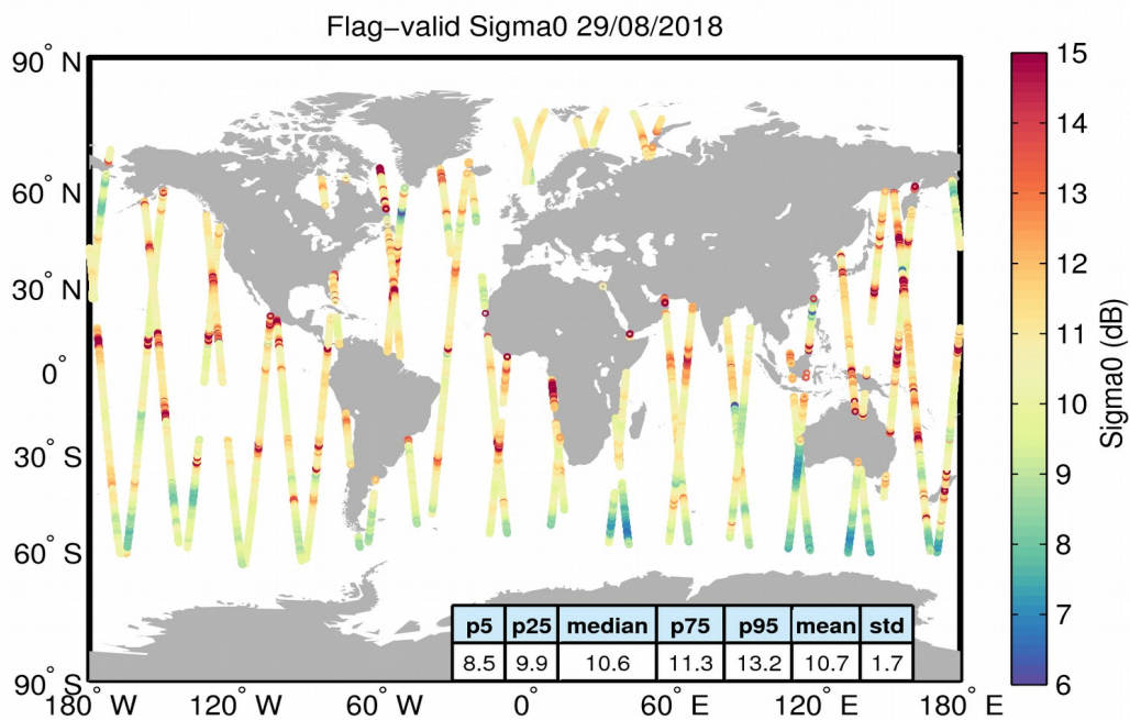
Figure 23. Geographical distribution of flag-valid sigma0 data over oceans and lakes for 29/08/2018. The statistical values shown in the table refer to the sigma0 in dB and are calculated over all measurements shown in the figure.
