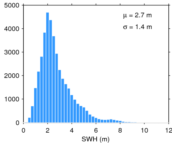
Figure 20. Histogram of science-valid SWH over oceans and lakes for 29/08/2018. The mean ( \mu ) and standard deviation ( \sigma ) are also shown. Note that values larger than 12 m are excluded from the histogram for the sake of readability but not from the computation of \mu and \sigma .
