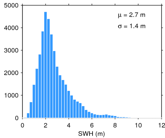
Figure 17. Histogram of flag-valid SWH over oceans and lakes for 29/08/2018. The mean ( \mu ) and standard deviation ( \sigma ) are also shown. Note that values larger than 12 m are excluded from the histogram for the sake of readability but not from the computation of \mu and \sigma .
