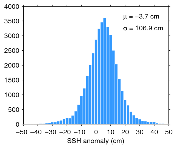
Figure 7. Histogram of flag-valid SSH anomaly over oceans and lakes for 29/08/2018. The mean ( \mu ) and standard deviation ( \sigma ) are also shown. Note that values outside [-50\ 50] cm are excluded from the histogram for the sake of readability but not from the computation of \mu and \sigma .
