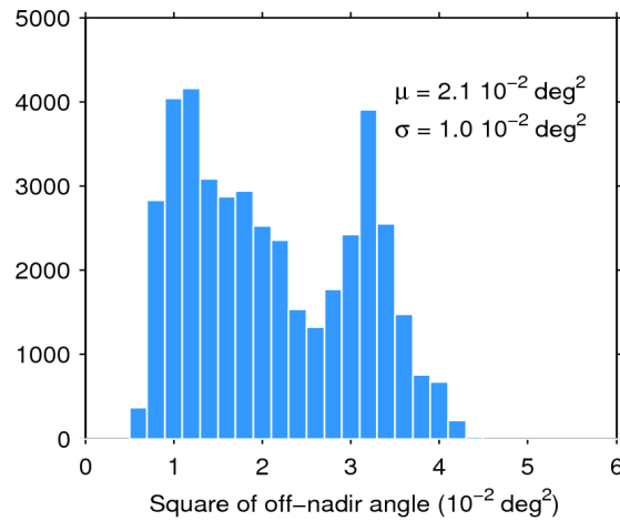
Figure 39. Histogram of flag-valid mispointing over oceans and lakes for 29/08/2018. The mean ( \mu ) and standard deviation ( \sigma ) are also shown. Note that values larger than 6 \cdot 10^{-2} \text{ deg}^2 are excluded from the histogram for the sake of readability but not from the computation of \mu and \sigma .
