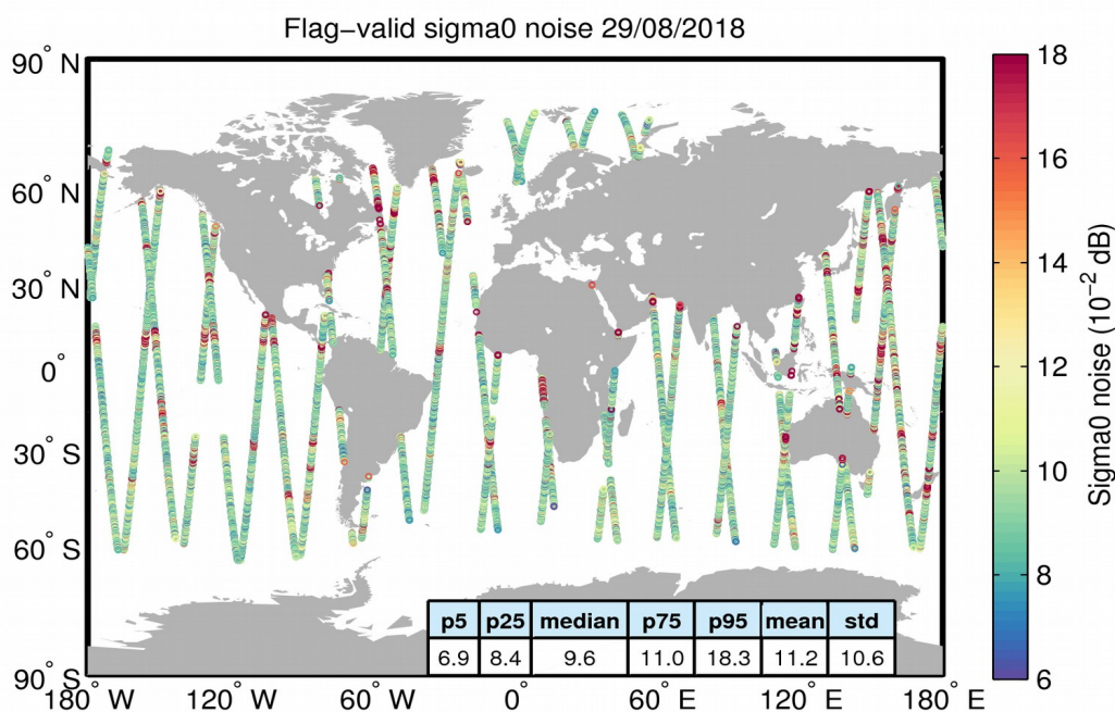
Figure 26. Geographical distribution of flag-valid 20-Hz sigma0 measurement noise over oceans and lakes for 29/08/2018. The statistical values shown in the table refer to the sigma0 noise and are calculated over all measurements shown in the figure.
