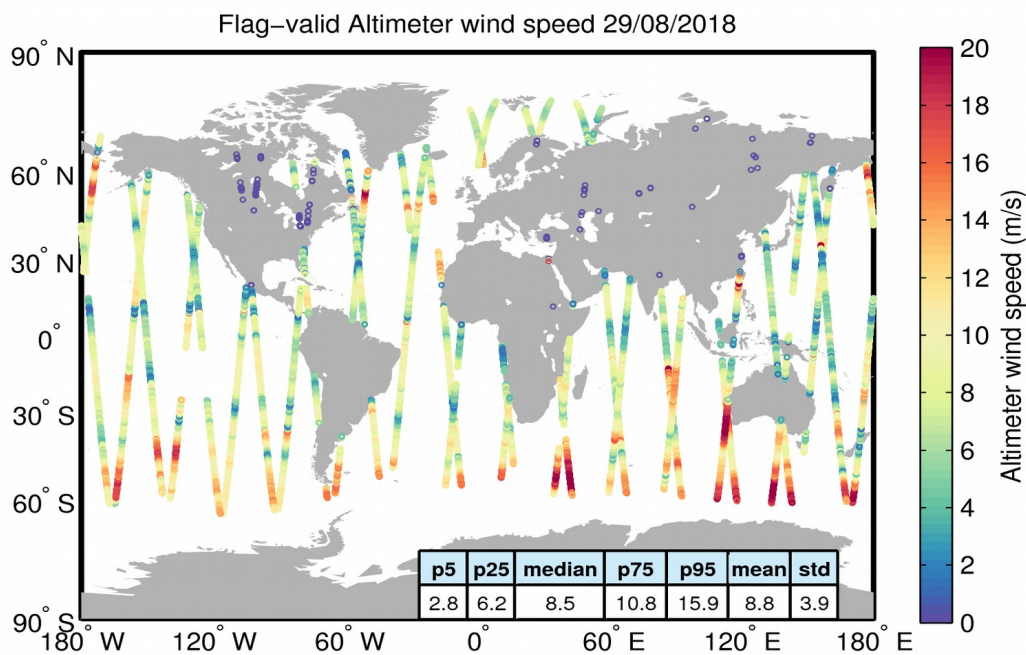
Figure 31. Geographical distribution of flag-valid wind data over oceans and lakes for 29/08/2018. The statistical values shown in the table refer to the wind in m/s and are calculated over all measurements shown in the figure.
