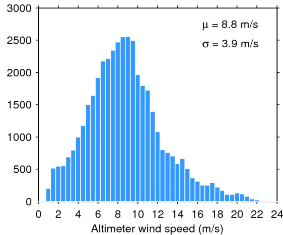
Figure 33. Histogram of flag-valid wind over oceans and lakes for 29/08/2018. The mean ( \mu ) and standard deviation ( \sigma ) are also shown. Note that values larger than 24 m/s are excluded from the histogram for the sake of readability but not from the computation of \mu and \sigma .
