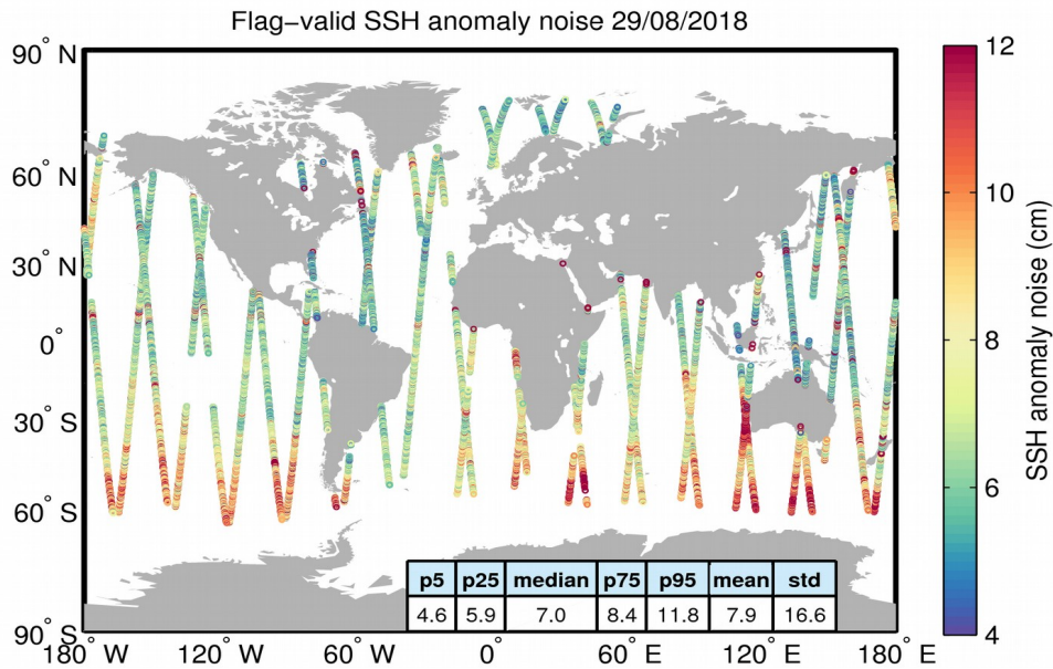
Figure 8. Geographical distribution of flag-valid 20-Hz SSH anomaly measurement noise over oceans and lakes for 29/08/2018. The statistical values shown in the table refer to the SSH anomaly noise and are calculated over all measurements shown in the figure.
