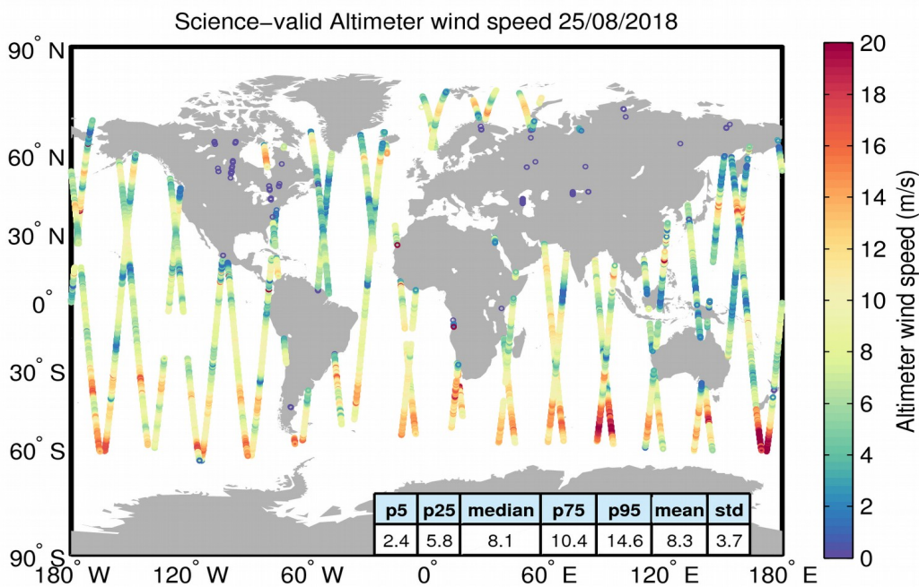
Figure 34. Geographical distribution of science-valid wind data over oceans and lakes for 25/08/2018. The statistical values shown in the table refer to the wind in m/s and are calculated over all measurements shown in the figure. Gray circles denote records that have been rejected based on the editing criteria described in Table 5.
