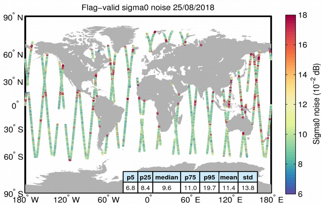
Figure 26. Geographical distribution of flag-valid 20-Hz sigma0 measurement noise over oceans and lakes for 25/08/2018. The statistical values shown in the table refer to the sigma0 noise and are calculated over all measurements shown in the figure.
