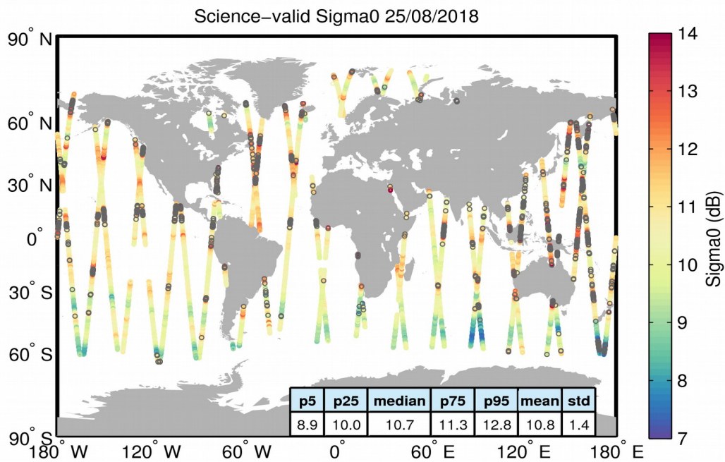
Figure 27. Geographical distribution of science-valid sigma0 data over oceans and lakes for 25/08/2018. The statistical values shown in the table refer to the sigma0 in dB and are calculated over all measurements shown in the figure. Gray circles denote records that have been rejected based on the editing criteria described in Table 4.
