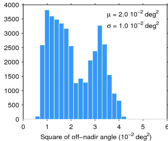
Figure 39. Histogram of flag-valid mispointing over oceans and lakes for 25/08/2018. The mean ( \mu ) and standard deviation ( \sigma ) are also shown. Note that values larger than 6 \cdot 10^{-2} \text{ deg}^2 are excluded from the histogram for the sake of readability but not from the computation of \mu and \sigma .
