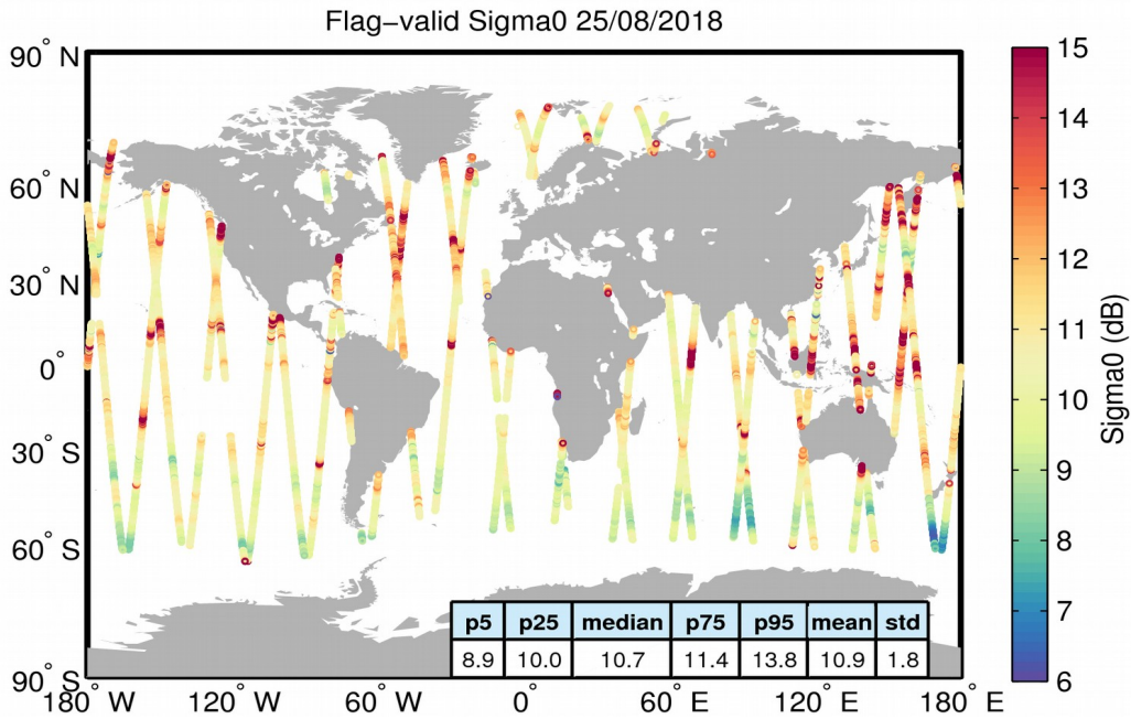
Figure 23. Geographical distribution of flag-valid sigma0 data over oceans and lakes for 25/08/2018. The statistical values shown in the table refer to the sigma0 in dB and are calculated over all measurements shown in the figure.
