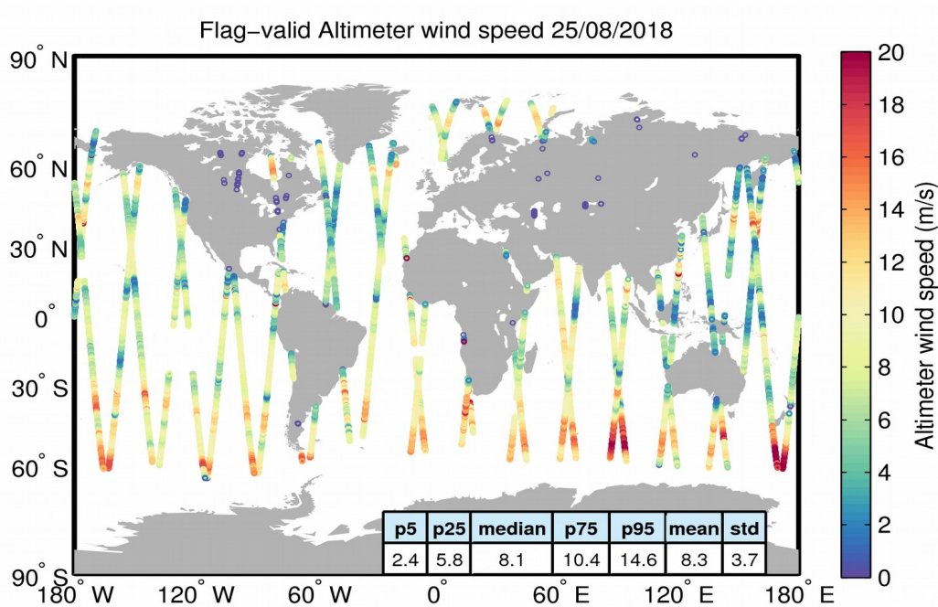
Figure 31. Geographical distribution of flag-valid wind data over oceans and lakes for 25/08/2018. The statistical values shown in the table refer to the wind in m/s and are calculated over all measurements shown in the figure.
