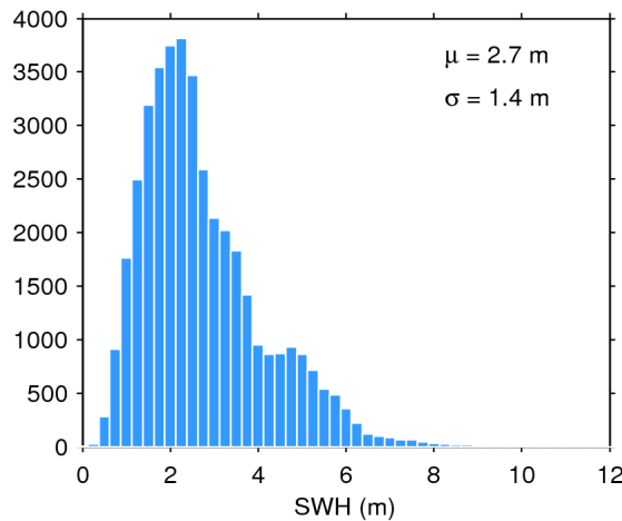
Figure 20. Histogram of science-valid SWH over oceans and lakes for 25/08/2018. The mean ( \mu ) and standard deviation ( \sigma ) are also shown. Note that values larger than 12 m are excluded from the histogram for the sake of readability but not from the computation of \mu and \sigma .
