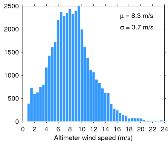
Figure 35. Histogram of science-valid wind over oceans and lakes for 25/08/2018. The mean ( \mu ) and standard deviation ( \sigma ) are also shown. Note that values larger than 24 m/s are excluded from the histogram for the sake of readability but not from the computation of \mu and \sigma .
