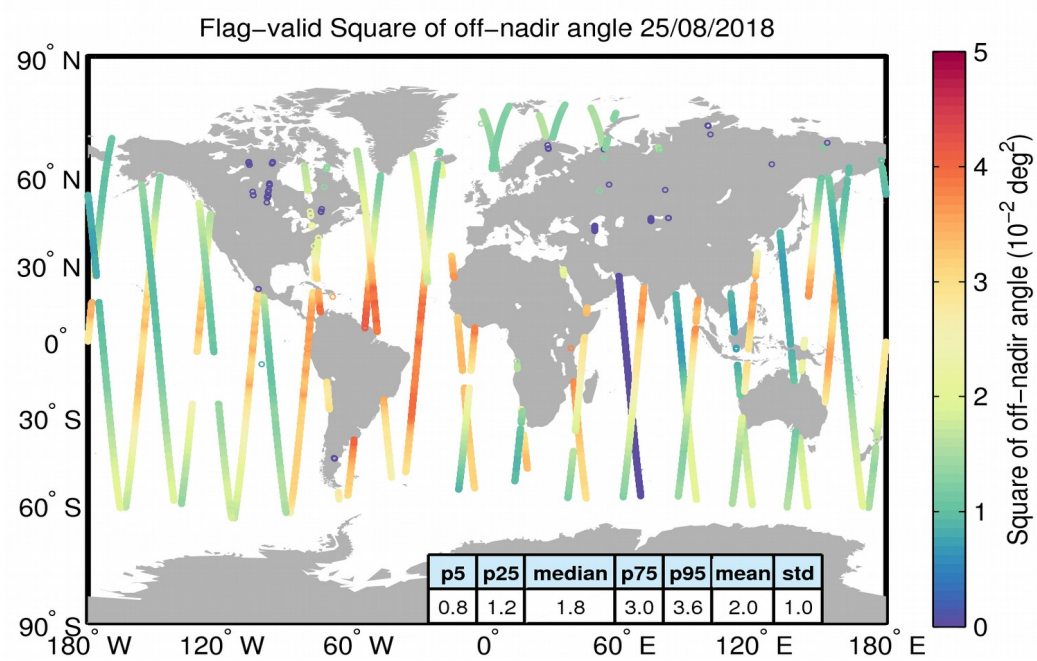
Figure 37. Geographical distribution of flag-valid mispointing data over oceans and lakes for 25/08/2018. The statistical values shown in the table refer to the mispointing in 10^{-2} \text{ deg}^2 and are calculated over all measurements shown in the figure.
