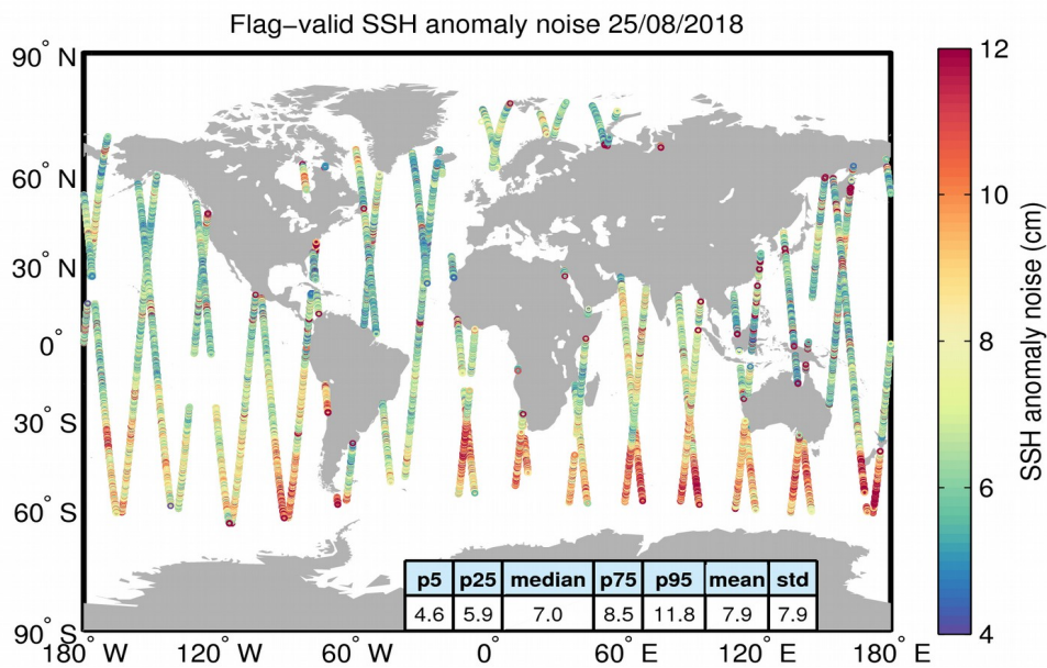
Figure 8. Geographical distribution of flag-valid 20-Hz SSH anomaly measurement noise over oceans and lakes for 25/08/2018. The statistical values shown in the table refer to the SSH anomaly noise and are calculated over all measurements shown in the figure.
