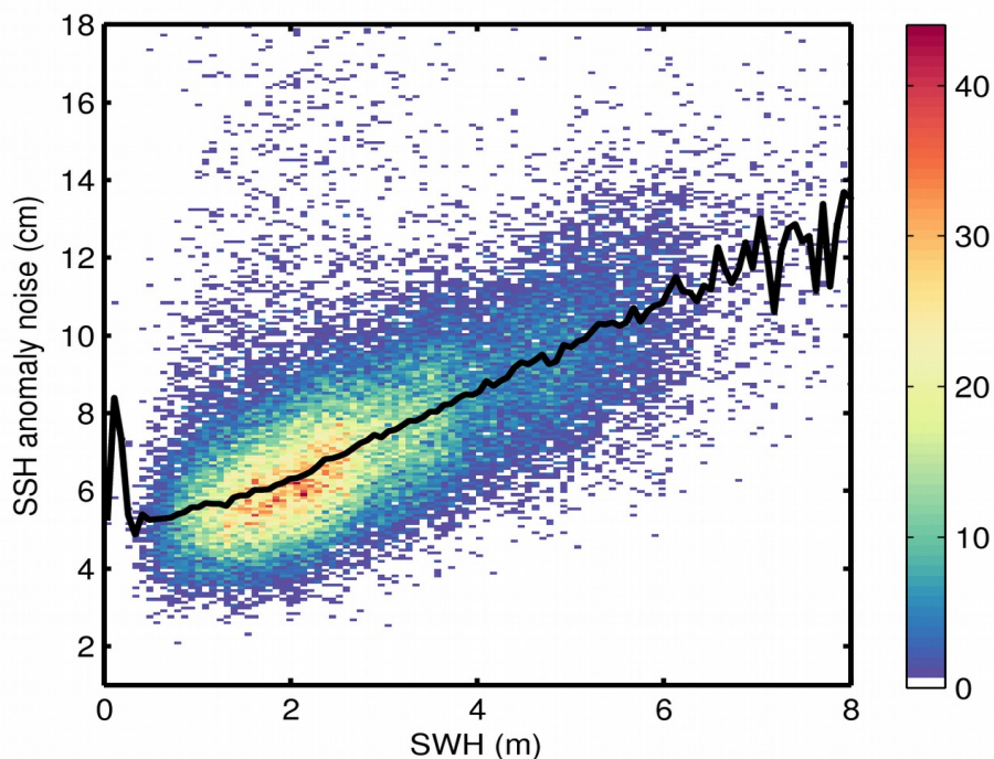
Figure 9. 2D histogram showing flag-valid SSH anomaly noise as a function of SWH for 25/08/2018. The black line denotes the median SSH anomaly noise as a function of SWH.
