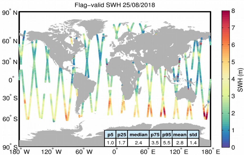
Figure 15. Geographical distribution of flag-valid SWH data over oceans and lakes for 25/08/2018. The statistical values shown in the table refer to the SWH in m and are calculated over all measurements shown in the figure.
