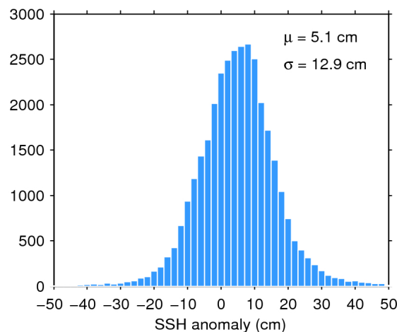
Figure 11. Histogram of science-valid SSH anomaly over oceans and lakes for 25/08/2018. The mean ( \mu ) and standard deviation ( \sigma ) are also shown. Note that values outside [-50 50] cm are excluded from the histogram for the sake of readability but not from the computation of \mu and \sigma .
