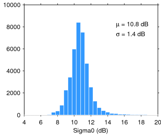
Figure 28. Histogram of science-valid sigma0 over oceans and lakes for 25/08/2018. The mean ( \mu ) and standard deviation ( \sigma ) are also shown. Note that values outside [4 20] dB are excluded from the histogram for the sake of readability but not from the computation of \mu and \sigma .
