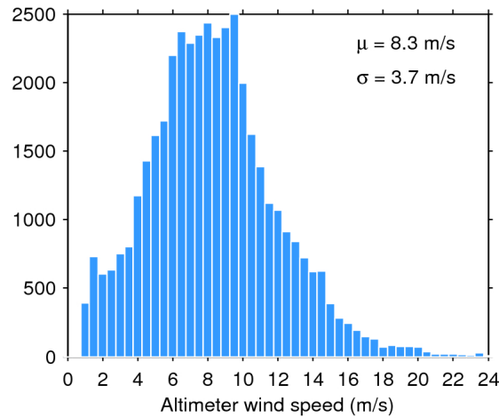
Figure 33. Histogram of flag-valid wind over oceans and lakes for 25/08/2018. The mean ( \mu ) and standard deviation ( \sigma ) are also shown. Note that values larger than 24 m/s are excluded from the histogram for the sake of readability but not from the computation of \mu and \sigma .
