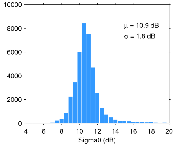
Figure 25. Histogram of flag-valid sigma0 over oceans and lakes for 25/08/2018. The mean ( \mu ) and standard deviation ( \sigma ) are also shown. Note that values outside [4 20] dB are excluded from the histogram for the sake of readability but not from the computation of \mu and \sigma .
