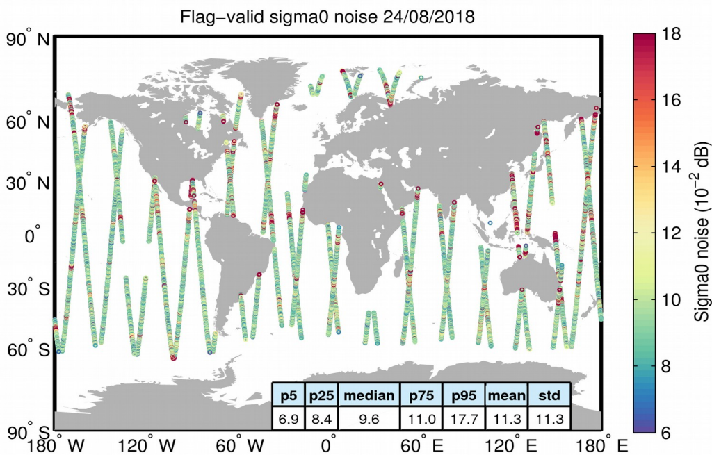
Figure 26. Geographical distribution of flag-valid 20-Hz sigma0 measurement noise over oceans and lakes for 24/08/2018. The statistical values shown in the table refer to the sigma0 noise and are calculated over all measurements shown in the figure.
