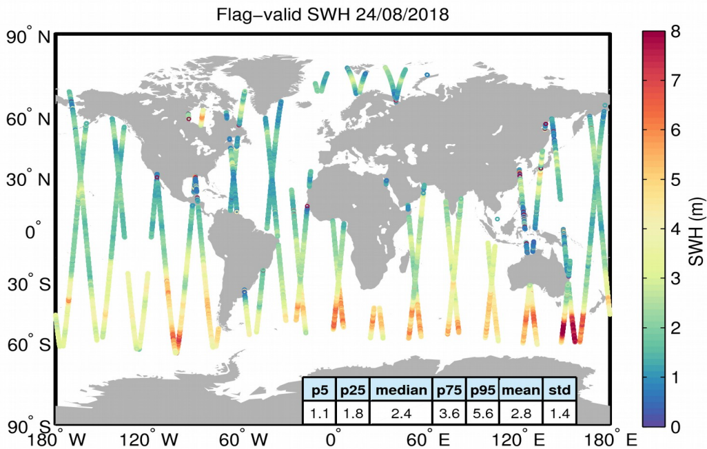
Figure 15. Geographical distribution of flag-valid SWH data over oceans and lakes for 24/08/2018. The statistical values shown in the table refer to the SWH in m and are calculated over all measurements shown in the figure.
