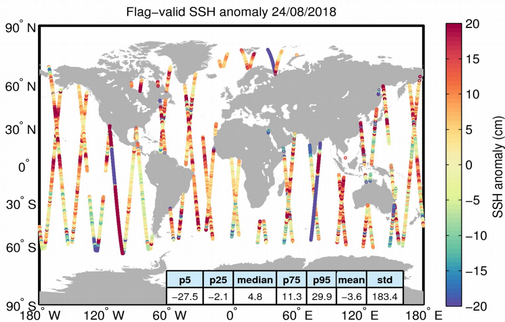
Figure 5. Geographical distribution of flag-valid 1-Hz SSH anomaly data over oceans and lakes for 24/08/2018. The statistical values shown in the table refer to the SSH anomaly in cm and are calculated over all measurements shown in the figure.
