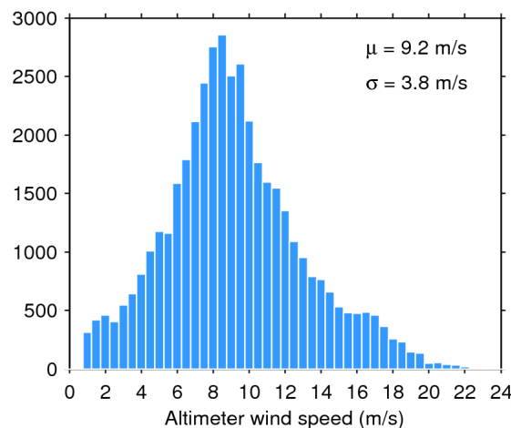
Figure 35. Histogram of science-valid wind over oceans and lakes for 24/08/2018. The mean ( \mu ) and standard deviation ( \sigma ) are also shown. Note that values larger than 24 m/s are excluded from the histogram for the sake of readability but not from the computation of \mu and \sigma .
