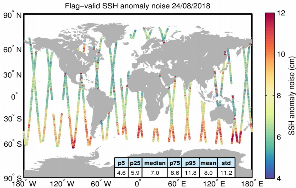
Figure 8. Geographical distribution of flag-valid 20-Hz SSH anomaly measurement noise over oceans and lakes for 24/08/2018. The statistical values shown in the table refer to the SSH anomaly noise and are calculated over all measurements shown in the figure.
