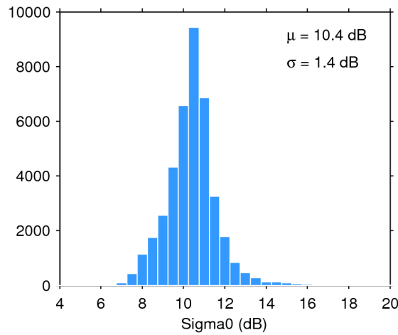
Figure 28. Histogram of science-valid sigma0 over oceans and lakes for 24/08/2018. The mean ( \mu ) and standard deviation ( \sigma ) are also shown. Note that values outside [4 20] dB are excluded from the histogram for the sake of readability but not from the computation of \mu and \sigma .
