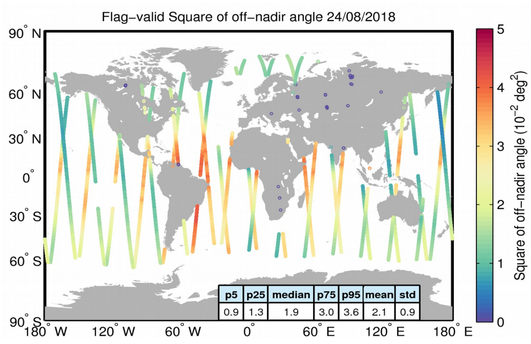
Figure 37. Geographical distribution of flag-valid mispointing data over oceans and lakes for 24/08/2018. The statistical values shown in the table refer to the mispointing in 10^{-2} deg 2 and are calculated over all measurements shown in the figure.
