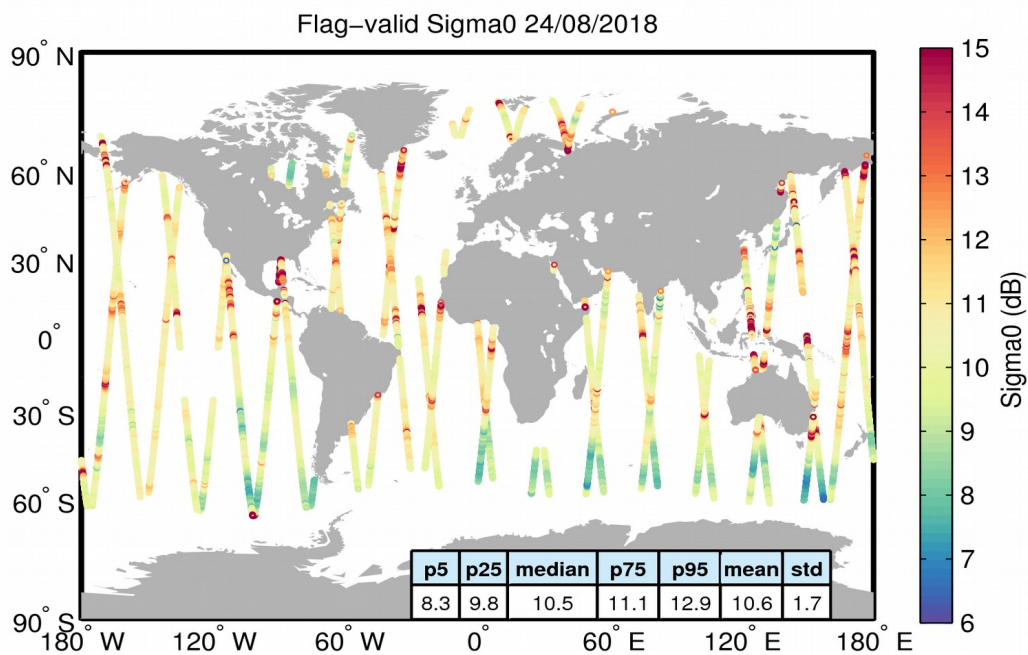
Figure 23. Geographical distribution of flag-valid sigma0 data over oceans and lakes for 24/08/2018. The statistical values shown in the table refer to the sigma0 in dB and are calculated over all measurements shown in the figure.
