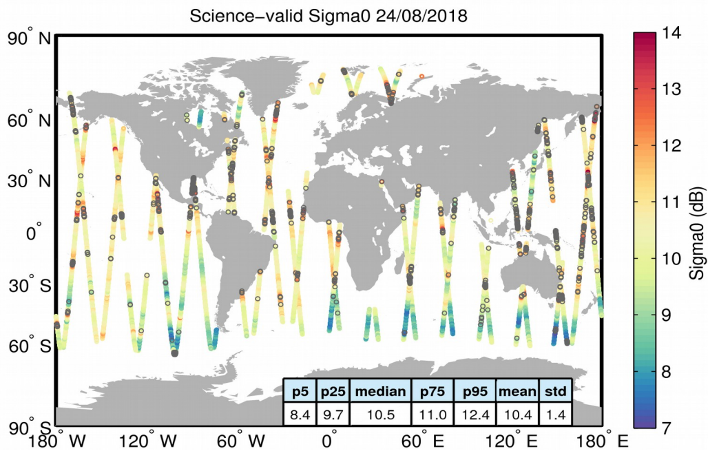
Figure 27. Geographical distribution of science-valid sigma0 data over oceans and lakes for 24/08/2018. The statistical values shown in the table refer to the sigma0 in dB and are calculated over all measurements shown in the figure. Gray circles denote records that have been rejected based on the editing criteria described in Table 4.
