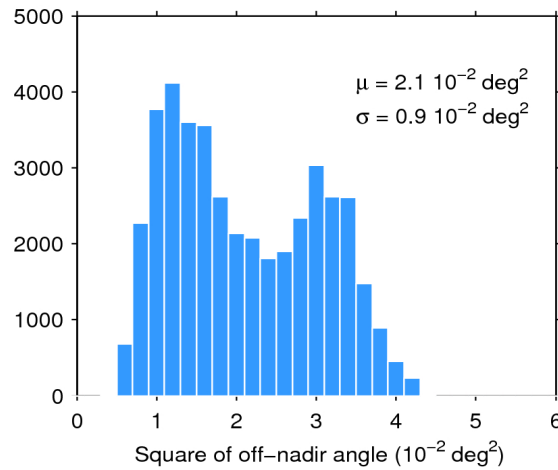
Figure 39. Histogram of flag-valid mispointing over oceans and lakes for 24/08/2018. The mean ( \mu ) and standard deviation ( \sigma ) are also shown. Note that values larger than 6 \cdot 10^{-2} \text{ deg}^2 are excluded from the histogram for the sake of readability but not from the computation of \mu and \sigma .
