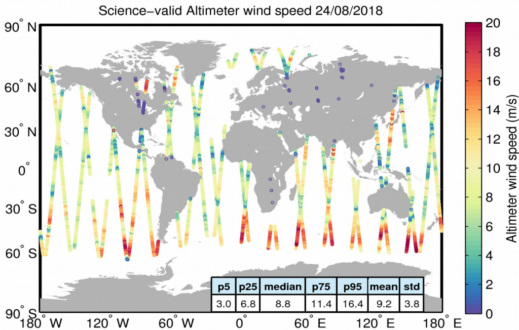
Figure 34. Geographical distribution of science-valid wind data over oceans and lakes for 24/08/2018. The statistical values shown in the table refer to the wind in m/s and are calculated over all measurements shown in the figure. Gray circles denote records that have been rejected based on the editing criteria described in Table 5.
