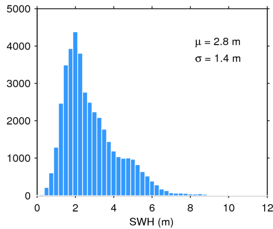
Figure 17. Histogram of flag-valid SWH over oceans and lakes for 24/08/2018. The mean ( \mu ) and standard deviation ( \sigma ) are also shown. Note that values larger than 12 m are excluded from the histogram for the sake of readability but not from the computation of \mu and \sigma .
