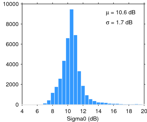
Figure 25. Histogram of flag-valid sigma0 over oceans and lakes for 24/08/2018. The mean ( \mu ) and standard deviation ( \sigma ) are also shown. Note that values outside [4 20] dB are excluded from the histogram for the sake of readability but not from the computation of \mu and \sigma .
