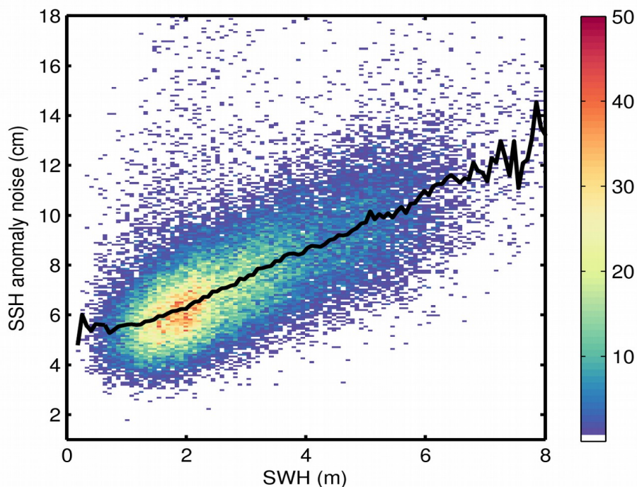
Figure 9. 2D histogram showing flag-valid SSH anomaly noise as a function of SWH for 24/08/2018. The black line denotes the median SSH anomaly noise as a function of SWH.
