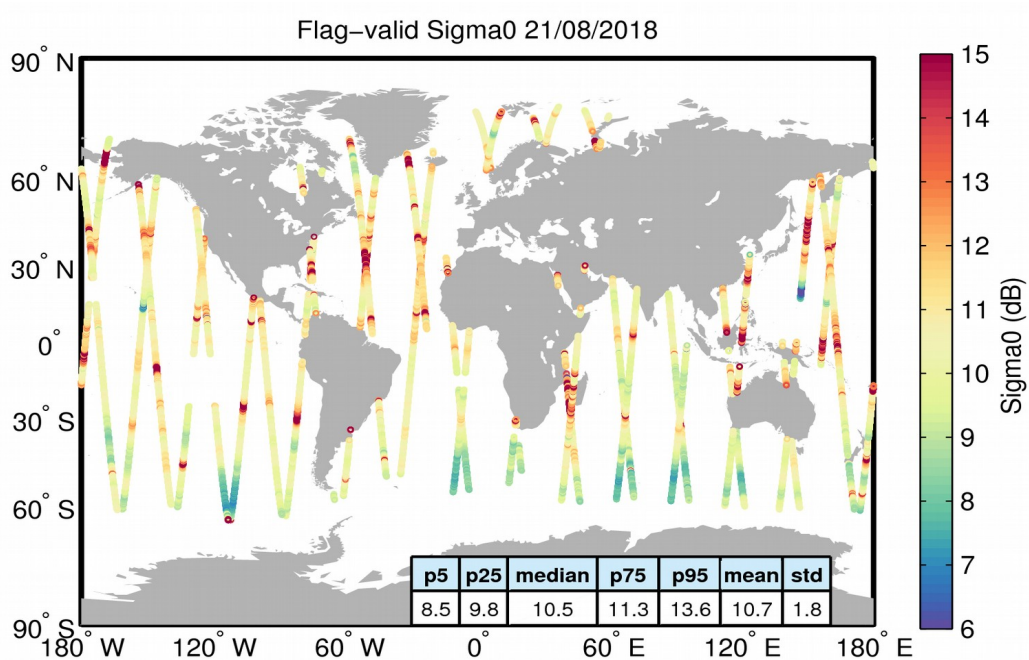
Figure 23. Geographical distribution of flag-valid sigma0 data over oceans and lakes for 21/08/2018. The statistical values shown in the table refer to the sigma0 in dB and are calculated over all measurements shown in the figure.
