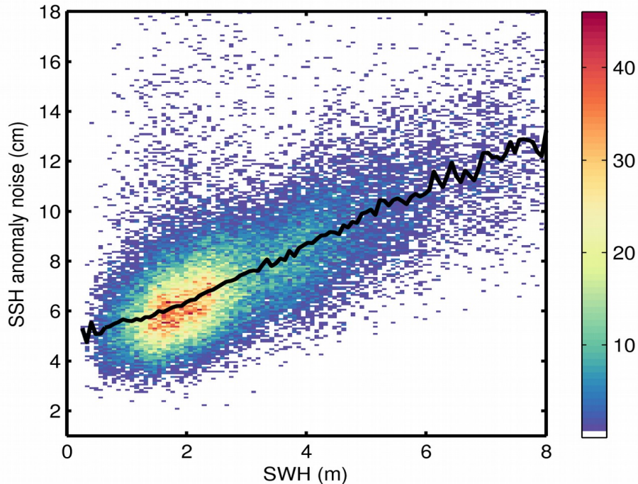
Figure 9. 2D histogram showing flag-valid SSH anomaly noise as a function of SWH for 21/08/2018. The black line denotes the median SSH anomaly noise as a function of SWH.
