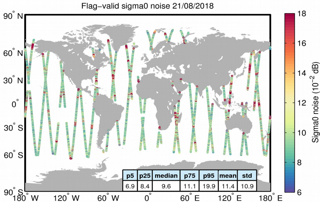
Figure 26. Geographical distribution of flag-valid 20-Hz sigma0 measurement noise over oceans and lakes for 21/08/2018. The statistical values shown in the table refer to the sigma0 noise and are calculated over all measurements shown in the figure.
