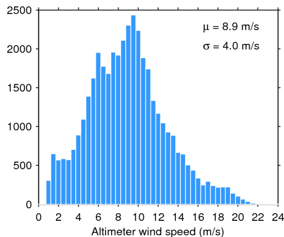
Figure 35. Histogram of science-valid wind over oceans and lakes for 21/08/2018. The mean ( \mu ) and standard deviation ( \sigma ) are also shown. Note that values larger than 24 m/s are excluded from the histogram for the sake of readability but not from the computation of \mu and \sigma .
