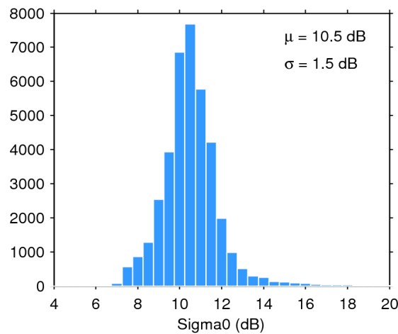
Figure 28. Histogram of science-valid sigma0 over oceans and lakes for 21/08/2018. The mean ( \mu ) and standard deviation ( \sigma ) are also shown. Note that values outside [4 20] dB are excluded from the histogram for the sake of readability but not from the computation of \mu and \sigma .
