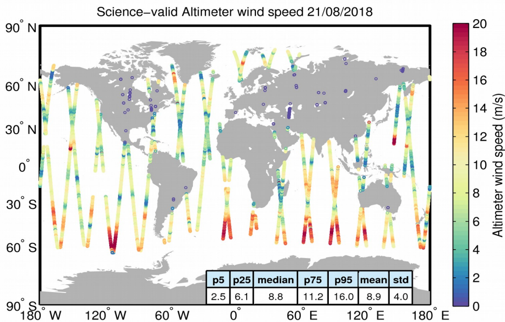
Figure 34. Geographical distribution of science-valid wind data over oceans and lakes for 21/08/2018. The statistical values shown in the table refer to the wind in m/s and are calculated over all measurements shown in the figure. Gray circles denote records that have been rejected based on the editing criteria described in Table 5.
