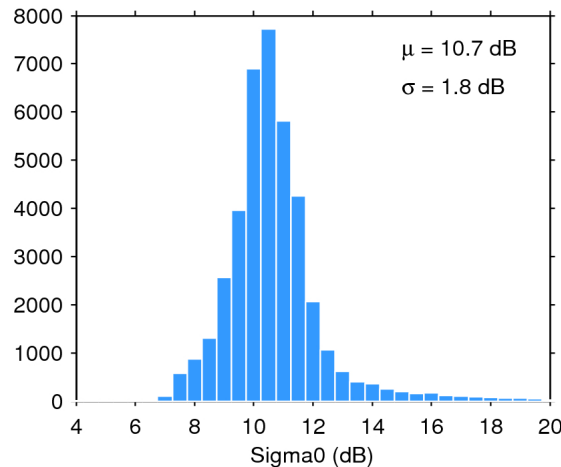
Figure 25. Histogram of flag-valid sigma0 over oceans and lakes for 21/08/2018. The mean ( \mu ) and standard deviation ( \sigma ) are also shown. Note that values outside [4 20] dB are excluded from the histogram for the sake of readability but not from the computation of \mu and \sigma .
