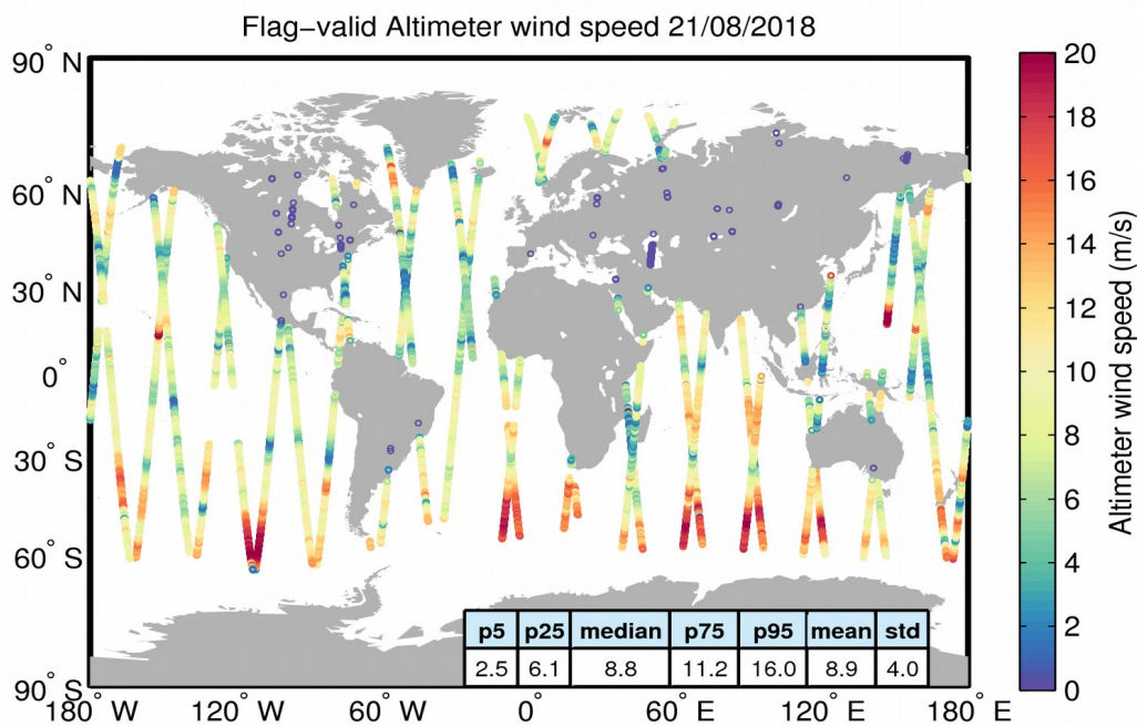
Figure 31. Geographical distribution of flag-valid wind data over oceans and lakes for 21/08/2018. The statistical values shown in the table refer to the wind in m/s and are calculated over all measurements shown in the figure.
