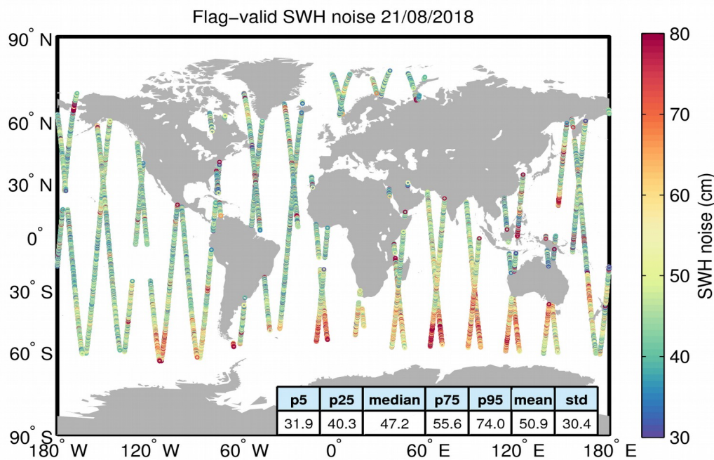
Figure 18. Geographical distribution of flag-valid 20-Hz SWH measurement noise over oceans and lakes for 21/08/2018. The statistical values shown in the table refer to the SWH noise and are calculated over all measurements shown in the figure.
