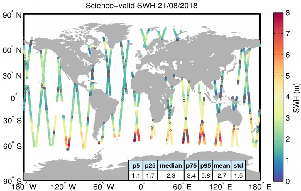
Figure 19. Geographical distribution of science-valid SWH data over oceans and lakes for 21/08/2018. The statistical values shown in the table refer to the SWH in m and are calculated over all measurements shown in the figure. Gray circles denote records that have been rejected based on the editing criteria described in Table 3.
