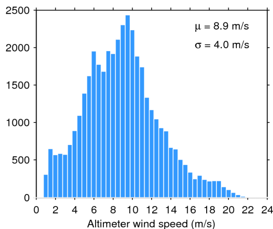
Figure 33. Histogram of flag-valid wind over oceans and lakes for 21/08/2018. The mean ( \mu ) and standard deviation ( \sigma ) are also shown. Note that values larger than 24 m/s are excluded from the histogram for the sake of readability but not from the computation of \mu and \sigma .
