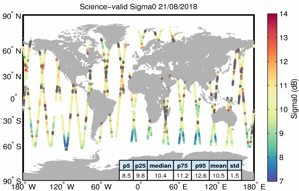
Figure 27. Geographical distribution of science-valid sigma0 data over oceans and lakes for 21/08/2018. The statistical values shown in the table refer to the sigma0 in dB and are calculated over all measurements shown in the figure. Gray circles denote records that have been rejected based on the editing criteria described in Table 4.
