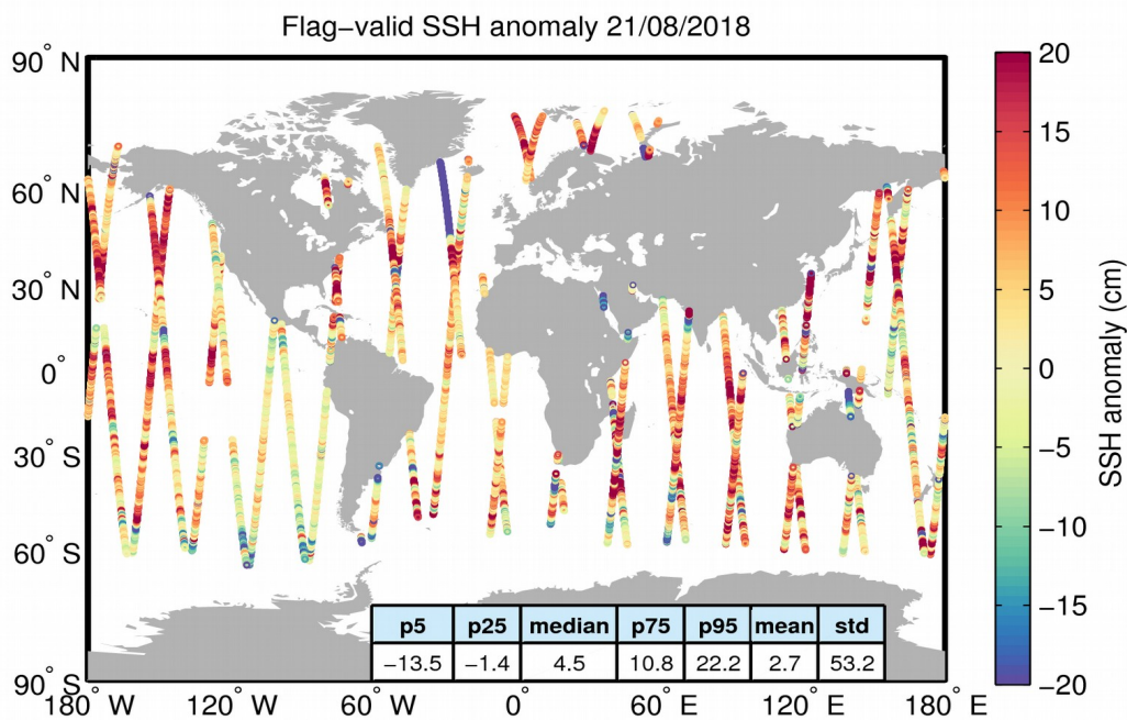
Figure 5. Geographical distribution of flag-valid 1-Hz SSH anomaly data over oceans and lakes for 21/08/2018. The statistical values shown in the table refer to the SSH anomaly in cm and are calculated over all measurements shown in the figure.
