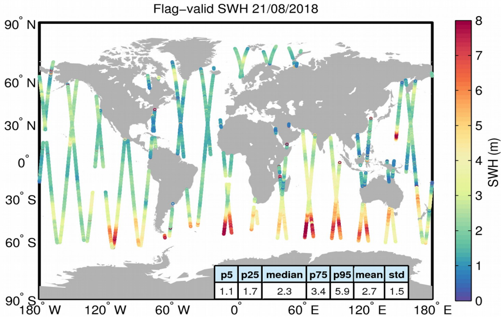
Figure 15. Geographical distribution of flag-valid SWH data over oceans and lakes for 21/08/2018. The statistical values shown in the table refer to the SWH in m and are calculated over all measurements shown in the figure.
