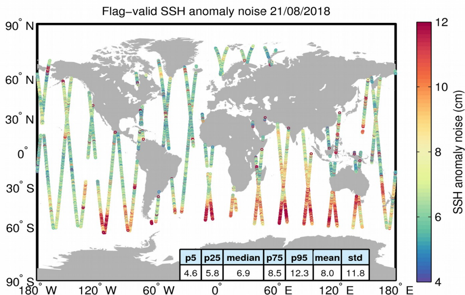
Figure 8. Geographical distribution of flag-valid 20-Hz SSH anomaly measurement noise over oceans and lakes for 21/08/2018. The statistical values shown in the table refer to the SSH anomaly noise and are calculated over all measurements shown in the figure.
