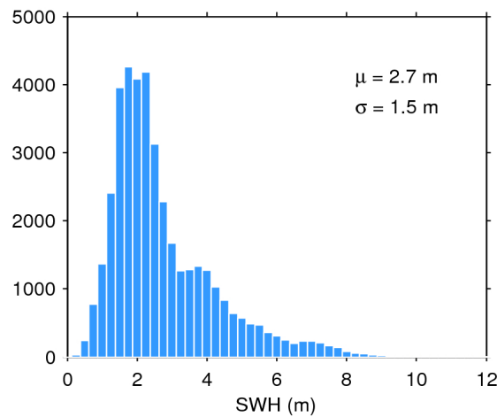
Figure 17. Histogram of flag-valid SWH over oceans and lakes for 21/08/2018. The mean ( \mu ) and standard deviation ( \sigma ) are also shown. Note that values larger than 12 m are excluded from the histogram for the sake of readability but not from the computation of \mu and \sigma .
