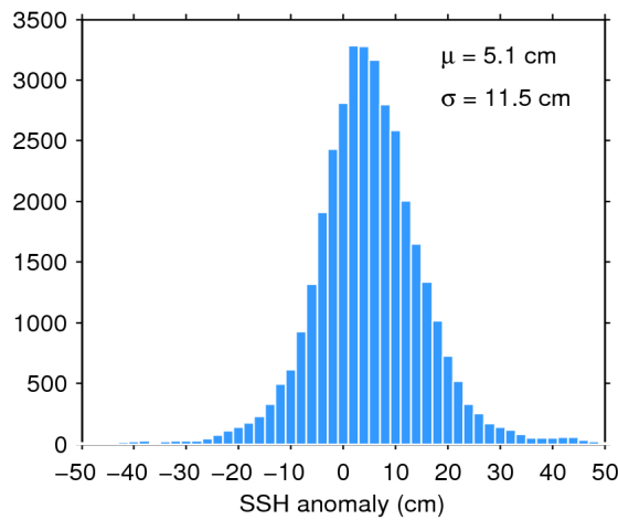
Figure 11. Histogram of science-valid SSH anomaly over oceans and lakes for 21/08/2018. The mean ( \mu ) and standard deviation ( \sigma ) are also shown. Note that values outside [-50 50] cm are excluded from the histogram for the sake of readability but not from the computation of \mu and \sigma .
