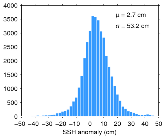
Figure 7. Histogram of flag-valid SSH anomaly over oceans and lakes for 21/08/2018. The mean ( \mu ) and standard deviation ( \sigma ) are also shown. Note that values outside [-50 50] cm are excluded from the histogram for the sake of readability but not from the computation of \mu and \sigma .
