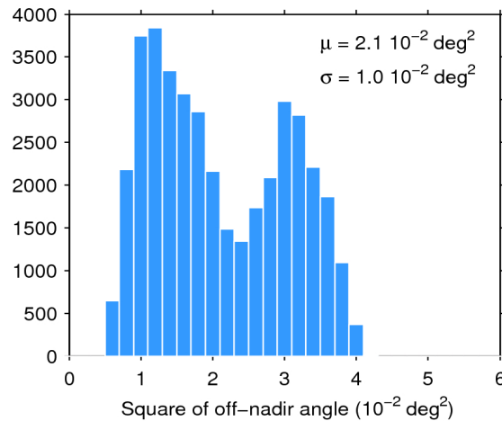
Figure 39. Histogram of flag-valid mispointing over oceans and lakes for 21/08/2018. The mean ( \mu ) and standard deviation ( \sigma ) are also shown. Note that values larger than 6 \cdot 10^{-2} \text{ deg}^2 are excluded from the histogram for the sake of readability but not from the computation of \mu and \sigma .
