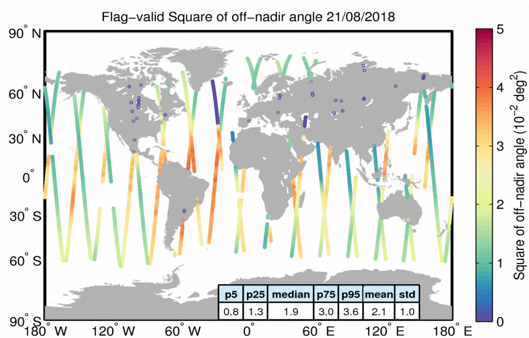
Figure 37. Geographical distribution of flag-valid mispointing data over oceans and lakes for 21/08/2018. The statistical values shown in the table refer to the mispointing in 10^{-2} deg 2 and are calculated over all measurements shown in the figure.
