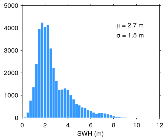
Figure 20. Histogram of science-valid SWH over oceans and lakes for 21/08/2018. The mean ( \mu ) and standard deviation ( \sigma ) are also shown. Note that values larger than 12 m are excluded from the histogram for the sake of readability but not from the computation of \mu and \sigma .
