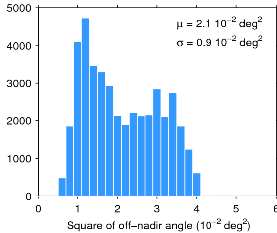
Figure 39. Histogram of flag-valid mispointing over oceans and lakes for 20/08/2018. The mean ( \mu ) and standard deviation ( \sigma ) are also shown. Note that values larger than 6 \cdot 10^{-2} \text{ deg}^2 are excluded from the histogram for the sake of readability but not from the computation of \mu and \sigma .
