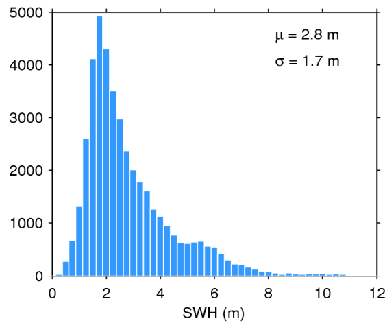
Figure 17. Histogram of flag-valid SWH over oceans and lakes for 20/08/2018. The mean ( \mu ) and standard deviation ( \sigma ) are also shown. Note that values larger than 12 m are excluded from the histogram for the sake of readability but not from the computation of \mu and \sigma .
