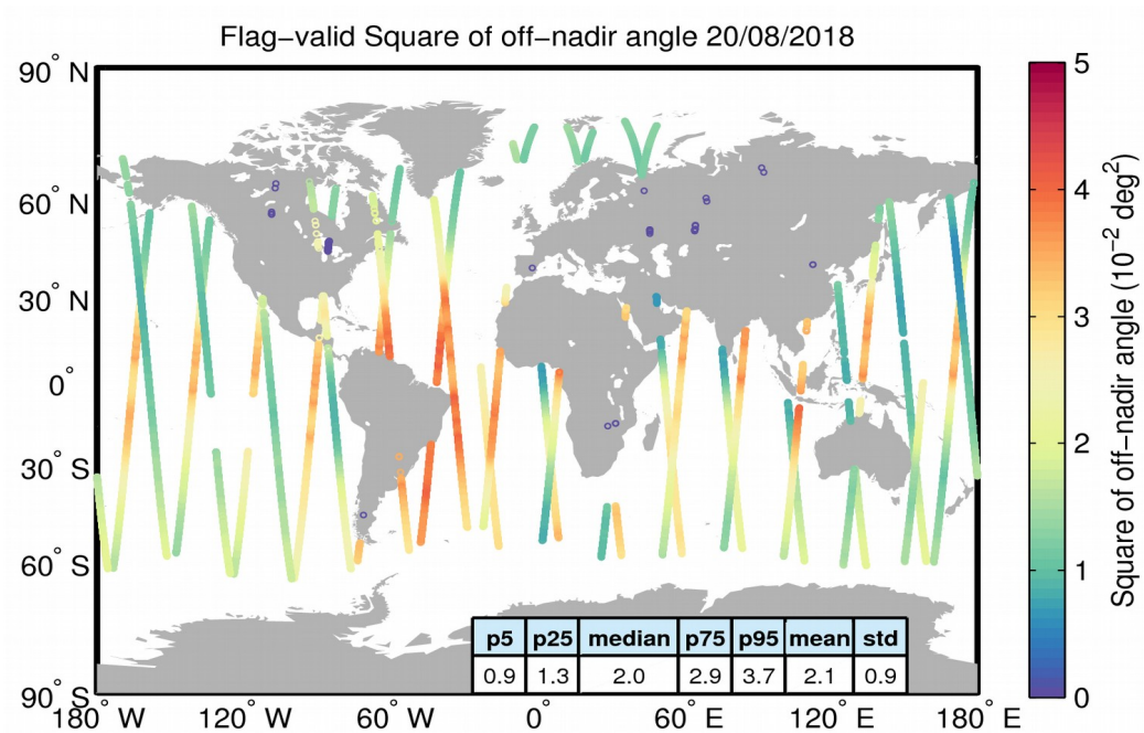
Figure 37. Geographical distribution of flag-valid mispointing data over oceans and lakes for 20/08/2018. The statistical values shown in the table refer to the mispointing in 10^{-2} deg 2 and are calculated over all measurements shown in the figure.
