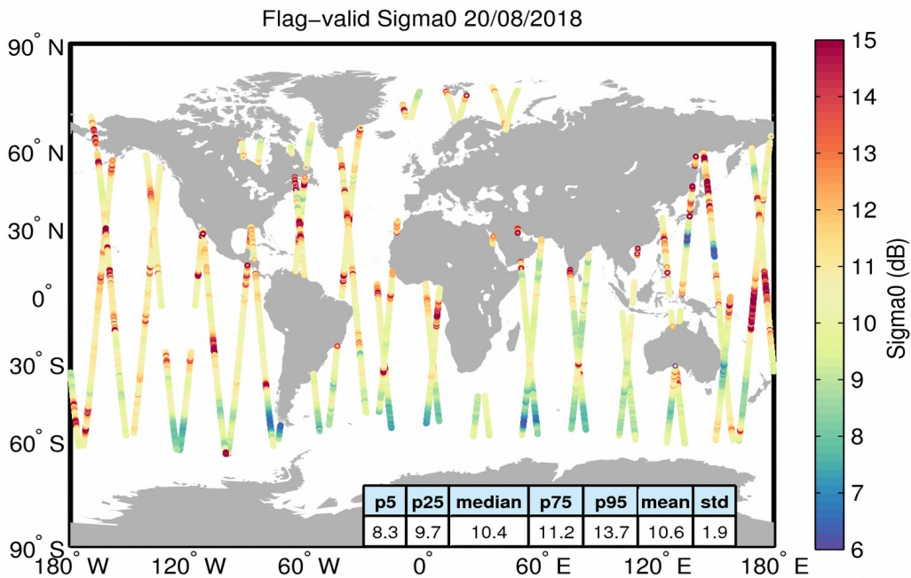
Figure 23. Geographical distribution of flag-valid sigma0 data over oceans and lakes for 20/08/2018. The statistical values shown in the table refer to the sigma0 in dB and are calculated over all measurements shown in the figure.
