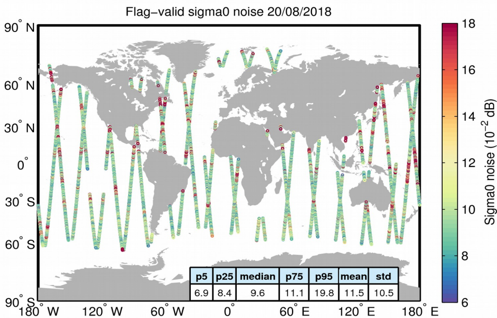
Figure 26. Geographical distribution of flag-valid 20-Hz sigma0 measurement noise over oceans and lakes for 20/08/2018. The statistical values shown in the table refer to the sigma0 noise and are calculated over all measurements shown in the figure.
