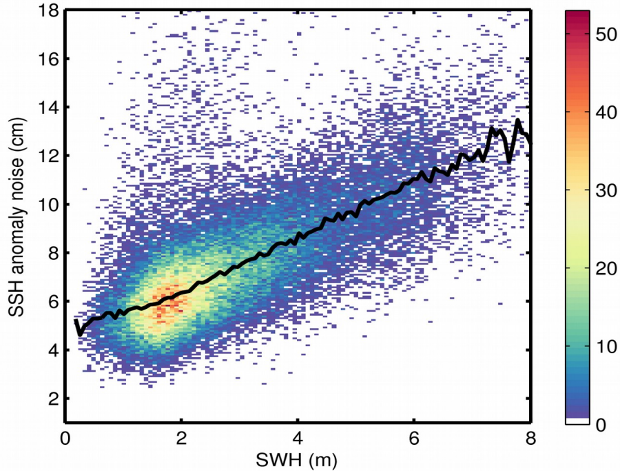
Figure 9. 2D histogram showing flag-valid SSH anomaly noise as a function of SWH for 20/08/2018. The black line denotes the median SSH anomaly noise as a function of SWH.
