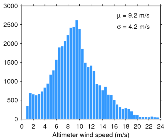
Figure 35. Histogram of science-valid wind over oceans and lakes for 20/08/2018. The mean ( \mu ) and standard deviation ( \sigma ) are also shown. Note that values larger than 24 m/s are excluded from the histogram for the sake of readability but not from the computation of \mu and \sigma .
