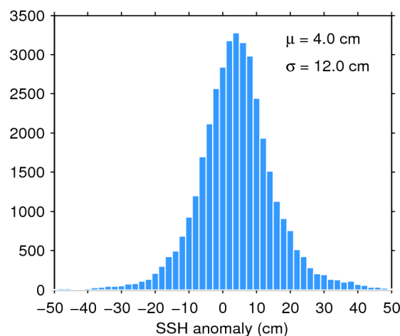
Figure 11. Histogram of science-valid SSH anomaly over oceans and lakes for 20/08/2018. The mean ( \mu ) and standard deviation ( \sigma ) are also shown. Note that values outside [-50 50] cm are excluded from the histogram for the sake of readability but not from the computation of \mu and \sigma .
