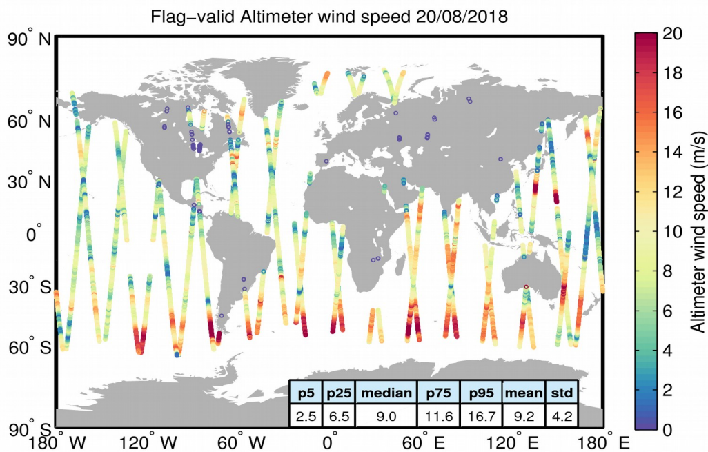
Figure 31. Geographical distribution of flag-valid wind data over oceans and lakes for 20/08/2018. The statistical values shown in the table refer to the wind in m/s and are calculated over all measurements shown in the figure.
