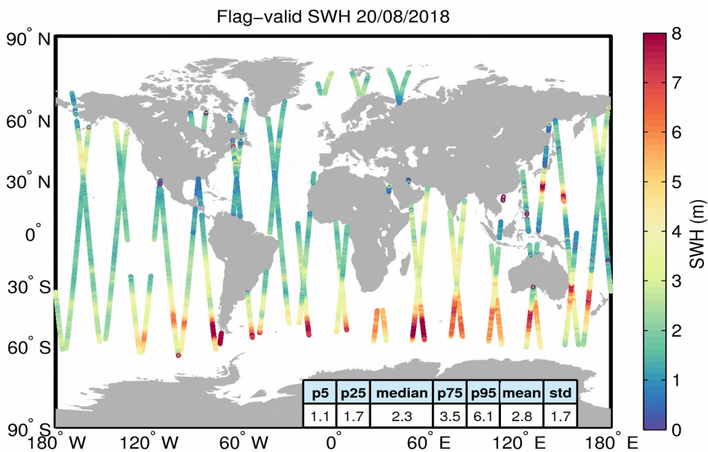
Figure 15. Geographical distribution of flag-valid SWH data over oceans and lakes for 20/08/2018. The statistical values shown in the table refer to the SWH in m and are calculated over all measurements shown in the figure.
