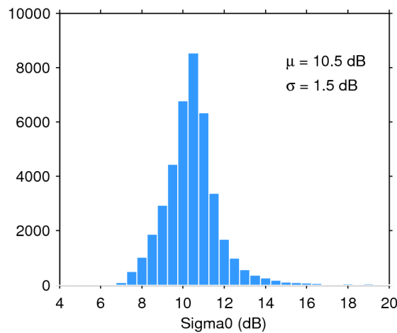
Figure 28. Histogram of science-valid sigma0 over oceans and lakes for 20/08/2018. The mean ( \mu ) and standard deviation ( \sigma ) are also shown. Note that values outside [4 20] dB are excluded from the histogram for the sake of readability but not from the computation of \mu and \sigma .
