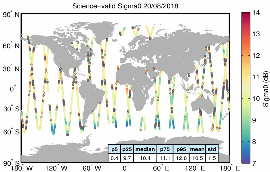
Figure 27. Geographical distribution of science-valid sigma0 data over oceans and lakes for 20/08/2018. The statistical values shown in the table refer to the sigma0 in dB and are calculated over all measurements shown in the figure. Gray circles denote records that have been rejected based on the editing criteria described in Table 4.
