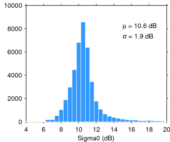
Figure 25. Histogram of flag-valid sigma0 over oceans and lakes for 20/08/2018. The mean ( \mu ) and standard deviation ( \sigma ) are also shown. Note that values outside [4 20] dB are excluded from the histogram for the sake of readability but not from the computation of \mu and \sigma .
