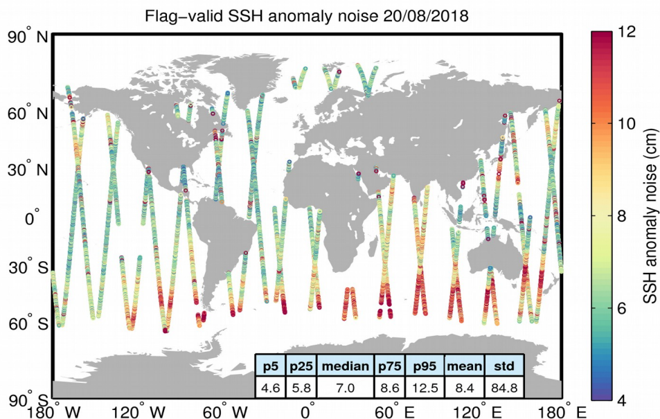
Figure 8. Geographical distribution of flag-valid 20-Hz SSH anomaly measurement noise over oceans and lakes for 20/08/2018. The statistical values shown in the table refer to the SSH anomaly noise and are calculated over all measurements shown in the figure.
