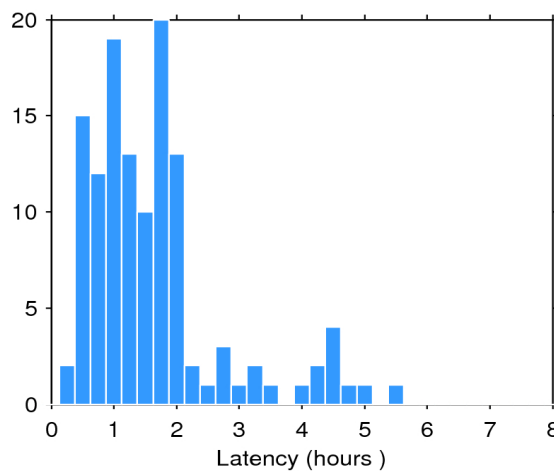
Figure 2. Histogram of the data latency for 20/08/2018. The y-axis denotes the number of files that are made available with a delay of x-hours with respect to the mean time of the records stored in the file.
