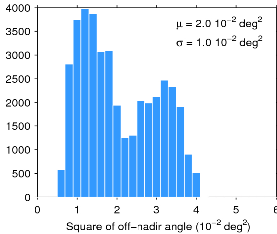
Figure 39. Histogram of flag-valid mispointing over oceans and lakes for 19/08/2018. The mean ( \mu ) and standard deviation ( \sigma ) are also shown. Note that values larger than 6 \cdot 10^{-2} \text{ deg}^2 are excluded from the histogram for the sake of readability but not from the computation of \mu and \sigma .
