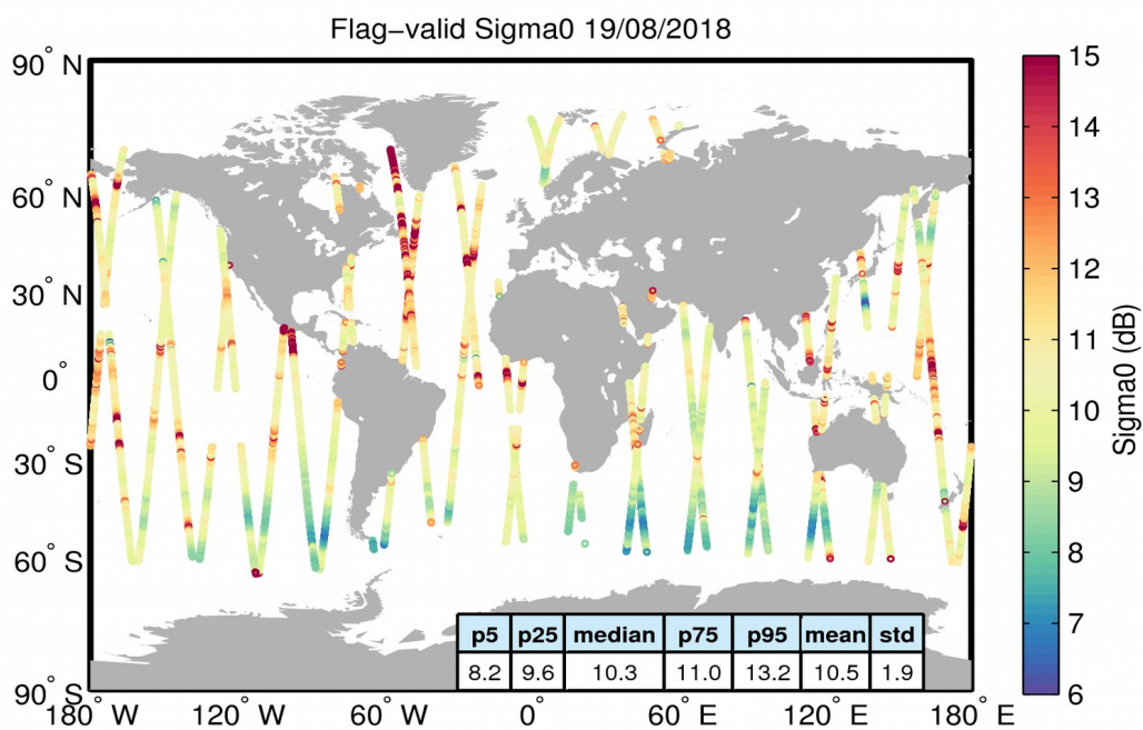
Figure 23. Geographical distribution of flag-valid sigma0 data over oceans and lakes for 19/08/2018. The statistical values shown in the table refer to the sigma0 in dB and are calculated over all measurements shown in the figure.
