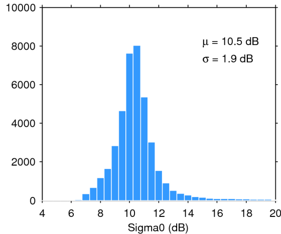
Figure 25. Histogram of flag-valid sigma0 over oceans and lakes for 19/08/2018. The mean ( \mu ) and standard deviation ( \sigma ) are also shown. Note that values outside [4 20] dB are excluded from the histogram for the sake of readability but not from the computation of \mu and \sigma .
