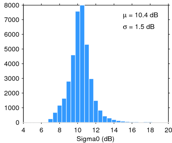
Figure 28. Histogram of science-valid sigma0 over oceans and lakes for 19/08/2018. The mean ( \mu ) and standard deviation ( \sigma ) are also shown. Note that values outside [4 20] dB are excluded from the histogram for the sake of readability but not from the computation of \mu and \sigma .
