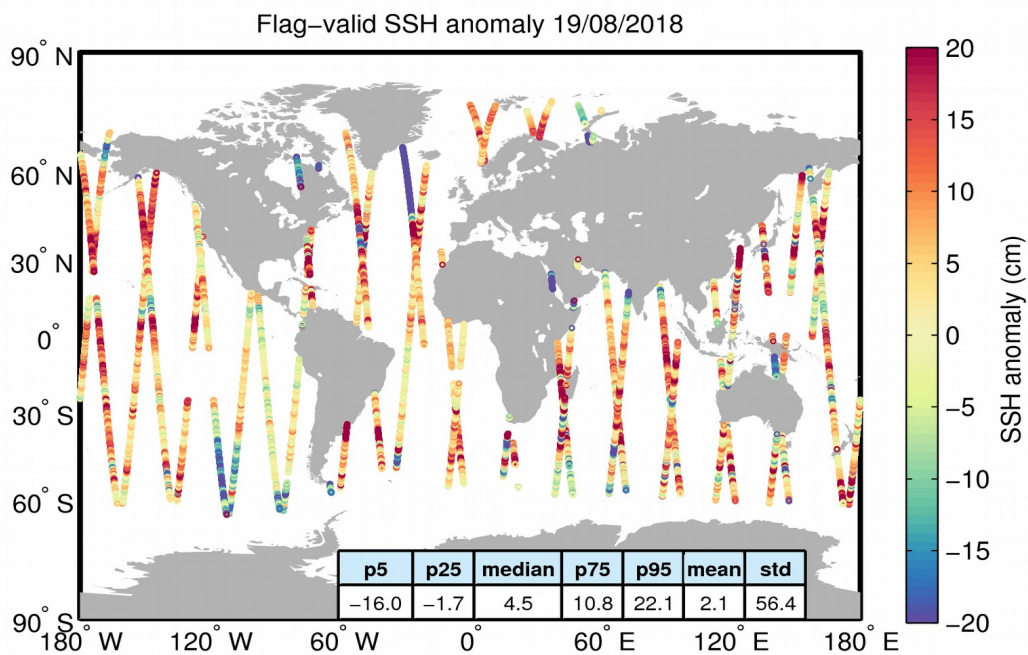
Figure 5. Geographical distribution of flag-valid 1-Hz SSH anomaly data over oceans and lakes for 19/08/2018. The statistical values shown in the table refer to the SSH anomaly in cm and are calculated over all measurements shown in the figure.
