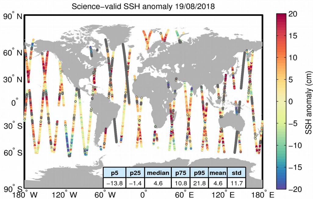
Figure 10. Geographical distribution of science-valid SSH anomaly data over oceans and lakes for 19/08/2018. The statistical values shown in the table refer to the SSH anomaly in cm and are calculated over all measurements shown in the figure. Gray circles denote records that have been rejected based on the editing criteria described in Table 2.
