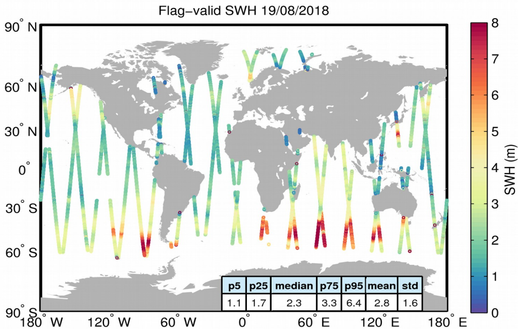
Figure 15. Geographical distribution of flag-valid SWH data over oceans and lakes for 19/08/2018. The statistical values shown in the table refer to the SWH in m and are calculated over all measurements shown in the figure.
