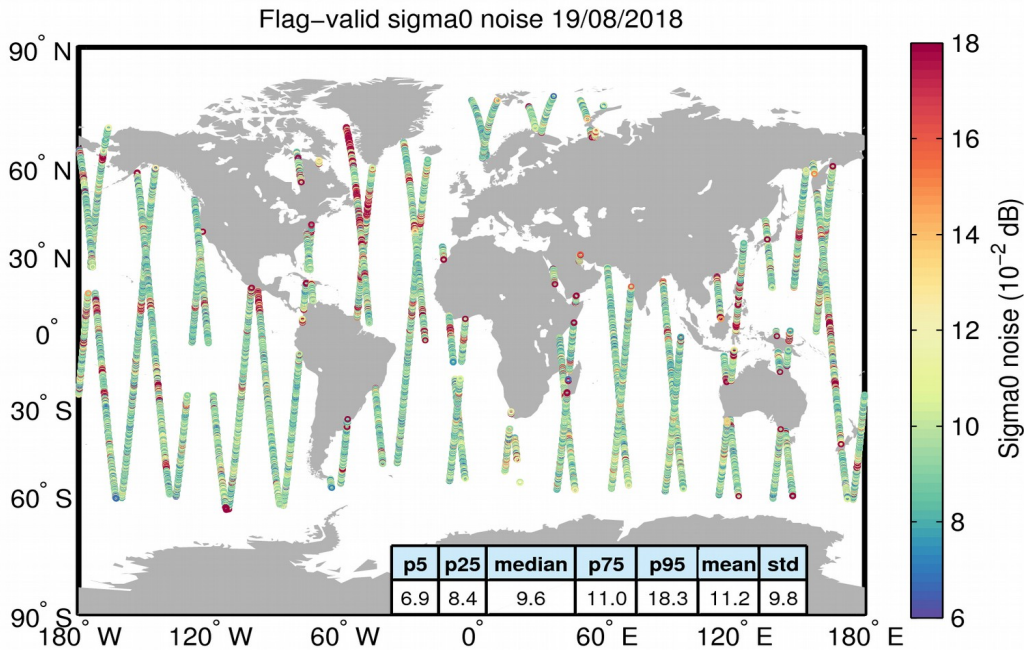
Figure 26. Geographical distribution of flag-valid 20-Hz sigma0 measurement noise over oceans and lakes for 19/08/2018. The statistical values shown in the table refer to the sigma0 noise and are calculated over all measurements shown in the figure.
