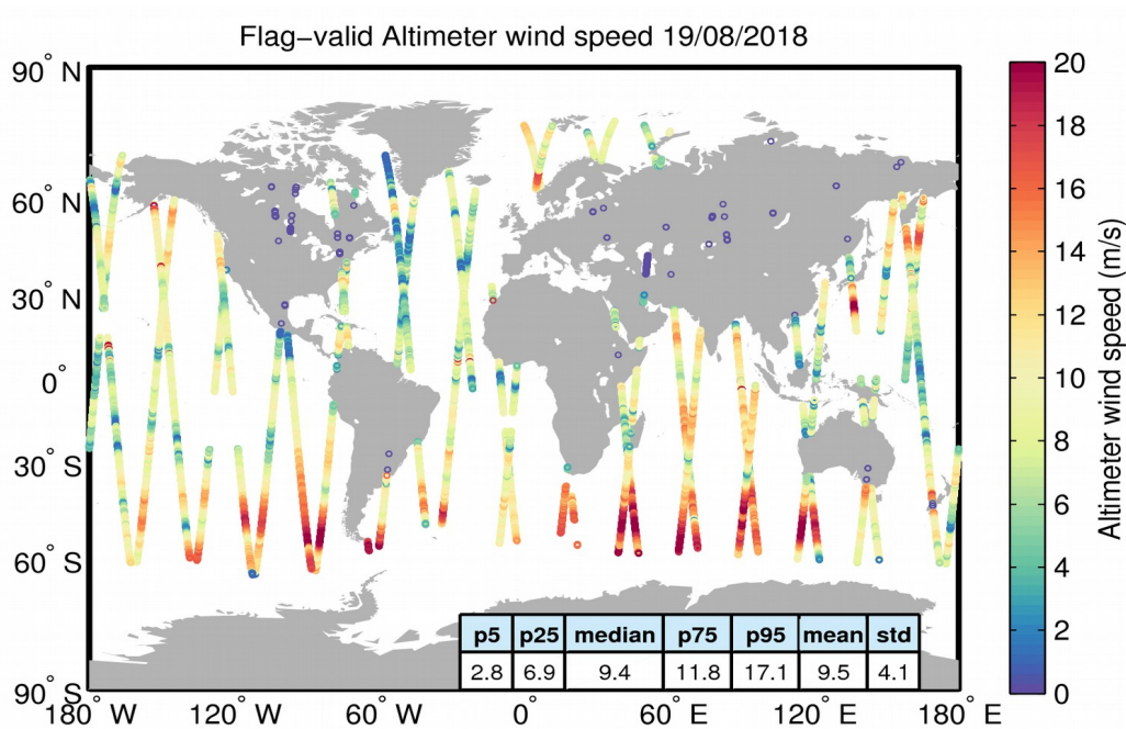
Figure 31. Geographical distribution of flag-valid wind data over oceans and lakes for 19/08/2018. The statistical values shown in the table refer to the wind in m/s and are calculated over all measurements shown in the figure.
