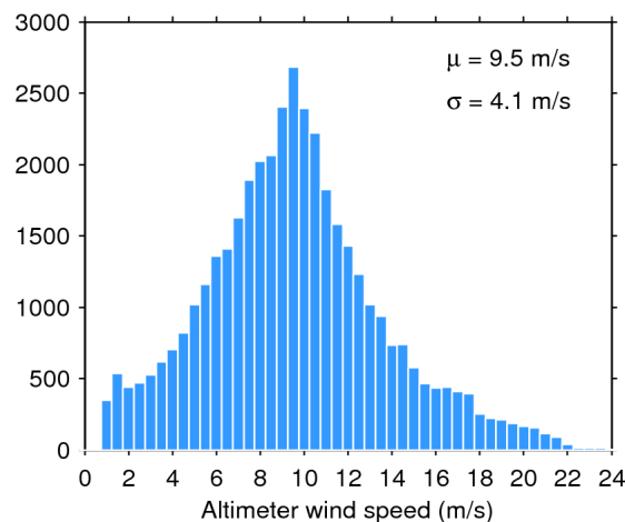
Figure 35. Histogram of science-valid wind over oceans and lakes for 19/08/2018. The mean ( \mu ) and standard deviation ( \sigma ) are also shown. Note that values larger than 24 m/s are excluded from the histogram for the sake of readability but not from the computation of \mu and \sigma .
