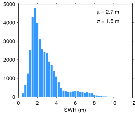
Figure 20. Histogram of science-valid SWH over oceans and lakes for 19/08/2018. The mean ( \mu ) and standard deviation ( \sigma ) are also shown. Note that values larger than 12 m are excluded from the histogram for the sake of readability but not from the computation of \mu and \sigma .
