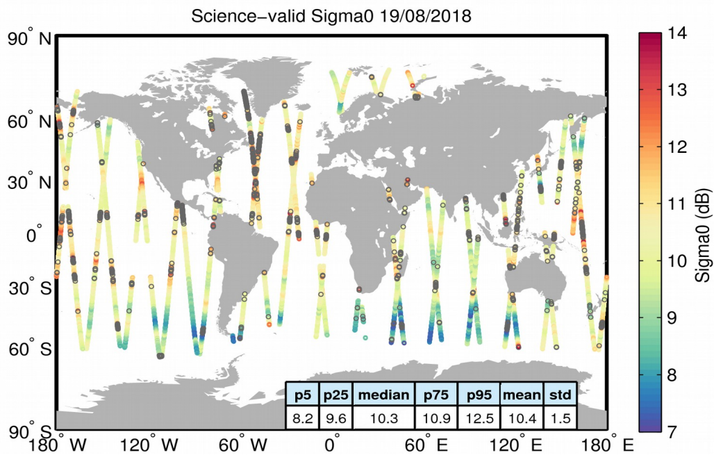
Figure 27. Geographical distribution of science-valid sigma0 data over oceans and lakes for 19/08/2018. The statistical values shown in the table refer to the sigma0 in dB and are calculated over all measurements shown in the figure. Gray circles denote records that have been rejected based on the editing criteria described in Table 4.
