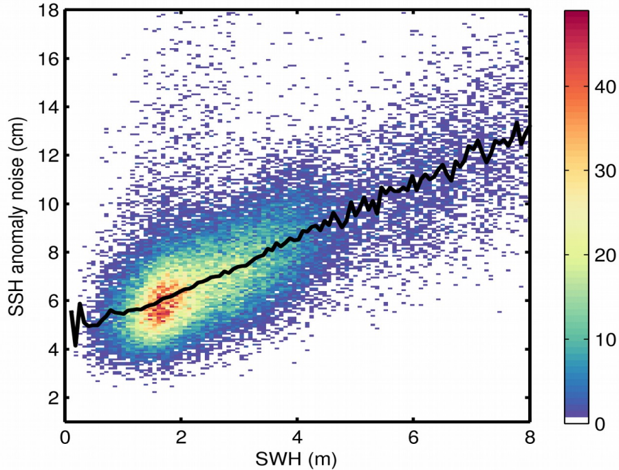
Figure 9. 2D histogram showing flag-valid SSH anomaly noise as a function of SWH for 19/08/2018. The black line denotes the median SSH anomaly noise as a function of SWH.
