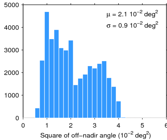
Figure 39. Histogram of flag-valid mispointing over oceans and lakes for 18/08/2018. The mean ( \mu ) and standard deviation ( \sigma ) are also shown. Note that values larger than 6 \cdot 10^{-2} \text{ deg}^2 are excluded from the histogram for the sake of readability but not from the computation of \mu and \sigma .
