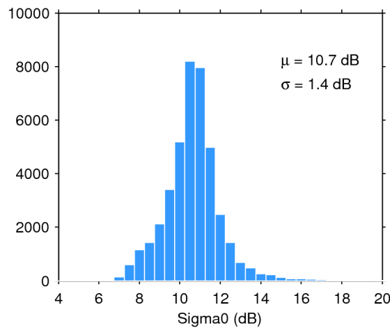
Figure 28. Histogram of science-valid sigma0 over oceans and lakes for 18/08/2018. The mean ( \mu ) and standard deviation ( \sigma ) are also shown. Note that values outside [4 20] dB are excluded from the histogram for the sake of readability but not from the computation of \mu and \sigma .
