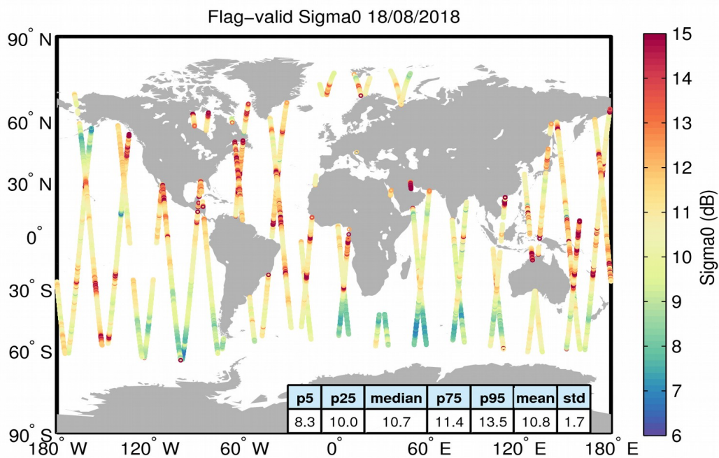
Figure 23. Geographical distribution of flag-valid sigma0 data over oceans and lakes for 18/08/2018. The statistical values shown in the table refer to the sigma0 in dB and are calculated over all measurements shown in the figure.
