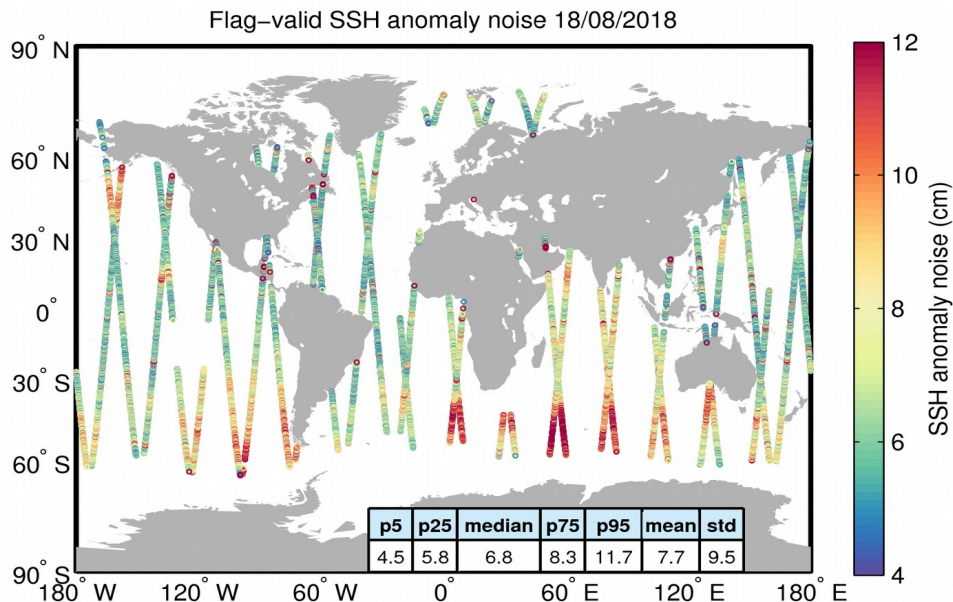
Figure 8. Geographical distribution of flag-valid 20-Hz SSH anomaly measurement noise over oceans and lakes for 18/08/2018. The statistical values shown in the table refer to the SSH anomaly noise and are calculated over all measurements shown in the figure.
