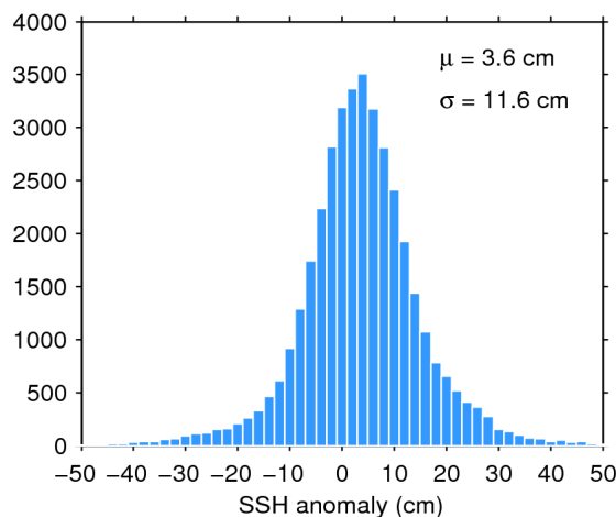
Figure 11. Histogram of science-valid SSH anomaly over oceans and lakes for 18/08/2018. The mean ( \mu ) and standard deviation ( \sigma ) are also shown. Note that values outside [-50 50] cm are excluded from the histogram for the sake of readability but not from the computation of \mu and \sigma .
