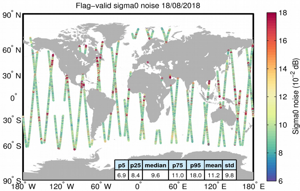
Figure 26. Geographical distribution of flag-valid 20-Hz sigma0 measurement noise over oceans and lakes for 18/08/2018. The statistical values shown in the table refer to the sigma0 noise and are calculated over all measurements shown in the figure.
