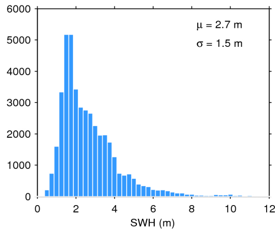
Figure 17. Histogram of flag-valid SWH over oceans and lakes for 18/08/2018. The mean ( \mu ) and standard deviation ( \sigma ) are also shown. Note that values larger than 12 m are excluded from the histogram for the sake of readability but not from the computation of \mu and \sigma .
