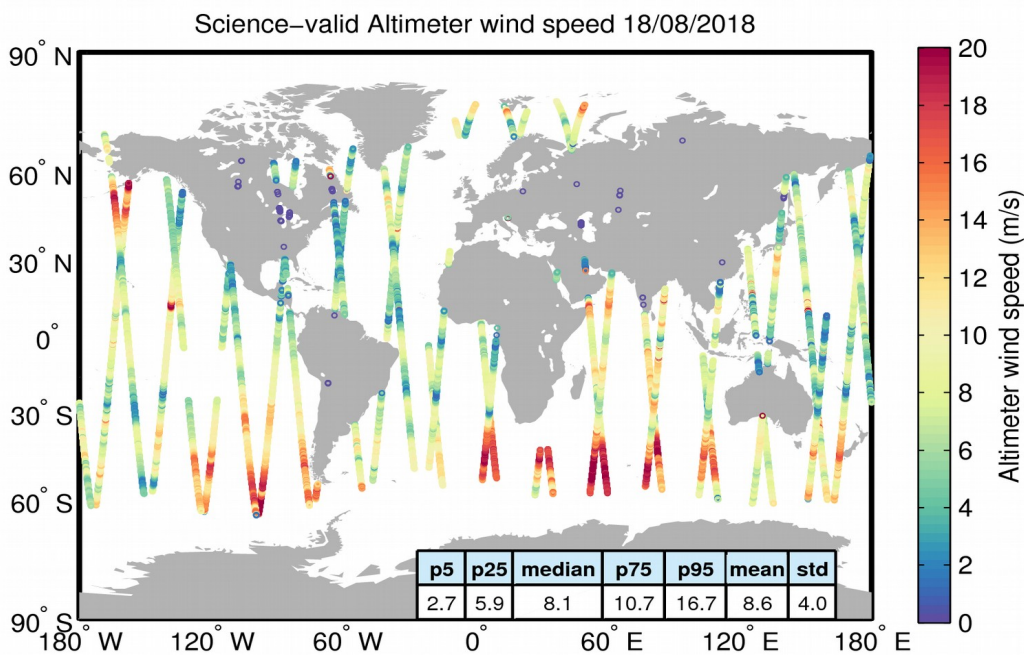
Figure 34. Geographical distribution of science-valid wind data over oceans and lakes for 18/08/2018. The statistical values shown in the table refer to the wind in m/s and are calculated over all measurements shown in the figure. Gray circles denote records that have been rejected based on the editing criteria described in Table 5.
