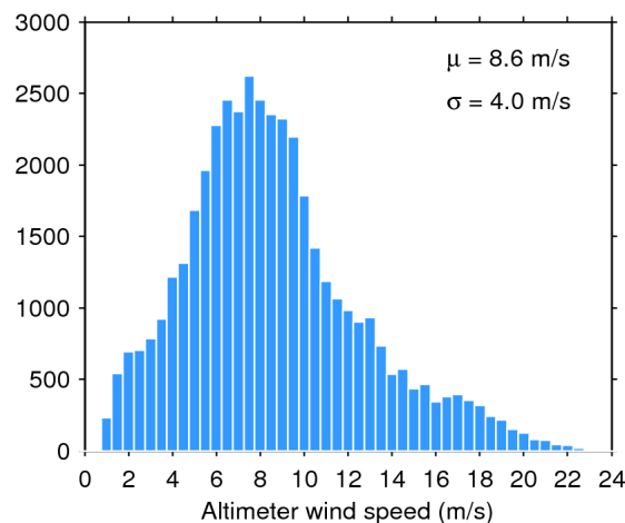
Figure 35. Histogram of science-valid wind over oceans and lakes for 18/08/2018. The mean ( \mu ) and standard deviation ( \sigma ) are also shown. Note that values larger than 24 m/s are excluded from the histogram for the sake of readability but not from the computation of \mu and \sigma .
