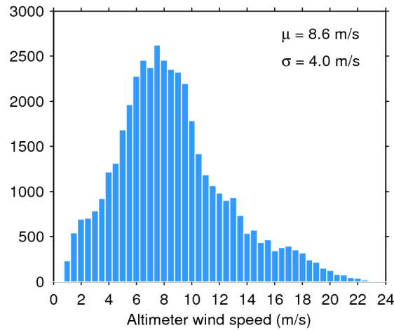
Figure 33. Histogram of flag-valid wind over oceans and lakes for 18/08/2018. The mean ( \mu ) and standard deviation ( \sigma ) are also shown. Note that values larger than 24 m/s are excluded from the histogram for the sake of readability but not from the computation of \mu and \sigma .
