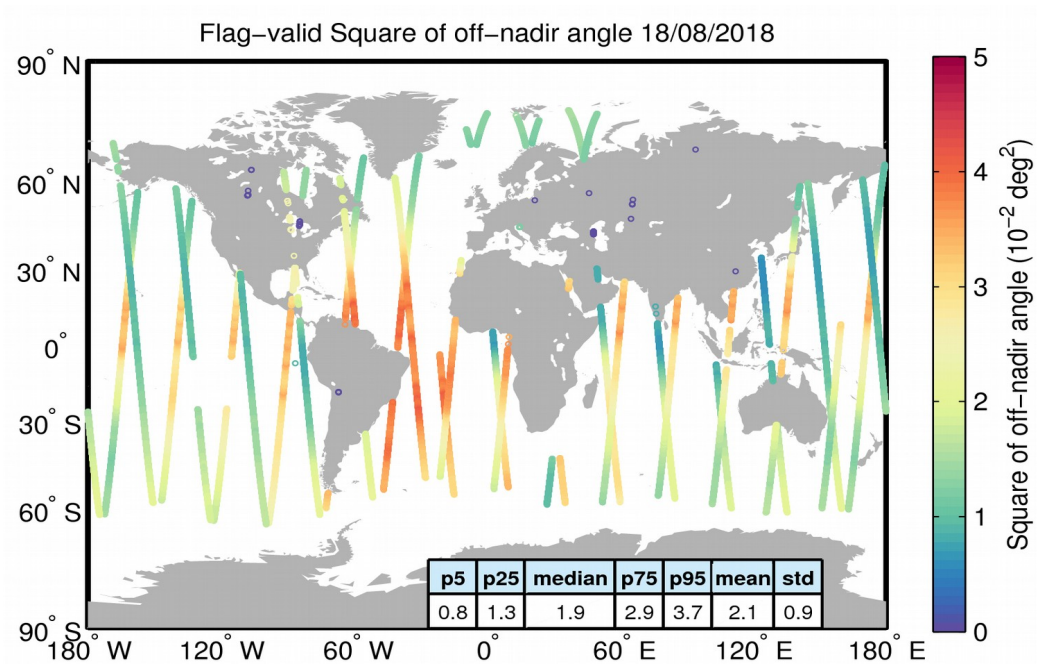
Figure 37. Geographical distribution of flag-valid mispointing data over oceans and lakes for 18/08/2018. The statistical values shown in the table refer to the mispointing in 10^{-2} deg 2 and are calculated over all measurements shown in the figure.
