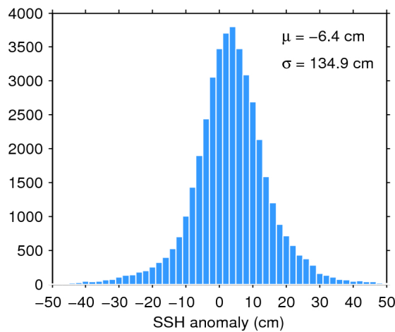
Figure 7. Histogram of flag-valid SSH anomaly over oceans and lakes for 18/08/2018. The mean ( \mu ) and standard deviation ( \sigma ) are also shown. Note that values outside [-50 50] cm are excluded from the histogram for the sake of readability but not from the computation of \mu and \sigma .
