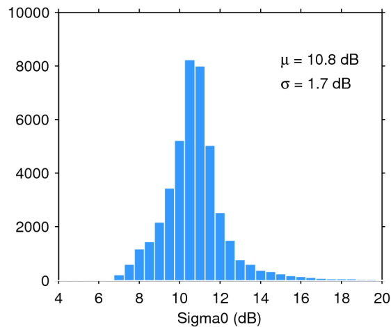
Figure 25. Histogram of flag-valid sigma0 over oceans and lakes for 18/08/2018. The mean ( \mu ) and standard deviation ( \sigma ) are also shown. Note that values outside [4 20] dB are excluded from the histogram for the sake of readability but not from the computation of \mu and \sigma .
