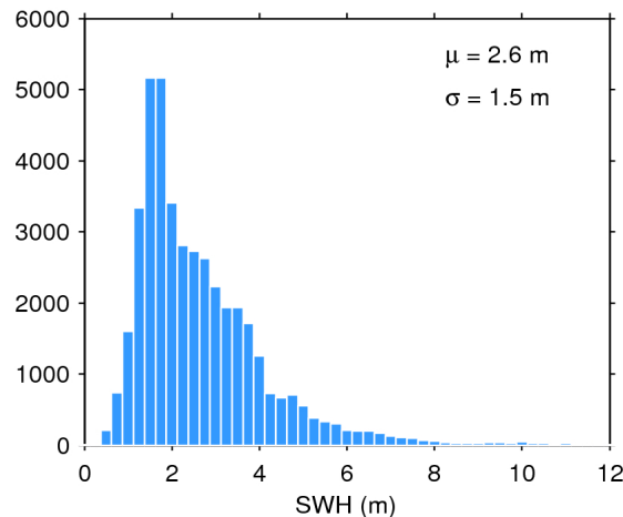
Figure 20. Histogram of science-valid SWH over oceans and lakes for 18/08/2018. The mean ( \mu ) and standard deviation ( \sigma ) are also shown. Note that values larger than 12 m are excluded from the histogram for the sake of readability but not from the computation of \mu and \sigma .
