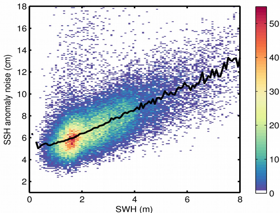
Figure 9. 2D histogram showing flag-valid SSH anomaly noise as a function of SWH for 18/08/2018. The black line denotes the median SSH anomaly noise as a function of SWH.
