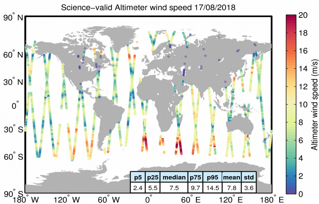
Figure 34. Geographical distribution of science-valid wind data over oceans and lakes for 17/08/2018. The statistical values shown in the table refer to the wind in m/s and are calculated over all measurements shown in the figure. Gray circles denote records that have been rejected based on the editing criteria described in Table 5.
