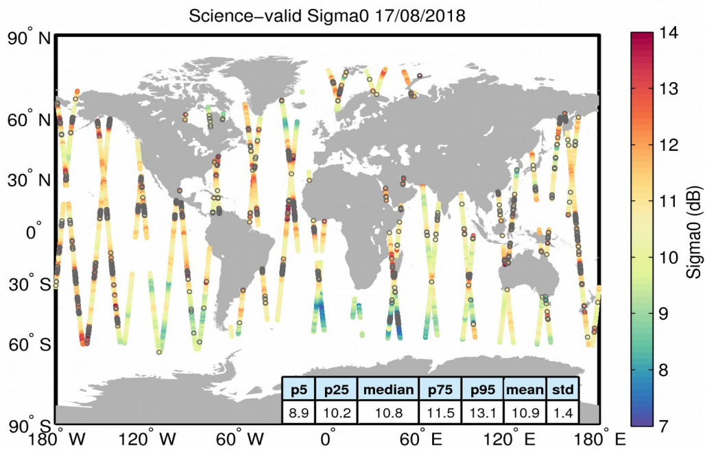
Figure 27. Geographical distribution of science-valid sigma0 data over oceans and lakes for 17/08/2018. The statistical values shown in the table refer to the sigma0 in dB and are calculated over all measurements shown in the figure. Gray circles denote records that have been rejected based on the editing criteria described in Table 4.
