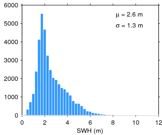
Figure 17. Histogram of flag-valid SWH over oceans and lakes for 17/08/2018. The mean ( \mu ) and standard deviation ( \sigma ) are also shown. Note that values larger than 12 m are excluded from the histogram for the sake of readability but not from the computation of \mu and \sigma .
