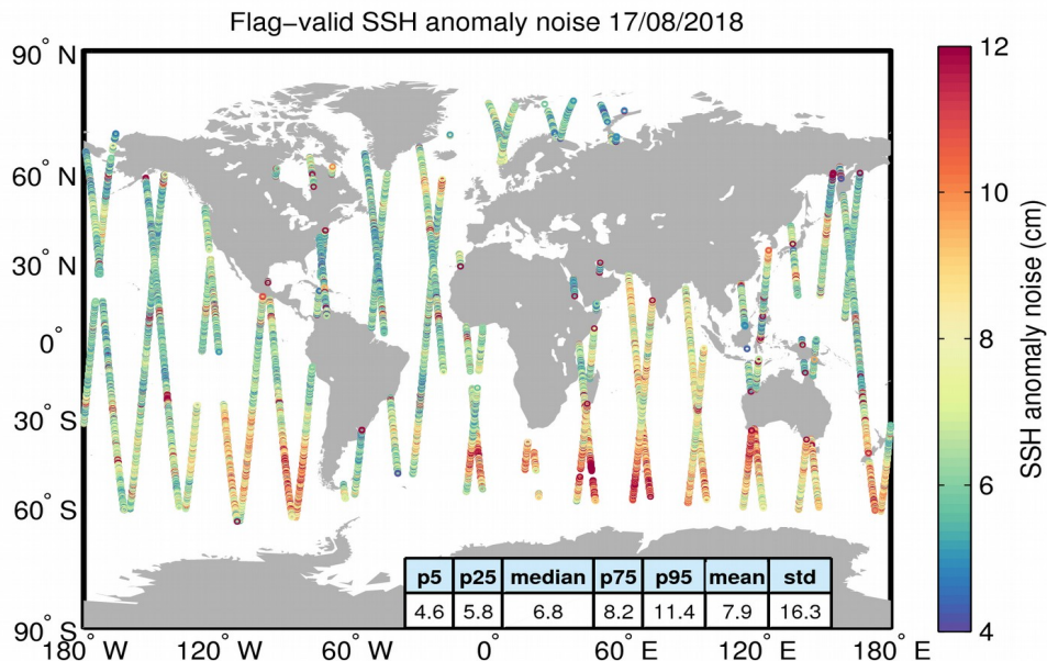
Figure 8. Geographical distribution of flag-valid 20-Hz SSH anomaly measurement noise over oceans and lakes for 17/08/2018. The statistical values shown in the table refer to the SSH anomaly noise and are calculated over all measurements shown in the figure.
