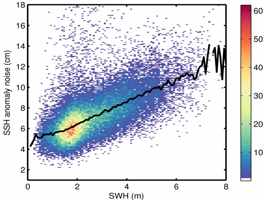
Figure 9. 2D histogram showing flag-valid SSH anomaly noise as a function of SWH for 17/08/2018. The black line denotes the median SSH anomaly noise as a function of SWH.
