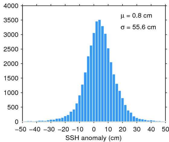
Figure 7. Histogram of flag-valid SSH anomaly over oceans and lakes for 17/08/2018. The mean ( \mu ) and standard deviation ( \sigma ) are also shown. Note that values outside [-50 50] cm are excluded from the histogram for the sake of readability but not from the computation of \mu and \sigma .
