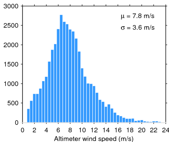
Figure 35. Histogram of science-valid wind over oceans and lakes for 17/08/2018. The mean ( \mu ) and standard deviation ( \sigma ) are also shown. Note that values larger than 24 m/s are excluded from the histogram for the sake of readability but not from the computation of \mu and \sigma .
