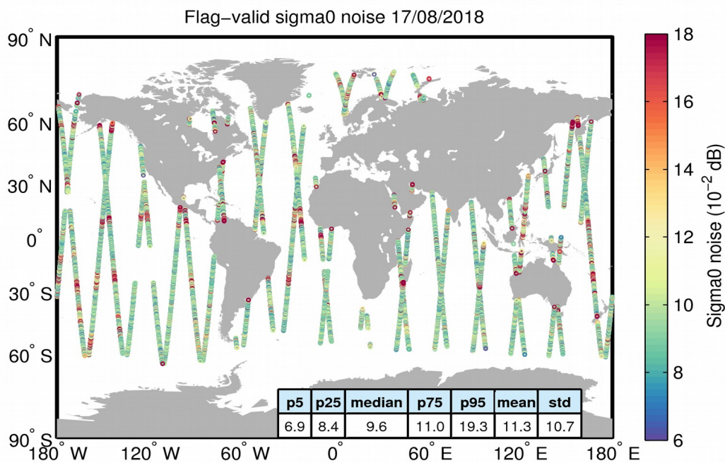
Figure 26. Geographical distribution of flag-valid 20-Hz sigma0 measurement noise over oceans and lakes for 17/08/2018. The statistical values shown in the table refer to the sigma0 noise and are calculated over all measurements shown in the figure.
