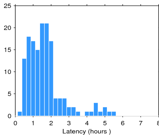
Figure 2. Histogram of the data latency for 17/08/2018. The y-axis denotes the number of files that are made available with a delay of x-hours with respect to the mean time of the records stored in the file.
