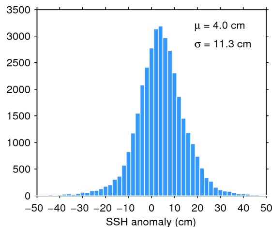
Figure 11. Histogram of science-valid SSH anomaly over oceans and lakes for 17/08/2018. The mean ( \mu ) and standard deviation ( \sigma ) are also shown. Note that values outside [-50 50] cm are excluded from the histogram for the sake of readability but not from the computation of \mu and \sigma .
