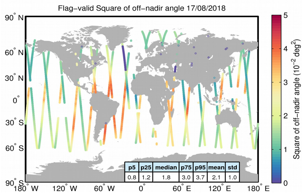
Figure 37. Geographical distribution of flag-valid mispointing data over oceans and lakes for 17/08/2018. The statistical values shown in the table refer to the mispointing in 10^{-2} \text{ deg}^2 and are calculated over all measurements shown in the figure.
