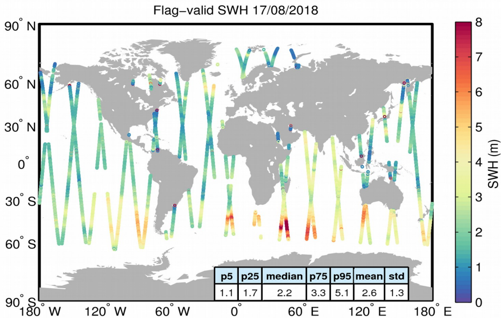
Figure 15. Geographical distribution of flag-valid SWH data over oceans and lakes for 17/08/2018. The statistical values shown in the table refer to the SWH in m and are calculated over all measurements shown in the figure.
