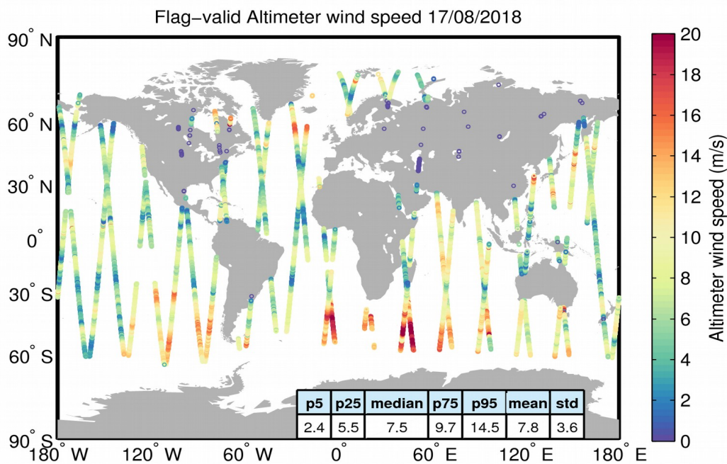
Figure 31. Geographical distribution of flag-valid wind data over oceans and lakes for 17/08/2018. The statistical values shown in the table refer to the wind in m/s and are calculated over all measurements shown in the figure.
