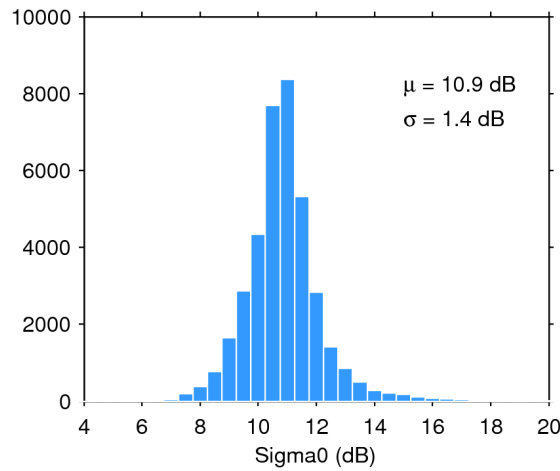
Figure 28. Histogram of science-valid sigma0 over oceans and lakes for 17/08/2018. The mean ( \mu ) and standard deviation ( \sigma ) are also shown. Note that values outside [4 20] dB are excluded from the histogram for the sake of readability but not from the computation of \mu and \sigma .
