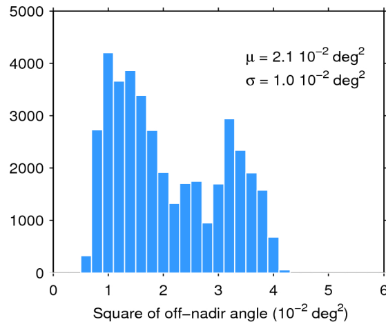
Figure 39. Histogram of flag-valid mispointing over oceans and lakes for 17/08/2018. The mean ( \mu ) and standard deviation ( \sigma ) are also shown. Note that values larger than 6 \cdot 10^{-2} \text{ deg}^2 are excluded from the histogram for the sake of readability but not from the computation of \mu and \sigma .
