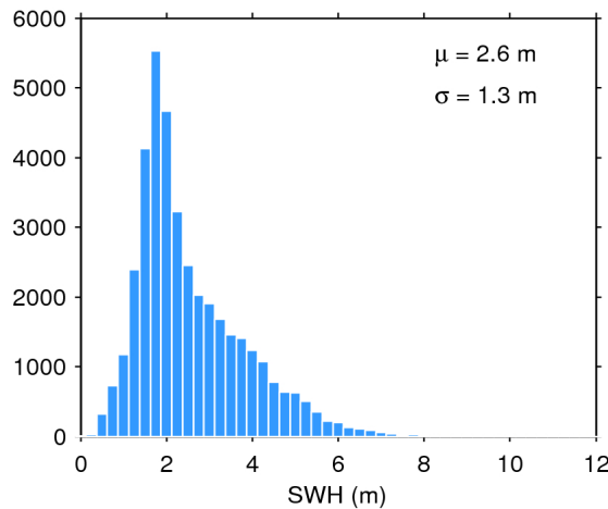
Figure 20. Histogram of science-valid SWH over oceans and lakes for 17/08/2018. The mean ( \mu ) and standard deviation ( \sigma ) are also shown. Note that values larger than 12 m are excluded from the histogram for the sake of readability but not from the computation of \mu and \sigma .
