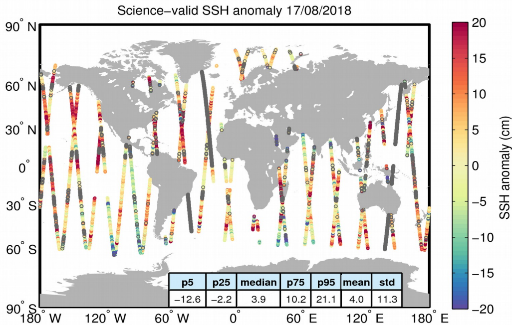
Figure 10. Geographical distribution of science-valid SSH anomaly data over oceans and lakes for 17/08/2018. The statistical values shown in the table refer to the SSH anomaly in cm and are calculated over all measurements shown in the figure. Gray circles denote records that have been rejected based on the editing criteria described in Table 2.
