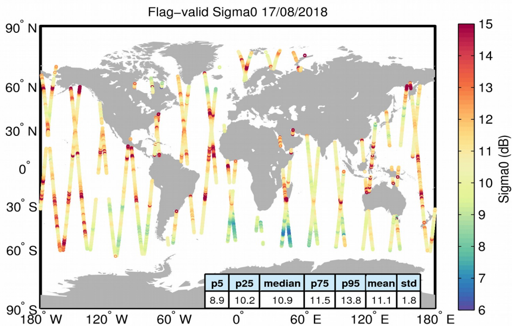
Figure 23. Geographical distribution of flag-valid sigma0 data over oceans and lakes for 17/08/2018. The statistical values shown in the table refer to the sigma0 in dB and are calculated over all measurements shown in the figure.
