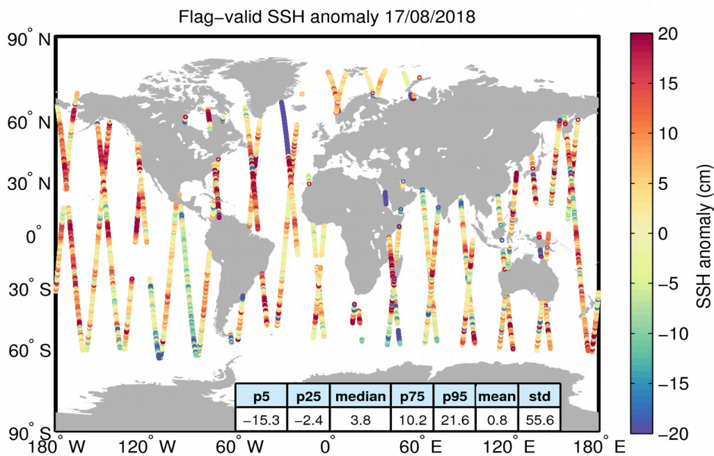
Figure 5. Geographical distribution of flag-valid 1-Hz SSH anomaly data over oceans and lakes for 17/08/2018. The statistical values shown in the table refer to the SSH anomaly in cm and are calculated over all measurements shown in the figure.
