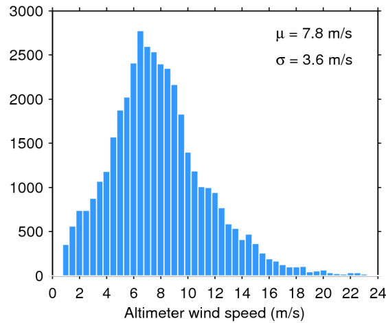
Figure 33. Histogram of flag-valid wind over oceans and lakes for 17/08/2018. The mean ( \mu ) and standard deviation ( \sigma ) are also shown. Note that values larger than 24 m/s are excluded from the histogram for the sake of readability but not from the computation of \mu and \sigma .
