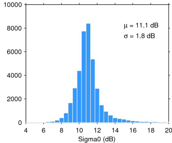
Figure 25. Histogram of flag-valid sigma0 over oceans and lakes for 17/08/2018. The mean ( \mu ) and standard deviation ( \sigma ) are also shown. Note that values outside [4 20] dB are excluded from the histogram for the sake of readability but not from the computation of \mu and \sigma .
