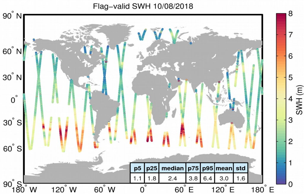
Figure 15. Geographical distribution of flag-valid SWH data over oceans and lakes for 10/08/2018. The statistical values shown in the table refer to the SWH in m and are calculated over all measurements shown in the figure.
