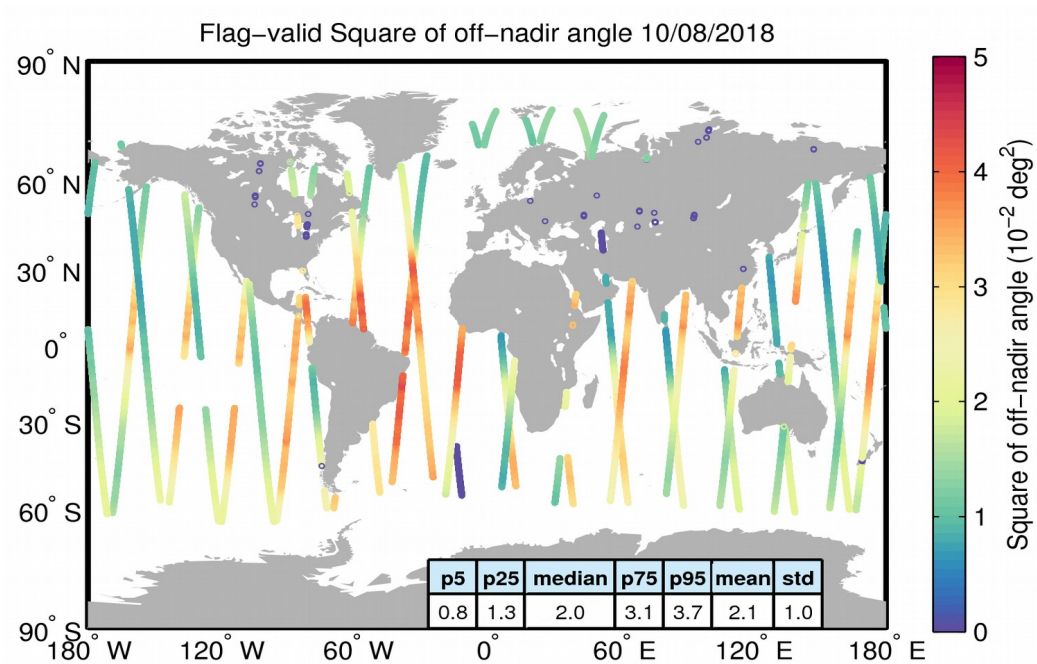
Figure 37. Geographical distribution of flag-valid mispointing data over oceans and lakes for 10/08/2018. The statistical values shown in the table refer to the mispointing in 10^{-2} \text{deg}^2 and are calculated over all measurements shown in the figure.
