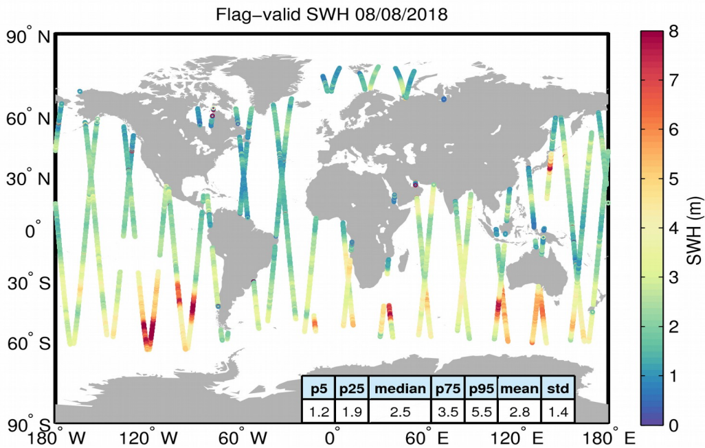
Figure 15. Geographical distribution of flag-valid SWH data over oceans and lakes for 08/08/2018. The statistical values shown in the table refer to the SWH in m and are calculated over all measurements shown in the figure.
