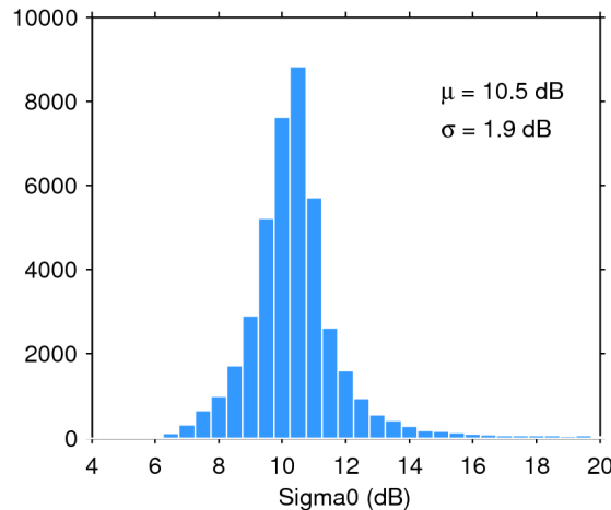
Figure 25. Histogram of flag-valid sigma0 over oceans and lakes for 08/08/2018. The mean ( \mu ) and standard deviation ( \sigma ) are also shown. Note that values outside [4 20] dB are excluded from the histogram for the sake of readability but not from the computation of \mu and \sigma .
