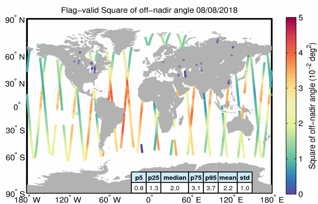
Figure 37. Geographical distribution of flag-valid mispointing data over oceans and lakes for 08/08/2018. The statistical values shown in the table refer to the mispointing in 10^{-2} \text{deg}^2 and are calculated over all measurements shown in the figure.
