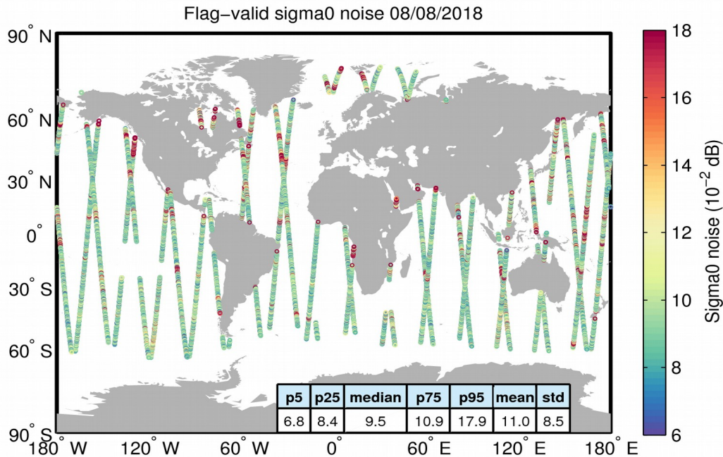
Figure 26. Geographical distribution of flag-valid 20-Hz sigma0 measurement noise over oceans and lakes for 08/08/2018. The statistical values shown in the table refer to the sigma0 noise and are calculated over all measurements shown in the figure.
