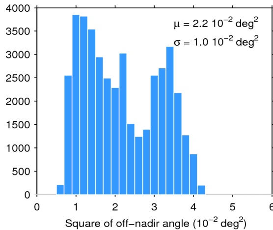
Figure 39. Histogram of flag-valid mispointing over oceans and lakes for 08/08/2018. The mean ( \mu ) and standard deviation ( \sigma ) are also shown. Note that values larger than 6 \cdot 10^{-2} \text{ deg}^2 are excluded from the histogram for the sake of readability but not from the computation of \mu and \sigma .
