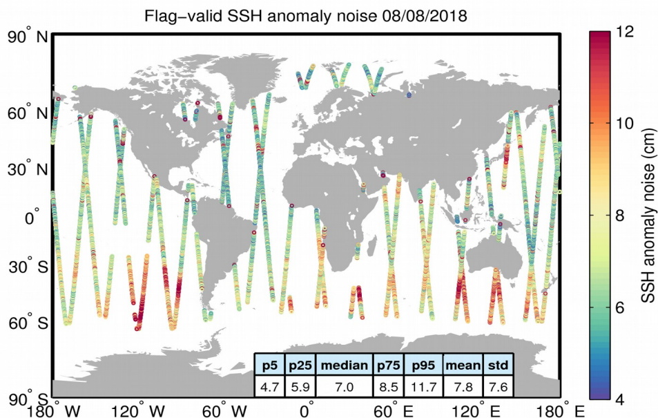
Figure 8. Geographical distribution of flag-valid 20-Hz SSH anomaly measurement noise over oceans and lakes for 08/08/2018. The statistical values shown in the table refer to the SSH anomaly noise and are calculated over all measurements shown in the figure.
