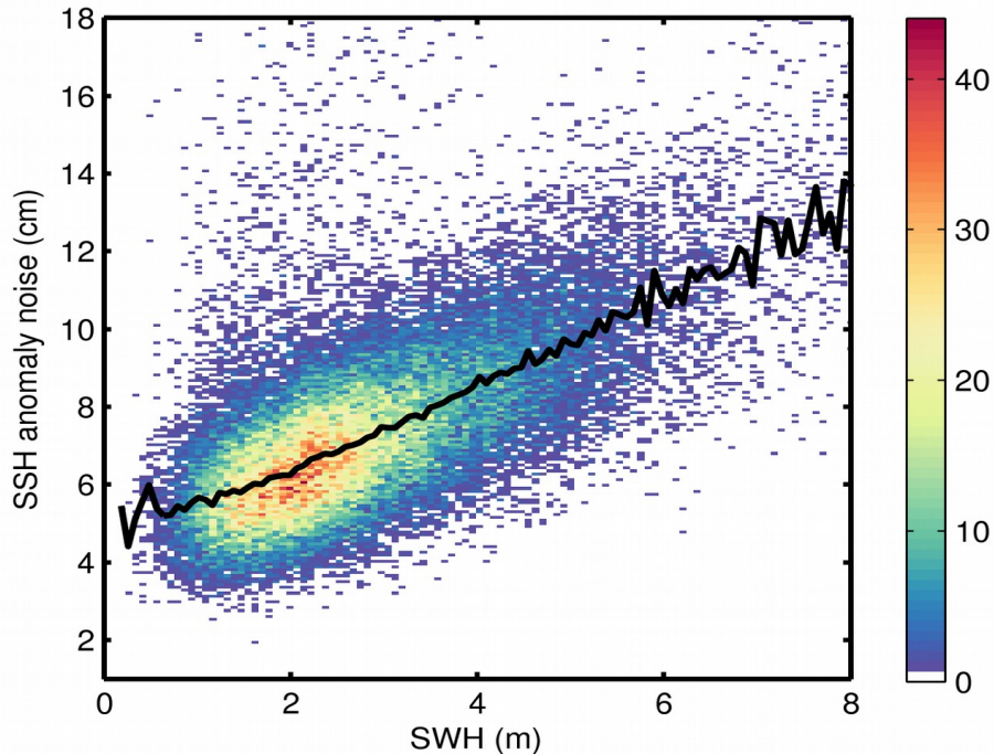
Figure 9. 2D histogram showing flag-valid SSH anomaly noise as a function of SWH for 08/08/2018. The black line denotes the median SSH anomaly noise as a function of SWH.
