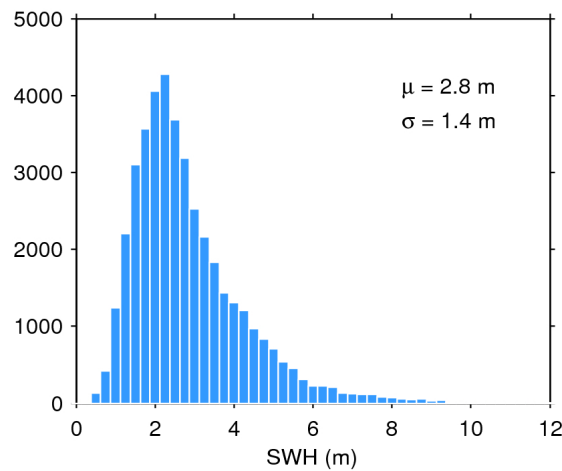
Figure 17. Histogram of flag-valid SWH over oceans and lakes for 08/08/2018. The mean ( \mu ) and standard deviation ( \sigma ) are also shown. Note that values larger than 12 m are excluded from the histogram for the sake of readability but not from the computation of \mu and \sigma .
