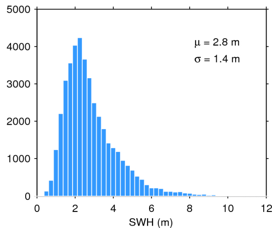
Figure 20. Histogram of science-valid SWH over oceans and lakes for 08/08/2018. The mean ( \mu ) and standard deviation ( \sigma ) are also shown. Note that values larger than 12 m are excluded from the histogram for the sake of readability but not from the computation of \mu and \sigma .
