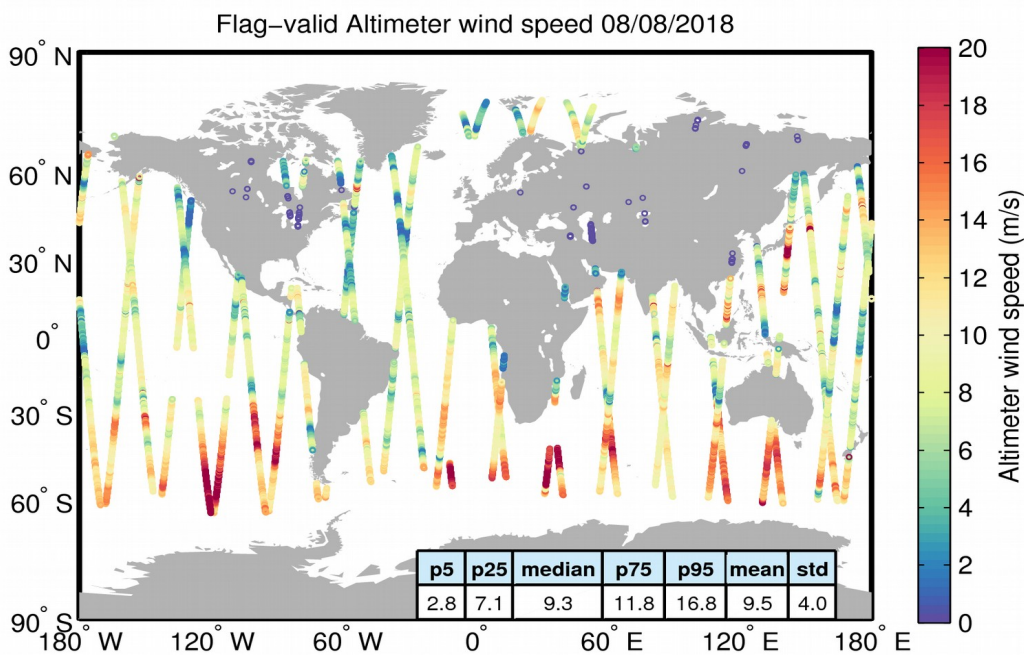
Figure 31. Geographical distribution of flag-valid wind data over oceans and lakes for 08/08/2018. The statistical values shown in the table refer to the wind in m/s and are calculated over all measurements shown in the figure.
