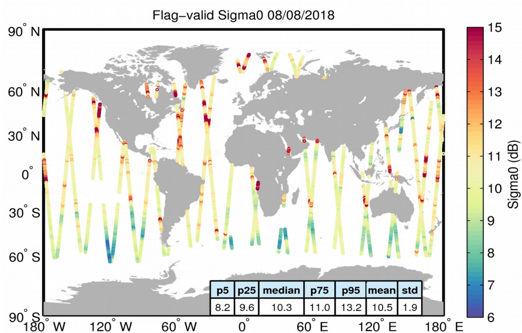
Figure 23. Geographical distribution of flag-valid sigma0 data over oceans and lakes for 08/08/2018. The statistical values shown in the table refer to the sigma0 in dB and are calculated over all measurements shown in the figure.
