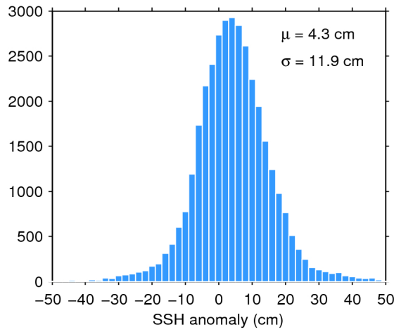
Figure 11. Histogram of science-valid SSH anomaly over oceans and lakes for 08/08/2018. The mean ( \mu ) and standard deviation ( \sigma ) are also shown. Note that values outside [-50 50] cm are excluded from the histogram for the sake of readability but not from the computation of \mu and \sigma .
