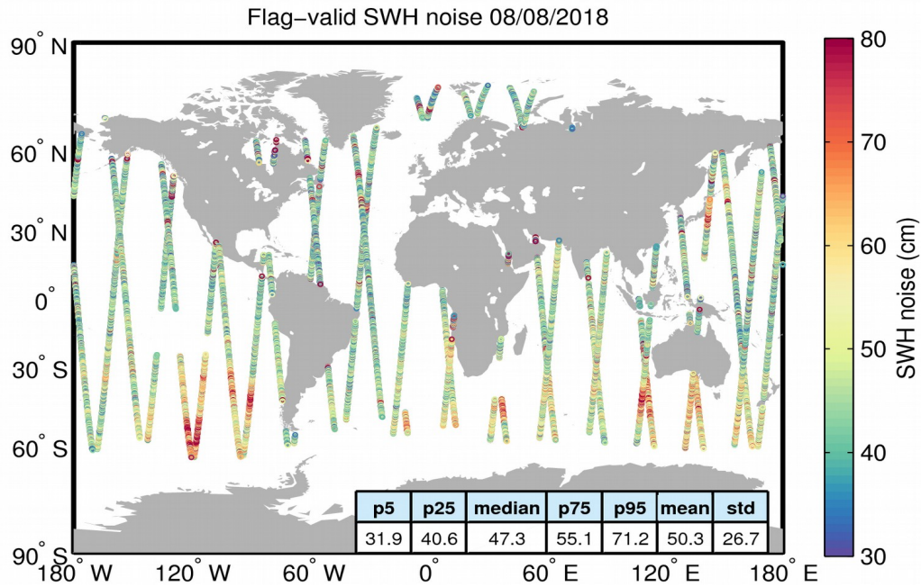
Figure 18. Geographical distribution of flag-valid 20-Hz SWH measurement noise over oceans and lakes for 08/08/2018. The statistical values shown in the figure refer to the SWH noise and are calculated over all measurements shown in the figure.
