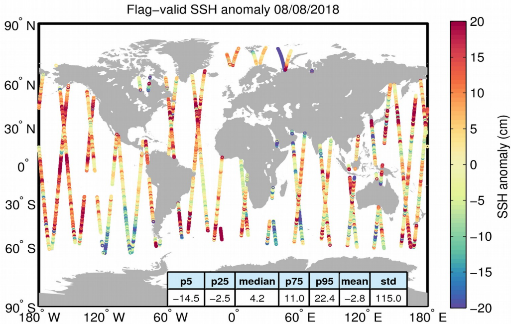
Figure 5. Geographical distribution of flag-valid 1-Hz SSH anomaly data over oceans and lakes for 08/08/2018. The statistical values shown in the table refer to the SSH anomaly in cm and are calculated over all measurements shown in the figure.
