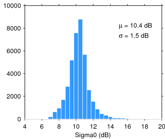
Figure 28. Histogram of science-valid sigma0 over oceans and lakes for 08/08/2018. The mean ( \mu ) and standard deviation ( \sigma ) are also shown. Note that values outside [4 20] dB are excluded from the histogram for the sake of readability but not from the computation of \mu and \sigma .
