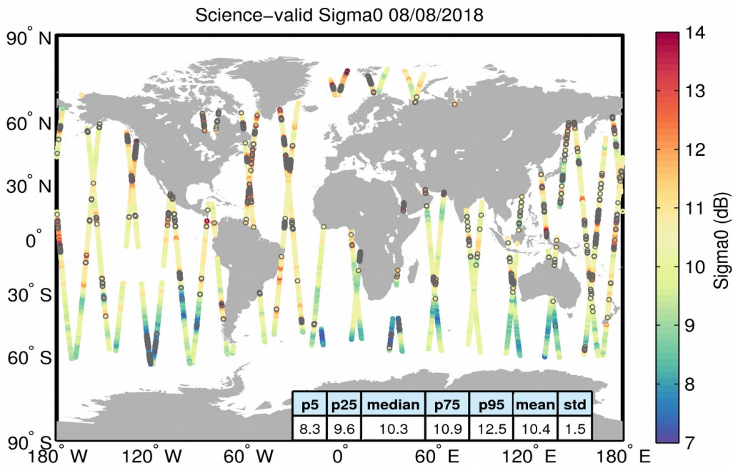
Figure 27. Geographical distribution of science-valid sigma0 data over oceans and lakes for 08/08/2018. The statistical values shown in the table refer to the sigma0 in dB and are calculated over all measurements shown in the figure. Gray circles denote records that have been rejected based on the editing criteria described in Table 4.
