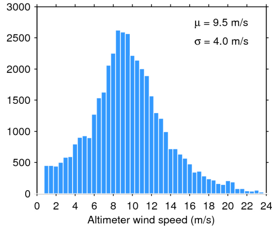
Figure 33. Histogram of flag-valid wind over oceans and lakes for 08/08/2018. The mean ( \mu ) and standard deviation ( \sigma ) are also shown. Note that values larger than 24 m/s are excluded from the histogram for the sake of readability but not from the computation of \mu and \sigma .
