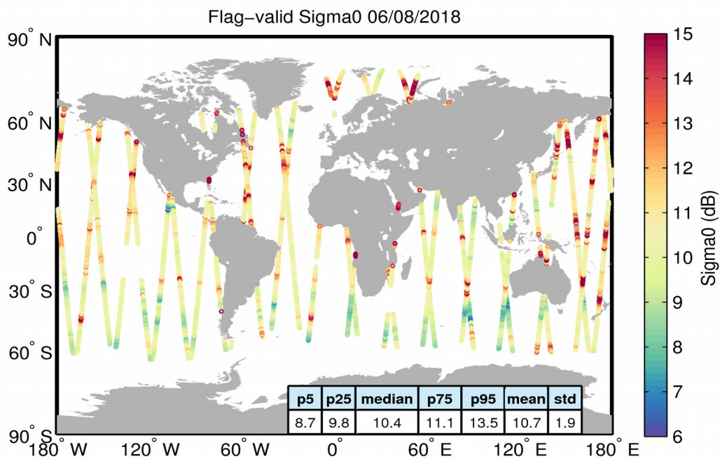
Figure 23. Geographical distribution of flag-valid sigma0 data over oceans and lakes for 06/08/2018. The statistical values shown in the table refer to the sigma0 in dB and are calculated over all measurements shown in the figure.
