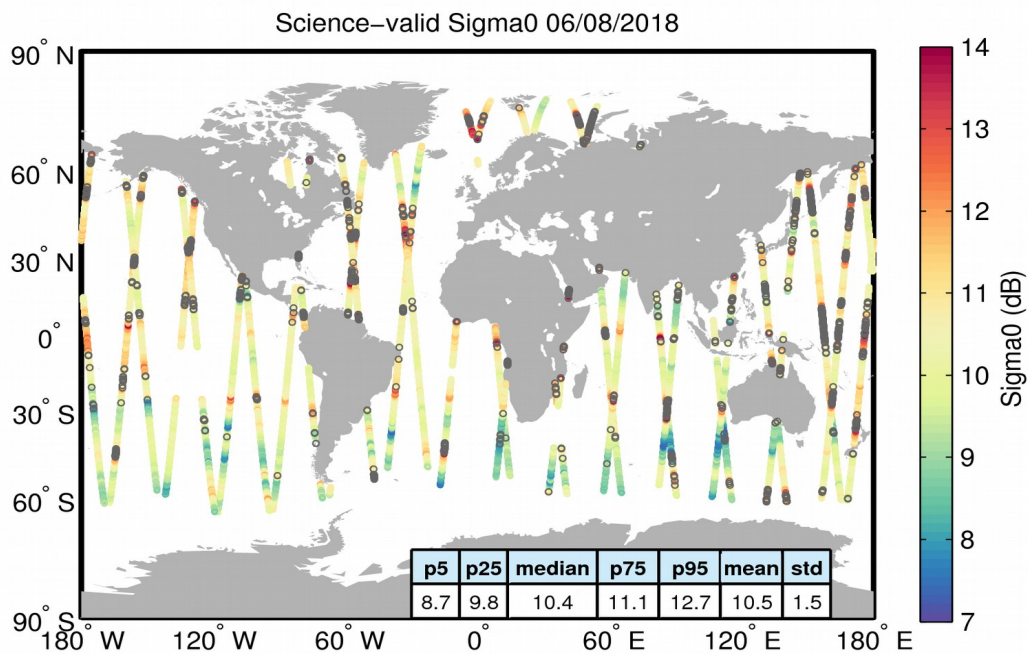
Figure 27. Geographical distribution of science-valid sigma0 data over oceans and lakes for 06/08/2018. The statistical values shown in the table refer to the sigma0 in dB and are calculated over all measurements shown in the figure. Gray circles denote records that have been rejected based on the editing criteria described in Table 4.
