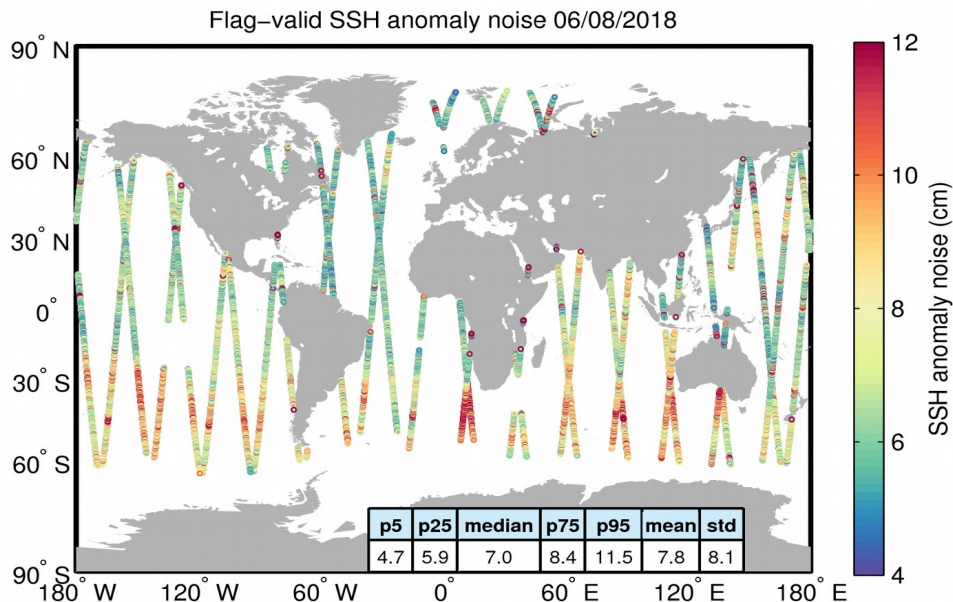
Figure 8. Geographical distribution of flag-valid 20-Hz SSH anomaly measurement noise over oceans and lakes for 06/08/2018. The statistical values shown in the table refer to the SSH anomaly noise and are calculated over all measurements shown in the figure.
