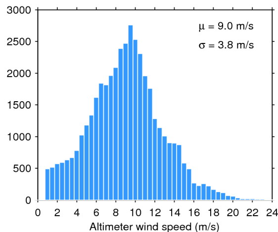
Figure 35. Histogram of science-valid wind over oceans and lakes for 06/08/2018. The mean ( \mu ) and standard deviation ( \sigma ) are also shown. Note that values larger than 24 m/s are excluded from the histogram for the sake of readability but not from the computation of \mu and \sigma .
