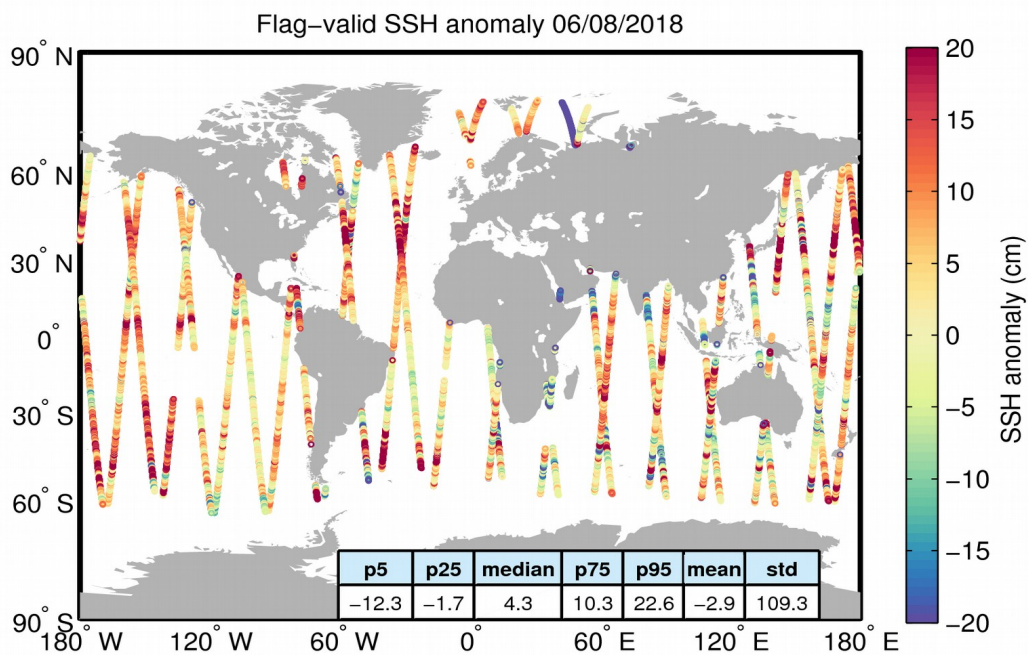
Figure 5. Geographical distribution of flag-valid 1-Hz SSH anomaly data over oceans and lakes for 06/08/2018. The statistical values shown in the table refer to the SSH anomaly in cm and are calculated over all measurements shown in the figure.
