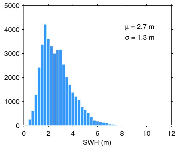
Figure 17. Histogram of flag-valid SWH over oceans and lakes for 06/08/2018. The mean ( \mu ) and standard deviation ( \sigma ) are also shown. Note that values larger than 12 m are excluded from the histogram for the sake of readability but not from the computation of \mu and \sigma .
