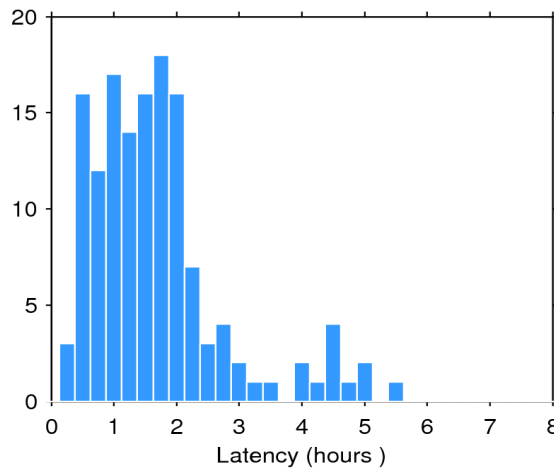
Figure 2. Histogram of the data latency for 06/08/2018. The y-axis denotes the number of files that are made available with a delay of x-hours with respect to the mean time of the records stored in the file.
