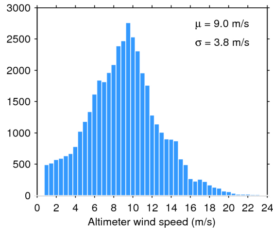
Figure 33. Histogram of flag-valid wind over oceans and lakes for 06/08/2018. The mean ( \mu ) and standard deviation ( \sigma ) are also shown. Note that values larger than 24 m/s are excluded from the histogram for the sake of readability but not from the computation of \mu and \sigma .
