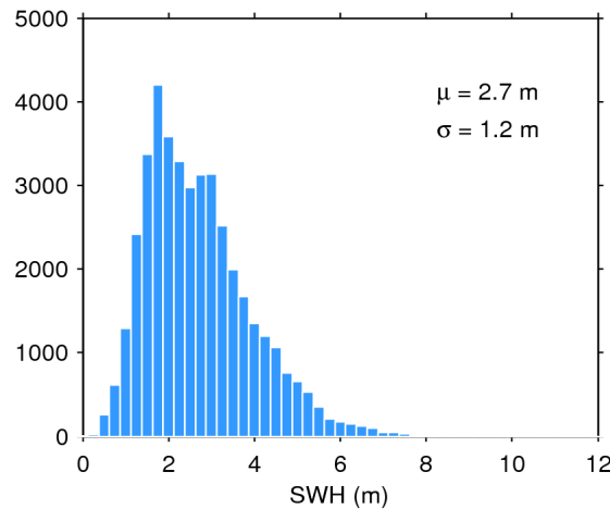
Figure 20. Histogram of science-valid SWH over oceans and lakes for 06/08/2018. The mean ( \mu ) and standard deviation ( \sigma ) are also shown. Note that values larger than 12 m are excluded from the histogram for the sake of readability but not from the computation of \mu and \sigma .
