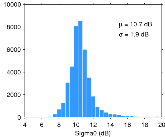
Figure 25. Histogram of flag-valid sigma0 over oceans and lakes for 06/08/2018. The mean ( \mu ) and standard deviation ( \sigma ) are also shown. Note that values outside [4 20] dB are excluded from the histogram for the sake of readability but not from the computation of \mu and \sigma .
