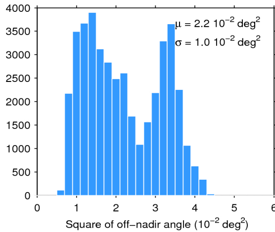
Figure 39. Histogram of flag-valid mispointing over oceans and lakes for 06/08/2018. The mean ( \mu ) and standard deviation ( \sigma ) are also shown. Note that values larger than 6 \cdot 10^{-2} \text{ deg}^2 are excluded from the histogram for the sake of readability but not from the computation of \mu and \sigma .
