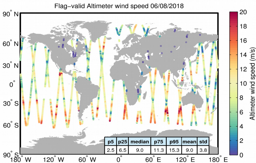
Figure 31. Geographical distribution of flag-valid wind data over oceans and lakes for 06/08/2018. The statistical values shown in the table refer to the wind in m/s and are calculated over all measurements shown in the figure.
