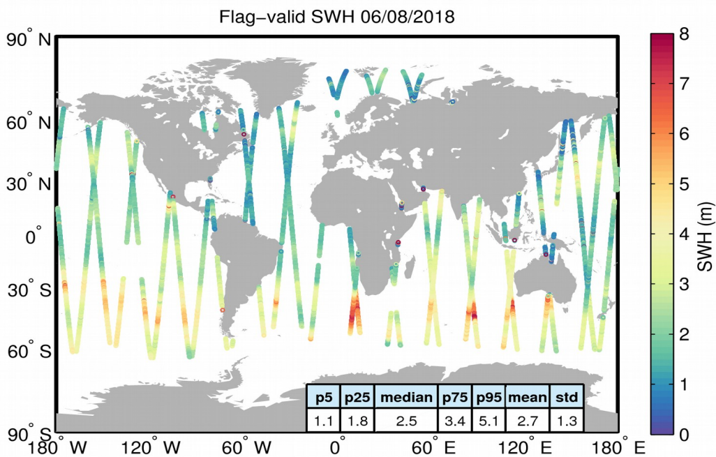
Figure 15. Geographical distribution of flag-valid SWH data over oceans and lakes for 06/08/2018. The statistical values shown in the table refer to the SWH in m and are calculated over all measurements shown in the figure.
