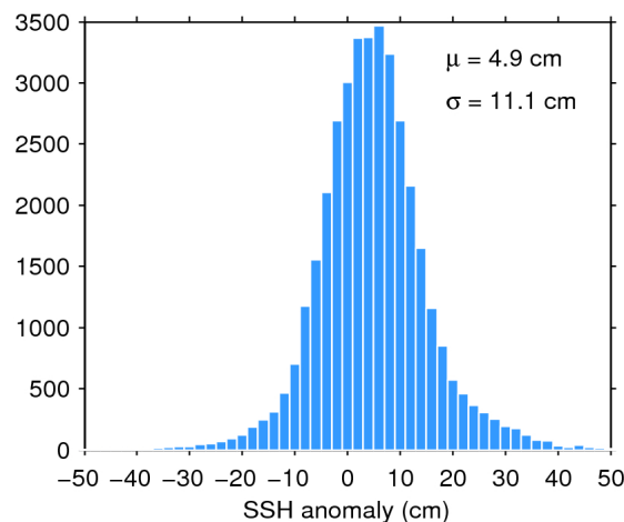
Figure 11. Histogram of science-valid SSH anomaly over oceans and lakes for 06/08/2018. The mean ( \mu ) and standard deviation ( \sigma ) are also shown. Note that values outside [-50 50] cm are excluded from the histogram for the sake of readability but not from the computation of \mu and \sigma .
