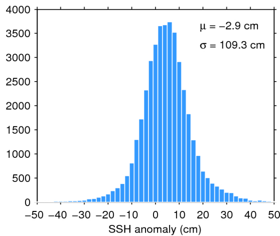
Figure 7. Histogram of flag-valid SSH anomaly over oceans and lakes for 06/08/2018. The mean ( \mu ) and standard deviation ( \sigma ) are also shown. Note that values outside [-50\ 50] cm are excluded from the histogram for the sake of readability but not from the computation of \mu and \sigma .
