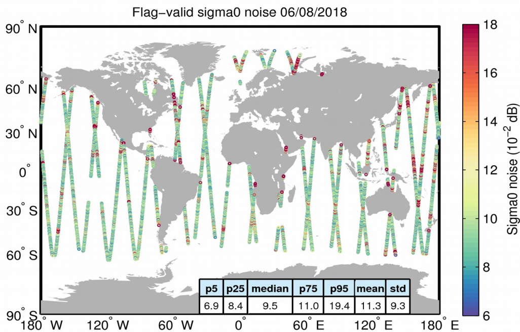
Figure 26. Geographical distribution of flag-valid 20-Hz sigma0 measurement noise over oceans and lakes for 06/08/2018. The statistical values shown in the table refer to the sigma0 noise and are calculated over all measurements shown in the figure.
