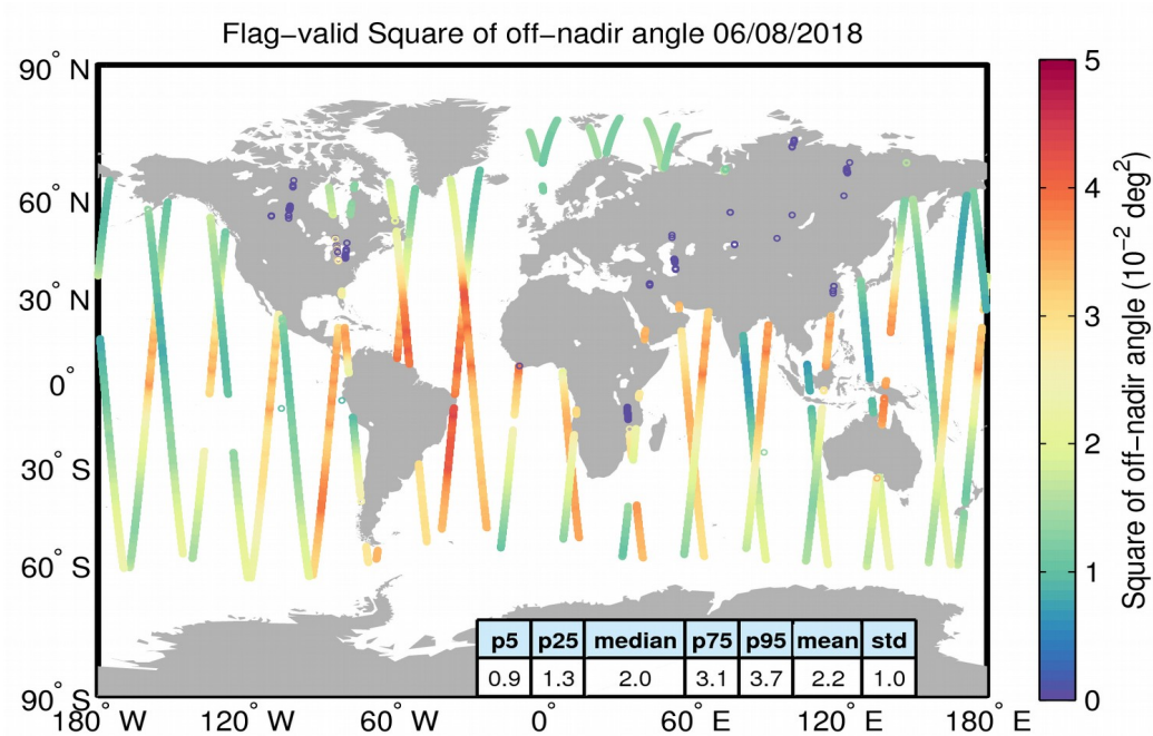
Figure 37. Geographical distribution of flag-valid mispointing data over oceans and lakes for 06/08/2018. The statistical values shown in the table refer to the mispointing in 10^{-2} \text{ deg}^2 and are calculated over all measurements shown in the figure.
