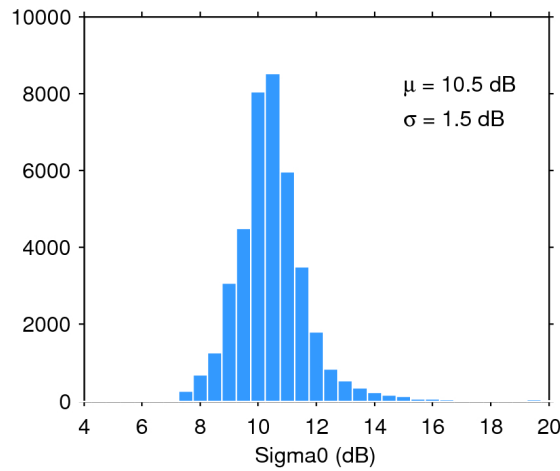
Figure 28. Histogram of science-valid sigma0 over oceans and lakes for 06/08/2018. The mean ( \mu ) and standard deviation ( \sigma ) are also shown. Note that values outside [4 20] dB are excluded from the histogram for the sake of readability but not from the computation of \mu and \sigma .
