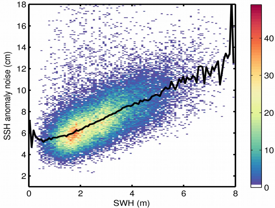
Figure 9. 2D histogram showing flag-valid SSH anomaly noise as a function of SWH for 06/08/2018. The black line denotes the median SSH anomaly noise as a function of SWH.
