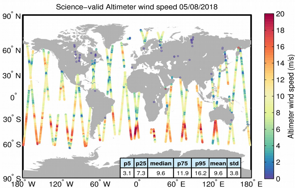
Figure 34. Geographical distribution of science-valid wind data over oceans and lakes for 05/08/2018. The statistical values shown in the table refer to the wind in m/s and are calculated over all measurements shown in the figure. Gray circles denote records that have been rejected based on the editing criteria described in Table 5.
