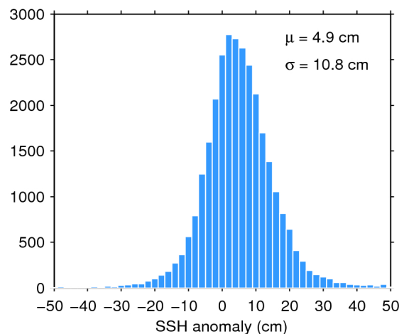
Figure 11. Histogram of science-valid SSH anomaly over oceans and lakes for 05/08/2018. The mean ( \mu ) and standard deviation ( \sigma ) are also shown. Note that values outside [-50 50] cm are excluded from the histogram for the sake of readability but not from the computation of \mu and \sigma .
