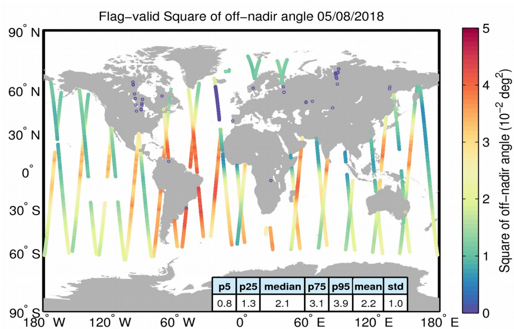
Figure 37. Geographical distribution of flag-valid mispointing data over oceans and lakes for 05/08/2018. The statistical values shown in the table refer to the mispointing in 10^{-2} \text{ deg}^2 and are calculated over all measurements shown in the figure.
