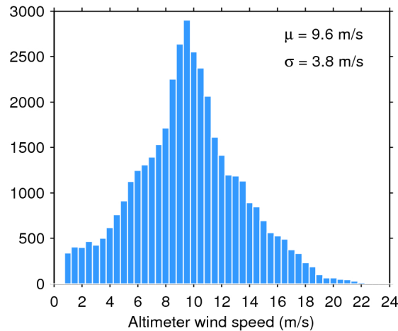
Figure 33. Histogram of flag-valid wind over oceans and lakes for 05/08/2018. The mean ( \mu ) and standard deviation ( \sigma ) are also shown. Note that values larger than 24 m/s are excluded from the histogram for the sake of readability but not from the computation of \mu and \sigma .
