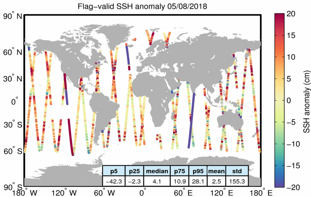
Figure 5. Geographical distribution of flag-valid 1-Hz SSH anomaly data over oceans and lakes for 05/08/2018. The statistical values shown in the table refer to the SSH anomaly in cm and are calculated over all measurements shown in the figure.
