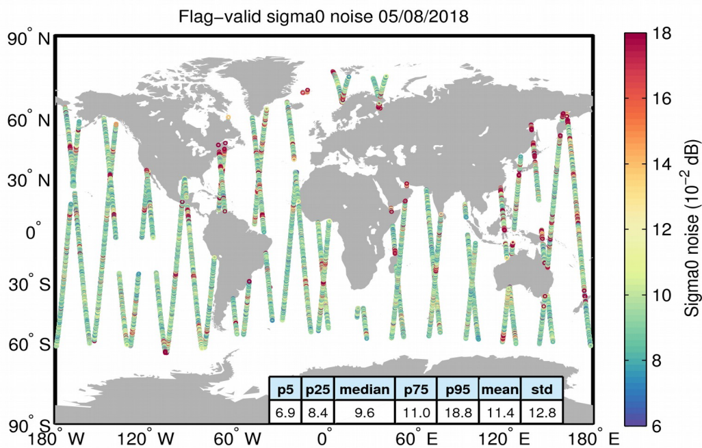
Figure 26. Geographical distribution of flag-valid 20-Hz sigma0 measurement noise over oceans and lakes for 05/08/2018. The statistical values shown in the table refer to the sigma0 noise and are calculated over all measurements shown in the figure.
