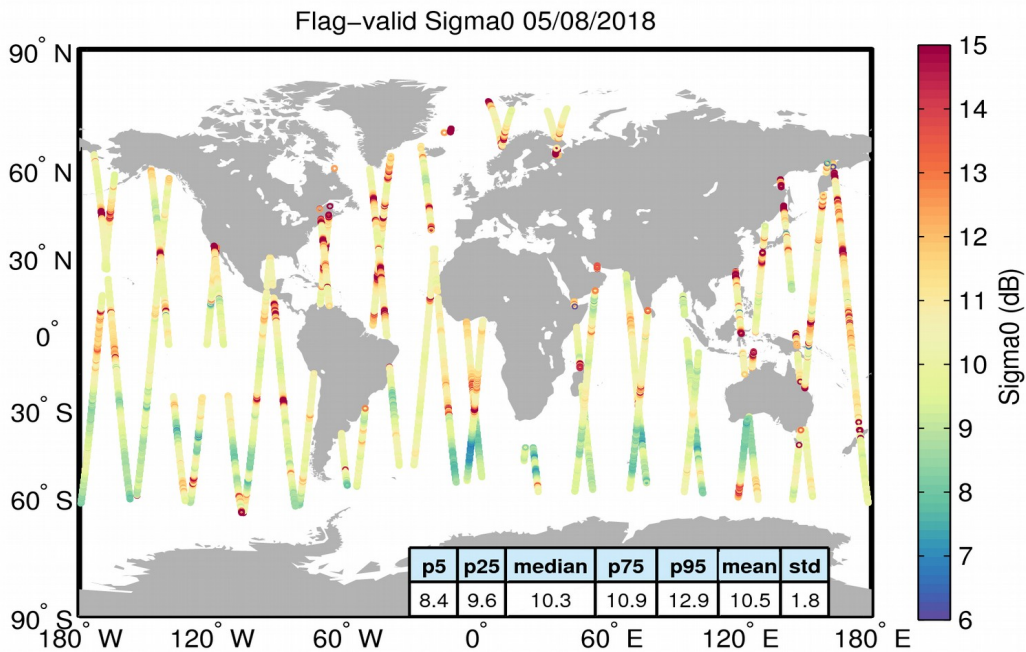
Figure 23. Geographical distribution of flag-valid sigma0 data over oceans and lakes for 05/08/2018. The statistical values shown in the table refer to the sigma0 in dB and are calculated over all measurements shown in the figure.
