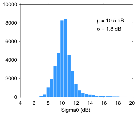
Figure 25. Histogram of flag-valid sigma0 over oceans and lakes for 05/08/2018. The mean ( \mu ) and standard deviation ( \sigma ) are also shown. Note that values outside [4 20] dB are excluded from the histogram for the sake of readability but not from the computation of \mu and \sigma .
