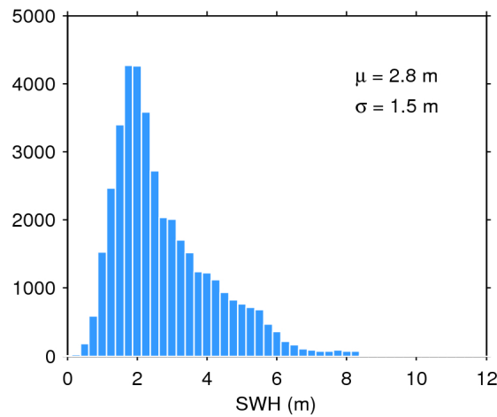
Figure 17. Histogram of flag-valid SWH over oceans and lakes for 05/08/2018. The mean ( \mu ) and standard deviation ( \sigma ) are also shown. Note that values larger than 12 m are excluded from the histogram for the sake of readability but not from the computation of \mu and \sigma .
