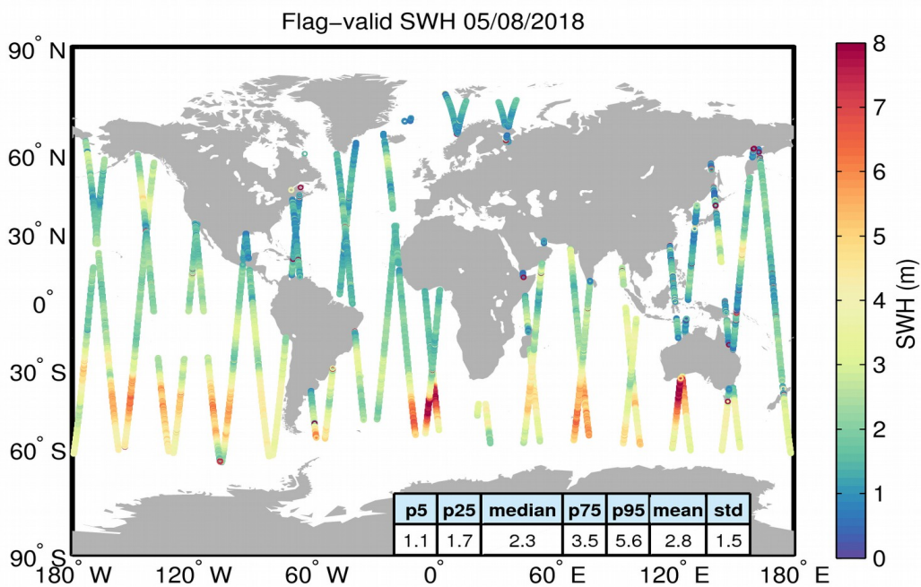
Figure 15. Geographical distribution of flag-valid SWH data over oceans and lakes for 05/08/2018. The statistical values shown in the table refer to the SWH in m and are calculated over all measurements shown in the figure.
