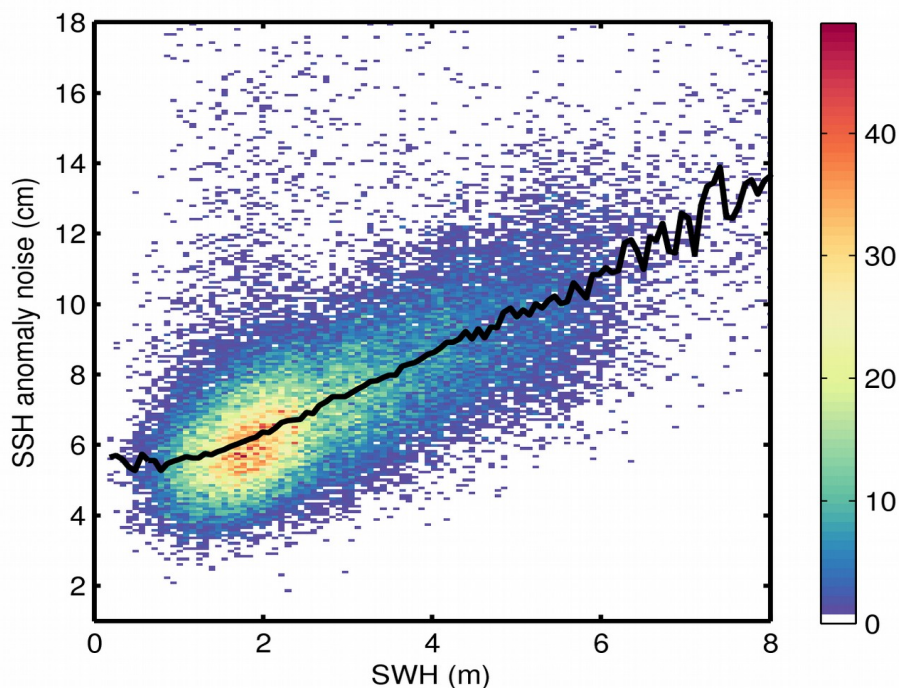
Figure 9. 2D histogram showing flag-valid SSH anomaly noise as a function of SWH for 05/08/2018. The black line denotes the median SSH anomaly noise as a function of SWH.
