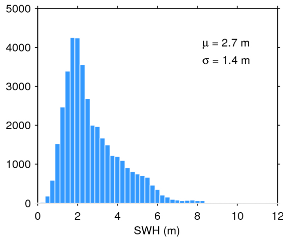
Figure 20. Histogram of science-valid SWH over oceans and lakes for 05/08/2018. The mean ( \mu ) and standard deviation ( \sigma ) are also shown. Note that values larger than 12 m are excluded from the histogram for the sake of readability but not from the computation of \mu and \sigma .
