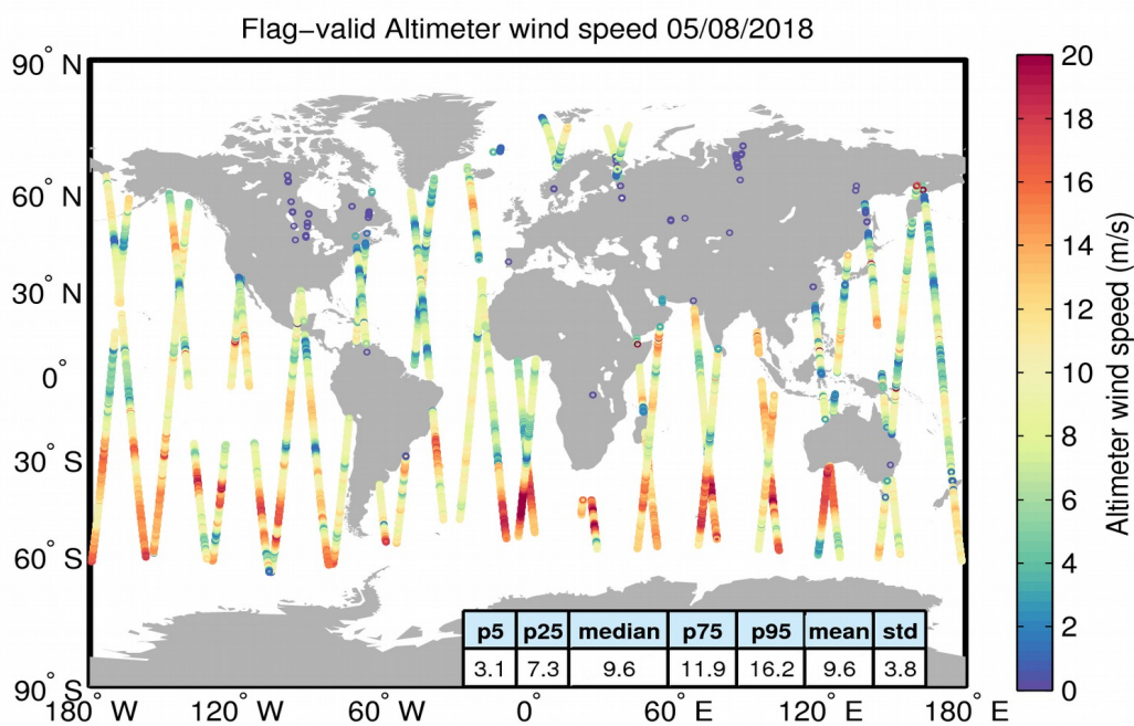
Figure 31. Geographical distribution of flag-valid wind data over oceans and lakes for 05/08/2018. The statistical values shown in the table refer to the wind in m/s and are calculated over all measurements shown in the figure.
