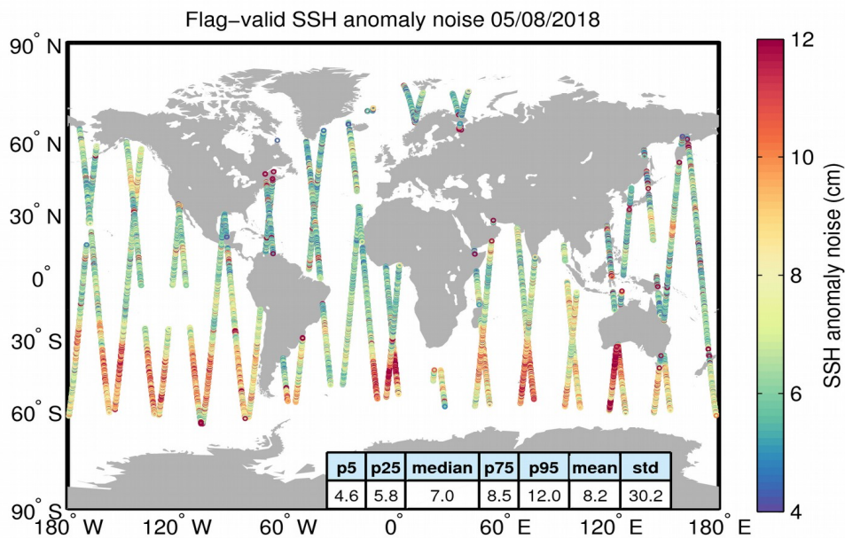
Figure 8. Geographical distribution of flag-valid 20-Hz SSH anomaly measurement noise over oceans and lakes for 05/08/2018. The statistical values shown in the table refer to the SSH anomaly noise and are calculated over all measurements shown in the figure.
