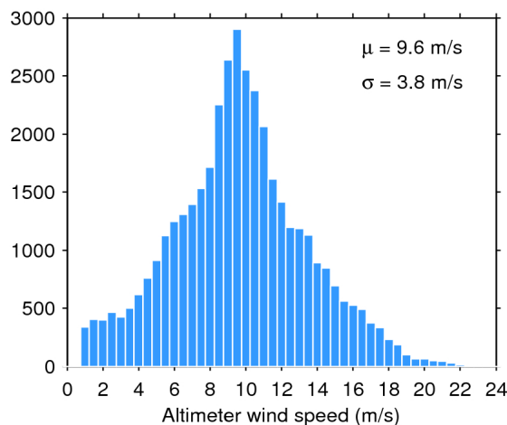
Figure 35. Histogram of science-valid wind over oceans and lakes for 05/08/2018. The mean ( \mu ) and standard deviation ( \sigma ) are also shown. Note that values larger than 24 m/s are excluded from the histogram for the sake of readability but not from the computation of \mu and \sigma .
