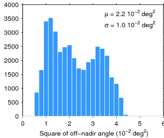
Figure 39. Histogram of flag-valid mispointing over oceans and lakes for 05/08/2018. The mean ( \mu ) and standard deviation ( \sigma ) are also shown. Note that values larger than 6 \cdot 10^{-2} \text{ deg}^2 are excluded from the histogram for the sake of readability but not from the computation of \mu and \sigma .
