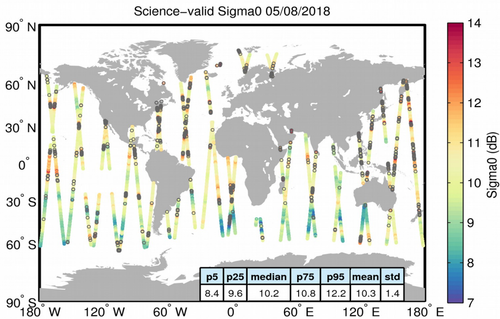
Figure 27. Geographical distribution of science-valid sigma0 data over oceans and lakes for 05/08/2018. The statistical values shown in the table refer to the sigma0 in dB and are calculated over all measurements shown in the figure. Gray circles denote records that have been rejected based on the editing criteria described in Table 4.
