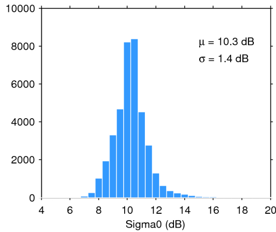
Figure 28. Histogram of science-valid sigma0 over oceans and lakes for 05/08/2018. The mean ( \mu ) and standard deviation ( \sigma ) are also shown. Note that values outside [4 20] dB are excluded from the histogram for the sake of readability but not from the computation of \mu and \sigma .
