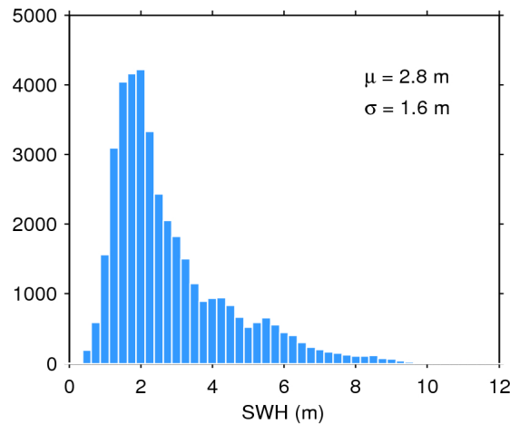
Figure 20. Histogram of science-valid SWH over oceans and lakes for 03/08/2018. The mean ( \mu ) and standard deviation ( \sigma ) are also shown. Note that values larger than 12 m are excluded from the histogram for the sake of readability but not from the computation of \mu and \sigma .
