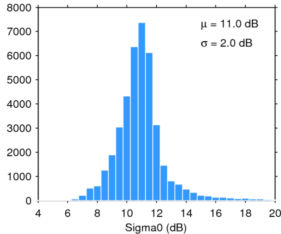
Figure 25. Histogram of flag-valid sigma0 over oceans and lakes for 03/08/2018. The mean ( \mu ) and standard deviation ( \sigma ) are also shown. Note that values outside [4 20] dB are excluded from the histogram for the sake of readability but not from the computation of \mu and \sigma .
