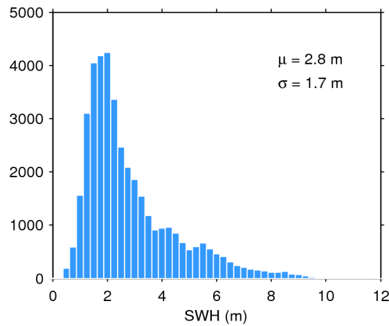
Figure 17. Histogram of flag-valid SWH over oceans and lakes for 03/08/2018. The mean ( \mu ) and standard deviation ( \sigma ) are also shown. Note that values larger than 12 m are excluded from the histogram for the sake of readability but not from the computation of \mu and \sigma .
