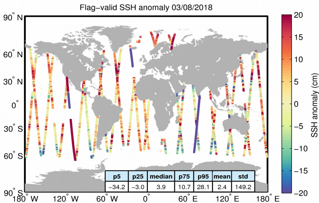
Figure 5. Geographical distribution of flag-valid 1-Hz SSH anomaly data over oceans and lakes for 03/08/2018. The statistical values shown in the table refer to the SSH anomaly in cm and are calculated over all measurements shown in the figure.
