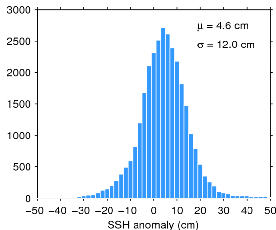
Figure 11. Histogram of science-valid SSH anomaly over oceans and lakes for 03/08/2018. The mean ( \mu ) and standard deviation ( \sigma ) are also shown. Note that values outside [-50 50] cm are excluded from the histogram for the sake of readability but not from the computation of \mu and \sigma .
