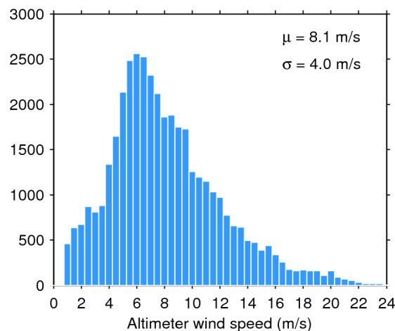
Figure 35. Histogram of science-valid wind over oceans and lakes for 03/08/2018. The mean ( \mu ) and standard deviation ( \sigma ) are also shown. Note that values larger than 24 m/s are excluded from the histogram for the sake of readability but not from the computation of \mu and \sigma .
