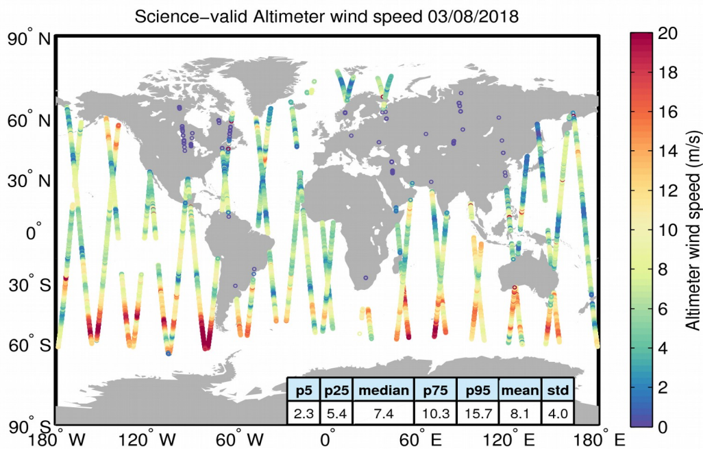
Figure 34. Geographical distribution of science-valid wind data over oceans and lakes for 03/08/2018. The statistical values shown in the table refer to the wind in m/s and are calculated over all measurements shown in the figure. Gray circles denote records that have been rejected based on the editing criteria described in Table 5.
