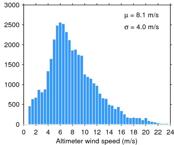
Figure 33. Histogram of flag-valid wind over oceans and lakes for 03/08/2018. The mean ( \mu ) and standard deviation ( \sigma ) are also shown. Note that values larger than 24 m/s are excluded from the histogram for the sake of readability but not from the computation of \mu and \sigma .
