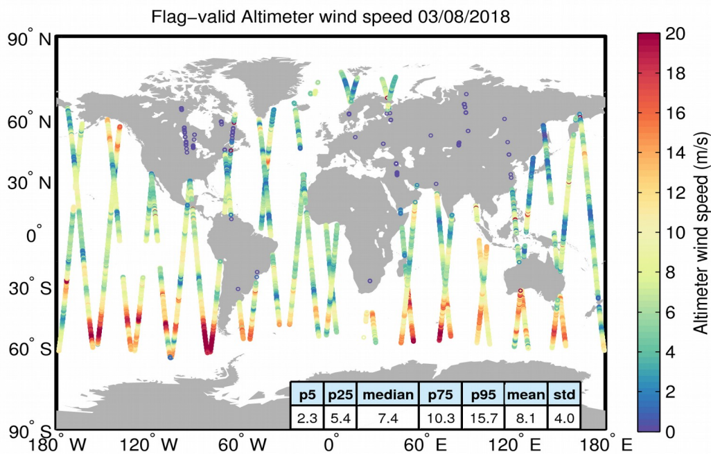
Figure 31. Geographical distribution of flag-valid wind data over oceans and lakes for 03/08/2018. The statistical values shown in the table refer to the wind in m/s and are calculated over all measurements shown in the figure.
