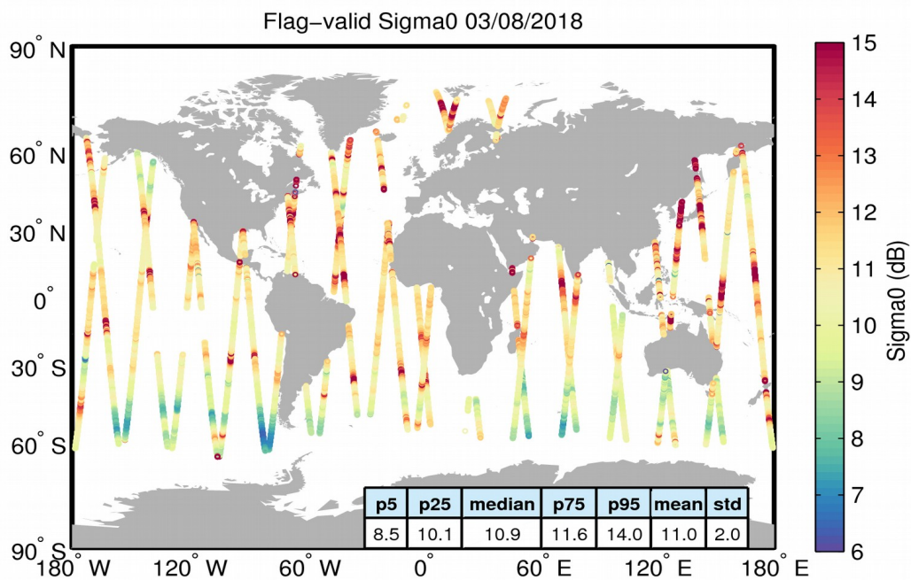
Figure 23. Geographical distribution of flag-valid sigma0 data over oceans and lakes for 03/08/2018. The statistical values shown in the table refer to the sigma0 in dB and are calculated over all measurements shown in the figure.
