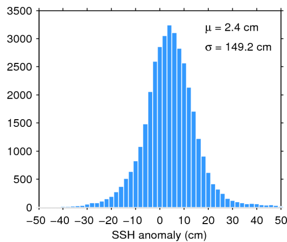
Figure 7. Histogram of flag-valid SSH anomaly over oceans and lakes for 03/08/2018. The mean ( \mu ) and standard deviation ( \sigma ) are also shown. Note that values outside [-50\ 50] cm are excluded from the histogram for the sake of readability but not from the computation of \mu and \sigma .
