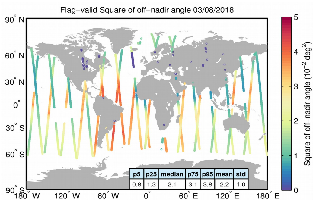
Figure 37. Geographical distribution of flag-valid mispointing data over oceans and lakes for 03/08/2018. The statistical values shown in the table refer to the mispointing in 10^{-2} \text{ deg}^2 and are calculated over all measurements shown in the figure.
