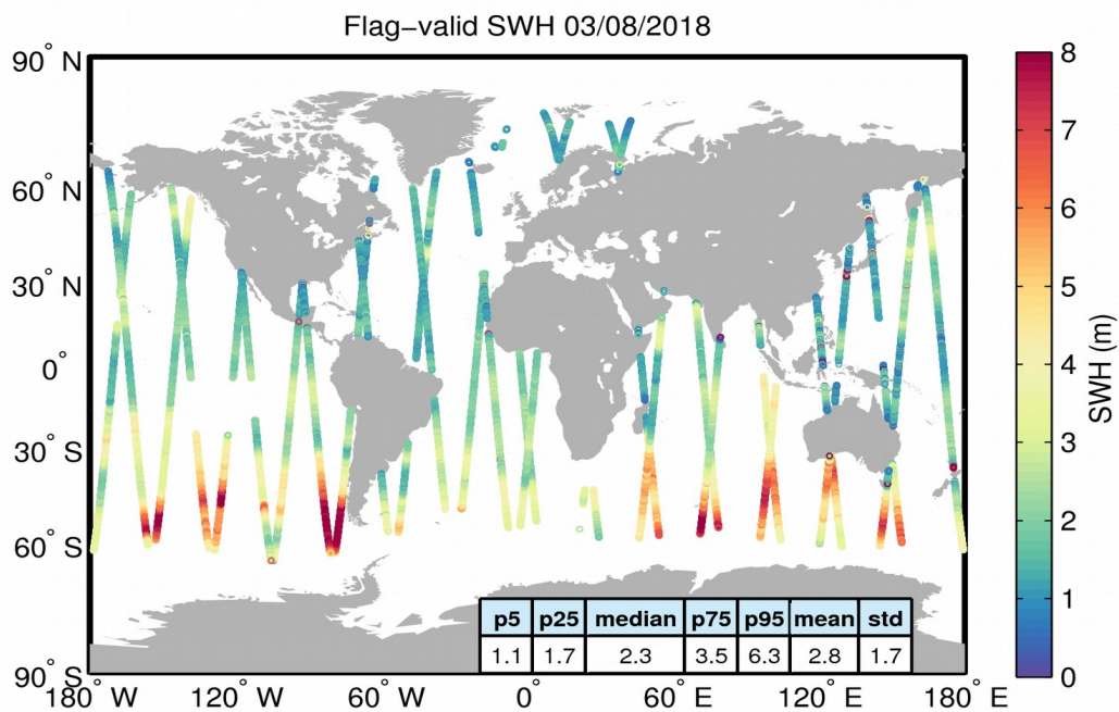
Figure 15. Geographical distribution of flag-valid SWH data over oceans and lakes for 03/08/2018. The statistical values shown in the table refer to the SWH in m and are calculated over all measurements shown in the figure.
