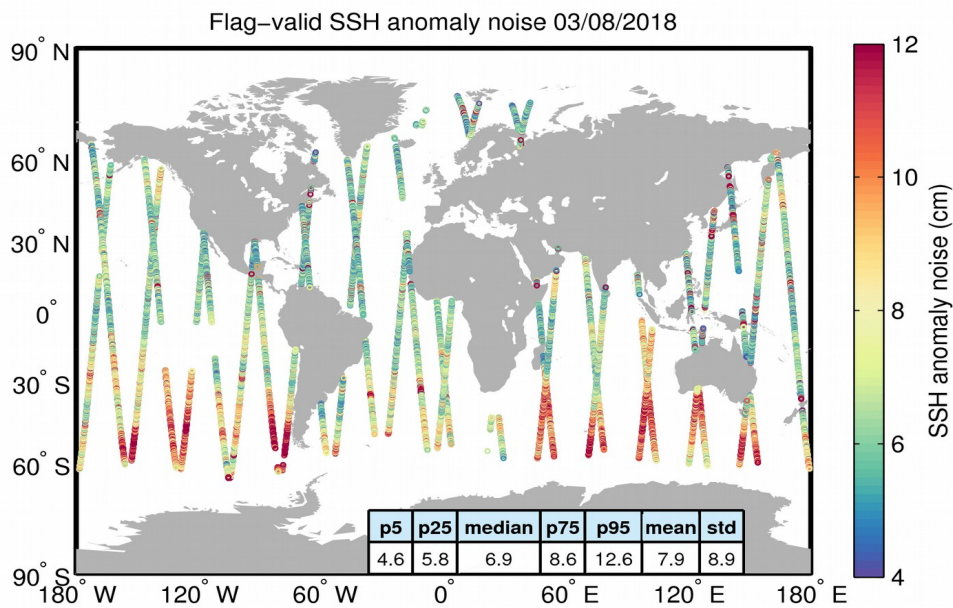
Figure 8. Geographical distribution of flag-valid 20-Hz SSH anomaly measurement noise over oceans and lakes for 03/08/2018. The statistical values shown in the table refer to the SSH anomaly noise and are calculated over all measurements shown in the figure.
