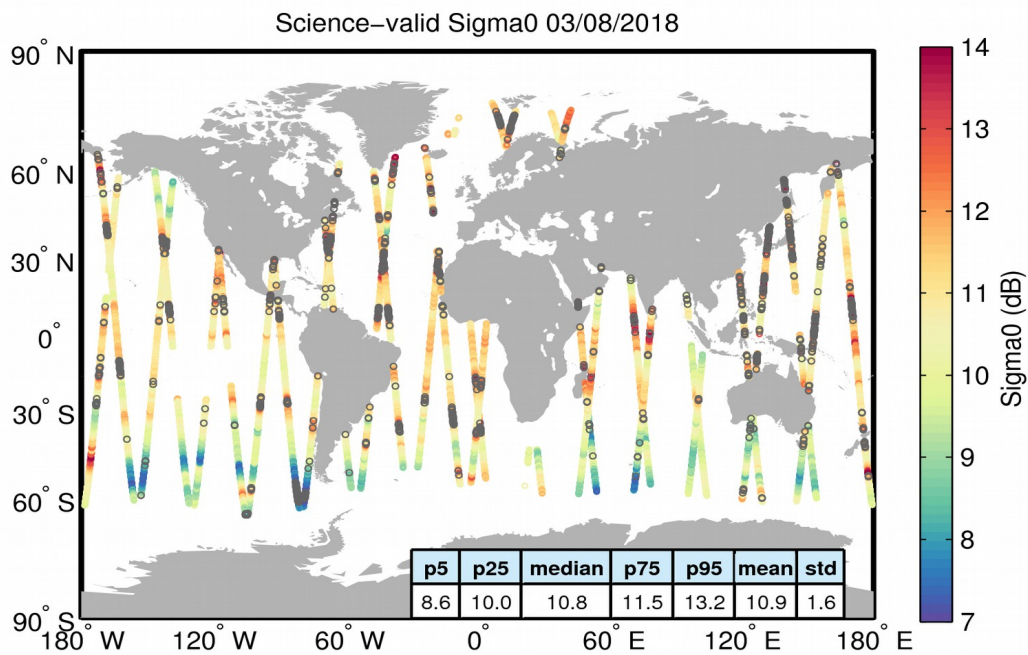
Figure 27. Geographical distribution of science-valid sigma0 data over oceans and lakes for 03/08/2018. The statistical values shown in the table refer to the sigma0 in dB and are calculated over all measurements shown in the figure. Gray circles denote records that have been rejected based on the editing criteria described in Table 4.
