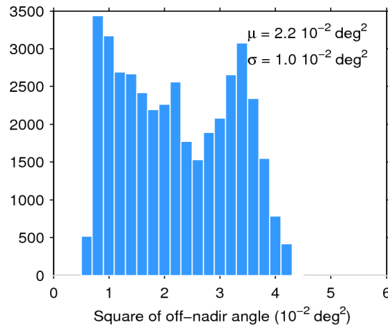
Figure 39. Histogram of flag-valid mispointing over oceans and lakes for 03/08/2018. The mean ( \mu ) and standard deviation ( \sigma ) are also shown. Note that values larger than 6 \cdot 10^{-2} \text{ deg}^2 are excluded from the histogram for the sake of readability but not from the computation of \mu and \sigma .
