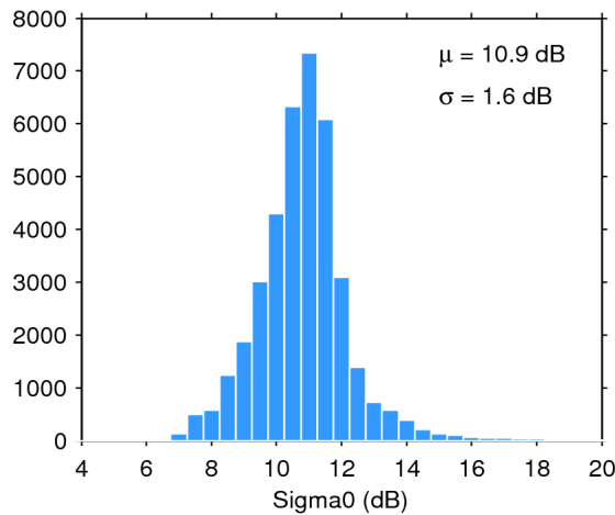
Figure 28. Histogram of science-valid sigma0 over oceans and lakes for 03/08/2018. The mean ( \mu ) and standard deviation ( \sigma ) are also shown. Note that values outside [4 20] dB are excluded from the histogram for the sake of readability but not from the computation of \mu and \sigma .
