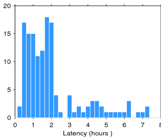
Figure 2. Histogram of the data latency for 03/08/2018. The y-axis denotes the number of files that are made available with a delay of x-hours with respect to the mean time of the records stored in the file.
