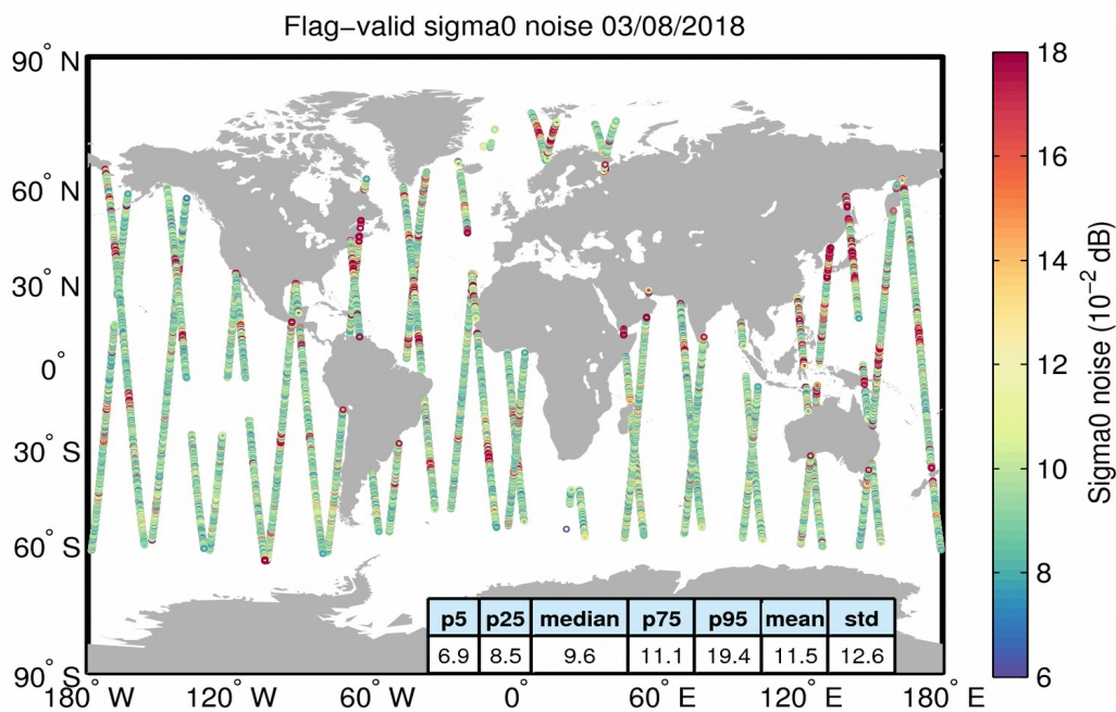
Figure 26. Geographical distribution of flag-valid 20-Hz sigma0 measurement noise over oceans and lakes for 03/08/2018. The statistical values shown in the table refer to the sigma0 noise and are calculated over all measurements shown in the figure.
