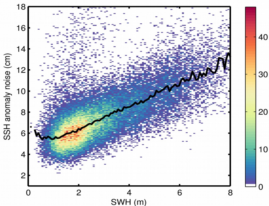
Figure 9. 2D histogram showing flag-valid SSH anomaly noise as a function of SWH for 03/08/2018. The black line denotes the median SSH anomaly noise as a function of SWH.
