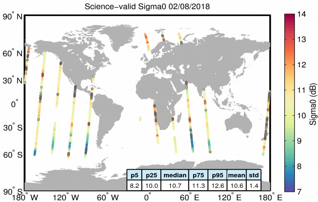
Figure 27. Geographical distribution of science-valid sigma0 data over oceans and lakes for 02/08/2018. The statistical values shown in the table refer to the sigma0 in dB and are calculated over all measurements shown in the figure. Gray circles denote records that have been rejected based on the editing criteria described in Table 4.
