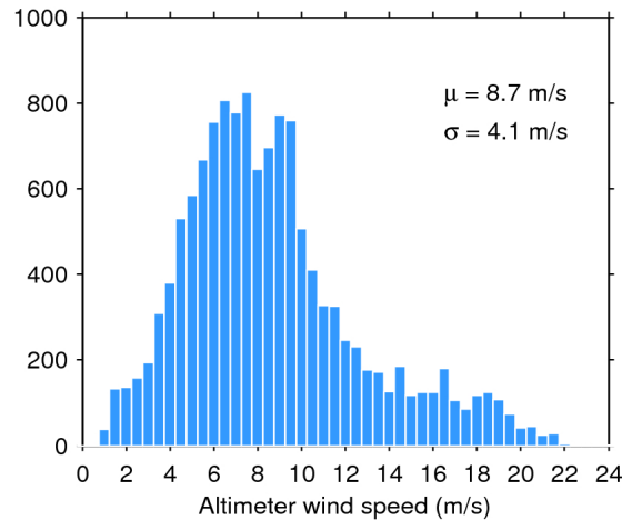
Figure 33. Histogram of flag-valid wind over oceans and lakes for 02/08/2018. The mean ( \mu ) and standard deviation ( \sigma ) are also shown. Note that values larger than 24 m/s are excluded from the histogram for the sake of readability but not from the computation of \mu and \sigma .
