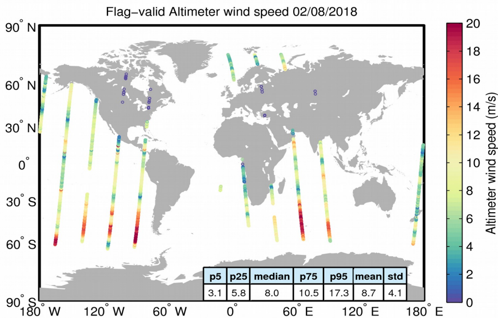
Figure 31. Geographical distribution of flag-valid wind data over oceans and lakes for 02/08/2018. The statistical values shown in the table refer to the wind in m/s and are calculated over all measurements shown in the figure.
