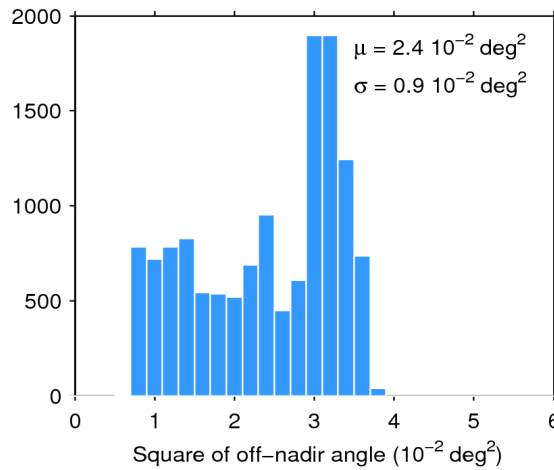
Figure 39. Histogram of flag-valid mispointing over oceans and lakes for 02/08/2018. The mean ( \mu ) and standard deviation ( \sigma ) are also shown. Note that values larger than 6 \cdot 10^{-2} \text{ deg}^2 are excluded from the histogram for the sake of readability but not from the computation of \mu and \sigma .
