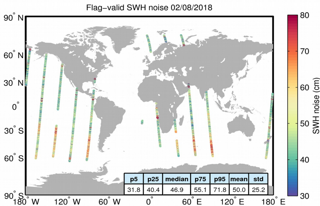
Figure 18. Geographical distribution of flag-valid 20-Hz SWH measurement noise over oceans and lakes for 02/08/2018. The statistical values shown in the figure refer to the SWH noise and are calculated over all measurements shown in the figure.
