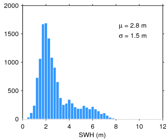
Figure 17. Histogram of flag-valid SWH over oceans and lakes for 02/08/2018. The mean ( \mu ) and standard deviation ( \sigma ) are also shown. Note that values larger than 12 m are excluded from the histogram for the sake of readability but not from the computation of \mu and \sigma .
