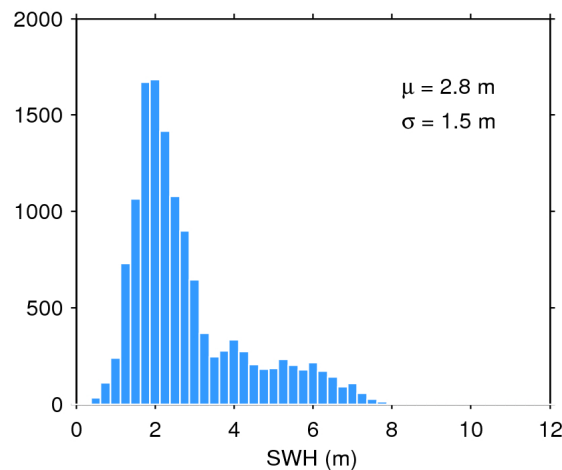
Figure 20. Histogram of science-valid SWH over oceans and lakes for 02/08/2018. The mean ( \mu ) and standard deviation ( \sigma ) are also shown. Note that values larger than 12 m are excluded from the histogram for the sake of readability but not from the computation of \mu and \sigma .
