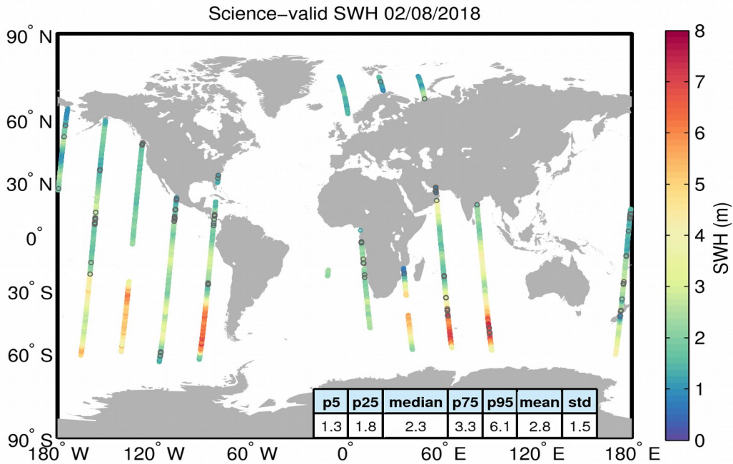
Figure 19. Geographical distribution of science-valid SWH data over oceans and lakes for 02/08/2018. The statistical values shown in the table refer to the SWH in m and are calculated over all measurements shown in the figure. Gray circles denote records that have been rejected based on the editing criteria described in Table 3.
