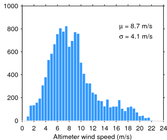
Figure 35. Histogram of science-valid wind over oceans and lakes for 02/08/2018. The mean ( \mu ) and standard deviation ( \sigma ) are also shown. Note that values larger than 24 m/s are excluded from the histogram for the sake of readability but not from the computation of \mu and \sigma .
