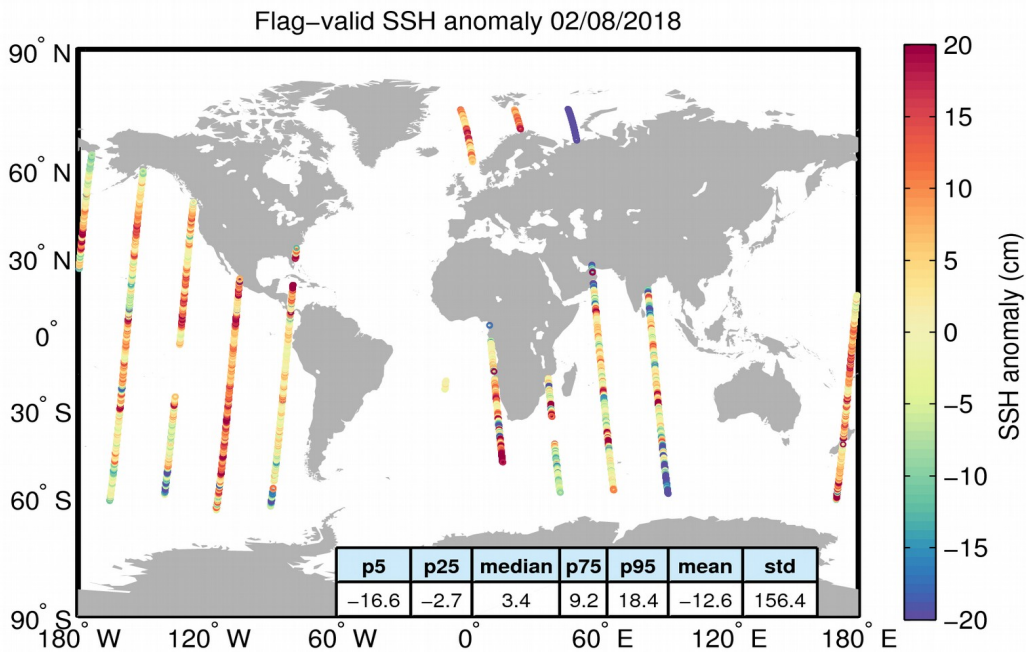
Figure 5. Geographical distribution of flag-valid 1-Hz SSH anomaly data over oceans and lakes for 02/08/2018. The statistical values shown in the table refer to the SSH anomaly in cm and are calculated over all measurements shown in the figure.
