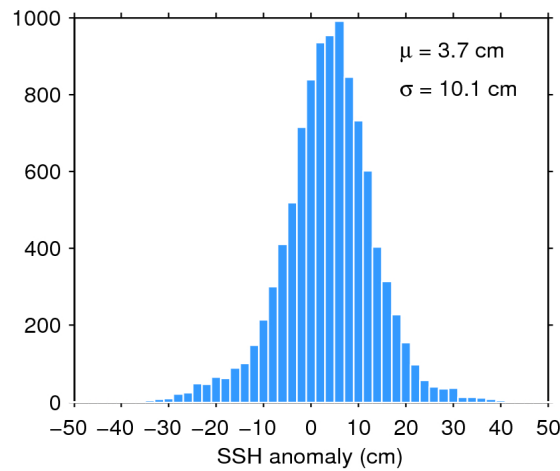
Figure 11. Histogram of science-valid SSH anomaly over oceans and lakes for 02/08/2018. The mean ( \mu ) and standard deviation ( \sigma ) are also shown. Note that values outside [-50 50] cm are excluded from the histogram for the sake of readability but not from the computation of \mu and \sigma .
