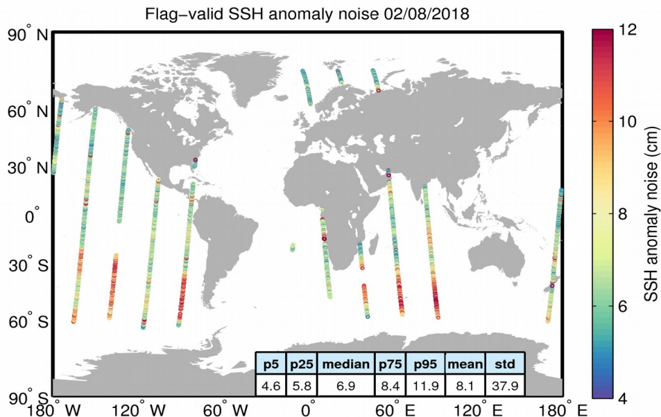
Figure 8. Geographical distribution of flag-valid 20-Hz SSH anomaly measurement noise over oceans and lakes for 02/08/2018. The statistical values shown in the table refer to the SSH anomaly noise and are calculated over all measurements shown in the figure.
