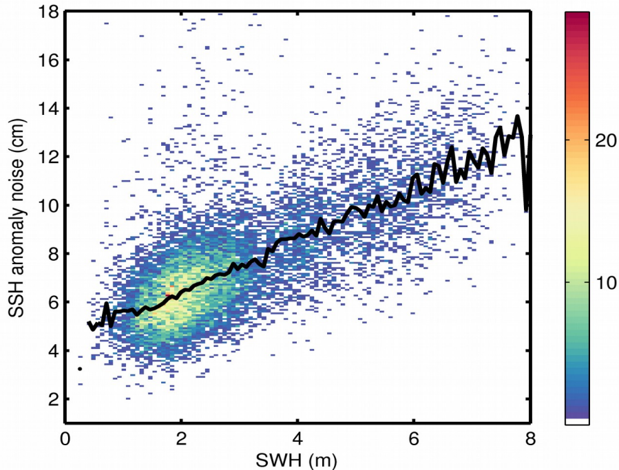
Figure 9. 2D histogram showing flag-valid SSH anomaly noise as a function of SWH for 02/08/2018. The black line denotes the median SSH anomaly noise as a function of SWH.
