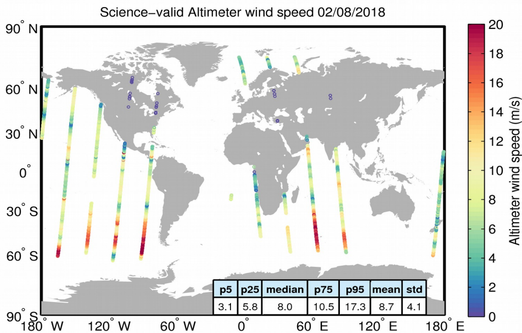
Figure 34. Geographical distribution of science-valid wind data over oceans and lakes for 02/08/2018. The statistical values shown in the table refer to the wind in m/s and are calculated over all measurements shown in the figure. Gray circles denote records that have been rejected based on the editing criteria described in Table 5.
