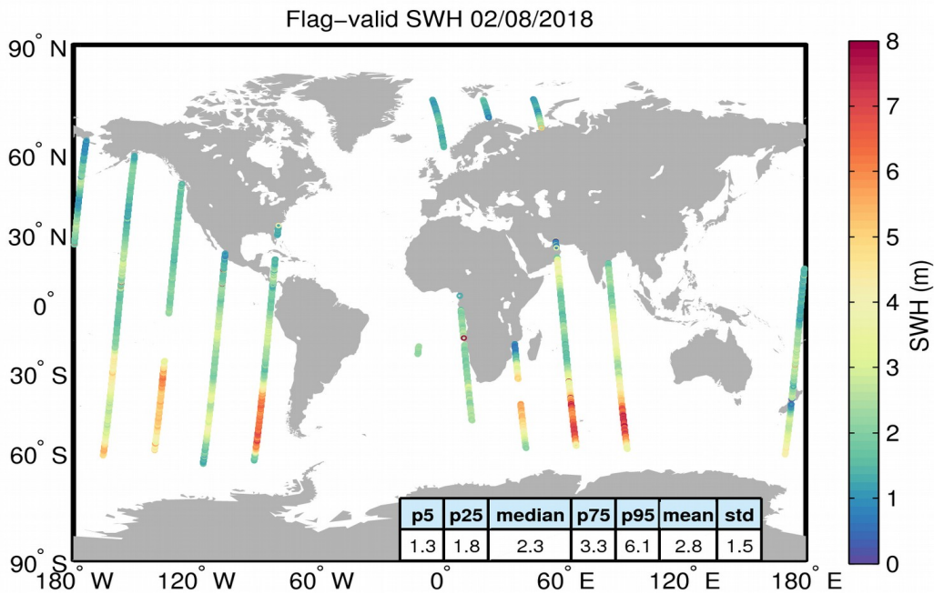
Figure 15. Geographical distribution of flag-valid SWH data over oceans and lakes for 02/08/2018. The statistical values shown in the table refer to the SWH in m and are calculated over all measurements shown in the figure.
