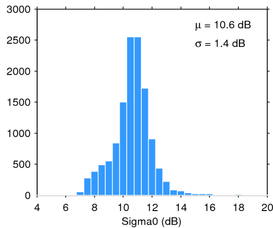
Figure 28. Histogram of science-valid sigma0 over oceans and lakes for 02/08/2018. The mean ( \mu ) and standard deviation ( \sigma ) are also shown. Note that values outside [4 20] dB are excluded from the histogram for the sake of readability but not from the computation of \mu and \sigma .
