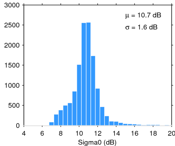
Figure 25. Histogram of flag-valid sigma0 over oceans and lakes for 02/08/2018. The mean ( \mu ) and standard deviation ( \sigma ) are also shown. Note that values outside [4 20] dB are excluded from the histogram for the sake of readability but not from the computation of \mu and \sigma .
