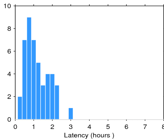
Figure 2. Histogram of the data latency for 02/08/2018. The y-axis denotes the number of files that are made available with a delay of x-hours with respect to the mean time of the records stored in the file.
