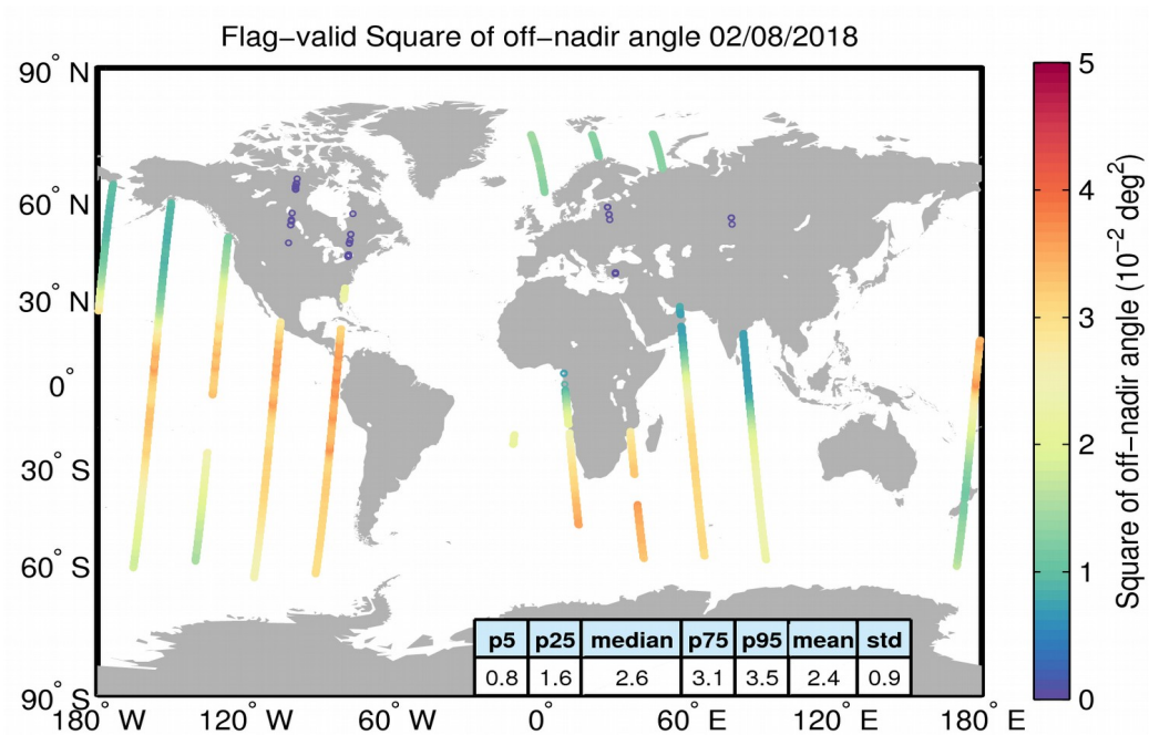
Figure 37. Geographical distribution of flag-valid mispointing data over oceans and lakes for 02/08/2018. The statistical values shown in the table refer to the mispointing in 10^{-2} deg 2 and are calculated over all measurements shown in the figure.
