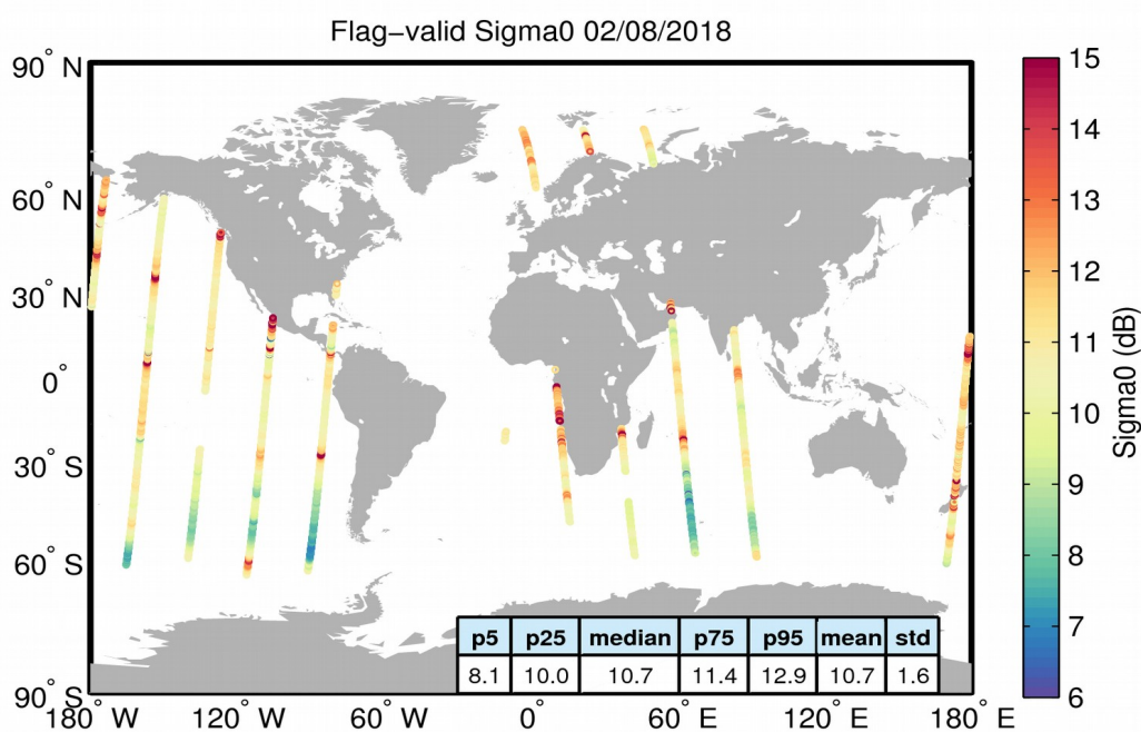
Figure 23. Geographical distribution of flag-valid sigma0 data over oceans and lakes for 02/08/2018. The statistical values shown in the table refer to the sigma0 in dB and are calculated over all measurements shown in the figure.
