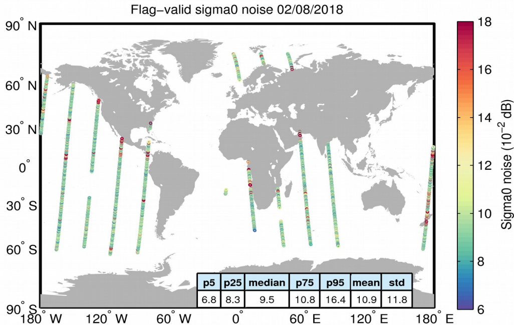
Figure 26. Geographical distribution of flag-valid 20-Hz sigma0 measurement noise over oceans and lakes for 02/08/2018. The statistical values shown in the table refer to the sigma0 noise and are calculated over all measurements shown in the figure.
