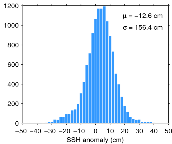
Figure 7. Histogram of flag-valid SSH anomaly over oceans and lakes for 02/08/2018. The mean ( \mu ) and standard deviation ( \sigma ) are also shown. Note that values outside [-50\ 50] cm are excluded from the histogram for the sake of readability but not from the computation of \mu and \sigma .
