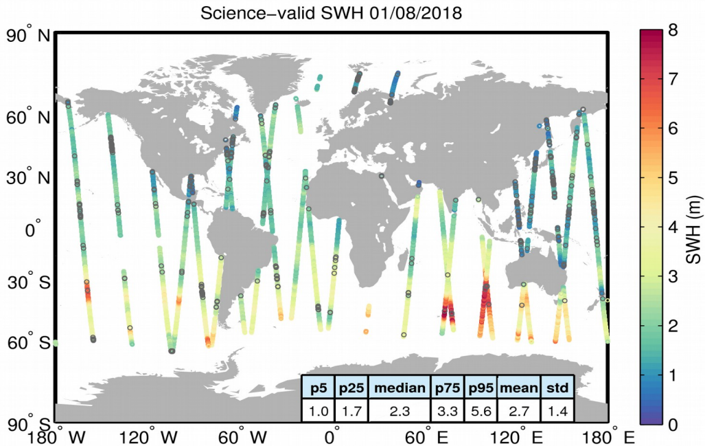
Figure 19. Geographical distribution of science-valid SWH data over oceans and lakes for 01/08/2018. The statistical values shown in the table refer to the SWH in m and are calculated over all measurements shown in the figure. Gray circles denote records that have been rejected based on the editing criteria described in Table 3.
