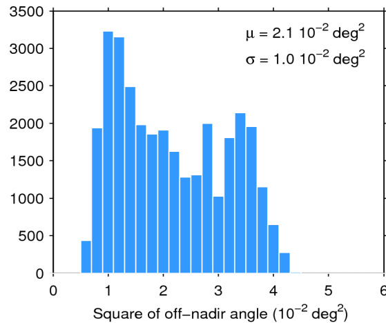
Figure 39. Histogram of flag-valid mispointing over oceans and lakes for 01/08/2018. The mean ( \mu ) and standard deviation ( \sigma ) are also shown. Note that values larger than 6 \cdot 10^{-2} \text{ deg}^2 are excluded from the histogram for the sake of readability but not from the computation of \mu and \sigma .
