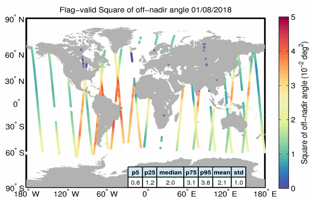
Figure 37. Geographical distribution of flag-valid mispointing data over oceans and lakes for 01/08/2018. The statistical values shown in the table refer to the mispointing in 10^{-2} \text{ deg}^2 and are calculated over all measurements shown in the figure.
