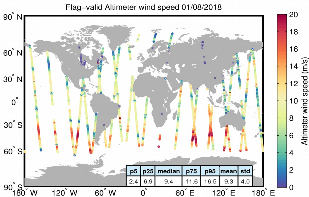
Figure 31. Geographical distribution of flag-valid wind data over oceans and lakes for 01/08/2018. The statistical values shown in the table refer to the wind in m/s and are calculated over all measurements shown in the figure.
