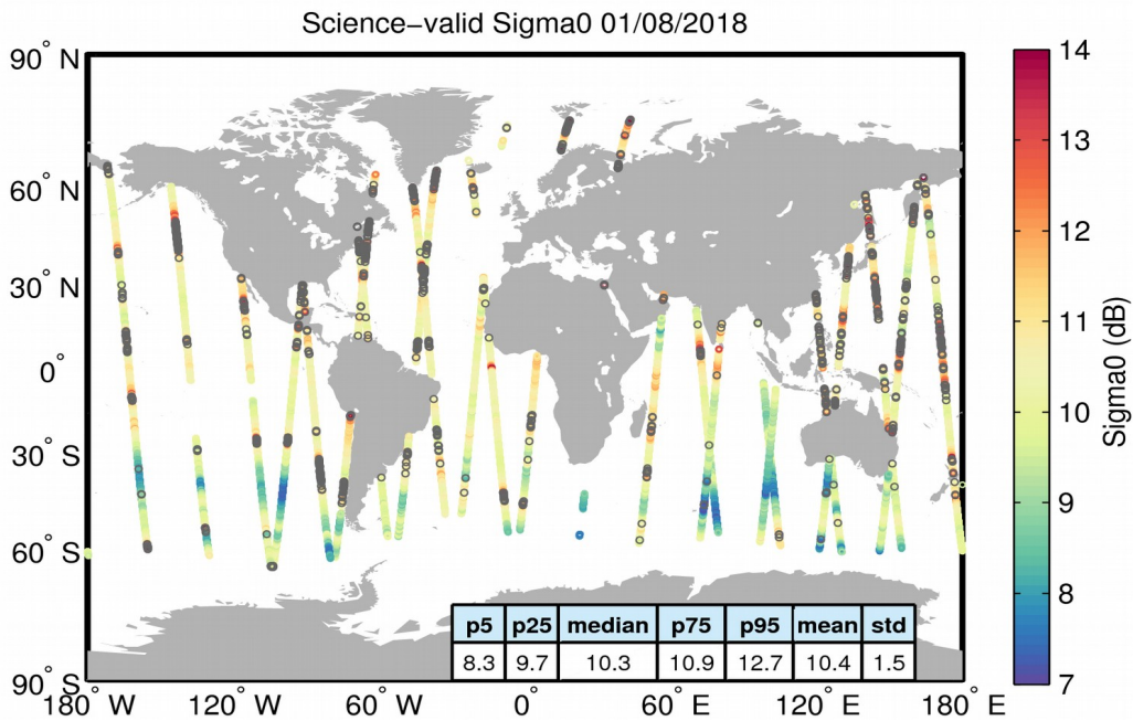
Figure 27. Geographical distribution of science-valid sigma0 data over oceans and lakes for 01/08/2018. The statistical values shown in the table refer to the sigma0 in dB and are calculated over all measurements shown in the figure. Gray circles denote records that have been rejected based on the editing criteria described in Table 4.
