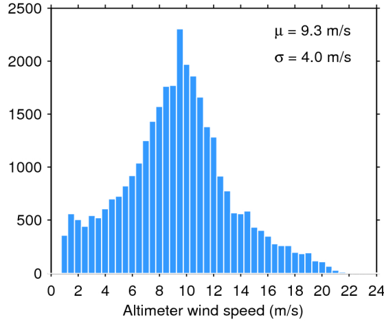
Figure 33. Histogram of flag-valid wind over oceans and lakes for 01/08/2018. The mean ( \mu ) and standard deviation ( \sigma ) are also shown. Note that values larger than 24 m/s are excluded from the histogram for the sake of readability but not from the computation of \mu and \sigma .
