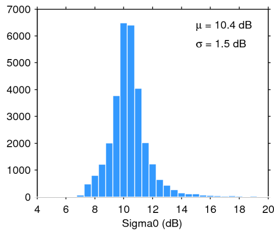
Figure 28. Histogram of science-valid sigma0 over oceans and lakes for 01/08/2018. The mean ( \mu ) and standard deviation ( \sigma ) are also shown. Note that values outside [4 20] dB are excluded from the histogram for the sake of readability but not from the computation of \mu and \sigma .
