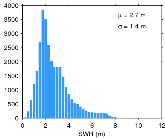
Figure 17. Histogram of flag-valid SWH over oceans and lakes for 01/08/2018. The mean ( \mu ) and standard deviation ( \sigma ) are also shown. Note that values larger than 12 m are excluded from the histogram for the sake of readability but not from the computation of \mu and \sigma .
