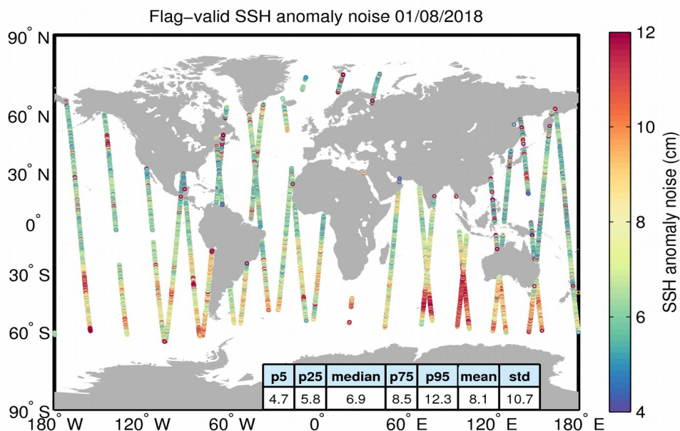
Figure 8. Geographical distribution of flag-valid 20-Hz SSH anomaly measurement noise over oceans and lakes for 01/08/2018. The statistical values shown in the table refer to the SSH anomaly noise and are calculated over all measurements shown in the figure.
