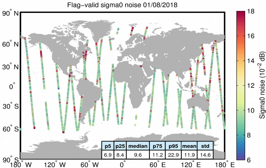
Figure 26. Geographical distribution of flag-valid 20-Hz sigma0 measurement noise over oceans and lakes for 01/08/2018. The statistical values shown in the table refer to the sigma0 noise and are calculated over all measurements shown in the figure.
