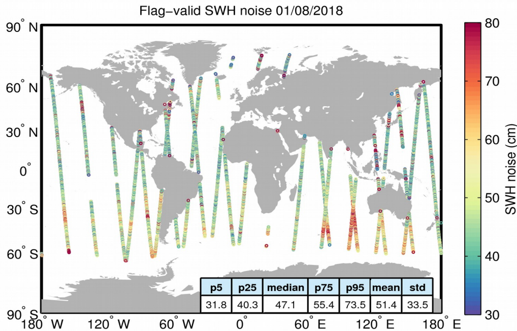
Figure 18. Geographical distribution of flag-valid 20-Hz SWH measurement noise over oceans and lakes for 01/08/2018. The statistical values shown in the figure refer to the SWH noise and are calculated over all measurements shown in the figure.
