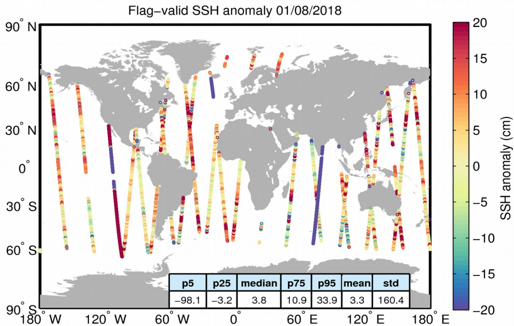
Figure 5. Geographical distribution of flag-valid 1-Hz SSH anomaly data over oceans and lakes for 01/08/2018. The statistical values shown in the table refer to the SSH anomaly in cm and are calculated over all measurements shown in the figure.
