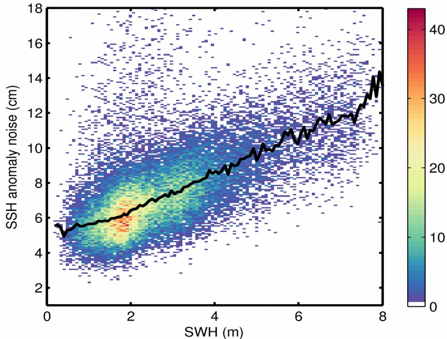
Figure 9. 2D histogram showing flag-valid SSH anomaly noise as a function of SWH for 01/08/2018. The black line denotes the median SSH anomaly noise as a function of SWH.
