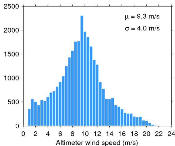
Figure 35. Histogram of science-valid wind over oceans and lakes for 01/08/2018. The mean ( \mu ) and standard deviation ( \sigma ) are also shown. Note that values larger than 24 m/s are excluded from the histogram for the sake of readability but not from the computation of \mu and \sigma .
