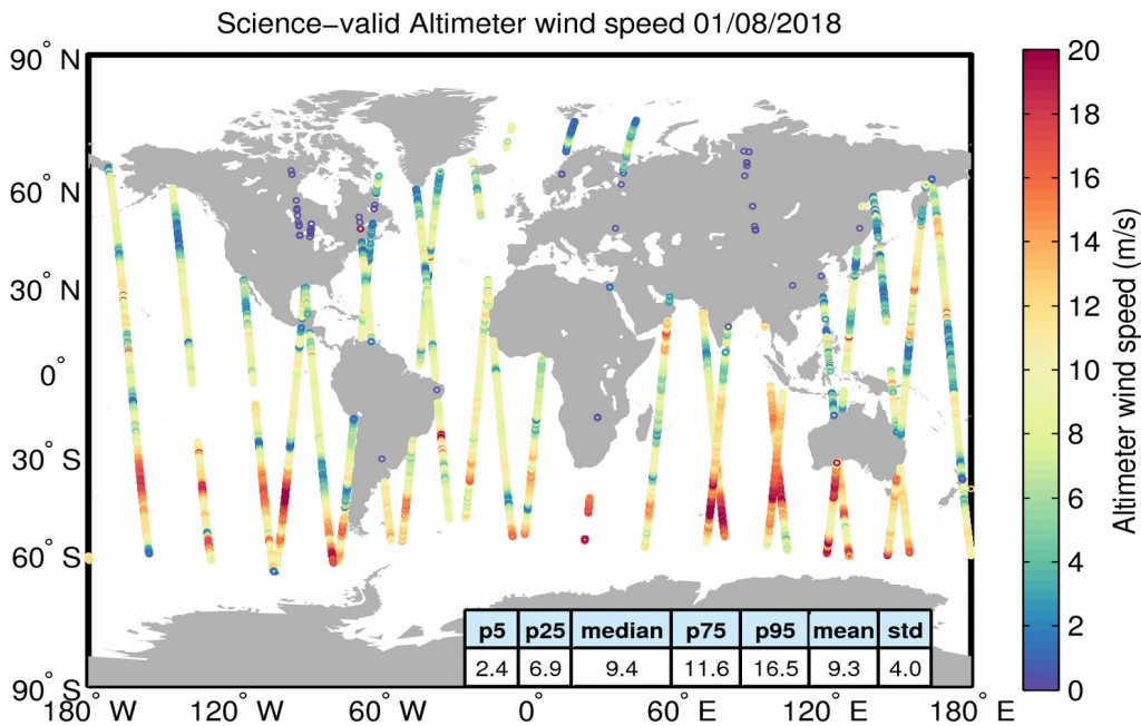
Figure 34. Geographical distribution of science-valid wind data over oceans and lakes for 01/08/2018. The statistical values shown in the table refer to the wind in m/s and are calculated over all measurements shown in the figure. Gray circles denote records that have been rejected based on the editing criteria described in Table 5.
