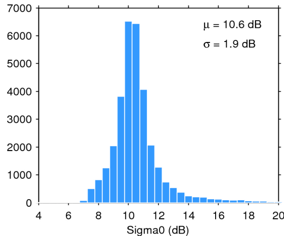
Figure 25. Histogram of flag-valid sigma0 over oceans and lakes for 01/08/2018. The mean ( \mu ) and standard deviation ( \sigma ) are also shown. Note that values outside [4 20] dB are excluded from the histogram for the sake of readability but not from the computation of \mu and \sigma .
