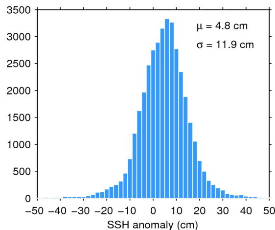
Figure 11. Histogram of science-valid SSH anomaly over oceans and lakes for 31/07/2018. The mean ( \mu ) and standard deviation ( \sigma ) are also shown. Note that values outside [-50 50] cm are excluded from the histogram for the sake of readability but not from the computation of \mu and \sigma .
