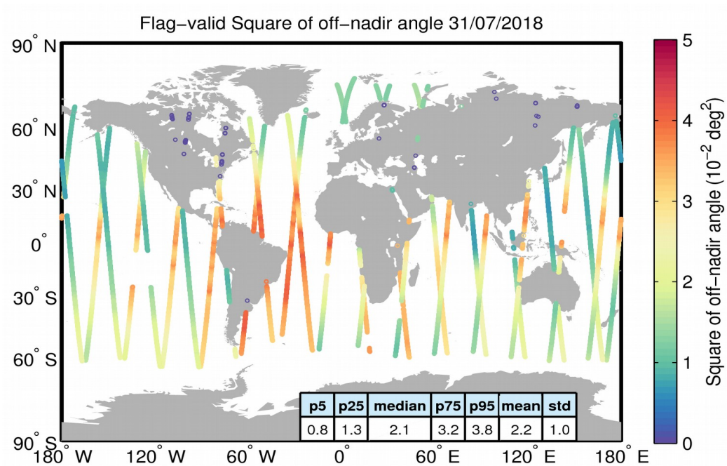
Figure 37. Geographical distribution of flag-valid mispointing data over oceans and lakes for 31/07/2018. The statistical values shown in the table refer to the mispointing in 10^{-2} \text{ deg}^2 and are calculated over all measurements shown in the figure.
