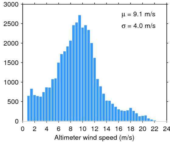
Figure 33. Histogram of flag-valid wind over oceans and lakes for 31/07/2018. The mean ( \mu ) and standard deviation ( \sigma ) are also shown. Note that values larger than 24 m/s are excluded from the histogram for the sake of readability but not from the computation of \mu and \sigma .
