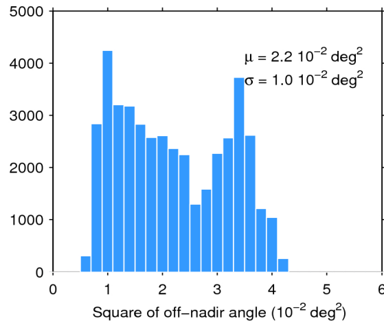
Figure 39. Histogram of flag-valid mispointing over oceans and lakes for 31/07/2018. The mean ( \mu ) and standard deviation ( \sigma ) are also shown. Note that values larger than 6 \cdot 10^{-2} \text{ deg}^2 are excluded from the histogram for the sake of readability but not from the computation of \mu and \sigma .
