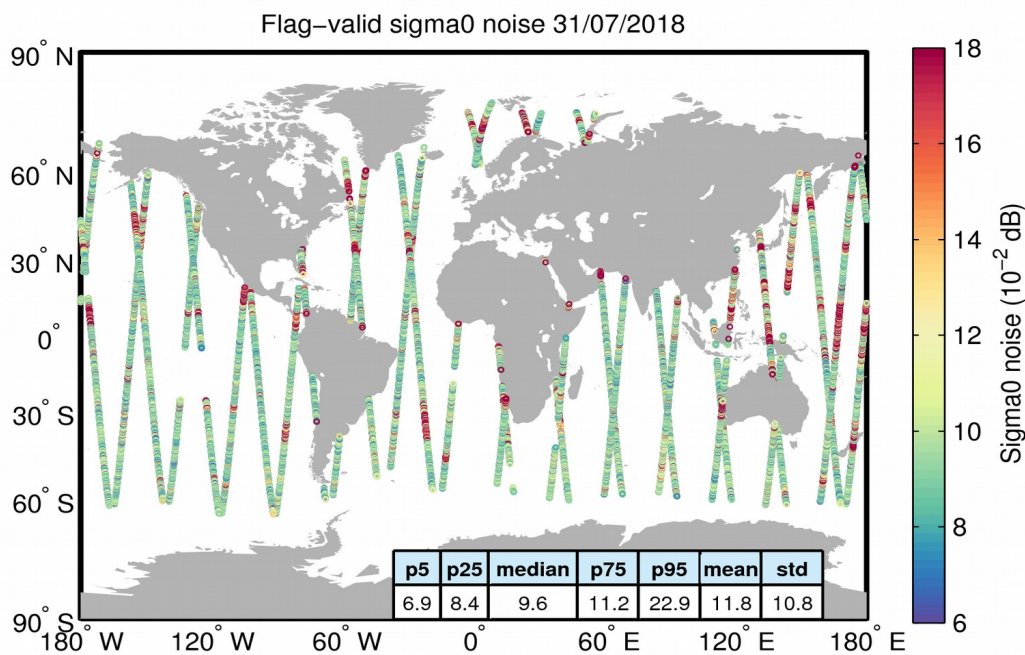
Figure 26. Geographical distribution of flag-valid 20-Hz sigma0 measurement noise over oceans and lakes for 31/07/2018. The statistical values shown in the table refer to the sigma0 noise and are calculated over all measurements shown in the figure.
