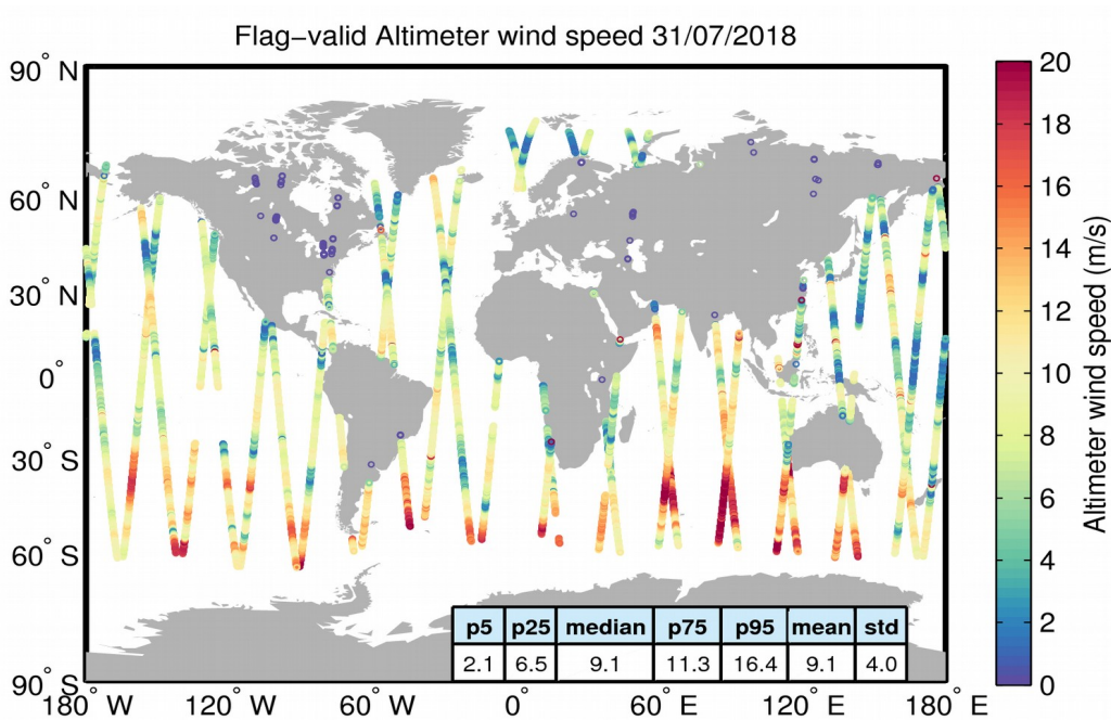
Figure 31. Geographical distribution of flag-valid wind data over oceans and lakes for 31/07/2018. The statistical values shown in the table refer to the wind in m/s and are calculated over all measurements shown in the figure.
