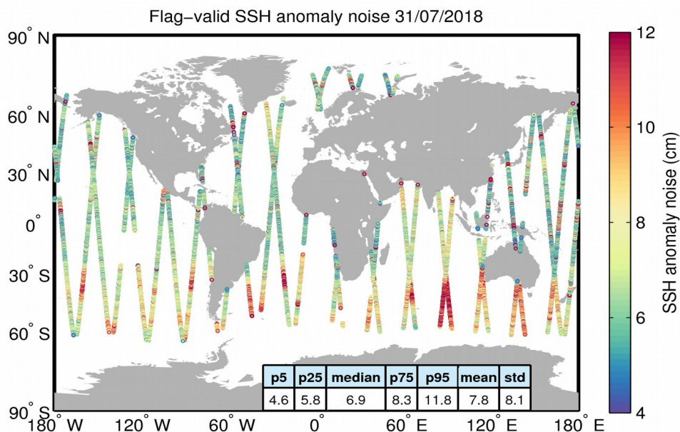
Figure 8. Geographical distribution of flag-valid 20-Hz SSH anomaly measurement noise over oceans and lakes for 31/07/2018. The statistical values shown in the table refer to the SSH anomaly noise and are calculated over all measurements shown in the figure.
