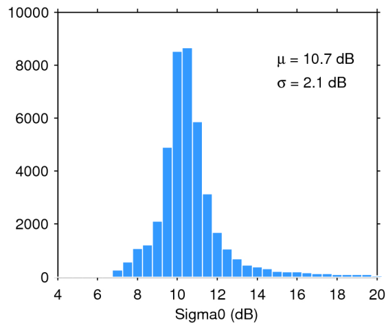
Figure 25. Histogram of flag-valid sigma0 over oceans and lakes for 31/07/2018. The mean ( \mu ) and standard deviation ( \sigma ) are also shown. Note that values outside [4 20] dB are excluded from the histogram for the sake of readability but not from the computation of \mu and \sigma .
