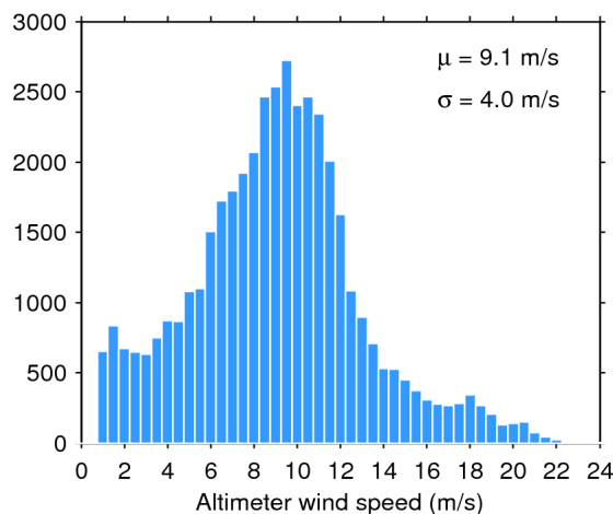
Figure 35. Histogram of science-valid wind over oceans and lakes for 31/07/2018. The mean ( \mu ) and standard deviation ( \sigma ) are also shown. Note that values larger than 24 m/s are excluded from the histogram for the sake of readability but not from the computation of \mu and \sigma .
