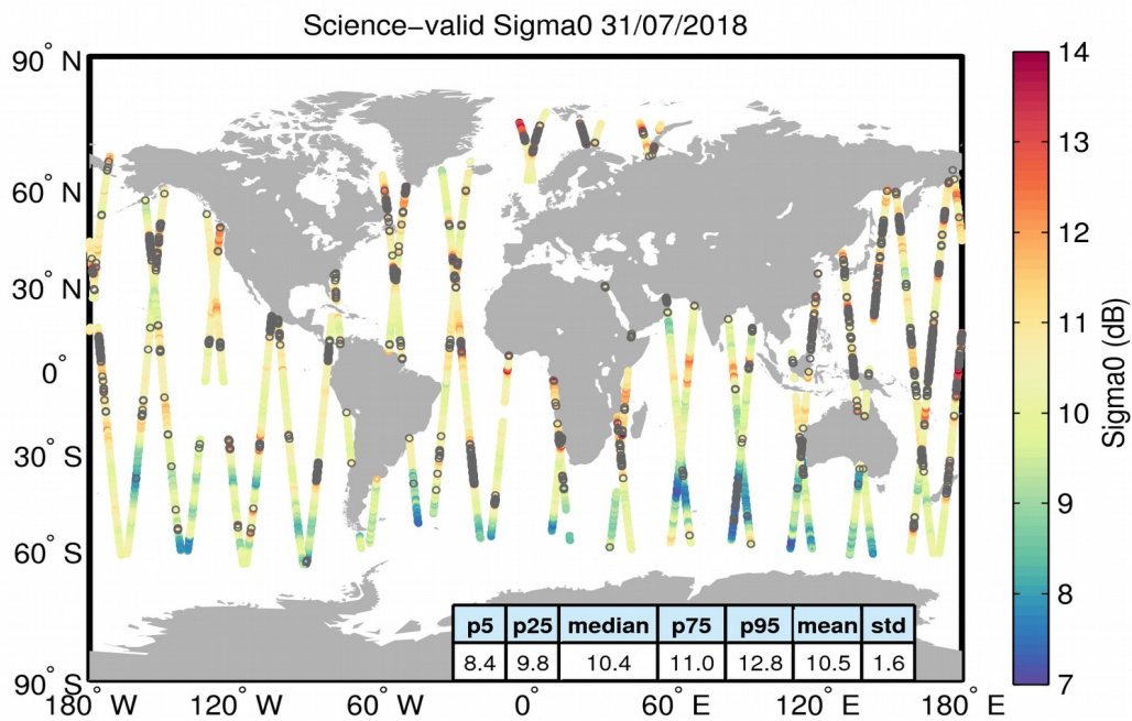
Figure 27. Geographical distribution of science-valid sigma0 data over oceans and lakes for 31/07/2018. The statistical values shown in the table refer to the sigma0 in dB and are calculated over all measurements shown in the figure. Gray circles denote records that have been rejected based on the editing criteria described in Table 4.
