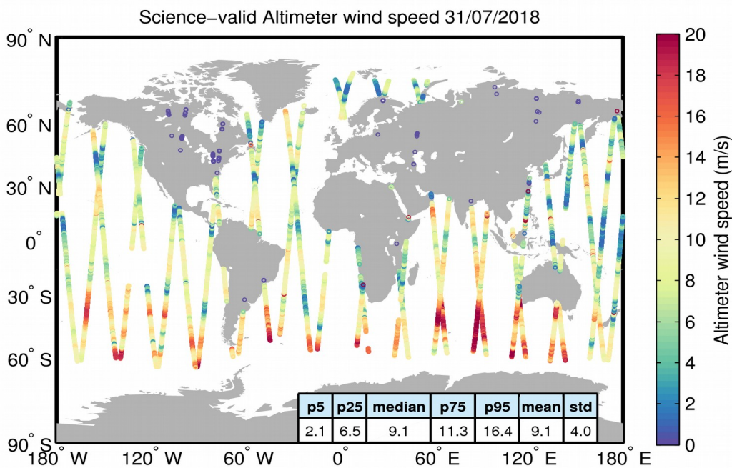
Figure 34. Geographical distribution of science-valid wind data over oceans and lakes for 31/07/2018. The statistical values shown in the table refer to the wind in m/s and are calculated over all measurements shown in the figure. Gray circles denote records that have been rejected based on the editing criteria described in Table 5.
