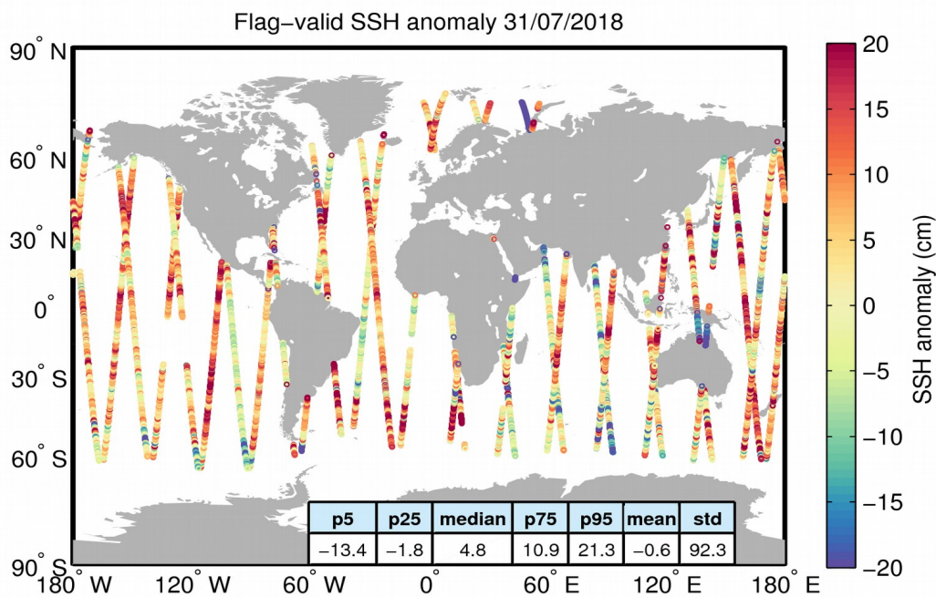
Figure 5. Geographical distribution of flag-valid 1-Hz SSH anomaly data over oceans and lakes for 31/07/2018. The statistical values shown in the table refer to the SSH anomaly in cm and are calculated over all measurements shown in the figure.
