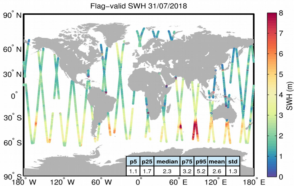
Figure 15. Geographical distribution of flag-valid SWH data over oceans and lakes for 31/07/2018. The statistical values shown in the table refer to the SWH in m and are calculated over all measurements shown in the figure.
