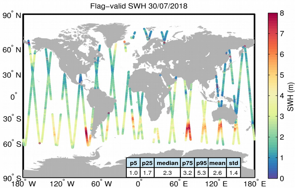
Figure 15. Geographical distribution of flag-valid SWH data over oceans and lakes for 30/07/2018. The statistical values shown in the table refer to the SWH in m and are calculated over all measurements shown in the figure.
