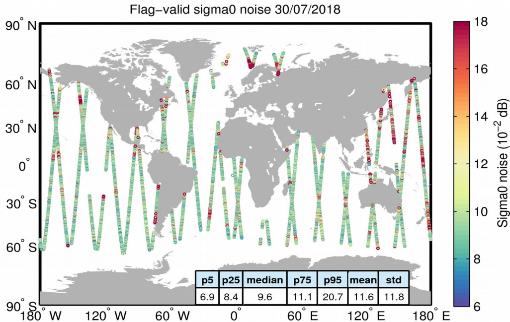
Figure 26. Geographical distribution of flag-valid 20-Hz sigma0 measurement noise over oceans and lakes for 30/07/2018. The statistical values shown in the table refer to the sigma0 noise and are calculated over all measurements shown in the figure.
