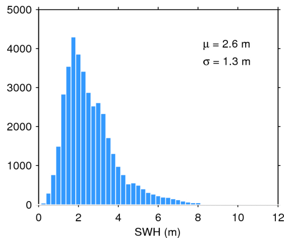
Figure 20. Histogram of science-valid SWH over oceans and lakes for 30/07/2018. The mean ( \mu ) and standard deviation ( \sigma ) are also shown. Note that values larger than 12 m are excluded from the histogram for the sake of readability but not from the computation of \mu and \sigma .
