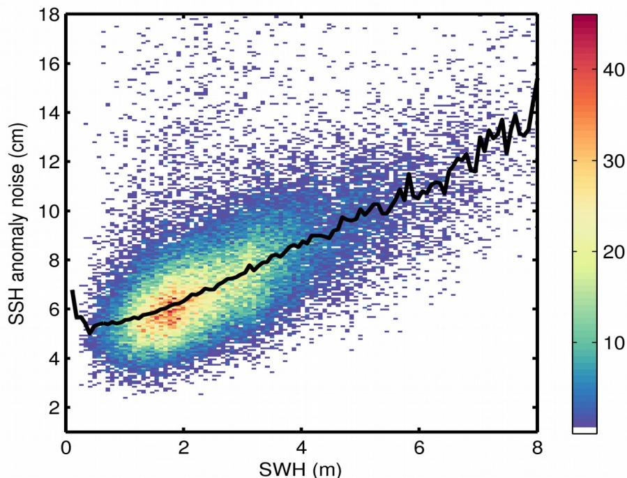
Figure 9. 2D histogram showing flag-valid SSH anomaly noise as a function of SWH for 30/07/2018. The black line denotes the median SSH anomaly noise as a function of SWH.
