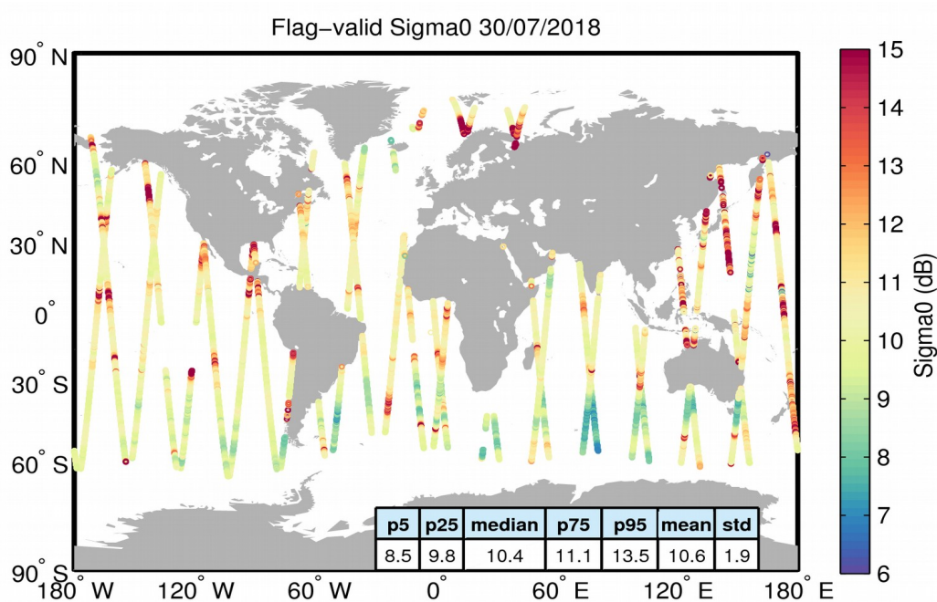
Figure 23. Geographical distribution of flag-valid sigma0 data over oceans and lakes for 30/07/2018. The statistical values shown in the table refer to the sigma0 in dB and are calculated over all measurements shown in the figure.
