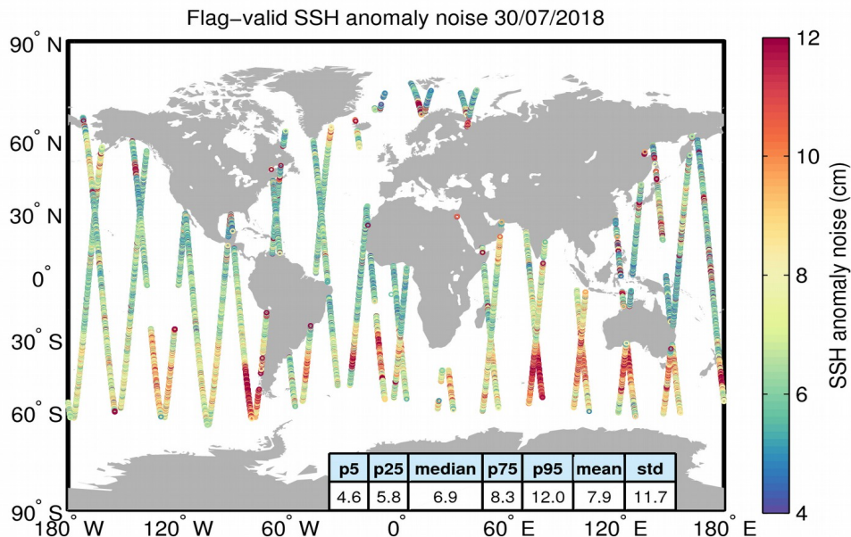
Figure 8. Geographical distribution of flag-valid 20-Hz SSH anomaly measurement noise over oceans and lakes for 30/07/2018. The statistical values shown in the table refer to the SSH anomaly noise and are calculated over all measurements shown in the figure.
