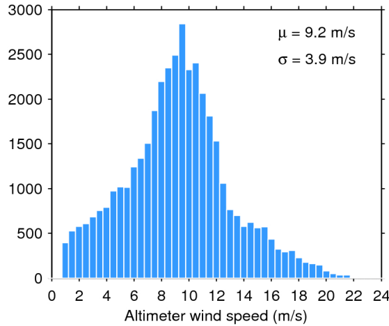
Figure 33. Histogram of flag-valid wind over oceans and lakes for 30/07/2018. The mean ( \mu ) and standard deviation ( \sigma ) are also shown. Note that values larger than 24 m/s are excluded from the histogram for the sake of readability but not from the computation of \mu and \sigma .
