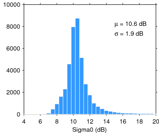
Figure 25. Histogram of flag-valid sigma0 over oceans and lakes for 30/07/2018. The mean ( \mu ) and standard deviation ( \sigma ) are also shown. Note that values outside [4 20] dB are excluded from the histogram for the sake of readability but not from the computation of \mu and \sigma .
