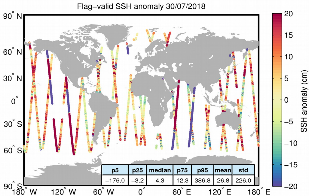
Figure 5. Geographical distribution of flag-valid 1-Hz SSH anomaly data over oceans and lakes for 30/07/2018. The statistical values shown in the table refer to the SSH anomaly in cm and are calculated over all measurements shown in the figure.
