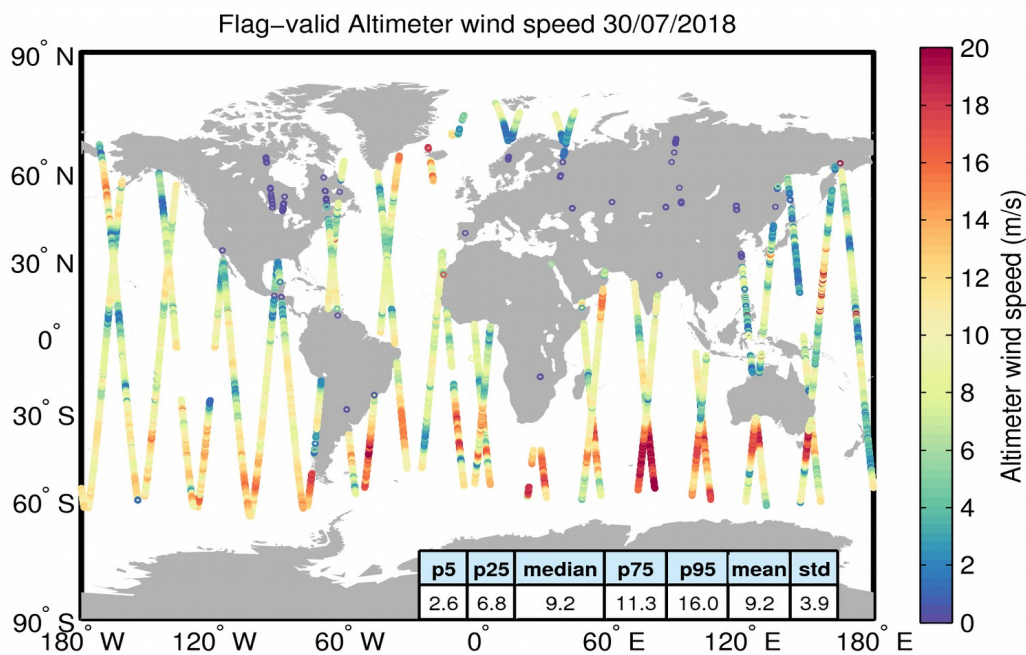
Figure 31. Geographical distribution of flag-valid wind data over oceans and lakes for 30/07/2018. The statistical values shown in the table refer to the wind in m/s and are calculated over all measurements shown in the figure.
