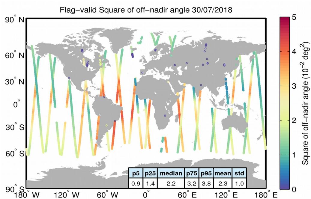
Figure 37. Geographical distribution of flag-valid mispointing data over oceans and lakes for 30/07/2018. The statistical values shown in the table refer to the mispointing in 10^{-2} deg 2 and are calculated over all measurements shown in the figure.
