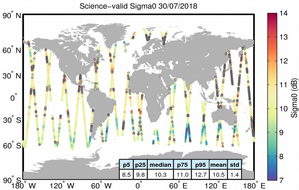
Figure 27. Geographical distribution of science-valid sigma0 data over oceans and lakes for 30/07/2018. The statistical values shown in the table refer to the sigma0 in dB and are calculated over all measurements shown in the figure. Gray circles denote records that have been rejected based on the editing criteria described in Table 4.
