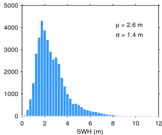
Figure 17. Histogram of flag-valid SWH over oceans and lakes for 30/07/2018. The mean ( \mu ) and standard deviation ( \sigma ) are also shown. Note that values larger than 12 m are excluded from the histogram for the sake of readability but not from the computation of \mu and \sigma .
