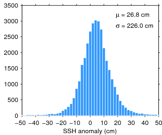
Figure 7. Histogram of flag-valid SSH anomaly over oceans and lakes for 30/07/2018. The mean ( \mu ) and standard deviation ( \sigma ) are also shown. Note that values outside [-50 50] cm are excluded from the histogram for the sake of readability but not from the computation of \mu and \sigma .
