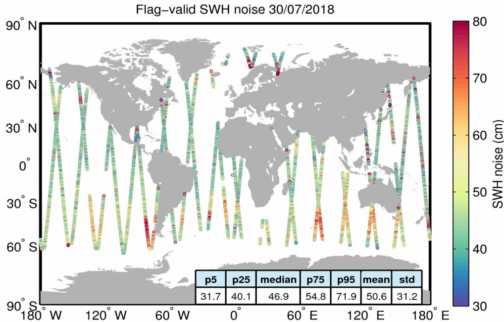
Figure 18. Geographical distribution of flag-valid 20-Hz SWH measurement noise over oceans and lakes for 30/07/2018. The statistical values shown in the table refer to the SWH noise and are calculated over all measurements shown in the figure.
