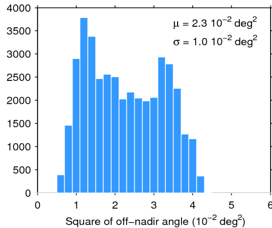
Figure 39. Histogram of flag-valid mispointing over oceans and lakes for 30/07/2018. The mean ( \mu ) and standard deviation ( \sigma ) are also shown. Note that values larger than 6 \cdot 10^{-2} \text{ deg}^2 are excluded from the histogram for the sake of readability but not from the computation of \mu and \sigma .
