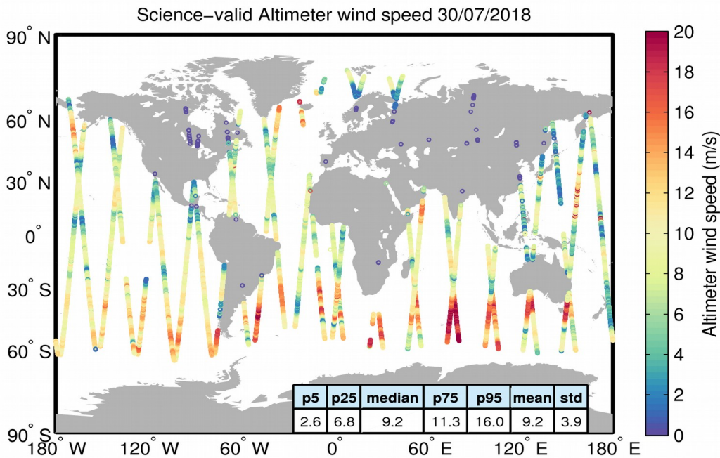
Figure 34. Geographical distribution of science-valid wind data over oceans and lakes for 30/07/2018. The statistical values shown in the table refer to the wind in m/s and are calculated over all measurements shown in the figure. Gray circles denote records that have been rejected based on the editing criteria described in Table 5.
