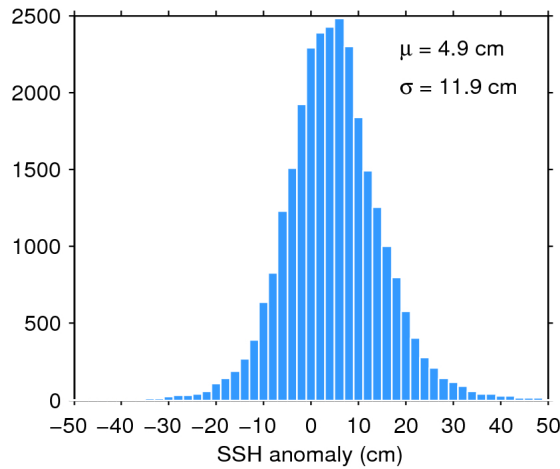
Figure 11. Histogram of science-valid SSH anomaly over oceans and lakes for 30/07/2018. The mean ( \mu ) and standard deviation ( \sigma ) are also shown. Note that values outside [-50 50] cm are excluded from the histogram for the sake of readability but not from the computation of \mu and \sigma .
