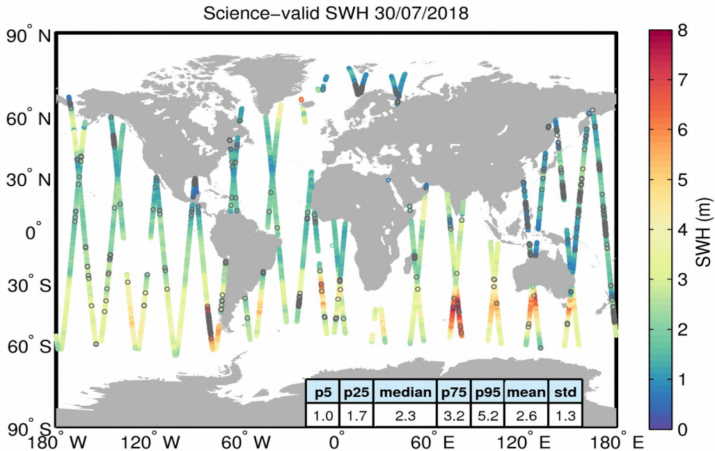
Figure 19. Geographical distribution of science-valid SWH data over oceans and lakes for 30/07/2018. The statistical values shown in the table refer to the SWH in m and are calculated over all measurements shown in the figure. Gray circles denote records that have been rejected based on the editing criteria described in Table 3.
