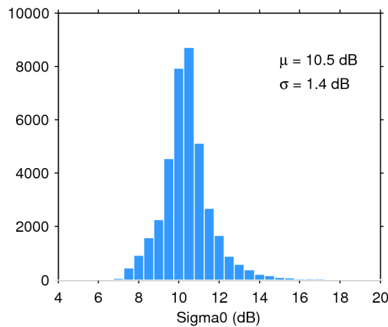
Figure 28. Histogram of science-valid sigma0 over oceans and lakes for 30/07/2018. The mean ( \mu ) and standard deviation ( \sigma ) are also shown. Note that values outside [4 20] dB are excluded from the histogram for the sake of readability but not from the computation of \mu and \sigma .
