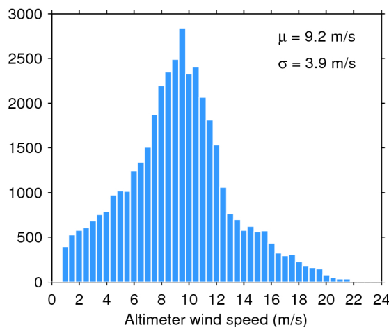
Figure 35. Histogram of science-valid wind over oceans and lakes for 30/07/2018. The mean ( \mu ) and standard deviation ( \sigma ) are also shown. Note that values larger than 24 m/s are excluded from the histogram for the sake of readability but not from the computation of \mu and \sigma .
