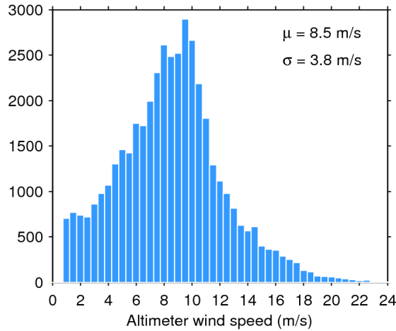
Figure 33. Histogram of flag-valid wind over oceans and lakes for 29/07/2018. The mean ( \mu ) and standard deviation ( \sigma ) are also shown. Note that values larger than 24 m/s are excluded from the histogram for the sake of readability but not from the computation of \mu and \sigma .
