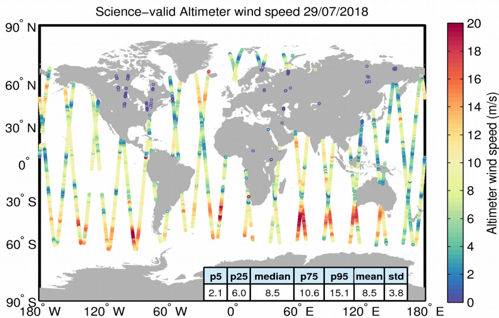
Figure 34. Geographical distribution of science-valid wind data over oceans and lakes for 29/07/2018. The statistical values shown in the table refer to the wind in m/s and are calculated over all measurements shown in the figure. Gray circles denote records that have been rejected based on the editing criteria described in Table 5.
