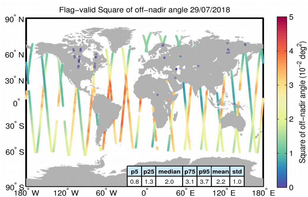
Figure 37. Geographical distribution of flag-valid mispointing data over oceans and lakes for 29/07/2018. The statistical values shown in the table refer to the mispointing in 10^{-2} deg 2 and are calculated over all measurements shown in the figure.
