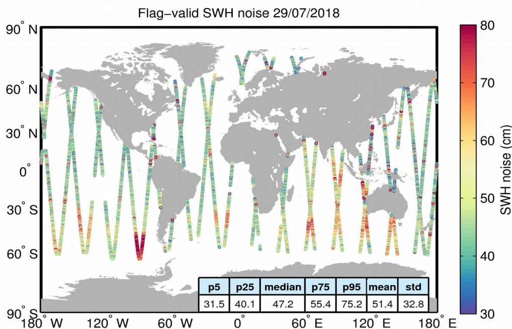
Figure 18. Geographical distribution of flag-valid 20-Hz SWH measurement noise over oceans and lakes for 29/07/2018. The statistical values shown in the figure refer to the SWH noise and are calculated over all measurements shown in the figure.
