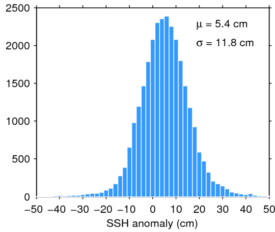
Figure 11. Histogram of science-valid SSH anomaly over oceans and lakes for 29/07/2018. The mean ( \mu ) and standard deviation ( \sigma ) are also shown. Note that values outside [-50 50] cm are excluded from the histogram for the sake of readability but not from the computation of \mu and \sigma .
