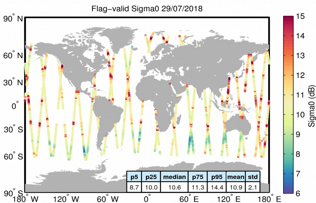
Figure 23. Geographical distribution of flag-valid sigma0 data over oceans and lakes for 29/07/2018. The statistical values shown in the table refer to the sigma0 in dB and are calculated over all measurements shown in the figure.
