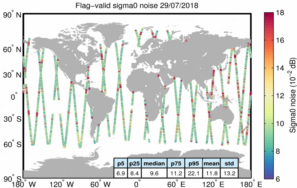
Figure 26. Geographical distribution of flag-valid 20-Hz sigma0 measurement noise over oceans and lakes for 29/07/2018. The statistical values shown in the table refer to the sigma0 noise and are calculated over all measurements shown in the figure.
