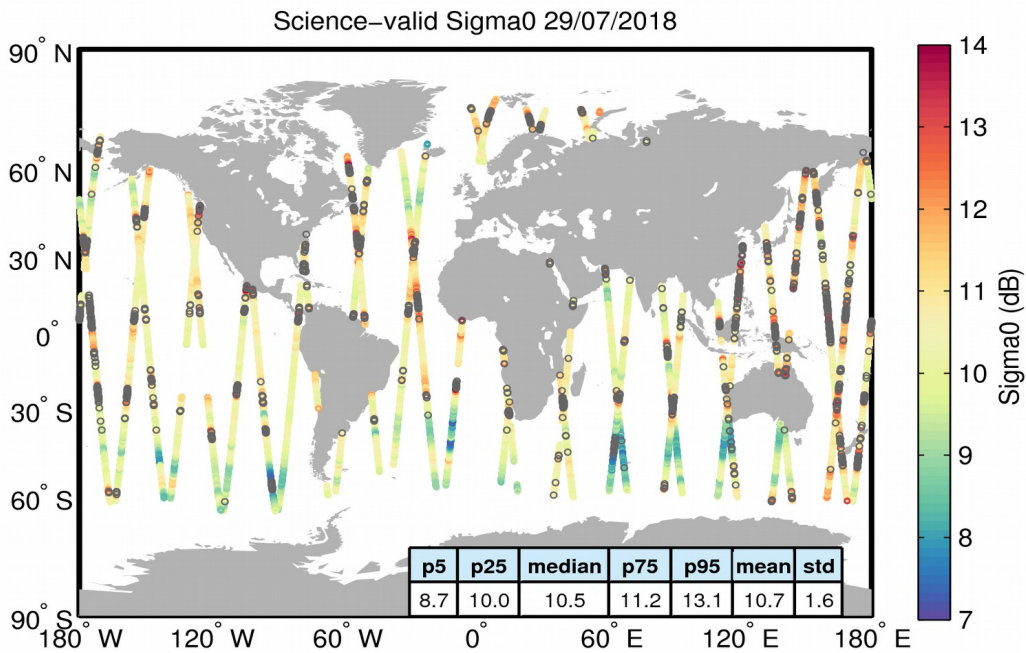
Figure 27. Geographical distribution of science-valid sigma0 data over oceans and lakes for 29/07/2018. The statistical values shown in the table refer to the sigma0 in dB and are calculated over all measurements shown in the figure. Gray circles denote records that have been rejected based on the editing criteria described in Table 4.
