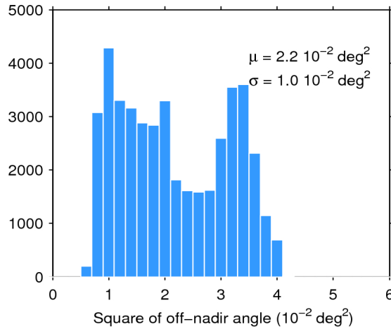
Figure 39. Histogram of flag-valid mispointing over oceans and lakes for 29/07/2018. The mean ( \mu ) and standard deviation ( \sigma ) are also shown. Note that values larger than 6 \cdot 10^{-2} \text{ deg}^2 are excluded from the histogram for the sake of readability but not from the computation of \mu and \sigma .
