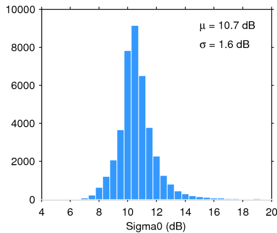
Figure 28. Histogram of science-valid sigma0 over oceans and lakes for 29/07/2018. The mean ( \mu ) and standard deviation ( \sigma ) are also shown. Note that values outside [4 20] dB are excluded from the histogram for the sake of readability but not from the computation of \mu and \sigma .
