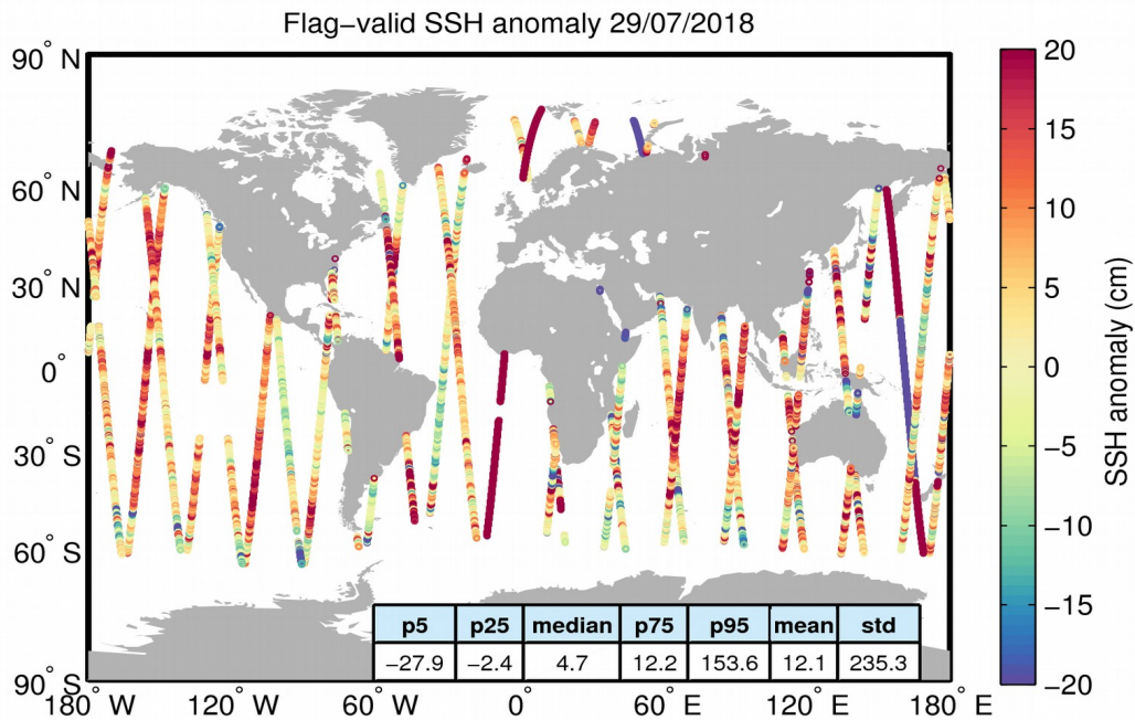
Figure 5. Geographical distribution of flag-valid 1-Hz SSH anomaly data over oceans and lakes for 29/07/2018. The statistical values shown in the table refer to the SSH anomaly in cm and are calculated over all measurements shown in the figure.
