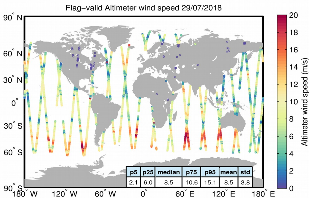
Figure 31. Geographical distribution of flag-valid wind data over oceans and lakes for 29/07/2018. The statistical values shown in the table refer to the wind in m/s and are calculated over all measurements shown in the figure.
