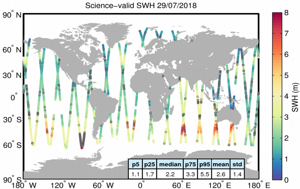
Figure 19. Geographical distribution of science-valid SWH data over oceans and lakes for 29/07/2018. The statistical values shown in the table refer to the SWH in m and are calculated over all measurements shown in the figure. Gray circles denote records that have been rejected based on the editing criteria described in Table 3.
