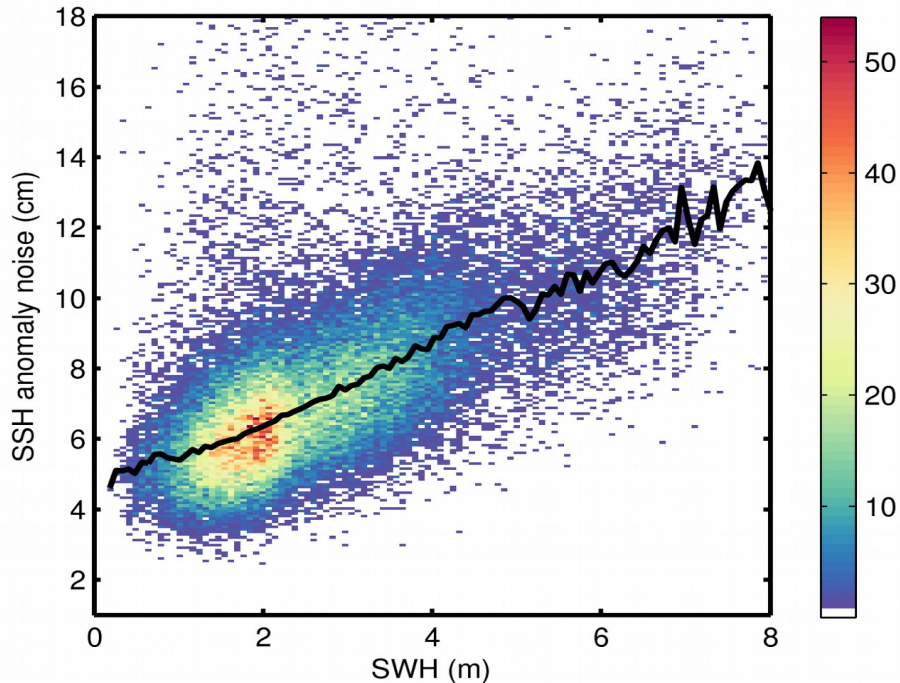
Figure 9. 2D histogram showing flag-valid SSH anomaly noise as a function of SWH for 29/07/2018. The black line denotes the median SSH anomaly noise as a function of SWH.
