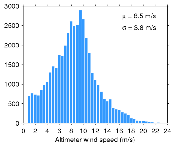
Figure 35. Histogram of science-valid wind over oceans and lakes for 29/07/2018. The mean ( \mu ) and standard deviation ( \sigma ) are also shown. Note that values larger than 24 m/s are excluded from the histogram for the sake of readability but not from the computation of \mu and \sigma .
