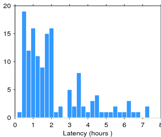
Figure 2. Histogram of the data latency for 28/07/2018. The y-axis denotes the number of files that are made available with a delay of x-hours with respect to the mean time of the records stored in the file.
