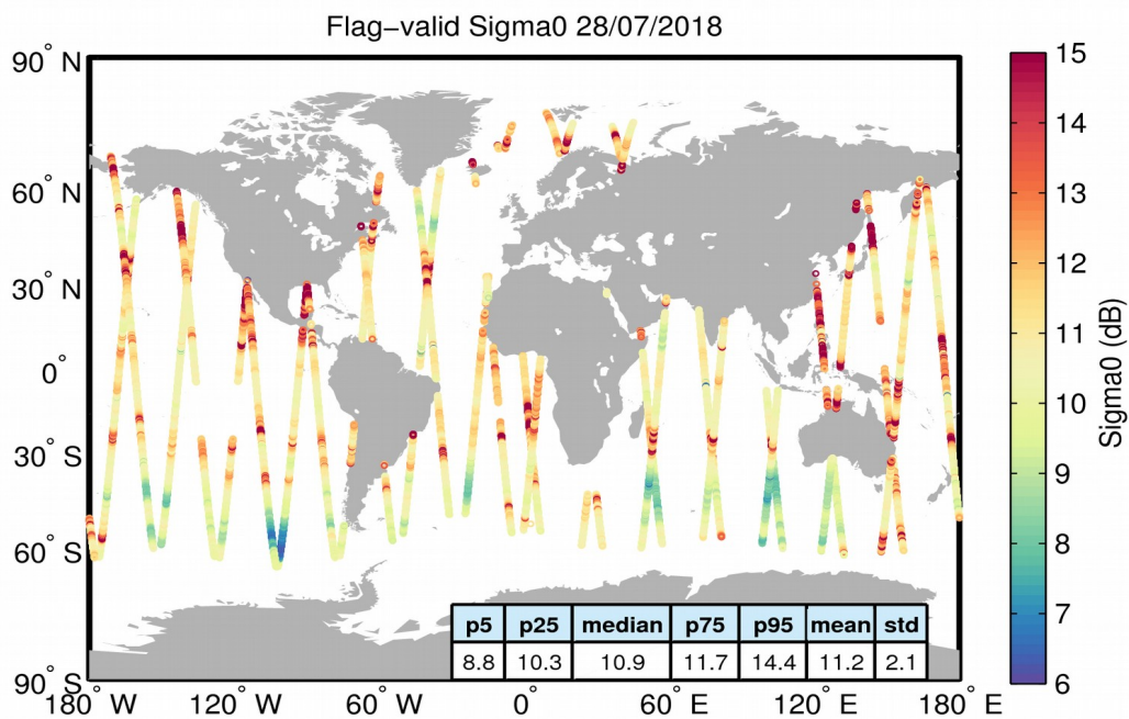
Figure 23. Geographical distribution of flag-valid sigma0 data over oceans and lakes for 28/07/2018. The statistical values shown in the table refer to the sigma0 in dB and are calculated over all measurements shown in the figure.
