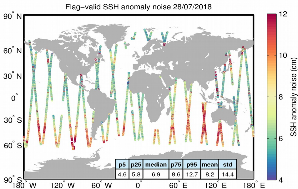
Figure 8. Geographical distribution of flag-valid 20-Hz SSH anomaly measurement noise over oceans and lakes for 28/07/2018. The statistical values shown in the table refer to the SSH anomaly noise and are calculated over all measurements shown in the figure.
