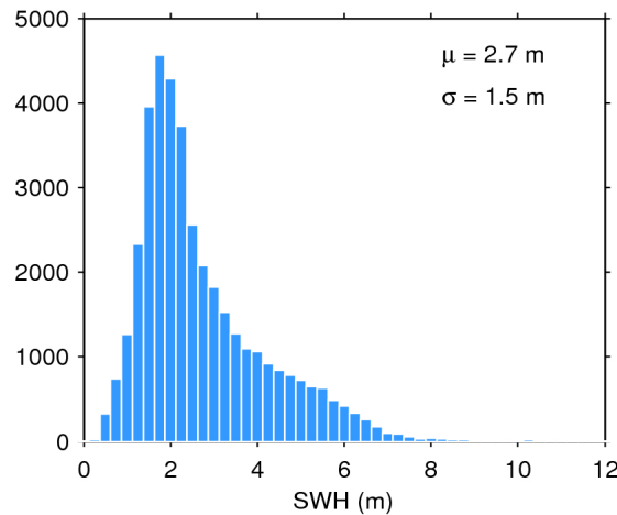
Figure 20. Histogram of science-valid SWH over oceans and lakes for 28/07/2018. The mean ( \mu ) and standard deviation ( \sigma ) are also shown. Note that values larger than 12 m are excluded from the histogram for the sake of readability but not from the computation of \mu and \sigma .
