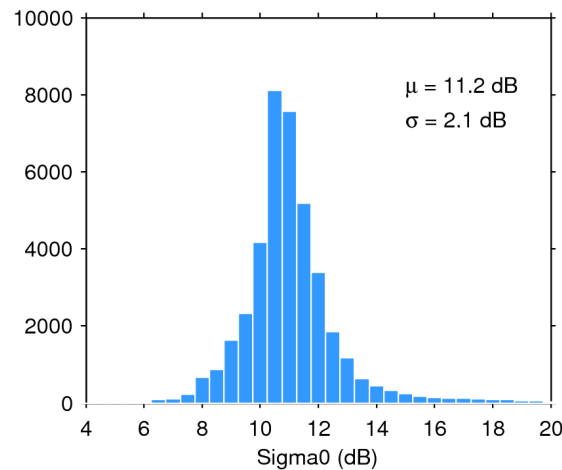
Figure 25. Histogram of flag-valid sigma0 over oceans and lakes for 28/07/2018. The mean ( \mu ) and standard deviation ( \sigma ) are also shown. Note that values outside [4 20] dB are excluded from the histogram for the sake of readability but not from the computation of \mu and \sigma .
