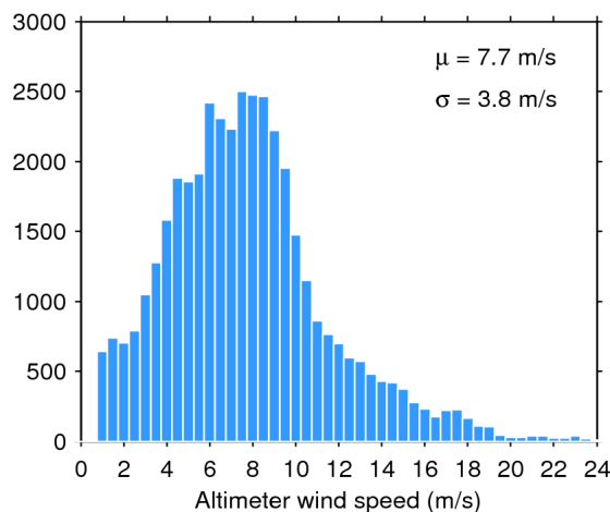
Figure 35. Histogram of science-valid wind over oceans and lakes for 28/07/2018. The mean ( \mu ) and standard deviation ( \sigma ) are also shown. Note that values larger than 24 m/s are excluded from the histogram for the sake of readability but not from the computation of \mu and \sigma .
