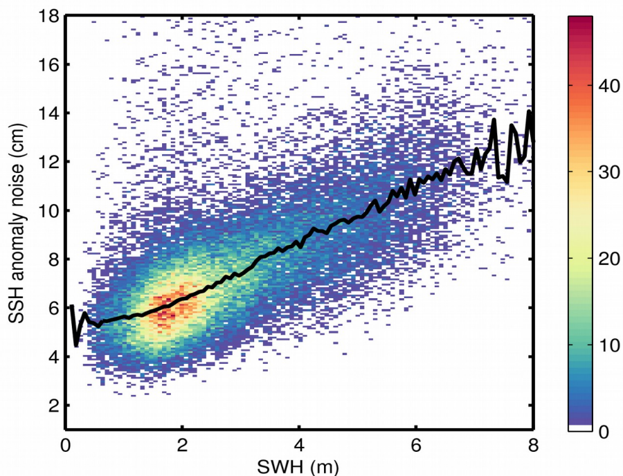
Figure 9. 2D histogram showing flag-valid SSH anomaly noise as a function of SWH for 28/07/2018. The black line denotes the median SSH anomaly noise as a function of SWH.
