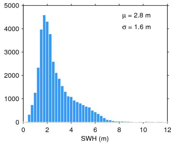
Figure 17. Histogram of flag-valid SWH over oceans and lakes for 28/07/2018. The mean ( \mu ) and standard deviation ( \sigma ) are also shown. Note that values larger than 12 m are excluded from the histogram for the sake of readability but not from the computation of \mu and \sigma .
