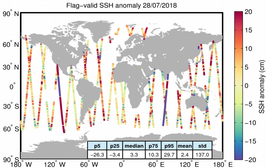
Figure 5. Geographical distribution of flag-valid 1-Hz SSH anomaly data over oceans and lakes for 28/07/2018. The statistical values shown in the table refer to the SSH anomaly in cm and are calculated over all measurements shown in the figure.
