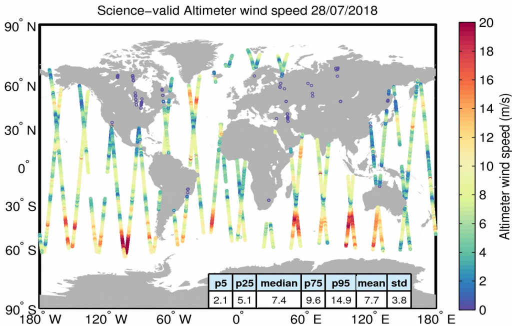
Figure 34. Geographical distribution of science-valid wind data over oceans and lakes for 28/07/2018. The statistical values shown in the table refer to the wind in m/s and are calculated over all measurements shown in the figure. Gray circles denote records that have been rejected based on the editing criteria described in Table 5.
