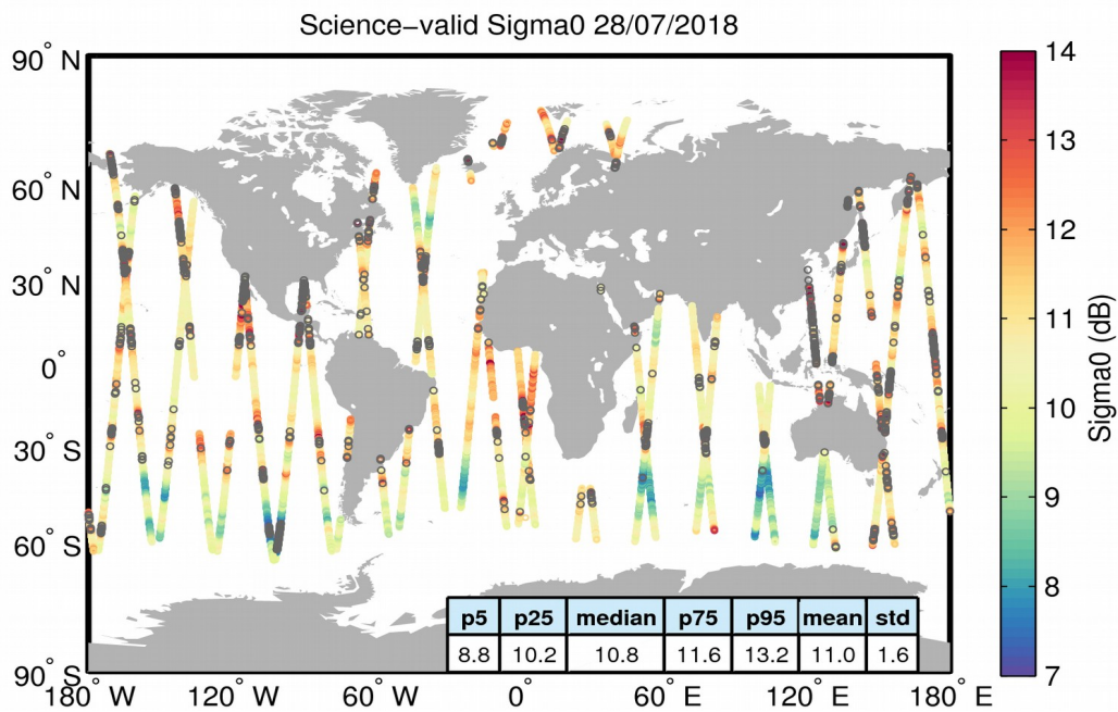
Figure 27. Geographical distribution of science-valid sigma0 data over oceans and lakes for 28/07/2018. The statistical values shown in the table refer to the sigma0 in dB and are calculated over all measurements shown in the figure. Gray circles denote records that have been rejected based on the editing criteria described in Table 4.
