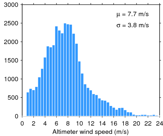
Figure 33. Histogram of flag-valid wind over oceans and lakes for 28/07/2018. The mean ( \mu ) and standard deviation ( \sigma ) are also shown. Note that values larger than 24 m/s are excluded from the histogram for the sake of readability but not from the computation of \mu and \sigma .
