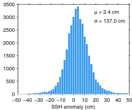
Figure 7. Histogram of flag-valid SSH anomaly over oceans and lakes for 28/07/2018. The mean ( \mu ) and standard deviation ( \sigma ) are also shown. Note that values outside [-50 50] cm are excluded from the histogram for the sake of readability but not from the computation of \mu and \sigma .
