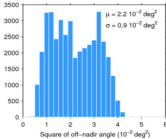
Figure 39. Histogram of flag-valid mispointing over oceans and lakes for 28/07/2018. The mean ( \mu ) and standard deviation ( \sigma ) are also shown. Note that values larger than 6 \cdot 10^{-2} \text{ deg}^2 are excluded from the histogram for the sake of readability but not from the computation of \mu and \sigma .
