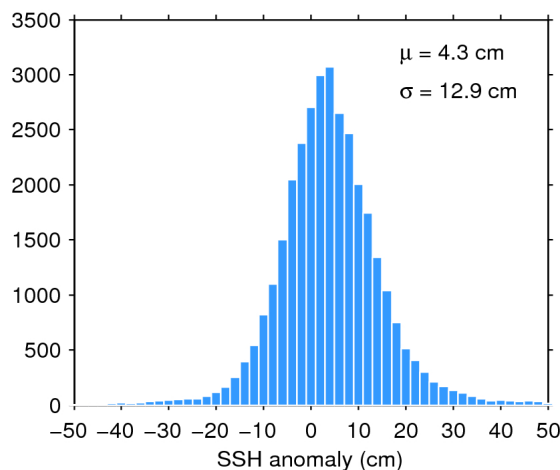
Figure 11. Histogram of science-valid SSH anomaly over oceans and lakes for 28/07/2018. The mean ( \mu ) and standard deviation ( \sigma ) are also shown. Note that values outside [-50 50] cm are excluded from the histogram for the sake of readability but not from the computation of \mu and \sigma .
