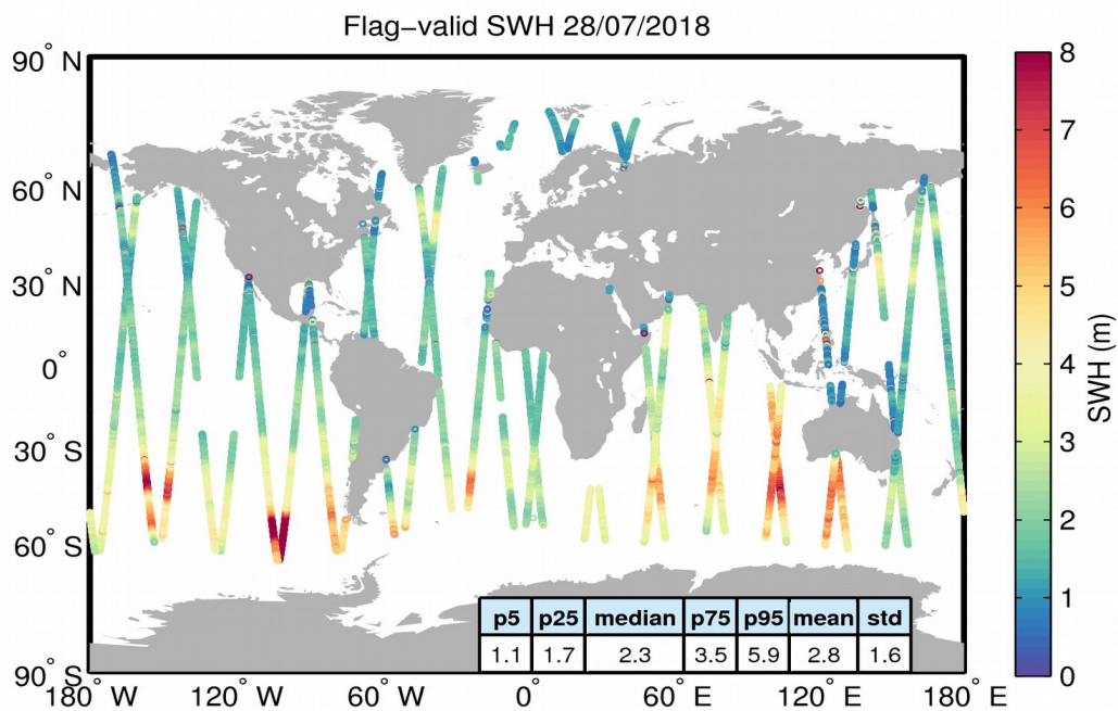
Figure 15. Geographical distribution of flag-valid SWH data over oceans and lakes for 28/07/2018. The statistical values shown in the table refer to the SWH in m and are calculated over all measurements shown in the figure.
