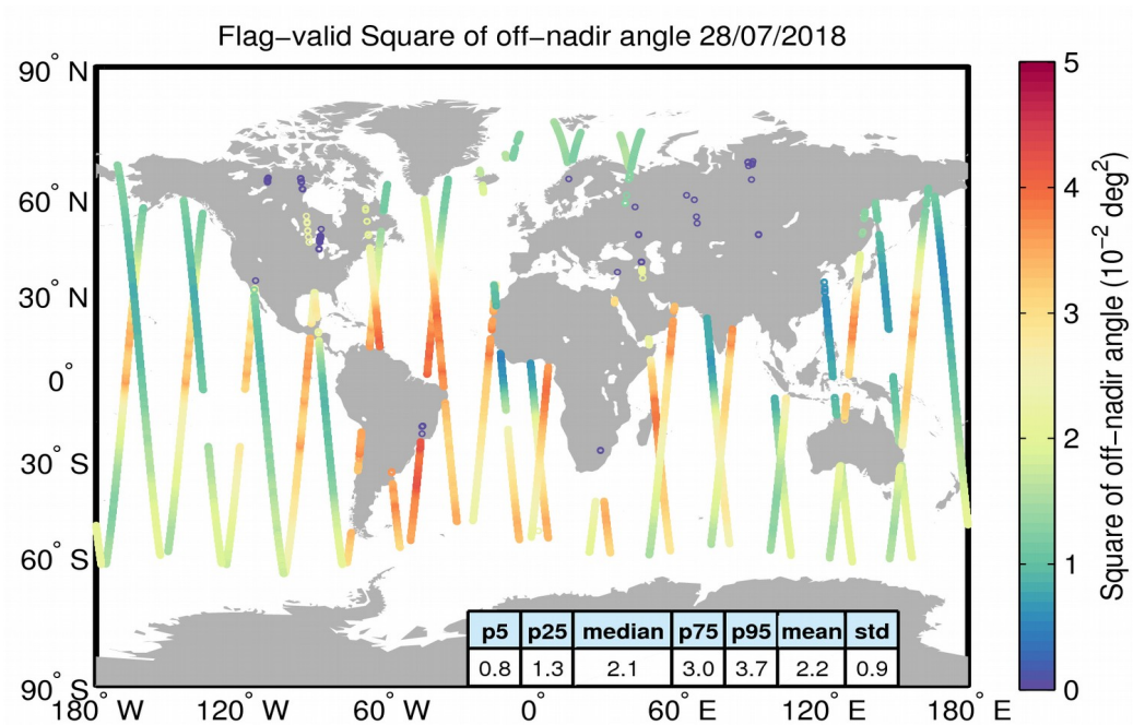
Figure 37. Geographical distribution of flag-valid mispointing data over oceans and lakes for 28/07/2018. The statistical values shown in the table refer to the mispointing in 10^{-2} \text{ deg}^2 and are calculated over all measurements shown in the figure.
