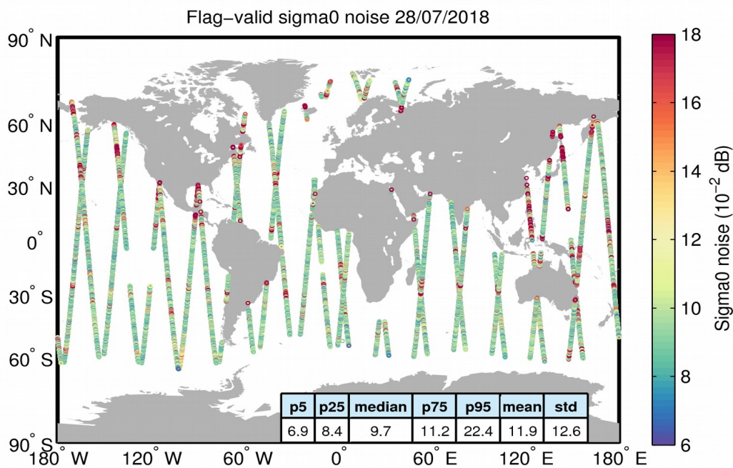
Figure 26. Geographical distribution of flag-valid 20-Hz sigma0 measurement noise over oceans and lakes for 28/07/2018. The statistical values shown in the table refer to the sigma0 noise and are calculated over all measurements shown in the figure.
