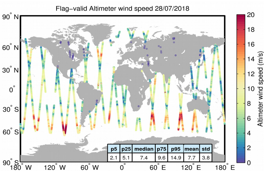
Figure 31. Geographical distribution of flag-valid wind data over oceans and lakes for 28/07/2018. The statistical values shown in the table refer to the wind in m/s and are calculated over all measurements shown in the figure.
