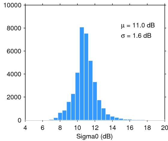
Figure 28. Histogram of science-valid sigma0 over oceans and lakes for 28/07/2018. The mean ( \mu ) and standard deviation ( \sigma ) are also shown. Note that values outside [4 20] dB are excluded from the histogram for the sake of readability but not from the computation of \mu and \sigma .
