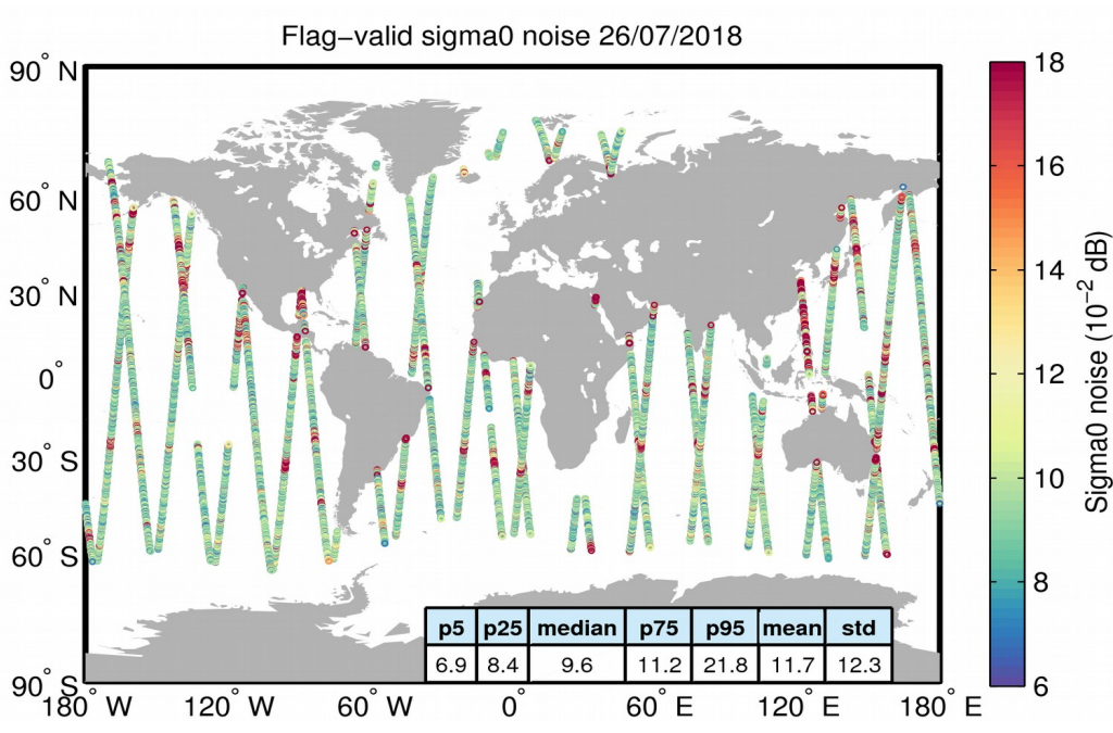
Figure 26. Geographical distribution of flag-valid 20-Hz sigma0 measurement noise over oceans and lakes for 26/07/2018. The statistical values shown in the table refer to the sigma0 noise and are calculated over all measurements shown in the figure.
