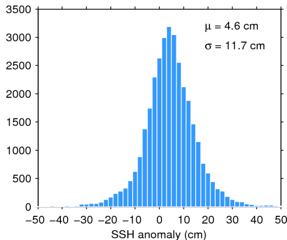
Figure 11. Histogram of science-valid SSH anomaly over oceans and lakes for 26/07/2018. The mean ( \mu ) and standard deviation ( \sigma ) are also shown. Note that values outside [-50 50] cm are excluded from the histogram for the sake of readability but not from the computation of \mu and \sigma .
