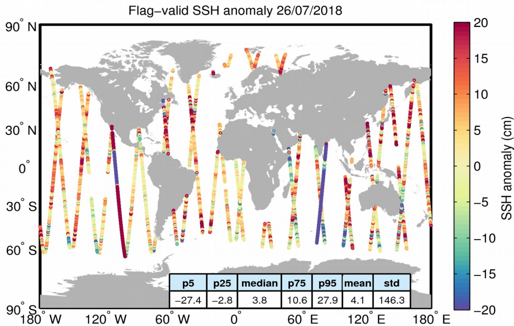
Figure 5. Geographical distribution of flag-valid 1-Hz SSH anomaly data over oceans and lakes for 26/07/2018. The statistical values shown in the table refer to the SSH anomaly in cm and are calculated over all measurements shown in the figure.
