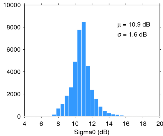
Figure 28. Histogram of science-valid sigma0 over oceans and lakes for 26/07/2018. The mean ( \mu ) and standard deviation ( \sigma ) are also shown. Note that values outside [4 20] dB are excluded from the histogram for the sake of readability but not from the computation of \mu and \sigma .
