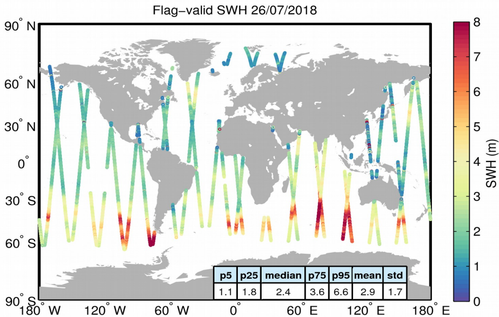
Figure 15. Geographical distribution of flag-valid SWH data over oceans and lakes for 26/07/2018. The statistical values shown in the table refer to the SWH in m and are calculated over all measurements shown in the figure.
