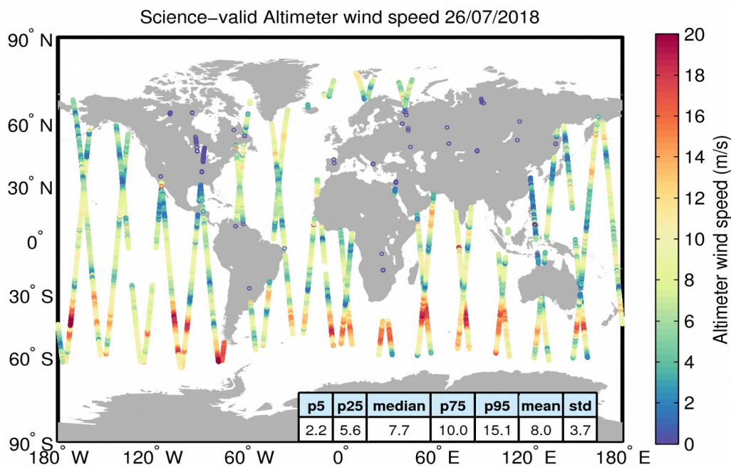
Figure 34. Geographical distribution of science-valid wind data over oceans and lakes for 26/07/2018. The statistical values shown in the table refer to the wind in m/s and are calculated over all measurements shown in the figure. Gray circles denote records that have been rejected based on the editing criteria described in Table 5.
