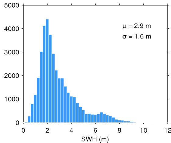
Figure 20. Histogram of science-valid SWH over oceans and lakes for 26/07/2018. The mean ( \mu ) and standard deviation ( \sigma ) are also shown. Note that values larger than 12 m are excluded from the histogram for the sake of readability but not from the computation of \mu and \sigma .
