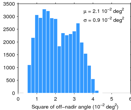
Figure 39. Histogram of flag-valid mispointing over oceans and lakes for 26/07/2018. The mean ( \mu ) and standard deviation ( \sigma ) are also shown. Note that values larger than 6 \cdot 10^{-2} \text{ deg}^2 are excluded from the histogram for the sake of readability but not from the computation of \mu and \sigma .
