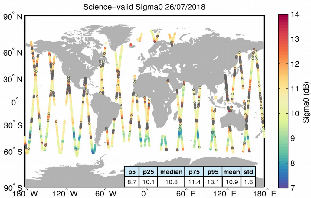
Figure 27. Geographical distribution of science-valid sigma0 data over oceans and lakes for 26/07/2018. The statistical values shown in the table refer to the sigma0 in dB and are calculated over all measurements shown in the figure. Gray circles denote records that have been rejected based on the editing criteria described in Table 4.
