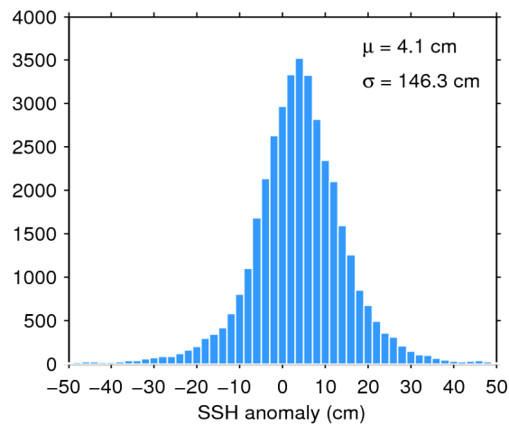
Figure 7. Histogram of flag-valid SSH anomaly over oceans and lakes for 26/07/2018. The mean ( \mu ) and standard deviation ( \sigma ) are also shown. Note that values outside [-50 50] cm are excluded from the histogram for the sake of readability but not from the computation of \mu and \sigma .
