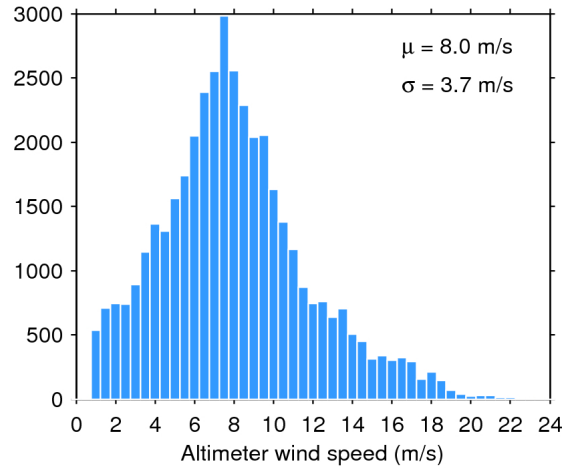
Figure 33. Histogram of flag-valid wind over oceans and lakes for 26/07/2018. The mean ( \mu ) and standard deviation ( \sigma ) are also shown. Note that values larger than 24 m/s are excluded from the histogram for the sake of readability but not from the computation of \mu and \sigma .
