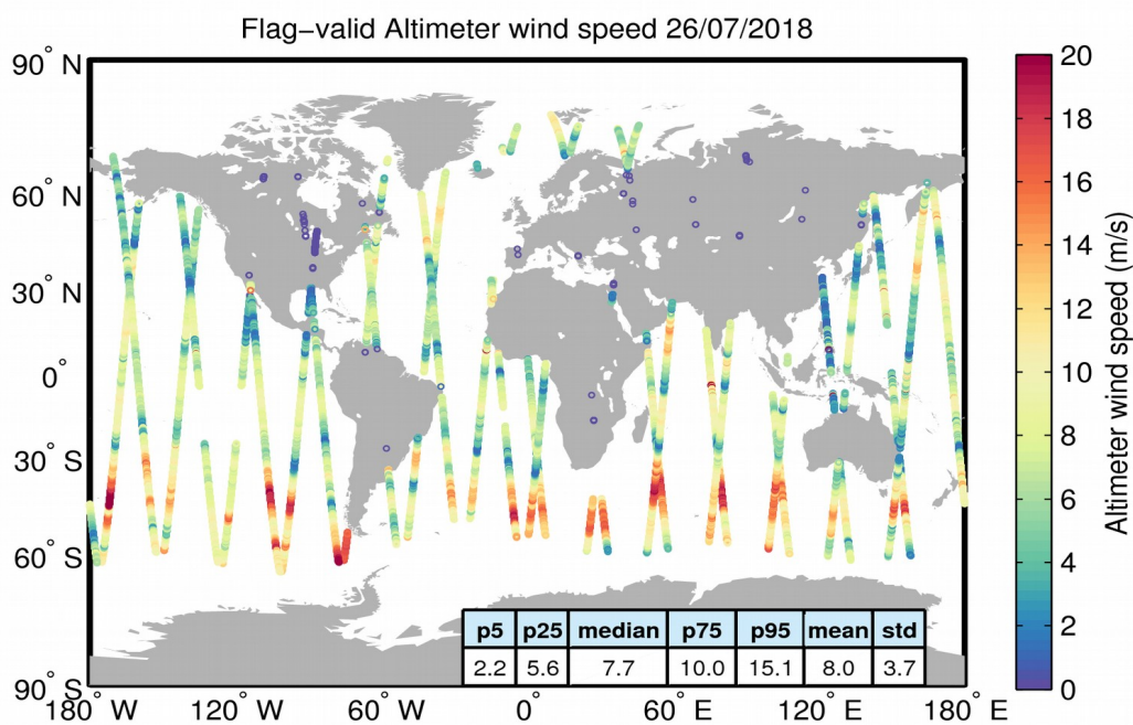
Figure 31. Geographical distribution of flag-valid wind data over oceans and lakes for 26/07/2018. The statistical values shown in the table refer to the wind in m/s and are calculated over all measurements shown in the figure.
