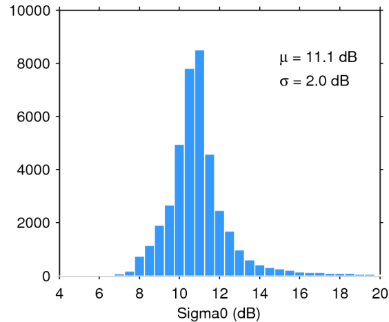
Figure 25. Histogram of flag-valid sigma0 over oceans and lakes for 26/07/2018. The mean ( \mu ) and standard deviation ( \sigma ) are also shown. Note that values outside [4 20] dB are excluded from the histogram for the sake of readability but not from the computation of \mu and \sigma .
