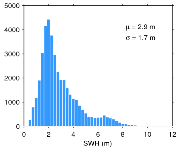
Figure 17. Histogram of flag-valid SWH over oceans and lakes for 26/07/2018. The mean ( \mu ) and standard deviation ( \sigma ) are also shown. Note that values larger than 12 m are excluded from the histogram for the sake of readability but not from the computation of \mu and \sigma .
