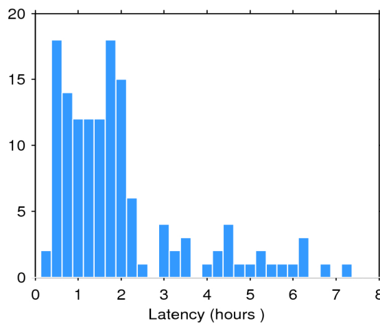
Figure 2. Histogram of the data latency for 26/07/2018. The y-axis denotes the number of files that are made available with a delay of x-hours with respect to the mean time of the records stored in the file.
