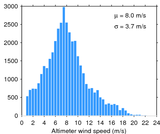
Figure 35. Histogram of science-valid wind over oceans and lakes for 26/07/2018. The mean ( \mu ) and standard deviation ( \sigma ) are also shown. Note that values larger than 24 m/s are excluded from the histogram for the sake of readability but not from the computation of \mu and \sigma .
