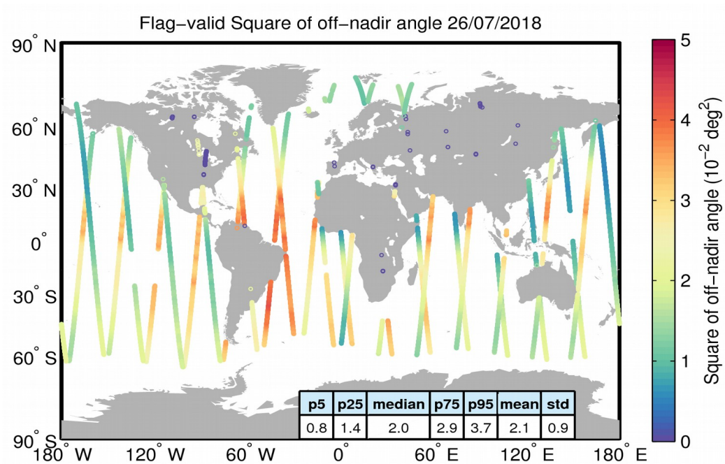
Figure 37. Geographical distribution of flag-valid mispointing data over oceans and lakes for 26/07/2018. The statistical values shown in the table refer to the mispointing in 10^{-2} \text{ deg}^2 and are calculated over all measurements shown in the figure.
