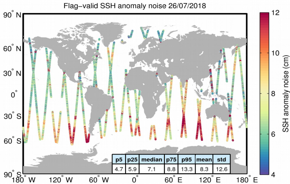
Figure 8. Geographical distribution of flag-valid 20-Hz SSH anomaly measurement noise over oceans and lakes for 26/07/2018. The statistical values shown in the table refer to the SSH anomaly noise and are calculated over all measurements shown in the figure.
