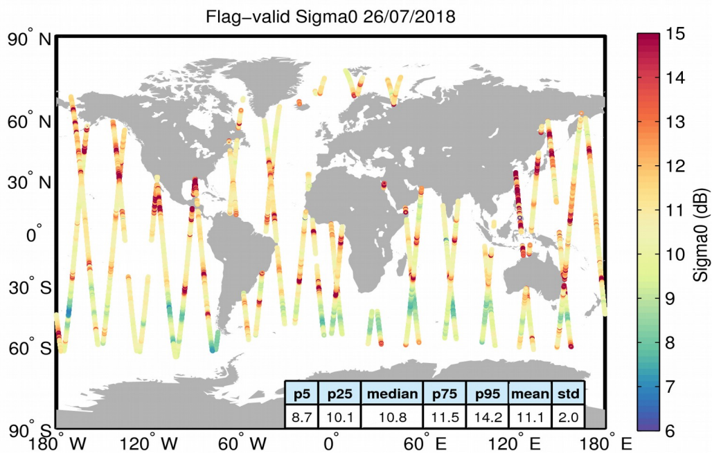
Figure 23. Geographical distribution of flag-valid sigma0 data over oceans and lakes for 26/07/2018. The statistical values shown in the table refer to the sigma0 in dB and are calculated over all measurements shown in the figure.
