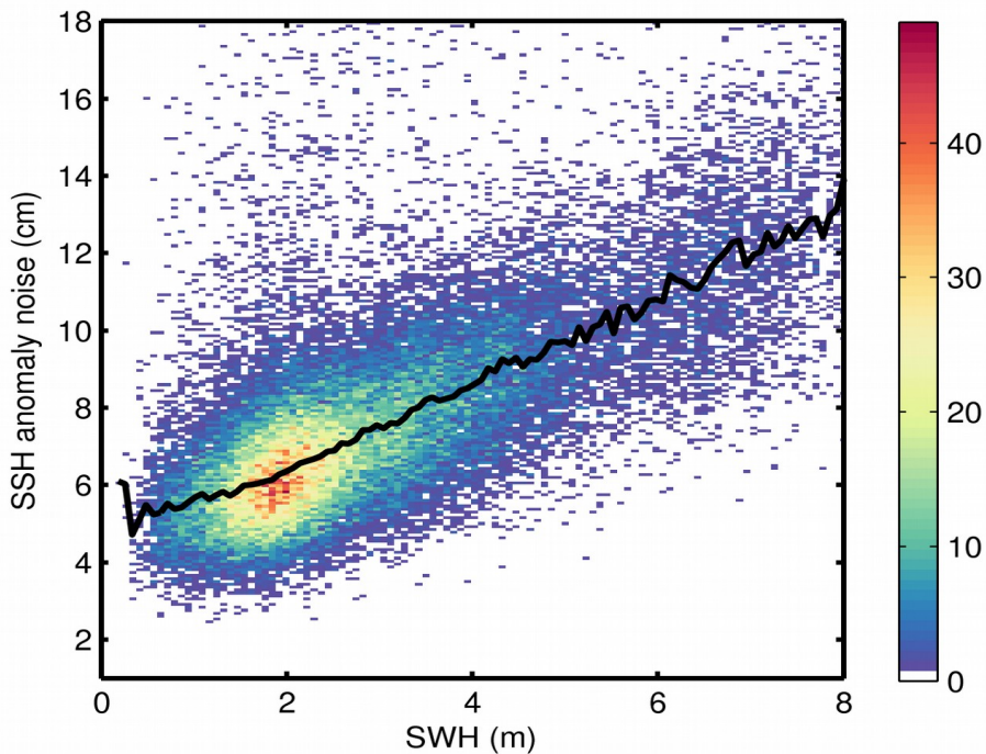
Figure 9. 2D histogram showing flag-valid SSH anomaly noise as a function of SWH for 26/07/2018. The black line denotes the median SSH anomaly noise as a function of SWH.
