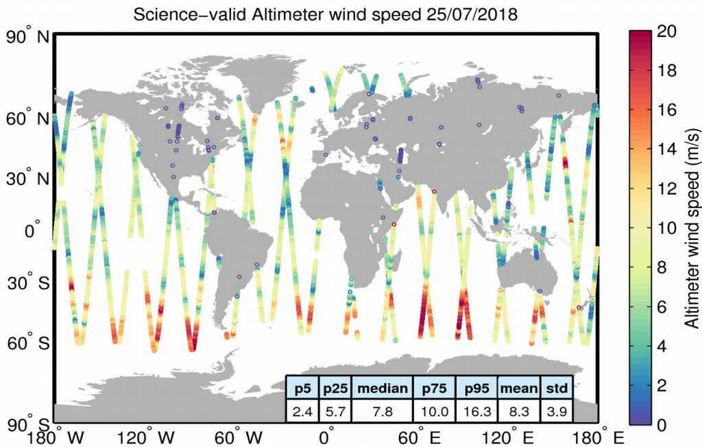
Figure 34. Geographical distribution of science-valid wind data over oceans and lakes for 25/07/2018. The statistical values shown in the table refer to the wind in m/s and are calculated over all measurements shown in the figure. Gray circles denote records that have been rejected based on the editing criteria described in Table 5.
