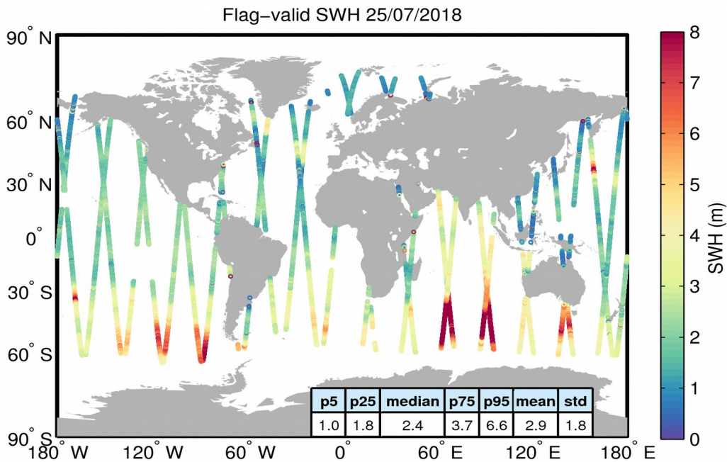
Figure 15. Geographical distribution of flag-valid SWH data over oceans and lakes for 25/07/2018. The statistical values shown in the table refer to the SWH in m and are calculated over all measurements shown in the figure.
