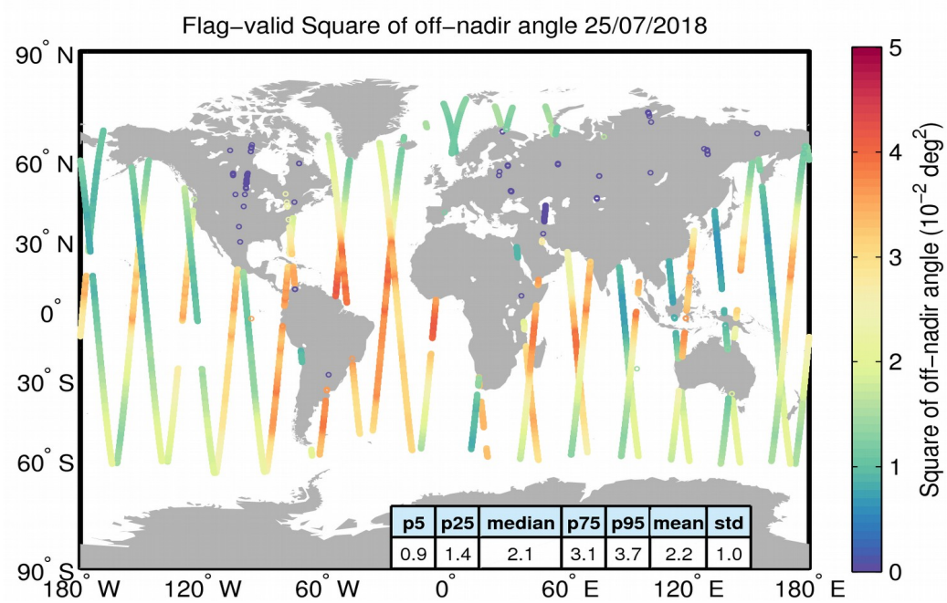
Figure 37. Geographical distribution of flag-valid mispointing data over oceans and lakes for 25/07/2018. The statistical values shown in the table refer to the mispointing in 10^{-2} deg 2 and are calculated over all measurements shown in the figure.
