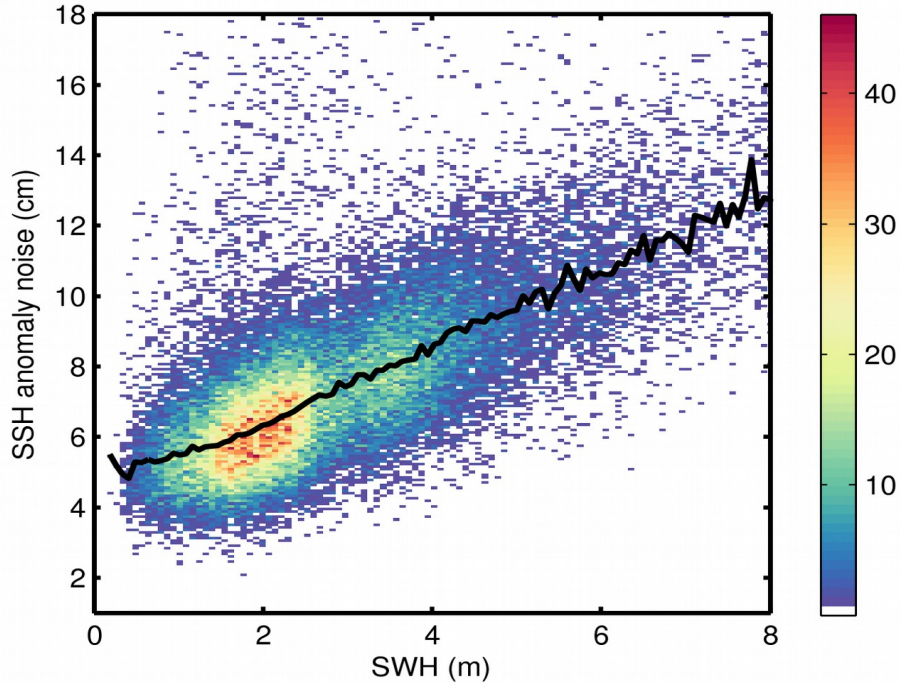
Figure 9. 2D histogram showing flag-valid SSH anomaly noise as a function of SWH for 25/07/2018. The black line denotes the median SSH anomaly noise as a function of SWH.
