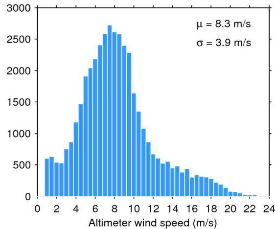
Figure 33. Histogram of flag-valid wind over oceans and lakes for 25/07/2018. The mean ( \mu ) and standard deviation ( \sigma ) are also shown. Note that values larger than 24 m/s are excluded from the histogram for the sake of readability but not from the computation of \mu and \sigma .
