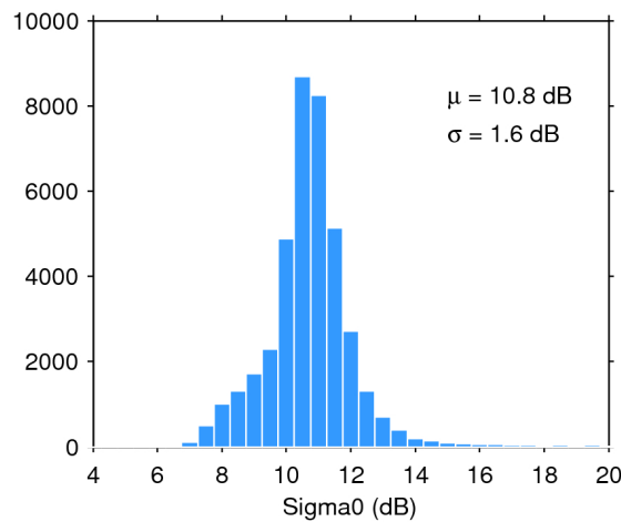
Figure 28. Histogram of science-valid sigma0 over oceans and lakes for 25/07/2018. The mean ( \mu ) and standard deviation ( \sigma ) are also shown. Note that values outside [4 20] dB are excluded from the histogram for the sake of readability but not from the computation of \mu and \sigma .
