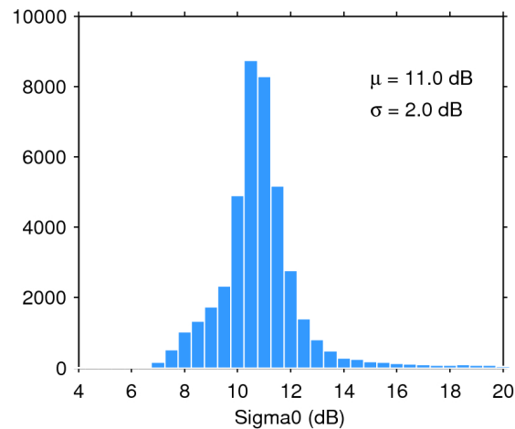
Figure 25. Histogram of flag-valid sigma0 over oceans and lakes for 25/07/2018. The mean ( \mu ) and standard deviation ( \sigma ) are also shown. Note that values outside [4 20] dB are excluded from the histogram for the sake of readability but not from the computation of \mu and \sigma .
