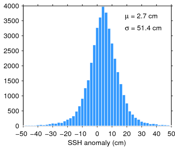
Figure 7. Histogram of flag-valid SSH anomaly over oceans and lakes for 25/07/2018. The mean ( \mu ) and standard deviation ( \sigma ) are also shown. Note that values outside [-50 50] cm are excluded from the histogram for the sake of readability but not from the computation of \mu and \sigma .
