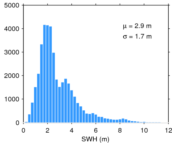
Figure 20. Histogram of science-valid SWH over oceans and lakes for 25/07/2018. The mean ( \mu ) and standard deviation ( \sigma ) are also shown. Note that values larger than 12 m are excluded from the histogram for the sake of readability but not from the computation of \mu and \sigma .
