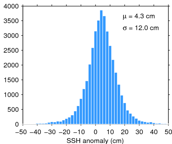
Figure 11. Histogram of science-valid SSH anomaly over oceans and lakes for 25/07/2018. The mean ( \mu ) and standard deviation ( \sigma ) are also shown. Note that values outside [-50 50] cm are excluded from the histogram for the sake of readability but not from the computation of \mu and \sigma .
