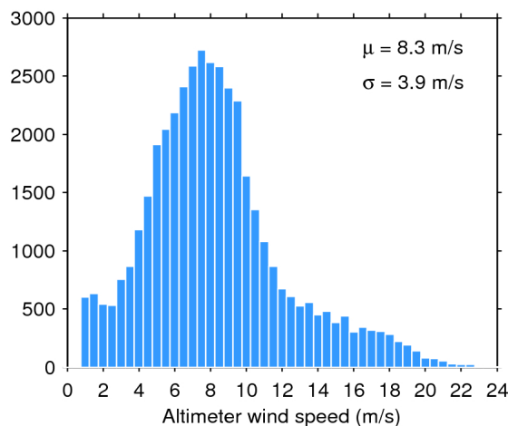
Figure 35. Histogram of science-valid wind over oceans and lakes for 25/07/2018. The mean ( \mu ) and standard deviation ( \sigma ) are also shown. Note that values larger than 24 m/s are excluded from the histogram for the sake of readability but not from the computation of \mu and \sigma .
