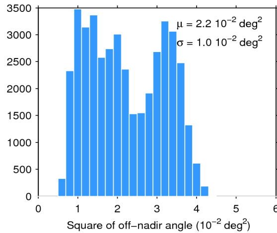
Figure 39. Histogram of flag-valid mispointing over oceans and lakes for 25/07/2018. The mean ( \mu ) and standard deviation ( \sigma ) are also shown. Note that values larger than 6 \cdot 10^{-2} \text{ deg}^2 are excluded from the histogram for the sake of readability but not from the computation of \mu and \sigma .
