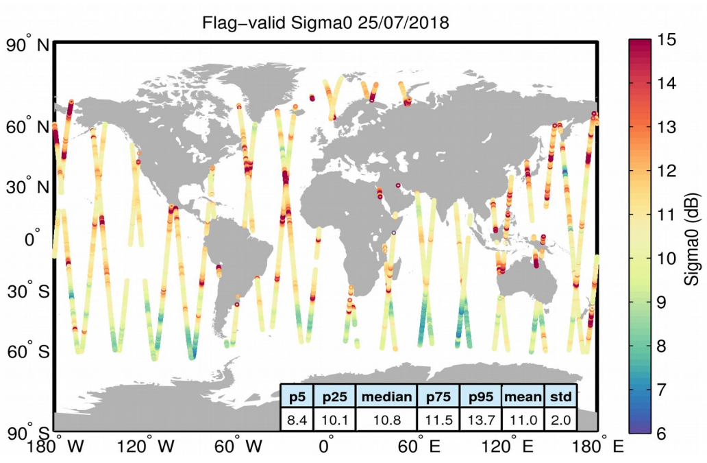
Figure 23. Geographical distribution of flag-valid sigma0 data over oceans and lakes for 25/07/2018. The statistical values shown in the table refer to the sigma0 in dB and are calculated over all measurements shown in the figure.
