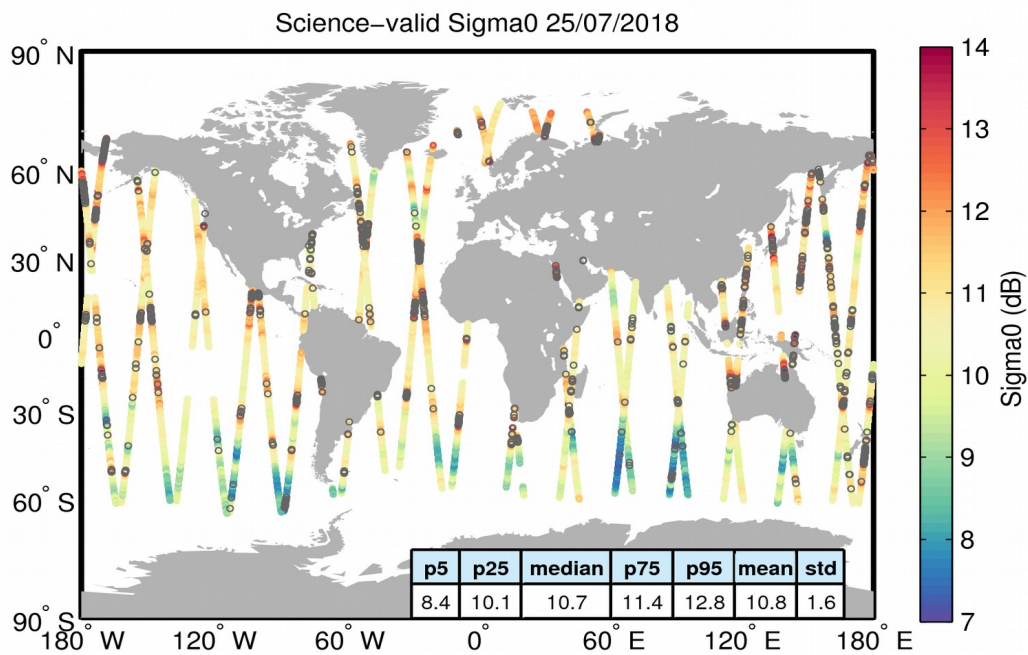
Figure 27. Geographical distribution of science-valid sigma0 data over oceans and lakes for 25/07/2018. The statistical values shown in the table refer to the sigma0 in dB and are calculated over all measurements shown in the figure. Gray circles denote records that have been rejected based on the editing criteria described in Table 4.
