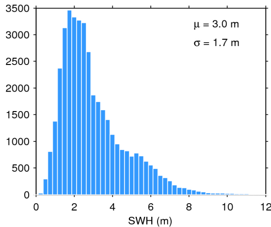
Figure 20. Histogram of science-valid SWH over oceans and lakes for 24/07/2018. The mean ( \mu ) and standard deviation ( \sigma ) are also shown. Note that values larger than 12 m are excluded from the histogram for the sake of readability but not from the computation of \mu and \sigma .
