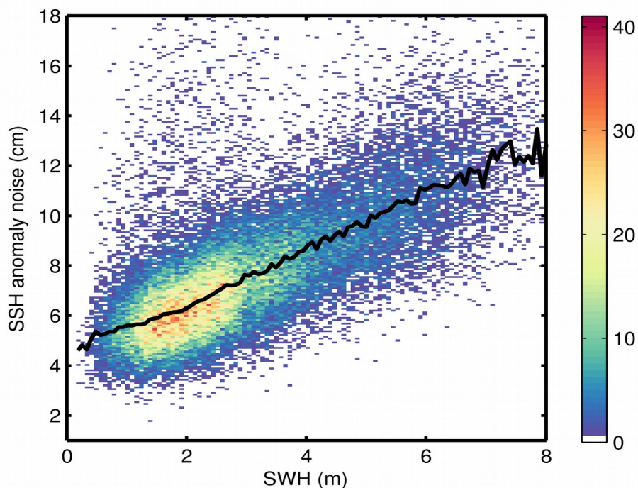
Figure 9. 2D histogram showing flag-valid SSH anomaly noise as a function of SWH for 24/07/2018. The black line denotes the median SSH anomaly noise as a function of SWH.
