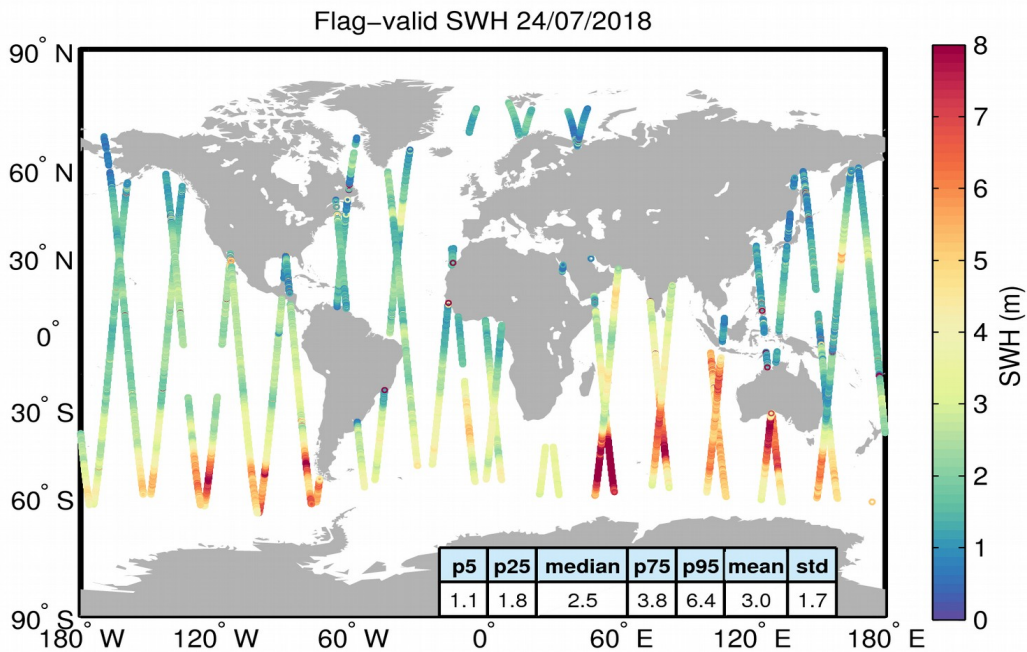
Figure 15. Geographical distribution of flag-valid SWH data over oceans and lakes for 24/07/2018. The statistical values shown in the table refer to the SWH in m and are calculated over all measurements shown in the figure.
