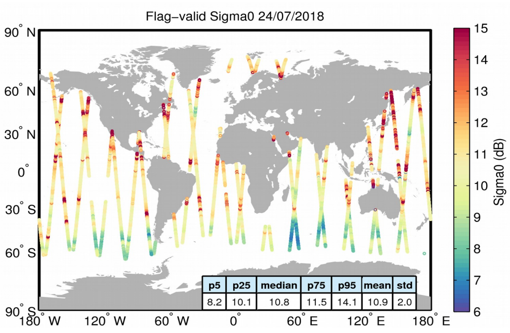
Figure 23. Geographical distribution of flag-valid sigma0 data over oceans and lakes for 24/07/2018. The statistical values shown in the table refer to the sigma0 in dB and are calculated over all measurements shown in the figure.
