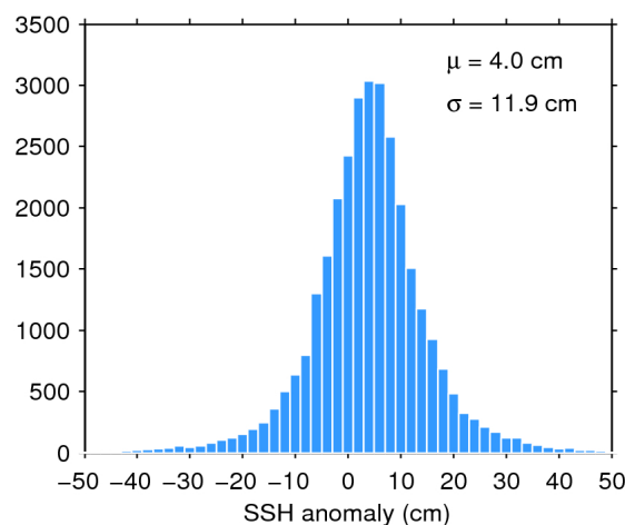
Figure 11. Histogram of science-valid SSH anomaly over oceans and lakes for 24/07/2018. The mean ( \mu ) and standard deviation ( \sigma ) are also shown. Note that values outside [-50 50] cm are excluded from the histogram for the sake of readability but not from the computation of \mu and \sigma .
