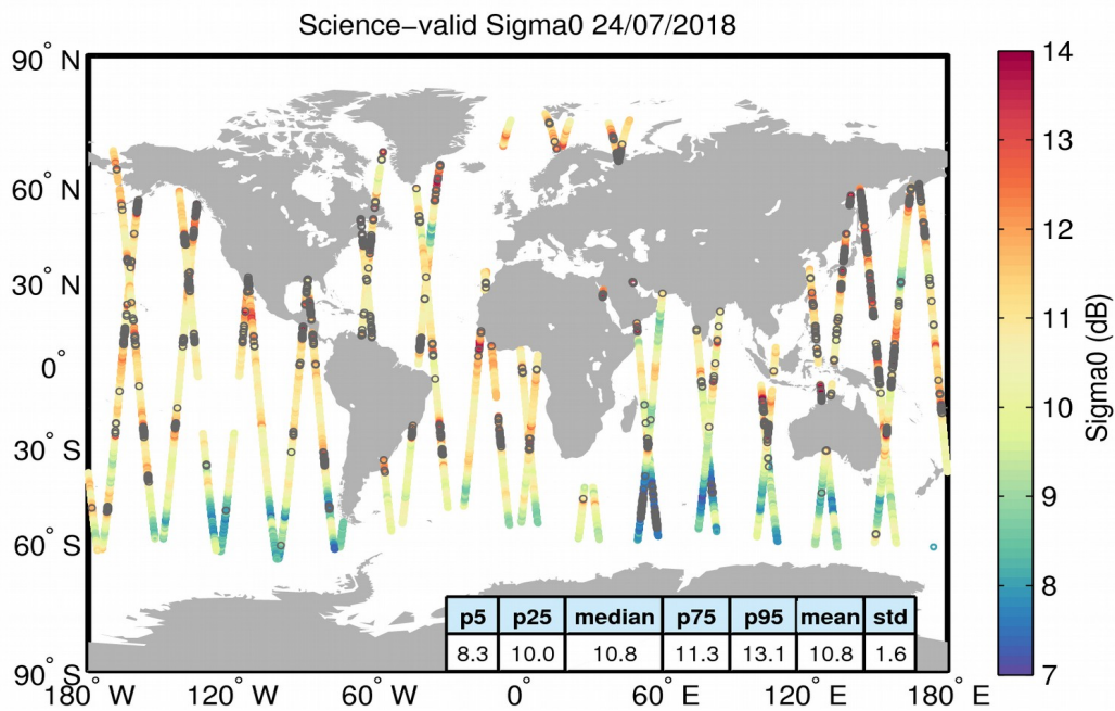
Figure 27. Geographical distribution of science-valid sigma0 data over oceans and lakes for 24/07/2018. The statistical values shown in the table refer to the sigma0 in dB and are calculated over all measurements shown in the figure. Gray circles denote records that have been rejected based on the editing criteria described in Table 4.
