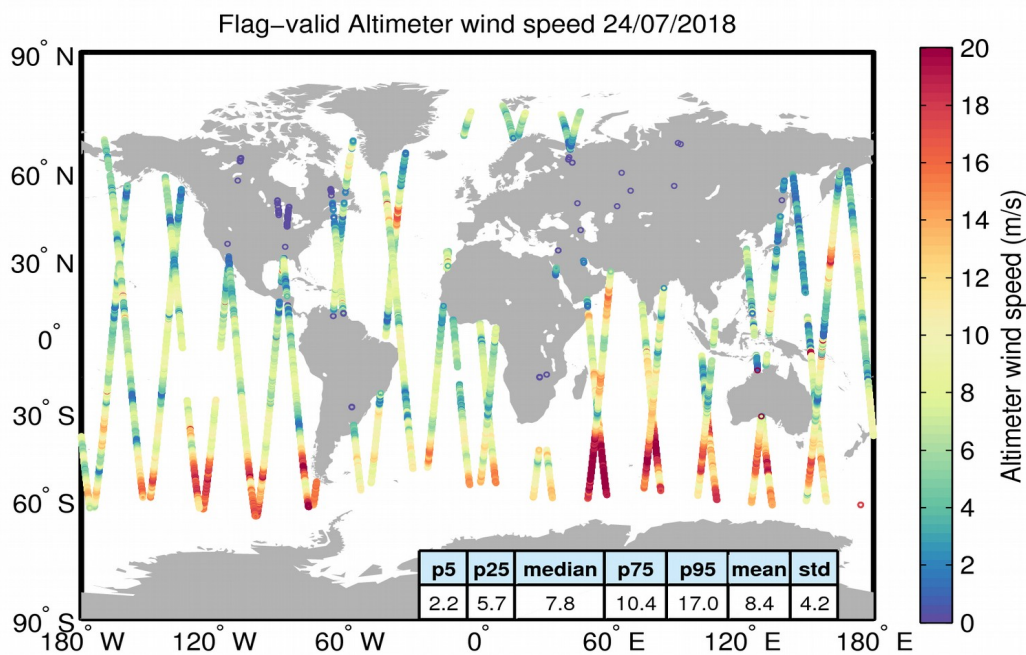
Figure 31. Geographical distribution of flag-valid wind data over oceans and lakes for 24/07/2018. The statistical values shown in the table refer to the wind in m/s and are calculated over all measurements shown in the figure.
