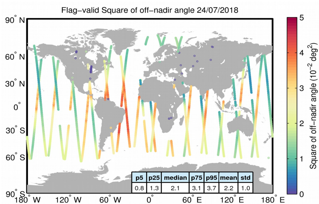
Figure 37. Geographical distribution of flag-valid mispointing data over oceans and lakes for 24/07/2018. The statistical values shown in the table refer to the mispointing in 10^{-2} \text{ deg}^2 and are calculated over all measurements shown in the figure.
