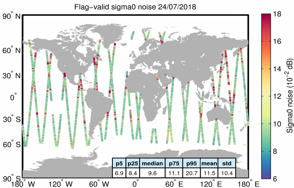
Figure 26. Geographical distribution of flag-valid 20-Hz sigma0 measurement noise over oceans and lakes for 24/07/2018. The statistical values shown in the table refer to the sigma0 noise and are calculated over all measurements shown in the figure.
