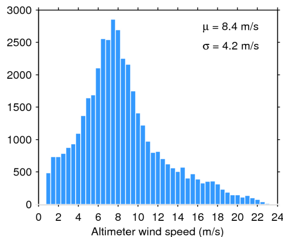
Figure 35. Histogram of science-valid wind over oceans and lakes for 24/07/2018. The mean ( \mu ) and standard deviation ( \sigma ) are also shown. Note that values larger than 24 m/s are excluded from the histogram for the sake of readability but not from the computation of \mu and \sigma .
