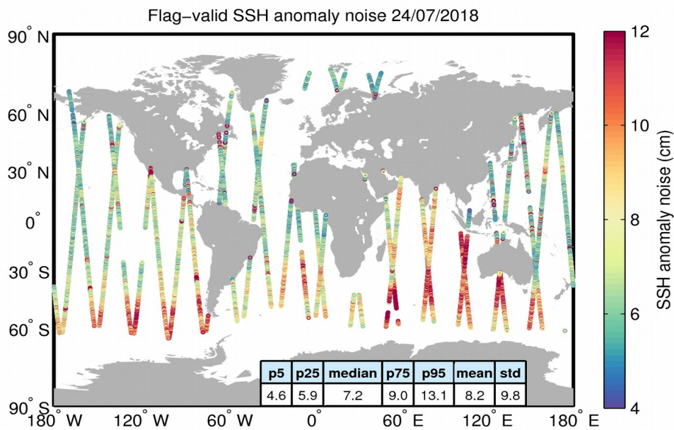
Figure 8. Geographical distribution of flag-valid 20-Hz SSH anomaly measurement noise over oceans and lakes for 24/07/2018. The statistical values shown in the table refer to the SSH anomaly noise and are calculated over all measurements shown in the figure.
