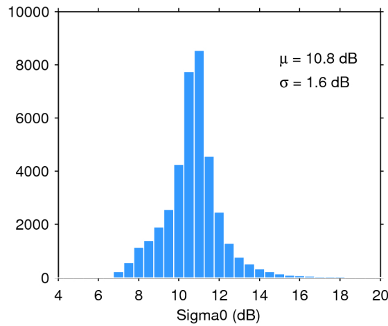
Figure 28. Histogram of science-valid sigma0 over oceans and lakes for 24/07/2018. The mean ( \mu ) and standard deviation ( \sigma ) are also shown. Note that values outside [4 20] dB are excluded from the histogram for the sake of readability but not from the computation of \mu and \sigma .
