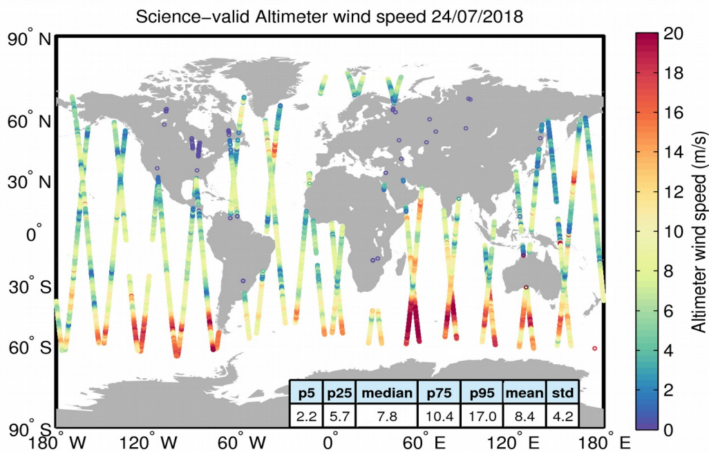
Figure 34. Geographical distribution of science-valid wind data over oceans and lakes for 24/07/2018. The statistical values shown in the table refer to the wind in m/s and are calculated over all measurements shown in the figure. Gray circles denote records that have been rejected based on the editing criteria described in Table 5.
