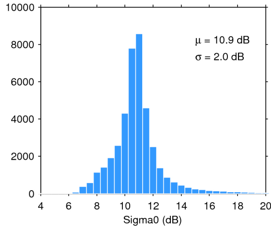
Figure 25. Histogram of flag-valid sigma0 over oceans and lakes for 24/07/2018. The mean ( \mu ) and standard deviation ( \sigma ) are also shown. Note that values outside [4 20] dB are excluded from the histogram for the sake of readability but not from the computation of \mu and \sigma .
