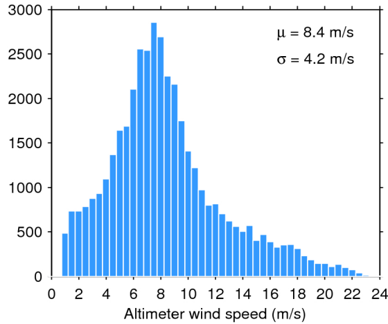
Figure 33. Histogram of flag-valid wind over oceans and lakes for 24/07/2018. The mean ( \mu ) and standard deviation ( \sigma ) are also shown. Note that values larger than 24 m/s are excluded from the histogram for the sake of readability but not from the computation of \mu and \sigma .
