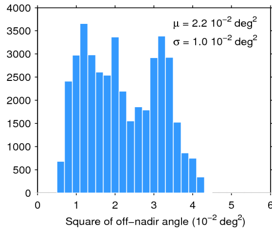
Figure 39. Histogram of flag-valid mispointing over oceans and lakes for 24/07/2018. The mean ( \mu ) and standard deviation ( \sigma ) are also shown. Note that values larger than 6 \cdot 10^{-2} \text{ deg}^2 are excluded from the histogram for the sake of readability but not from the computation of \mu and \sigma .
