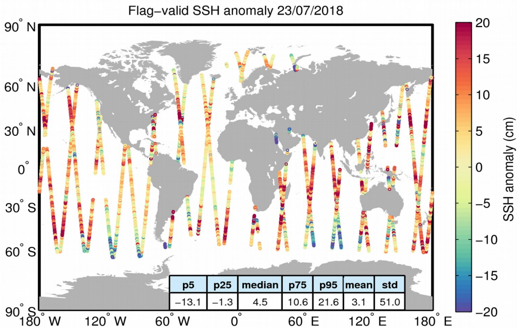
Figure 5. Geographical distribution of flag-valid 1-Hz SSH anomaly data over oceans and lakes for 23/07/2018. The statistical values shown in the table refer to the SSH anomaly in cm and are calculated over all measurements shown in the figure.
