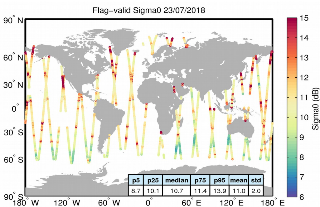
Figure 23. Geographical distribution of flag-valid sigma0 data over oceans and lakes for 23/07/2018. The statistical values shown in the table refer to the sigma0 in dB and are calculated over all measurements shown in the figure.
