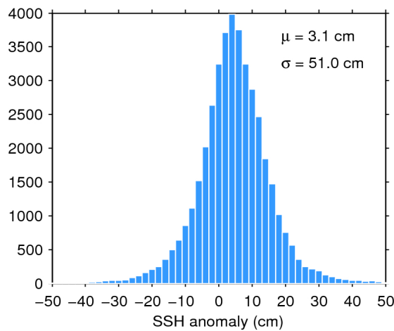
Figure 7. Histogram of flag-valid SSH anomaly over oceans and lakes for 23/07/2018. The mean ( \mu ) and standard deviation ( \sigma ) are also shown. Note that values outside [-50 50] cm are excluded from the histogram for the sake of readability but not from the computation of \mu and \sigma .
