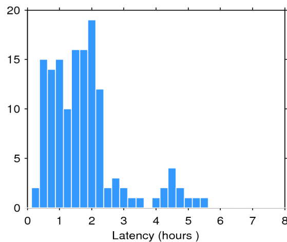
Figure 2. Histogram of the data latency for 23/07/2018. The y-axis denotes the number of files that are made available with a delay of x-hours with respect to the mean time of the records stored in the file.
