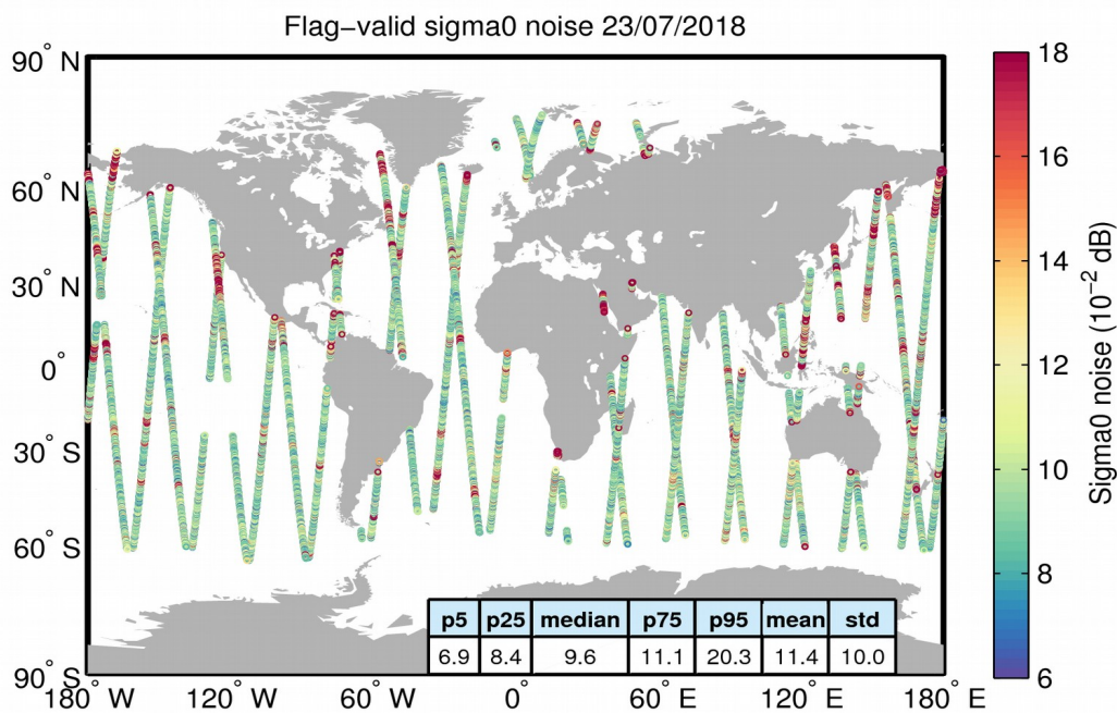
Figure 26. Geographical distribution of flag-valid 20-Hz sigma0 measurement noise over oceans and lakes for 23/07/2018. The statistical values shown in the table refer to the sigma0 noise and are calculated over all measurements shown in the figure.
