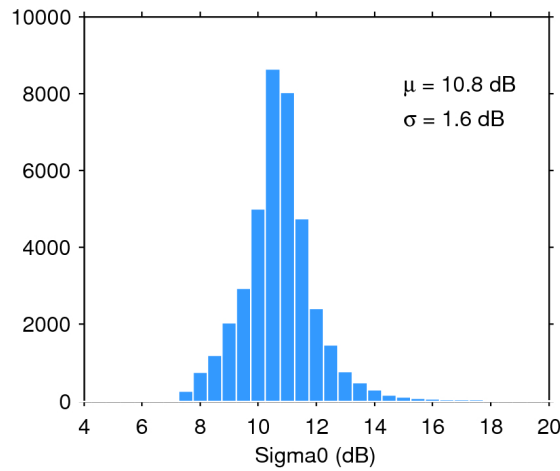
Figure 28. Histogram of science-valid sigma0 over oceans and lakes for 23/07/2018. The mean ( \mu ) and standard deviation ( \sigma ) are also shown. Note that values outside [4 20] dB are excluded from the histogram for the sake of readability but not from the computation of \mu and \sigma .
