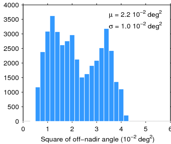
Figure 39. Histogram of flag-valid mispointing over oceans and lakes for 23/07/2018. The mean ( \mu ) and standard deviation ( \sigma ) are also shown. Note that values larger than 6 \cdot 10^{-2} \text{ deg}^2 are excluded from the histogram for the sake of readability but not from the computation of \mu and \sigma .
