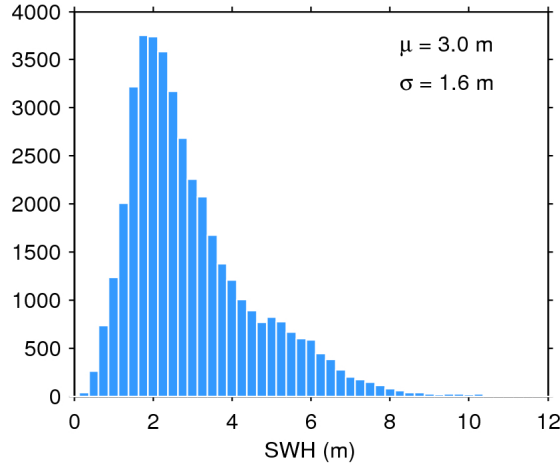
Figure 17. Histogram of flag-valid SWH over oceans and lakes for 23/07/2018. The mean ( \mu ) and standard deviation ( \sigma ) are also shown. Note that values larger than 12 m are excluded from the histogram for the sake of readability but not from the computation of \mu and \sigma .
