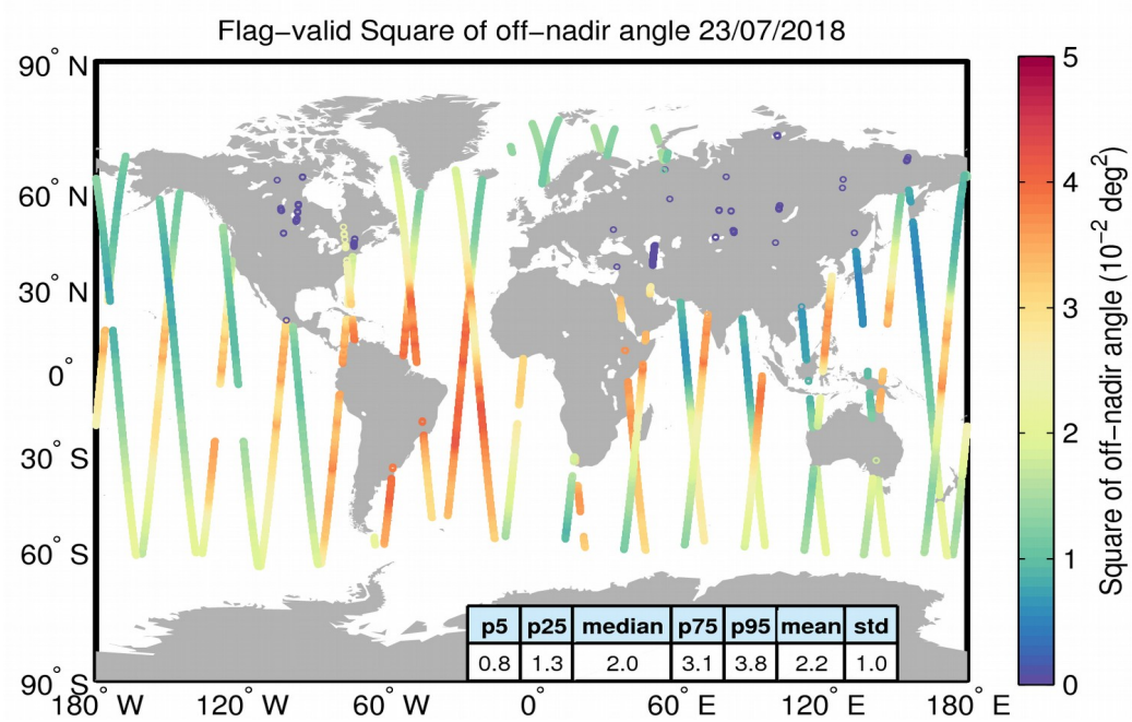
Figure 37. Geographical distribution of flag-valid mispointing data over oceans and lakes for 23/07/2018. The statistical values shown in the table refer to the mispointing in 10^{-2} \text{ deg}^2 and are calculated over all measurements shown in the figure.
