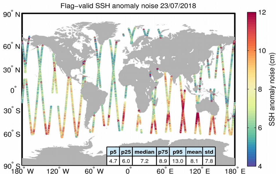
Figure 8. Geographical distribution of flag-valid 20-Hz SSH anomaly measurement noise over oceans and lakes for 23/07/2018. The statistical values shown in the table refer to the SSH anomaly noise and are calculated over all measurements shown in the figure.
