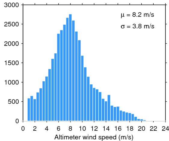
Figure 33. Histogram of flag-valid wind over oceans and lakes for 23/07/2018. The mean ( \mu ) and standard deviation ( \sigma ) are also shown. Note that values larger than 24 m/s are excluded from the histogram for the sake of readability but not from the computation of \mu and \sigma .
