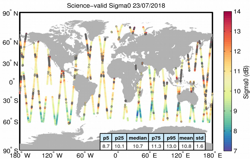
Figure 27. Geographical distribution of science-valid sigma0 data over oceans and lakes for 23/07/2018. The statistical values shown in the table refer to the sigma0 in dB and are calculated over all measurements shown in the figure. Gray circles denote records that have been rejected based on the editing criteria described in Table 4.
