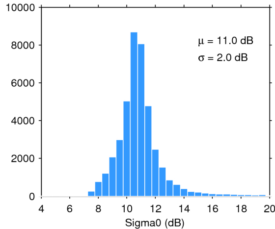
Figure 25. Histogram of flag-valid sigma0 over oceans and lakes for 23/07/2018. The mean ( \mu ) and standard deviation ( \sigma ) are also shown. Note that values outside [4 20] dB are excluded from the histogram for the sake of readability but not from the computation of \mu and \sigma .
