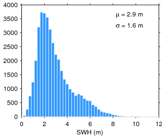
Figure 20. Histogram of science-valid SWH over oceans and lakes for 23/07/2018. The mean ( \mu ) and standard deviation ( \sigma ) are also shown. Note that values larger than 12 m are excluded from the histogram for the sake of readability but not from the computation of \mu and \sigma .
