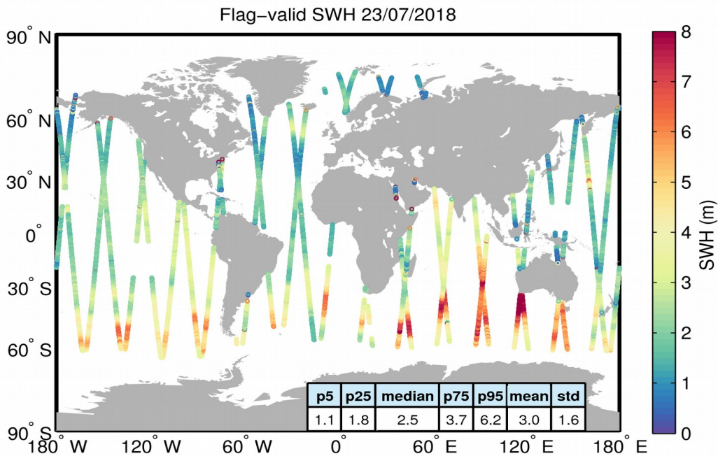
Figure 15. Geographical distribution of flag-valid SWH data over oceans and lakes for 23/07/2018. The statistical values shown in the table refer to the SWH in m and are calculated over all measurements shown in the figure.
