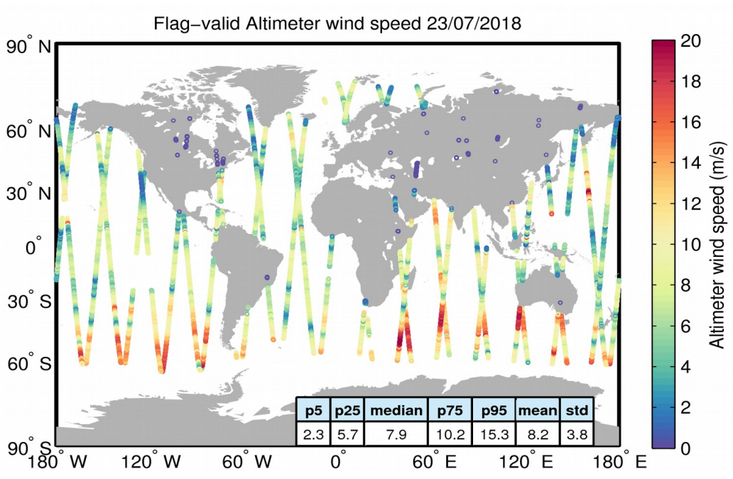
Figure 31. Geographical distribution of flag-valid wind data over oceans and lakes for 23/07/2018. The statistical values shown in the table refer to the wind in m/s and are calculated over all measurements shown in the figure.
