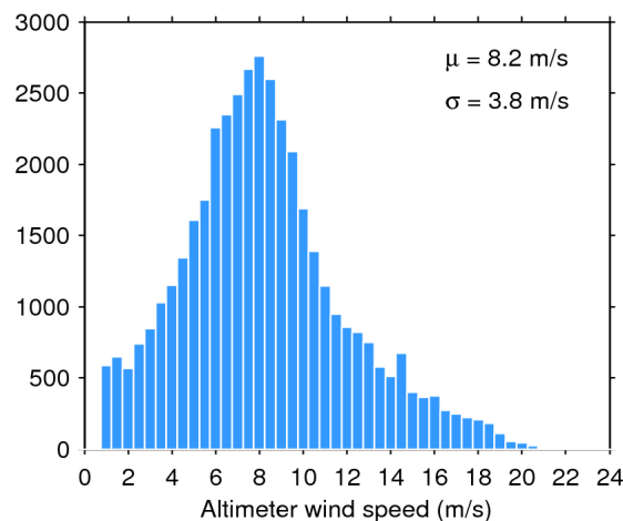
Figure 35. Histogram of science-valid wind over oceans and lakes for 23/07/2018. The mean ( \mu ) and standard deviation ( \sigma ) are also shown. Note that values larger than 24 m/s are excluded from the histogram for the sake of readability but not from the computation of \mu and \sigma .
