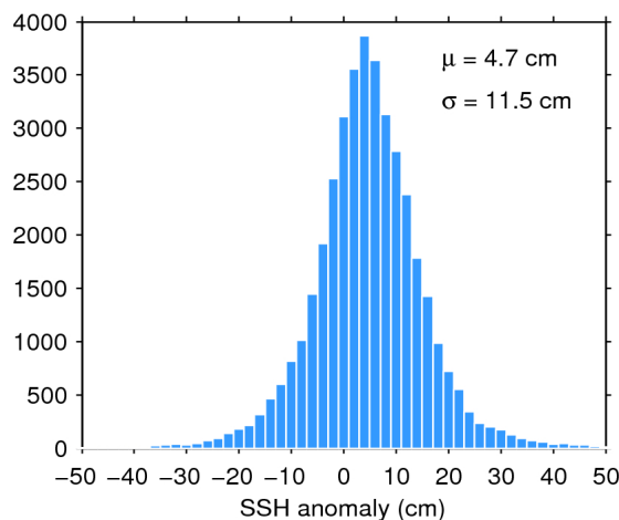
Figure 11. Histogram of science-valid SSH anomaly over oceans and lakes for 23/07/2018. The mean ( \mu ) and standard deviation ( \sigma ) are also shown. Note that values outside [-50 50] cm are excluded from the histogram for the sake of readability but not from the computation of \mu and \sigma .
