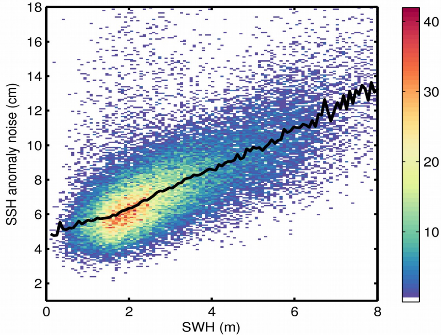
Figure 9. 2D histogram showing flag-valid SSH anomaly noise as a function of SWH for 23/07/2018. The black line denotes the median SSH anomaly noise as a function of SWH.
