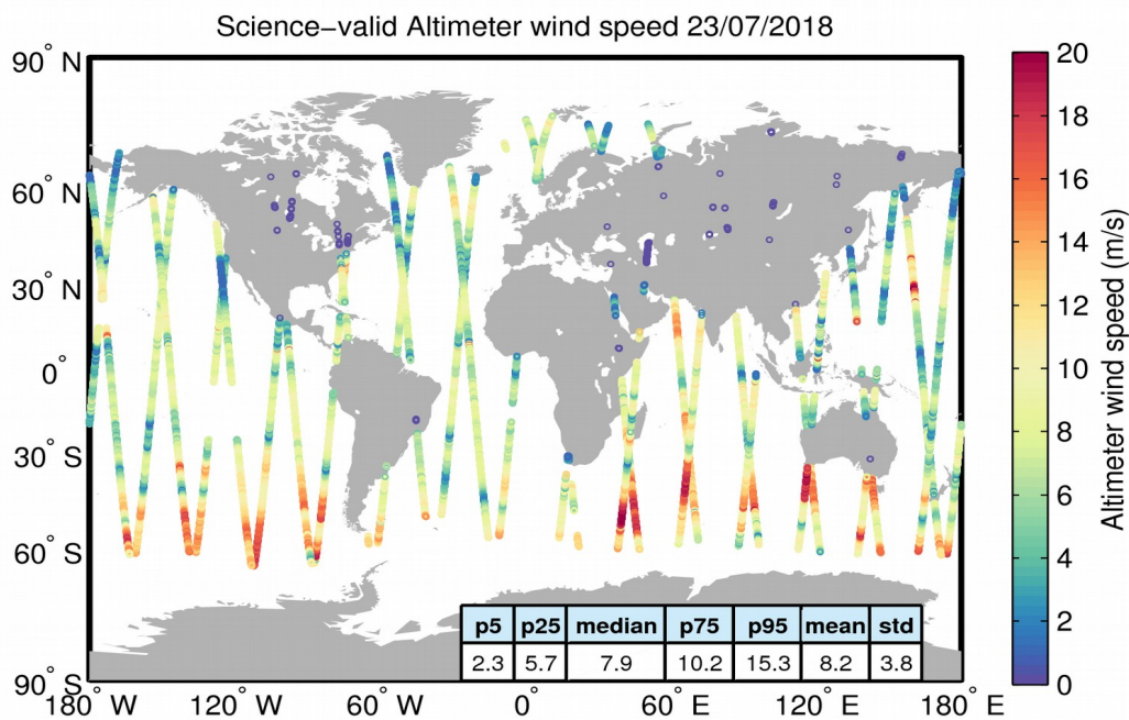
Figure 34. Geographical distribution of science-valid wind data over oceans and lakes for 23/07/2018. The statistical values shown in the table refer to the wind in m/s and are calculated over all measurements shown in the figure. Gray circles denote records that have been rejected based on the editing criteria described in Table 5.
