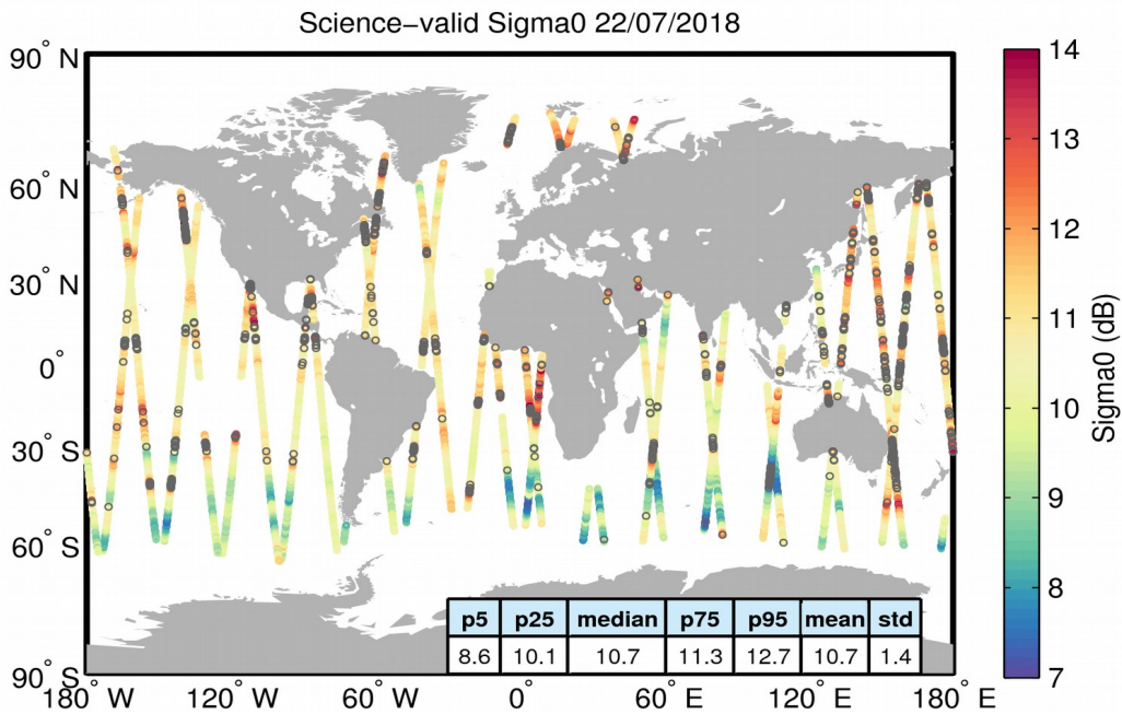
Figure 27. Geographical distribution of science-valid sigma0 data over oceans and lakes for 22/07/2018. The statistical values shown in the table refer to the sigma0 in dB and are calculated over all measurements shown in the figure. Gray circles denote records that have been rejected based on the editing criteria described in Table 4.
