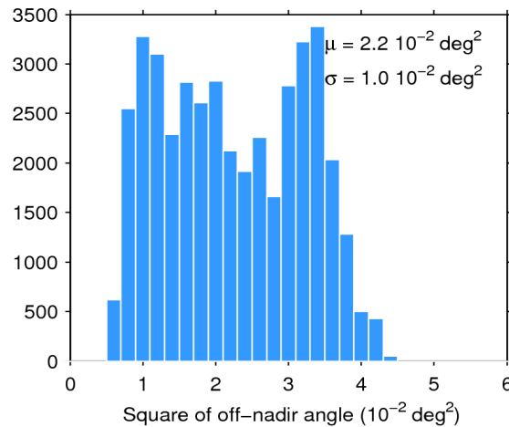
Figure 39. Histogram of flag-valid mispointing over oceans and lakes for 22/07/2018. The mean ( \mu ) and standard deviation ( \sigma ) are also shown. Note that values larger than 6 \cdot 10^{-2} \text{ deg}^2 are excluded from the histogram for the sake of readability but not from the computation of \mu and \sigma .
