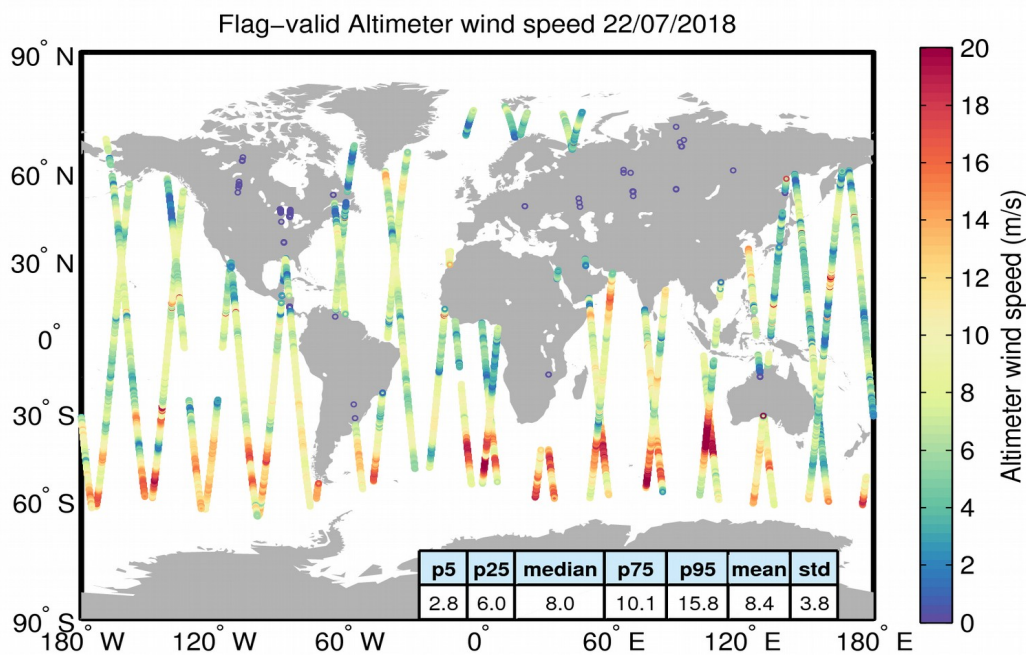
Figure 31. Geographical distribution of flag-valid wind data over oceans and lakes for 22/07/2018. The statistical values shown in the table refer to the wind in m/s and are calculated over all measurements shown in the figure.
