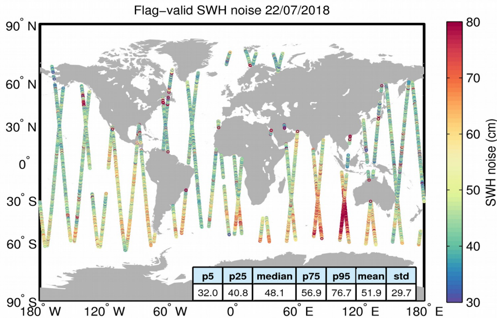
Figure 18. Geographical distribution of flag-valid 20-Hz SWH measurement noise over oceans and lakes for 22/07/2018. The statistical values shown in the figure refer to the SWH noise and are calculated over all measurements shown in the figure.
