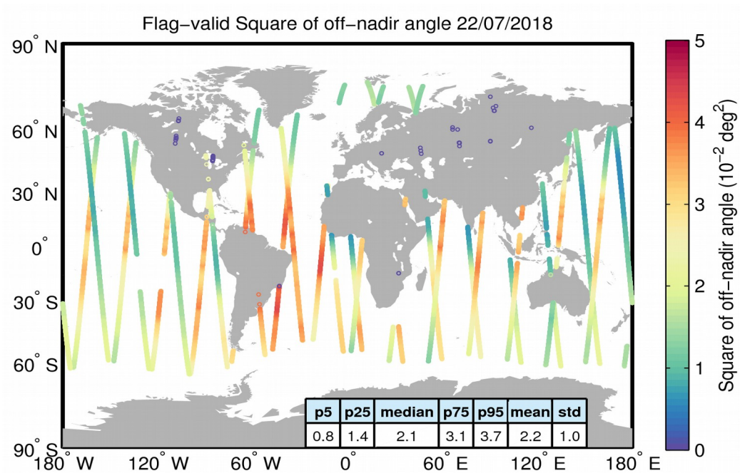
Figure 37. Geographical distribution of flag-valid mispointing data over oceans and lakes for 22/07/2018. The statistical values shown in the table refer to the mispointing in 10^{-2} deg 2 and are calculated over all measurements shown in the figure.
