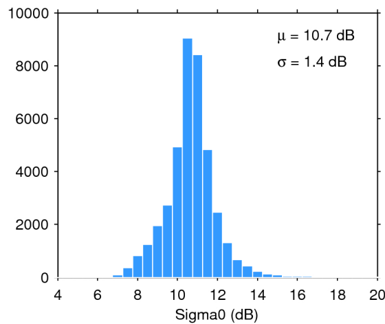
Figure 28. Histogram of science-valid sigma0 over oceans and lakes for 22/07/2018. The mean ( \mu ) and standard deviation ( \sigma ) are also shown. Note that values outside [4 20] dB are excluded from the histogram for the sake of readability but not from the computation of \mu and \sigma .
