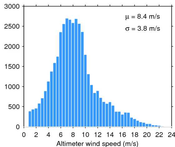
Figure 35. Histogram of science-valid wind over oceans and lakes for 22/07/2018. The mean ( \mu ) and standard deviation ( \sigma ) are also shown. Note that values larger than 24 m/s are excluded from the histogram for the sake of readability but not from the computation of \mu and \sigma .
