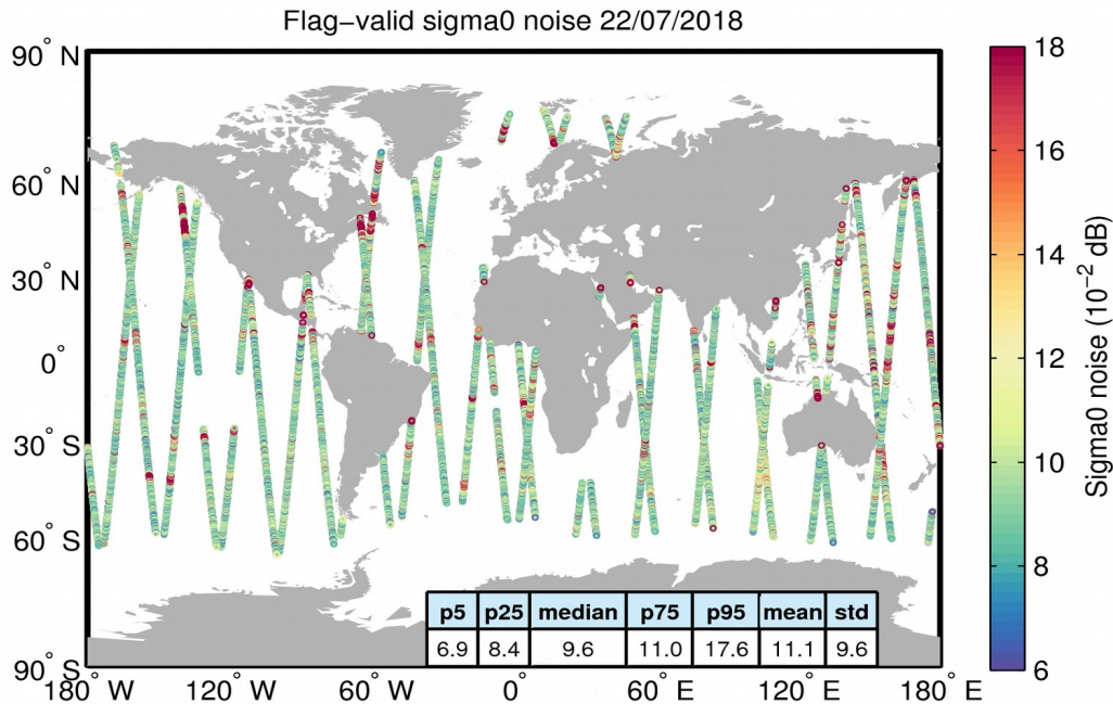
Figure 26. Geographical distribution of flag-valid 20-Hz sigma0 measurement noise over oceans and lakes for 22/07/2018. The statistical values shown in the table refer to the sigma0 noise and are calculated over all measurements shown in the figure.
