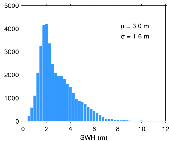
Figure 20. Histogram of science-valid SWH over oceans and lakes for 22/07/2018. The mean ( \mu ) and standard deviation ( \sigma ) are also shown. Note that values larger than 12 m are excluded from the histogram for the sake of readability but not from the computation of \mu and \sigma .
