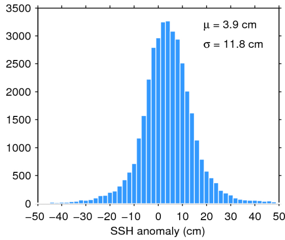
Figure 11. Histogram of science-valid SSH anomaly over oceans and lakes for 22/07/2018. The mean ( \mu ) and standard deviation ( \sigma ) are also shown. Note that values outside [-50 50] cm are excluded from the histogram for the sake of readability but not from the computation of \mu and \sigma .
