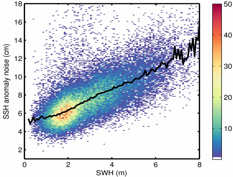
Figure 9. 2D histogram showing flag-valid SSH anomaly noise as a function of SWH for 22/07/2018. The black line denotes the median SSH anomaly noise as a function of SWH.
