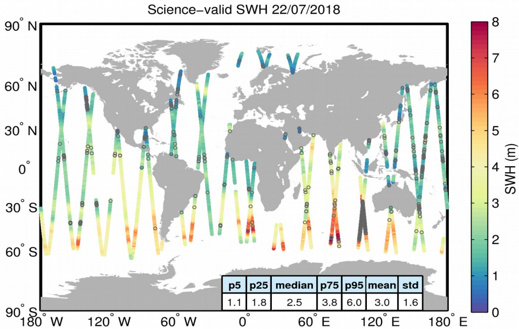
Figure 19. Geographical distribution of science-valid SWH data over oceans and lakes for 22/07/2018. The statistical values shown in the table refer to the SWH in m and are calculated over all measurements shown in the figure. Gray circles denote records that have been rejected based on the editing criteria described in Table 3.
