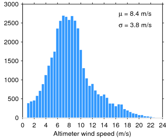
Figure 33. Histogram of flag-valid wind over oceans and lakes for 22/07/2018. The mean ( \mu ) and standard deviation ( \sigma ) are also shown. Note that values larger than 24 m/s are excluded from the histogram for the sake of readability but not from the computation of \mu and \sigma .
