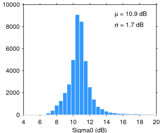
Figure 25. Histogram of flag-valid sigma0 over oceans and lakes for 22/07/2018. The mean ( \mu ) and standard deviation ( \sigma ) are also shown. Note that values outside [4 20] dB are excluded from the histogram for the sake of readability but not from the computation of \mu and \sigma .
