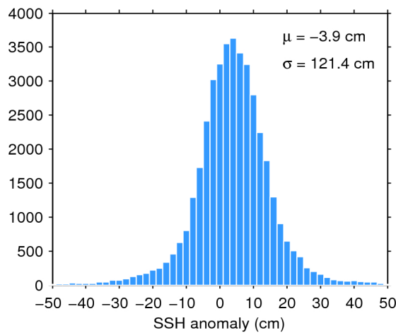
Figure 7. Histogram of flag-valid SSH anomaly over oceans and lakes for 22/07/2018. The mean ( \mu ) and standard deviation ( \sigma ) are also shown. Note that values outside [-50 50] cm are excluded from the histogram for the sake of readability but not from the computation of \mu and \sigma .
