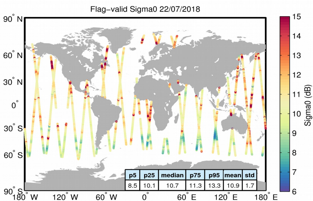
Figure 23. Geographical distribution of flag-valid sigma0 data over oceans and lakes for 22/07/2018. The statistical values shown in the table refer to the sigma0 in dB and are calculated over all measurements shown in the figure.
