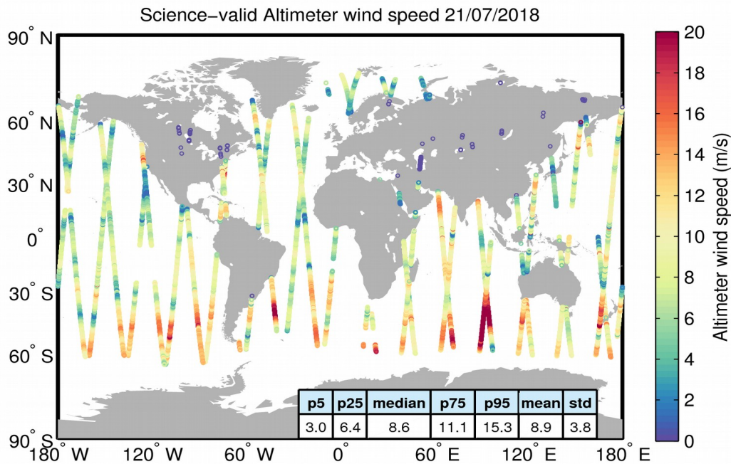
Figure 34. Geographical distribution of science-valid wind data over oceans and lakes for 21/07/2018. The statistical values shown in the table refer to the wind in m/s and are calculated over all measurements shown in the figure. Gray circles denote records that have been rejected based on the editing criteria described in Table 5.
