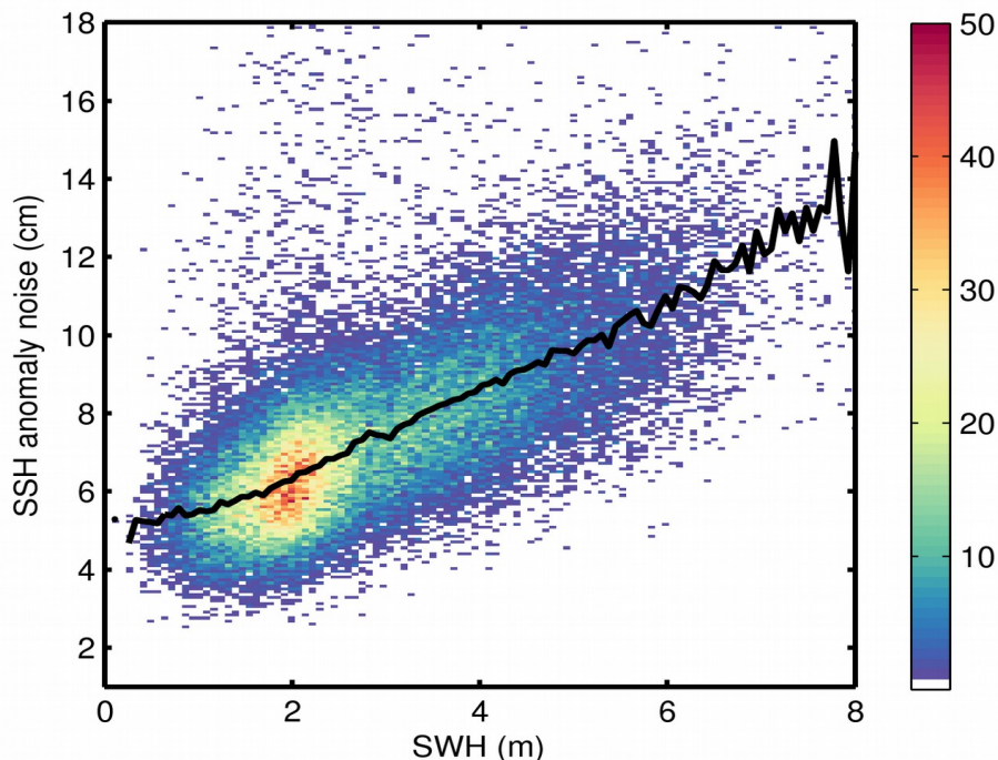
Figure 9. 2D histogram showing flag-valid SSH anomaly noise as a function of SWH for 21/07/2018. The black line denotes the median SSH anomaly noise as a function of SWH.
