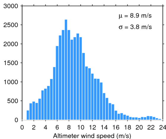
Figure 35. Histogram of science-valid wind over oceans and lakes for 21/07/2018. The mean ( \mu ) and standard deviation ( \sigma ) are also shown. Note that values larger than 24 m/s are excluded from the histogram for the sake of readability but not from the computation of \mu and \sigma .
