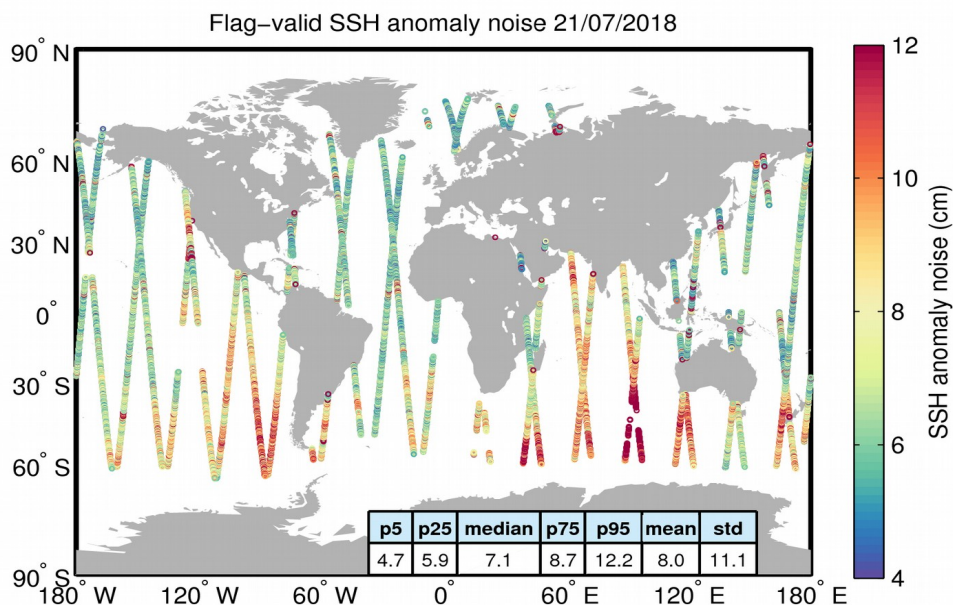
Figure 8. Geographical distribution of flag-valid 20-Hz SSH anomaly measurement noise over oceans and lakes for 21/07/2018. The statistical values shown in the table refer to the SSH anomaly noise and are calculated over all measurements shown in the figure.
