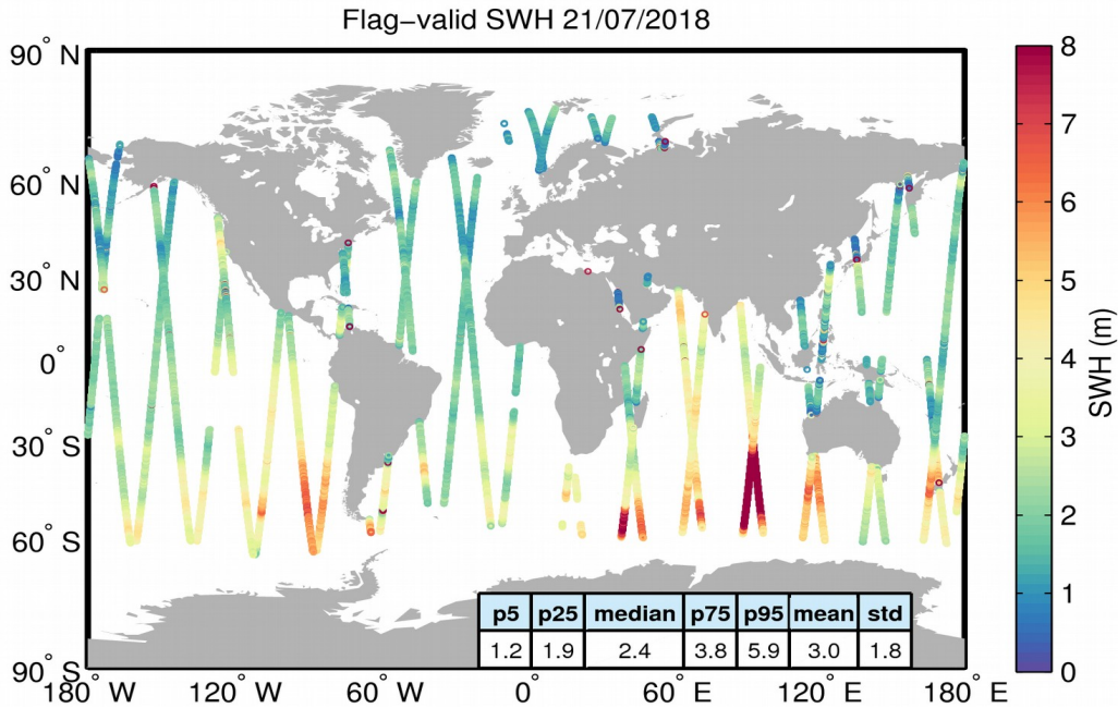
Figure 15. Geographical distribution of flag-valid SWH data over oceans and lakes for 21/07/2018. The statistical values shown in the table refer to the SWH in m and are calculated over all measurements shown in the figure.
