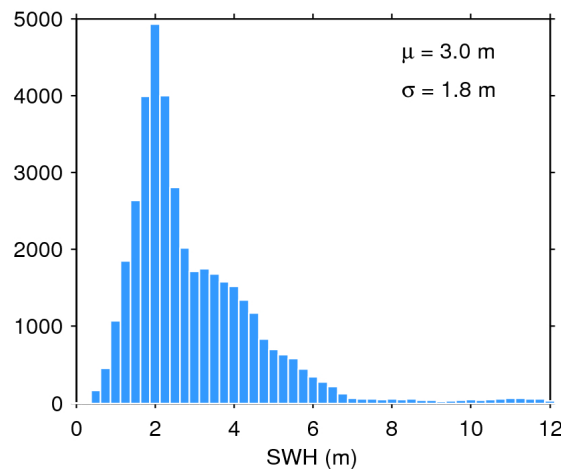
Figure 17. Histogram of flag-valid SWH over oceans and lakes for 21/07/2018. The mean ( \mu ) and standard deviation ( \sigma ) are also shown. Note that values larger than 12 m are excluded from the histogram for the sake of readability but not from the computation of \mu and \sigma .
