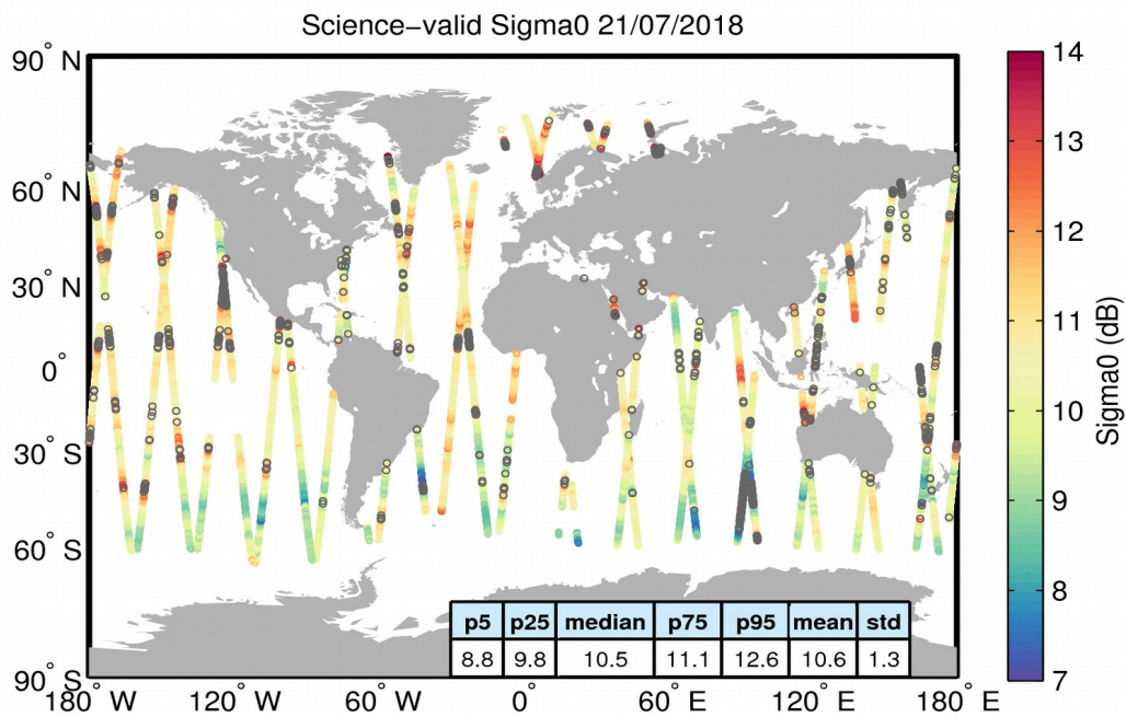
Figure 27. Geographical distribution of science-valid sigma0 data over oceans and lakes for 21/07/2018. The statistical values shown in the table refer to the sigma0 in dB and are calculated over all measurements shown in the figure. Gray circles denote records that have been rejected based on the editing criteria described in Table 4.
