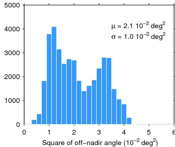
Figure 39. Histogram of flag-valid mispointing over oceans and lakes for 21/07/2018. The mean ( \mu ) and standard deviation ( \sigma ) are also shown. Note that values larger than 6 \cdot 10^{-2} \text{ deg}^2 are excluded from the histogram for the sake of readability but not from the computation of \mu and \sigma .
