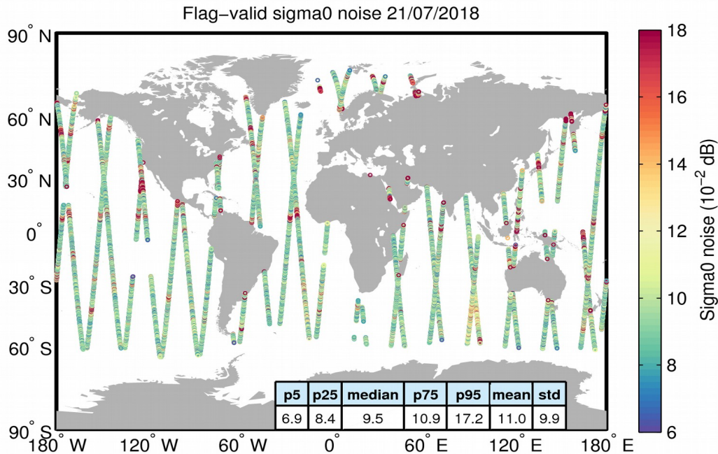
Figure 26. Geographical distribution of flag-valid 20-Hz sigma0 measurement noise over oceans and lakes for 21/07/2018. The statistical values shown in the table refer to the sigma0 noise and are calculated over all measurements shown in the figure.
