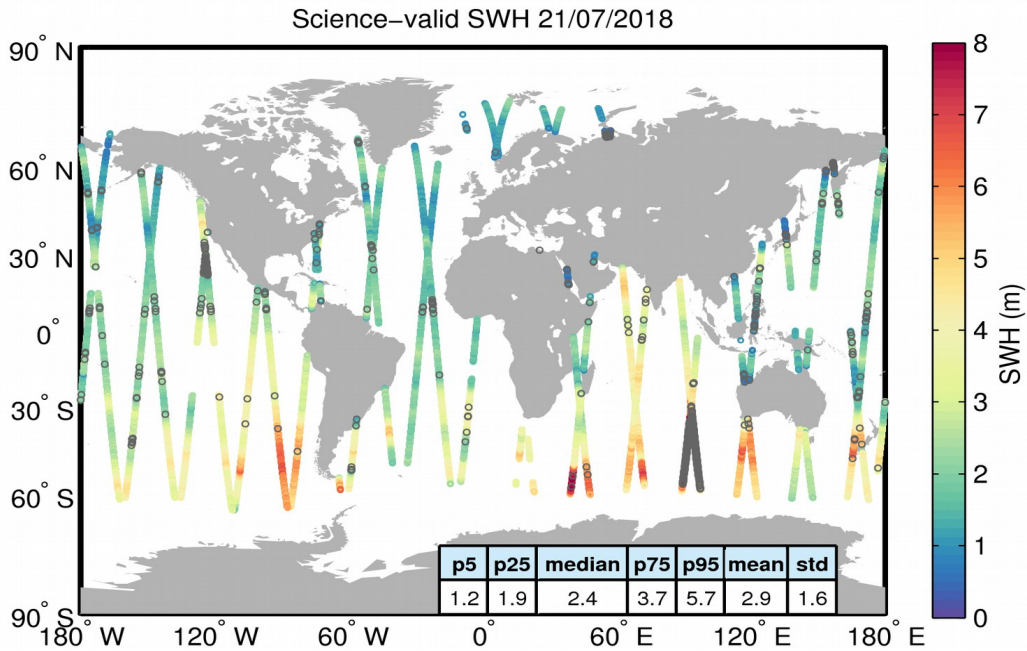
Figure 19. Geographical distribution of science-valid SWH data over oceans and lakes for 21/07/2018. The statistical values shown in the table refer to the SWH in m and are calculated over all measurements shown in the figure. Gray circles denote records that have been rejected based on the editing criteria described in Table 3.
