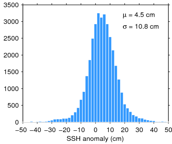
Figure 11. Histogram of science-valid SSH anomaly over oceans and lakes for 21/07/2018. The mean ( \mu ) and standard deviation ( \sigma ) are also shown. Note that values outside [-50 50] cm are excluded from the histogram for the sake of readability but not from the computation of \mu and \sigma .
