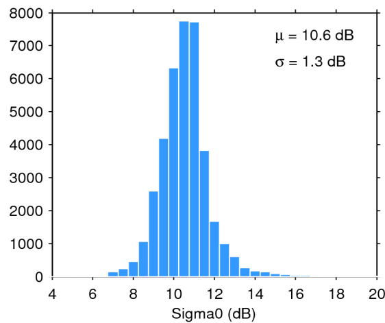
Figure 28. Histogram of science-valid sigma0 over oceans and lakes for 21/07/2018. The mean ( \mu ) and standard deviation ( \sigma ) are also shown. Note that values outside [4 20] dB are excluded from the histogram for the sake of readability but not from the computation of \mu and \sigma .
