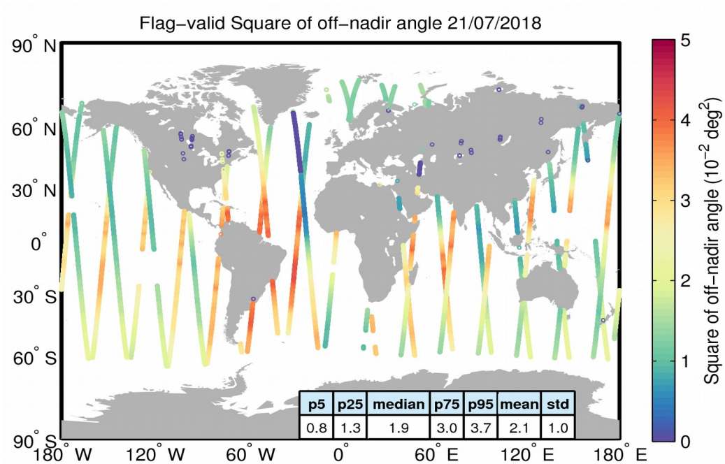
Figure 37. Geographical distribution of flag-valid mispointing data over oceans and lakes for 21/07/2018. The statistical values shown in the table refer to the mispointing in 10^{-2} deg 2 and are calculated over all measurements shown in the figure.
