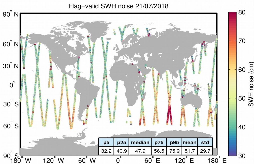
Figure 18. Geographical distribution of flag-valid 20-Hz SWH measurement noise over oceans and lakes for 21/07/2018. The statistical values shown in the figure refer to the SWH noise and are calculated over all measurements shown in the figure.
