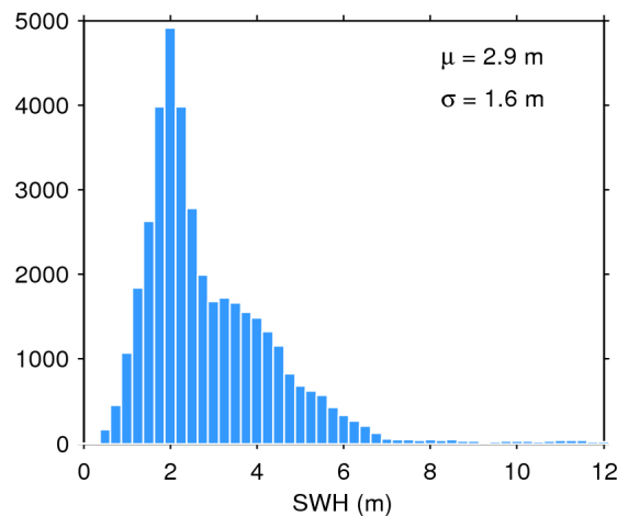
Figure 20. Histogram of science-valid SWH over oceans and lakes for 21/07/2018. The mean ( \mu ) and standard deviation ( \sigma ) are also shown. Note that values larger than 12 m are excluded from the histogram for the sake of readability but not from the computation of \mu and \sigma .
