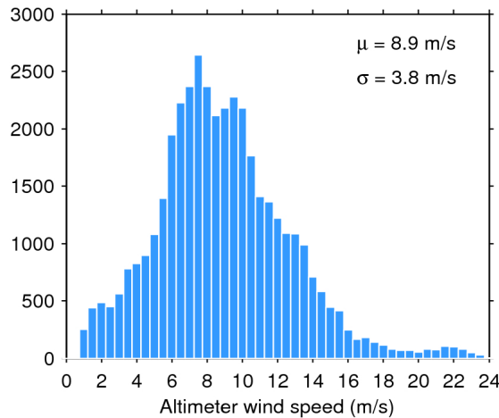
Figure 33. Histogram of flag-valid wind over oceans and lakes for 21/07/2018. The mean ( \mu ) and standard deviation ( \sigma ) are also shown. Note that values larger than 24 m/s are excluded from the histogram for the sake of readability but not from the computation of \mu and \sigma .
