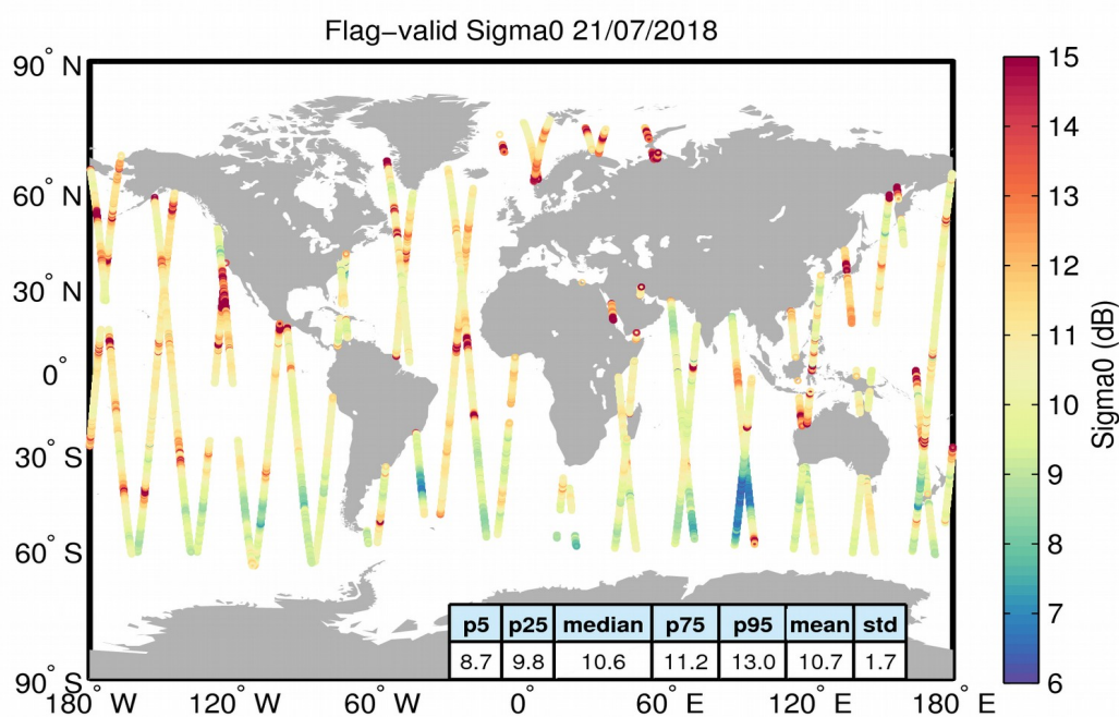
Figure 23. Geographical distribution of flag-valid sigma0 data over oceans and lakes for 21/07/2018. The statistical values shown in the table refer to the sigma0 in dB and are calculated over all measurements shown in the figure.
