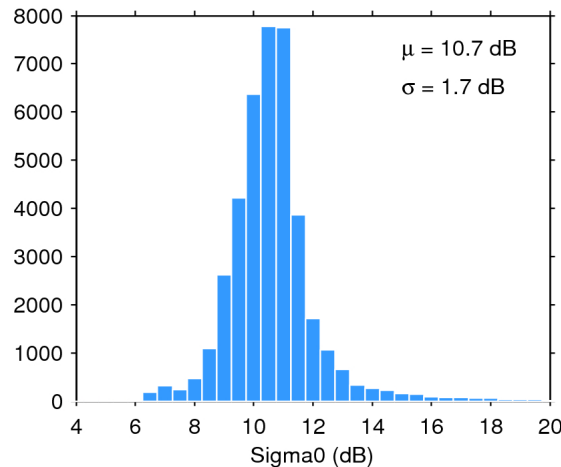
Figure 25. Histogram of flag-valid sigma0 over oceans and lakes for 21/07/2018. The mean ( \mu ) and standard deviation ( \sigma ) are also shown. Note that values outside [4 20] dB are excluded from the histogram for the sake of readability but not from the computation of \mu and \sigma .
