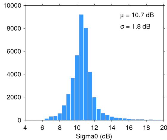
Figure 25. Histogram of flag-valid sigma0 over oceans and lakes for 20/07/2018. The mean ( \mu ) and standard deviation ( \sigma ) are also shown. Note that values outside [4 20] dB are excluded from the histogram for the sake of readability but not from the computation of \mu and \sigma .
