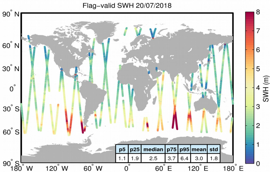
Figure 15. Geographical distribution of flag-valid SWH data over oceans and lakes for 20/07/2018. The statistical values shown in the table refer to the SWH in m and are calculated over all measurements shown in the figure.
