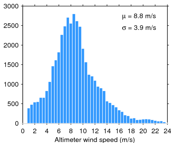
Figure 35. Histogram of science-valid wind over oceans and lakes for 20/07/2018. The mean ( \mu ) and standard deviation ( \sigma ) are also shown. Note that values larger than 24 m/s are excluded from the histogram for the sake of readability but not from the computation of \mu and \sigma .
