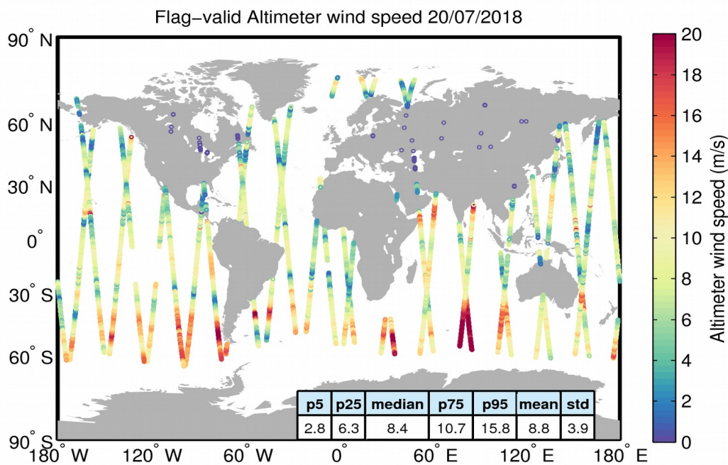
Figure 31. Geographical distribution of flag-valid wind data over oceans and lakes for 20/07/2018. The statistical values shown in the table refer to the wind in m/s and are calculated over all measurements shown in the figure.
