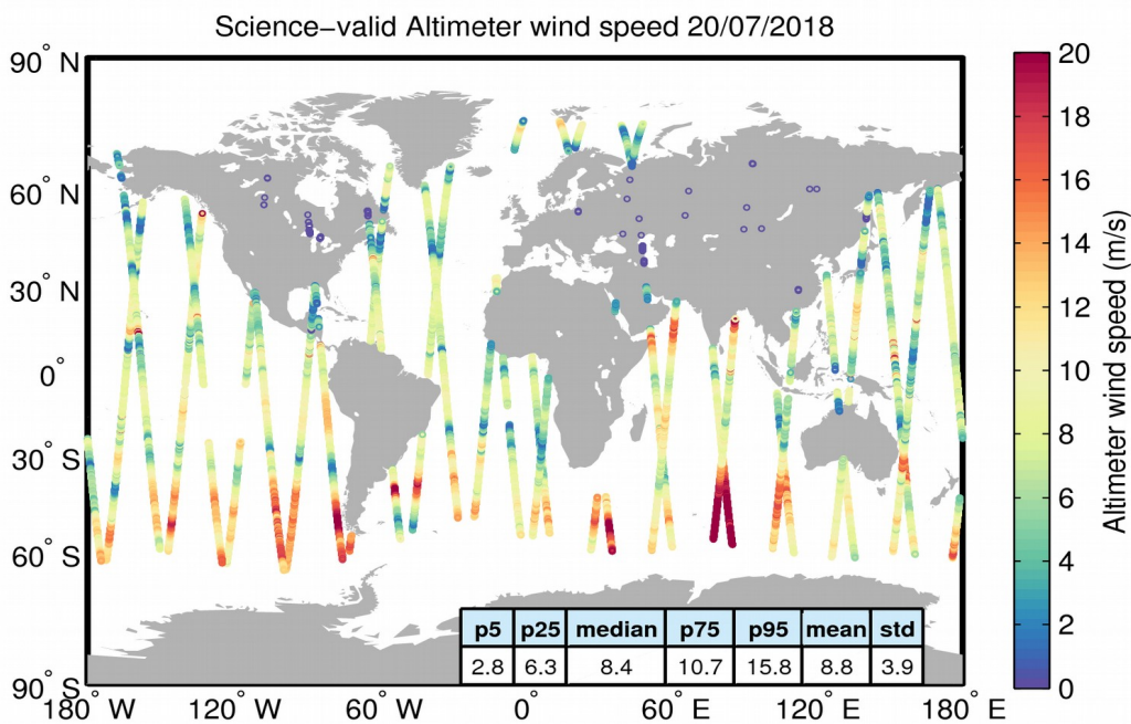
Figure 34. Geographical distribution of science-valid wind data over oceans and lakes for 20/07/2018. The statistical values shown in the table refer to the wind in m/s and are calculated over all measurements shown in the figure. Gray circles denote records that have been rejected based on the editing criteria described in Table 5.
