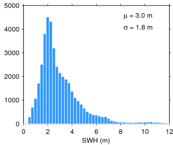
Figure 17. Histogram of flag-valid SWH over oceans and lakes for 20/07/2018. The mean ( \mu ) and standard deviation ( \sigma ) are also shown. Note that values larger than 12 m are excluded from the histogram for the sake of readability but not from the computation of \mu and \sigma .
