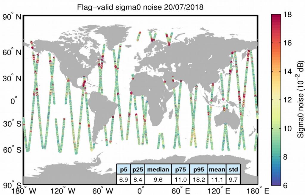
Figure 26. Geographical distribution of flag-valid 20-Hz sigma0 measurement noise over oceans and lakes for 20/07/2018. The statistical values shown in the table refer to the sigma0 noise and are calculated over all measurements shown in the figure.
