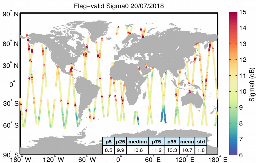
Figure 23. Geographical distribution of flag-valid sigma0 data over oceans and lakes for 20/07/2018. The statistical values shown in the table refer to the sigma0 in dB and are calculated over all measurements shown in the figure.
