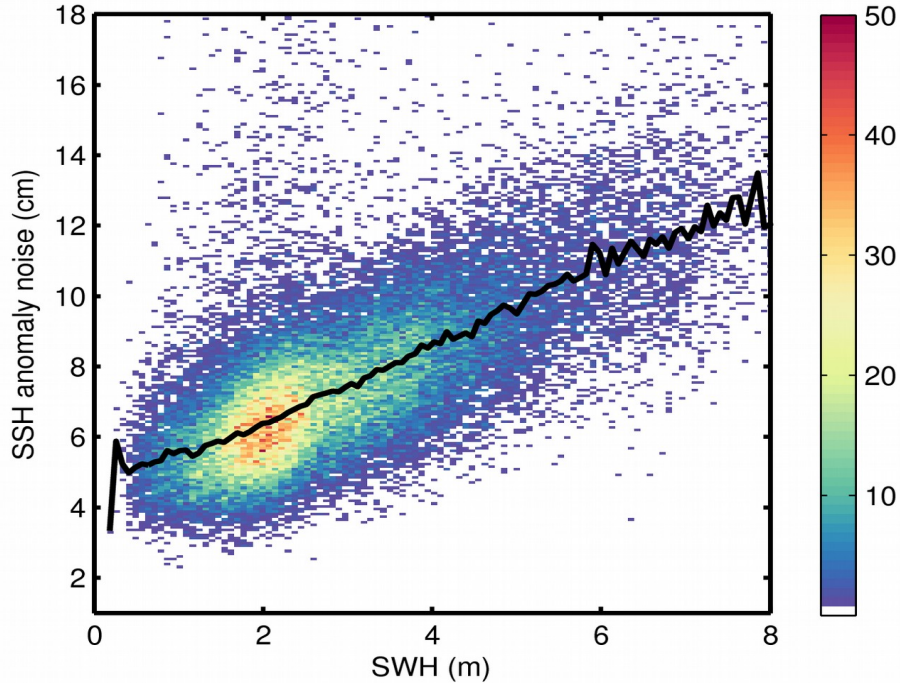
Figure 9. 2D histogram showing flag-valid SSH anomaly noise as a function of SWH for 20/07/2018. The black line denotes the median SSH anomaly noise as a function of SWH.
