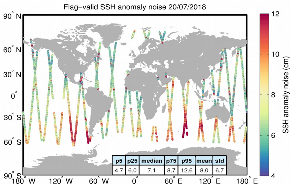
Figure 8. Geographical distribution of flag-valid 20-Hz SSH anomaly measurement noise over oceans and lakes for 20/07/2018. The statistical values shown in the table refer to the SSH anomaly noise and are calculated over all measurements shown in the figure.
