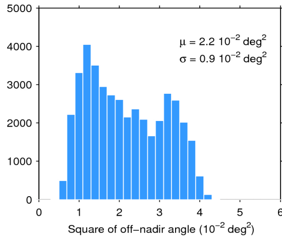
Figure 39. Histogram of flag-valid mispointing over oceans and lakes for 20/07/2018. The mean ( \mu ) and standard deviation ( \sigma ) are also shown. Note that values larger than 6 \cdot 10^{-2} \text{ deg}^2 are excluded from the histogram for the sake of readability but not from the computation of \mu and \sigma .
