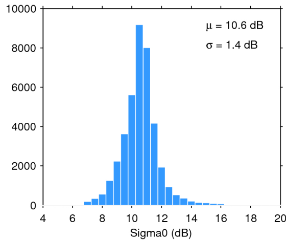
Figure 28. Histogram of science-valid sigma0 over oceans and lakes for 20/07/2018. The mean ( \mu ) and standard deviation ( \sigma ) are also shown. Note that values outside [4 20] dB are excluded from the histogram for the sake of readability but not from the computation of \mu and \sigma .
