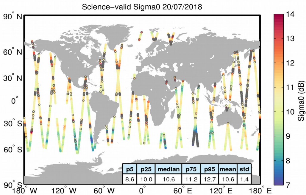
Figure 27. Geographical distribution of science-valid sigma0 data over oceans and lakes for 20/07/2018. The statistical values shown in the table refer to the sigma0 in dB and are calculated over all measurements shown in the figure. Gray circles denote records that have been rejected based on the editing criteria described in Table 4.
