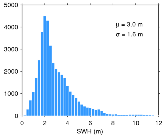
Figure 20. Histogram of science-valid SWH over oceans and lakes for 20/07/2018. The mean ( \mu ) and standard deviation ( \sigma ) are also shown. Note that values larger than 12 m are excluded from the histogram for the sake of readability but not from the computation of \mu and \sigma .
