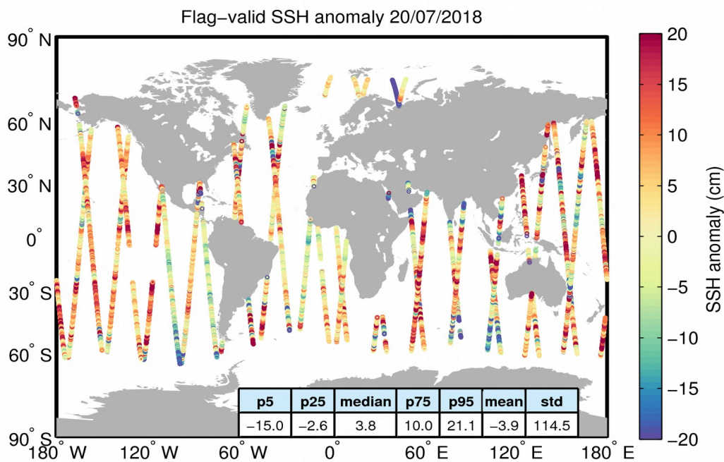
Figure 5. Geographical distribution of flag-valid 1-Hz SSH anomaly data over oceans and lakes for 20/07/2018. The statistical values shown in the table refer to the SSH anomaly in cm and are calculated over all measurements shown in the figure.
