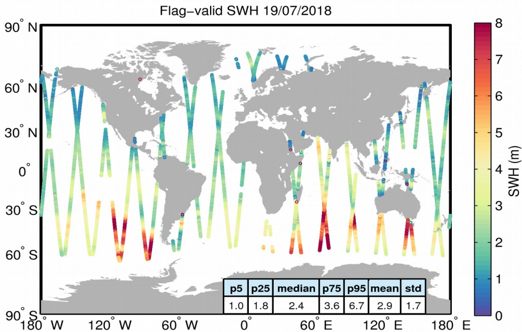
Figure 15. Geographical distribution of flag-valid SWH data over oceans and lakes for 19/07/2018. The statistical values shown in the table refer to the SWH in m and are calculated over all measurements shown in the figure.
