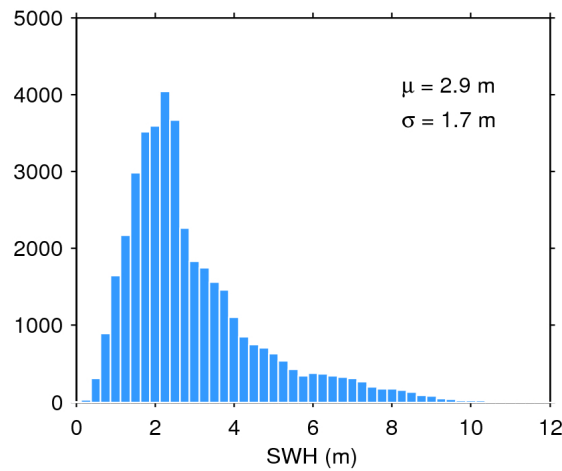
Figure 17. Histogram of flag-valid SWH over oceans and lakes for 19/07/2018. The mean ( \mu ) and standard deviation ( \sigma ) are also shown. Note that values larger than 12 m are excluded from the histogram for the sake of readability but not from the computation of \mu and \sigma .
