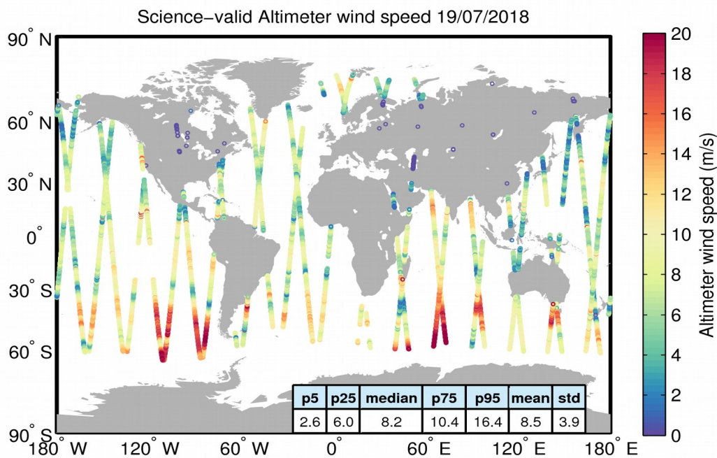
Figure 34. Geographical distribution of science-valid wind data over oceans and lakes for 19/07/2018. The statistical values shown in the table refer to the wind in m/s and are calculated over all measurements shown in the figure. Gray circles denote records that have been rejected based on the editing criteria described in Table 5.
