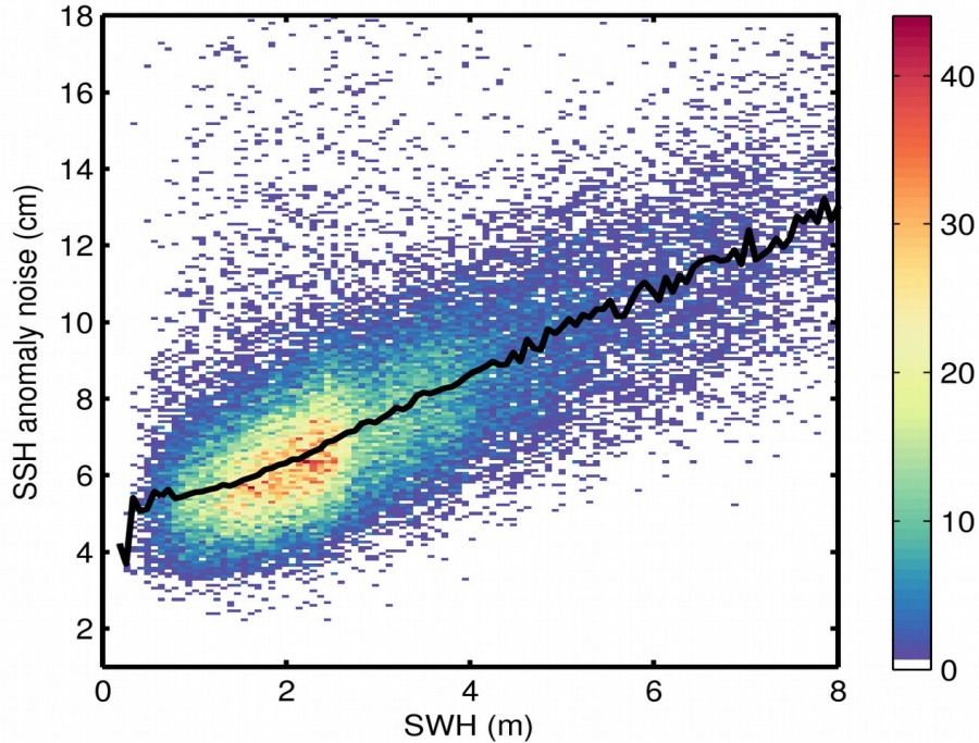
Figure 9. 2D histogram showing flag-valid SSH anomaly noise as a function of SWH for 19/07/2018. The black line denotes the median SSH anomaly noise as a function of SWH.
