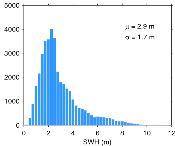
Figure 20. Histogram of science-valid SWH over oceans and lakes for 19/07/2018. The mean ( \mu ) and standard deviation ( \sigma ) are also shown. Note that values larger than 12 m are excluded from the histogram for the sake of readability but not from the computation of \mu and \sigma .
