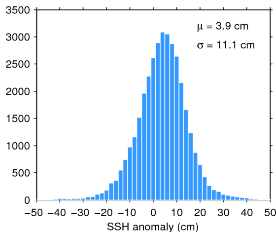
Figure 11. Histogram of science-valid SSH anomaly over oceans and lakes for 19/07/2018. The mean ( \mu ) and standard deviation ( \sigma ) are also shown. Note that values outside [-50 50] cm are excluded from the histogram for the sake of readability but not from the computation of \mu and \sigma .
