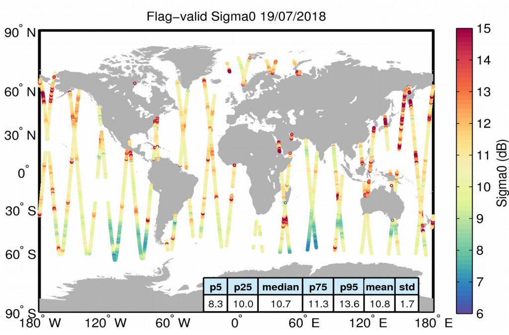
Figure 23. Geographical distribution of flag-valid sigma0 data over oceans and lakes for 19/07/2018. The statistical values shown in the table refer to the sigma0 in dB and are calculated over all measurements shown in the figure.
