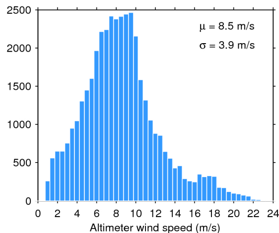
Figure 35. Histogram of science-valid wind over oceans and lakes for 19/07/2018. The mean ( \mu ) and standard deviation ( \sigma ) are also shown. Note that values larger than 24 m/s are excluded from the histogram for the sake of readability but not from the computation of \mu and \sigma .
