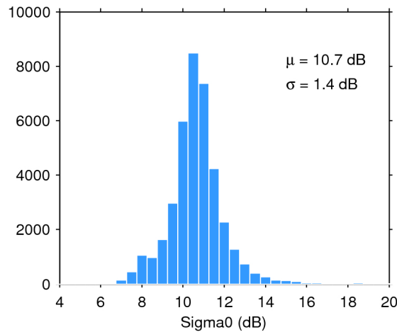
Figure 28. Histogram of science-valid sigma0 over oceans and lakes for 19/07/2018. The mean ( \mu ) and standard deviation ( \sigma ) are also shown. Note that values outside [4 20] dB are excluded from the histogram for the sake of readability but not from the computation of \mu and \sigma .
