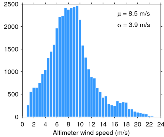
Figure 33. Histogram of flag-valid wind over oceans and lakes for 19/07/2018. The mean ( \mu ) and standard deviation ( \sigma ) are also shown. Note that values larger than 24 m/s are excluded from the histogram for the sake of readability but not from the computation of \mu and \sigma .
