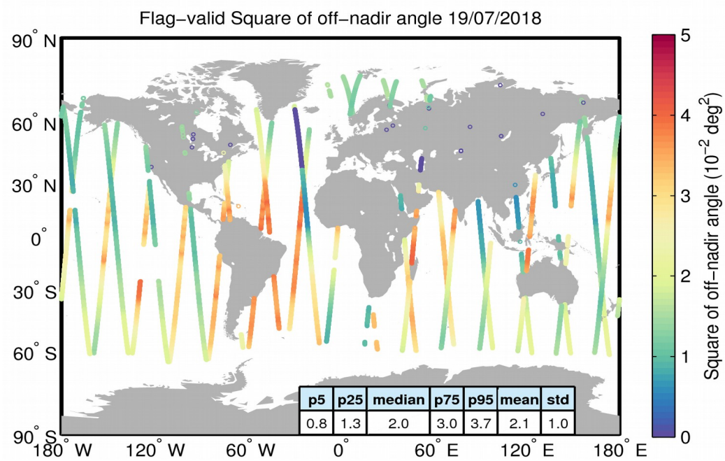
Figure 37. Geographical distribution of flag-valid mispointing data over oceans and lakes for 19/07/2018. The statistical values shown in the table refer to the mispointing in 10^{-2} deg 2 and are calculated over all measurements shown in the figure.
