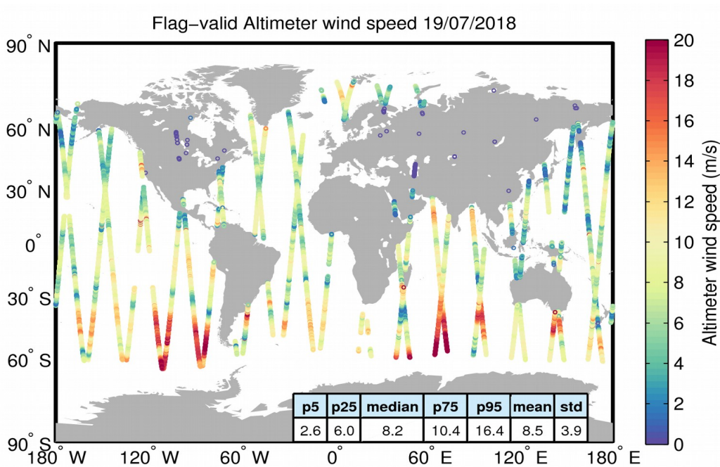
Figure 31. Geographical distribution of flag-valid wind data over oceans and lakes for 19/07/2018. The statistical values shown in the table refer to the wind in m/s and are calculated over all measurements shown in the figure.
