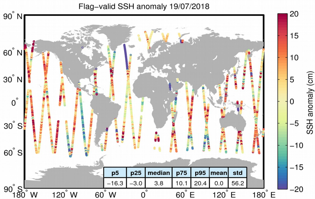
Figure 5. Geographical distribution of flag-valid 1-Hz SSH anomaly data over oceans and lakes for 19/07/2018. The statistical values shown in the table refer to the SSH anomaly in cm and are calculated over all measurements shown in the figure.
