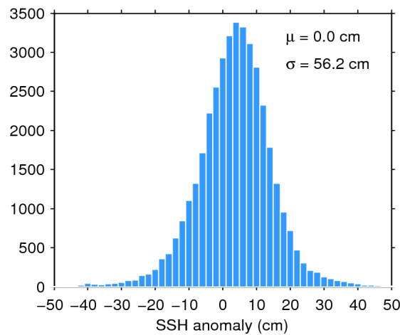
Figure 7. Histogram of flag-valid SSH anomaly over oceans and lakes for 19/07/2018. The mean ( \mu ) and standard deviation ( \sigma ) are also shown. Note that values outside [-50 50] cm are excluded from the histogram for the sake of readability but not from the computation of \mu and \sigma .
