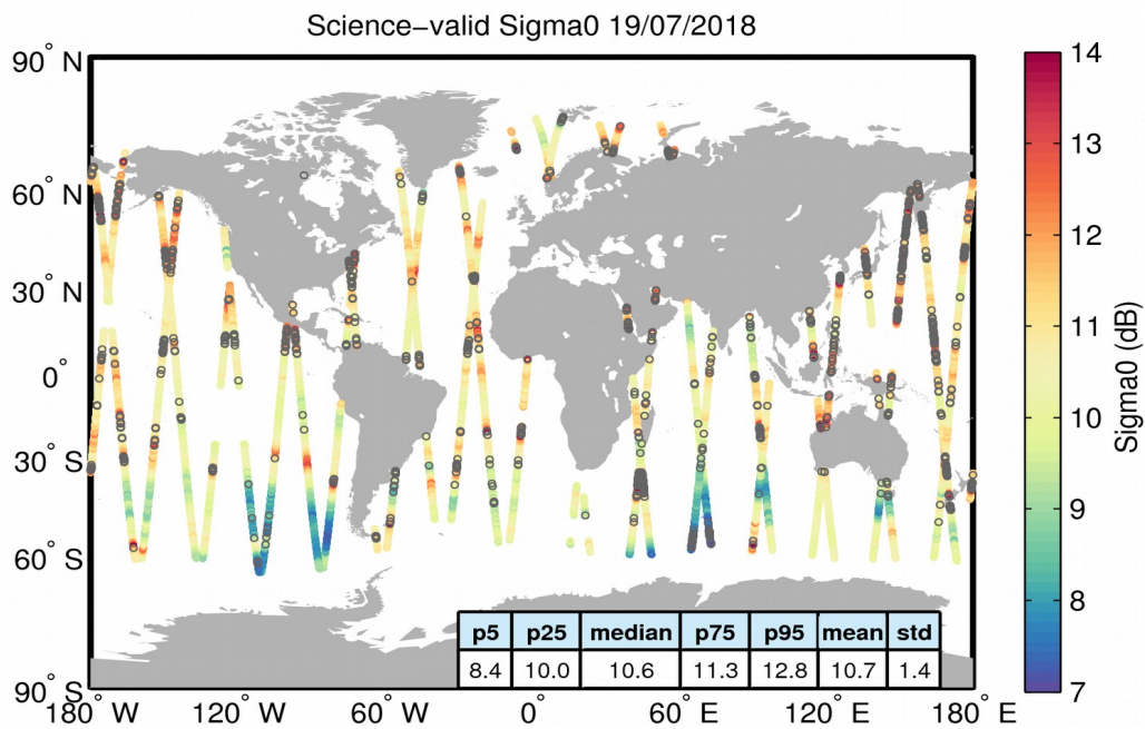
Figure 27. Geographical distribution of science-valid sigma0 data over oceans and lakes for 19/07/2018. The statistical values shown in the table refer to the sigma0 in dB and are calculated over all measurements shown in the figure. Gray circles denote records that have been rejected based on the editing criteria described in Table 4.
