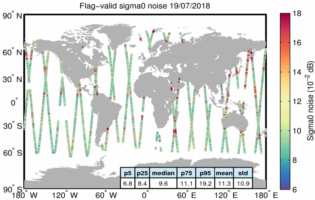
Figure 26. Geographical distribution of flag-valid 20-Hz sigma0 measurement noise over oceans and lakes for 19/07/2018. The statistical values shown in the table refer to the sigma0 noise and are calculated over all measurements shown in the figure.
