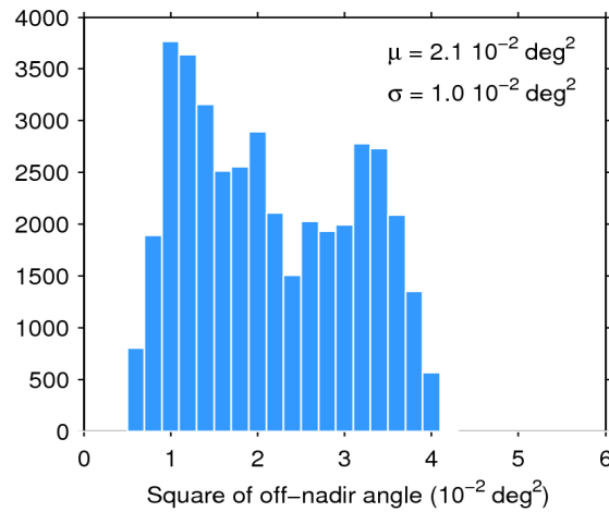
Figure 39. Histogram of flag-valid mispointing over oceans and lakes for 19/07/2018. The mean ( \mu ) and standard deviation ( \sigma ) are also shown. Note that values larger than 6 \cdot 10^{-2} \text{ deg}^2 are excluded from the histogram for the sake of readability but not from the computation of \mu and \sigma .
