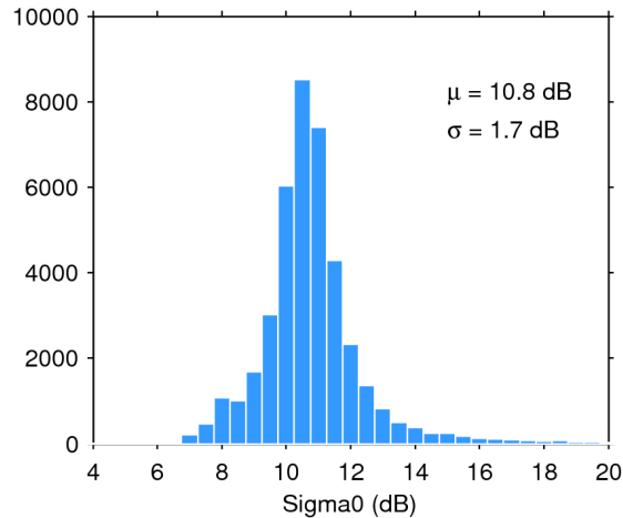
Figure 25. Histogram of flag-valid sigma0 over oceans and lakes for 19/07/2018. The mean ( \mu ) and standard deviation ( \sigma ) are also shown. Note that values outside [4 20] dB are excluded from the histogram for the sake of readability but not from the computation of \mu and \sigma .
