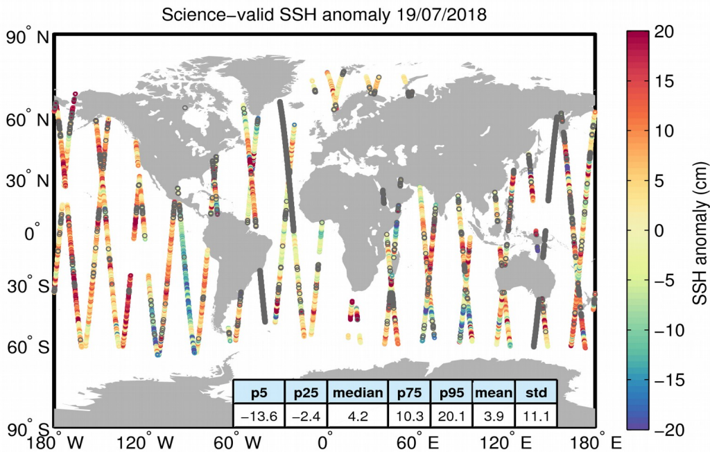
Figure 10. Geographical distribution of science-valid SSH anomaly data over oceans and lakes for 19/07/2018. The statistical values shown in the table refer to the SSH anomaly in cm and are calculated over all measurements shown in the figure. Gray circles denote records that have been rejected based on the editing criteria described in Table 2.
