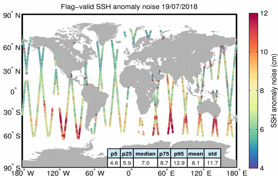
Figure 8. Geographical distribution of flag-valid 20-Hz SSH anomaly measurement noise over oceans and lakes for 19/07/2018. The statistical values shown in the table refer to the SSH anomaly noise and are calculated over all measurements shown in the figure.
