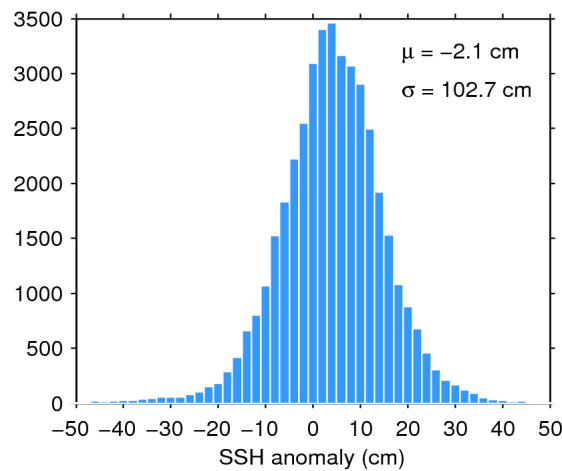
Figure 7. Histogram of flag-valid SSH anomaly over oceans and lakes for 18/07/2018. The mean ( \mu ) and standard deviation ( \sigma ) are also shown. Note that values outside [-50\ 50] cm are excluded from the histogram for the sake of readability but not from the computation of \mu and \sigma .
