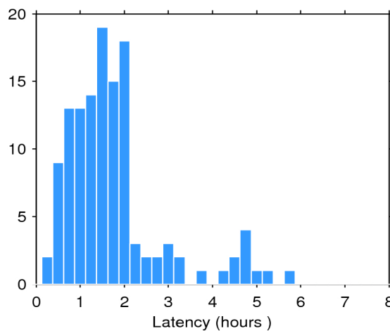
Figure 2. Histogram of the data latency for 18/07/2018. The y-axis denotes the number of files that are made available with a delay of x-hours with respect to the mean time of the records stored in the file.
