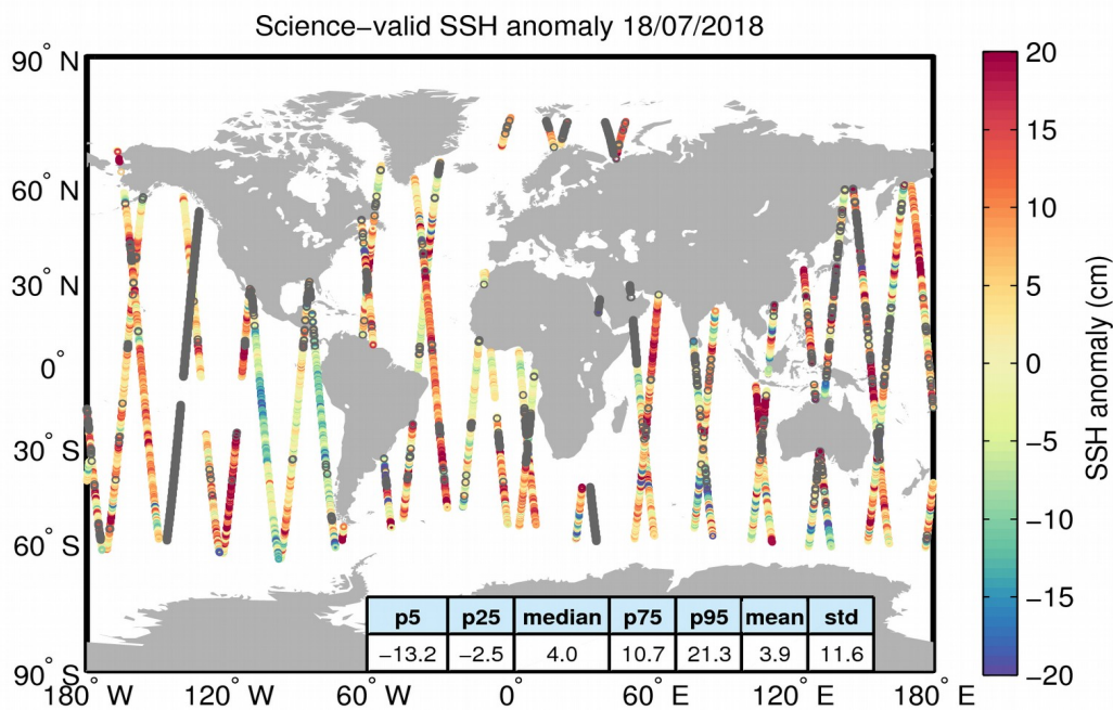
Figure 10. Geographical distribution of science-valid SSH anomaly data over oceans and lakes for 18/07/2018. The statistical values shown in the table refer to the SSH anomaly in cm and are calculated over all measurements shown in the figure. Gray circles denote records that have been rejected based on the editing criteria described in Table 2.
