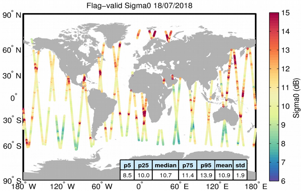
Figure 23. Geographical distribution of flag-valid sigma0 data over oceans and lakes for 18/07/2018. The statistical values shown in the table refer to the sigma0 in dB and are calculated over all measurements shown in the figure.
