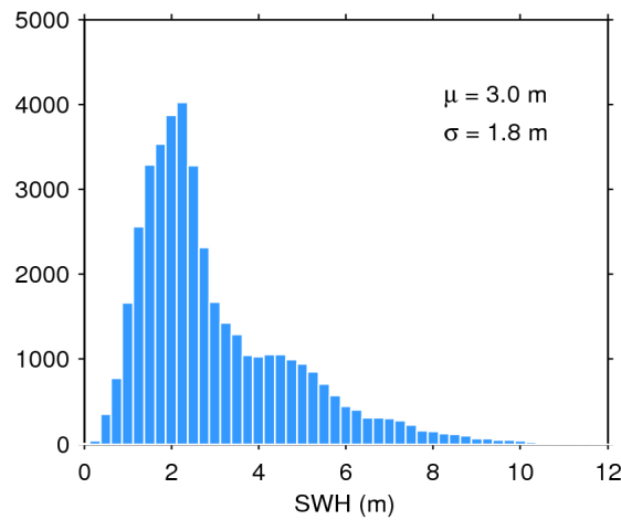
Figure 17. Histogram of flag-valid SWH over oceans and lakes for 18/07/2018. The mean ( \mu ) and standard deviation ( \sigma ) are also shown. Note that values larger than 12 m are excluded from the histogram for the sake of readability but not from the computation of \mu and \sigma .
