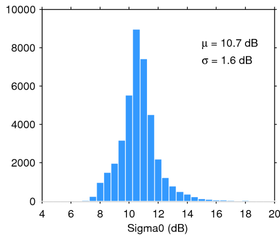
Figure 28. Histogram of science-valid sigma0 over oceans and lakes for 18/07/2018. The mean ( \mu ) and standard deviation ( \sigma ) are also shown. Note that values outside [4 20] dB are excluded from the histogram for the sake of readability but not from the computation of \mu and \sigma .
