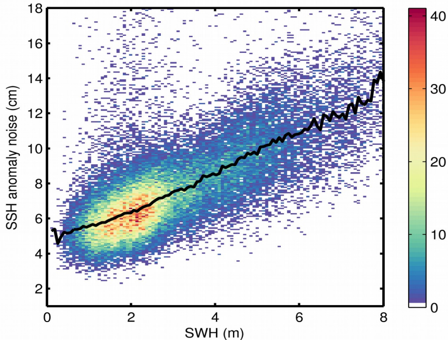
Figure 9. 2D histogram showing flag-valid SSH anomaly noise as a function of SWH for 18/07/2018. The black line denotes the median SSH anomaly noise as a function of SWH.
