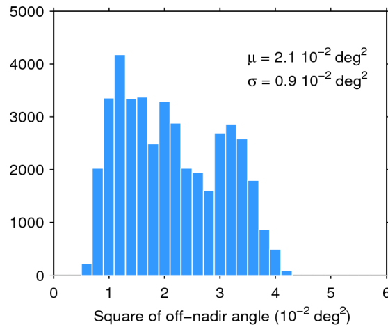
Figure 39. Histogram of flag-valid mispointing over oceans and lakes for 18/07/2018. The mean ( \mu ) and standard deviation ( \sigma ) are also shown. Note that values larger than 6 \cdot 10^{-2} \text{ deg}^2 are excluded from the histogram for the sake of readability but not from the computation of \mu and \sigma .
