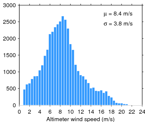
Figure 35. Histogram of science-valid wind over oceans and lakes for 18/07/2018. The mean ( \mu ) and standard deviation ( \sigma ) are also shown. Note that values larger than 24 m/s are excluded from the histogram for the sake of readability but not from the computation of \mu and \sigma .
