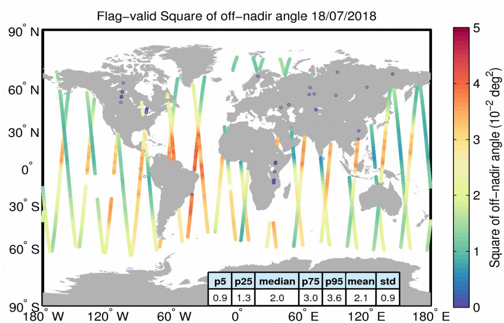
Figure 37. Geographical distribution of flag-valid mispointing data over oceans and lakes for 18/07/2018. The statistical values shown in the table refer to the mispointing in 10^{-2} deg 2 and are calculated over all measurements shown in the figure.
