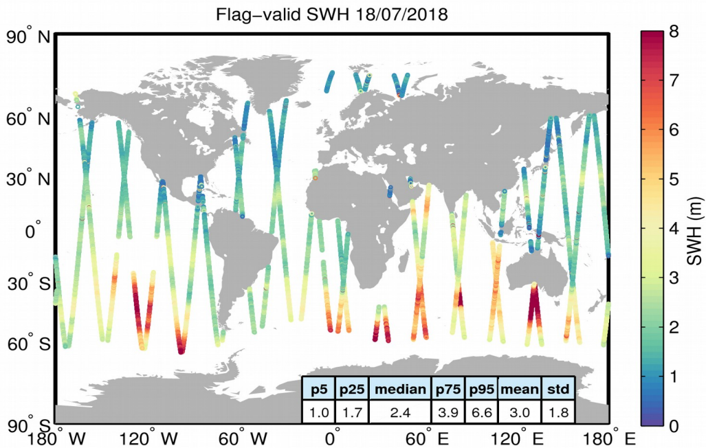
Figure 15. Geographical distribution of flag-valid SWH data over oceans and lakes for 18/07/2018. The statistical values shown in the table refer to the SWH in m and are calculated over all measurements shown in the figure.
