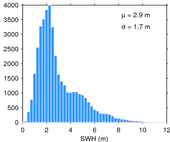
Figure 20. Histogram of science-valid SWH over oceans and lakes for 18/07/2018. The mean ( \mu ) and standard deviation ( \sigma ) are also shown. Note that values larger than 12 m are excluded from the histogram for the sake of readability but not from the computation of \mu and \sigma .
