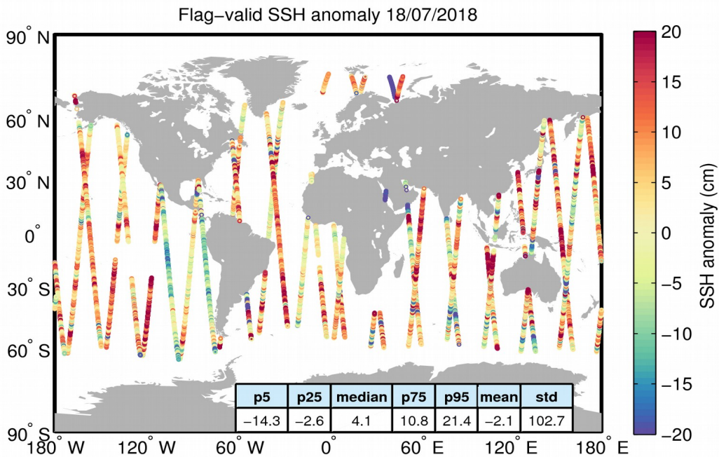
Figure 5. Geographical distribution of flag-valid 1-Hz SSH anomaly data over oceans and lakes for 18/07/2018. The statistical values shown in the table refer to the SSH anomaly in cm and are calculated over all measurements shown in the figure.
