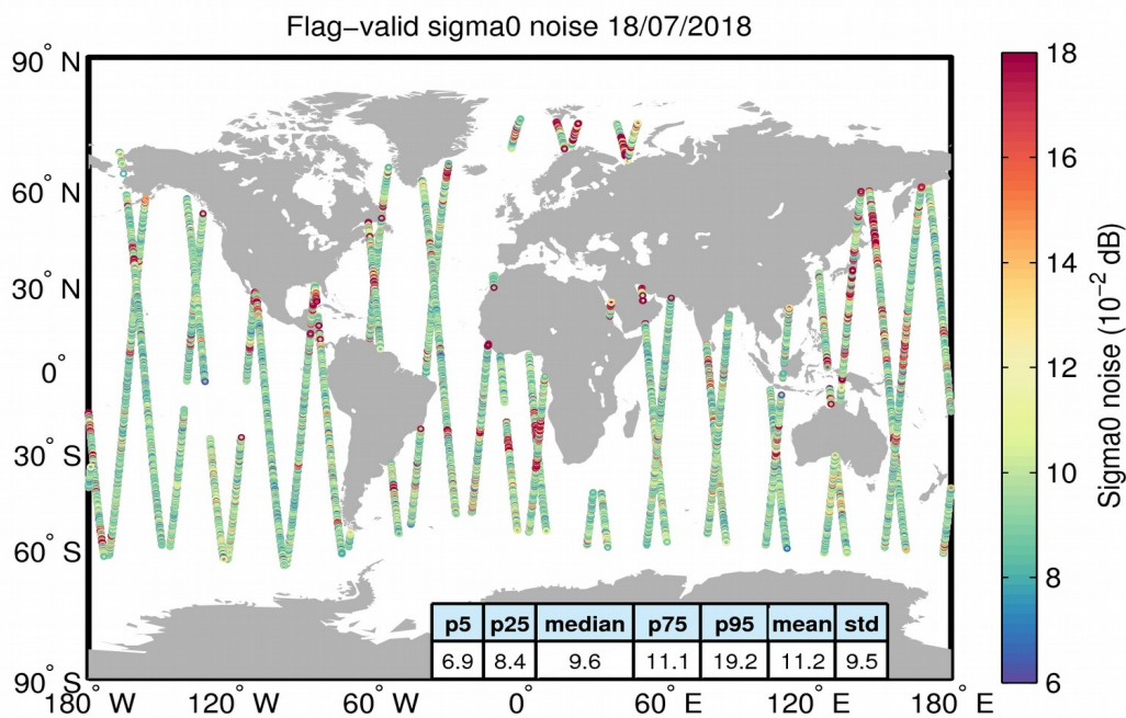
Figure 26. Geographical distribution of flag-valid 20-Hz sigma0 measurement noise over oceans and lakes for 18/07/2018. The statistical values shown in the table refer to the sigma0 noise and are calculated over all measurements shown in the figure.
