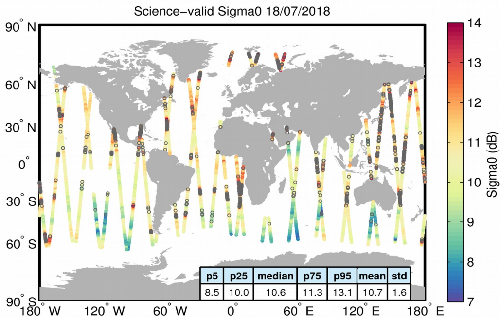
Figure 27. Geographical distribution of science-valid sigma0 data over oceans and lakes for 18/07/2018. The statistical values shown in the table refer to the sigma0 in dB and are calculated over all measurements shown in the figure. Gray circles denote records that have been rejected based on the editing criteria described in Table 4.
