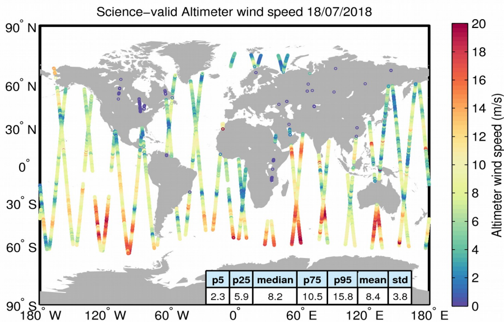
Figure 34. Geographical distribution of science-valid wind data over oceans and lakes for 18/07/2018. The statistical values shown in the table refer to the wind in m/s and are calculated over all measurements shown in the figure. Gray circles denote records that have been rejected based on the editing criteria described in Table 5.
