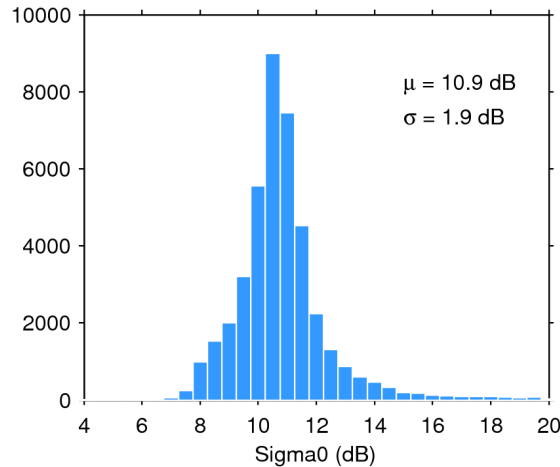
Figure 25. Histogram of flag-valid sigma0 over oceans and lakes for 18/07/2018. The mean ( \mu ) and standard deviation ( \sigma ) are also shown. Note that values outside [4 20] dB are excluded from the histogram for the sake of readability but not from the computation of \mu and \sigma .
