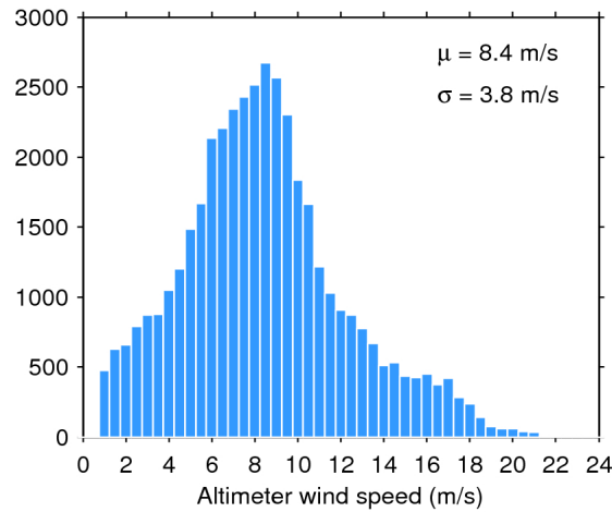
Figure 33. Histogram of flag-valid wind over oceans and lakes for 18/07/2018. The mean ( \mu ) and standard deviation ( \sigma ) are also shown. Note that values larger than 24 m/s are excluded from the histogram for the sake of readability but not from the computation of \mu and \sigma .
