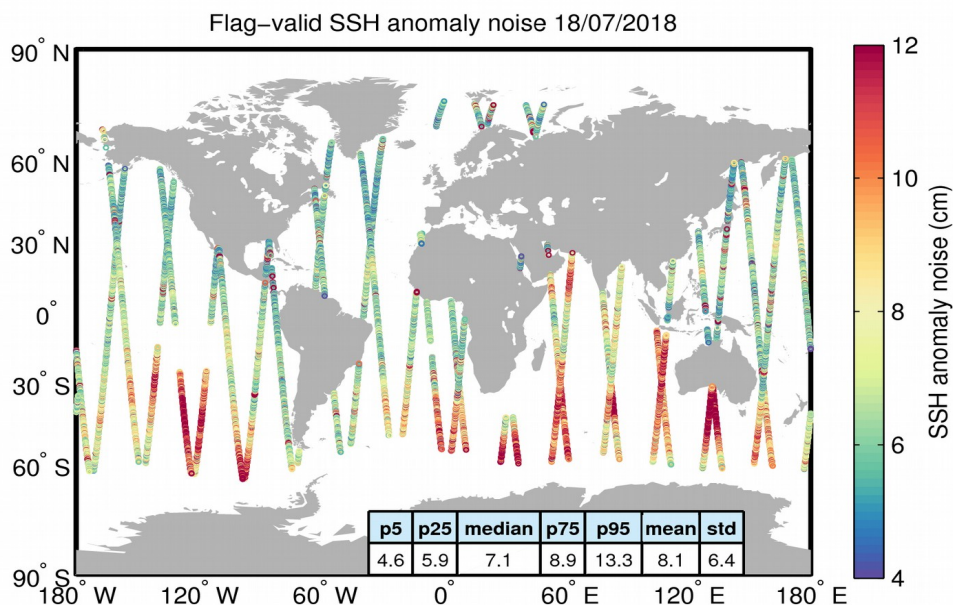
Figure 8. Geographical distribution of flag-valid 20-Hz SSH anomaly measurement noise over oceans and lakes for 18/07/2018. The statistical values shown in the table refer to the SSH anomaly noise and are calculated over all measurements shown in the figure.
