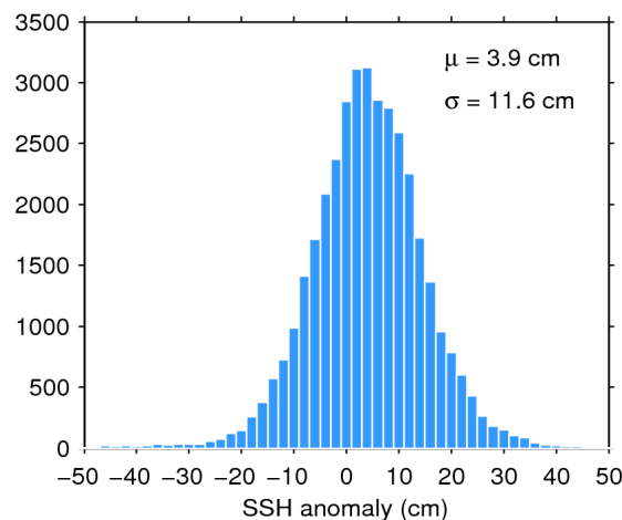
Figure 11. Histogram of science-valid SSH anomaly over oceans and lakes for 18/07/2018. The mean ( \mu ) and standard deviation ( \sigma ) are also shown. Note that values outside [-50 50] cm are excluded from the histogram for the sake of readability but not from the computation of \mu and \sigma .
