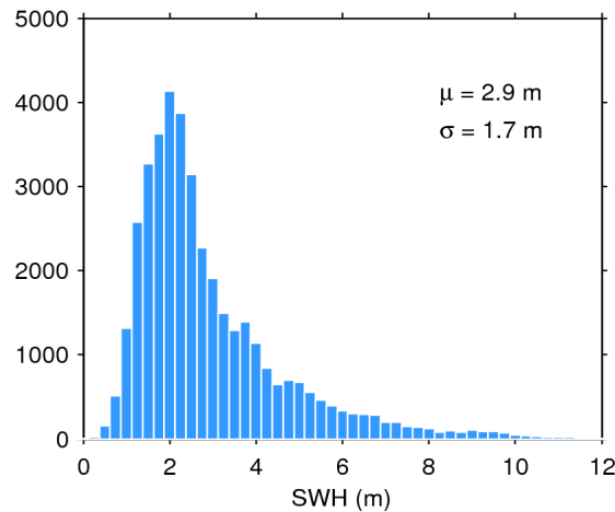
Figure 20. Histogram of science-valid SWH over oceans and lakes for 17/07/2018. The mean ( \mu ) and standard deviation ( \sigma ) are also shown. Note that values larger than 12 m are excluded from the histogram for the sake of readability but not from the computation of \mu and \sigma .
