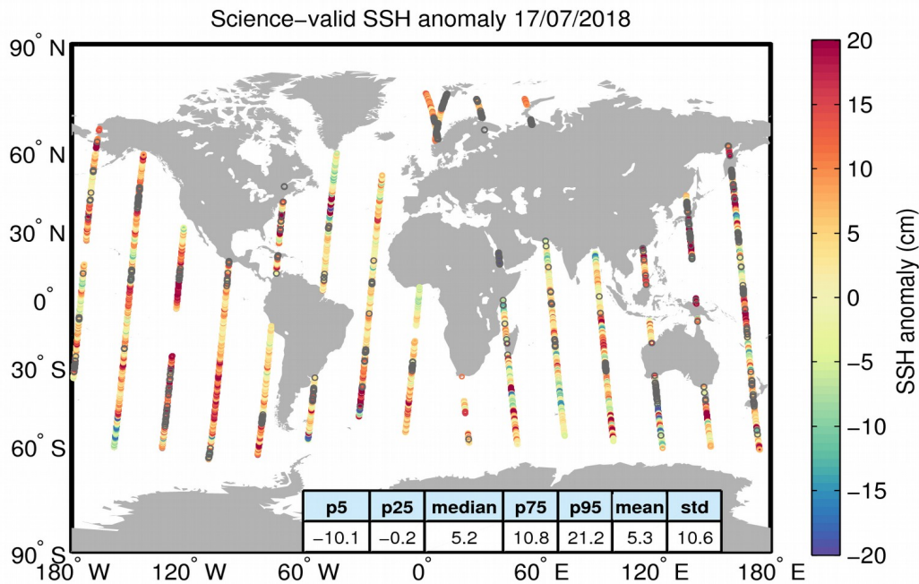
Figure 10. Geographical distribution of science-valid SSH anomaly data over oceans and lakes for 17/07/2018. The statistical values shown in the table refer to the SSH anomaly in cm and are calculated over all measurements shown in the figure. Gray circles denote records that have been rejected based on the editing criteria described in Table 2.
