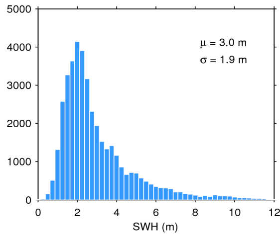
Figure 17. Histogram of flag-valid SWH over oceans and lakes for 17/07/2018. The mean ( \mu ) and standard deviation ( \sigma ) are also shown. Note that values larger than 12 m are excluded from the histogram for the sake of readability but not from the computation of \mu and \sigma .
