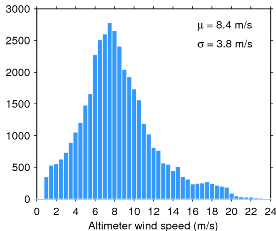
Figure 35. Histogram of science-valid wind over oceans and lakes for 17/07/2018. The mean ( \mu ) and standard deviation ( \sigma ) are also shown. Note that values larger than 24 m/s are excluded from the histogram for the sake of readability but not from the computation of \mu and \sigma .
