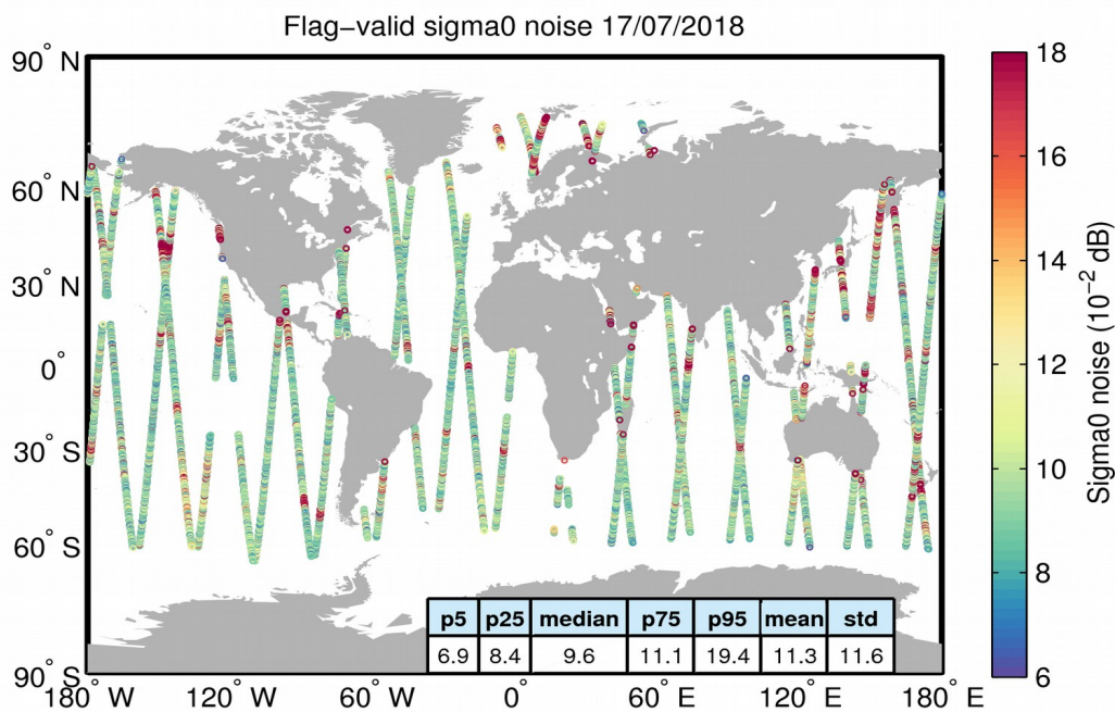
Figure 26. Geographical distribution of flag-valid 20-Hz sigma0 measurement noise over oceans and lakes for 17/07/2018. The statistical values shown in the table refer to the sigma0 noise and are calculated over all measurements shown in the figure.
