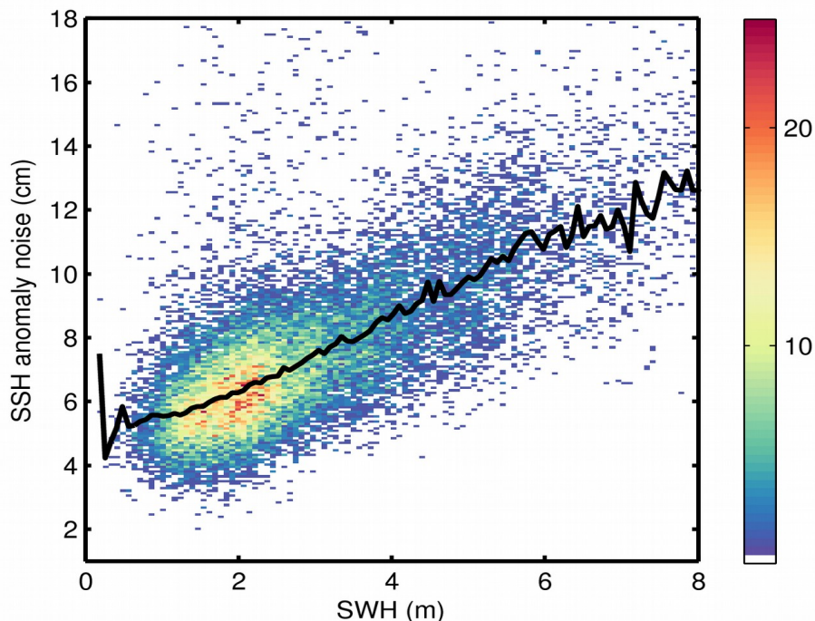
Figure 9. 2D histogram showing flag-valid SSH anomaly noise as a function of SWH for 17/07/2018. The black line denotes the median SSH anomaly noise as a function of SWH.
