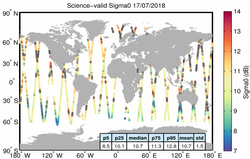
Figure 27. Geographical distribution of science-valid sigma0 data over oceans and lakes for 17/07/2018. The statistical values shown in the table refer to the sigma0 in dB and are calculated over all measurements shown in the figure. Gray circles denote records that have been rejected based on the editing criteria described in Table 4.
