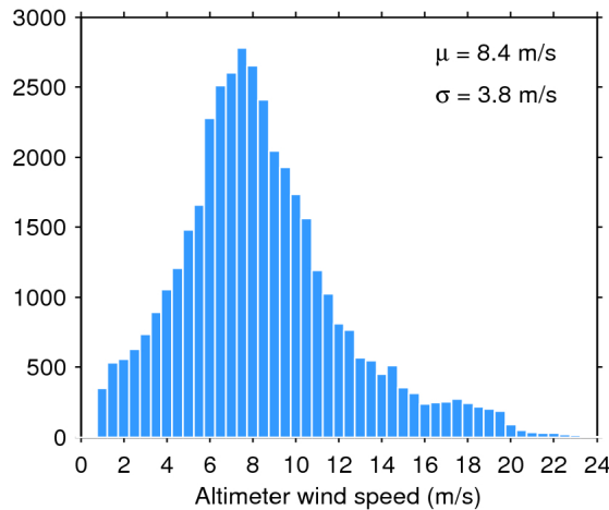
Figure 33. Histogram of flag-valid wind over oceans and lakes for 17/07/2018. The mean ( \mu ) and standard deviation ( \sigma ) are also shown. Note that values larger than 24 m/s are excluded from the histogram for the sake of readability but not from the computation of \mu and \sigma .
