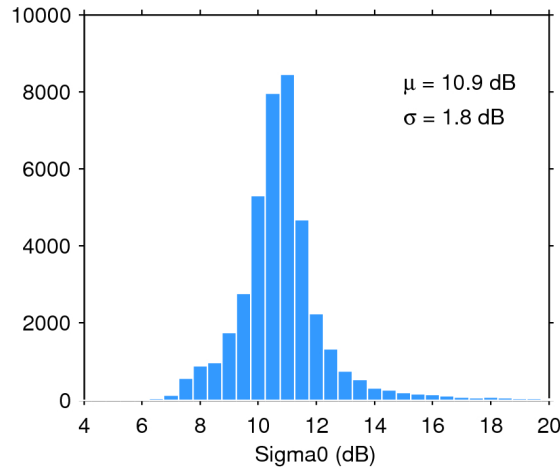
Figure 25. Histogram of flag-valid sigma0 over oceans and lakes for 17/07/2018. The mean ( \mu ) and standard deviation ( \sigma ) are also shown. Note that values outside [4 20] dB are excluded from the histogram for the sake of readability but not from the computation of \mu and \sigma .
