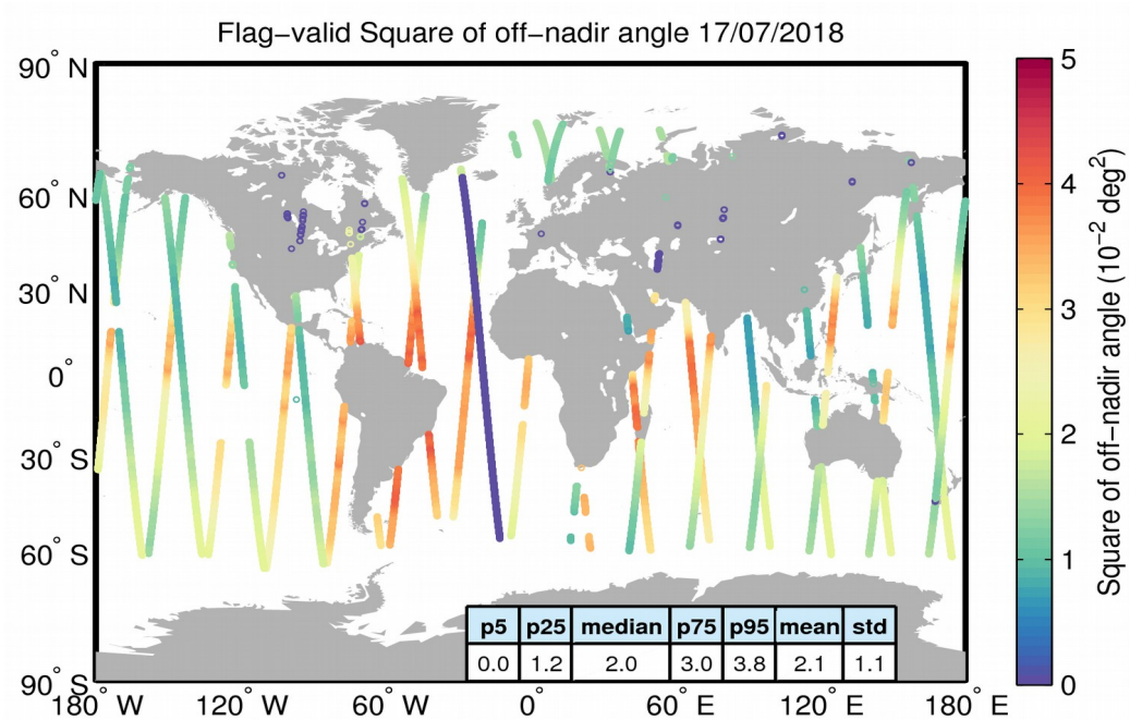
Figure 37. Geographical distribution of flag-valid mispointing data over oceans and lakes for 17/07/2018. The statistical values shown in the table refer to the mispointing in 10^{-2} deg 2 and are calculated over all measurements shown in the figure.
