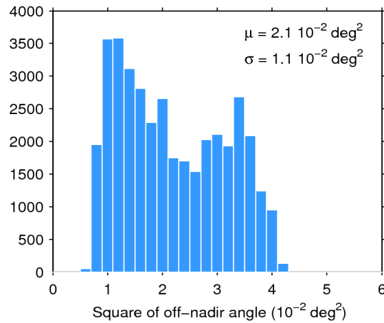
Figure 39. Histogram of flag-valid mispointing over oceans and lakes for 17/07/2018. The mean ( \mu ) and standard deviation ( \sigma ) are also shown. Note that values larger than 6 \cdot 10^{-2} \text{ deg}^2 are excluded from the histogram for the sake of readability but not from the computation of \mu and \sigma .
