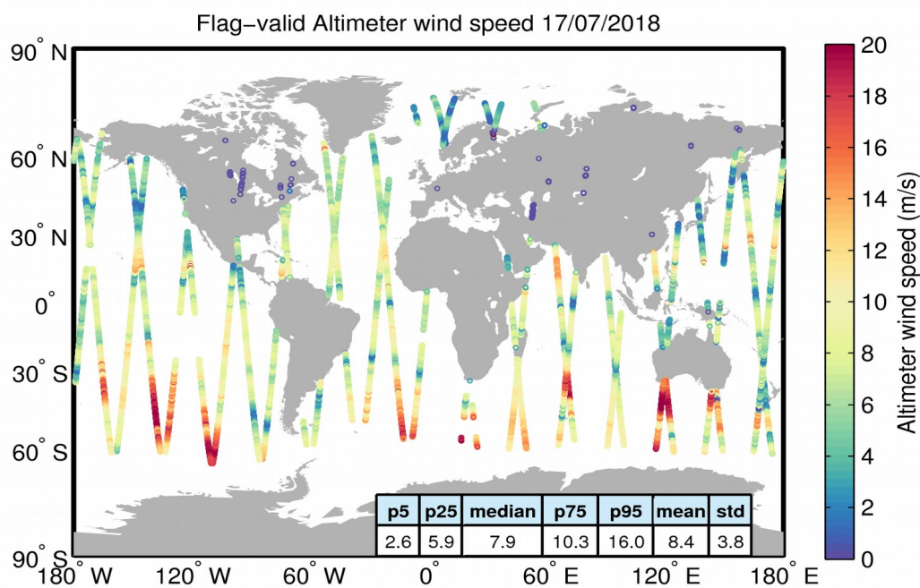
Figure 31. Geographical distribution of flag-valid wind data over oceans and lakes for 17/07/2018. The statistical values shown in the table refer to the wind in m/s and are calculated over all measurements shown in the figure.
