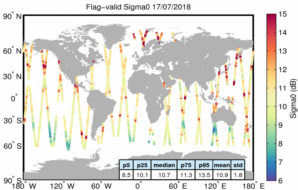
Figure 23. Geographical distribution of flag-valid sigma0 data over oceans and lakes for 17/07/2018. The statistical values shown in the table refer to the sigma0 in dB and are calculated over all measurements shown in the figure.
