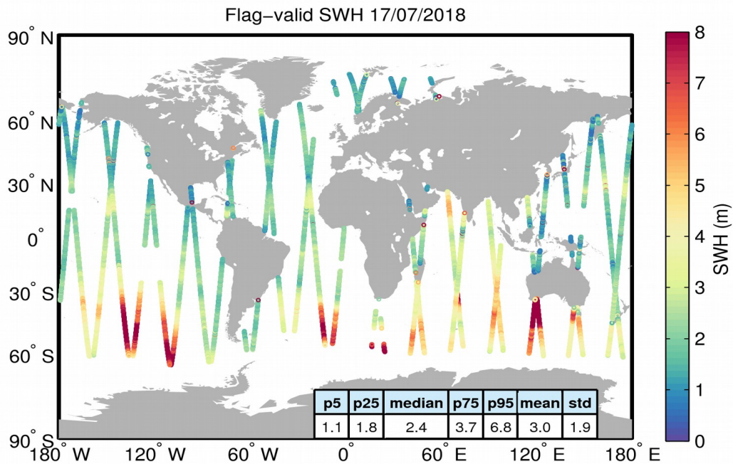
Figure 15. Geographical distribution of flag-valid SWH data over oceans and lakes for 17/07/2018. The statistical values shown in the table refer to the SWH in m and are calculated over all measurements shown in the figure.
