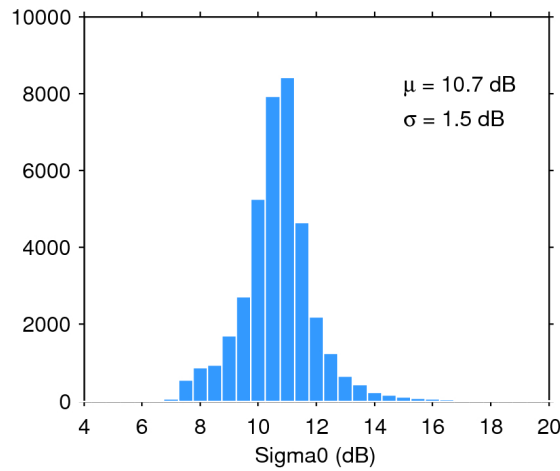
Figure 28. Histogram of science-valid sigma0 over oceans and lakes for 17/07/2018. The mean ( \mu ) and standard deviation ( \sigma ) are also shown. Note that values outside [4 20] dB are excluded from the histogram for the sake of readability but not from the computation of \mu and \sigma .
