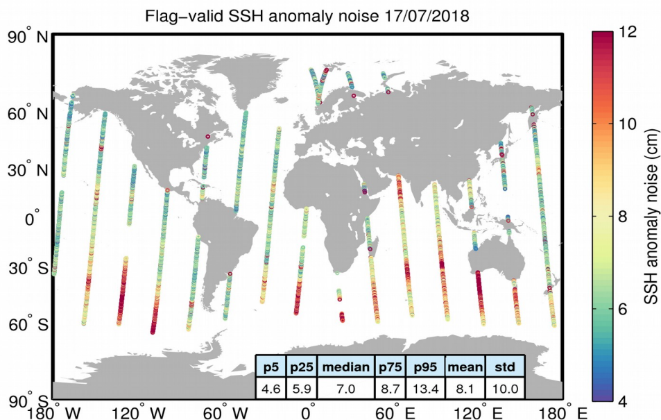
Figure 8. Geographical distribution of flag-valid 20-Hz SSH anomaly measurement noise over oceans and lakes for 17/07/2018. The statistical values shown in the table refer to the SSH anomaly noise and are calculated over all measurements shown in the figure.
