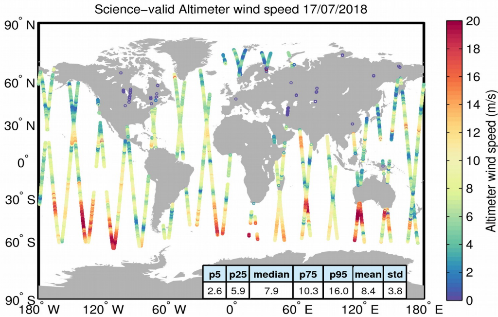
Figure 34. Geographical distribution of science-valid wind data over oceans and lakes for 17/07/2018. The statistical values shown in the table refer to the wind in m/s and are calculated over all measurements shown in the figure. Gray circles denote records that have been rejected based on the editing criteria described in Table 5.
