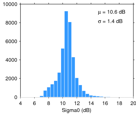
Figure 28. Histogram of science-valid sigma0 over oceans and lakes for 16/07/2018. The mean ( \mu ) and standard deviation ( \sigma ) are also shown. Note that values outside [4 20] dB are excluded from the histogram for the sake of readability but not from the computation of \mu and \sigma .
