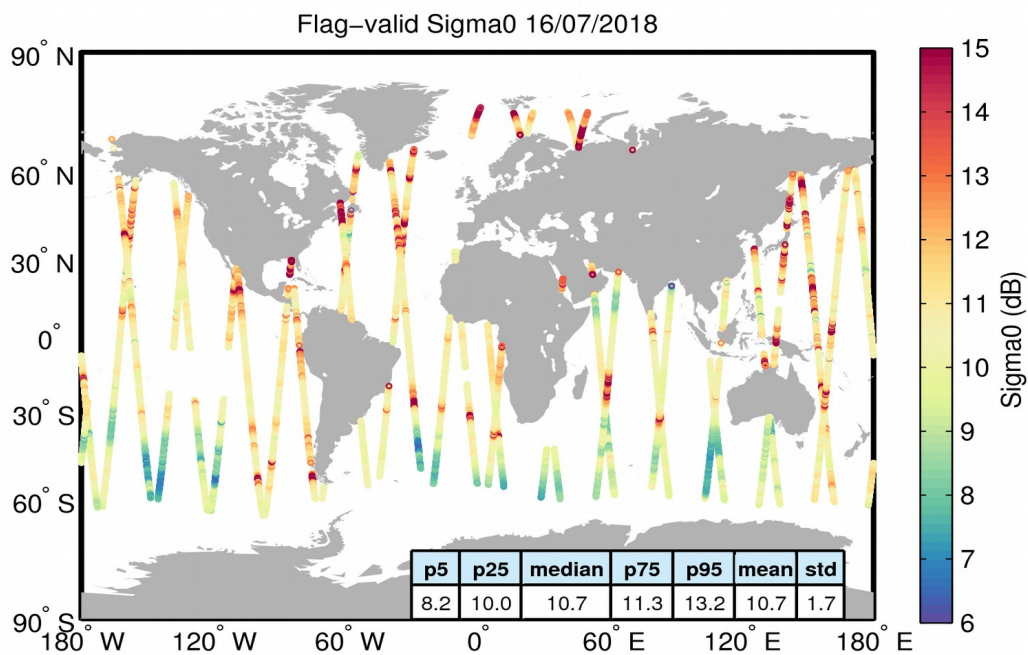
Figure 23. Geographical distribution of flag-valid sigma0 data over oceans and lakes for 16/07/2018. The statistical values shown in the table refer to the sigma0 in dB and are calculated over all measurements shown in the figure.
