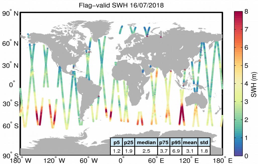
Figure 15. Geographical distribution of flag-valid SWH data over oceans and lakes for 16/07/2018. The statistical values shown in the table refer to the SWH in m and are calculated over all measurements shown in the figure.
