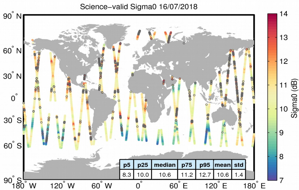
Figure 27. Geographical distribution of science-valid sigma0 data over oceans and lakes for 16/07/2018. The statistical values shown in the table refer to the sigma0 in dB and are calculated over all measurements shown in the figure. Gray circles denote records that have been rejected based on the editing criteria described in Table 4.
