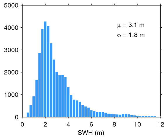
Figure 17. Histogram of flag-valid SWH over oceans and lakes for 16/07/2018. The mean ( \mu ) and standard deviation ( \sigma ) are also shown. Note that values larger than 12 m are excluded from the histogram for the sake of readability but not from the computation of \mu and \sigma .
