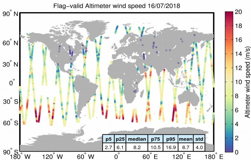
Figure 31. Geographical distribution of flag-valid wind data over oceans and lakes for 16/07/2018. The statistical values shown in the table refer to the wind in m/s and are calculated over all measurements shown in the figure.
