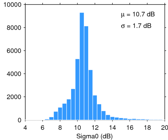
Figure 25. Histogram of flag-valid sigma0 over oceans and lakes for 16/07/2018. The mean ( \mu ) and standard deviation ( \sigma ) are also shown. Note that values outside [4 20] dB are excluded from the histogram for the sake of readability but not from the computation of \mu and \sigma .
