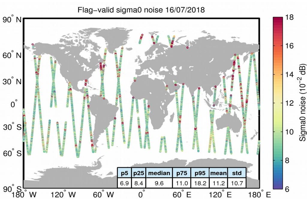
Figure 26. Geographical distribution of flag-valid 20-Hz sigma0 measurement noise over oceans and lakes for 16/07/2018. The statistical values shown in the table refer to the sigma0 noise and are calculated over all measurements shown in the figure.
