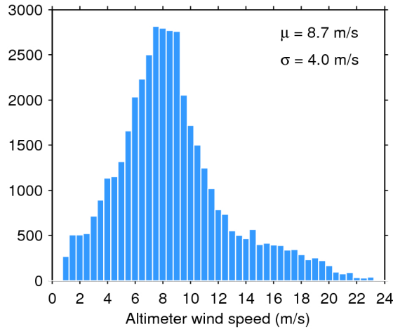
Figure 33. Histogram of flag-valid wind over oceans and lakes for 16/07/2018. The mean ( \mu ) and standard deviation ( \sigma ) are also shown. Note that values larger than 24 m/s are excluded from the histogram for the sake of readability but not from the computation of \mu and \sigma .
