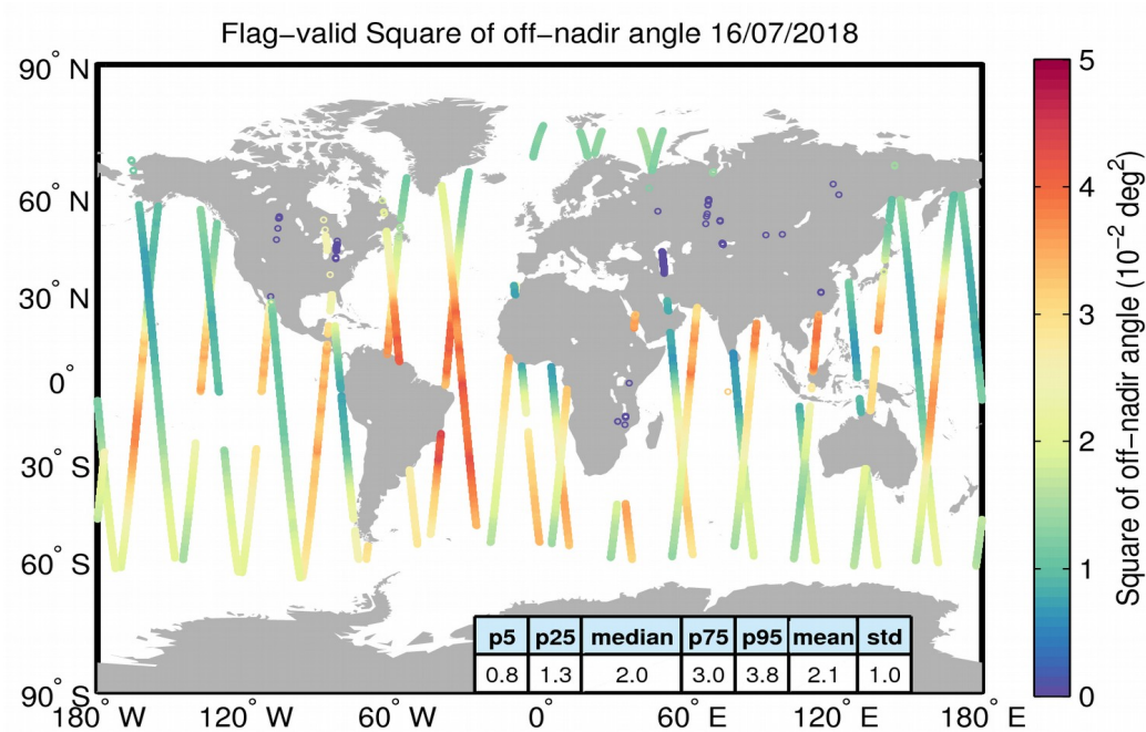
Figure 37. Geographical distribution of flag-valid mispointing data over oceans and lakes for 16/07/2018. The statistical values shown in the table refer to the mispointing in 10^{-2} \text{ deg}^2 and are calculated over all measurements shown in the figure.
