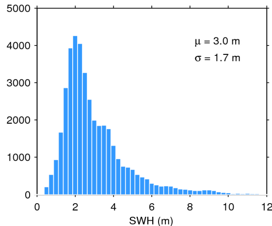
Figure 20. Histogram of science-valid SWH over oceans and lakes for 16/07/2018. The mean ( \mu ) and standard deviation ( \sigma ) are also shown. Note that values larger than 12 m are excluded from the histogram for the sake of readability but not from the computation of \mu and \sigma .
