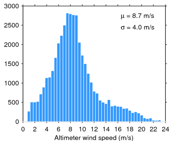
Figure 35. Histogram of science-valid wind over oceans and lakes for 16/07/2018. The mean ( \mu ) and standard deviation ( \sigma ) are also shown. Note that values larger than 24 m/s are excluded from the histogram for the sake of readability but not from the computation of \mu and \sigma .
