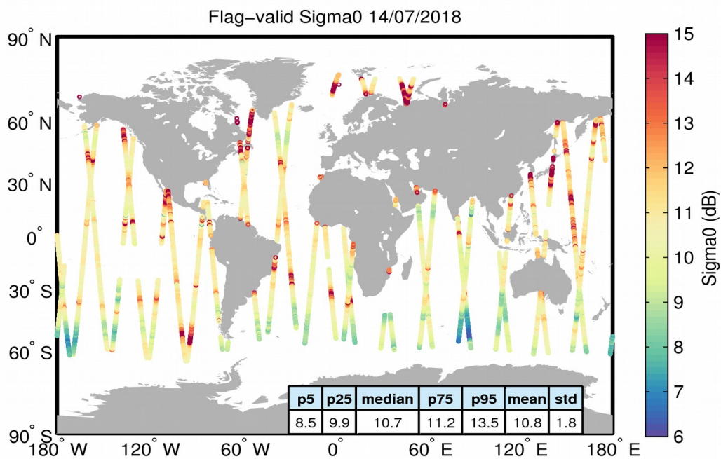
Figure 23. Geographical distribution of flag-valid sigma0 data over oceans and lakes for 14/07/2018. The statistical values shown in the table refer to the sigma0 in dB and are calculated over all measurements shown in the figure.
