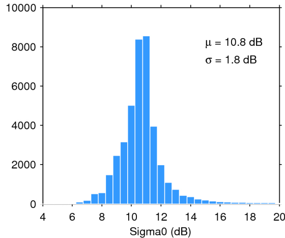
Figure 25. Histogram of flag-valid sigma0 over oceans and lakes for 14/07/2018. The mean ( \mu ) and standard deviation ( \sigma ) are also shown. Note that values outside [4 20] dB are excluded from the histogram for the sake of readability but not from the computation of \mu and \sigma .
