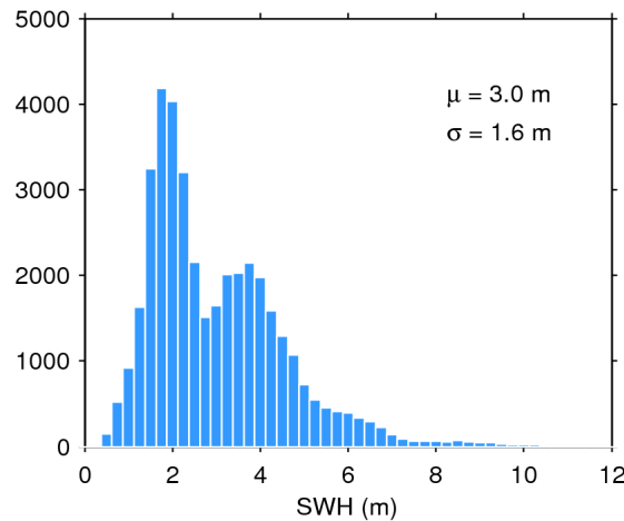
Figure 20. Histogram of science-valid SWH over oceans and lakes for 14/07/2018. The mean ( \mu ) and standard deviation ( \sigma ) are also shown. Note that values larger than 12 m are excluded from the histogram for the sake of readability but not from the computation of \mu and \sigma .
