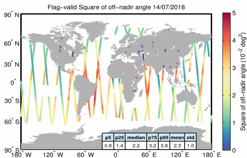
Figure 37. Geographical distribution of flag-valid mispointing data over oceans and lakes for 14/07/2018. The statistical values shown in the table refer to the mispointing in 10^{-2} deg 2 and are calculated over all measurements shown in the figure.
