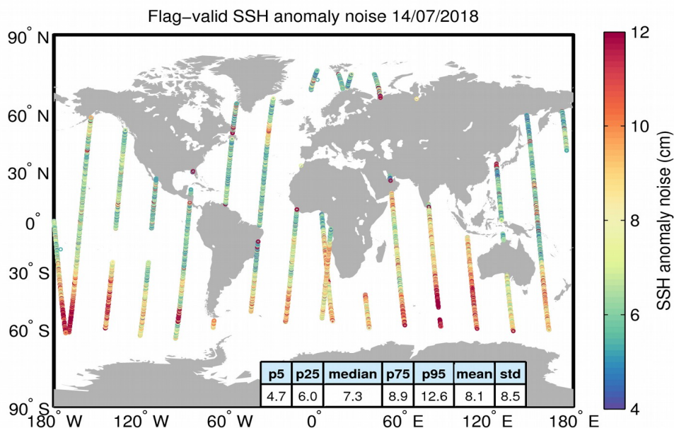
Figure 8. Geographical distribution of flag-valid 20-Hz SSH anomaly measurement noise over oceans and lakes for 14/07/2018. The statistical values shown in the table refer to the SSH anomaly noise and are calculated over all measurements shown in the figure.
