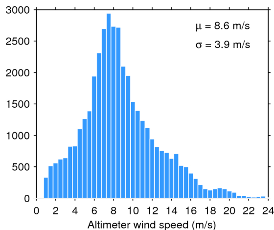
Figure 35. Histogram of science-valid wind over oceans and lakes for 14/07/2018. The mean ( \mu ) and standard deviation ( \sigma ) are also shown. Note that values larger than 24 m/s are excluded from the histogram for the sake of readability but not from the computation of \mu and \sigma .
