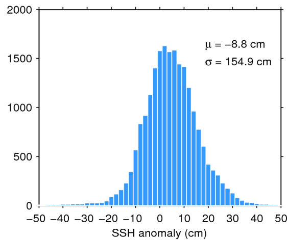
Figure 7. Histogram of flag-valid SSH anomaly over oceans and lakes for 14/07/2018. The mean ( \mu ) and standard deviation ( \sigma ) are also shown. Note that values outside [-50 50] cm are excluded from the histogram for the sake of readability but not from the computation of \mu and \sigma .
