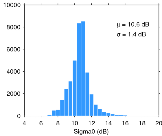
Figure 28. Histogram of science-valid sigma0 over oceans and lakes for 14/07/2018. The mean ( \mu ) and standard deviation ( \sigma ) are also shown. Note that values outside [4 20] dB are excluded from the histogram for the sake of readability but not from the computation of \mu and \sigma .
