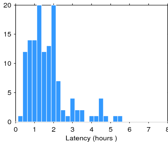
Figure 2. Histogram of the data latency for 14/07/2018. The y-axis denotes the number of files that are made available with a delay of x-hours with respect to the mean time of the records stored in the file.
