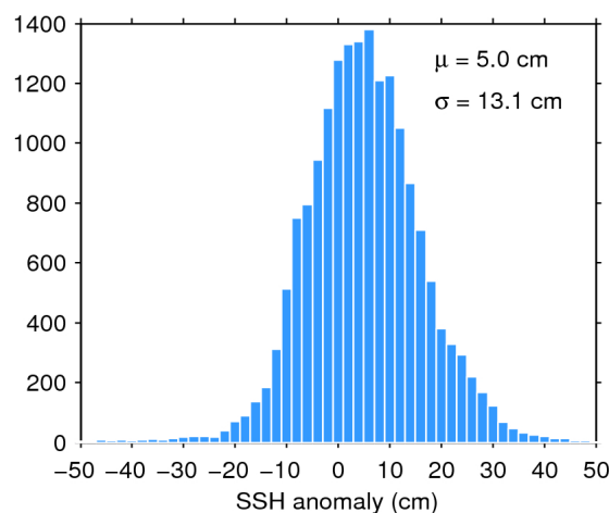
Figure 11. Histogram of science-valid SSH anomaly over oceans and lakes for 14/07/2018. The mean ( \mu ) and standard deviation ( \sigma ) are also shown. Note that values outside [-50 50] cm are excluded from the histogram for the sake of readability but not from the computation of \mu and \sigma .
