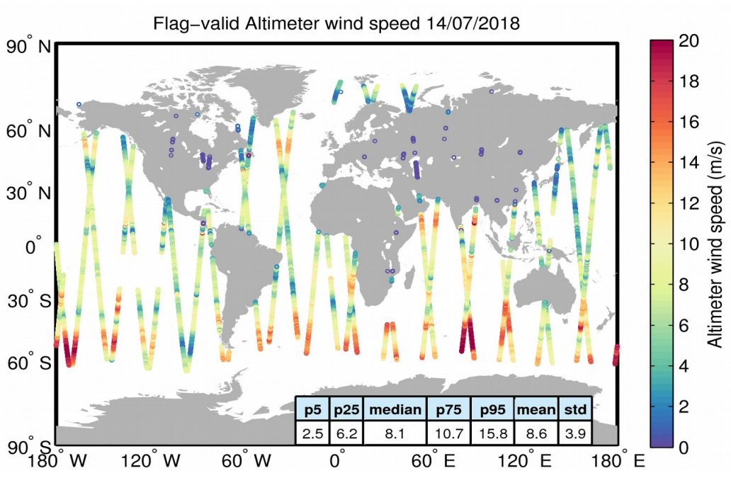
Figure 31. Geographical distribution of flag-valid wind data over oceans and lakes for 14/07/2018. The statistical values shown in the table refer to the wind in m/s and are calculated over all measurements shown in the figure.
