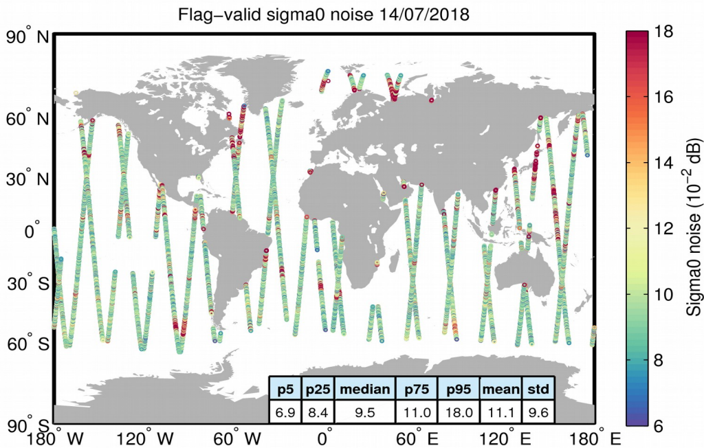
Figure 26. Geographical distribution of flag-valid 20-Hz sigma0 measurement noise over oceans and lakes for 14/07/2018. The statistical values shown in the table refer to the sigma0 noise and are calculated over all measurements shown in the figure.
