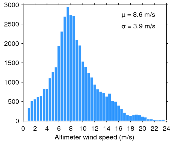
Figure 33. Histogram of flag-valid wind over oceans and lakes for 14/07/2018. The mean ( \mu ) and standard deviation ( \sigma ) are also shown. Note that values larger than 24 m/s are excluded from the histogram for the sake of readability but not from the computation of \mu and \sigma .
