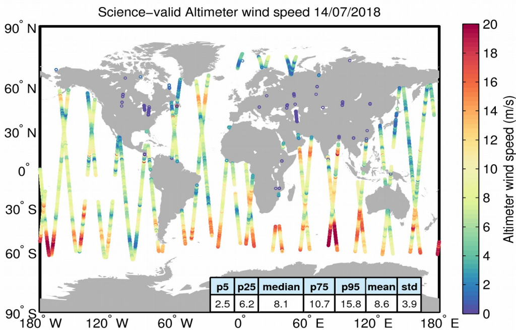
Figure 34. Geographical distribution of science-valid wind data over oceans and lakes for 14/07/2018. The statistical values shown in the table refer to the wind in m/s and are calculated over all measurements shown in the figure. Gray circles denote records that have been rejected based on the editing criteria described in Table 5.
