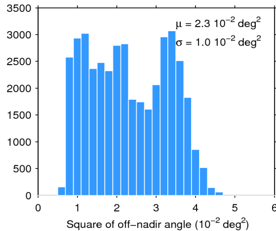
Figure 39. Histogram of flag-valid mispointing over oceans and lakes for 14/07/2018. The mean ( \mu ) and standard deviation ( \sigma ) are also shown. Note that values larger than 6 \cdot 10^{-2} \text{ deg}^2 are excluded from the histogram for the sake of readability but not from the computation of \mu and \sigma .
