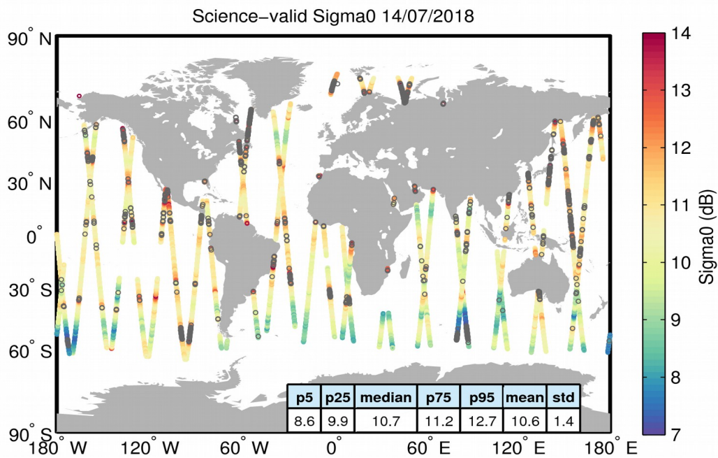
Figure 27. Geographical distribution of science-valid sigma0 data over oceans and lakes for 14/07/2018. The statistical values shown in the table refer to the sigma0 in dB and are calculated over all measurements shown in the figure. Gray circles denote records that have been rejected based on the editing criteria described in Table 4.
