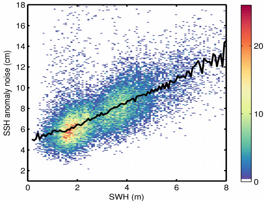
Figure 9. 2D histogram showing flag-valid SSH anomaly noise as a function of SWH for 14/07/2018. The black line denotes the median SSH anomaly noise as a function of SWH.
