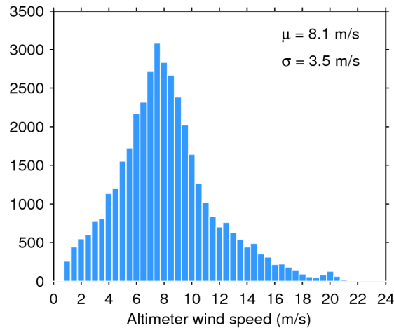
Figure 33. Histogram of flag-valid wind over oceans and lakes for 13/07/2018. The mean ( \mu ) and standard deviation ( \sigma ) are also shown. Note that values larger than 24 m/s are excluded from the histogram for the sake of readability but not from the computation of \mu and \sigma .
