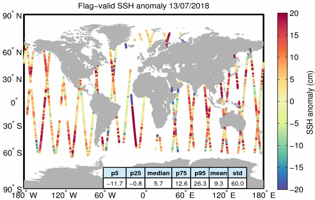
Figure 5. Geographical distribution of flag-valid 1-Hz SSH anomaly data over oceans and lakes for 13/07/2018. The statistical values shown in the table refer to the SSH anomaly in cm and are calculated over all measurements shown in the figure.
