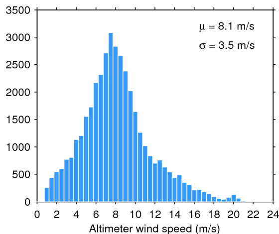
Figure 35. Histogram of science-valid wind over oceans and lakes for 13/07/2018. The mean ( \mu ) and standard deviation ( \sigma ) are also shown. Note that values larger than 24 m/s are excluded from the histogram for the sake of readability but not from the computation of \mu and \sigma .
