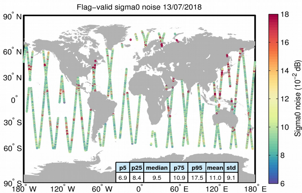
Figure 26. Geographical distribution of flag-valid 20-Hz sigma0 measurement noise over oceans and lakes for 13/07/2018. The statistical values shown in the table refer to the sigma0 noise and are calculated over all measurements shown in the figure.
