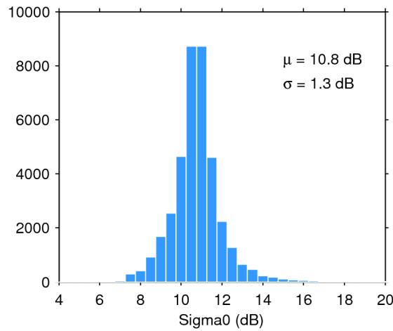
Figure 28. Histogram of science-valid sigma0 over oceans and lakes for 13/07/2018. The mean ( \mu ) and standard deviation ( \sigma ) are also shown. Note that values outside [4 20] dB are excluded from the histogram for the sake of readability but not from the computation of \mu and \sigma .
