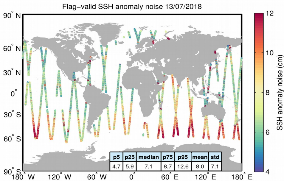
Figure 8. Geographical distribution of flag-valid 20-Hz SSH anomaly measurement noise over oceans and lakes for 13/07/2018. The statistical values shown in the table refer to the SSH anomaly noise and are calculated over all measurements shown in the figure.
