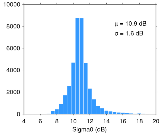
Figure 25. Histogram of flag-valid sigma0 over oceans and lakes for 13/07/2018. The mean ( \mu ) and standard deviation ( \sigma ) are also shown. Note that values outside [4 20] dB are excluded from the histogram for the sake of readability but not from the computation of \mu and \sigma .
