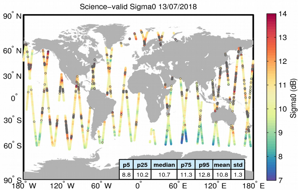
Figure 27. Geographical distribution of science-valid sigma0 data over oceans and lakes for 13/07/2018. The statistical values shown in the table refer to the sigma0 in dB and are calculated over all measurements shown in the figure. Gray circles denote records that have been rejected based on the editing criteria described in Table 4.
