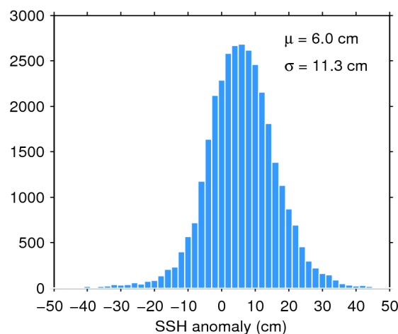
Figure 11. Histogram of science-valid SSH anomaly over oceans and lakes for 13/07/2018. The mean ( \mu ) and standard deviation ( \sigma ) are also shown. Note that values outside [-50 50] cm are excluded from the histogram for the sake of readability but not from the computation of \mu and \sigma .
