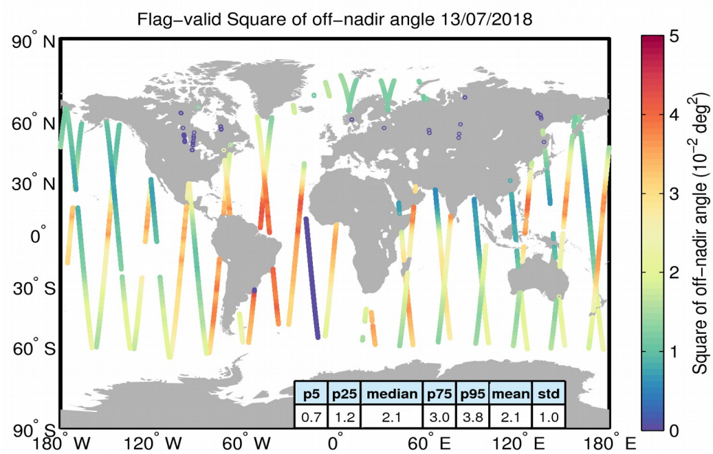
Figure 37. Geographical distribution of flag-valid mispointing data over oceans and lakes for 13/07/2018. The statistical values shown in the table refer to the mispointing in 10^{-2} \text{ deg}^2 and are calculated over all measurements shown in the figure.
