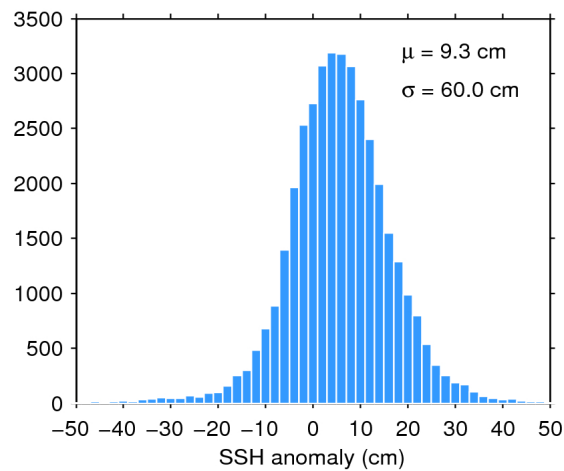
Figure 7. Histogram of flag-valid SSH anomaly over oceans and lakes for 13/07/2018. The mean ( \mu ) and standard deviation ( \sigma ) are also shown. Note that values outside [-50 50] cm are excluded from the histogram for the sake of readability but not from the computation of \mu and \sigma .
