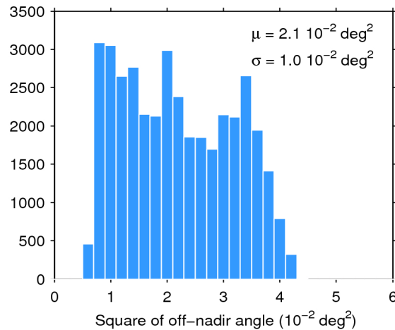
Figure 39. Histogram of flag-valid mispointing over oceans and lakes for 13/07/2018. The mean ( \mu ) and standard deviation ( \sigma ) are also shown. Note that values larger than 6 \cdot 10^{-2} \text{ deg}^2 are excluded from the histogram for the sake of readability but not from the computation of \mu and \sigma .
