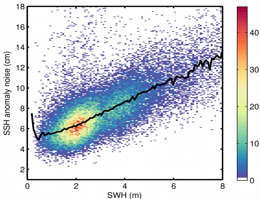
Figure 9. 2D histogram showing flag-valid SSH anomaly noise as a function of SWH for 13/07/2018. The black line denotes the median SSH anomaly noise as a function of SWH.
