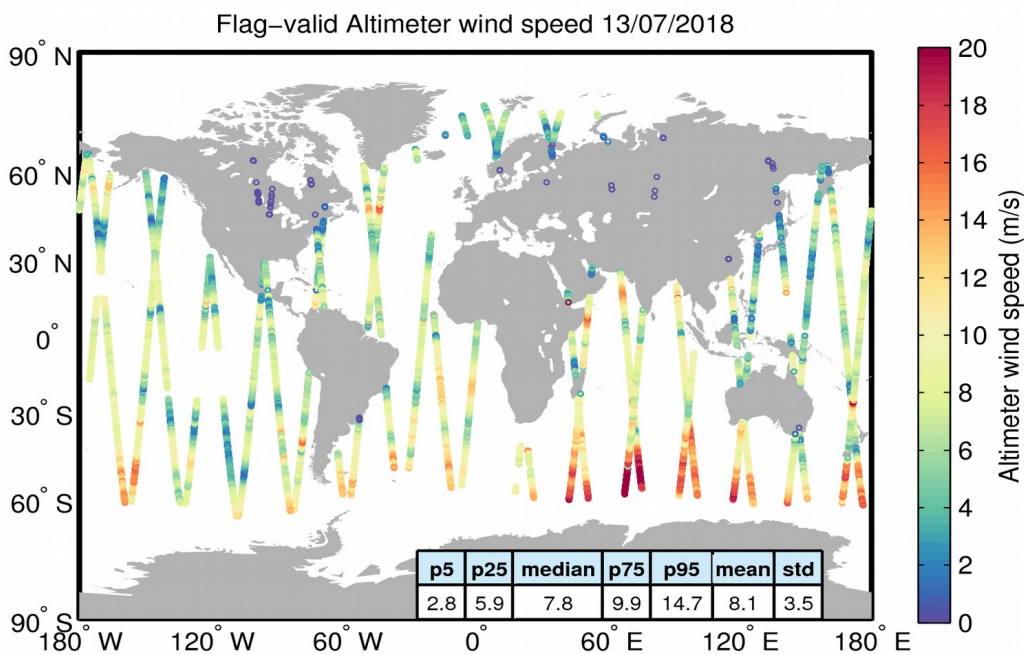
Figure 31. Geographical distribution of flag-valid wind data over oceans and lakes for 13/07/2018. The statistical values shown in the table refer to the wind in m/s and are calculated over all measurements shown in the figure.
