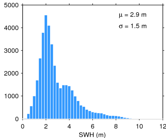
Figure 20. Histogram of science-valid SWH over oceans and lakes for 13/07/2018. The mean ( \mu ) and standard deviation ( \sigma ) are also shown. Note that values larger than 12 m are excluded from the histogram for the sake of readability but not from the computation of \mu and \sigma .
