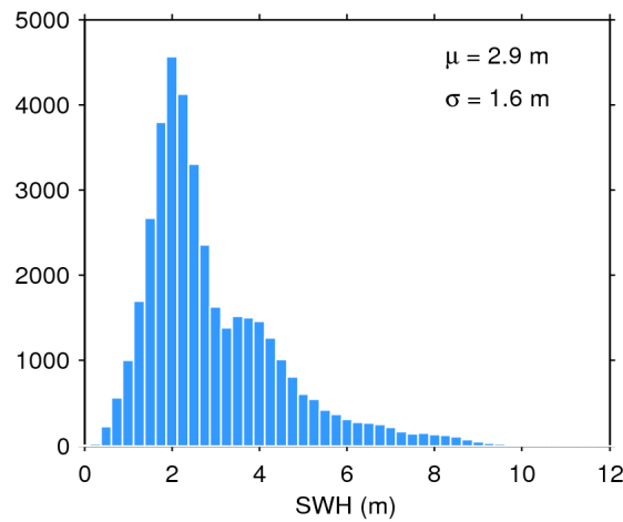
Figure 17. Histogram of flag-valid SWH over oceans and lakes for 13/07/2018. The mean ( \mu ) and standard deviation ( \sigma ) are also shown. Note that values larger than 12 m are excluded from the histogram for the sake of readability but not from the computation of \mu and \sigma .
