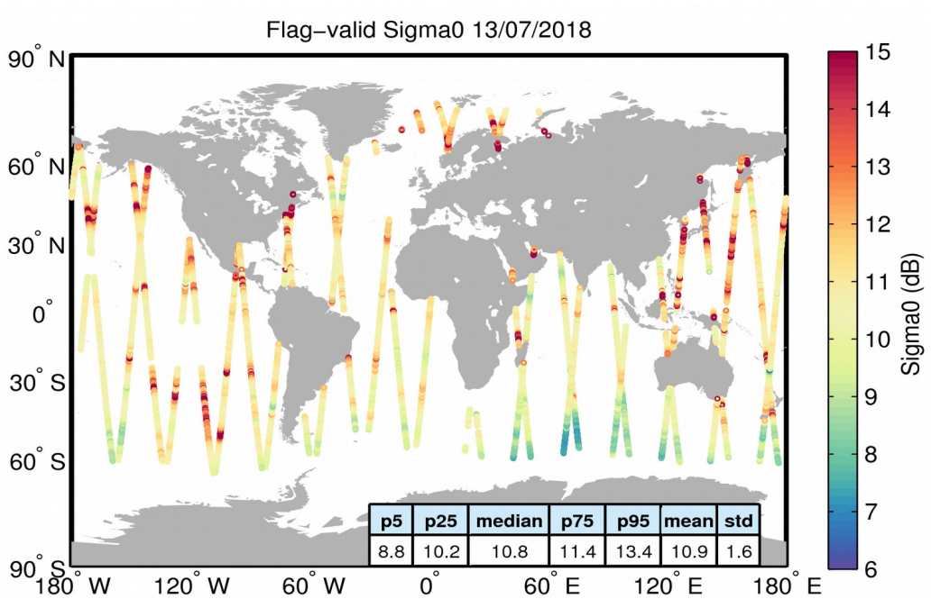
Figure 23. Geographical distribution of flag-valid sigma0 data over oceans and lakes for 13/07/2018. The statistical values shown in the table refer to the sigma0 in dB and are calculated over all measurements shown in the figure.
