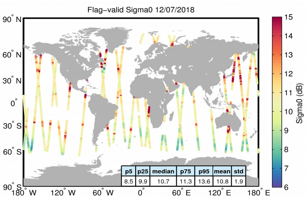
Figure 23. Geographical distribution of flag-valid sigma0 data over oceans and lakes for 12/07/2018. The statistical values shown in the table refer to the sigma0 in dB and are calculated over all measurements shown in the figure.
