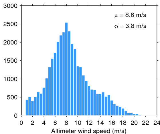
Figure 35. Histogram of science-valid wind over oceans and lakes for 12/07/2018. The mean ( \mu ) and standard deviation ( \sigma ) are also shown. Note that values larger than 24 m/s are excluded from the histogram for the sake of readability but not from the computation of \mu and \sigma .
