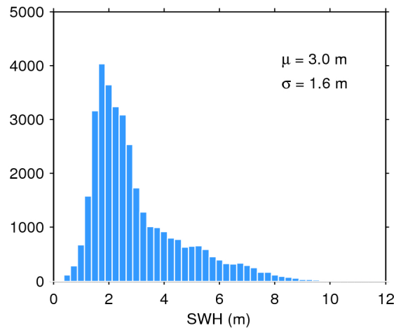
Figure 20. Histogram of science-valid SWH over oceans and lakes for 12/07/2018. The mean ( \mu ) and standard deviation ( \sigma ) are also shown. Note that values larger than 12 m are excluded from the histogram for the sake of readability but not from the computation of \mu and \sigma .
