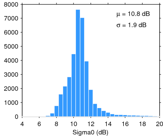
Figure 25. Histogram of flag-valid sigma0 over oceans and lakes for 12/07/2018. The mean ( \mu ) and standard deviation ( \sigma ) are also shown. Note that values outside [4 20] dB are excluded from the histogram for the sake of readability but not from the computation of \mu and \sigma .
