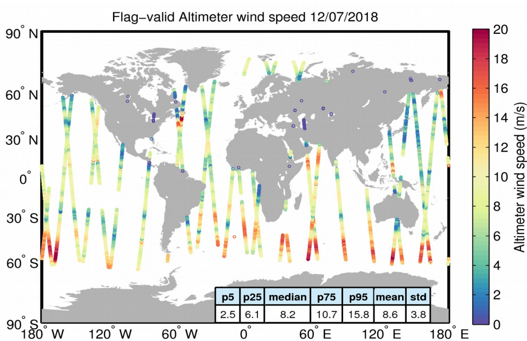
Figure 31. Geographical distribution of flag-valid wind data over oceans and lakes for 12/07/2018. The statistical values shown in the table refer to the wind in m/s and are calculated over all measurements shown in the figure.
