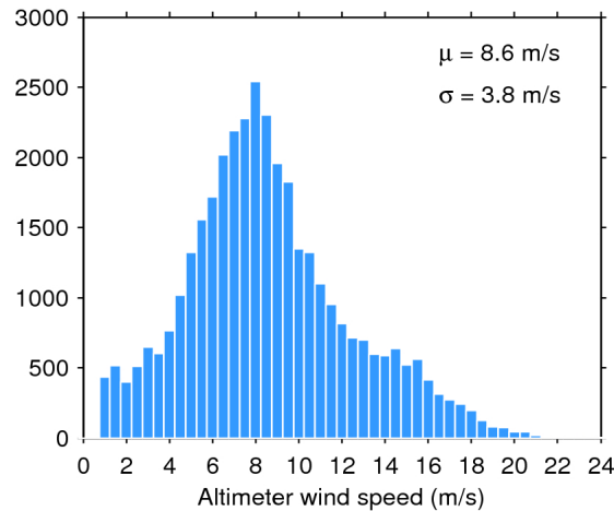
Figure 33. Histogram of flag-valid wind over oceans and lakes for 12/07/2018. The mean ( \mu ) and standard deviation ( \sigma ) are also shown. Note that values larger than 24 m/s are excluded from the histogram for the sake of readability but not from the computation of \mu and \sigma .
