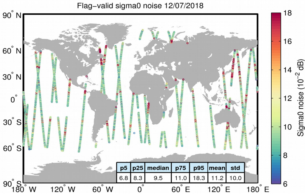
Figure 26. Geographical distribution of flag-valid 20-Hz sigma0 measurement noise over oceans and lakes for 12/07/2018. The statistical values shown in the table refer to the sigma0 noise and are calculated over all measurements shown in the figure.
