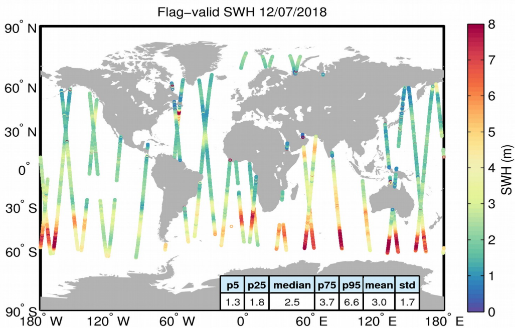
Figure 15. Geographical distribution of flag-valid SWH data over oceans and lakes for 12/07/2018. The statistical values shown in the table refer to the SWH in m and are calculated over all measurements shown in the figure.
