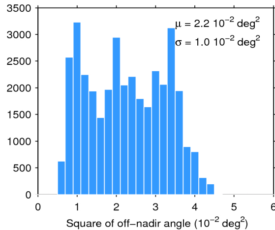
Figure 39. Histogram of flag-valid mispointing over oceans and lakes for 12/07/2018. The mean ( \mu ) and standard deviation ( \sigma ) are also shown. Note that values larger than 6 \cdot 10^{-2} \text{ deg}^2 are excluded from the histogram for the sake of readability but not from the computation of \mu and \sigma .
