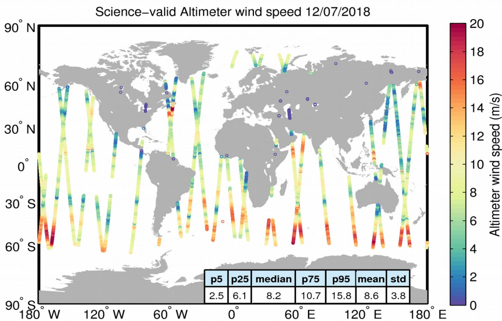
Figure 34. Geographical distribution of science-valid wind data over oceans and lakes for 12/07/2018. The statistical values shown in the table refer to the wind in m/s and are calculated over all measurements shown in the figure. Gray circles denote records that have been rejected based on the editing criteria described in Table 5.
