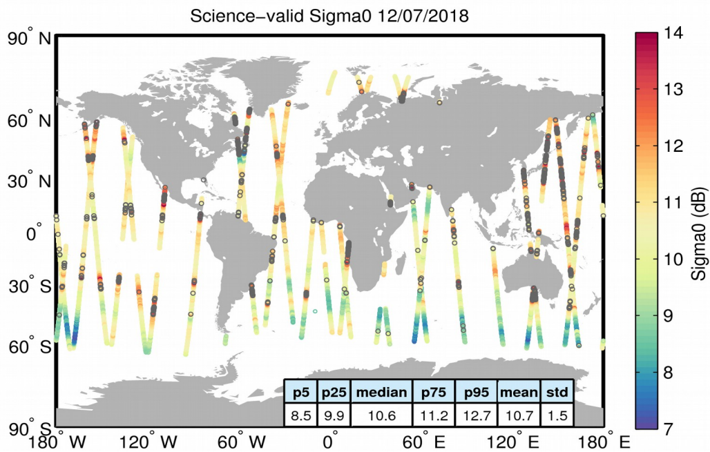
Figure 27. Geographical distribution of science-valid sigma0 data over oceans and lakes for 12/07/2018. The statistical values shown in the table refer to the sigma0 in dB and are calculated over all measurements shown in the figure. Gray circles denote records that have been rejected based on the editing criteria described in Table 4.
