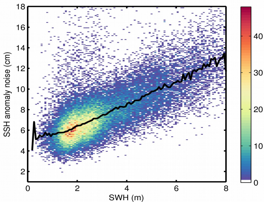
Figure 9. 2D histogram showing flag-valid SSH anomaly noise as a function of SWH for 12/07/2018. The black line denotes the median SSH anomaly noise as a function of SWH.
