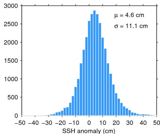
Figure 11. Histogram of science-valid SSH anomaly over oceans and lakes for 12/07/2018. The mean ( \mu ) and standard deviation ( \sigma ) are also shown. Note that values outside [-50 50] cm are excluded from the histogram for the sake of readability but not from the computation of \mu and \sigma .
