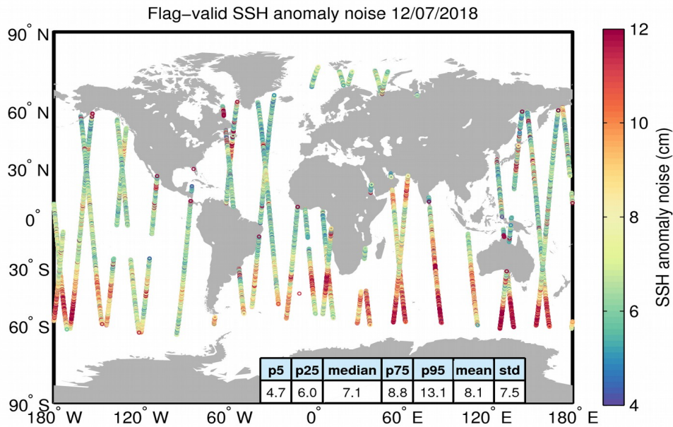
Figure 8. Geographical distribution of flag-valid 20-Hz SSH anomaly measurement noise over oceans and lakes for 12/07/2018. The statistical values shown in the table refer to the SSH anomaly noise and are calculated over all measurements shown in the figure.
