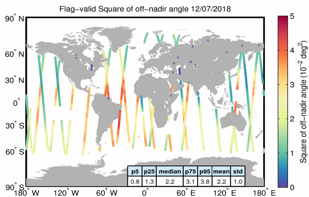
Figure 37. Geographical distribution of flag-valid mispointing data over oceans and lakes for 12/07/2018. The statistical values shown in the table refer to the mispointing in 10^{-2} \text{ deg}^2 and are calculated over all measurements shown in the figure.
