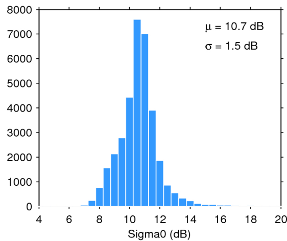
Figure 28. Histogram of science-valid sigma0 over oceans and lakes for 12/07/2018. The mean ( \mu ) and standard deviation ( \sigma ) are also shown. Note that values outside [4 20] dB are excluded from the histogram for the sake of readability but not from the computation of \mu and \sigma .
