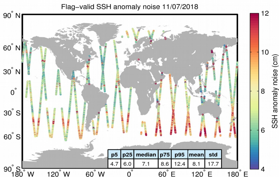
Figure 8. Geographical distribution of flag-valid 20-Hz SSH anomaly measurement noise over oceans and lakes for 11/07/2018. The statistical values shown in the table refer to the SSH anomaly noise and are calculated over all measurements shown in the figure.
