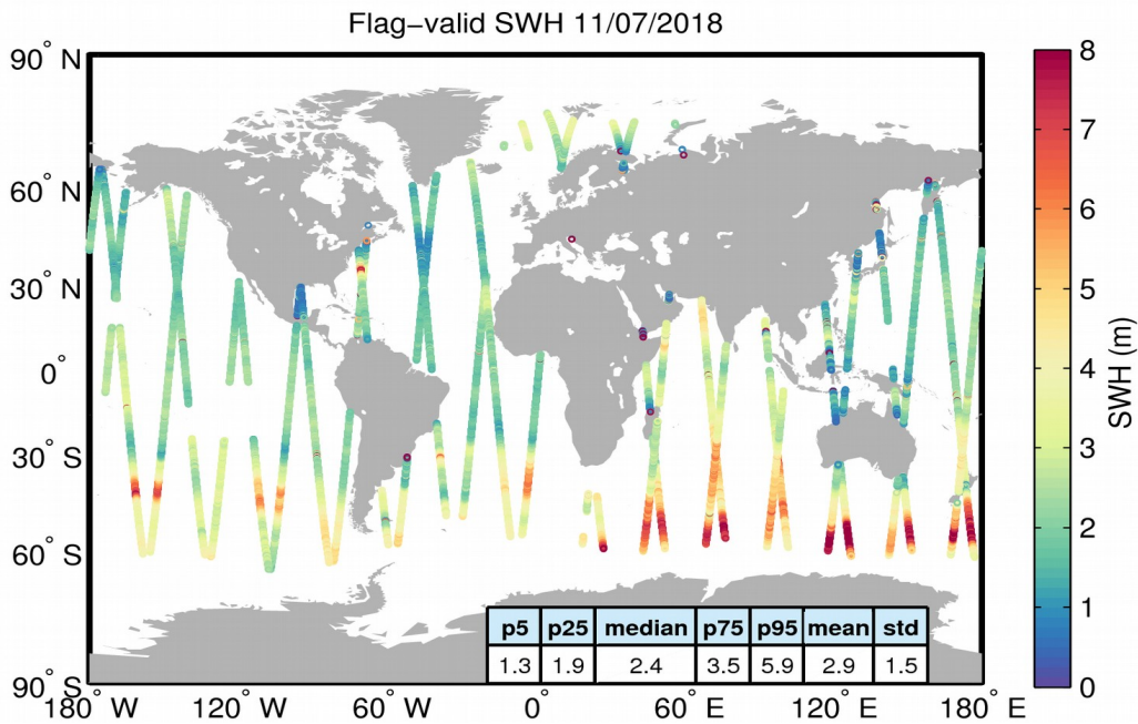
Figure 15. Geographical distribution of flag-valid SWH data over oceans and lakes for 11/07/2018. The statistical values shown in the table refer to the SWH in m and are calculated over all measurements shown in the figure.
