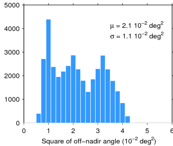
Figure 39. Histogram of flag-valid mispointing over oceans and lakes for 11/07/2018. The mean ( \mu ) and standard deviation ( \sigma ) are also shown. Note that values larger than 6 \cdot 10^{-2} \text{ deg}^2 are excluded from the histogram for the sake of readability but not from the computation of \mu and \sigma .
