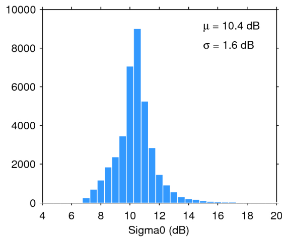
Figure 28. Histogram of science-valid sigma0 over oceans and lakes for 11/07/2018. The mean ( \mu ) and standard deviation ( \sigma ) are also shown. Note that values outside [4 20] dB are excluded from the histogram for the sake of readability but not from the computation of \mu and \sigma .
