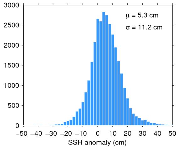
Figure 11. Histogram of science-valid SSH anomaly over oceans and lakes for 11/07/2018. The mean ( \mu ) and standard deviation ( \sigma ) are also shown. Note that values outside [-50 50] cm are excluded from the histogram for the sake of readability but not from the computation of \mu and \sigma .
