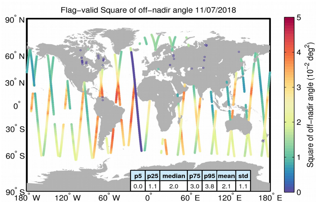
Figure 37. Geographical distribution of flag-valid mispointing data over oceans and lakes for 11/07/2018. The statistical values shown in the table refer to the mispointing in 10^{-2} \text{ deg}^2 and are calculated over all measurements shown in the figure.
