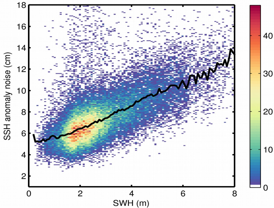
Figure 9. 2D histogram showing flag-valid SSH anomaly noise as a function of SWH for 11/07/2018. The black line denotes the median SSH anomaly noise as a function of SWH.
