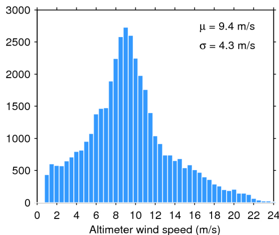
Figure 35. Histogram of science-valid wind over oceans and lakes for 11/07/2018. The mean ( \mu ) and standard deviation ( \sigma ) are also shown. Note that values larger than 24 m/s are excluded from the histogram for the sake of readability but not from the computation of \mu and \sigma .
