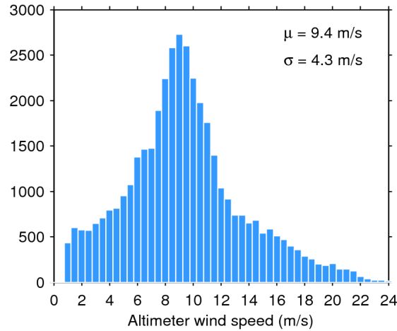
Figure 33. Histogram of flag-valid wind over oceans and lakes for 11/07/2018. The mean ( \mu ) and standard deviation ( \sigma ) are also shown. Note that values larger than 24 m/s are excluded from the histogram for the sake of readability but not from the computation of \mu and \sigma .
