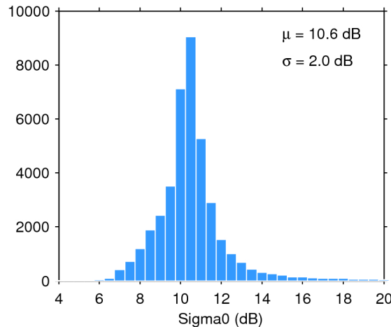
Figure 25. Histogram of flag-valid sigma0 over oceans and lakes for 11/07/2018. The mean ( \mu ) and standard deviation ( \sigma ) are also shown. Note that values outside [4 20] dB are excluded from the histogram for the sake of readability but not from the computation of \mu and \sigma .
