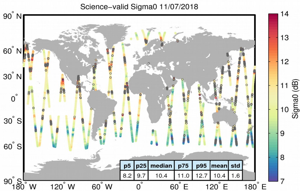
Figure 27. Geographical distribution of science-valid sigma0 data over oceans and lakes for 11/07/2018. The statistical values shown in the table refer to the sigma0 in dB and are calculated over all measurements shown in the figure. Gray circles denote records that have been rejected based on the editing criteria described in Table 4.
