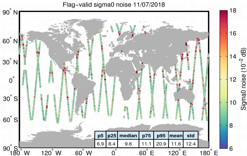
Figure 26. Geographical distribution of flag-valid 20-Hz sigma0 measurement noise over oceans and lakes for 11/07/2018. The statistical values shown in the table refer to the sigma0 noise and are calculated over all measurements shown in the figure.
