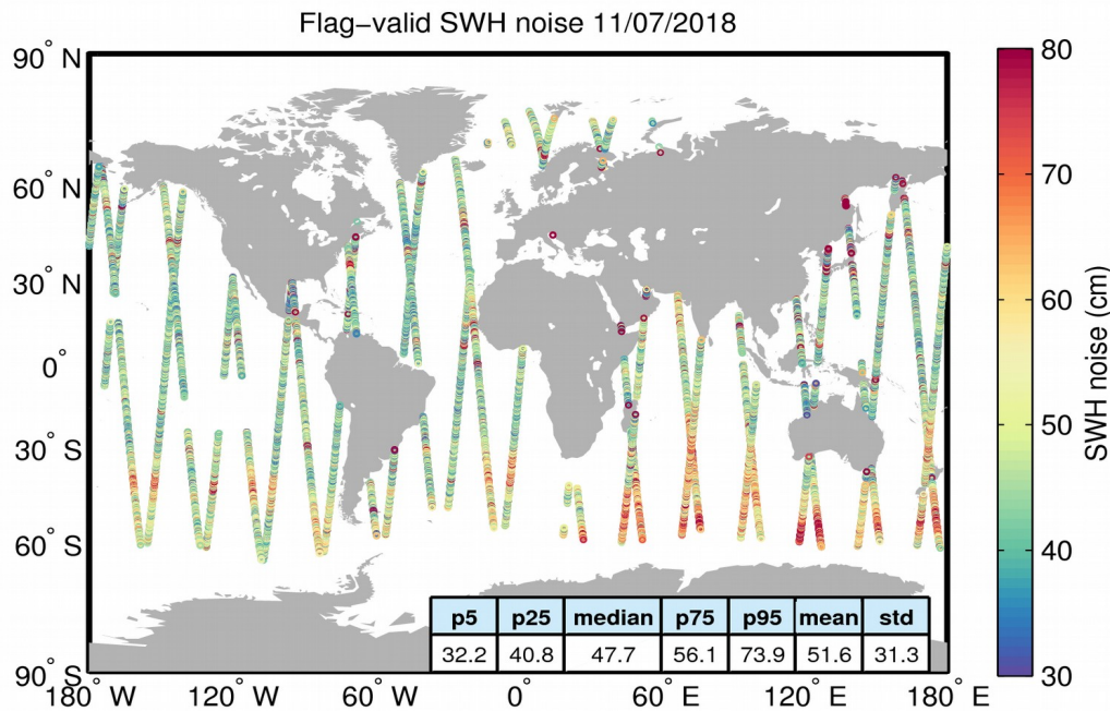
Figure 18. Geographical distribution of flag-valid 20-Hz SWH measurement noise over oceans and lakes for 11/07/2018. The statistical values shown in the figure refer to the SWH noise and are calculated over all measurements shown in the figure.
