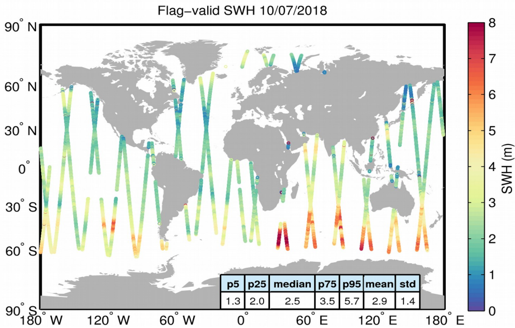
Figure 15. Geographical distribution of flag-valid SWH data over oceans and lakes for 10/07/2018. The statistical values shown in the table refer to the SWH in m and are calculated over all measurements shown in the figure.
