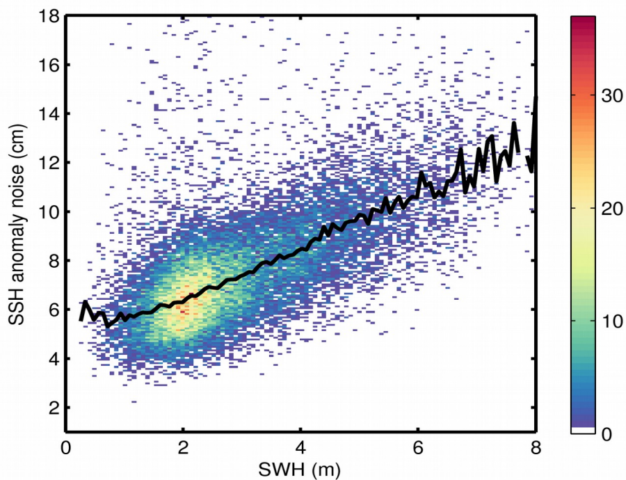
Figure 9. 2D histogram showing flag-valid SSH anomaly noise as a function of SWH for 10/07/2018. The black line denotes the median SSH anomaly noise as a function of SWH.
