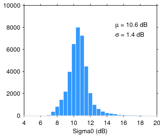
Figure 28. Histogram of science-valid sigma0 over oceans and lakes for 10/07/2018. The mean ( \mu ) and standard deviation ( \sigma ) are also shown. Note that values outside [4 20] dB are excluded from the histogram for the sake of readability but not from the computation of \mu and \sigma .
