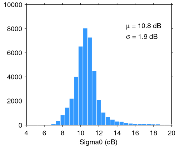
Figure 25. Histogram of flag-valid sigma0 over oceans and lakes for 10/07/2018. The mean ( \mu ) and standard deviation ( \sigma ) are also shown. Note that values outside [4 20] dB are excluded from the histogram for the sake of readability but not from the computation of \mu and \sigma .
