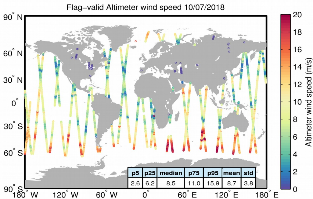
Figure 31. Geographical distribution of flag-valid wind data over oceans and lakes for 10/07/2018. The statistical values shown in the table refer to the wind in m/s and are calculated over all measurements shown in the figure.
