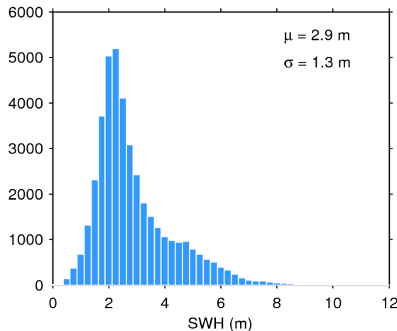
Figure 20. Histogram of science-valid SWH over oceans and lakes for 10/07/2018. The mean ( \mu ) and standard deviation ( \sigma ) are also shown. Note that values larger than 12 m are excluded from the histogram for the sake of readability but not from the computation of \mu and \sigma .
