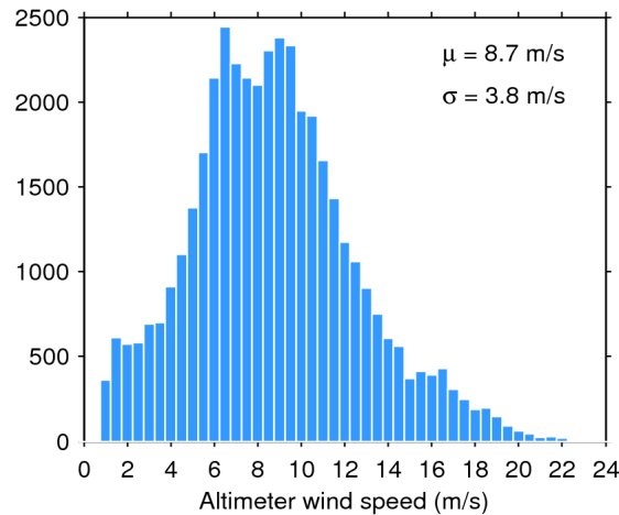
Figure 33. Histogram of flag-valid wind over oceans and lakes for 10/07/2018. The mean ( \mu ) and standard deviation ( \sigma ) are also shown. Note that values larger than 24 m/s are excluded from the histogram for the sake of readability but not from the computation of \mu and \sigma .
