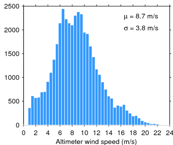
Figure 35. Histogram of science-valid wind over oceans and lakes for 10/07/2018. The mean ( \mu ) and standard deviation ( \sigma ) are also shown. Note that values larger than 24 m/s are excluded from the histogram for the sake of readability but not from the computation of \mu and \sigma .
