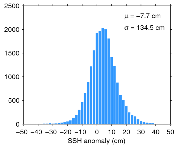
Figure 7. Histogram of flag-valid SSH anomaly over oceans and lakes for 10/07/2018. The mean ( \mu ) and standard deviation ( \sigma ) are also shown. Note that values outside [-50 50] cm are excluded from the histogram for the sake of readability but not from the computation of \mu and \sigma .
