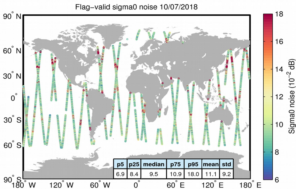
Figure 26. Geographical distribution of flag-valid 20-Hz sigma0 measurement noise over oceans and lakes for 10/07/2018. The statistical values shown in the table refer to the sigma0 noise and are calculated over all measurements shown in the figure.
