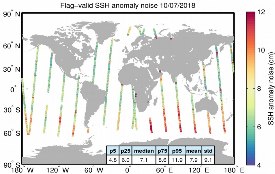
Figure 8. Geographical distribution of flag-valid 20-Hz SSH anomaly measurement noise over oceans and lakes for 10/07/2018. The statistical values shown in the table refer to the SSH anomaly noise and are calculated over all measurements shown in the figure.
