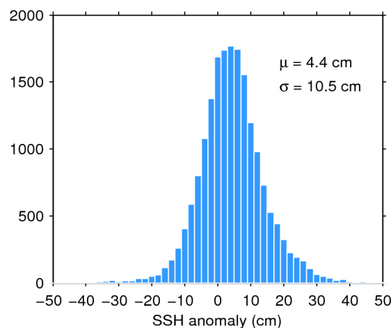
Figure 11. Histogram of science-valid SSH anomaly over oceans and lakes for 10/07/2018. The mean ( \mu ) and standard deviation ( \sigma ) are also shown. Note that values outside [-50 50] cm are excluded from the histogram for the sake of readability but not from the computation of \mu and \sigma .
