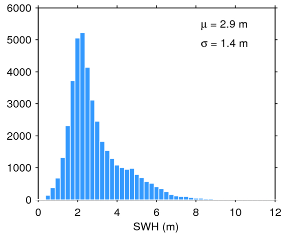
Figure 17. Histogram of flag-valid SWH over oceans and lakes for 10/07/2018. The mean ( \mu ) and standard deviation ( \sigma ) are also shown. Note that values larger than 12 m are excluded from the histogram for the sake of readability but not from the computation of \mu and \sigma .
