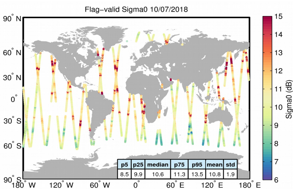
Figure 23. Geographical distribution of flag-valid sigma0 data over oceans and lakes for 10/07/2018. The statistical values shown in the table refer to the sigma0 in dB and are calculated over all measurements shown in the figure.
