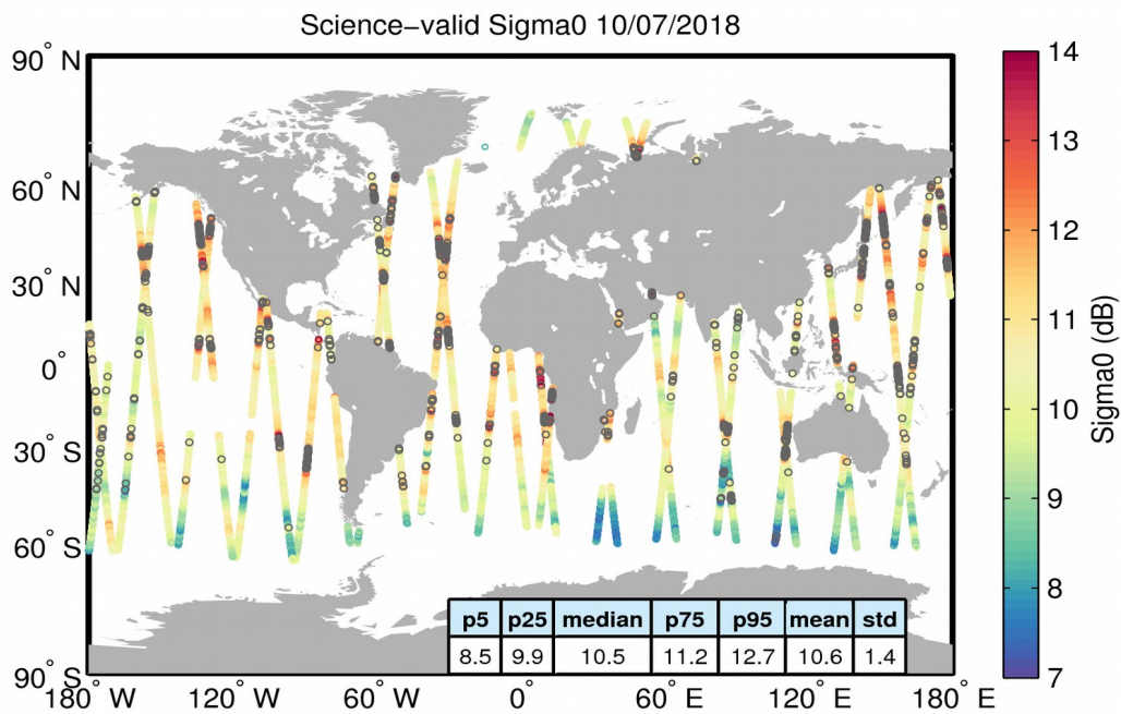
Figure 27. Geographical distribution of science-valid sigma0 data over oceans and lakes for 10/07/2018. The statistical values shown in the table refer to the sigma0 in dB and are calculated over all measurements shown in the figure. Gray circles denote records that have been rejected based on the editing criteria described in Table 4.
