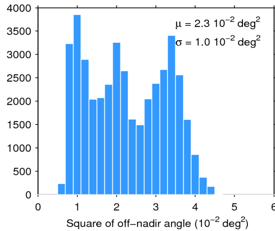
Figure 39. Histogram of flag-valid mispointing over oceans and lakes for 10/07/2018. The mean ( \mu ) and standard deviation ( \sigma ) are also shown. Note that values larger than 6 \cdot 10^{-2} \text{ deg}^2 are excluded from the histogram for the sake of readability but not from the computation of \mu and \sigma .
