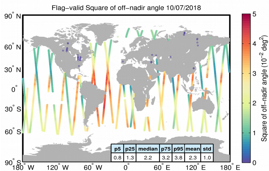
Figure 37. Geographical distribution of flag-valid mispointing data over oceans and lakes for 10/07/2018. The statistical values shown in the table refer to the mispointing in 10^{-2} deg 2 and are calculated over all measurements shown in the figure.
