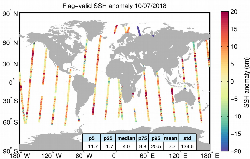
Figure 5. Geographical distribution of flag-valid 1-Hz SSH anomaly data over oceans and lakes for 10/07/2018. The statistical values shown in the table refer to the SSH anomaly in cm and are calculated over all measurements shown in the figure.
