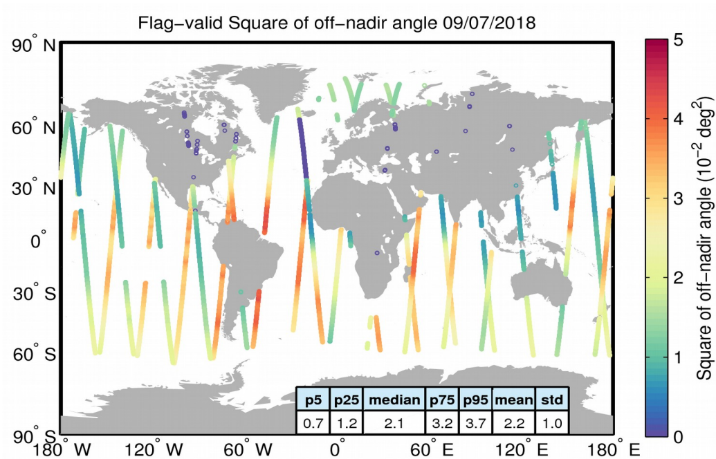
Figure 37. Geographical distribution of flag-valid mispointing data over oceans and lakes for 09/07/2018. The statistical values shown in the table refer to the mispointing in 10^{-2} \text{deg}^2 and are calculated over all measurements shown in the figure.
