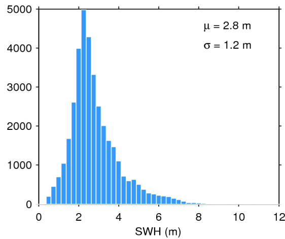
Figure 17. Histogram of flag-valid SWH over oceans and lakes for 09/07/2018. The mean ( \mu ) and standard deviation ( \sigma ) are also shown. Note that values larger than 12 m are excluded from the histogram for the sake of readability but not from the computation of \mu and \sigma .
