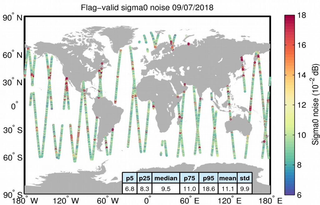
Figure 26. Geographical distribution of flag-valid 20-Hz sigma0 measurement noise over oceans and lakes for 09/07/2018. The statistical values shown in the table refer to the sigma0 noise and are calculated over all measurements shown in the figure.
