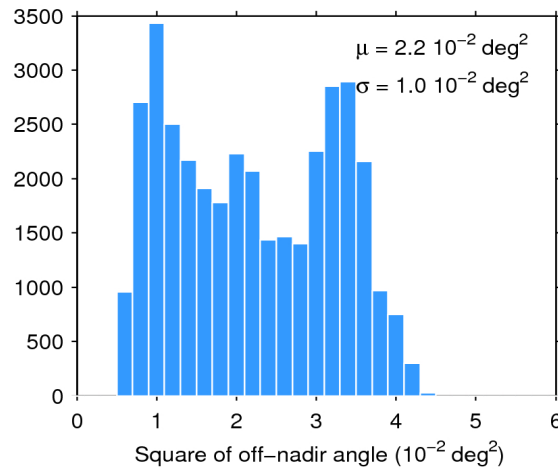
Figure 39. Histogram of flag-valid mispointing over oceans and lakes for 09/07/2018. The mean ( \mu ) and standard deviation ( \sigma ) are also shown. Note that values larger than 6 \cdot 10^{-2} \text{ deg}^2 are excluded from the histogram for the sake of readability but not from the computation of \mu and \sigma .
