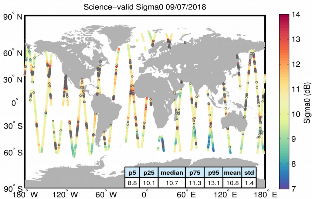
Figure 27. Geographical distribution of science-valid sigma0 data over oceans and lakes for 09/07/2018. The statistical values shown in the table refer to the sigma0 in dB and are calculated over all measurements shown in the figure. Gray circles denote records that have been rejected based on the editing criteria described in Table 4.
