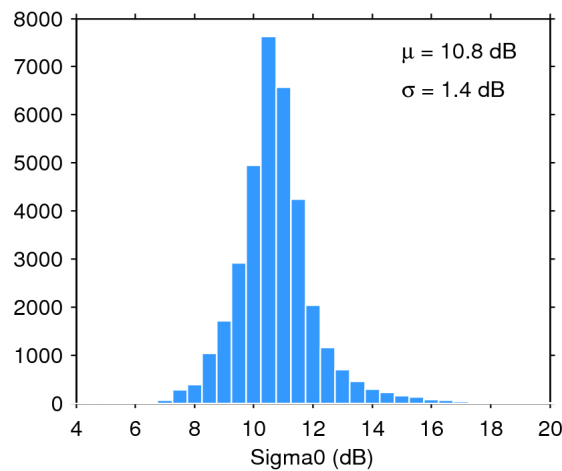
Figure 28. Histogram of science-valid sigma0 over oceans and lakes for 09/07/2018. The mean ( \mu ) and standard deviation ( \sigma ) are also shown. Note that values outside [4 20] dB are excluded from the histogram for the sake of readability but not from the computation of \mu and \sigma .
