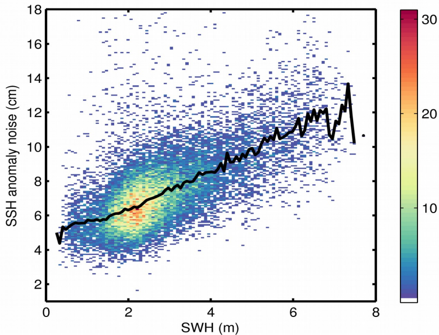
Figure 9. 2D histogram showing flag-valid SSH anomaly noise as a function of SWH for 09/07/2018. The black line denotes the median SSH anomaly noise as a function of SWH.
