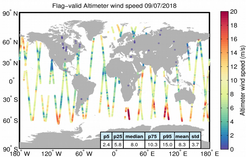
Figure 31. Geographical distribution of flag-valid wind data over oceans and lakes for 09/07/2018. The statistical values shown in the table refer to the wind in m/s and are calculated over all measurements shown in the figure.
