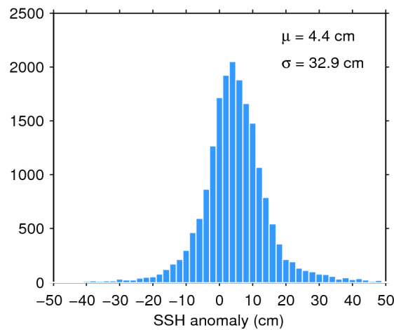
Figure 7. Histogram of flag-valid SSH anomaly over oceans and lakes for 09/07/2018. The mean ( \mu ) and standard deviation ( \sigma ) are also shown. Note that values outside [-50 \ 50] cm are excluded from the histogram for the sake of readability but not from the computation of \mu and \sigma .
