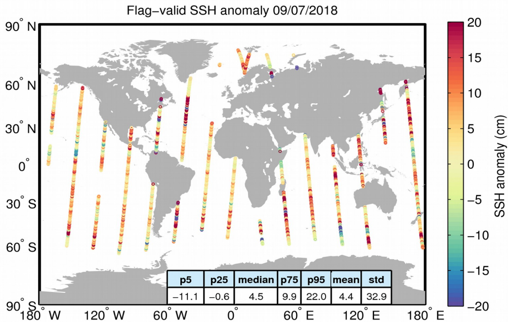
Figure 5. Geographical distribution of flag-valid 1-Hz SSH anomaly data over oceans and lakes for 09/07/2018. The statistical values shown in the table refer to the SSH anomaly in cm and are calculated over all measurements shown in the figure.
