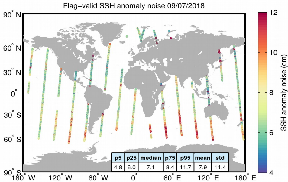
Figure 8. Geographical distribution of flag-valid 20-Hz SSH anomaly measurement noise over oceans and lakes for 09/07/2018. The statistical values shown in the table refer to the SSH anomaly noise and are calculated over all measurements shown in the figure.
