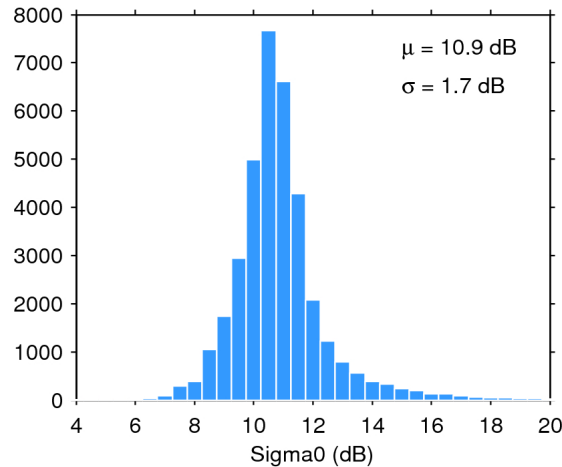
Figure 25. Histogram of flag-valid sigma0 over oceans and lakes for 09/07/2018. The mean ( \mu ) and standard deviation ( \sigma ) are also shown. Note that values outside [4 20] dB are excluded from the histogram for the sake of readability but not from the computation of \mu and \sigma .
