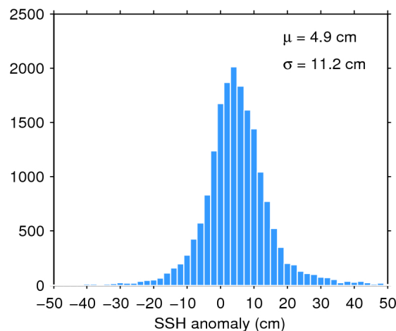
Figure 11. Histogram of science-valid SSH anomaly over oceans and lakes for 09/07/2018. The mean ( \mu ) and standard deviation ( \sigma ) are also shown. Note that values outside [-50 50] cm are excluded from the histogram for the sake of readability but not from the computation of \mu and \sigma .
