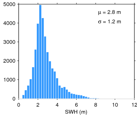
Figure 20. Histogram of science-valid SWH over oceans and lakes for 09/07/2018. The mean ( \mu ) and standard deviation ( \sigma ) are also shown. Note that values larger than 12 m are excluded from the histogram for the sake of readability but not from the computation of \mu and \sigma .
