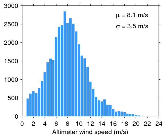
Figure 35. Histogram of science-valid wind over oceans and lakes for 08/07/2018. The mean ( \mu ) and standard deviation ( \sigma ) are also shown. Note that values larger than 24 m/s are excluded from the histogram for the sake of readability but not from the computation of \mu and \sigma .
