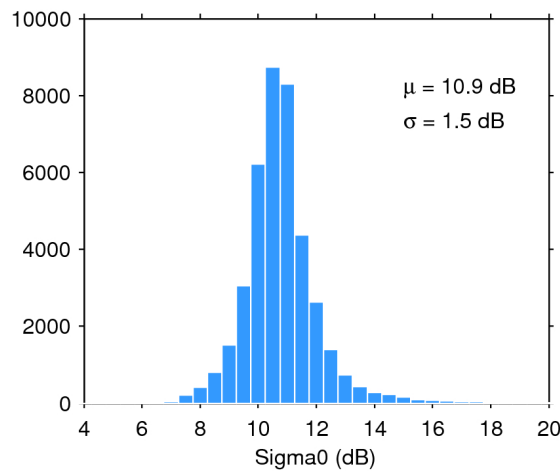
Figure 28. Histogram of science-valid sigma0 over oceans and lakes for 08/07/2018. The mean ( \mu ) and standard deviation ( \sigma ) are also shown. Note that values outside [4 20] dB are excluded from the histogram for the sake of readability but not from the computation of \mu and \sigma .
