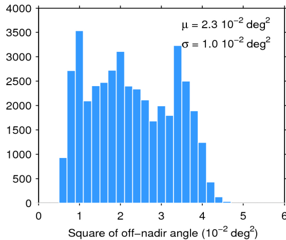
Figure 39. Histogram of flag-valid mispointing over oceans and lakes for 08/07/2018. The mean ( \mu ) and standard deviation ( \sigma ) are also shown. Note that values larger than 6 \cdot 10^{-2} \text{ deg}^2 are excluded from the histogram for the sake of readability but not from the computation of \mu and \sigma .
