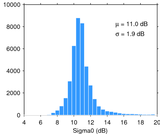
Figure 25. Histogram of flag-valid sigma0 over oceans and lakes for 08/07/2018. The mean ( \mu ) and standard deviation ( \sigma ) are also shown. Note that values outside [4 20] dB are excluded from the histogram for the sake of readability but not from the computation of \mu and \sigma .
