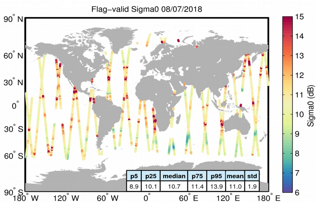
Figure 23. Geographical distribution of flag-valid sigma0 data over oceans and lakes for 08/07/2018. The statistical values shown in the table refer to the sigma0 in dB and are calculated over all measurements shown in the figure.
