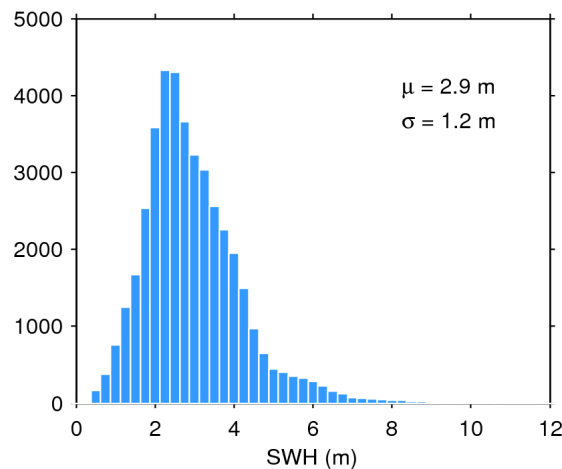
Figure 17. Histogram of flag-valid SWH over oceans and lakes for 08/07/2018. The mean ( \mu ) and standard deviation ( \sigma ) are also shown. Note that values larger than 12 m are excluded from the histogram for the sake of readability but not from the computation of \mu and \sigma .
