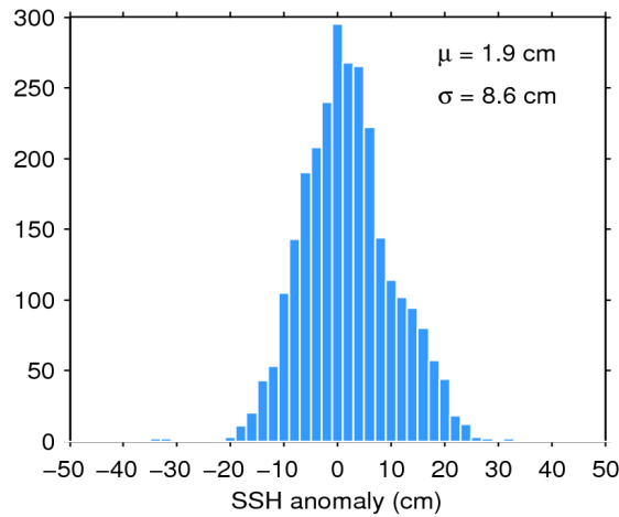
Figure 11. Histogram of science-valid SSH anomaly over oceans and lakes for 08/07/2018. The mean ( \mu ) and standard deviation ( \sigma ) are also shown. Note that values outside [-50 50] cm are excluded from the histogram for the sake of readability but not from the computation of \mu and \sigma .
