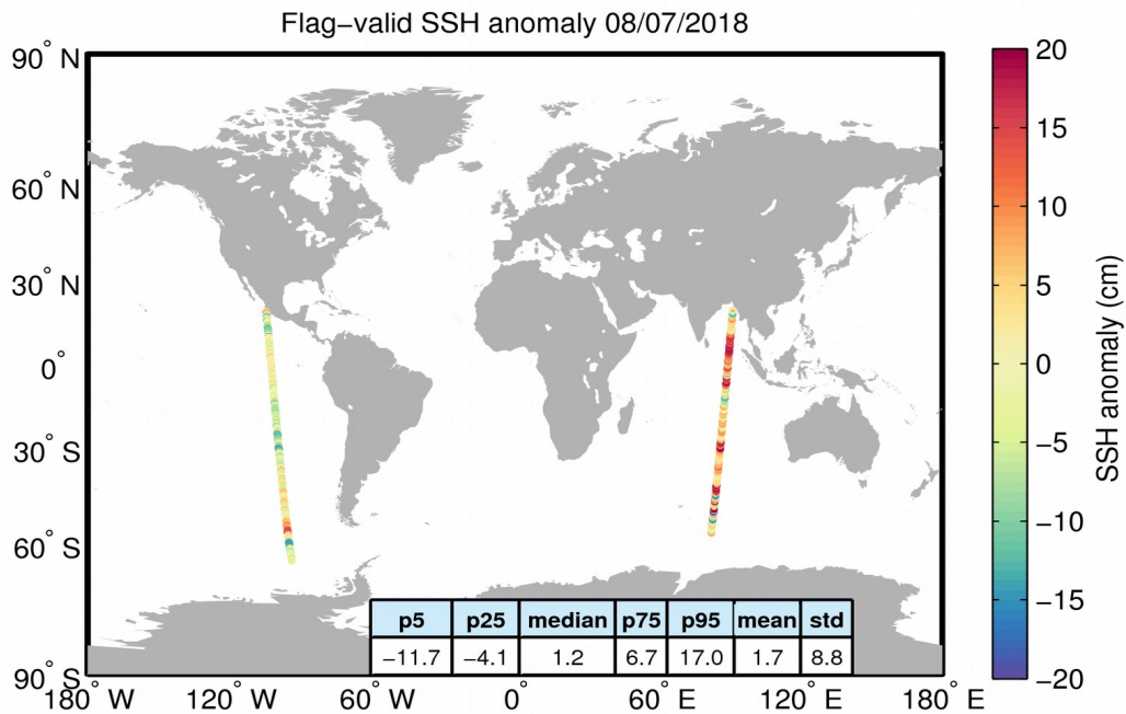
Figure 5. Geographical distribution of flag-valid 1-Hz SSH anomaly data over oceans and lakes for 08/07/2018. The statistical values shown in the table refer to the SSH anomaly in cm and are calculated over all measurements shown in the figure.
