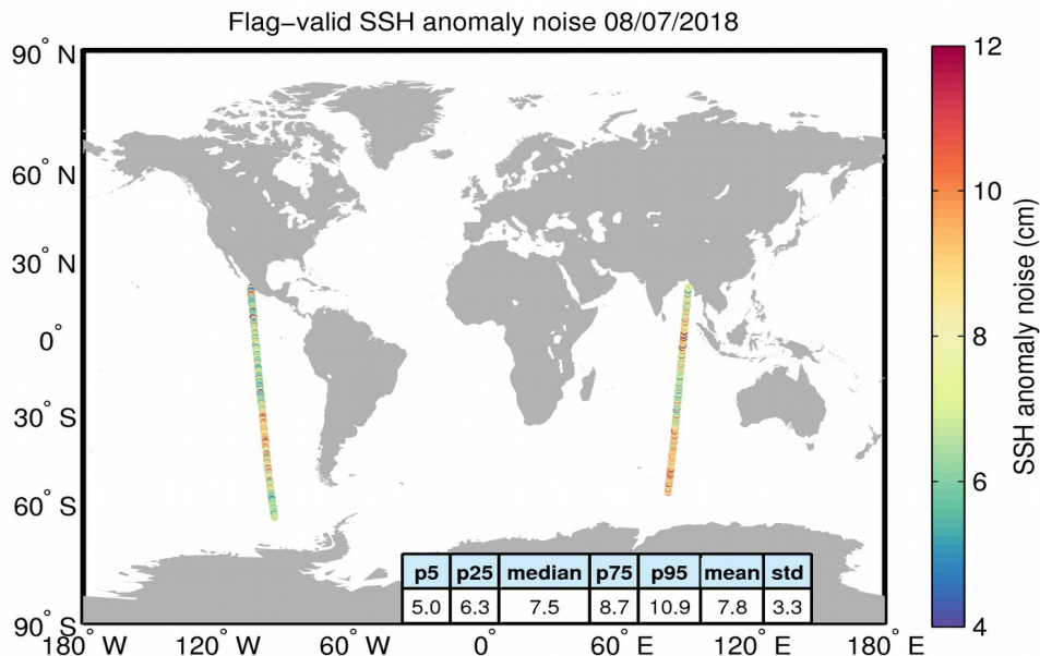
Figure 8. Geographical distribution of flag-valid 20-Hz SSH anomaly measurement noise over oceans and lakes for 08/07/2018. The statistical values shown in the table refer to the SSH anomaly noise and are calculated over all measurements shown in the figure.
