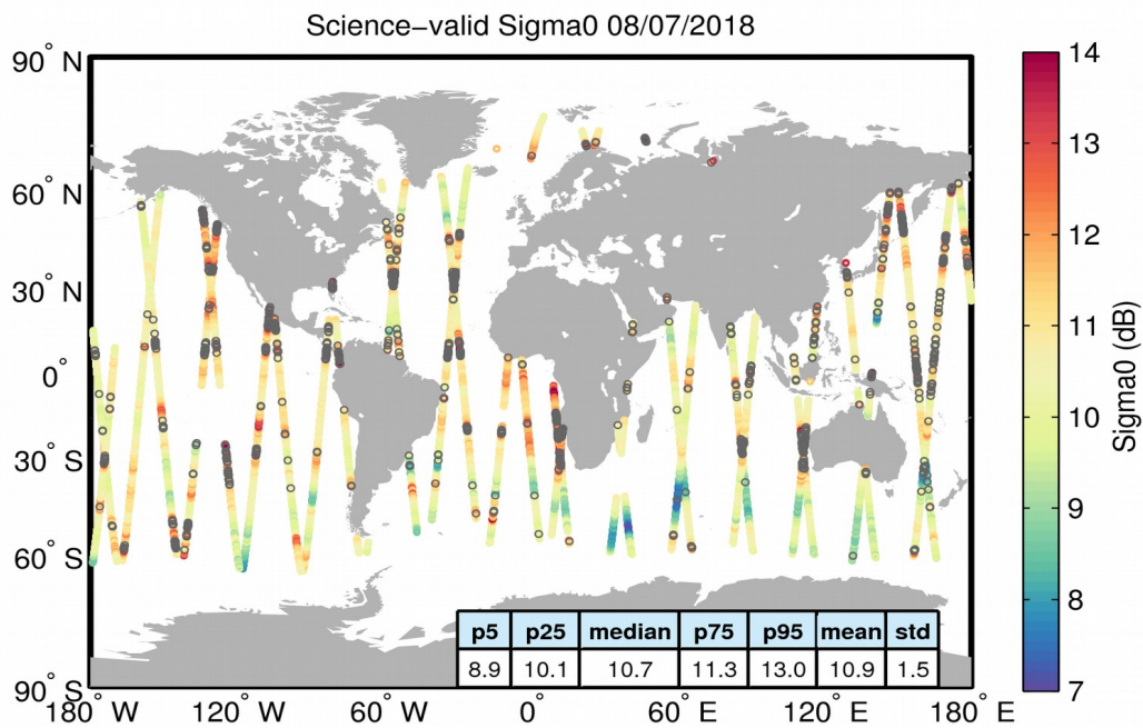
Figure 27. Geographical distribution of science-valid sigma0 data over oceans and lakes for 08/07/2018. The statistical values shown in the table refer to the sigma0 in dB and are calculated over all measurements shown in the figure. Gray circles denote records that have been rejected based on the editing criteria described in Table 4.
