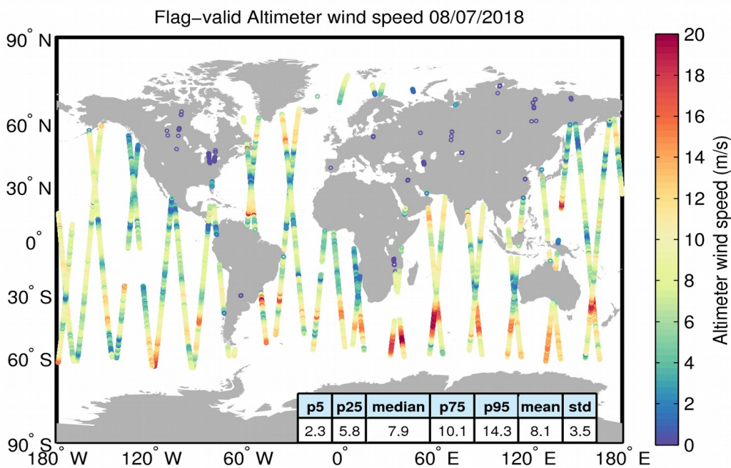
Figure 31. Geographical distribution of flag-valid wind data over oceans and lakes for 08/07/2018. The statistical values shown in the table refer to the wind in m/s and are calculated over all measurements shown in the figure.
