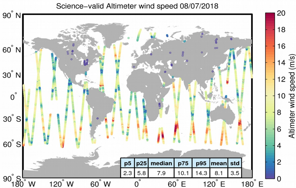
Figure 34. Geographical distribution of science-valid wind data over oceans and lakes for 08/07/2018. The statistical values shown in the table refer to the wind in m/s and are calculated over all measurements shown in the figure. Gray circles denote records that have been rejected based on the editing criteria described in Table 5.
