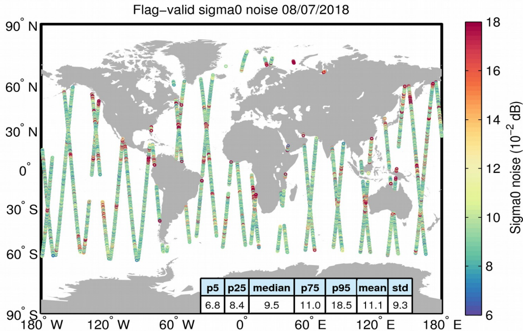
Figure 26. Geographical distribution of flag-valid 20-Hz sigma0 measurement noise over oceans and lakes for 08/07/2018. The statistical values shown in the table refer to the sigma0 noise and are calculated over all measurements shown in the figure.
