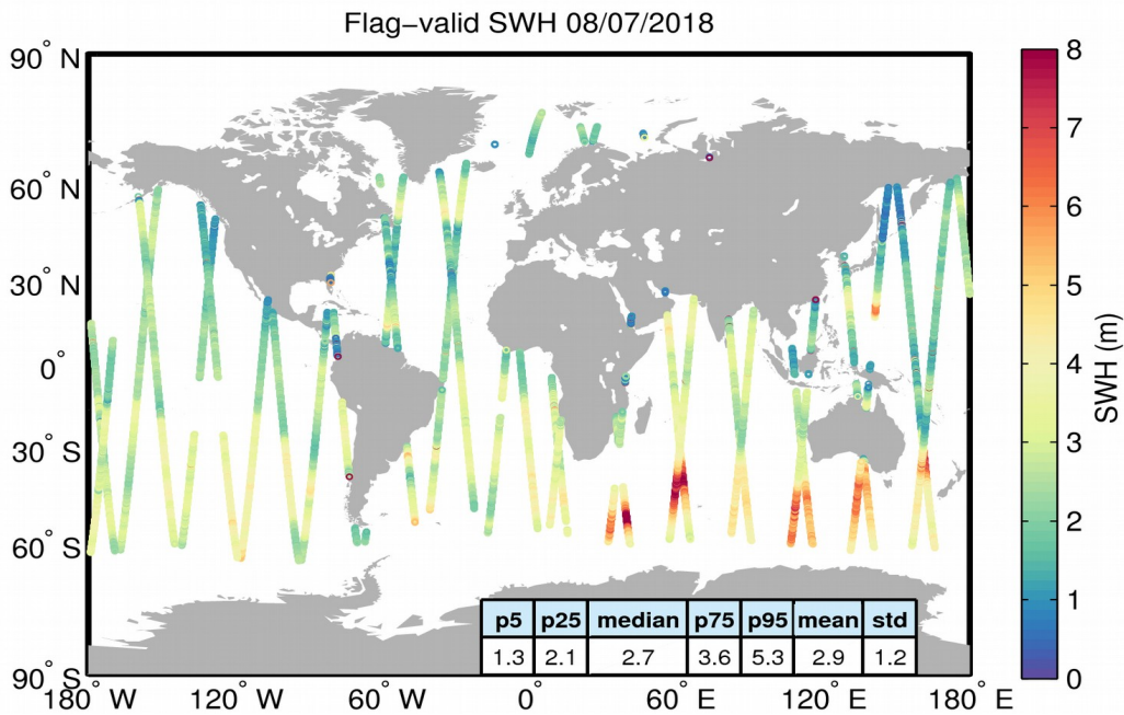
Figure 15. Geographical distribution of flag-valid SWH data over oceans and lakes for 08/07/2018. The statistical values shown in the table refer to the SWH in m and are calculated over all measurements shown in the figure.
