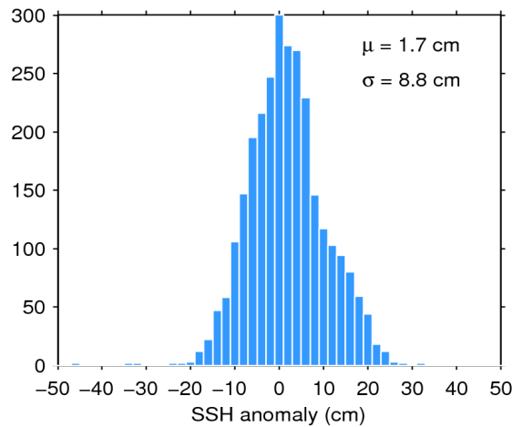
Figure 7. Histogram of flag-valid SSH anomaly over oceans and lakes for 08/07/2018. The mean ( \mu ) and standard deviation ( \sigma ) are also shown. Note that values outside [-50 50] cm are excluded from the histogram for the sake of readability but not from the computation of \mu and \sigma .
