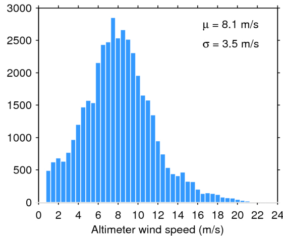
Figure 33. Histogram of flag-valid wind over oceans and lakes for 08/07/2018. The mean ( \mu ) and standard deviation ( \sigma ) are also shown. Note that values larger than 24 m/s are excluded from the histogram for the sake of readability but not from the computation of \mu and \sigma .
