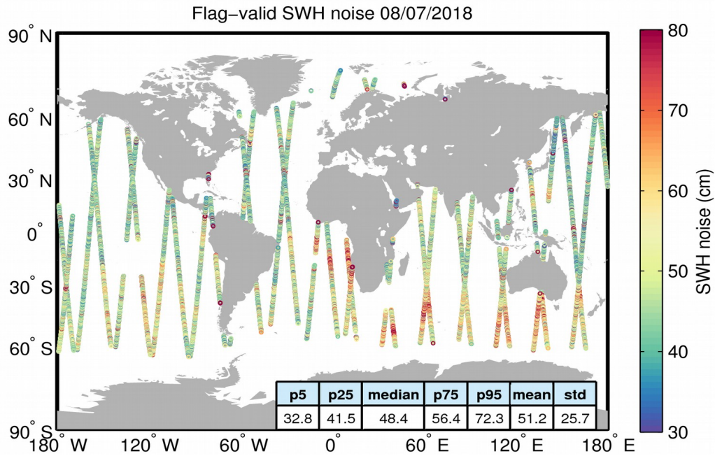
Figure 18. Geographical distribution of flag-valid 20-Hz SWH measurement noise over oceans and lakes for 08/07/2018. The statistical values shown in the figure refer to the SWH noise and are calculated over all measurements shown in the figure.
