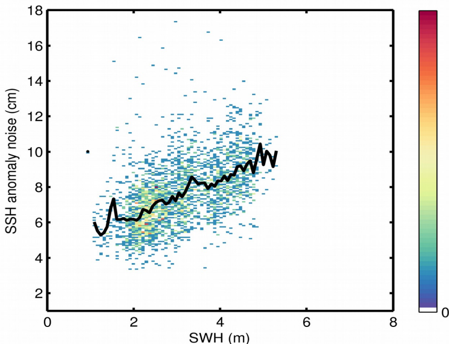
Figure 9. 2D histogram showing flag-valid SSH anomaly noise as a function of SWH for 08/07/2018. The black line denotes the median SSH anomaly noise as a function of SWH.
