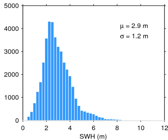
Figure 20. Histogram of science-valid SWH over oceans and lakes for 08/07/2018. The mean ( \mu ) and standard deviation ( \sigma ) are also shown. Note that values larger than 12 m are excluded from the histogram for the sake of readability but not from the computation of \mu and \sigma .
