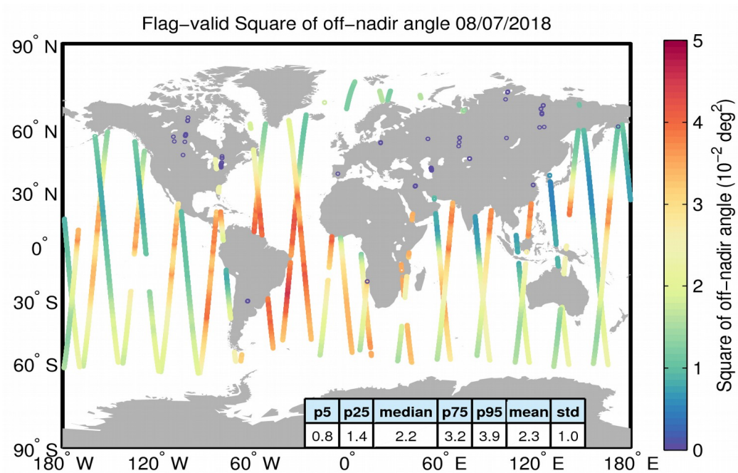
Figure 37. Geographical distribution of flag-valid mispointing data over oceans and lakes for 08/07/2018. The statistical values shown in the table refer to the mispointing in 10^{-2} \text{ deg}^2 and are calculated over all measurements shown in the figure.
