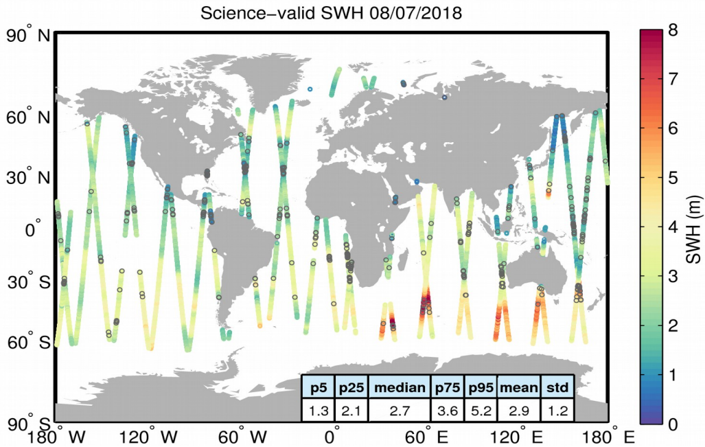
Figure 19. Geographical distribution of science-valid SWH data over oceans and lakes for 08/07/2018. The statistical values shown in the table refer to the SWH in m and are calculated over all measurements shown in the figure. Gray circles denote records that have been rejected based on the editing criteria described in Table 3.
