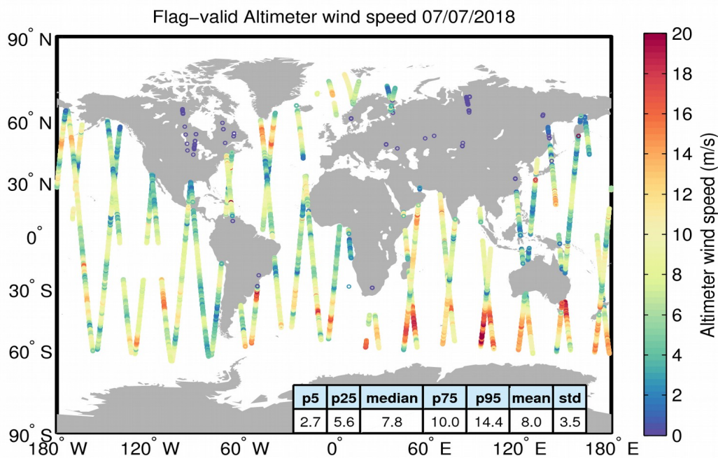
Figure 31. Geographical distribution of flag-valid wind data over oceans and lakes for 07/07/2018. The statistical values shown in the table refer to the wind in m/s and are calculated over all measurements shown in the figure.
