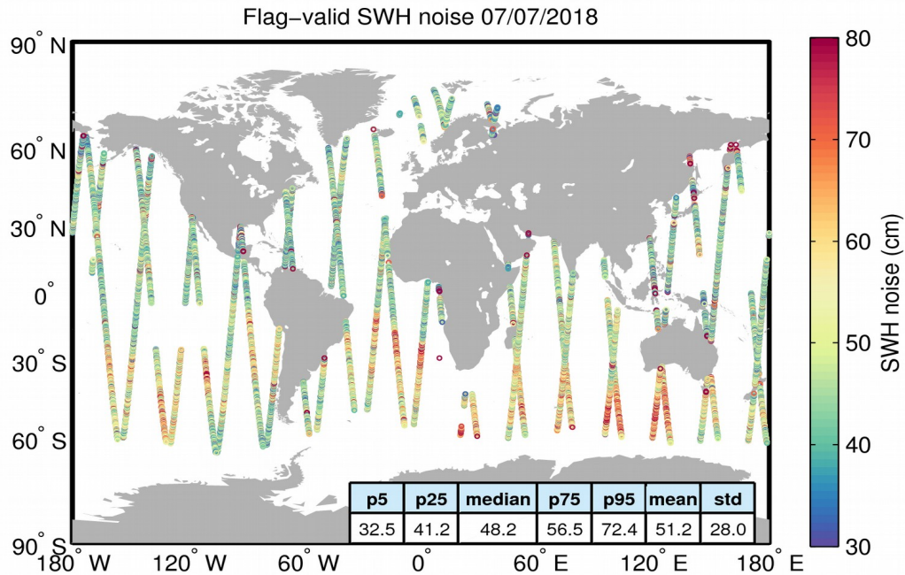
Figure 18. Geographical distribution of flag-valid 20-Hz SWH measurement noise over oceans and lakes for 07/07/2018. The statistical values shown in the figure refer to the SWH noise and are calculated over all measurements shown in the figure.
