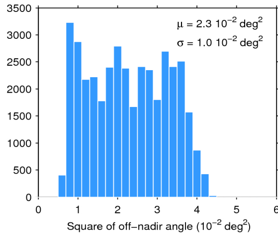
Figure 39. Histogram of flag-valid mispointing over oceans and lakes for 07/07/2018. The mean ( \mu ) and standard deviation ( \sigma ) are also shown. Note that values larger than 6 \cdot 10^{-2} \text{ deg}^2 are excluded from the histogram for the sake of readability but not from the computation of \mu and \sigma .
