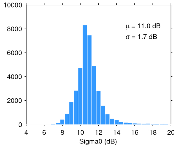
Figure 25. Histogram of flag-valid sigma0 over oceans and lakes for 07/07/2018. The mean ( \mu ) and standard deviation ( \sigma ) are also shown. Note that values outside [4 20] dB are excluded from the histogram for the sake of readability but not from the computation of \mu and \sigma .
