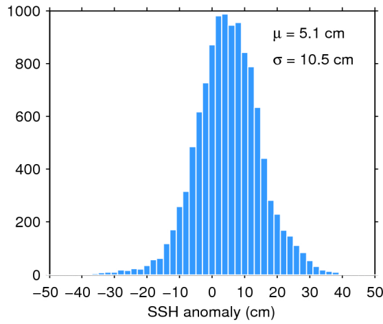
Figure 11. Histogram of science-valid SSH anomaly over oceans and lakes for 07/07/2018. The mean ( \mu ) and standard deviation ( \sigma ) are also shown. Note that values outside [-50 50] cm are excluded from the histogram for the sake of readability but not from the computation of \mu and \sigma .
