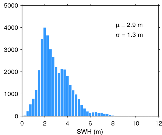
Figure 20. Histogram of science-valid SWH over oceans and lakes for 07/07/2018. The mean ( \mu ) and standard deviation ( \sigma ) are also shown. Note that values larger than 12 m are excluded from the histogram for the sake of readability but not from the computation of \mu and \sigma .
