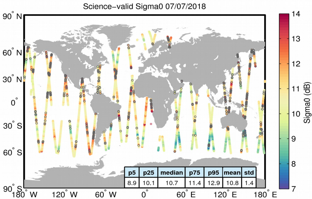
Figure 27. Geographical distribution of science-valid sigma0 data over oceans and lakes for 07/07/2018. The statistical values shown in the table refer to the sigma0 in dB and are calculated over all measurements shown in the figure. Gray circles denote records that have been rejected based on the editing criteria described in Table 4.
