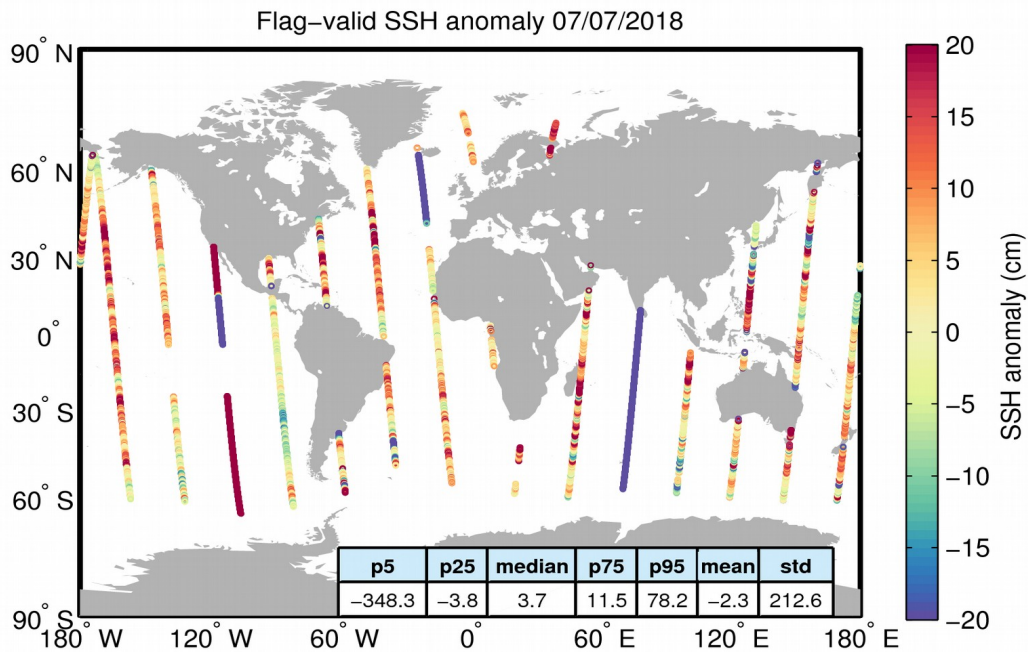
Figure 5. Geographical distribution of flag-valid 1-Hz SSH anomaly data over oceans and lakes for 07/07/2018. The statistical values shown in the table refer to the SSH anomaly in cm and are calculated over all measurements shown in the figure.
