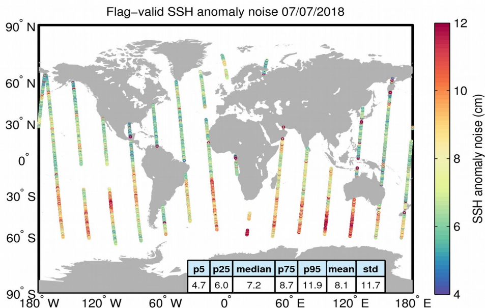
Figure 8. Geographical distribution of flag-valid 20-Hz SSH anomaly measurement noise over oceans and lakes for 07/07/2018. The statistical values shown in the table refer to the SSH anomaly noise and are calculated over all measurements shown in the figure.
