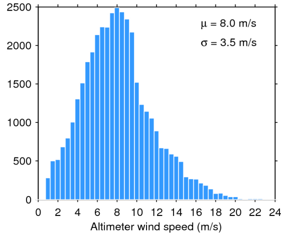
Figure 33. Histogram of flag-valid wind over oceans and lakes for 07/07/2018. The mean ( \mu ) and standard deviation ( \sigma ) are also shown. Note that values larger than 24 m/s are excluded from the histogram for the sake of readability but not from the computation of \mu and \sigma .
