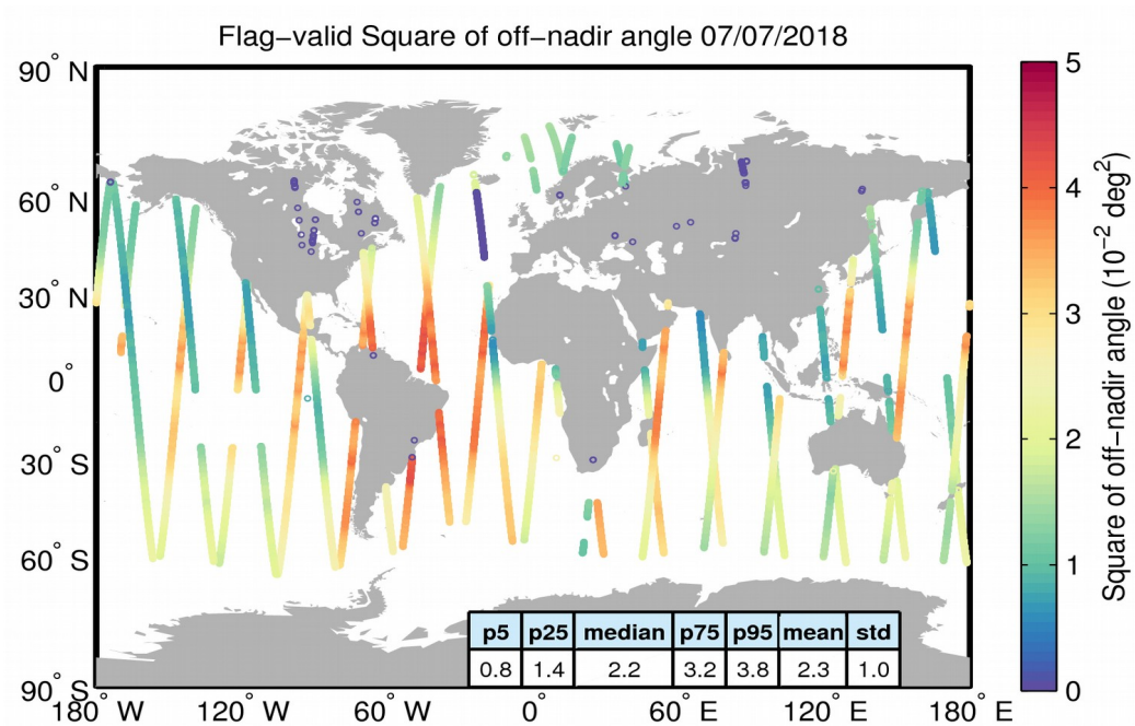
Figure 37. Geographical distribution of flag-valid mispointing data over oceans and lakes for 07/07/2018. The statistical values shown in the table refer to the mispointing in 10^{-2} \text{ deg}^2 and are calculated over all measurements shown in the figure.
