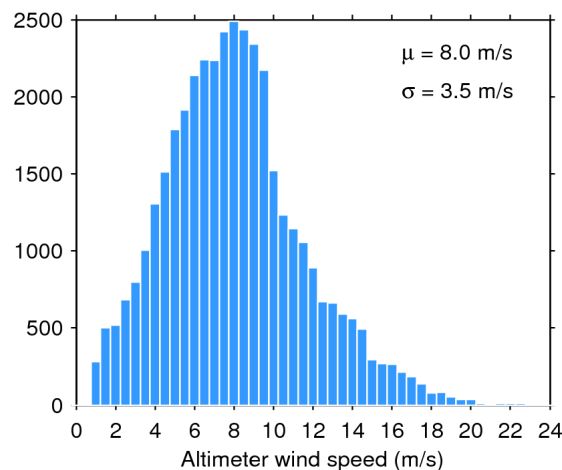
Figure 35. Histogram of science-valid wind over oceans and lakes for 07/07/2018. The mean ( \mu ) and standard deviation ( \sigma ) are also shown. Note that values larger than 24 m/s are excluded from the histogram for the sake of readability but not from the computation of \mu and \sigma .
