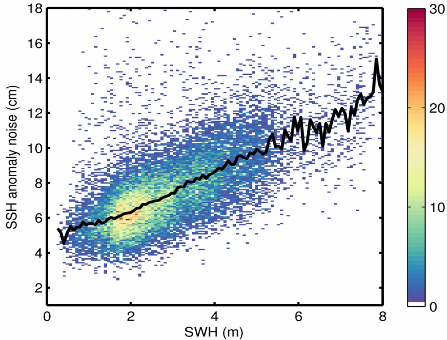
Figure 9. 2D histogram showing flag-valid SSH anomaly noise as a function of SWH for 07/07/2018. The black line denotes the median SSH anomaly noise as a function of SWH.
