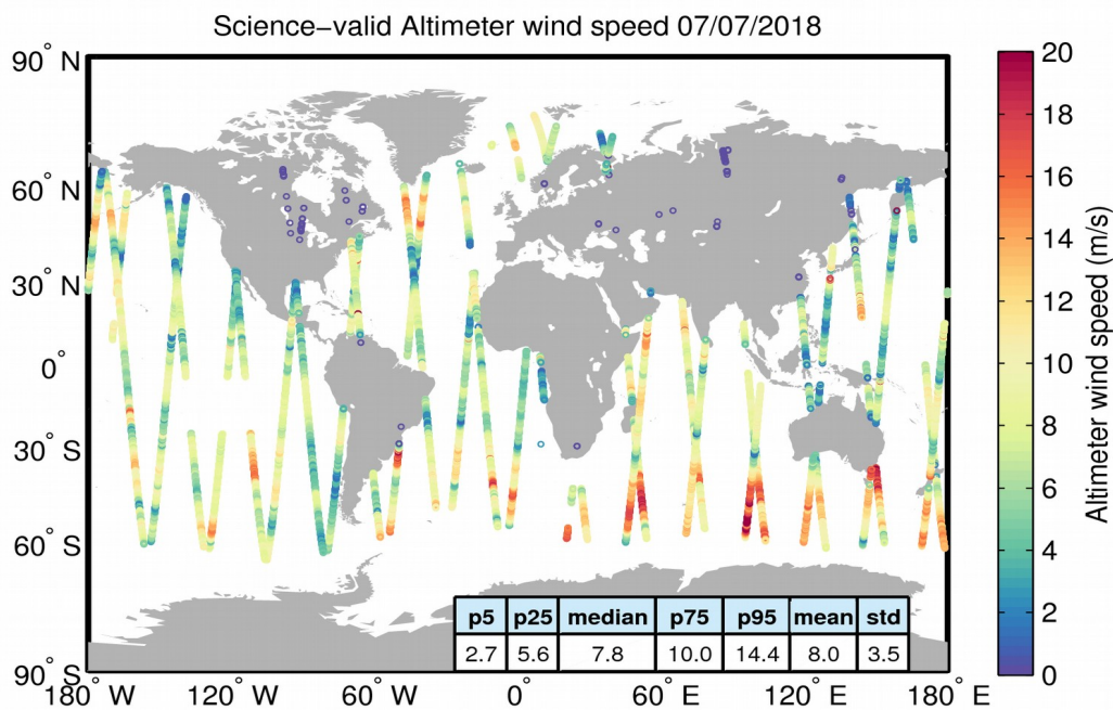
Figure 34. Geographical distribution of science-valid wind data over oceans and lakes for 07/07/2018. The statistical values shown in the table refer to the wind in m/s and are calculated over all measurements shown in the figure. Gray circles denote records that have been rejected based on the editing criteria described in Table 5.
