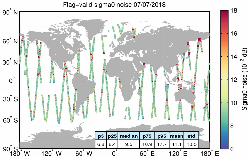
Figure 26. Geographical distribution of flag-valid 20-Hz sigma0 measurement noise over oceans and lakes for 07/07/2018. The statistical values shown in the table refer to the sigma0 noise and are calculated over all measurements shown in the figure.
