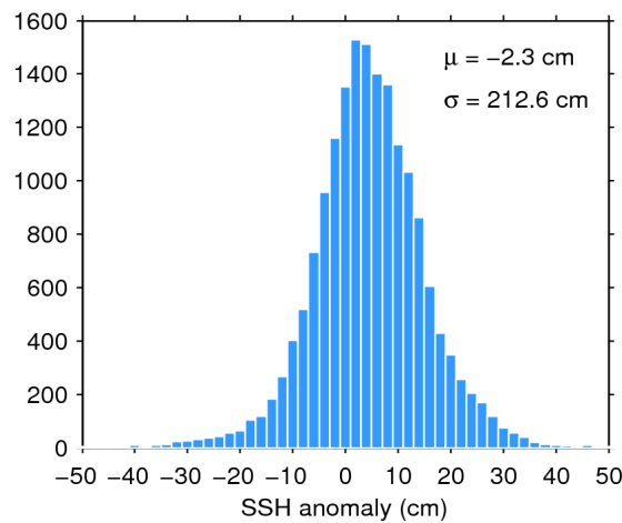
Figure 7. Histogram of flag-valid SSH anomaly over oceans and lakes for 07/07/2018. The mean ( \mu ) and standard deviation ( \sigma ) are also shown. Note that values outside [-50\ 50] cm are excluded from the histogram for the sake of readability but not from the computation of \mu and \sigma .
