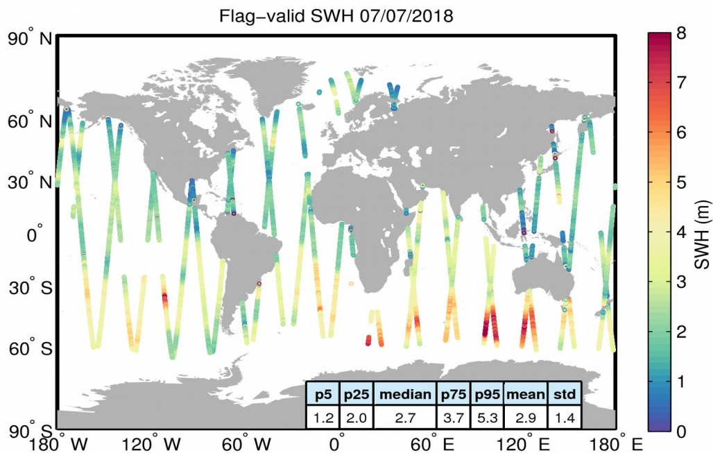
Figure 15. Geographical distribution of flag-valid SWH data over oceans and lakes for 07/07/2018. The statistical values shown in the table refer to the SWH in m and are calculated over all measurements shown in the figure.
