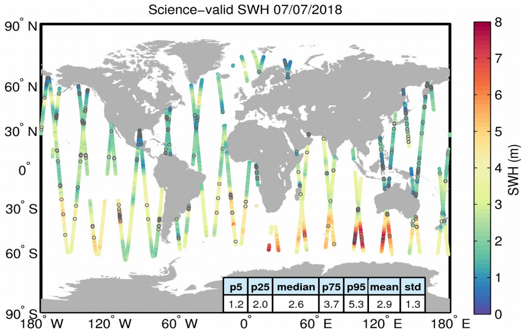
Figure 19. Geographical distribution of science-valid SWH data over oceans and lakes for 07/07/2018. The statistical values shown in the table refer to the SWH in m and are calculated over all measurements shown in the figure. Gray circles denote records that have been rejected based on the editing criteria described in Table 3.
