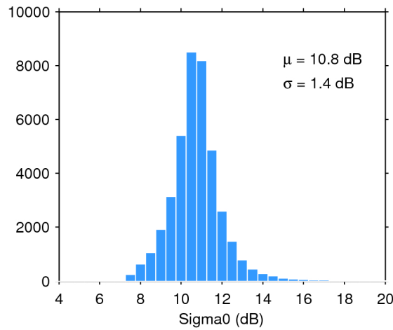
Figure 28. Histogram of science-valid sigma0 over oceans and lakes for 06/07/2018. The mean ( \mu ) and standard deviation ( \sigma ) are also shown. Note that values outside [4 20] dB are excluded from the histogram for the sake of readability but not from the computation of \mu and \sigma .
