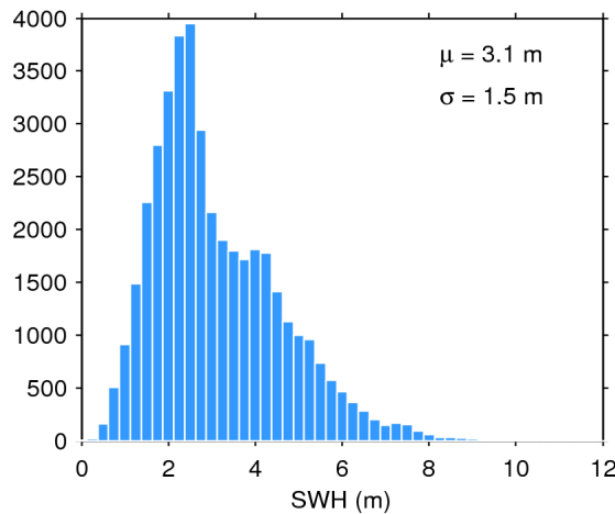
Figure 20. Histogram of science-valid SWH over oceans and lakes for 06/07/2018. The mean ( \mu ) and standard deviation ( \sigma ) are also shown. Note that values larger than 12 m are excluded from the histogram for the sake of readability but not from the computation of \mu and \sigma .
