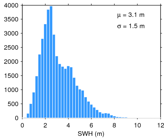
Figure 17. Histogram of flag-valid SWH over oceans and lakes for 06/07/2018. The mean ( \mu ) and standard deviation ( \sigma ) are also shown. Note that values larger than 12 m are excluded from the histogram for the sake of readability but not from the computation of \mu and \sigma .
