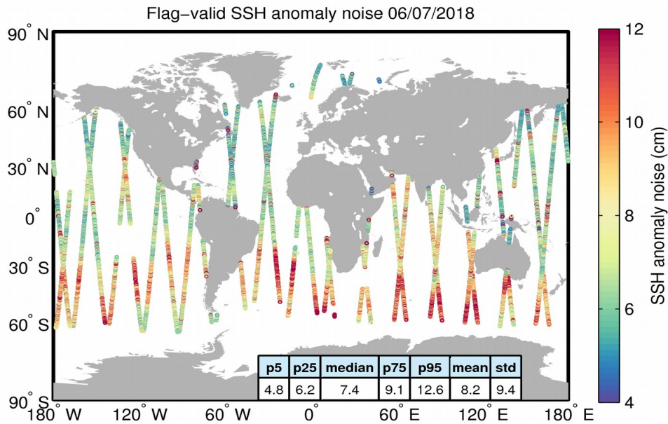
Figure 8. Geographical distribution of flag-valid 20-Hz SSH anomaly measurement noise over oceans and lakes for 06/07/2018. The statistical values shown in the table refer to the SSH anomaly noise and are calculated over all measurements shown in the figure.
