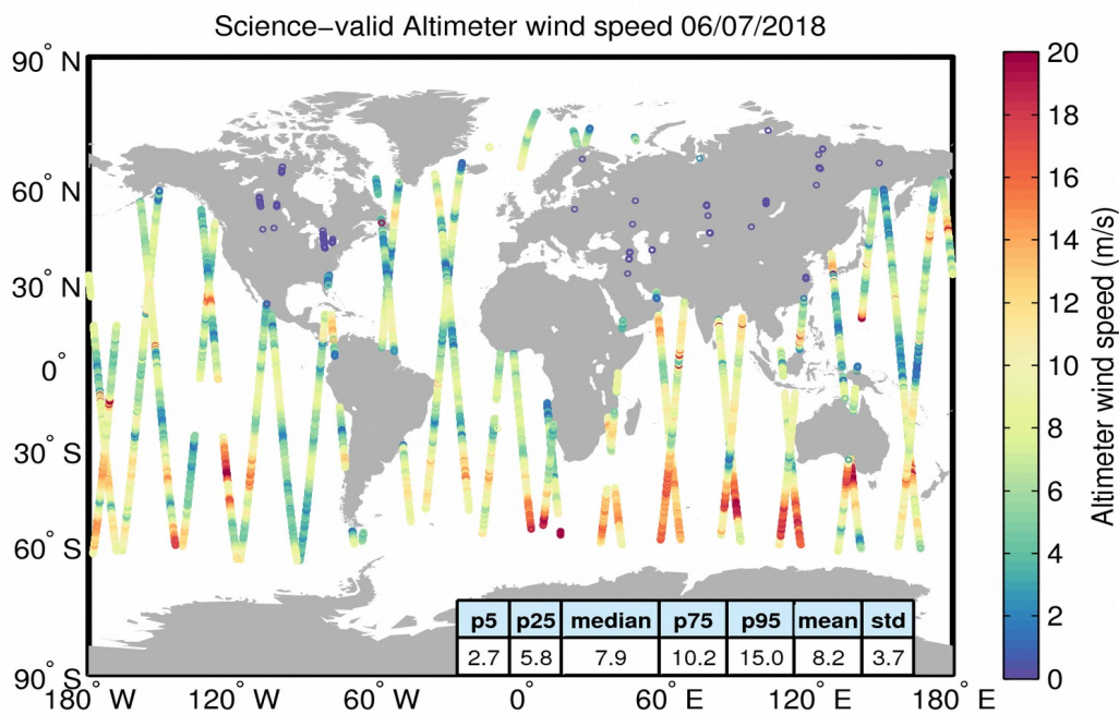
Figure 34. Geographical distribution of science-valid wind data over oceans and lakes for 06/07/2018. The statistical values shown in the table refer to the wind in m/s and are calculated over all measurements shown in the figure. Gray circles denote records that have been rejected based on the editing criteria described in Table 5.
