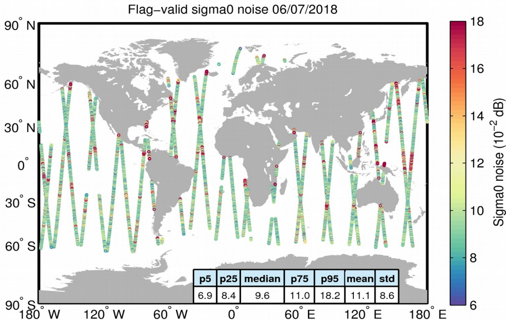
Figure 26. Geographical distribution of flag-valid 20-Hz sigma0 measurement noise over oceans and lakes for 06/07/2018. The statistical values shown in the table refer to the sigma0 noise and are calculated over all measurements shown in the figure.
