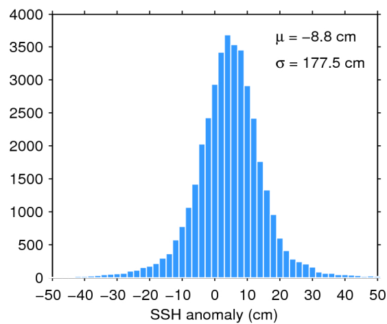
Figure 7. Histogram of flag-valid SSH anomaly over oceans and lakes for 06/07/2018. The mean ( \mu ) and standard deviation ( \sigma ) are also shown. Note that values outside [-50 50] cm are excluded from the histogram for the sake of readability but not from the computation of \mu and \sigma .
