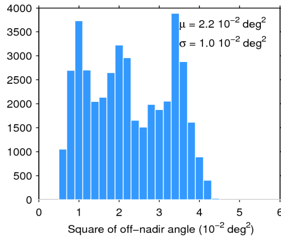
Figure 39. Histogram of flag-valid mispointing over oceans and lakes for 06/07/2018. The mean ( \mu ) and standard deviation ( \sigma ) are also shown. Note that values larger than 6 \cdot 10^{-2} \text{ deg}^2 are excluded from the histogram for the sake of readability but not from the computation of \mu and \sigma .
