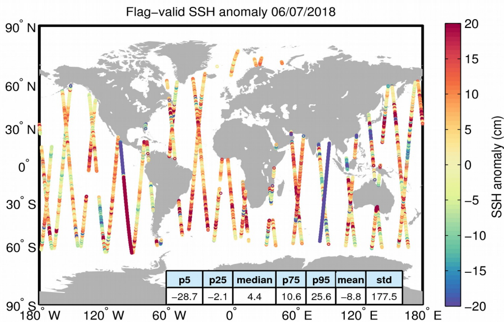
Figure 5. Geographical distribution of flag-valid 1-Hz SSH anomaly data over oceans and lakes for 06/07/2018. The statistical values shown in the table refer to the SSH anomaly in cm and are calculated over all measurements shown in the figure.
