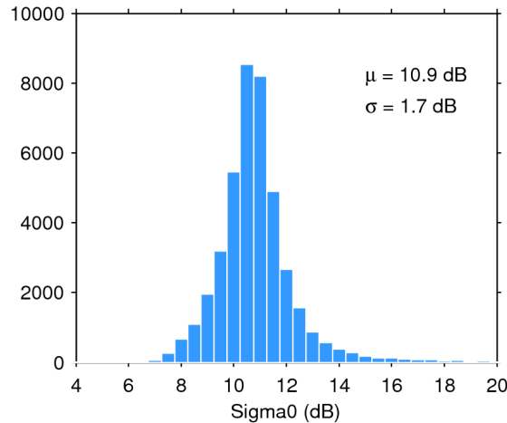
Figure 25. Histogram of flag-valid sigma0 over oceans and lakes for 06/07/2018. The mean ( \mu ) and standard deviation ( \sigma ) are also shown. Note that values outside [4 20] dB are excluded from the histogram for the sake of readability but not from the computation of \mu and \sigma .
