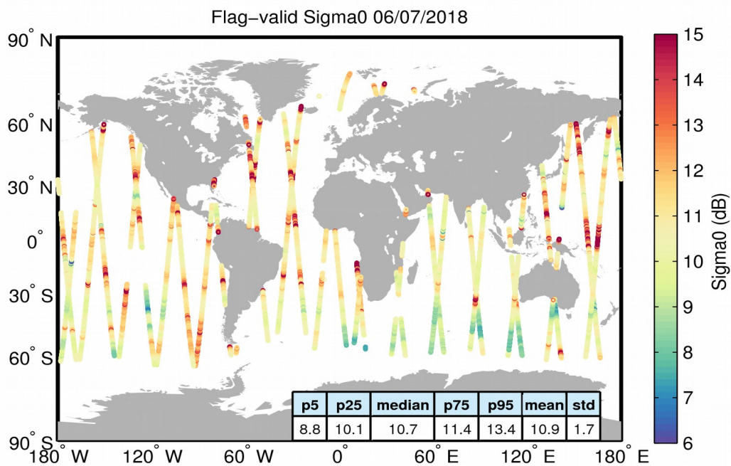
Figure 23. Geographical distribution of flag-valid sigma0 data over oceans and lakes for 06/07/2018. The statistical values shown in the table refer to the sigma0 in dB and are calculated over all measurements shown in the figure.
