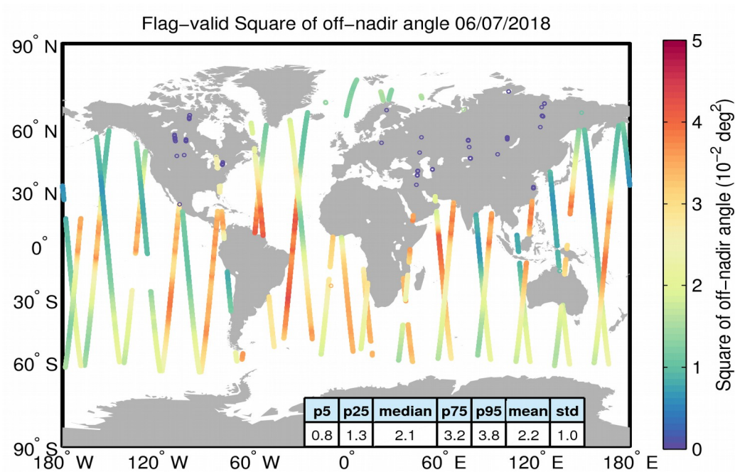
Figure 37. Geographical distribution of flag-valid mispointing data over oceans and lakes for 06/07/2018. The statistical values shown in the table refer to the mispointing in 10^{-2} \text{ deg}^2 and are calculated over all measurements shown in the figure.
