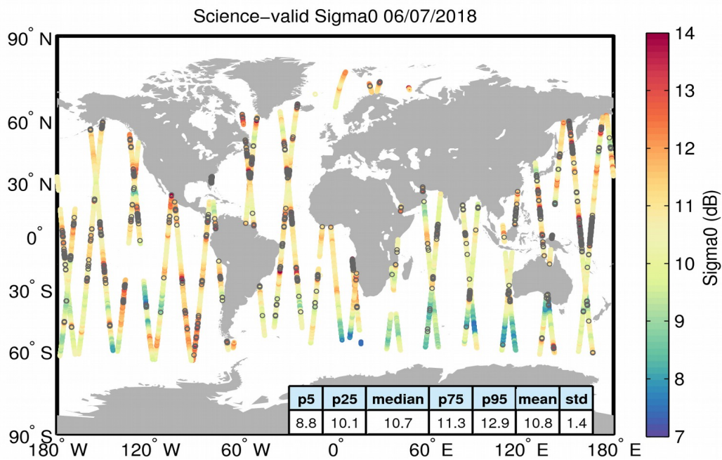
Figure 27. Geographical distribution of science-valid sigma0 data over oceans and lakes for 06/07/2018. The statistical values shown in the table refer to the sigma0 in dB and are calculated over all measurements shown in the figure. Gray circles denote records that have been rejected based on the editing criteria described in Table 4.
