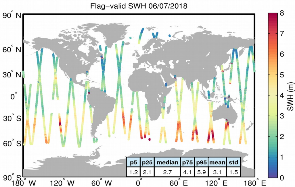
Figure 15. Geographical distribution of flag-valid SWH data over oceans and lakes for 06/07/2018. The statistical values shown in the table refer to the SWH in m and are calculated over all measurements shown in the figure.
