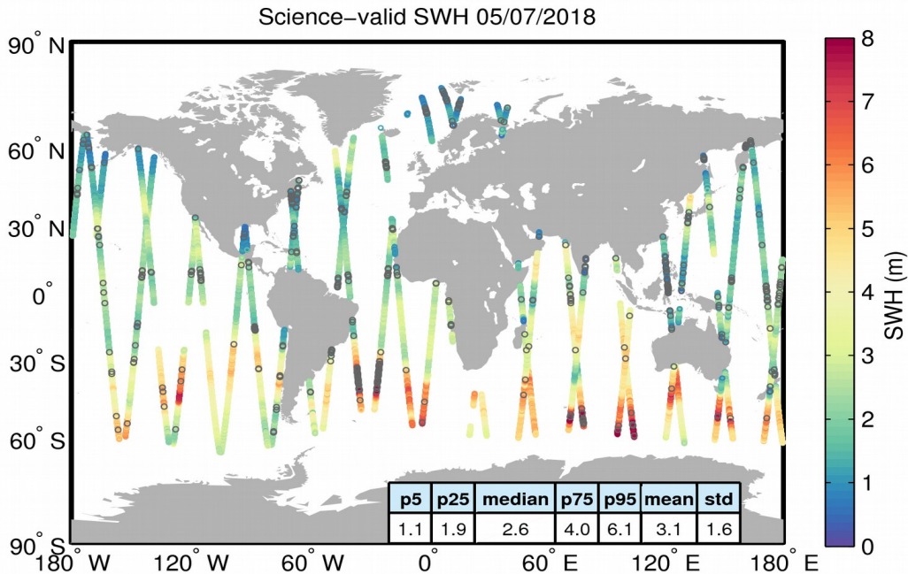
Figure 19. Geographical distribution of science-valid SWH data over oceans and lakes for 05/07/2018. The statistical values shown in the table refer to the SWH in m and are calculated over all measurements shown in the figure. Gray circles denote records that have been rejected based on the editing criteria described in Table 3.
