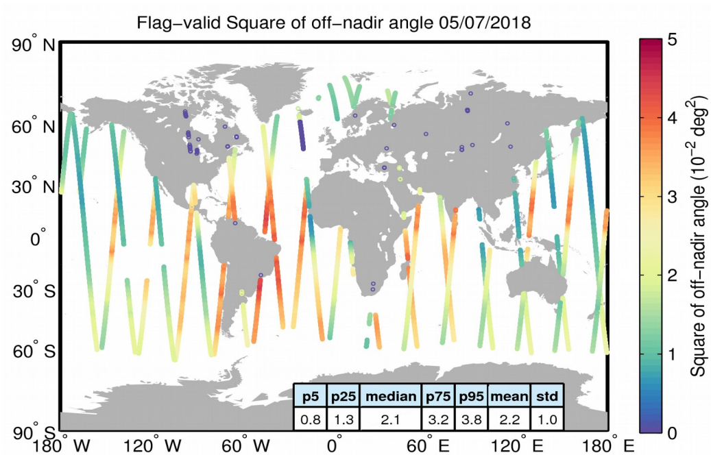
Figure 37. Geographical distribution of flag-valid mispointing data over oceans and lakes for 05/07/2018. The statistical values shown in the table refer to the mispointing in 10^{-2} \text{deg}^2 and are calculated over all measurements shown in the figure.
