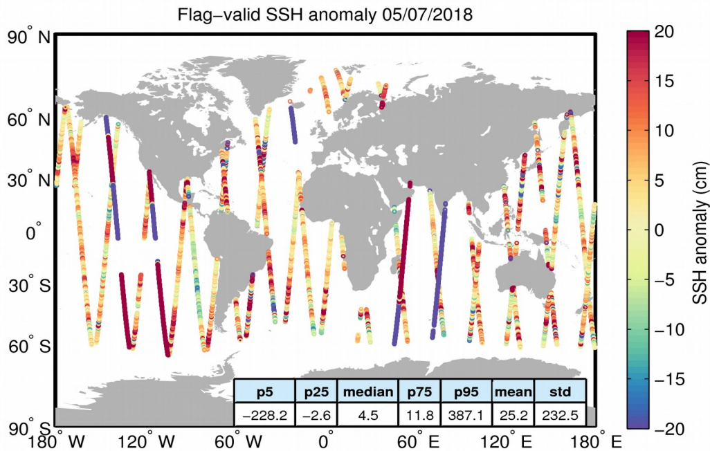
Figure 5. Geographical distribution of flag-valid 1-Hz SSH anomaly data over oceans and lakes for 05/07/2018. The statistical values shown in the table refer to the SSH anomaly in cm and are calculated over all measurements shown in the figure.
