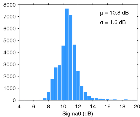
Figure 28. Histogram of science-valid sigma0 over oceans and lakes for 05/07/2018. The mean ( \mu ) and standard deviation ( \sigma ) are also shown. Note that values outside [4 20] dB are excluded from the histogram for the sake of readability but not from the computation of \mu and \sigma .
