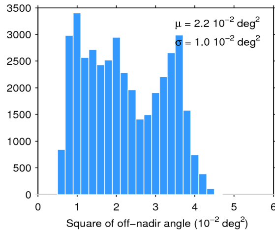
Figure 39. Histogram of flag-valid mispointing over oceans and lakes for 05/07/2018. The mean ( \mu ) and standard deviation ( \sigma ) are also shown. Note that values larger than 6 \cdot 10^{-2} \text{ deg}^2 are excluded from the histogram for the sake of readability but not from the computation of \mu and \sigma .
