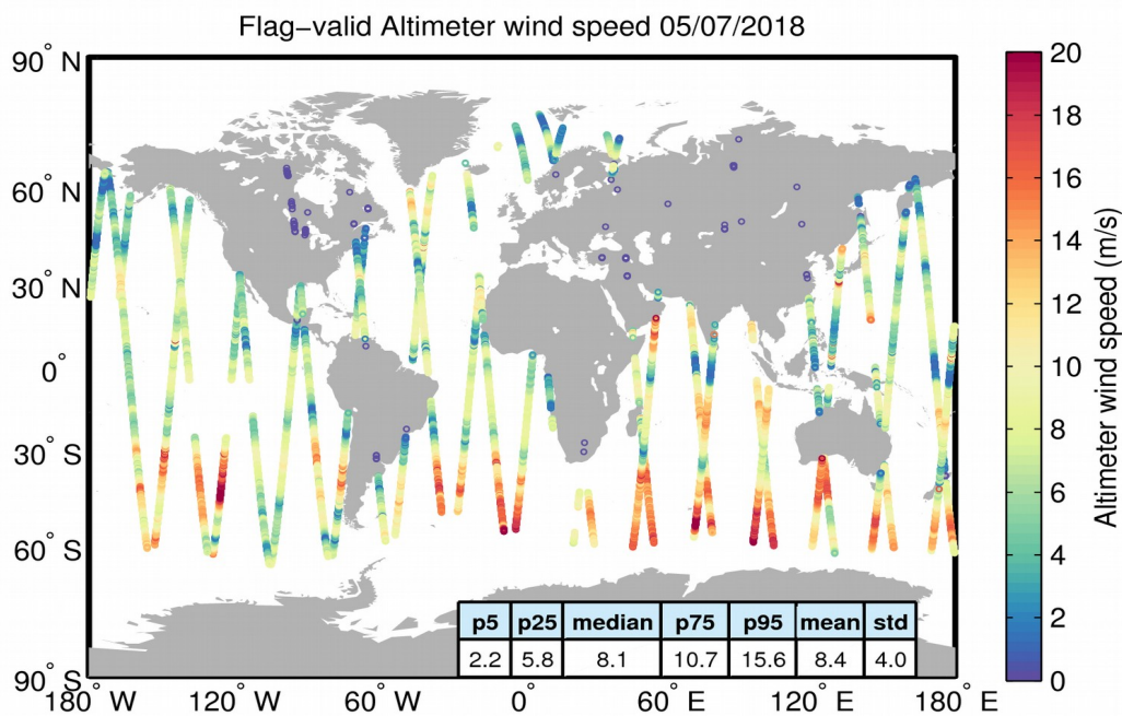
Figure 31. Geographical distribution of flag-valid wind data over oceans and lakes for 05/07/2018. The statistical values shown in the table refer to the wind in m/s and are calculated over all measurements shown in the figure.
