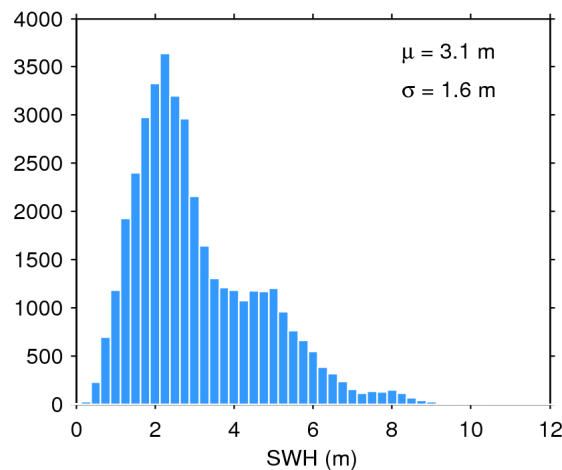
Figure 20. Histogram of science-valid SWH over oceans and lakes for 05/07/2018. The mean ( \mu ) and standard deviation ( \sigma ) are also shown. Note that values larger than 12 m are excluded from the histogram for the sake of readability but not from the computation of \mu and \sigma .
