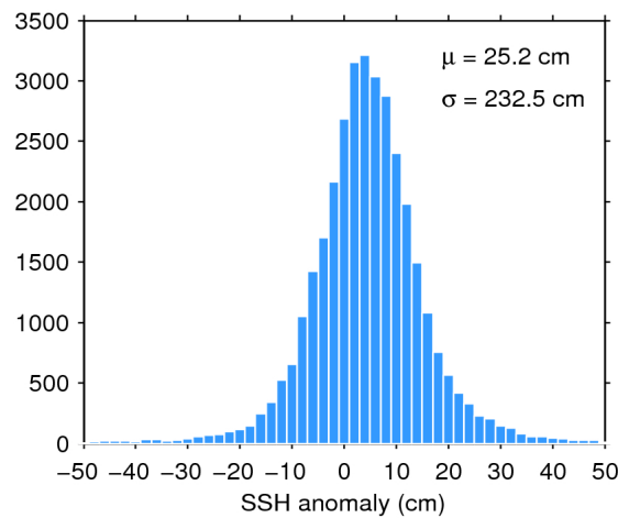
Figure 7. Histogram of flag-valid SSH anomaly over oceans and lakes for 05/07/2018. The mean ( \mu ) and standard deviation ( \sigma ) are also shown. Note that values outside [-50 50] cm are excluded from the histogram for the sake of readability but not from the computation of \mu and \sigma .
