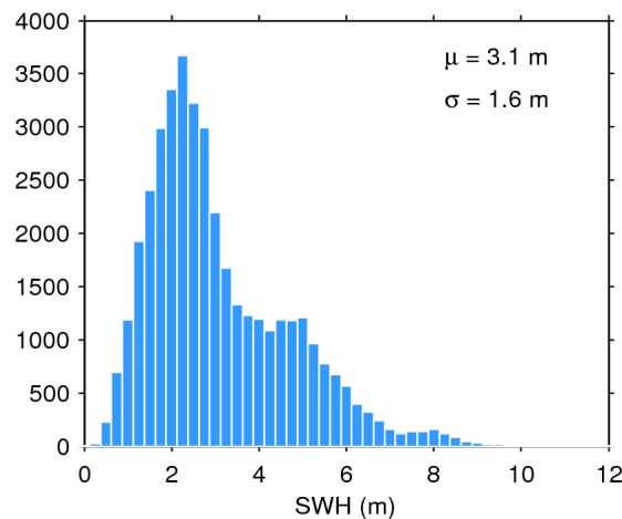
Figure 17. Histogram of flag-valid SWH over oceans and lakes for 05/07/2018. The mean ( \mu ) and standard deviation ( \sigma ) are also shown. Note that values larger than 12 m are excluded from the histogram for the sake of readability but not from the computation of \mu and \sigma .
