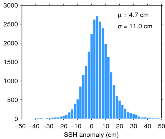
Figure 11. Histogram of science-valid SSH anomaly over oceans and lakes for 05/07/2018. The mean ( \mu ) and standard deviation ( \sigma ) are also shown. Note that values outside [-50 50] cm are excluded from the histogram for the sake of readability but not from the computation of \mu and \sigma .
