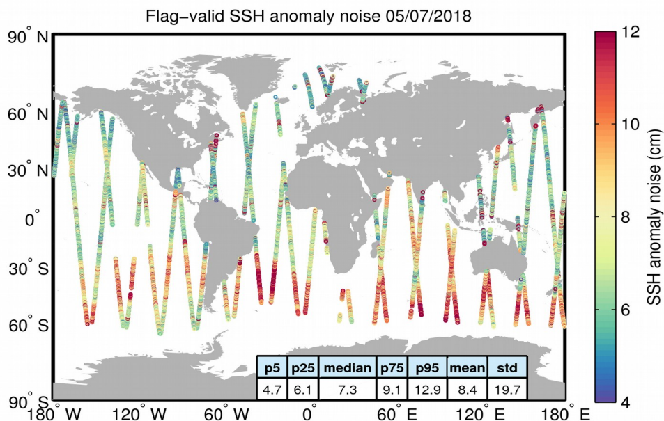
Figure 8. Geographical distribution of flag-valid 20-Hz SSH anomaly measurement noise over oceans and lakes for 05/07/2018. The statistical values shown in the table refer to the SSH anomaly noise and are calculated over all measurements shown in the figure.
