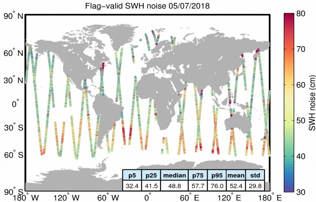
Figure 18. Geographical distribution of flag-valid 20-Hz SWH measurement noise over oceans and lakes for 05/07/2018. The statistical values shown in the figure refer to the SWH noise and are calculated over all measurements shown in the figure.
