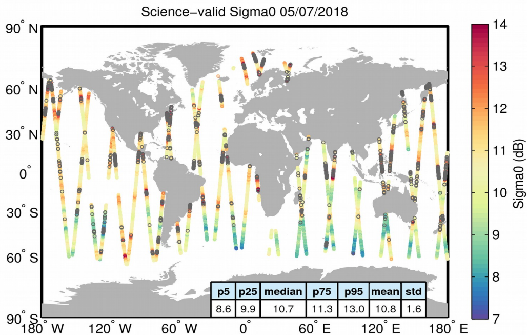
Figure 27. Geographical distribution of science-valid sigma0 data over oceans and lakes for 05/07/2018. The statistical values shown in the table refer to the sigma0 in dB and are calculated over all measurements shown in the figure. Gray circles denote records that have been rejected based on the editing criteria described in Table 4.
