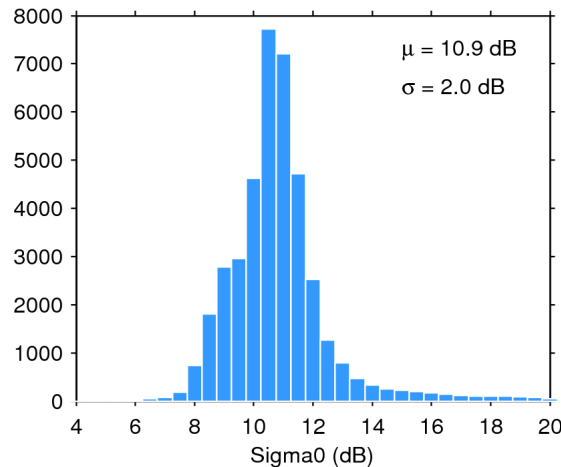
Figure 25. Histogram of flag-valid sigma0 over oceans and lakes for 05/07/2018. The mean ( \mu ) and standard deviation ( \sigma ) are also shown. Note that values outside [4 20] dB are excluded from the histogram for the sake of readability but not from the computation of \mu and \sigma .
