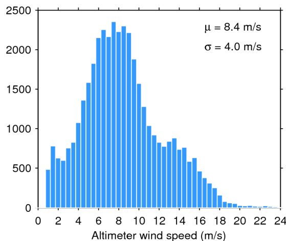
Figure 35. Histogram of science-valid wind over oceans and lakes for 05/07/2018. The mean ( \mu ) and standard deviation ( \sigma ) are also shown. Note that values larger than 24 m/s are excluded from the histogram for the sake of readability but not from the computation of \mu and \sigma .
