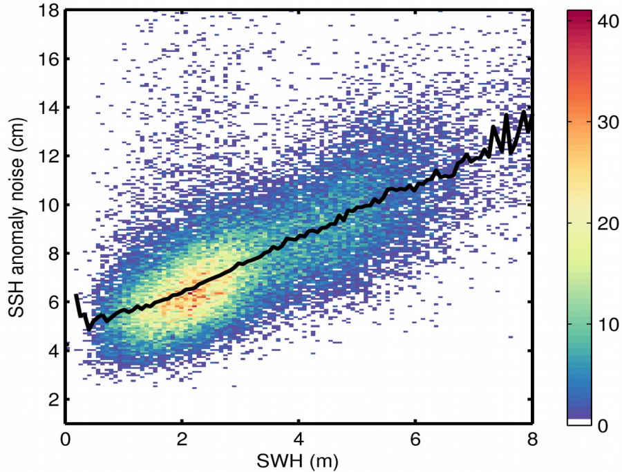
Figure 9. 2D histogram showing flag-valid SSH anomaly noise as a function of SWH for 05/07/2018. The black line denotes the median SSH anomaly noise as a function of SWH.
