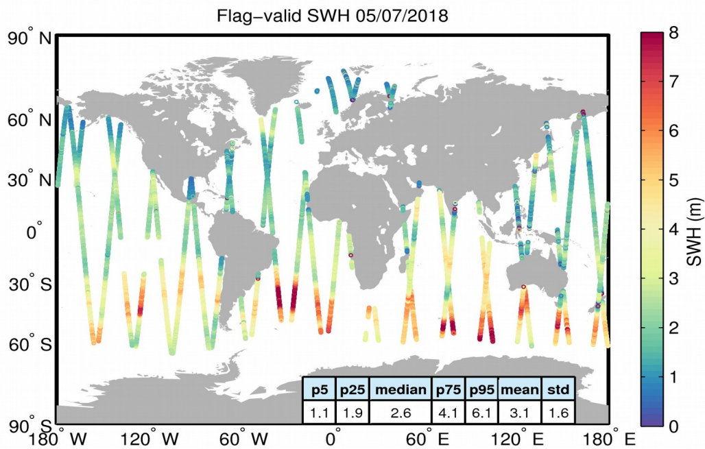
Figure 15. Geographical distribution of flag-valid SWH data over oceans and lakes for 05/07/2018. The statistical values shown in the table refer to the SWH in m and are calculated over all measurements shown in the figure.
