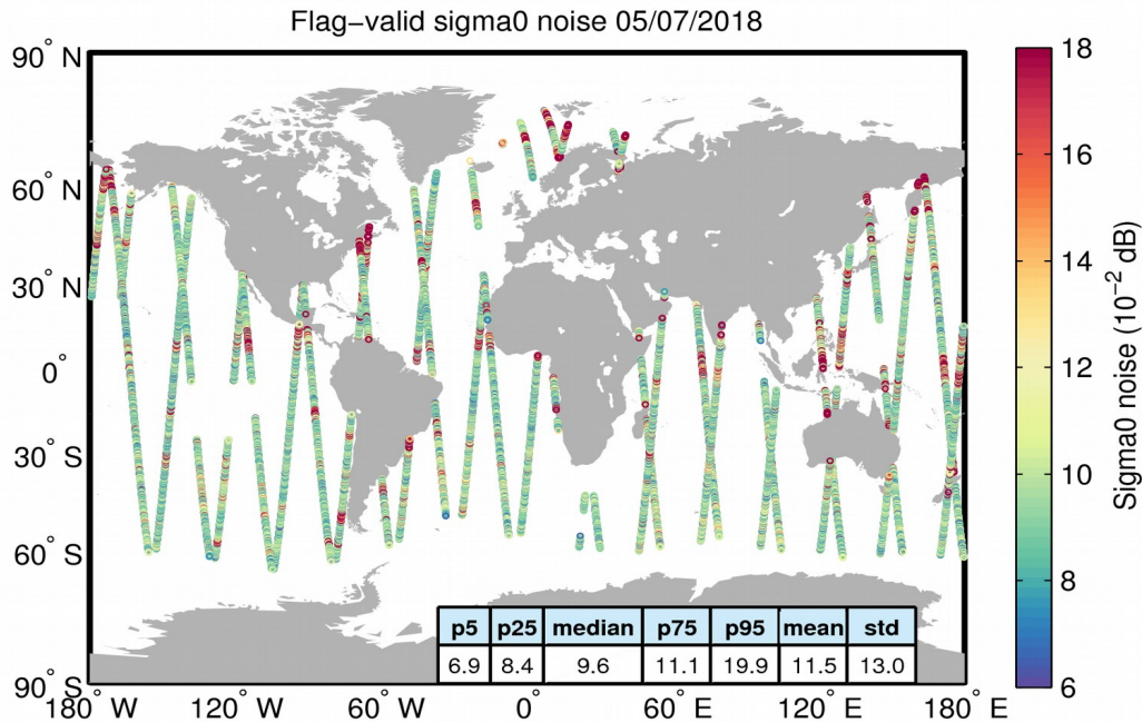
Figure 26. Geographical distribution of flag-valid 20-Hz sigma0 measurement noise over oceans and lakes for 05/07/2018. The statistical values shown in the table refer to the sigma0 noise and are calculated over all measurements shown in the figure.
