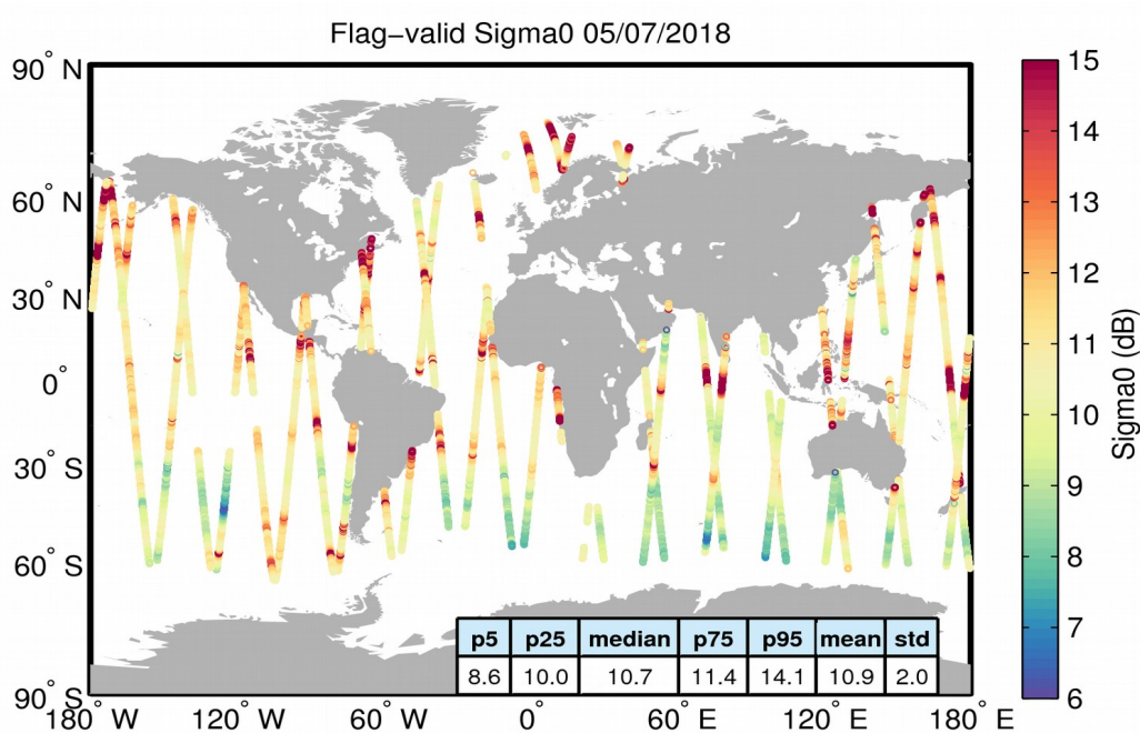
Figure 23. Geographical distribution of flag-valid sigma0 data over oceans and lakes for 05/07/2018. The statistical values shown in the table refer to the sigma0 in dB and are calculated over all measurements shown in the figure.
