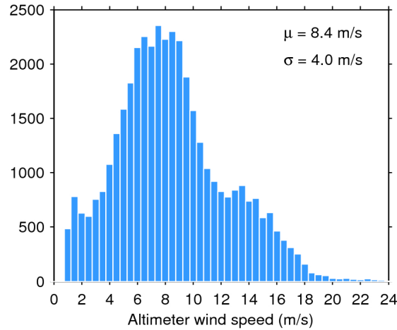
Figure 33. Histogram of flag-valid wind over oceans and lakes for 05/07/2018. The mean ( \mu ) and standard deviation ( \sigma ) are also shown. Note that values larger than 24 m/s are excluded from the histogram for the sake of readability but not from the computation of \mu and \sigma .
