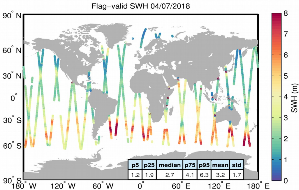
Figure 15. Geographical distribution of flag-valid SWH data over oceans and lakes for 04/07/2018. The statistical values shown in the table refer to the SWH in m and are calculated over all measurements shown in the figure.
