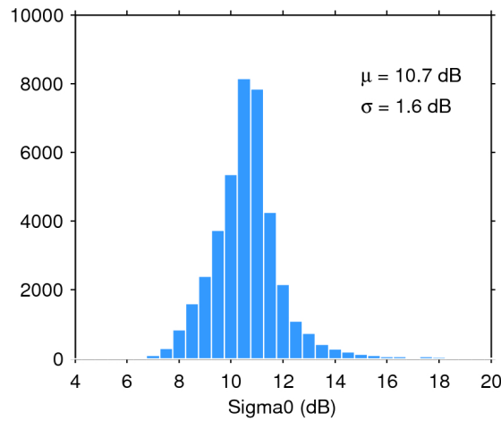
Figure 28. Histogram of science-valid sigma0 over oceans and lakes for 04/07/2018. The mean ( \mu ) and standard deviation ( \sigma ) are also shown. Note that values outside [4 20] dB are excluded from the histogram for the sake of readability but not from the computation of \mu and \sigma .
