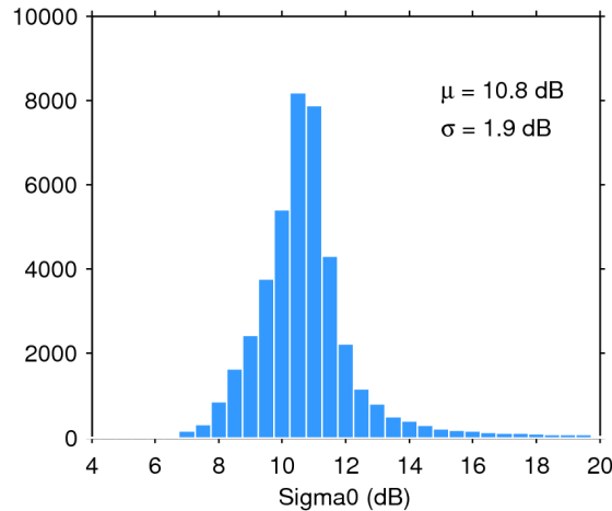
Figure 25. Histogram of flag-valid sigma0 over oceans and lakes for 04/07/2018. The mean ( \mu ) and standard deviation ( \sigma ) are also shown. Note that values outside [4 20] dB are excluded from the histogram for the sake of readability but not from the computation of \mu and \sigma .
