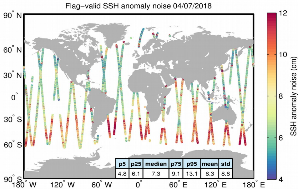
Figure 8. Geographical distribution of flag-valid 20-Hz SSH anomaly measurement noise over oceans and lakes for 04/07/2018. The statistical values shown in the table refer to the SSH anomaly noise and are calculated over all measurements shown in the figure.
