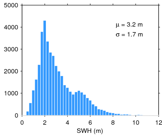
Figure 17. Histogram of flag-valid SWH over oceans and lakes for 04/07/2018. The mean ( \mu ) and standard deviation ( \sigma ) are also shown. Note that values larger than 12 m are excluded from the histogram for the sake of readability but not from the computation of \mu and \sigma .
