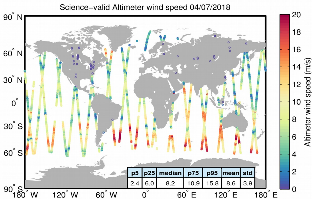
Figure 34. Geographical distribution of science-valid wind data over oceans and lakes for 04/07/2018. The statistical values shown in the table refer to the wind in m/s and are calculated over all measurements shown in the figure. Gray circles denote records that have been rejected based on the editing criteria described in Table 5.
