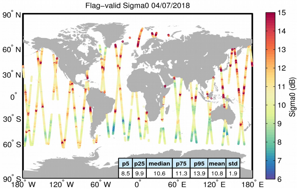
Figure 23. Geographical distribution of flag-valid sigma0 data over oceans and lakes for 04/07/2018. The statistical values shown in the table refer to the sigma0 in dB and are calculated over all measurements shown in the figure.
