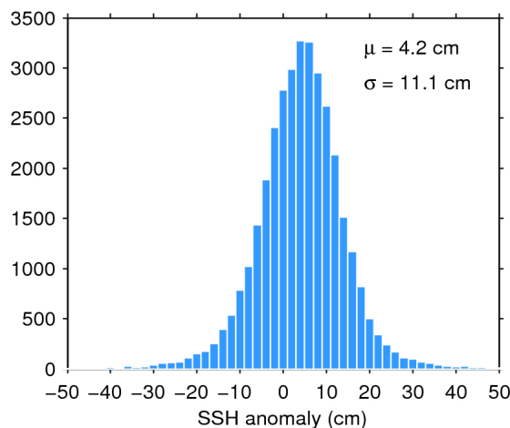
Figure 11. Histogram of science-valid SSH anomaly over oceans and lakes for 04/07/2018. The mean ( \mu ) and standard deviation ( \sigma ) are also shown. Note that values outside [-50 50] cm are excluded from the histogram for the sake of readability but not from the computation of \mu and \sigma .
