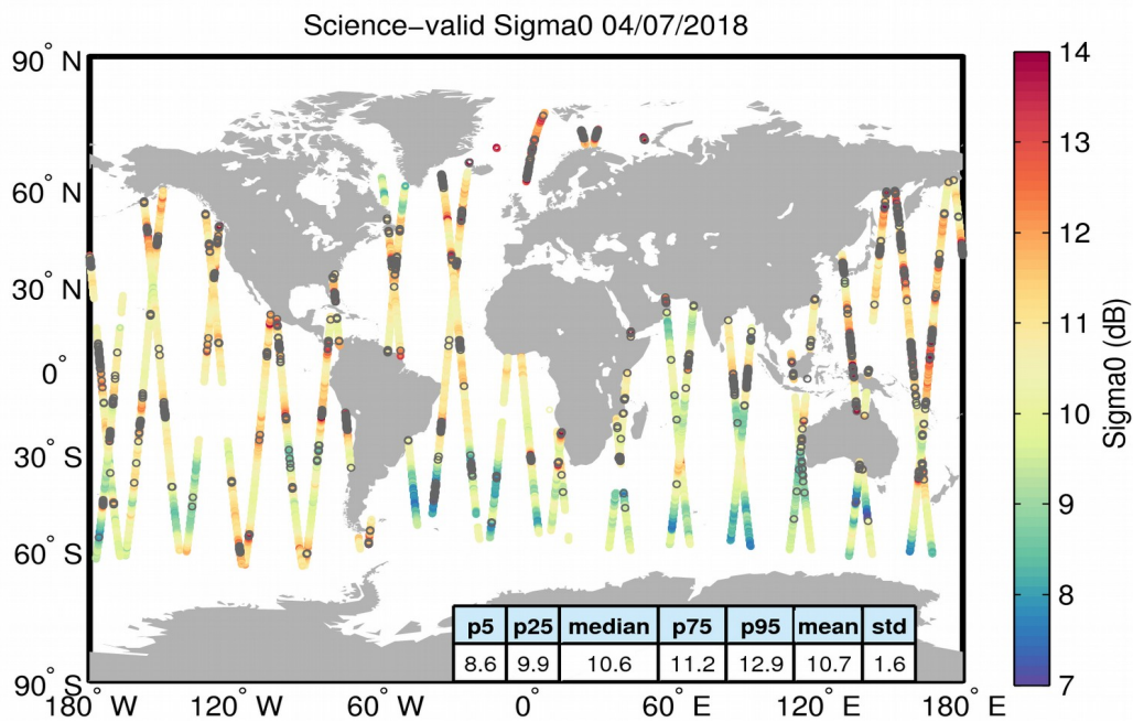
Figure 27. Geographical distribution of science-valid sigma0 data over oceans and lakes for 04/07/2018. The statistical values shown in the table refer to the sigma0 in dB and are calculated over all measurements shown in the figure. Gray circles denote records that have been rejected based on the editing criteria described in Table 4.
