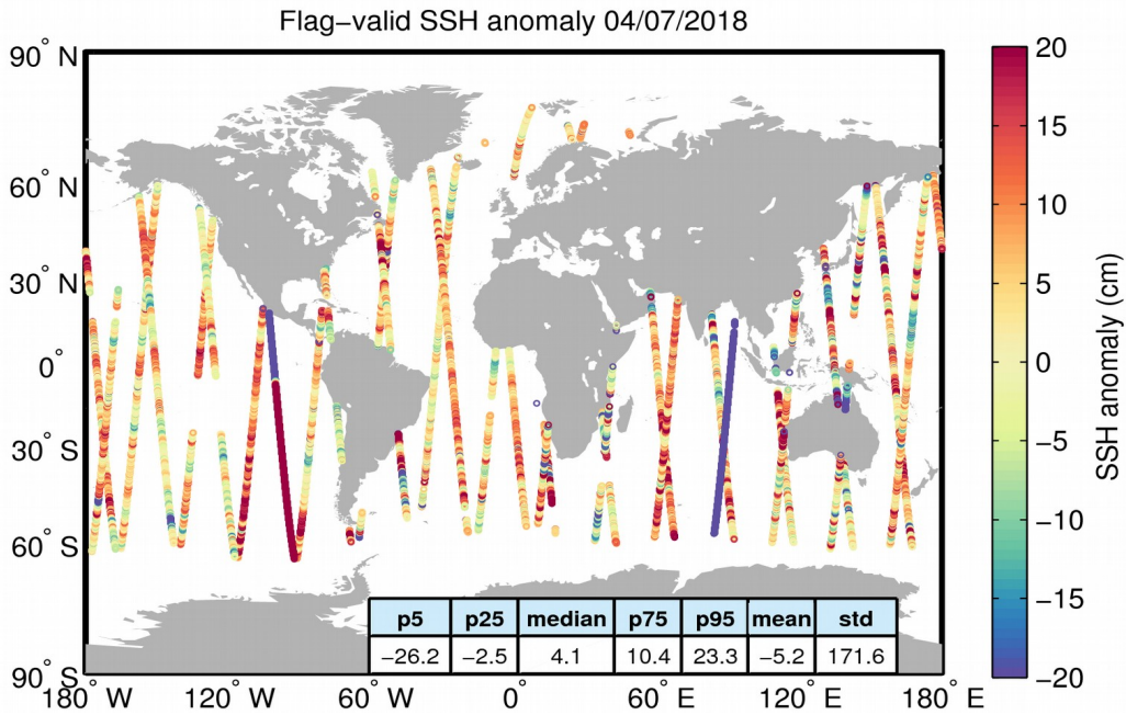
Figure 5. Geographical distribution of flag-valid 1-Hz SSH anomaly data over oceans and lakes for 04/07/2018. The statistical values shown in the table refer to the SSH anomaly in cm and are calculated over all measurements shown in the figure.
