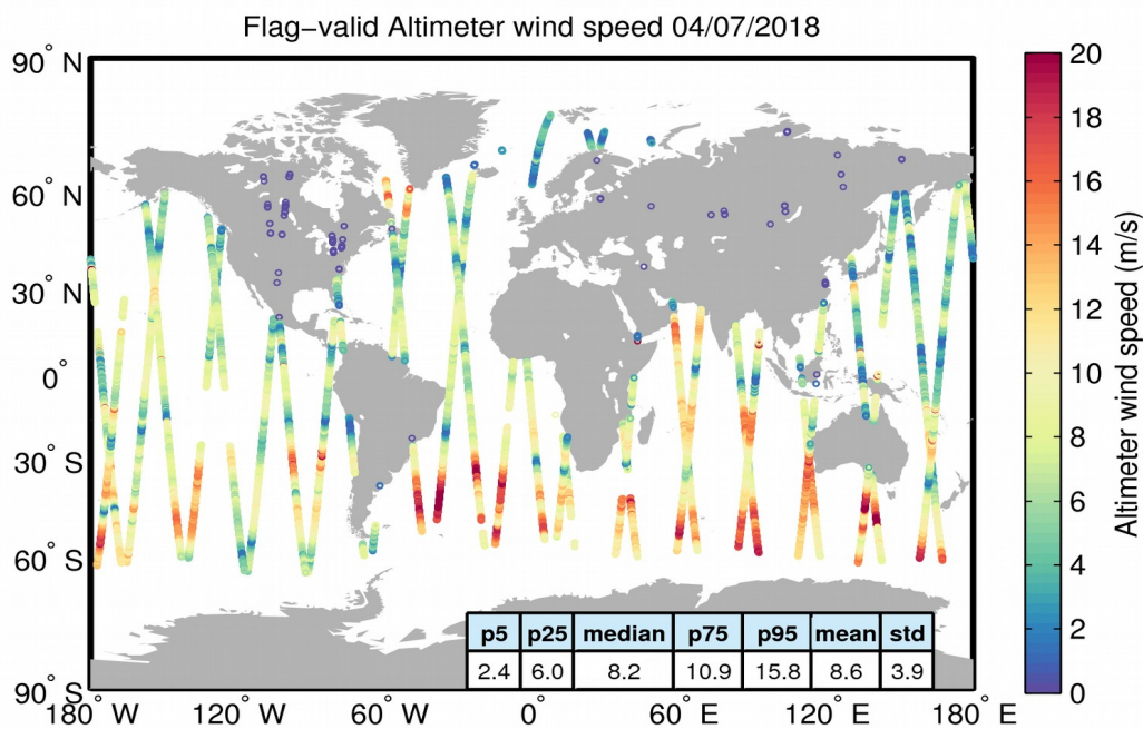
Figure 31. Geographical distribution of flag-valid wind data over oceans and lakes for 04/07/2018. The statistical values shown in the table refer to the wind in m/s and are calculated over all measurements shown in the figure.
