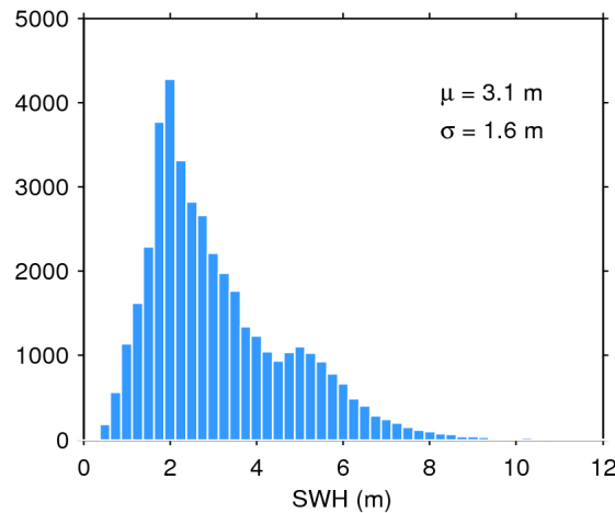
Figure 20. Histogram of science-valid SWH over oceans and lakes for 04/07/2018. The mean ( \mu ) and standard deviation ( \sigma ) are also shown. Note that values larger than 12 m are excluded from the histogram for the sake of readability but not from the computation of \mu and \sigma .
