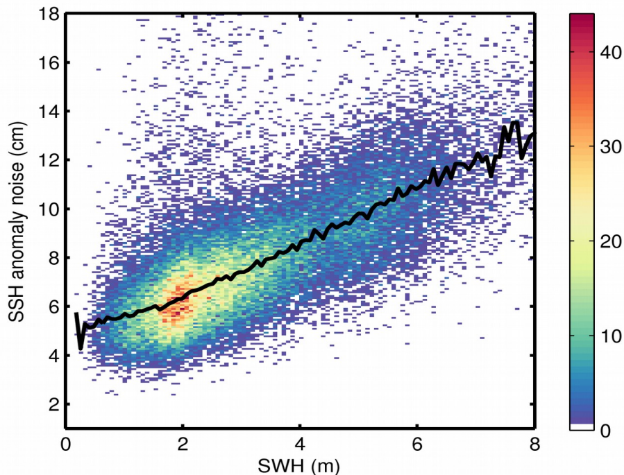
Figure 9. 2D histogram showing flag-valid SSH anomaly noise as a function of SWH for 04/07/2018. The black line denotes the median SSH anomaly noise as a function of SWH.
