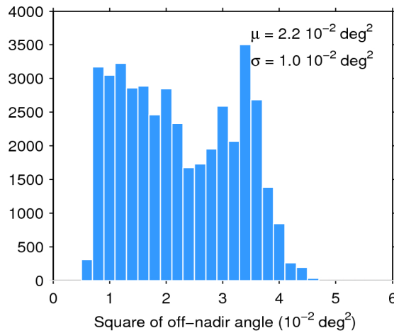
Figure 39. Histogram of flag-valid mispointing over oceans and lakes for 04/07/2018. The mean ( \mu ) and standard deviation ( \sigma ) are also shown. Note that values larger than 6 \cdot 10^{-2} \text{ deg}^2 are excluded from the histogram for the sake of readability but not from the computation of \mu and \sigma .
