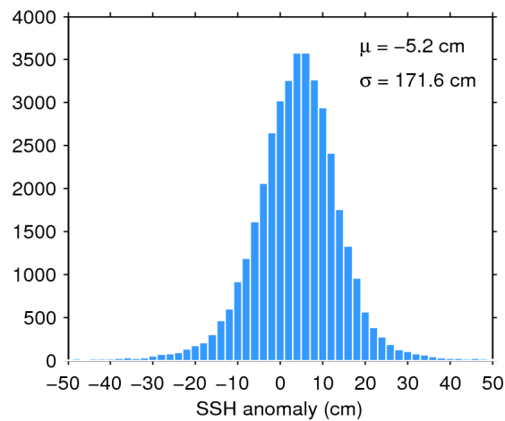
Figure 7. Histogram of flag-valid SSH anomaly over oceans and lakes for 04/07/2018. The mean ( \mu ) and standard deviation ( \sigma ) are also shown. Note that values outside [-50 50] cm are excluded from the histogram for the sake of readability but not from the computation of \mu and \sigma .
