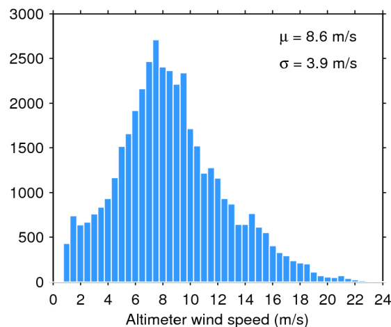
Figure 35. Histogram of science-valid wind over oceans and lakes for 04/07/2018. The mean ( \mu ) and standard deviation ( \sigma ) are also shown. Note that values larger than 24 m/s are excluded from the histogram for the sake of readability but not from the computation of \mu and \sigma .
