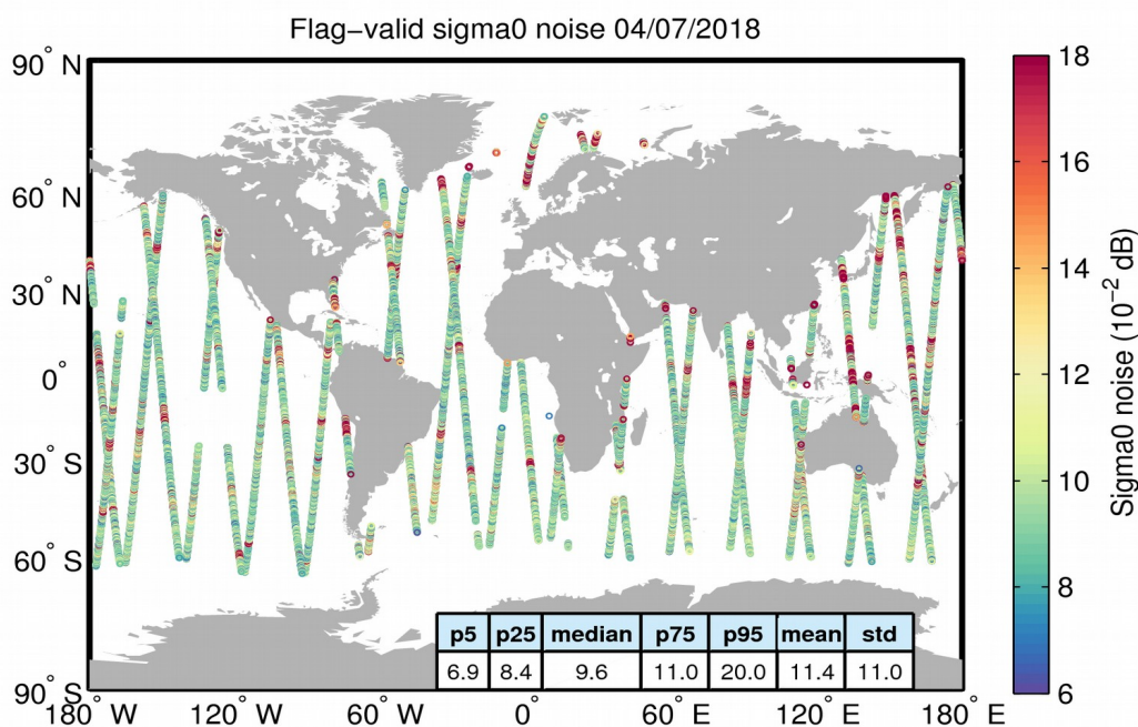
Figure 26. Geographical distribution of flag-valid 20-Hz sigma0 measurement noise over oceans and lakes for 04/07/2018. The statistical values shown in the table refer to the sigma0 noise and are calculated over all measurements shown in the figure.
