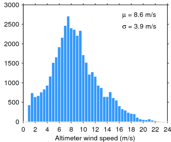
Figure 33. Histogram of flag-valid wind over oceans and lakes for 04/07/2018. The mean ( \mu ) and standard deviation ( \sigma ) are also shown. Note that values larger than 24 m/s are excluded from the histogram for the sake of readability but not from the computation of \mu and \sigma .
