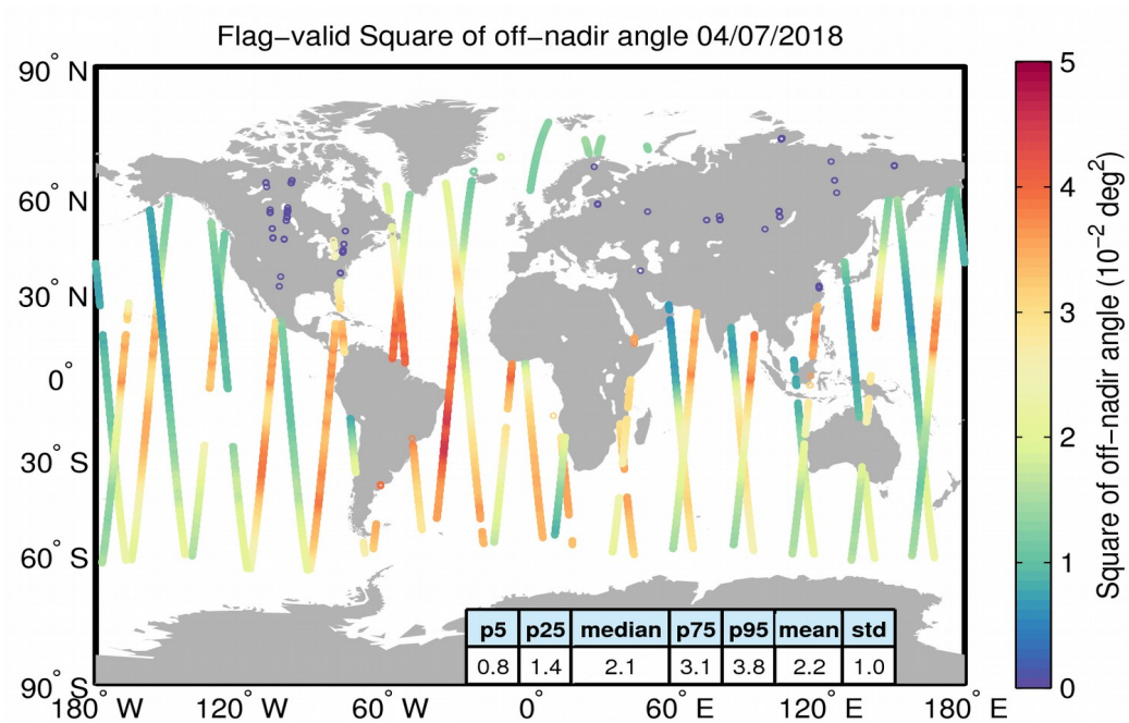
Figure 37. Geographical distribution of flag-valid mispointing data over oceans and lakes for 04/07/2018. The statistical values shown in the table refer to the mispointing in 10^{-2} \text{ deg}^2 and are calculated over all measurements shown in the figure.
