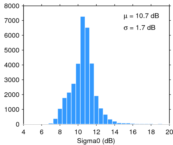
Figure 28. Histogram of science-valid sigma0 over oceans and lakes for 03/07/2018. The mean ( \mu ) and standard deviation ( \sigma ) are also shown. Note that values outside [4 20] dB are excluded from the histogram for the sake of readability but not from the computation of \mu and \sigma .
