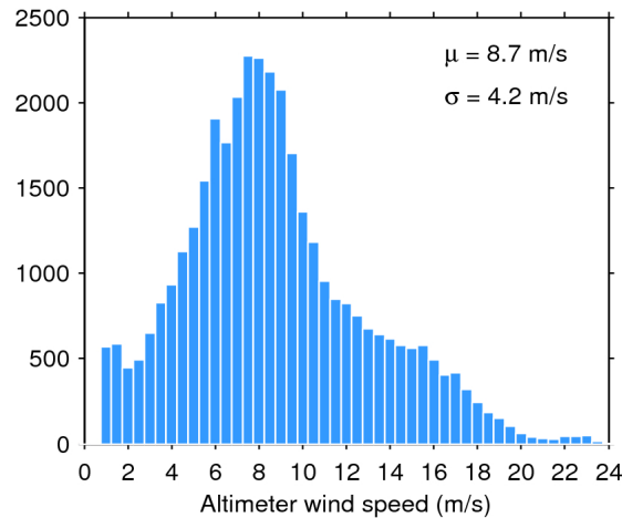
Figure 33. Histogram of flag-valid wind over oceans and lakes for 03/07/2018. The mean ( \mu ) and standard deviation ( \sigma ) are also shown. Note that values larger than 24 m/s are excluded from the histogram for the sake of readability but not from the computation of \mu and \sigma .
