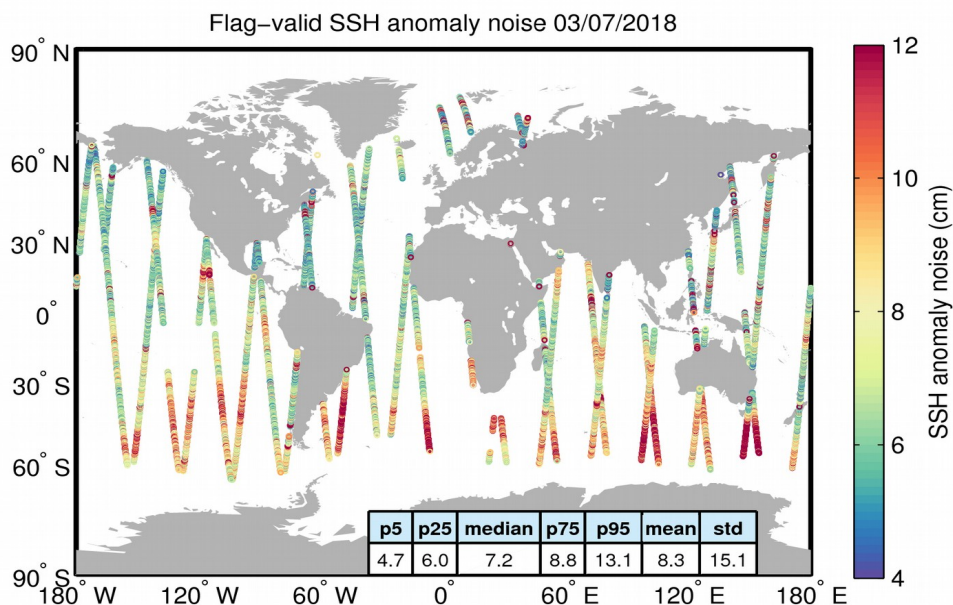
Figure 8. Geographical distribution of flag-valid 20-Hz SSH anomaly measurement noise over oceans and lakes for 03/07/2018. The statistical values shown in the table refer to the SSH anomaly noise and are calculated over all measurements shown in the figure.
