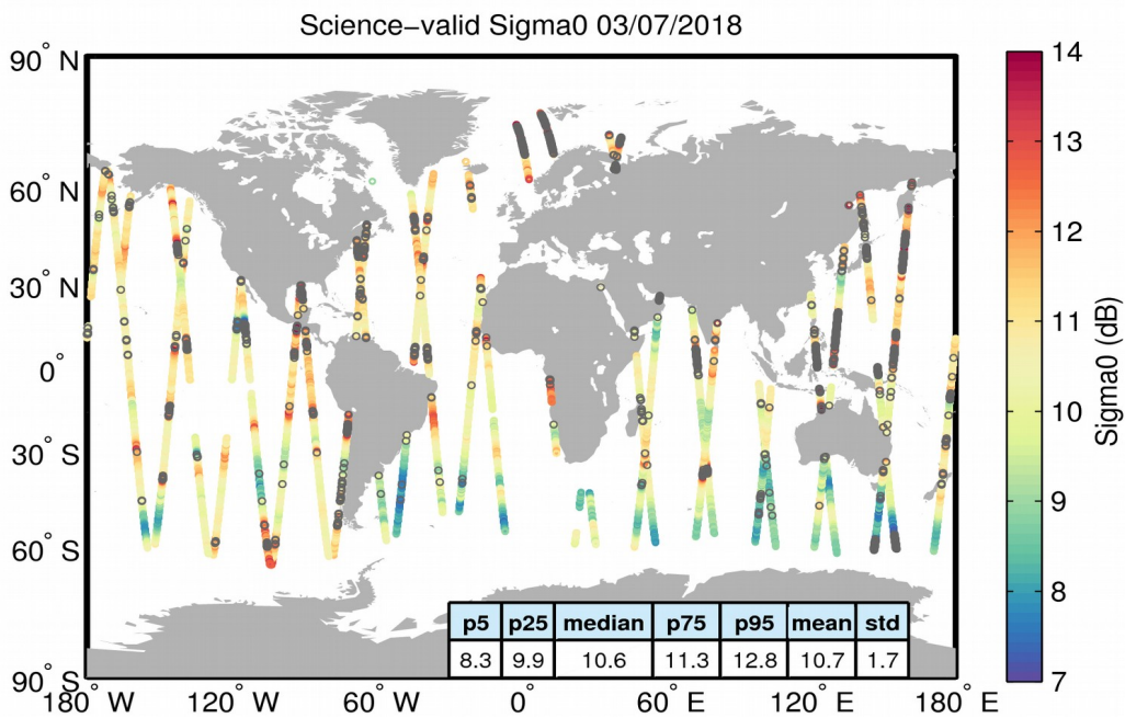
Figure 27. Geographical distribution of science-valid sigma0 data over oceans and lakes for 03/07/2018. The statistical values shown in the table refer to the sigma0 in dB and are calculated over all measurements shown in the figure. Gray circles denote records that have been rejected based on the editing criteria described in Table 4.
