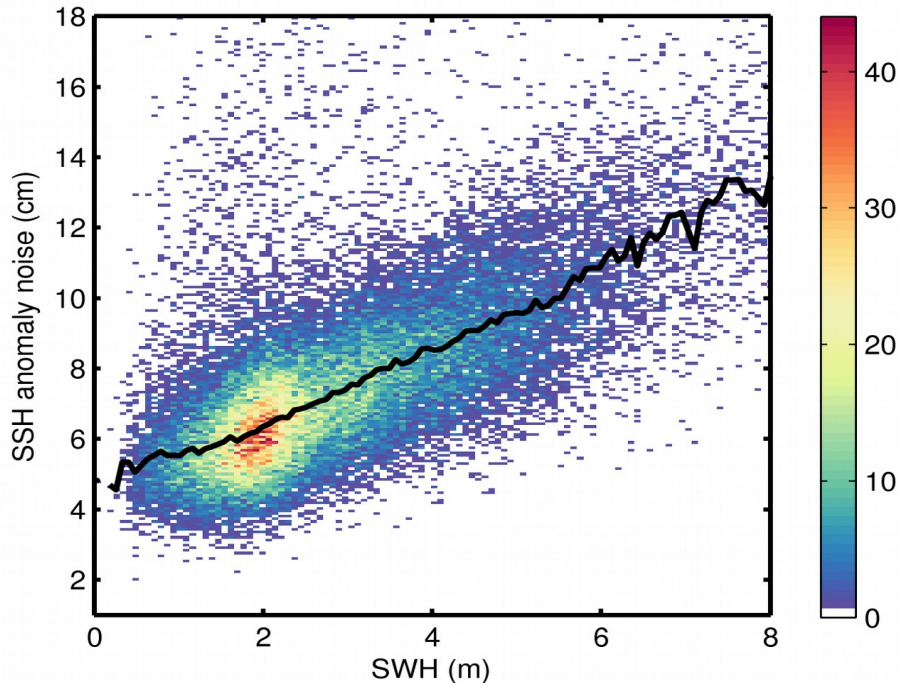
Figure 9. 2D histogram showing flag-valid SSH anomaly noise as a function of SWH for 03/07/2018. The black line denotes the median SSH anomaly noise as a function of SWH.
