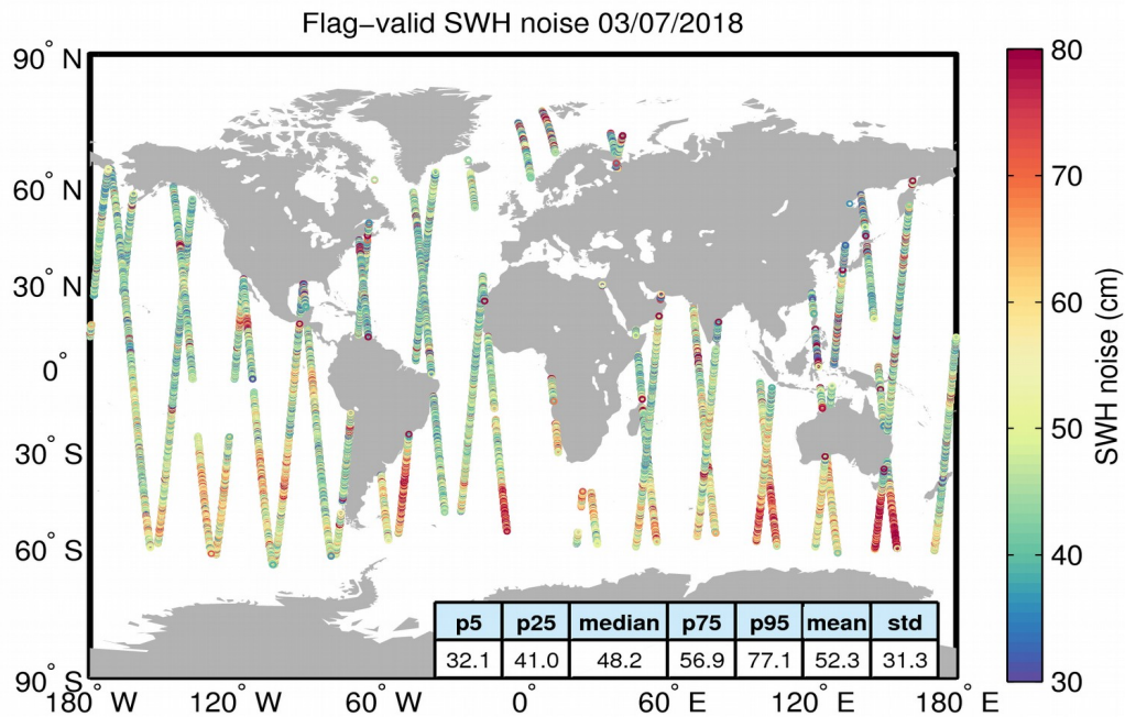
Figure 18. Geographical distribution of flag-valid 20-Hz SWH measurement noise over oceans and lakes for 03/07/2018. The statistical values shown in the figure refer to the SWH noise and are calculated over all measurements shown in the figure.
