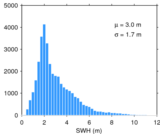
Figure 17. Histogram of flag-valid SWH over oceans and lakes for 03/07/2018. The mean ( \mu ) and standard deviation ( \sigma ) are also shown. Note that values larger than 12 m are excluded from the histogram for the sake of readability but not from the computation of \mu and \sigma .
