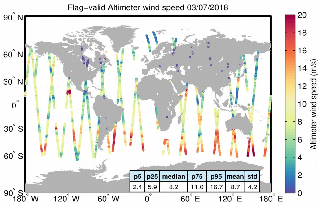
Figure 31. Geographical distribution of flag-valid wind data over oceans and lakes for 03/07/2018. The statistical values shown in the table refer to the wind in m/s and are calculated over all measurements shown in the figure.
