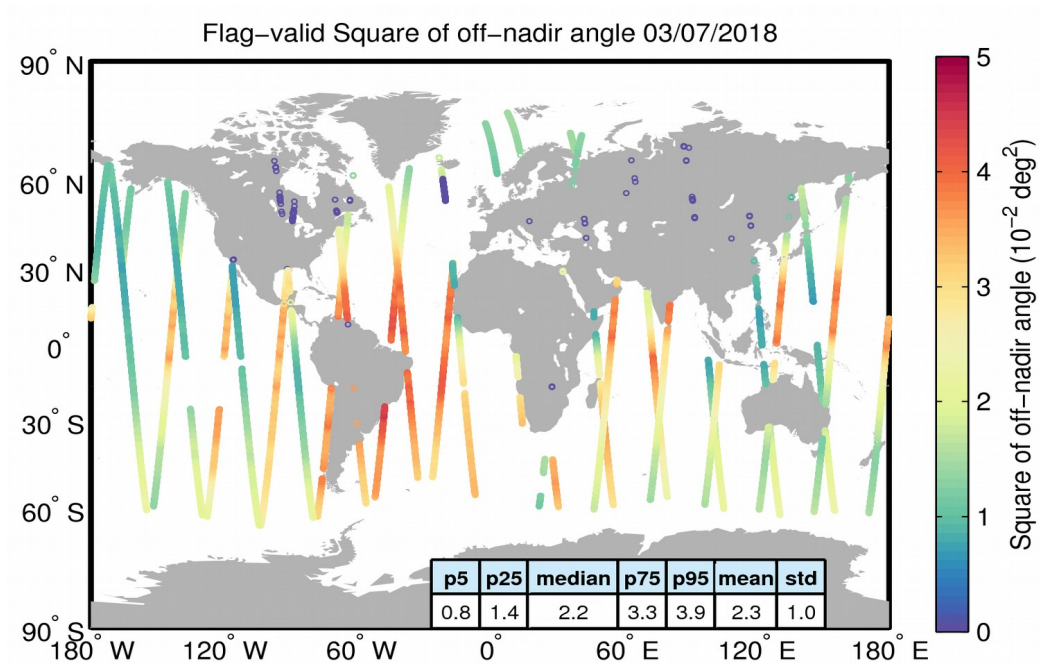
Figure 37. Geographical distribution of flag-valid mispointing data over oceans and lakes for 03/07/2018. The statistical values shown in the table refer to the mispointing in 10^{-2} \text{deg}^2 and are calculated over all measurements shown in the figure.
