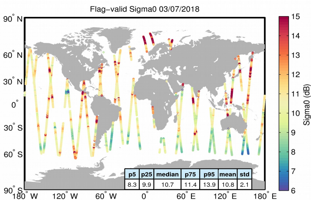
Figure 23. Geographical distribution of flag-valid sigma0 data over oceans and lakes for 03/07/2018. The statistical values shown in the table refer to the sigma0 in dB and are calculated over all measurements shown in the figure.
