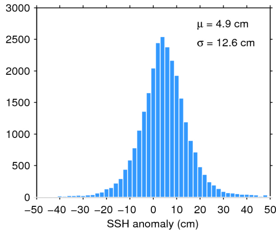
Figure 11. Histogram of science-valid SSH anomaly over oceans and lakes for 03/07/2018. The mean ( \mu ) and standard deviation ( \sigma ) are also shown. Note that values outside [-50 50] cm are excluded from the histogram for the sake of readability but not from the computation of \mu and \sigma .
