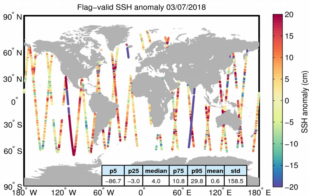
Figure 5. Geographical distribution of flag-valid 1-Hz SSH anomaly data over oceans and lakes for 03/07/2018. The statistical values shown in the table refer to the SSH anomaly in cm and are calculated over all measurements shown in the figure.
