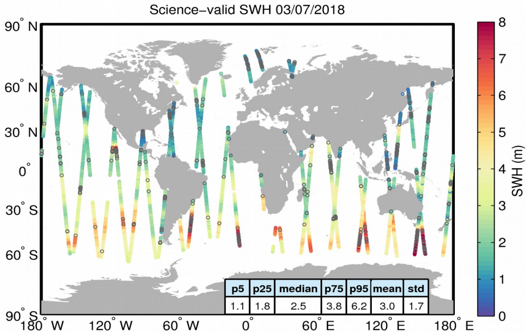
Figure 19. Geographical distribution of science-valid SWH data over oceans and lakes for 03/07/2018. The statistical values shown in the table refer to the SWH in m and are calculated over all measurements shown in the figure. Gray circles denote records that have been rejected based on the editing criteria described in Table 3.
