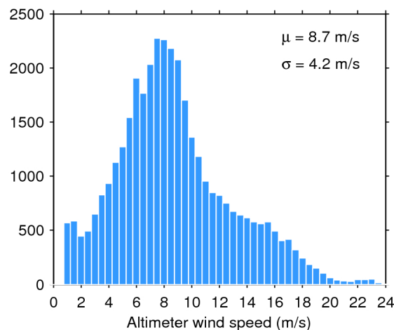
Figure 35. Histogram of science-valid wind over oceans and lakes for 03/07/2018. The mean ( \mu ) and standard deviation ( \sigma ) are also shown. Note that values larger than 24 m/s are excluded from the histogram for the sake of readability but not from the computation of \mu and \sigma .
