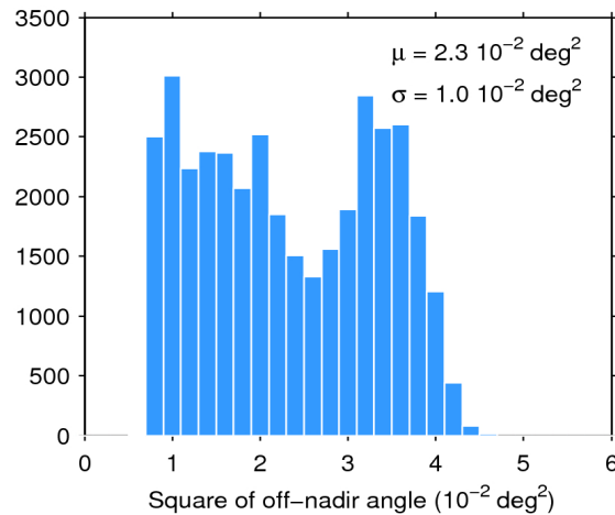
Figure 39. Histogram of flag-valid mispointing over oceans and lakes for 03/07/2018. The mean ( \mu ) and standard deviation ( \sigma ) are also shown. Note that values larger than 6 \cdot 10^{-2} \text{ deg}^2 are excluded from the histogram for the sake of readability but not from the computation of \mu and \sigma .
