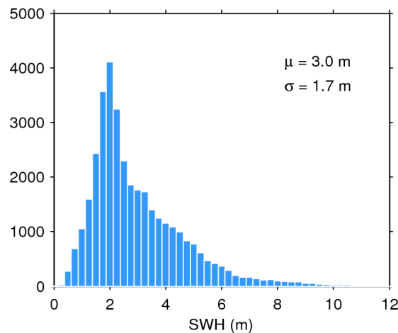
Figure 20. Histogram of science-valid SWH over oceans and lakes for 03/07/2018. The mean ( \mu ) and standard deviation ( \sigma ) are also shown. Note that values larger than 12 m are excluded from the histogram for the sake of readability but not from the computation of \mu and \sigma .
