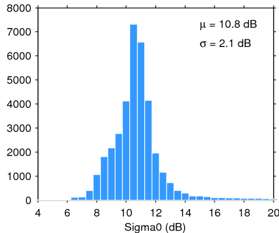
Figure 25. Histogram of flag-valid sigma0 over oceans and lakes for 03/07/2018. The mean ( \mu ) and standard deviation ( \sigma ) are also shown. Note that values outside [4 20] dB are excluded from the histogram for the sake of readability but not from the computation of \mu and \sigma .
