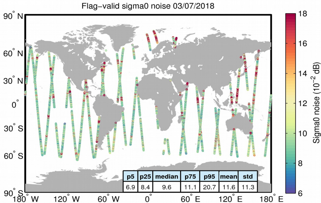
Figure 26. Geographical distribution of flag-valid 20-Hz sigma0 measurement noise over oceans and lakes for 03/07/2018. The statistical values shown in the table refer to the sigma0 noise and are calculated over all measurements shown in the figure.
